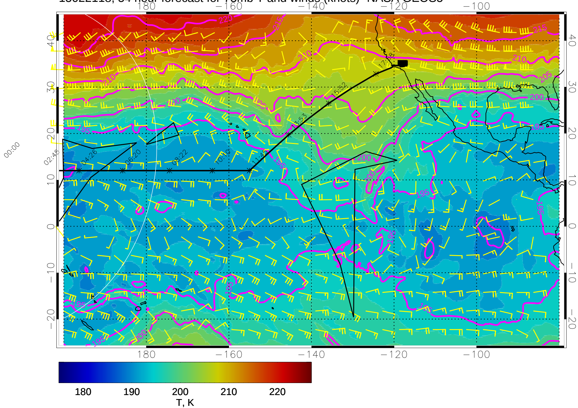
15022118, 54 hour forecast for 73mb T and winds (knots)- NASA GEOS5
