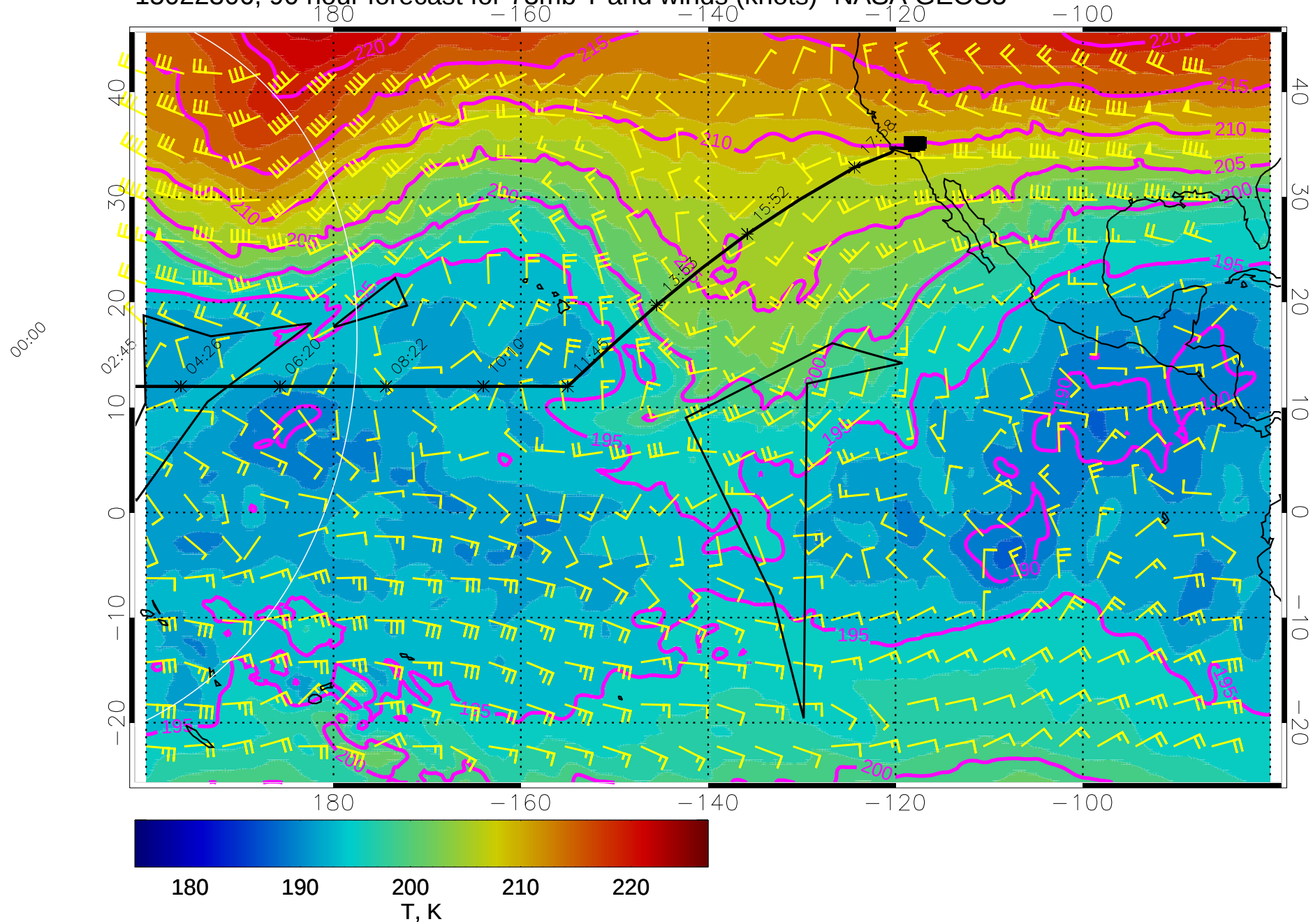
15022306, 90 hour forecast for 73mb T and winds (knots)- NASA GEOS5
