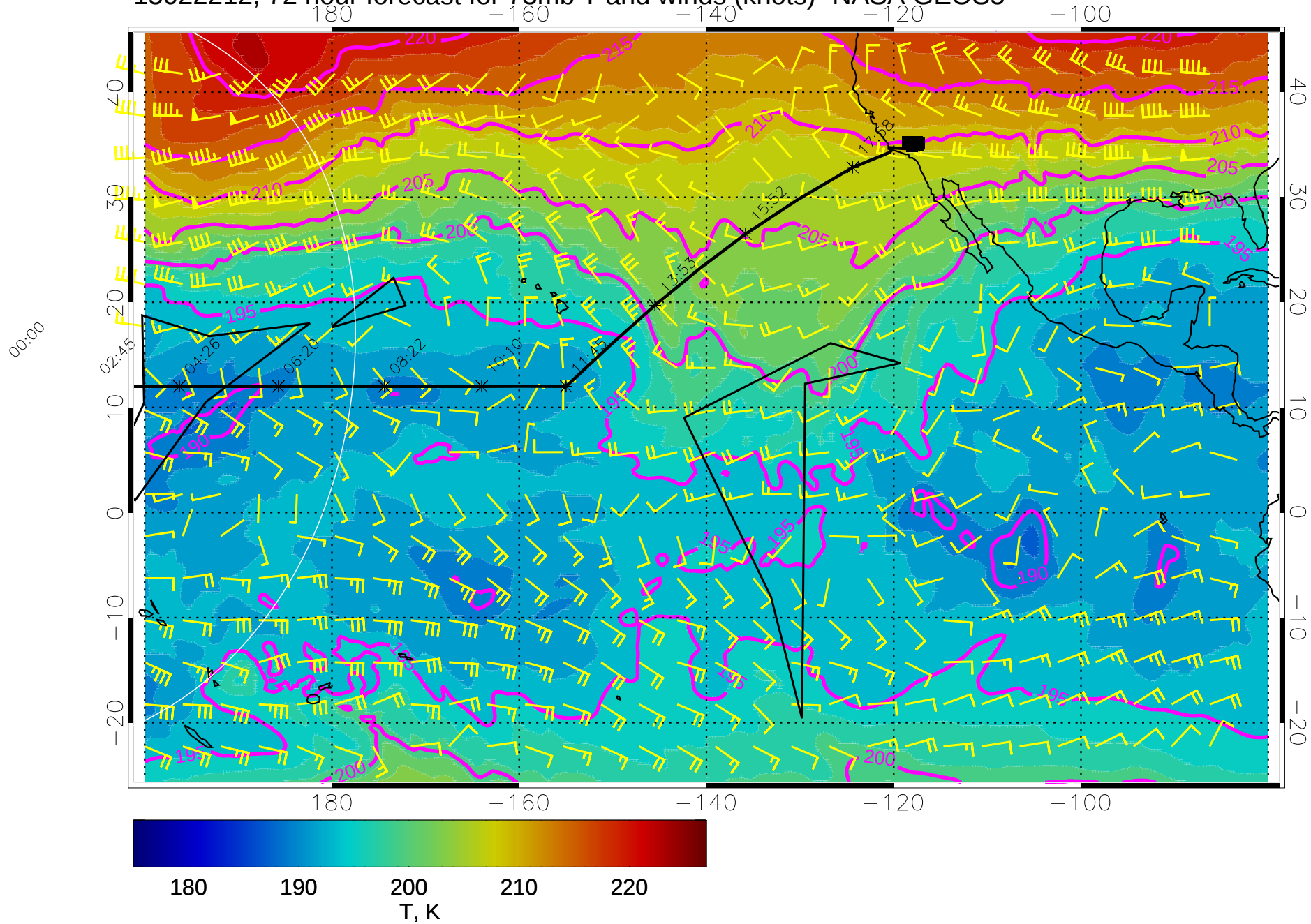
15022212, 72 hour forecast for 73mb T and winds (knots)- NASA GEOS5
