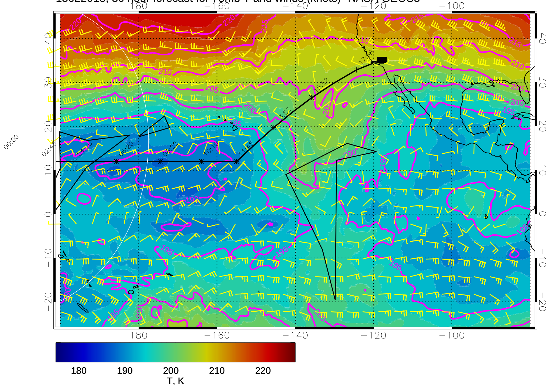
15022018, 30 hour forecast for 73mb T and winds (knots)- NASA GEOS5
