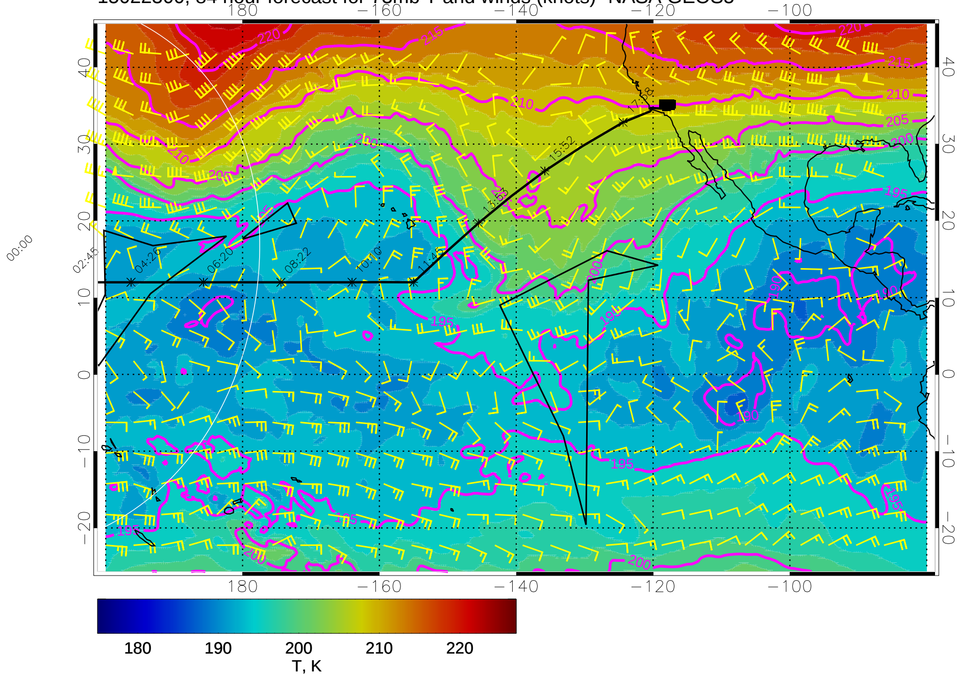
15022300, 84 hour forecast for 73mb T and winds (knots)- NASA GEOS5
