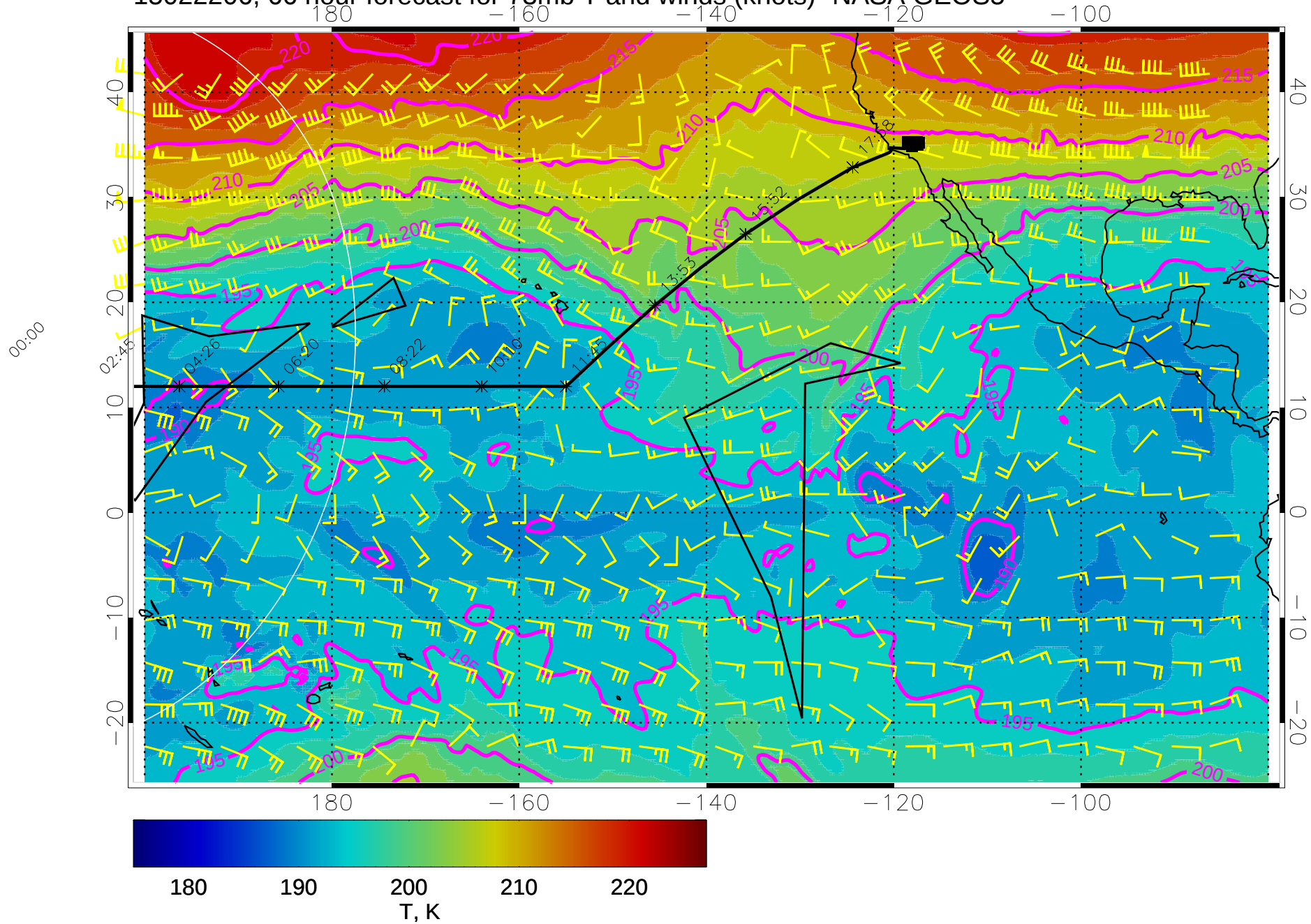
15022206, 66 hour forecast for 73mb T and winds (knots)- NASA GEOS5
