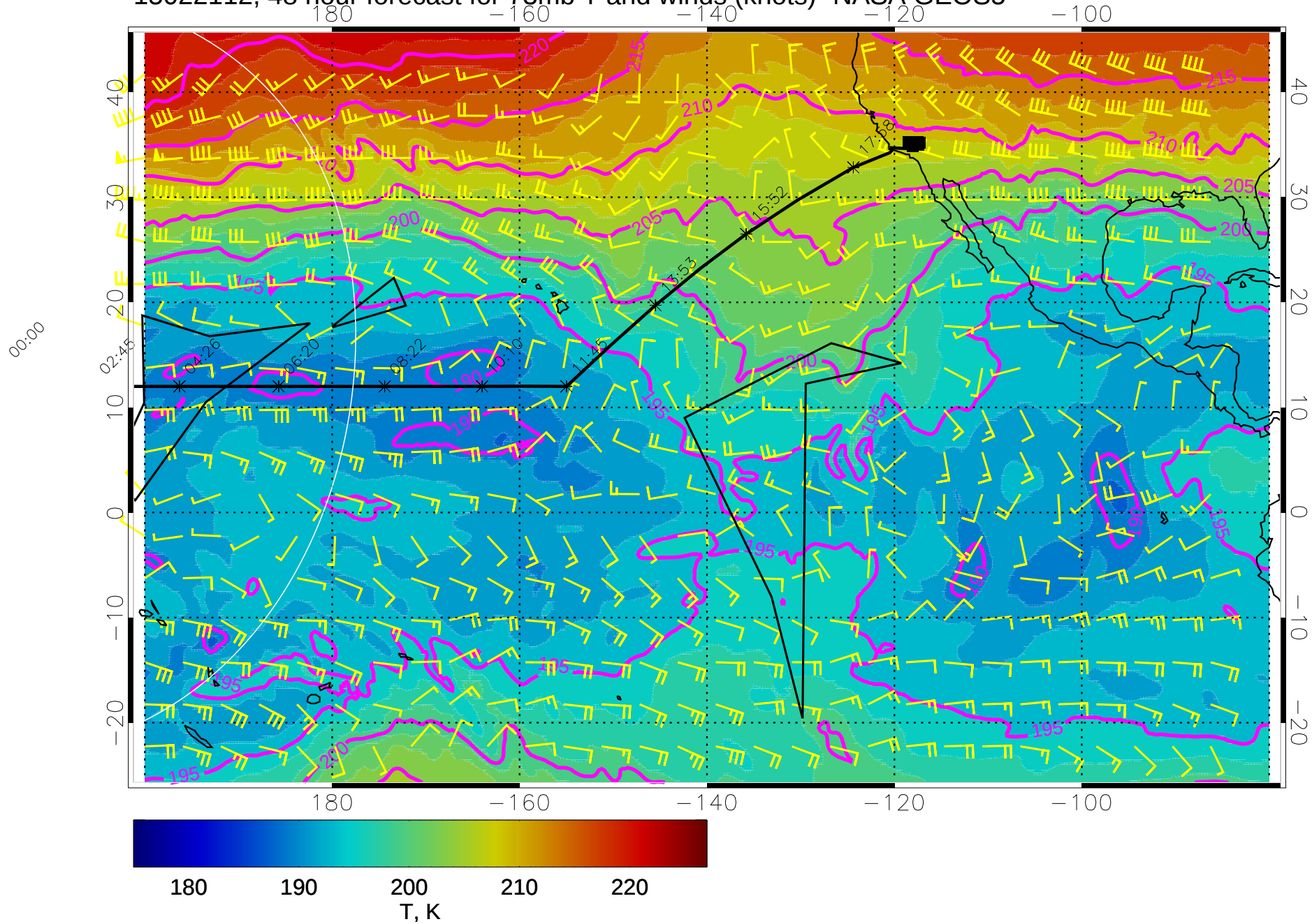
15022112, 48 hour forecast for 73mb T and winds (knots)- NASA GEOS5
