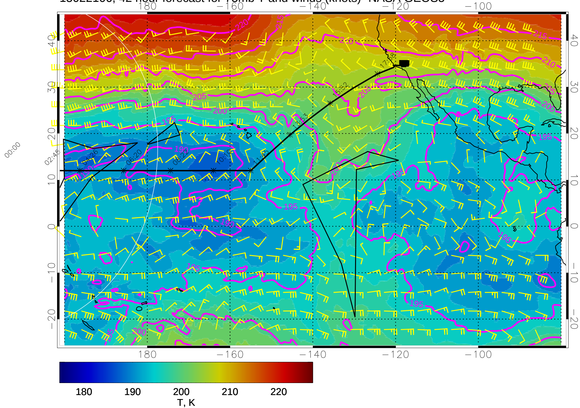
15022106, 42 hour forecast for 73mb T and winds (knots)- NASA GEOS5
