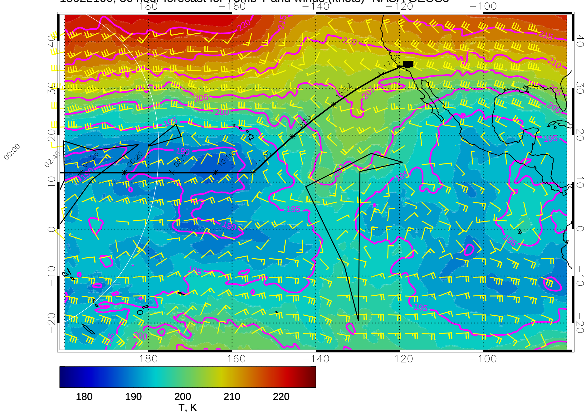
15022100, 36 hour forecast for 73mb T and winds (knots)- NASA GEOS5
