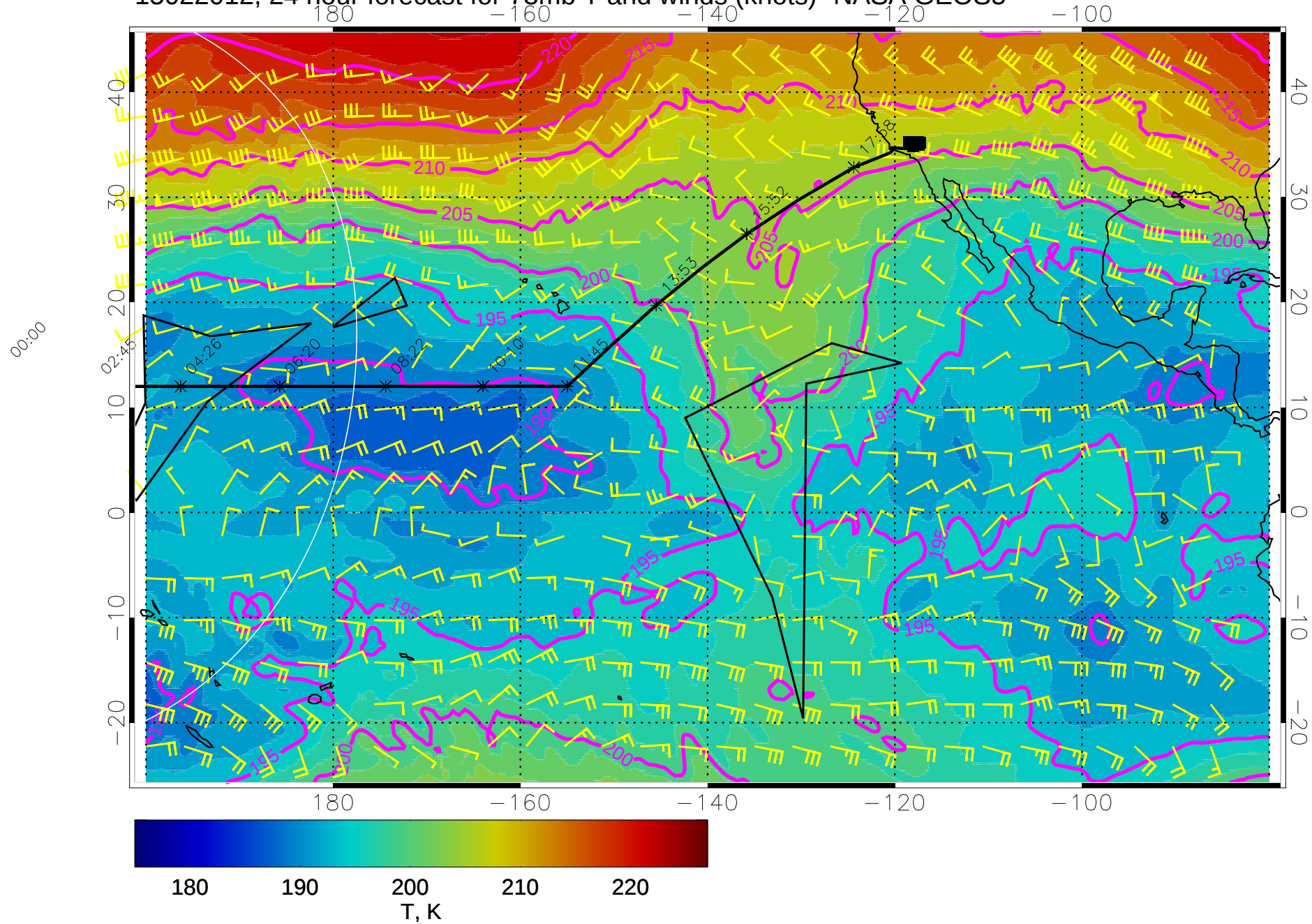
15022012, 24 hour forecast for 73mb T and winds (knots)- NASA GEOS5
