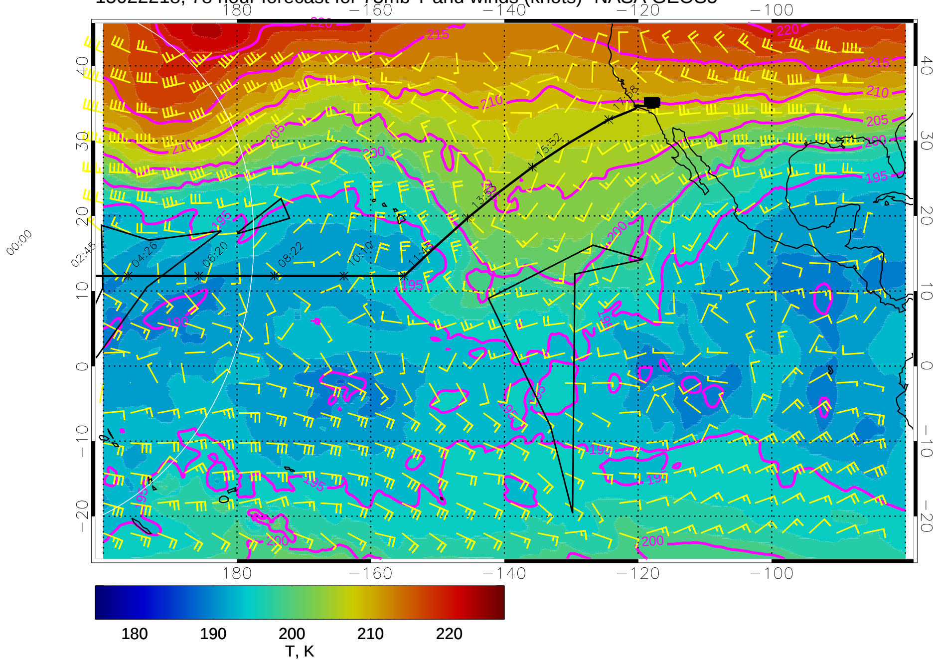
15022218, 78 hour forecast for 73mb T and winds (knots)- NASA GEOS5
