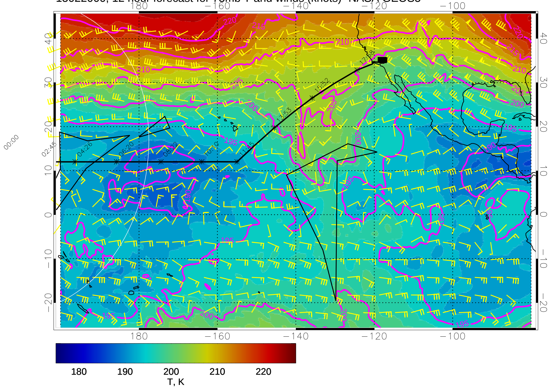
15022000, 12 hour forecast for 73mb T and winds (knots)- NASA GEOS5
