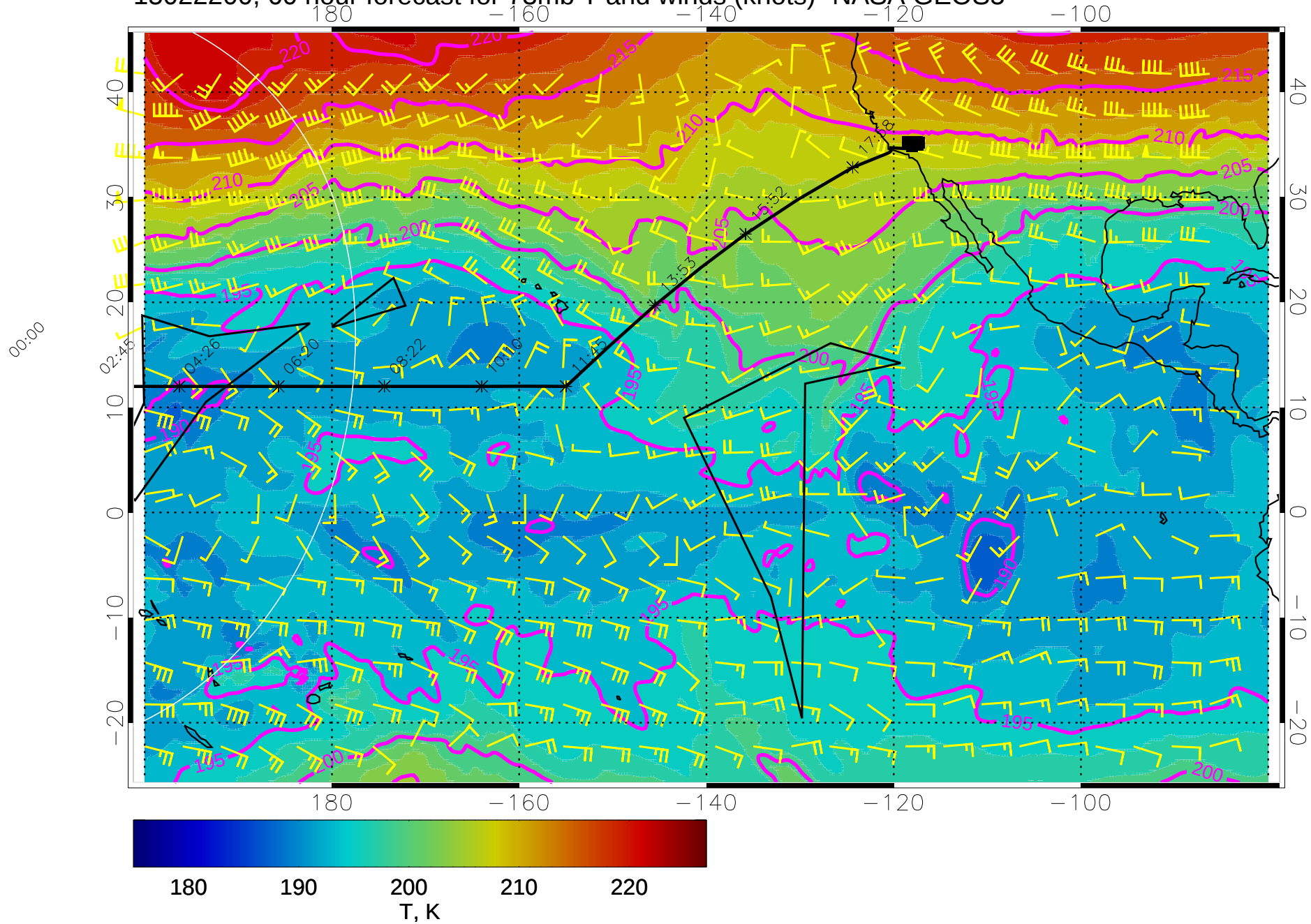
15022200, 60 hour forecast for 73mb T and winds (knots)- NASA GEOS5
