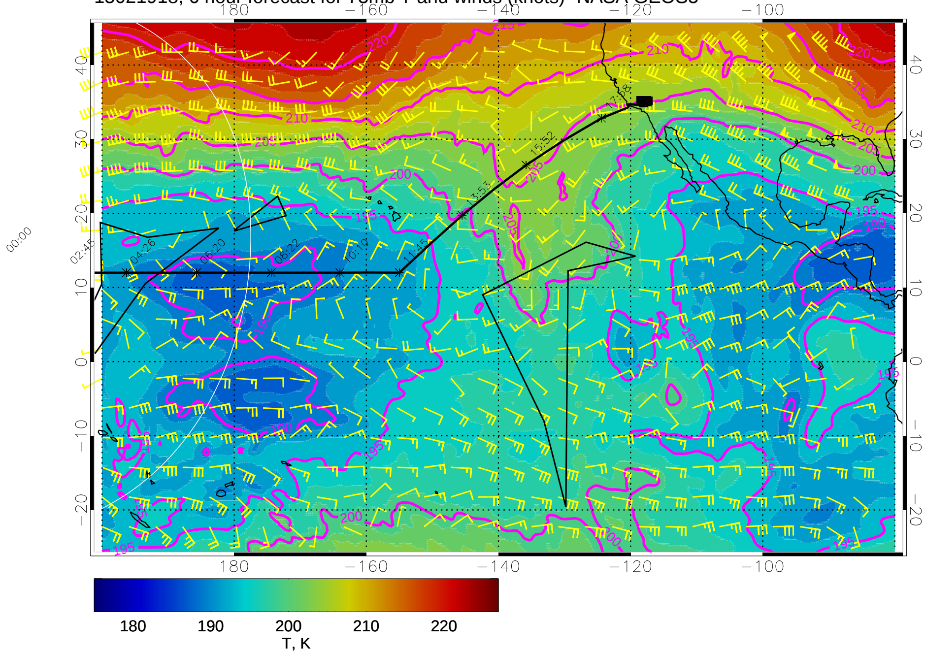
15021918, 6 hour forecast for 73mb T and winds (knots)- NASA GEOS5
