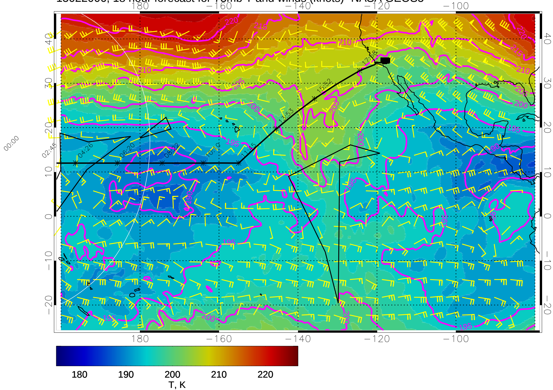
15022006, 18 hour forecast for 73mb T and winds (knots)- NASA GEOS5
