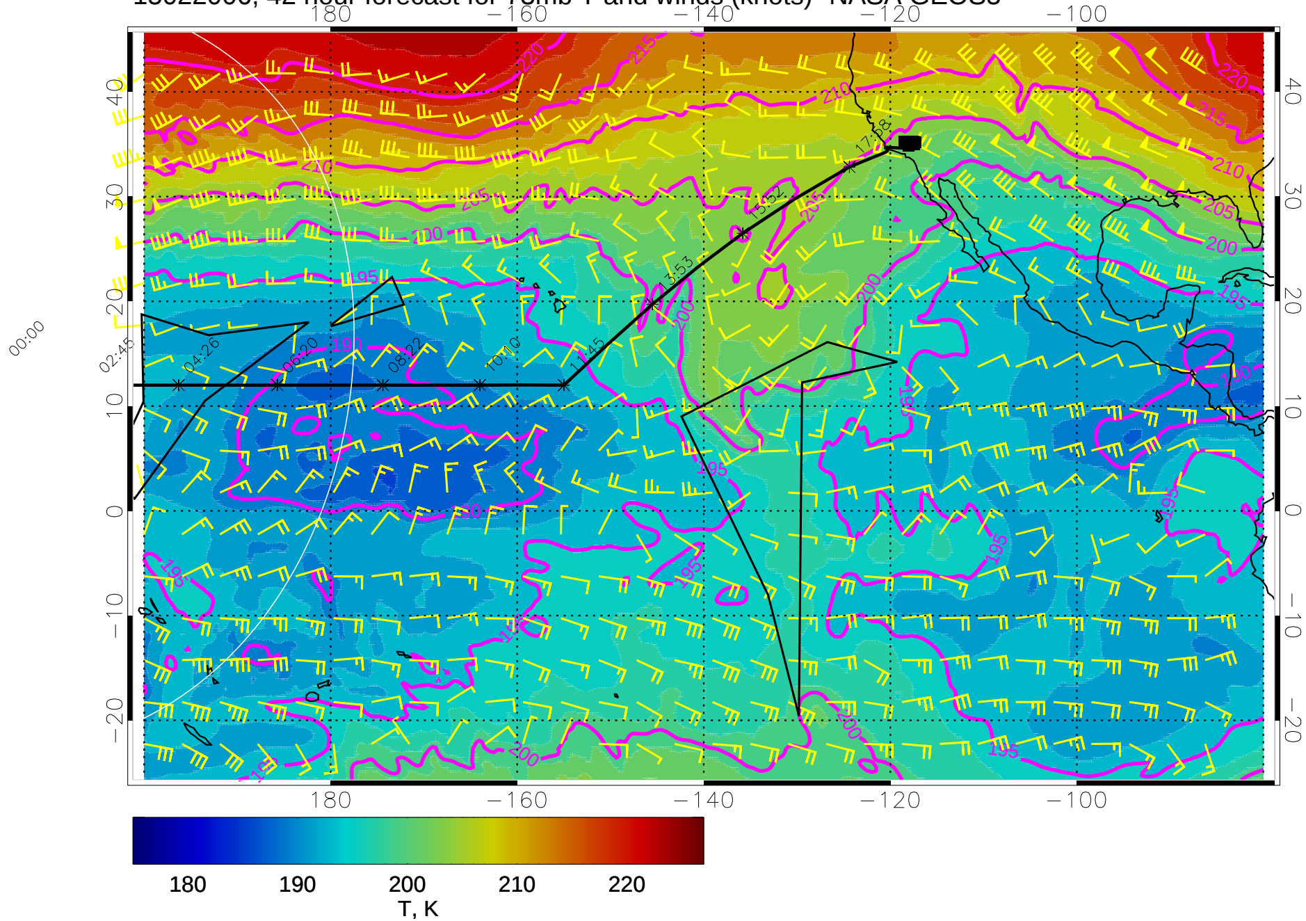
15022006, 42 hour forecast for 73mb T and winds (knots)- NASA GEOS5
