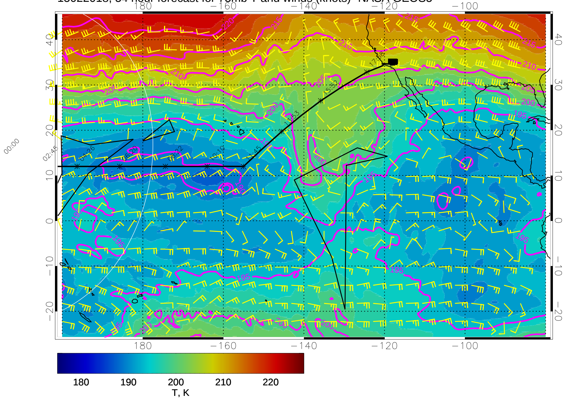
15022018, 54 hour forecast for 73mb T and winds (knots)- NASA GEOS5
