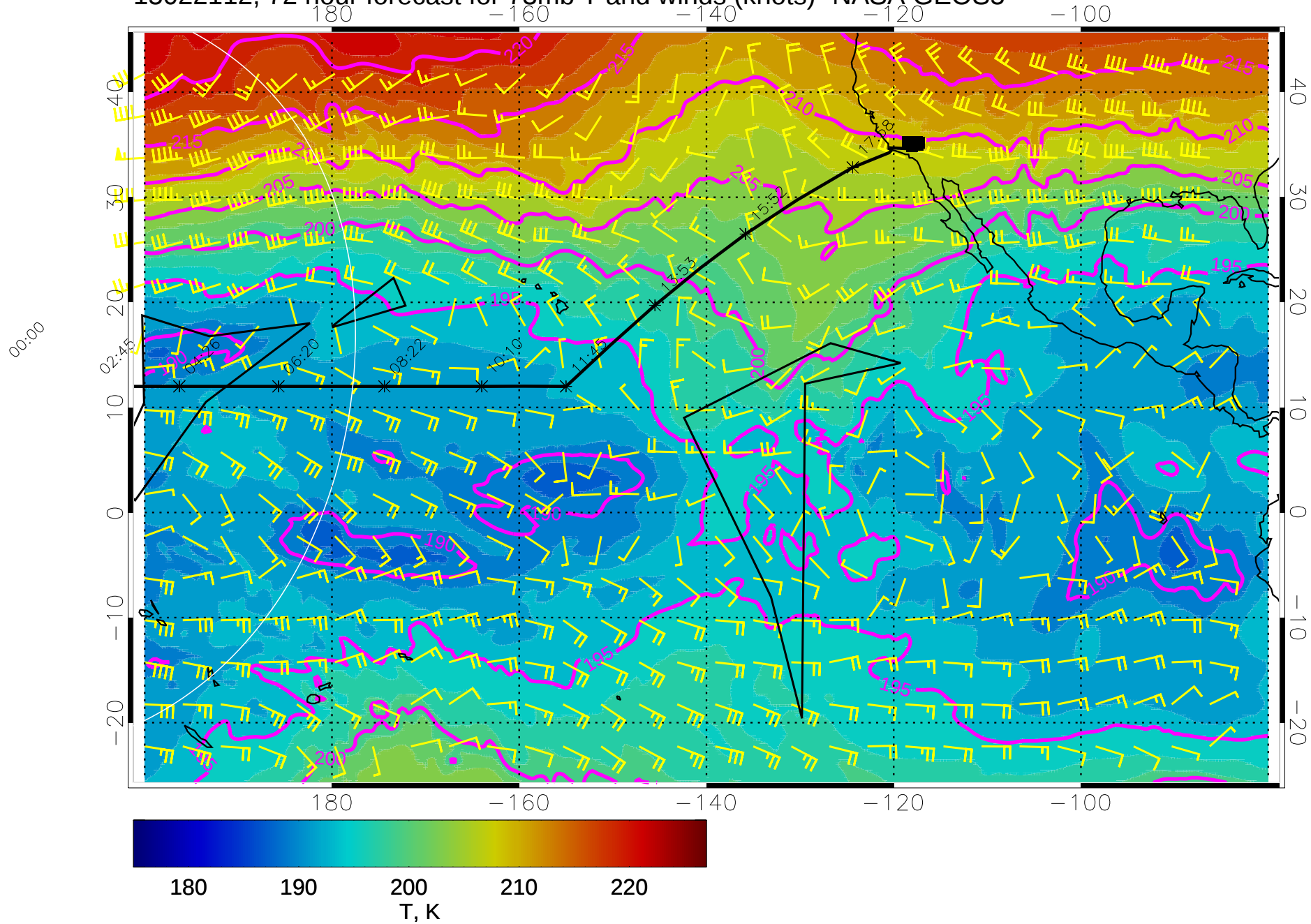
15022112, 72 hour forecast for 73mb T and winds (knots)- NASA GEOS5
