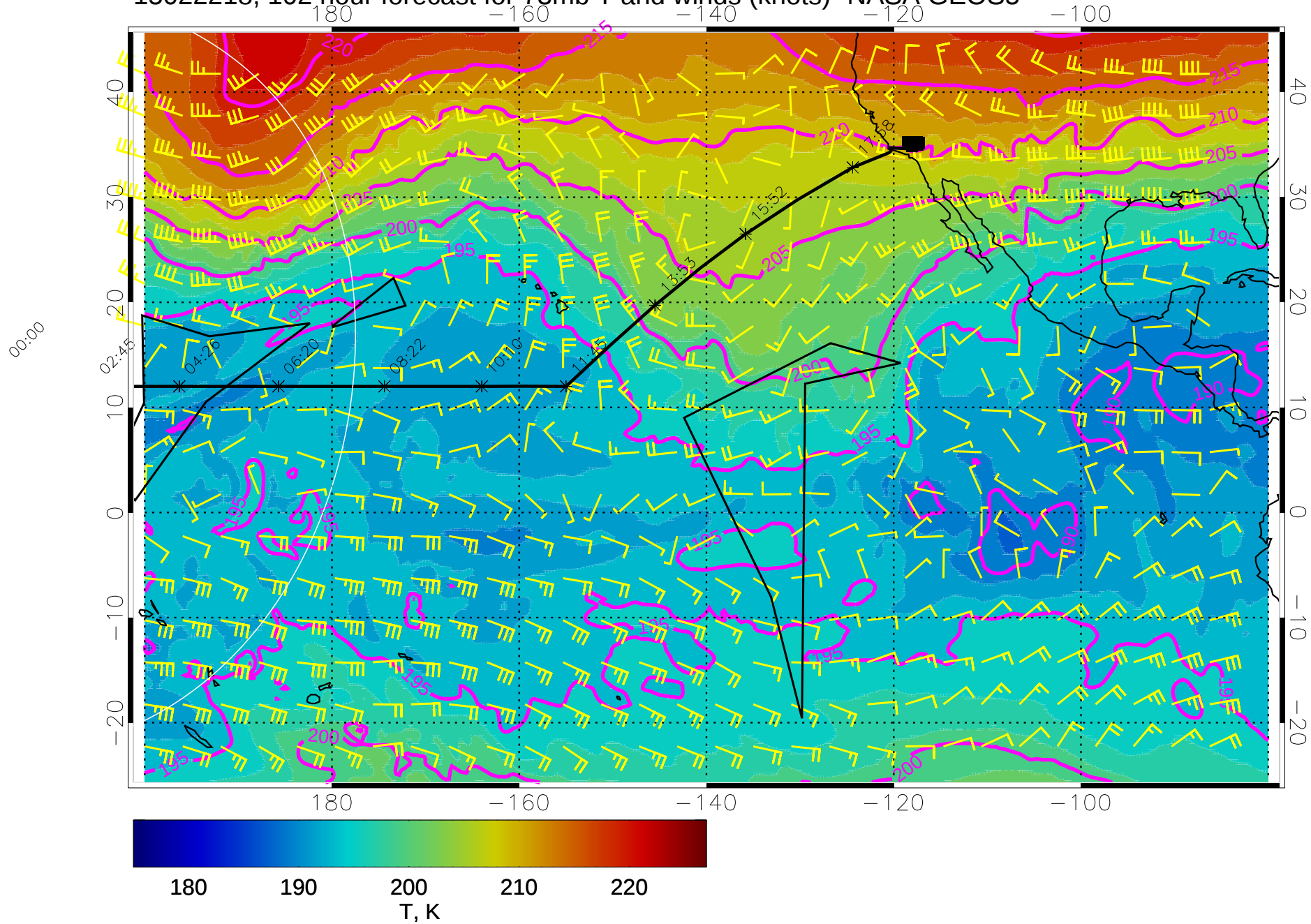
15022218, 102 hour forecast for 73mb T and winds (knots)- NASA GEOS5
