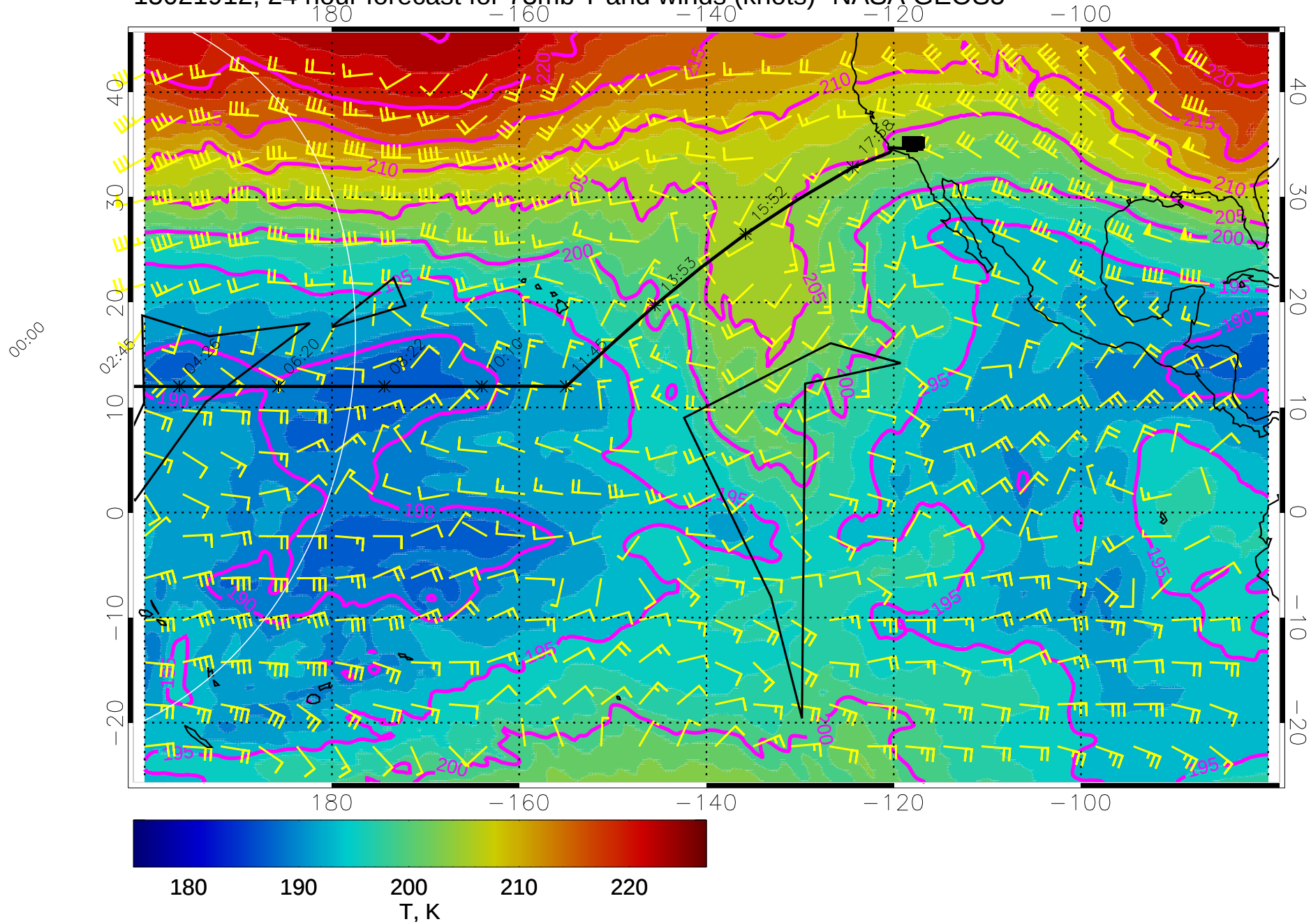
15021912, 24 hour forecast for 73mb T and winds (knots)- NASA GEOS5
