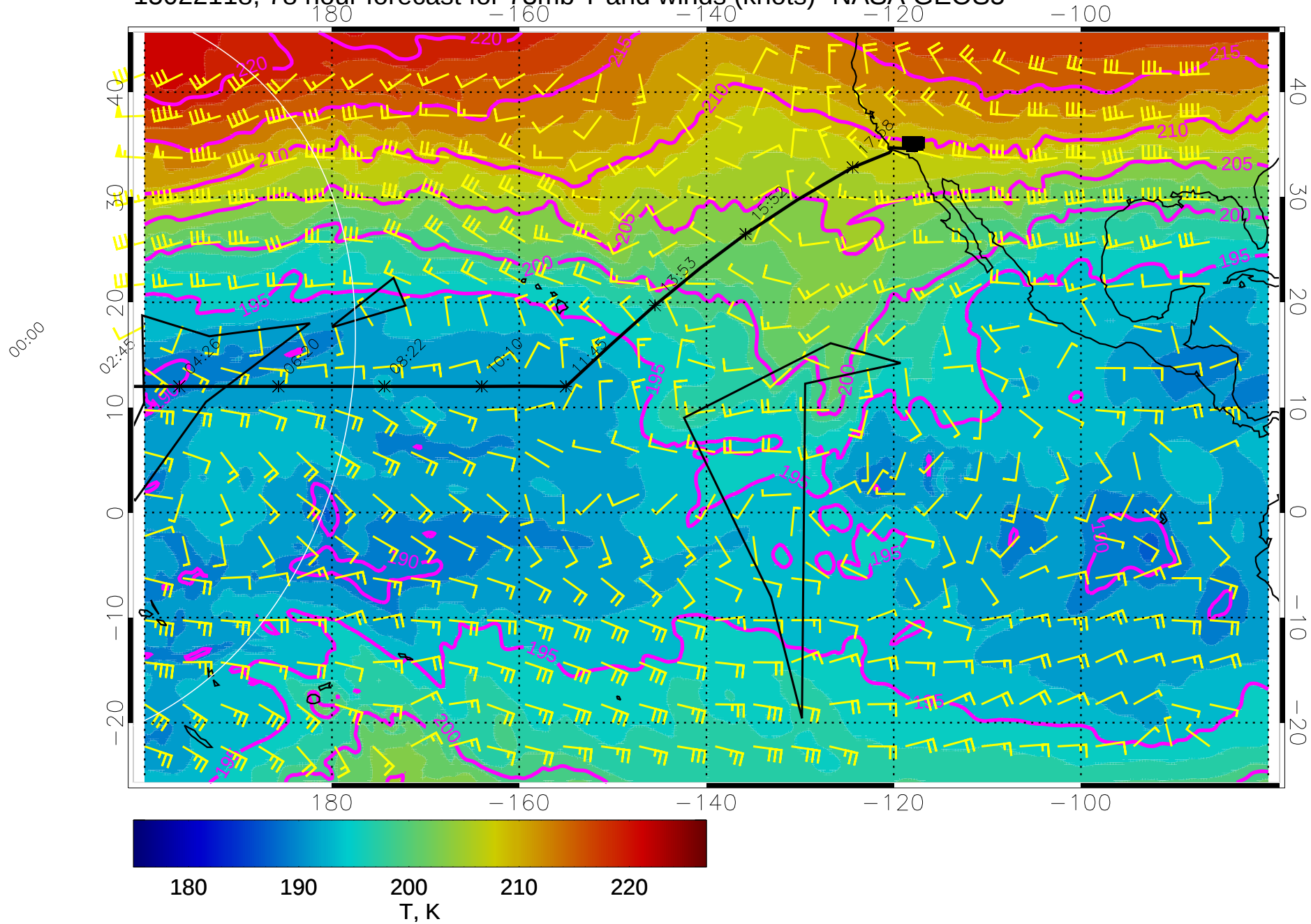
15022118, 78 hour forecast for 73mb T and winds (knots)- NASA GEOS5
