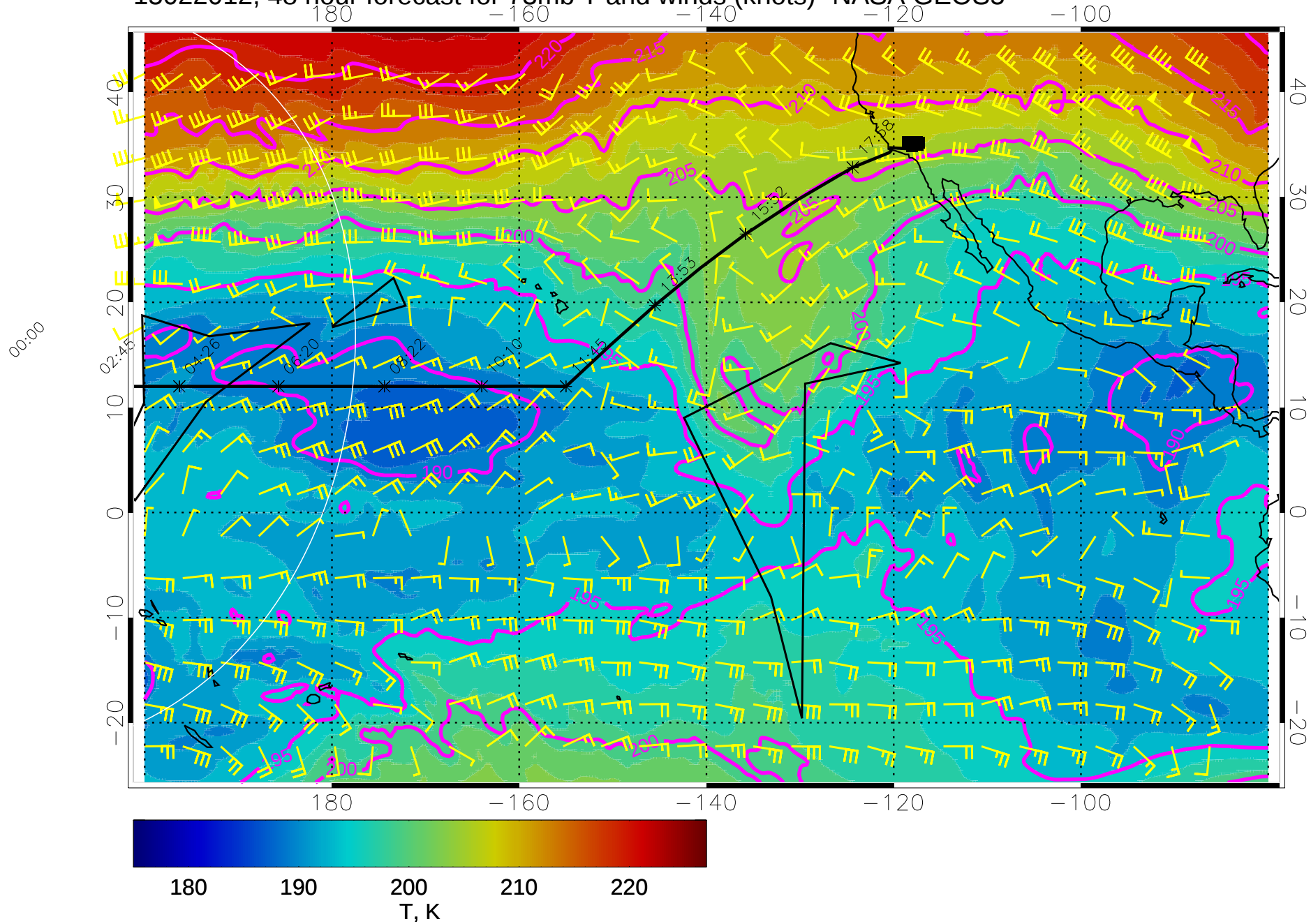
15022012, 48 hour forecast for 73mb T and winds (knots)- NASA GEOS5
