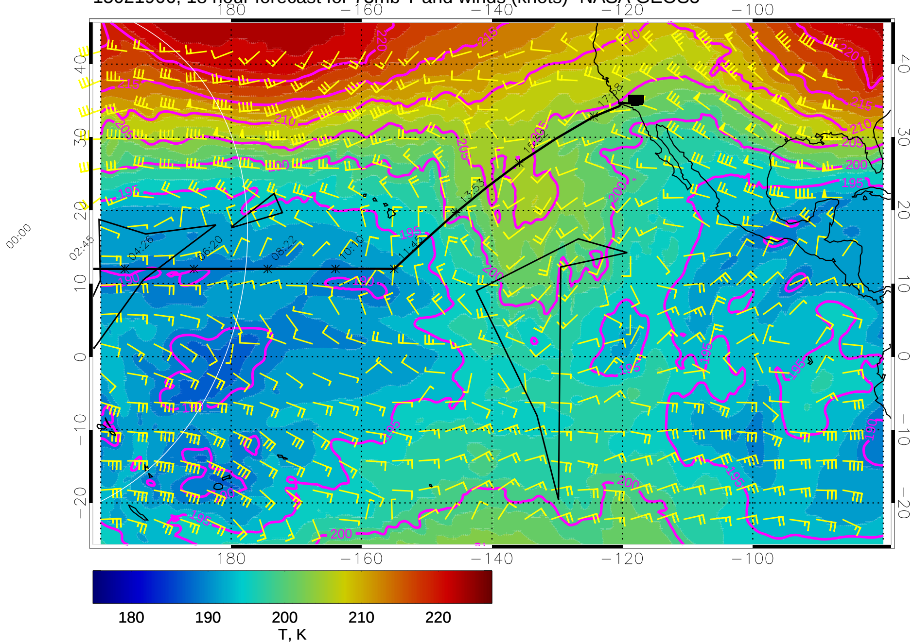
15021906, 18 hour forecast for 73mb T and winds (knots)- NASA GEOS5
