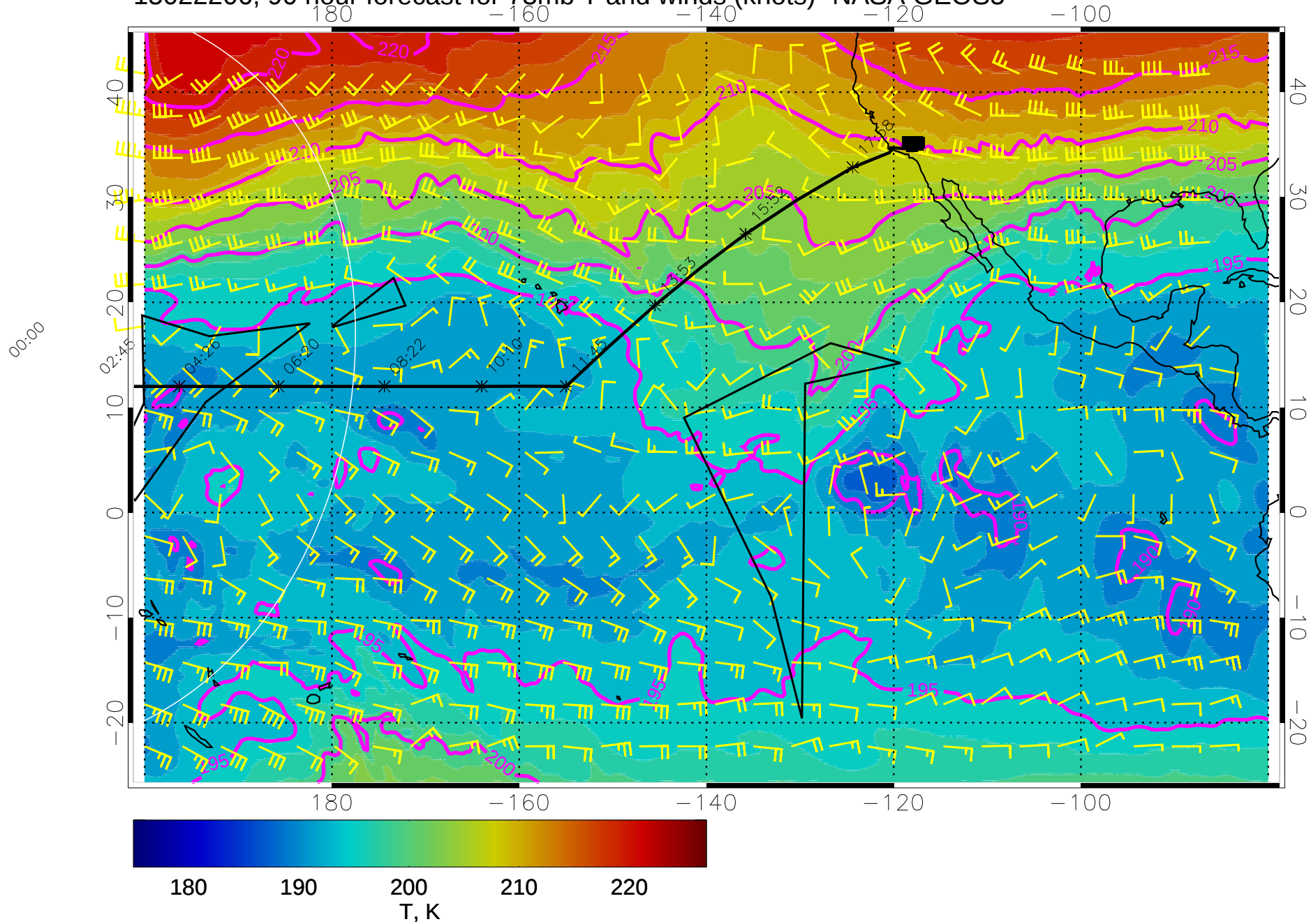
15022206, 90 hour forecast for 73mb T and winds (knots)- NASA GEOS5
