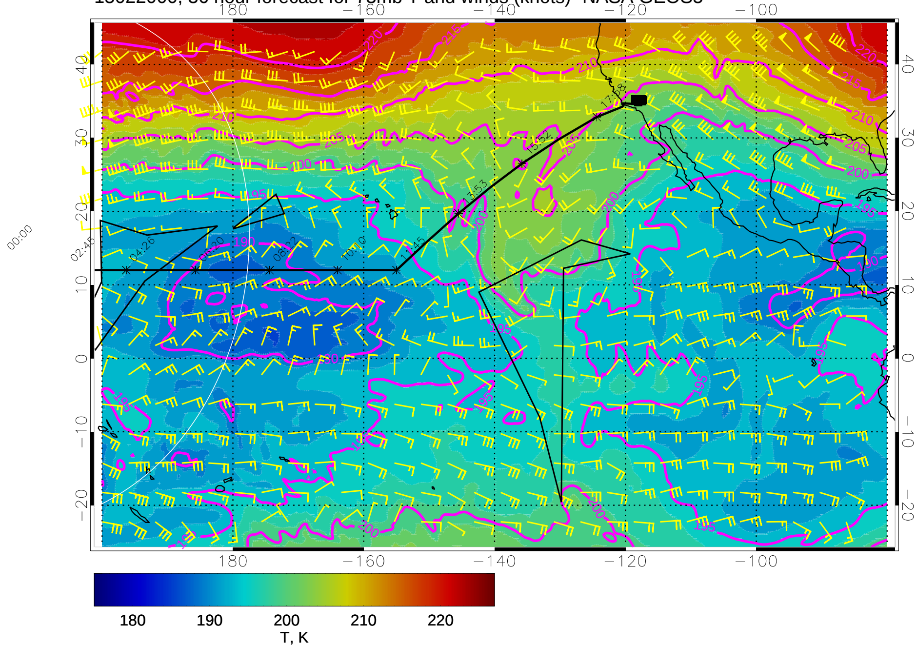
15022000, 36 hour forecast for 73mb T and winds (knots)- NASA GEOS5
