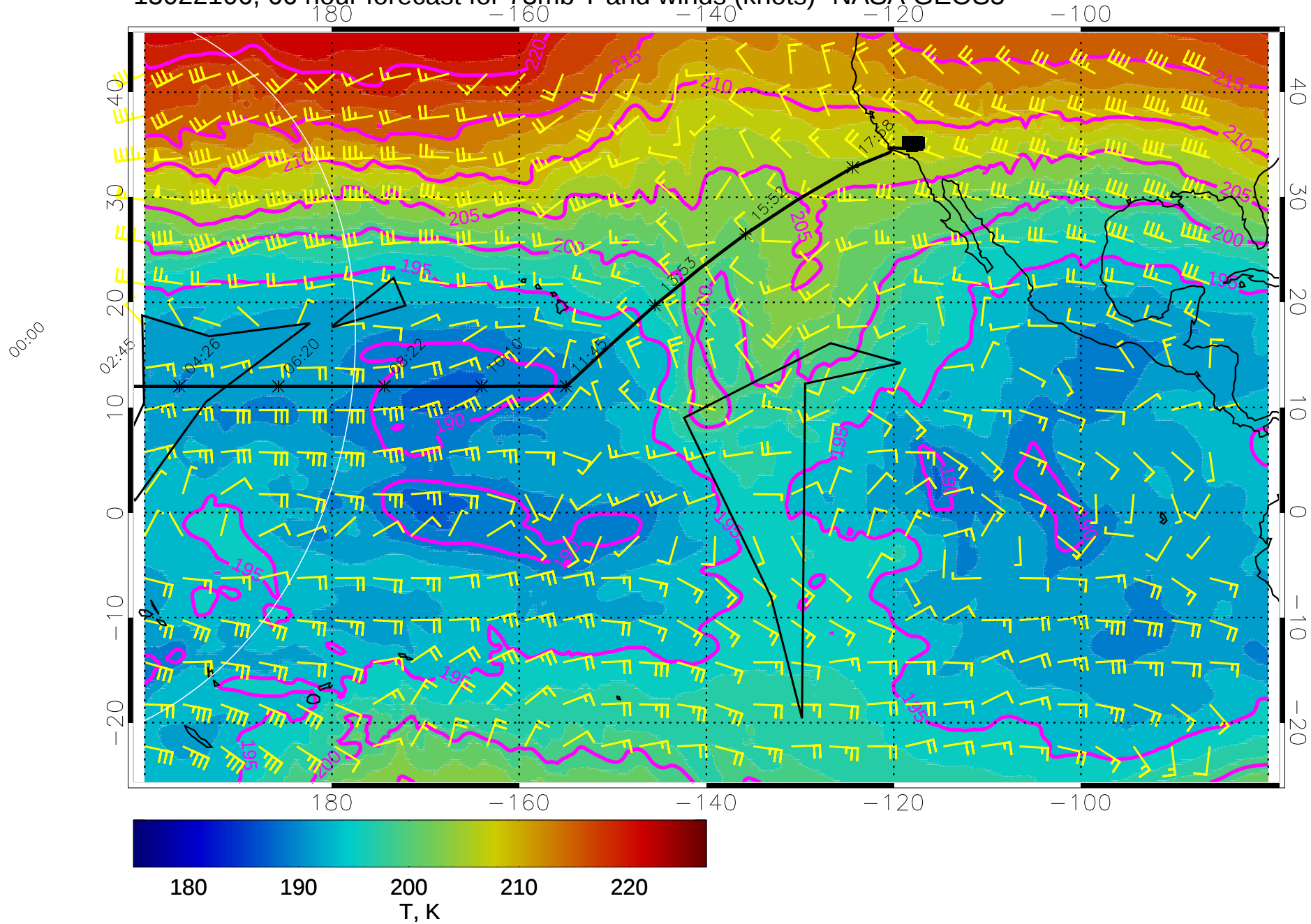
15022106, 66 hour forecast for 73mb T and winds (knots)- NASA GEOS5
