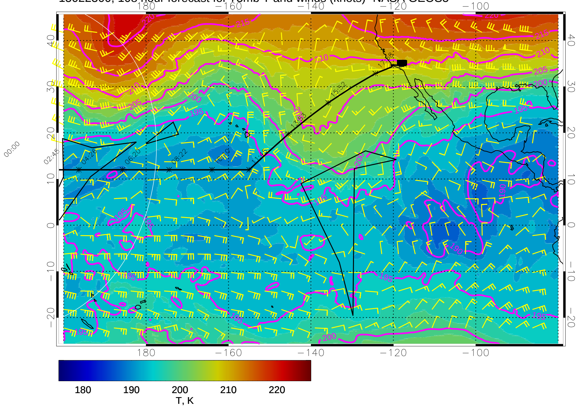
15022300, 108 hour forecast for 73mb T and winds (knots)- NASA GEOS5
