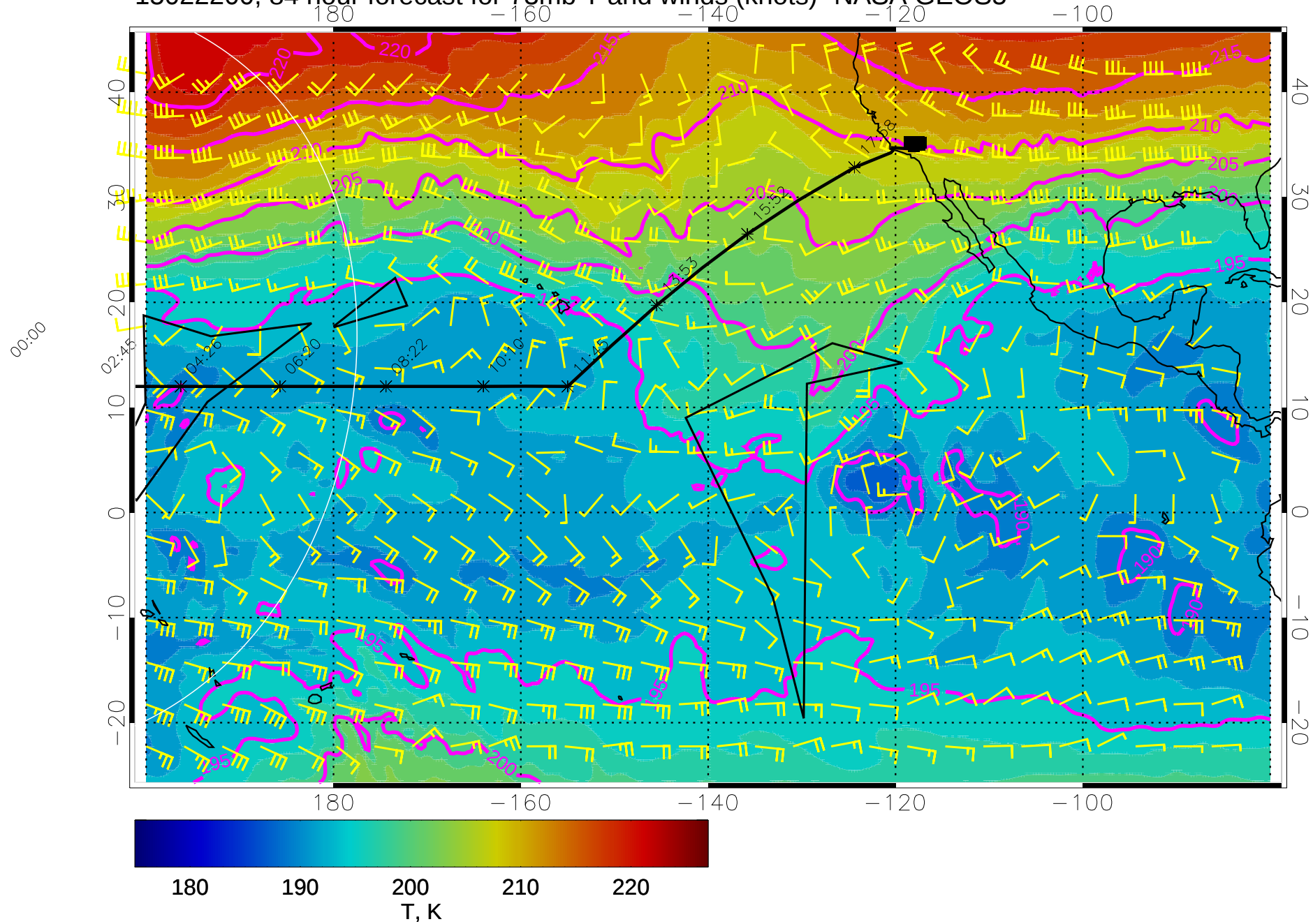
15022200, 84 hour forecast for 73mb T and winds (knots)- NASA GEOS5
