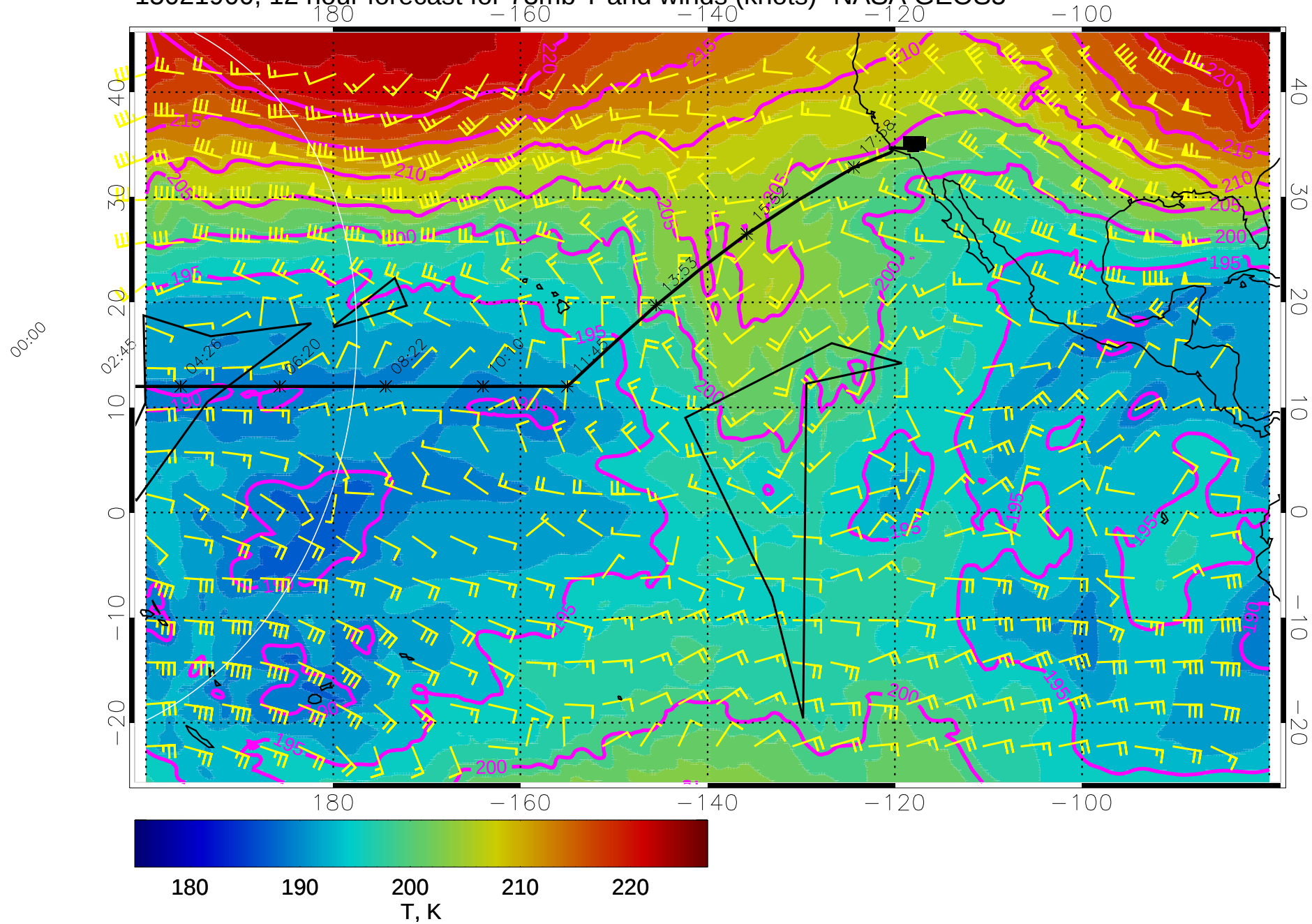
15021900, 12 hour forecast for 73mb T and winds (knots)- NASA GEOS5
