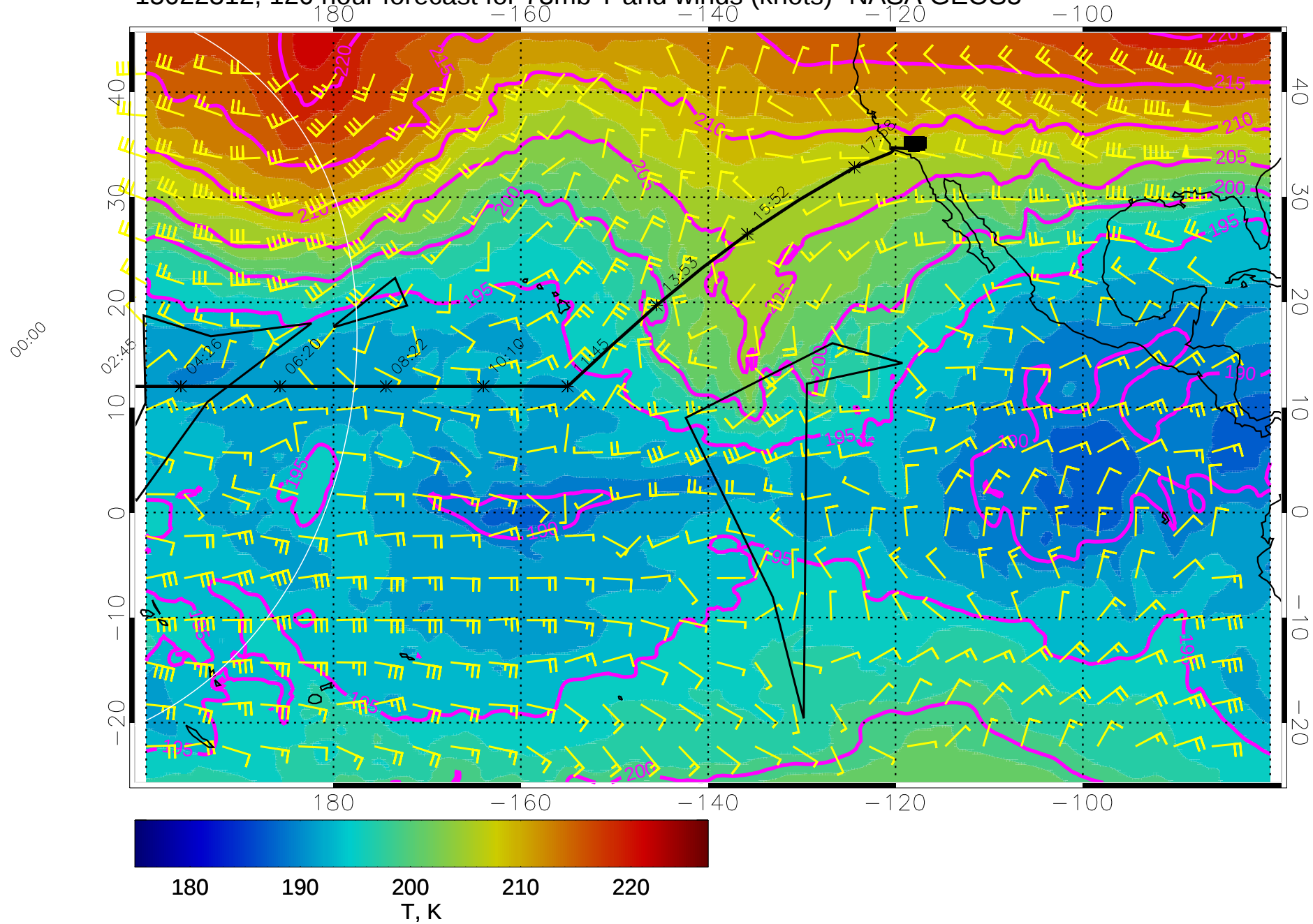
15022312, 120 hour forecast for 73mb T and winds (knots)- NASA GEOS5
