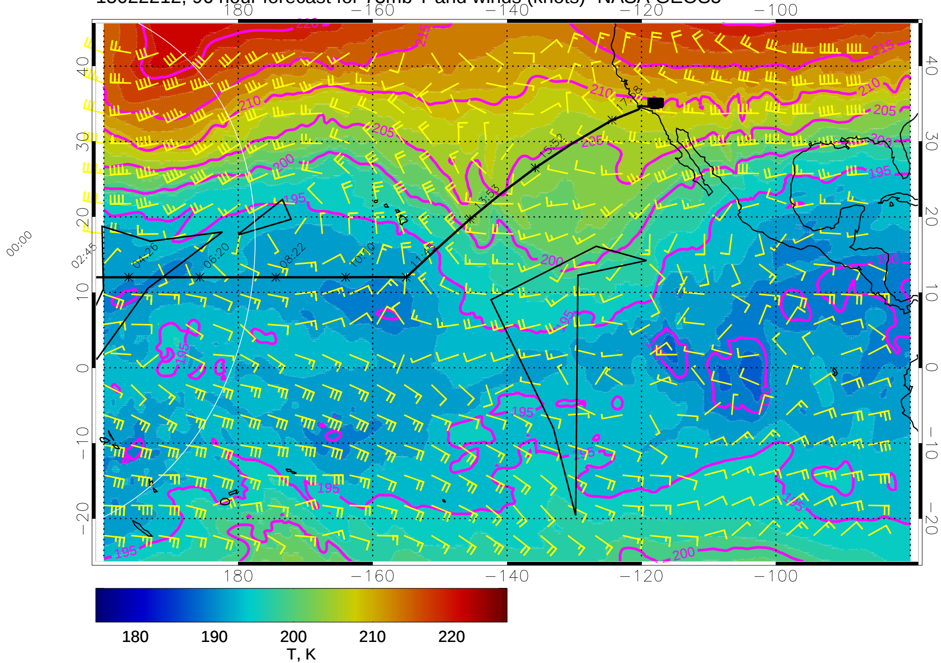
15022212, 96 hour forecast for 73mb T and winds (knots)- NASA GEOS5
