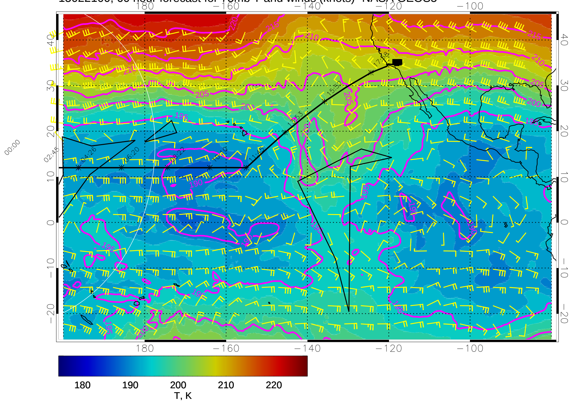
15022100, 60 hour forecast for 73mb T and winds (knots)- NASA GEOS5
