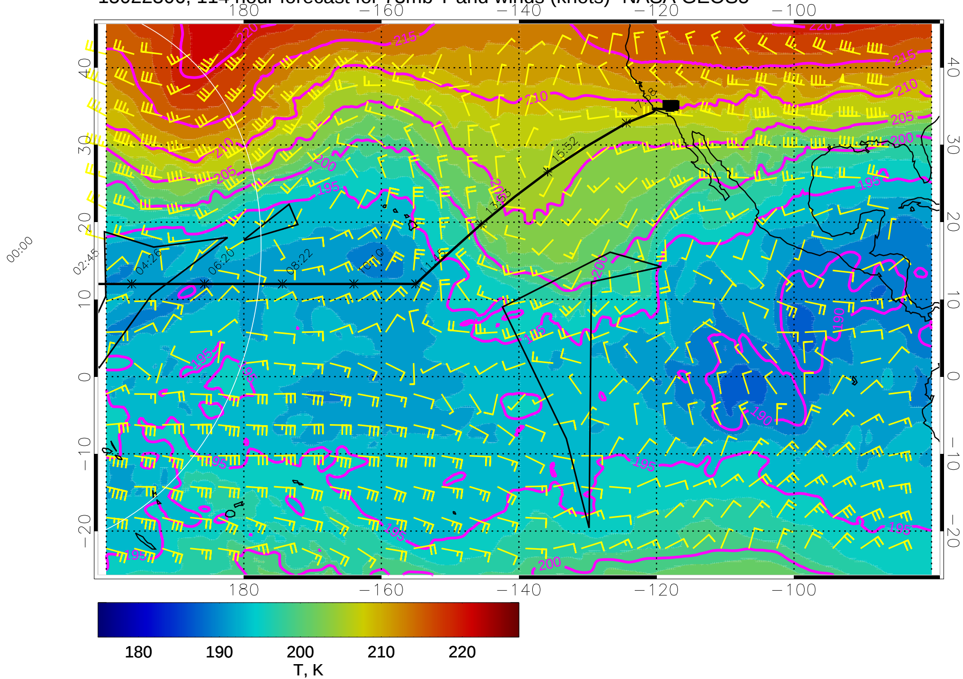
15022306, 114 hour forecast for 73mb T and winds (knots)- NASA GEOS5
