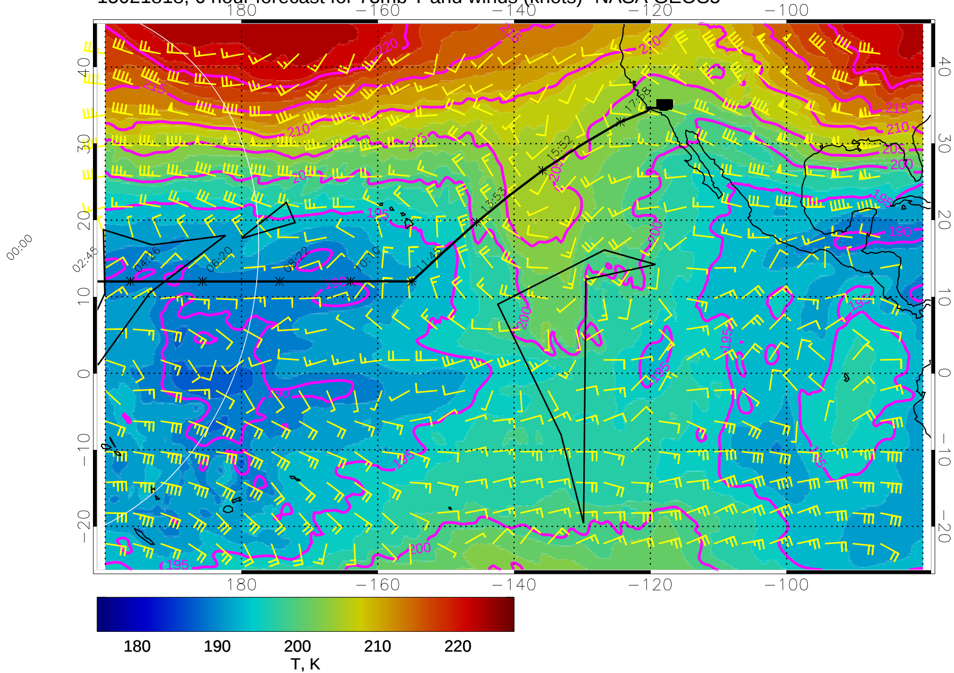
15021818, 6 hour forecast for 73mb T and winds (knots)- NASA GEOS5
