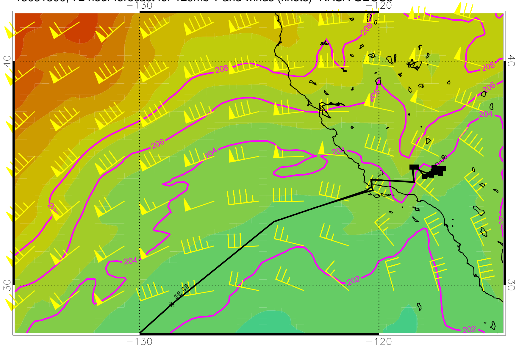
15031500, 72 hour forecast for 120mb T and winds (knots)- NASA GEOS5
