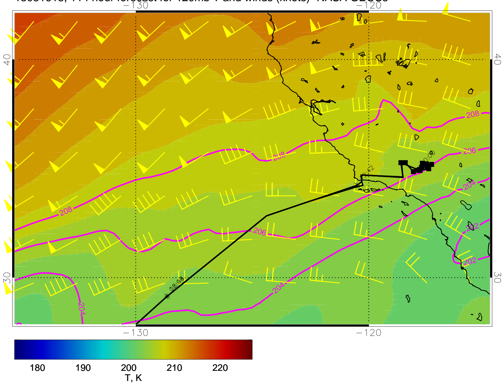
15031618, 114 hour forecast for 120mb T and winds (knots)- NASA GEOS5
