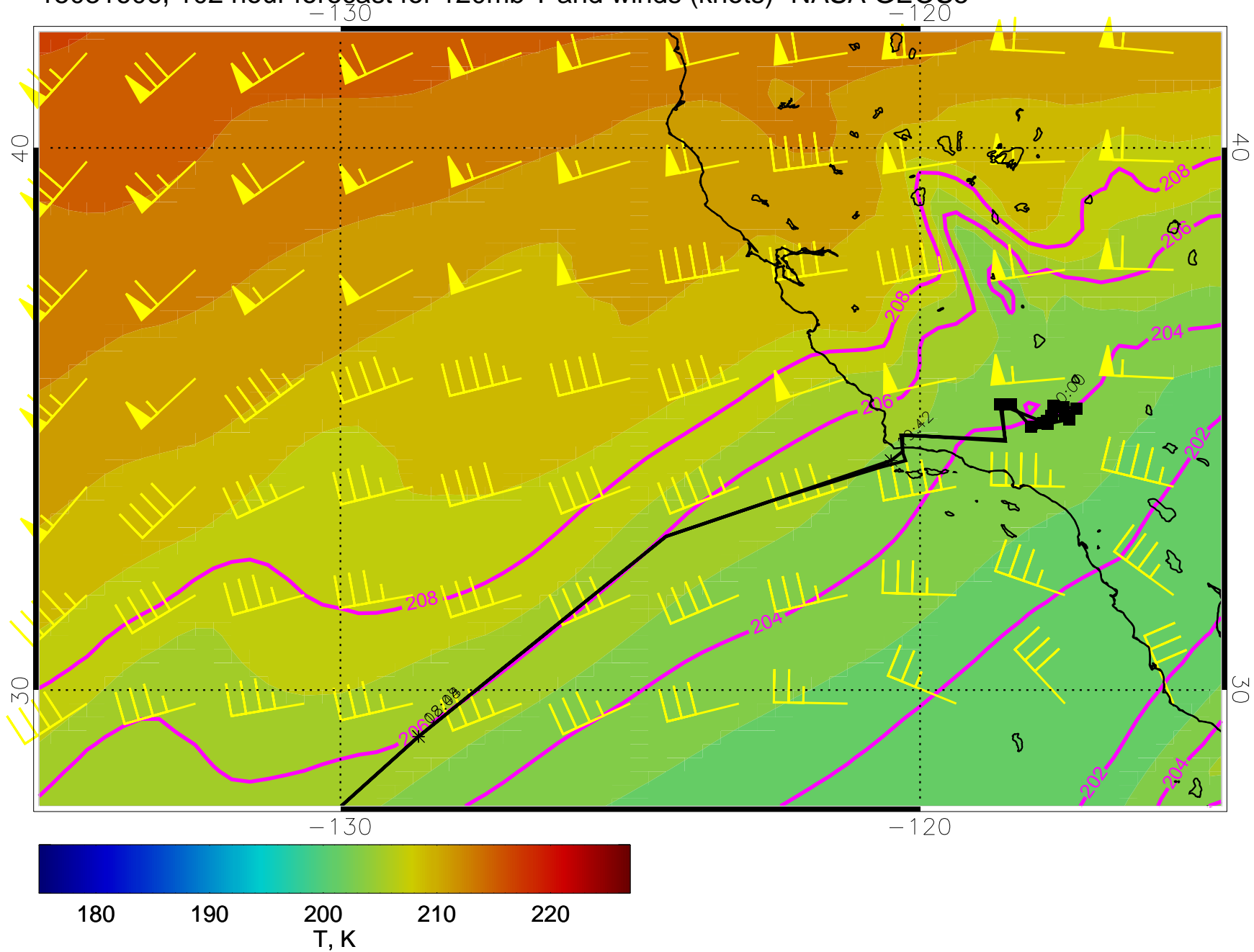
15031606, 102 hour forecast for 120mb T and winds (knots)- NASA GEOS5
