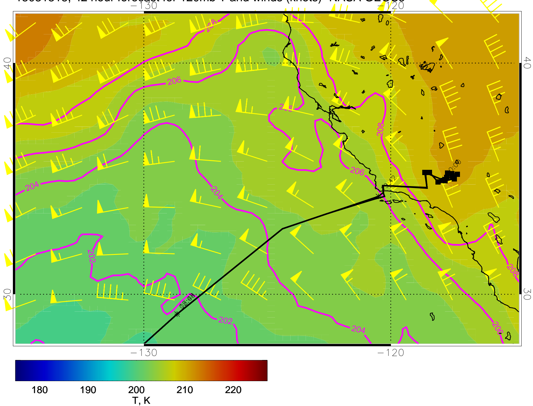
15031318, 42 hour forecast for 120mb T and winds (knots)- NASA GEOS5
