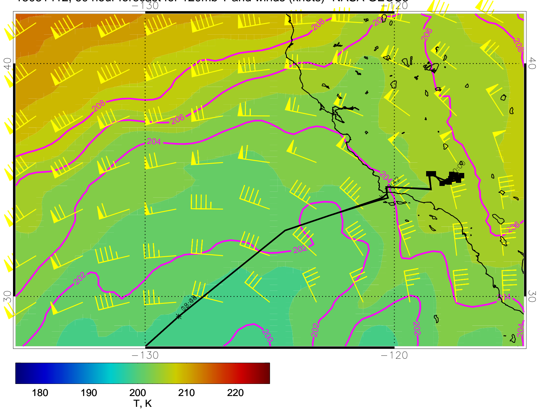
15031412, 60 hour forecast for 120mb T and winds (knots)- NASA GEOS5
