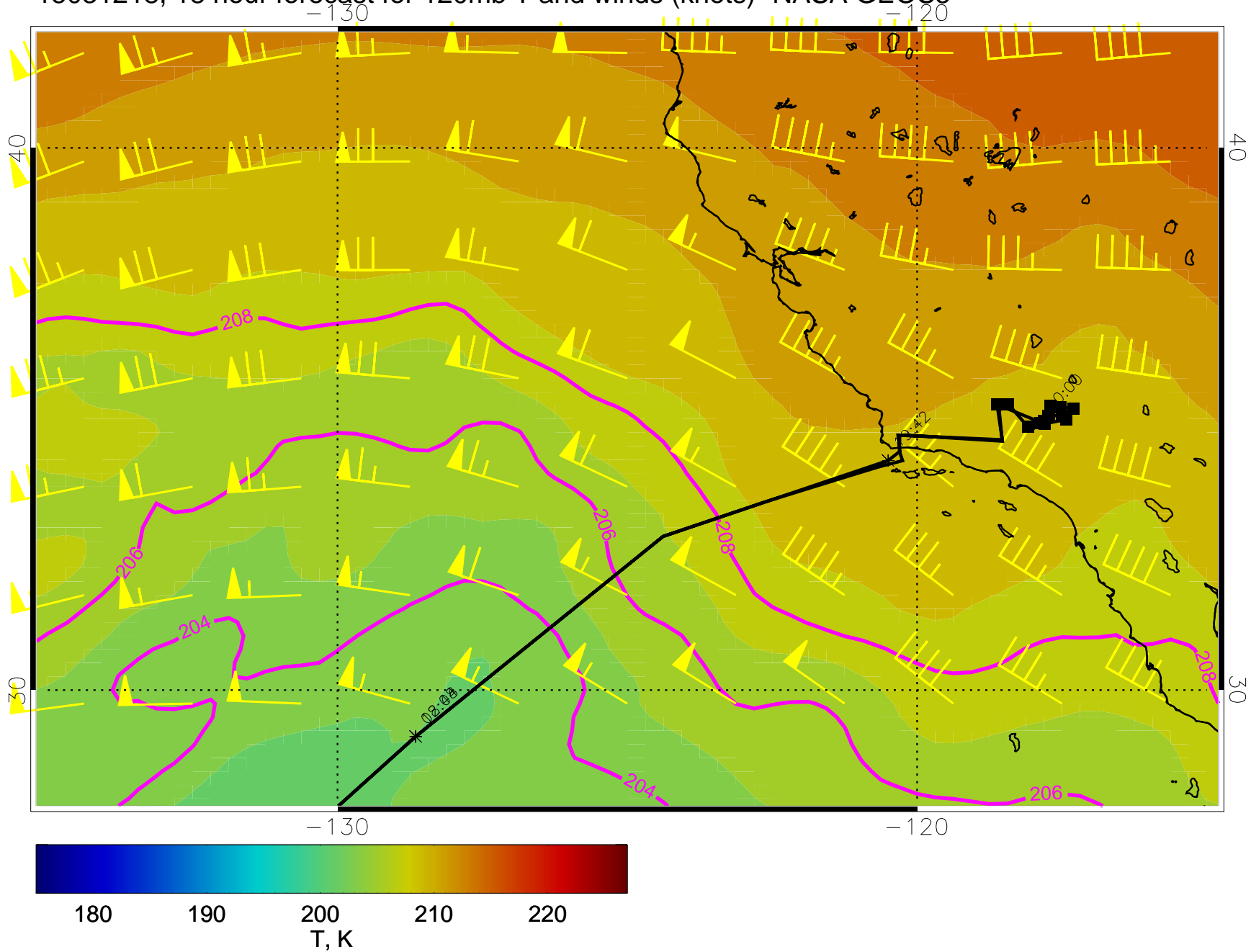
15031218, 18 hour forecast for 120mb T and winds (knots)- NASA GEOS5
