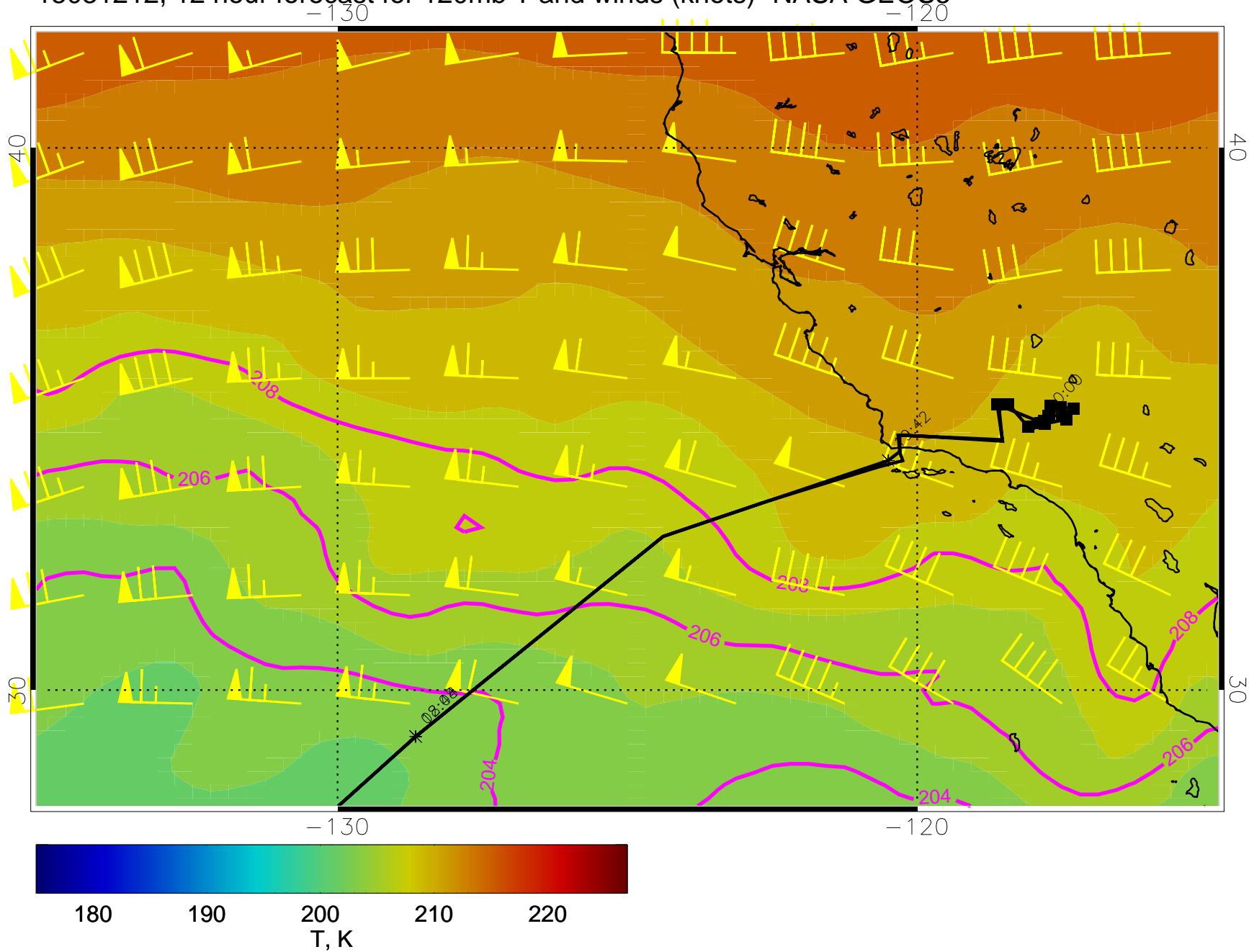
15031212, 12 hour forecast for 120mb T and winds (knots)- NASA GEOS5
