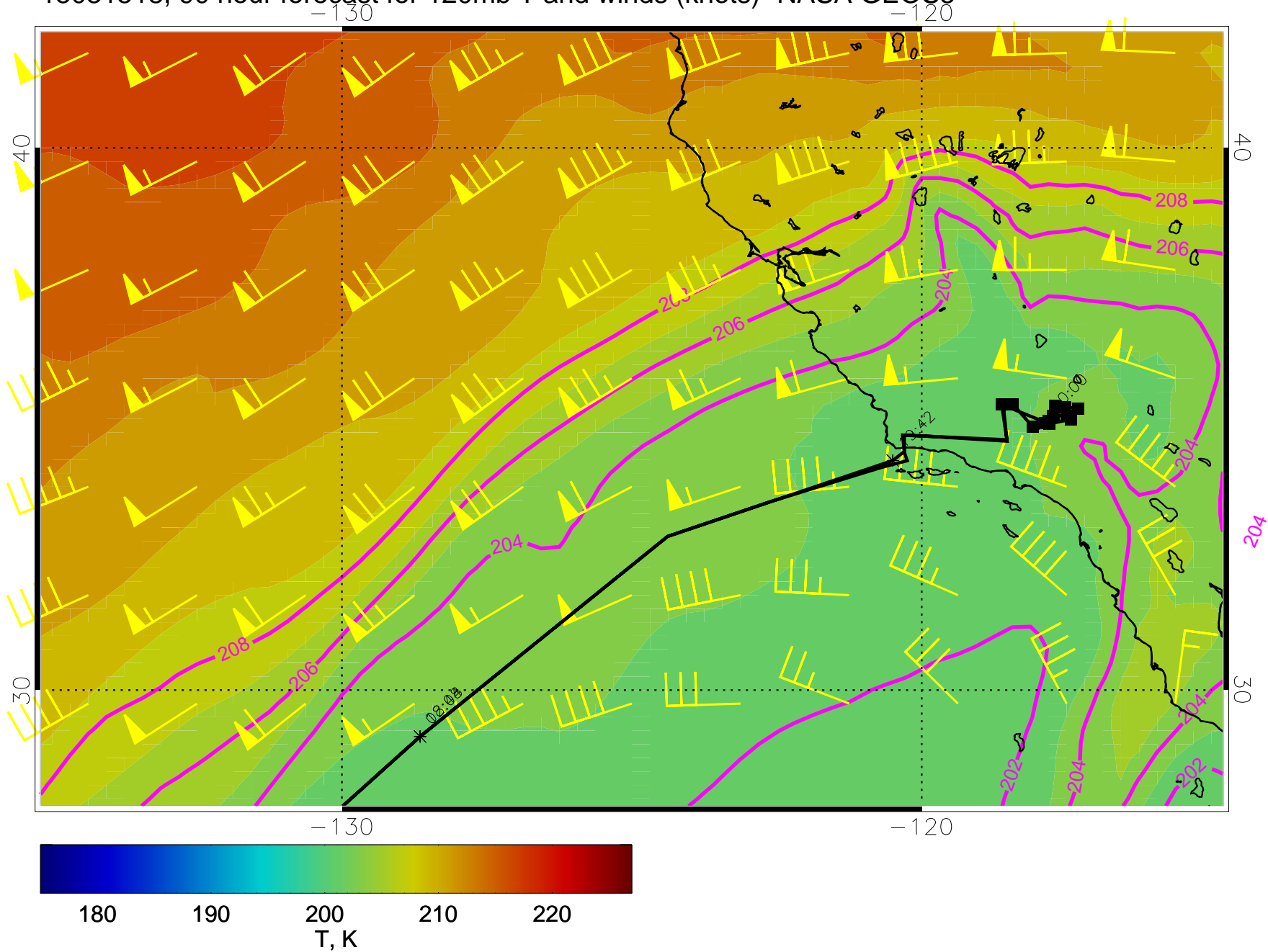
15031518, 90 hour forecast for 120mb T and winds (knots)- NASA GEOS5
