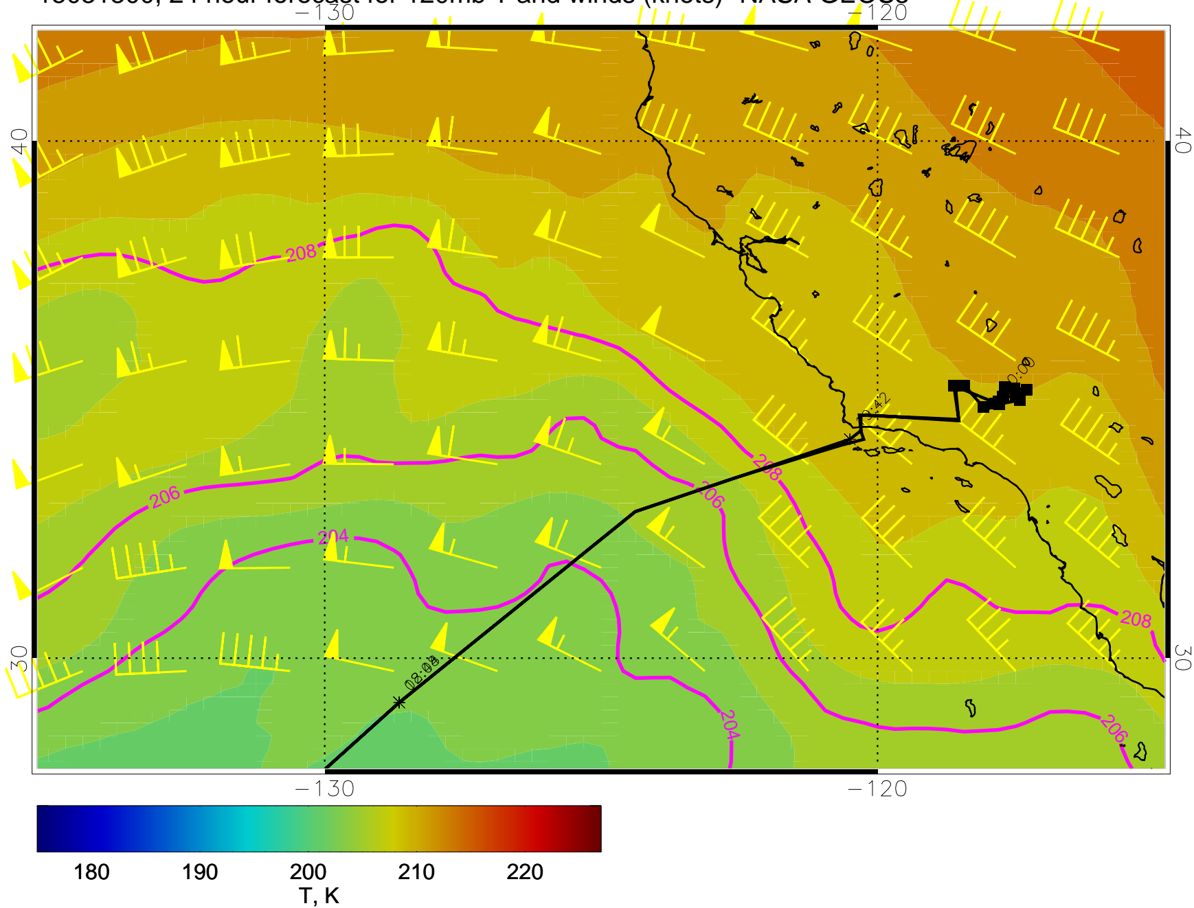
15031300, 24 hour forecast for 120mb T and winds (knots)- NASA GEOS5
