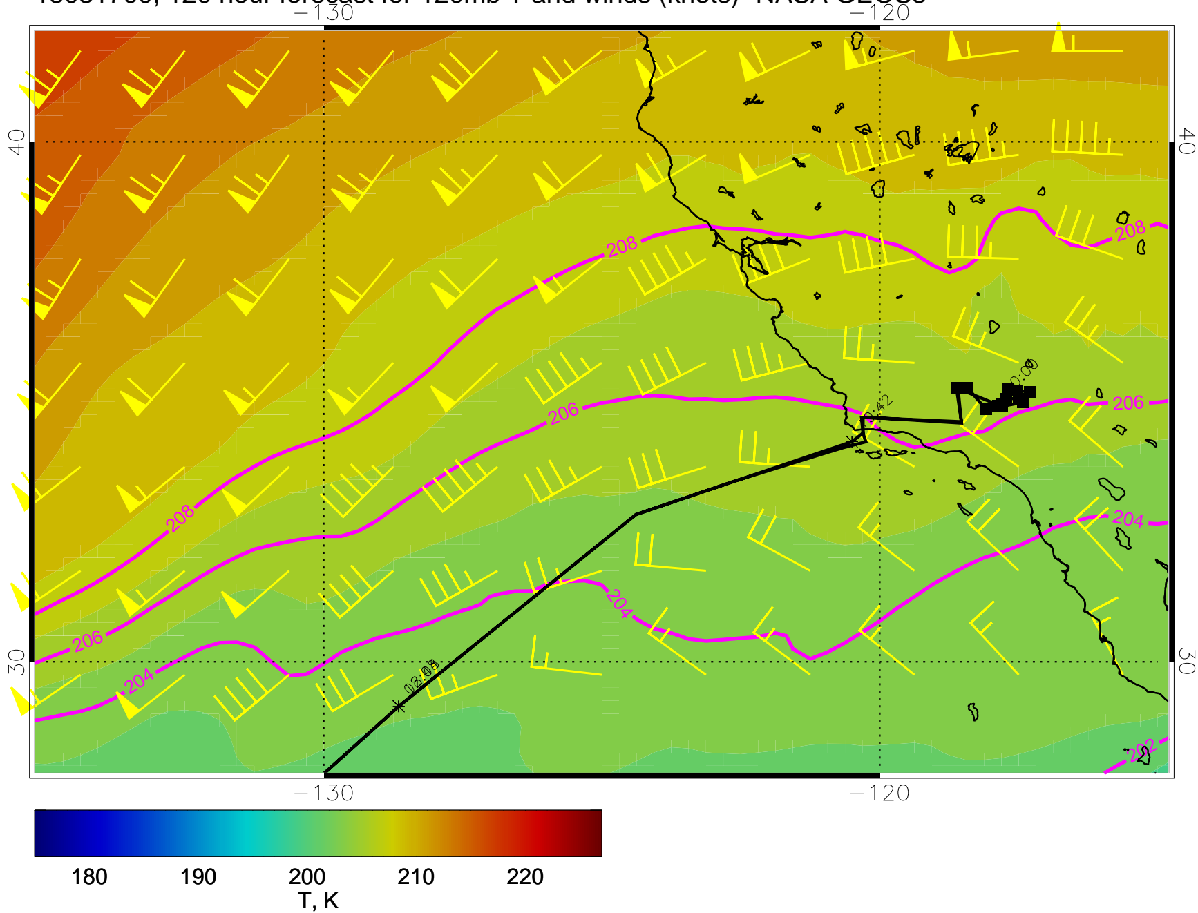
15031700, 120 hour forecast for 120mb T and winds (knots)- NASA GEOS5
