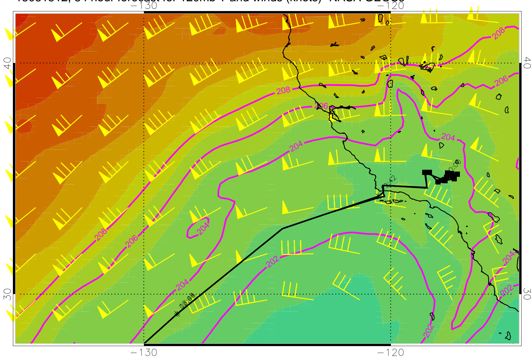
15031512, 84 hour forecast for 120mb T and winds (knots)- NASA GEOS5
