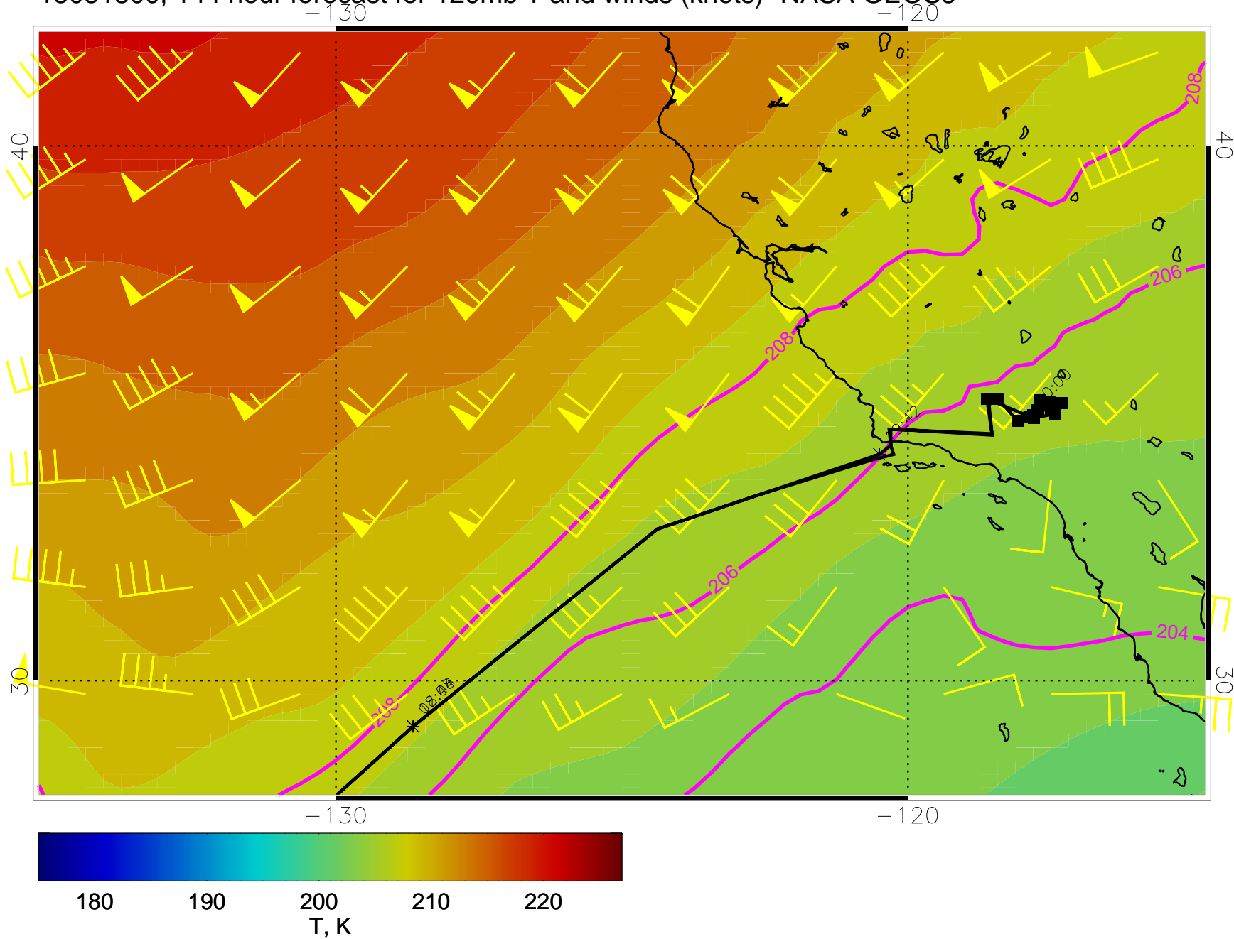
15031800, 144 hour forecast for 120mb T and winds (knots)- NASA GEOS5
