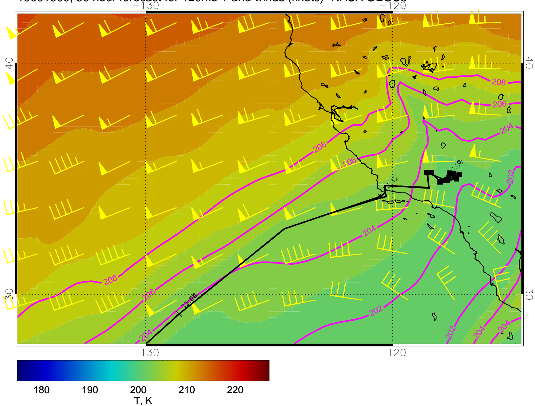
15031600, 96 hour forecast for 120mb T and winds (knots)- NASA GEOS5
