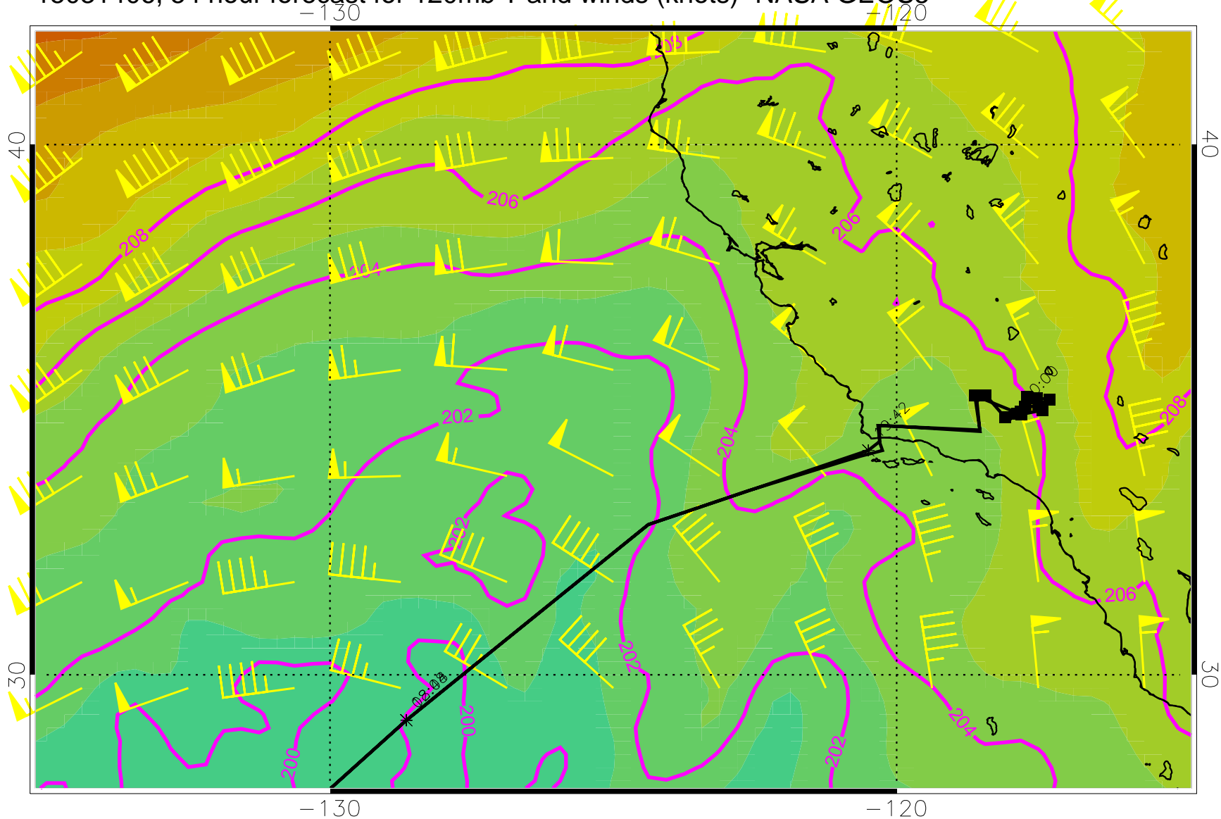
15031406, 54 hour forecast for 120mb T and winds (knots)- NASA GEOS5
