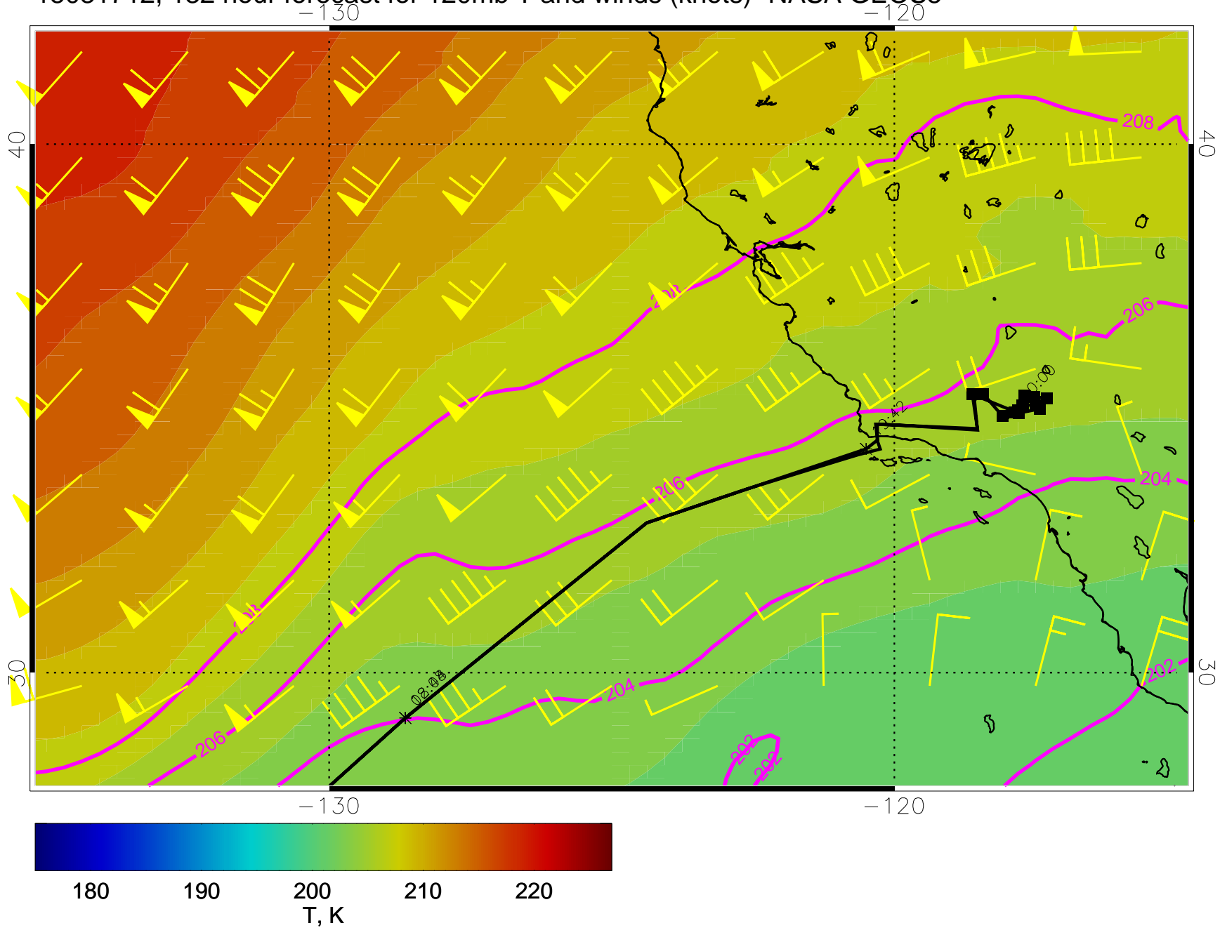
15031712, 132 hour forecast for 120mb T and winds (knots)- NASA GEOS5
