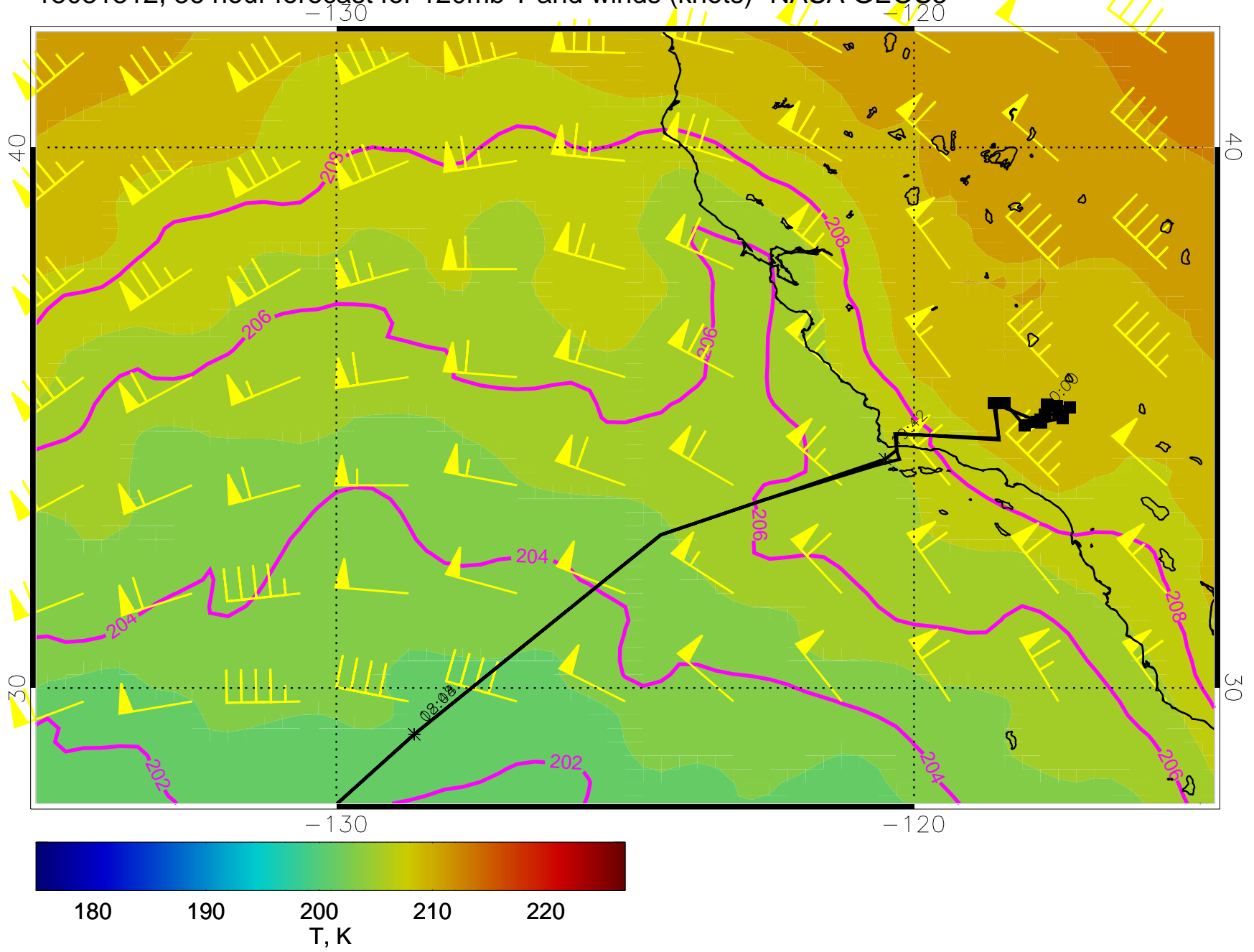
15031312, 36 hour forecast for 120mb T and winds (knots)- NASA GEOS5
