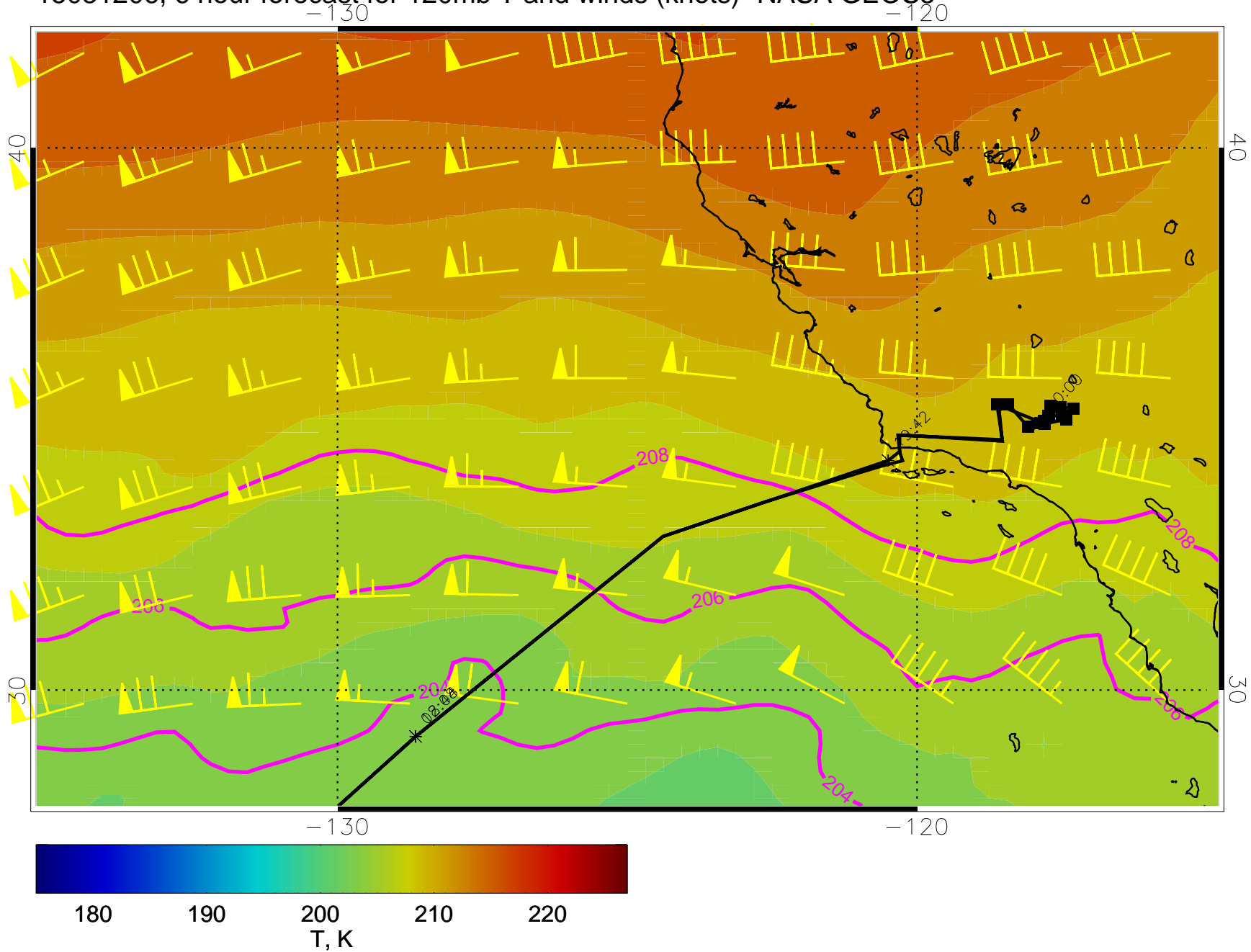
15031206, 6 hour forecast for 120mb T and winds (knots)- NASA GEOS5
