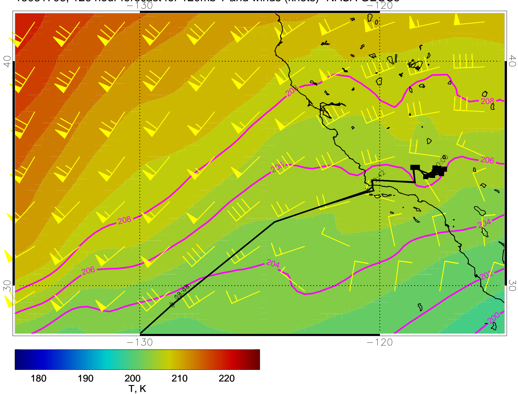
15031706, 126 hour forecast for 120mb T and winds (knots)- NASA GEOS5
