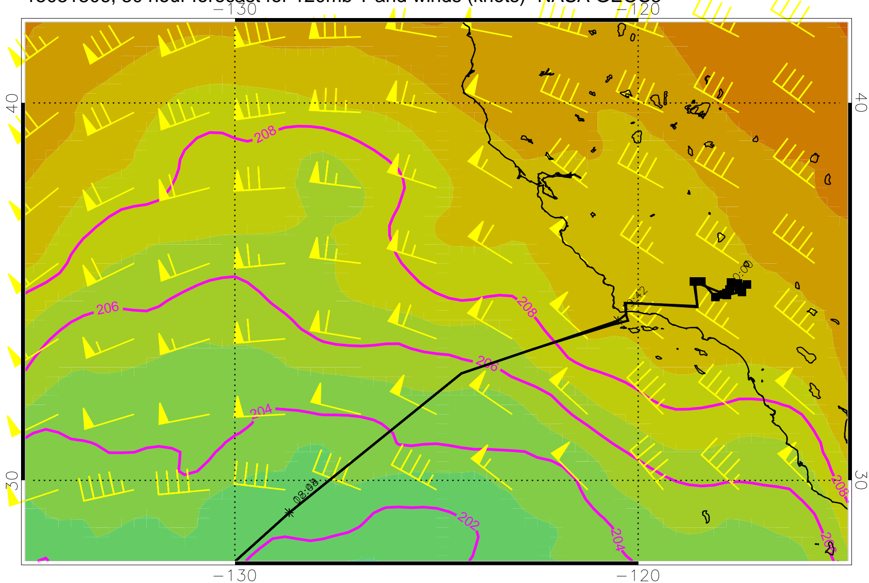
15031306, 30 hour forecast for 120mb T and winds (knots)- NASA GEOS5
