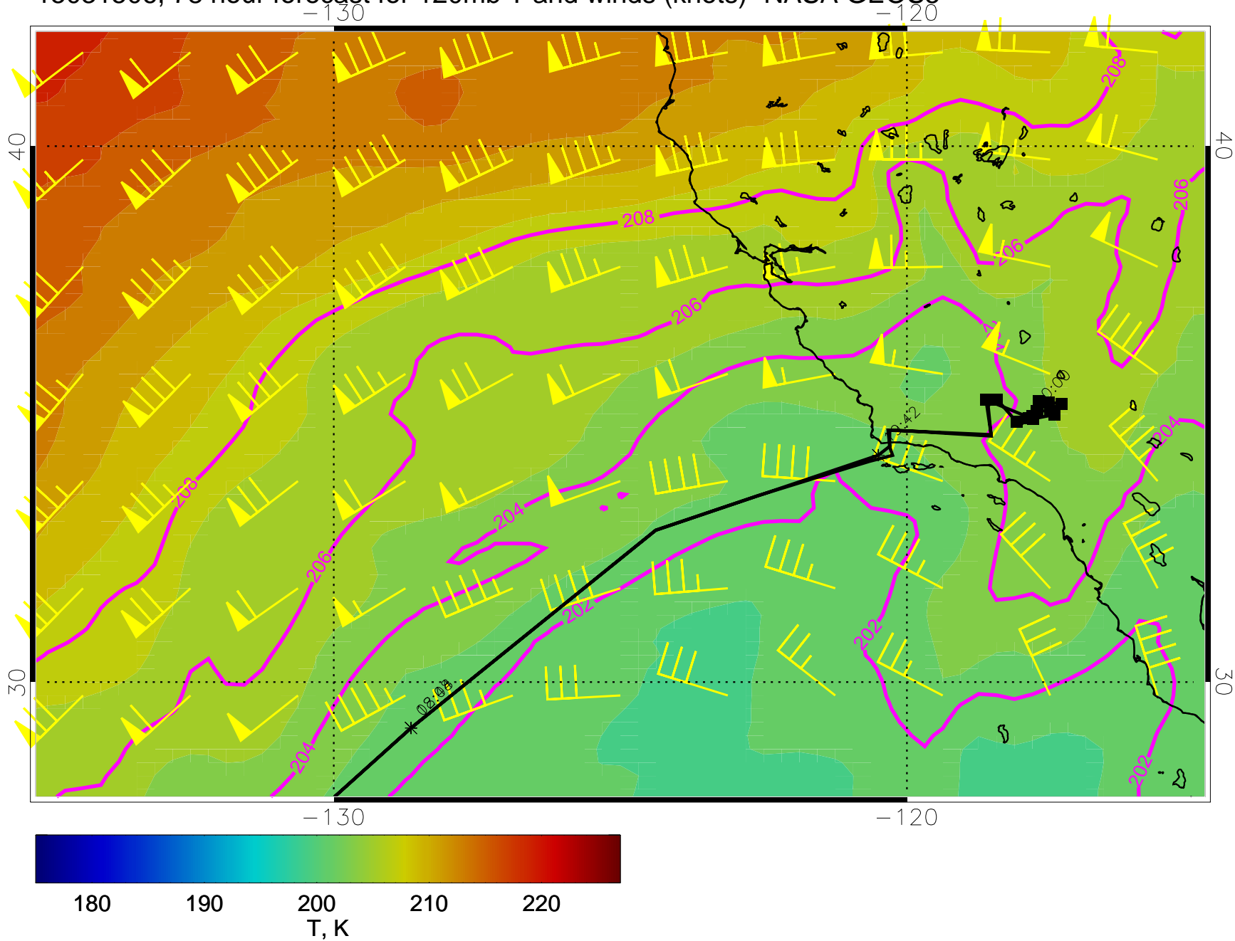
15031506, 78 hour forecast for 120mb T and winds (knots)- NASA GEOS5
