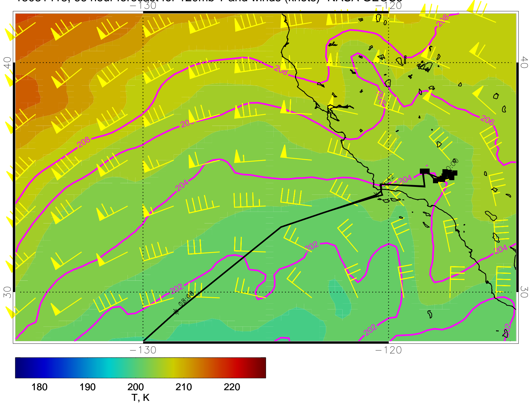
15031418, 66 hour forecast for 120mb T and winds (knots)- NASA GEOS5
