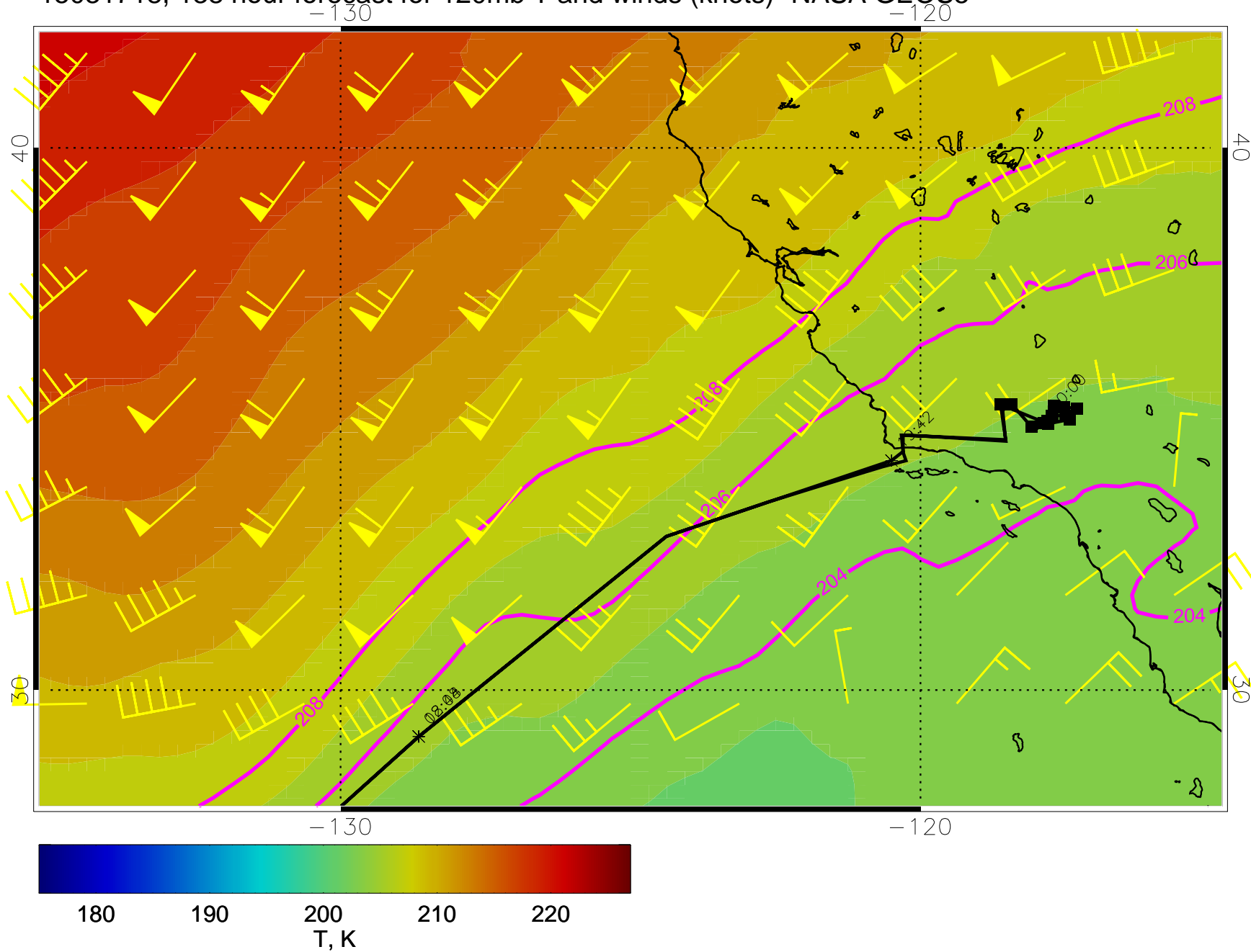
15031718, 138 hour forecast for 120mb T and winds (knots)- NASA GEOS5
