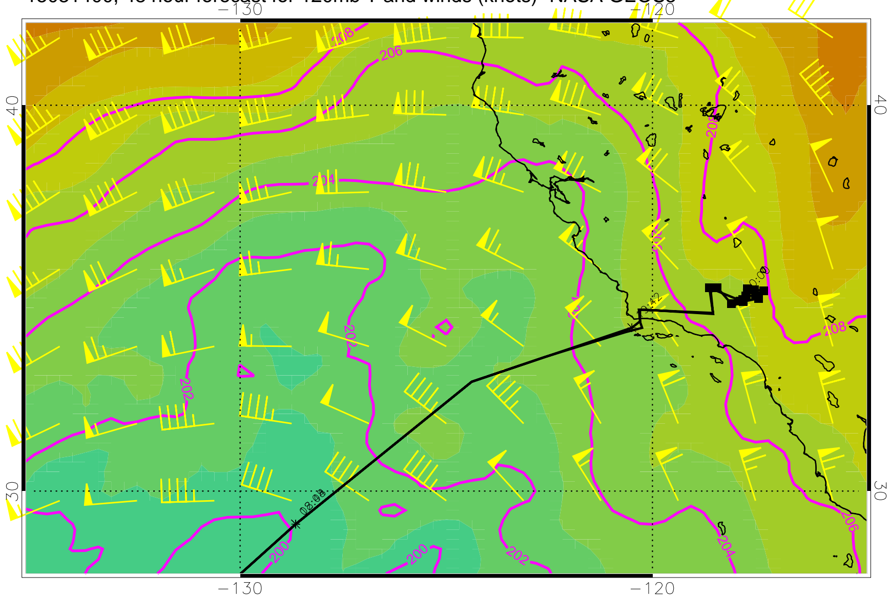
15031400, 48 hour forecast for 120mb T and winds (knots)- NASA GEOS5
