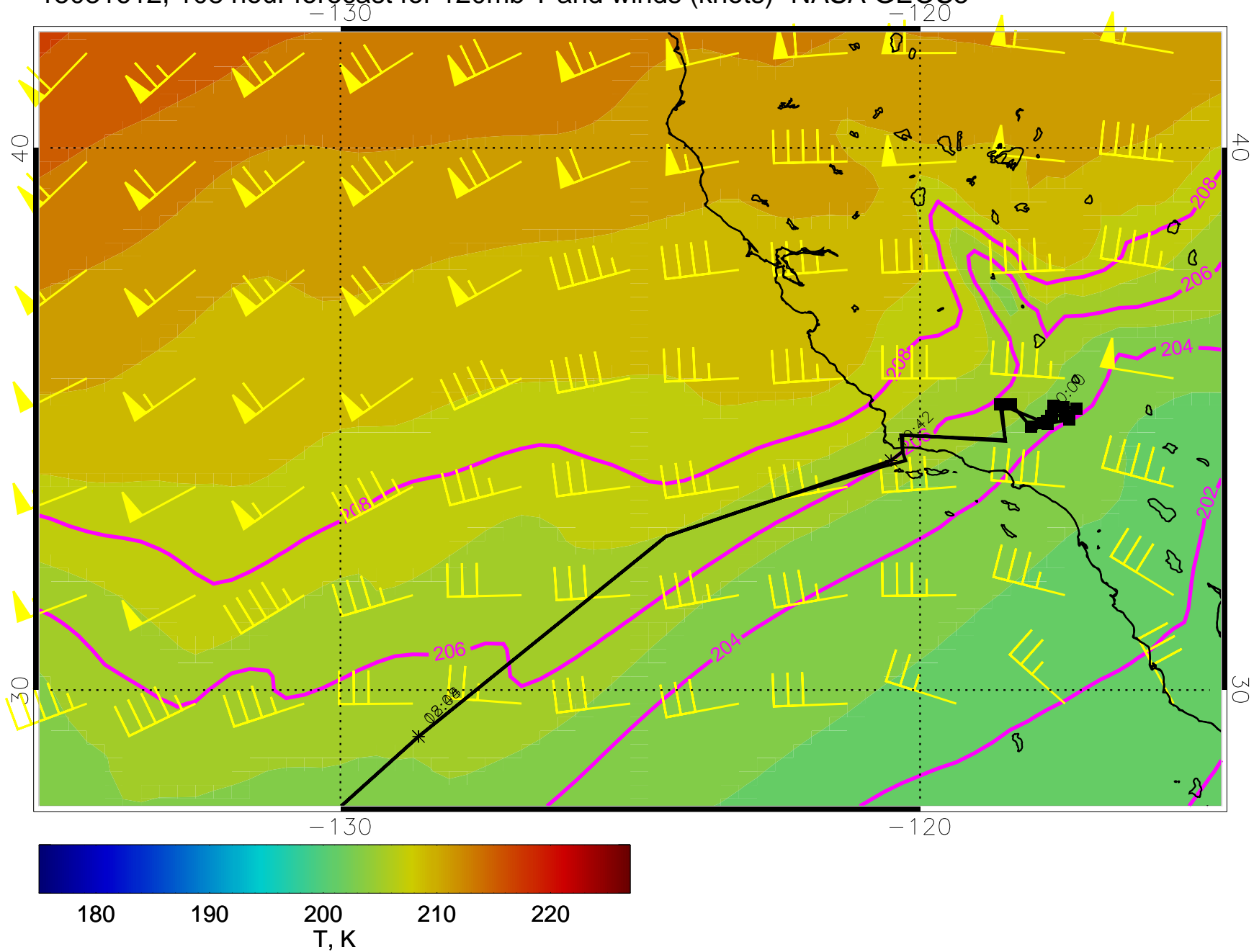
15031612, 108 hour forecast for 120mb T and winds (knots)- NASA GEOS5
