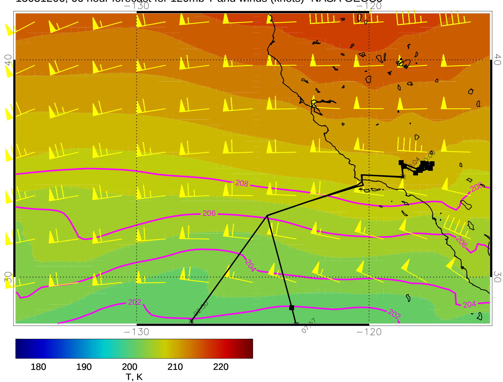
15031206, 66 hour forecast for 120mb T and winds (knots)- NASA GEOS5
