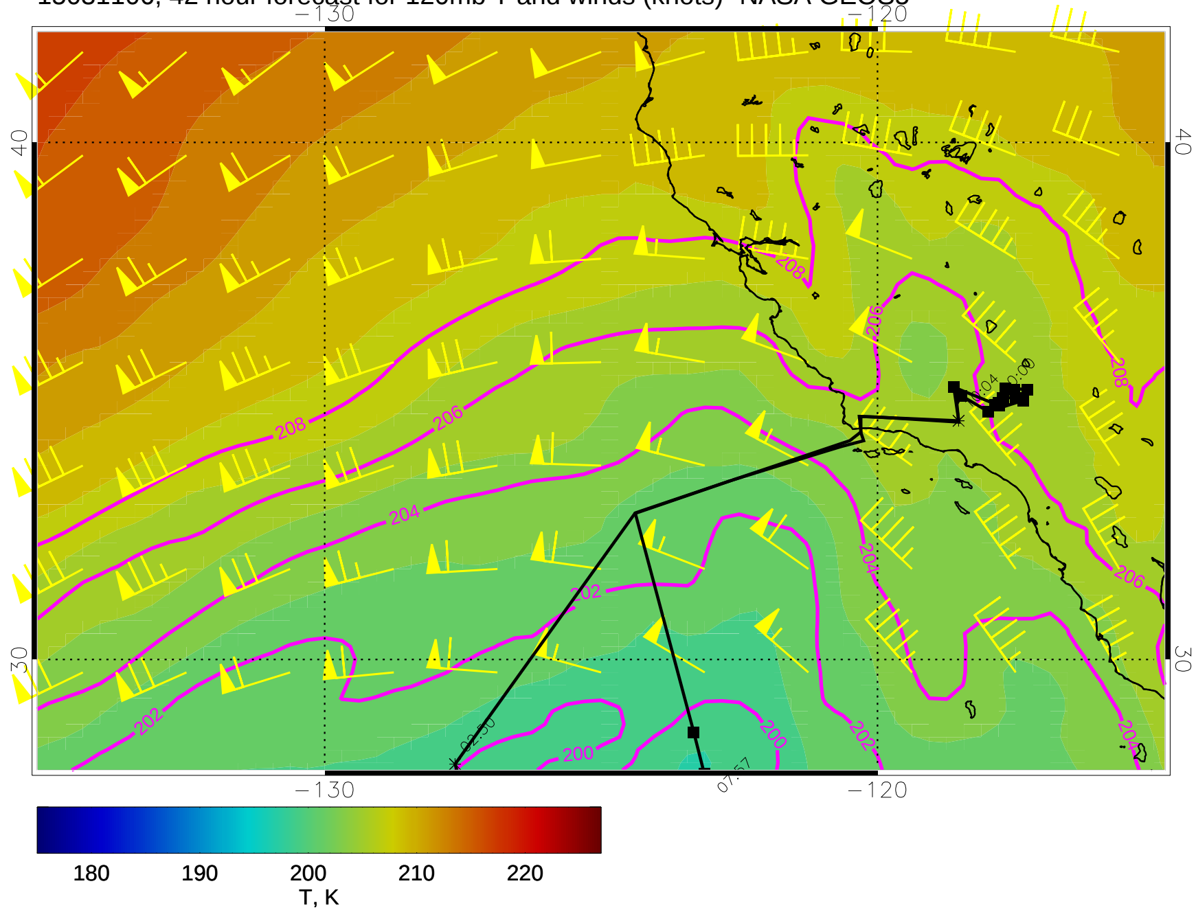
15031106, 42 hour forecast for 120mb T and winds (knots)- NASA GEOS5
