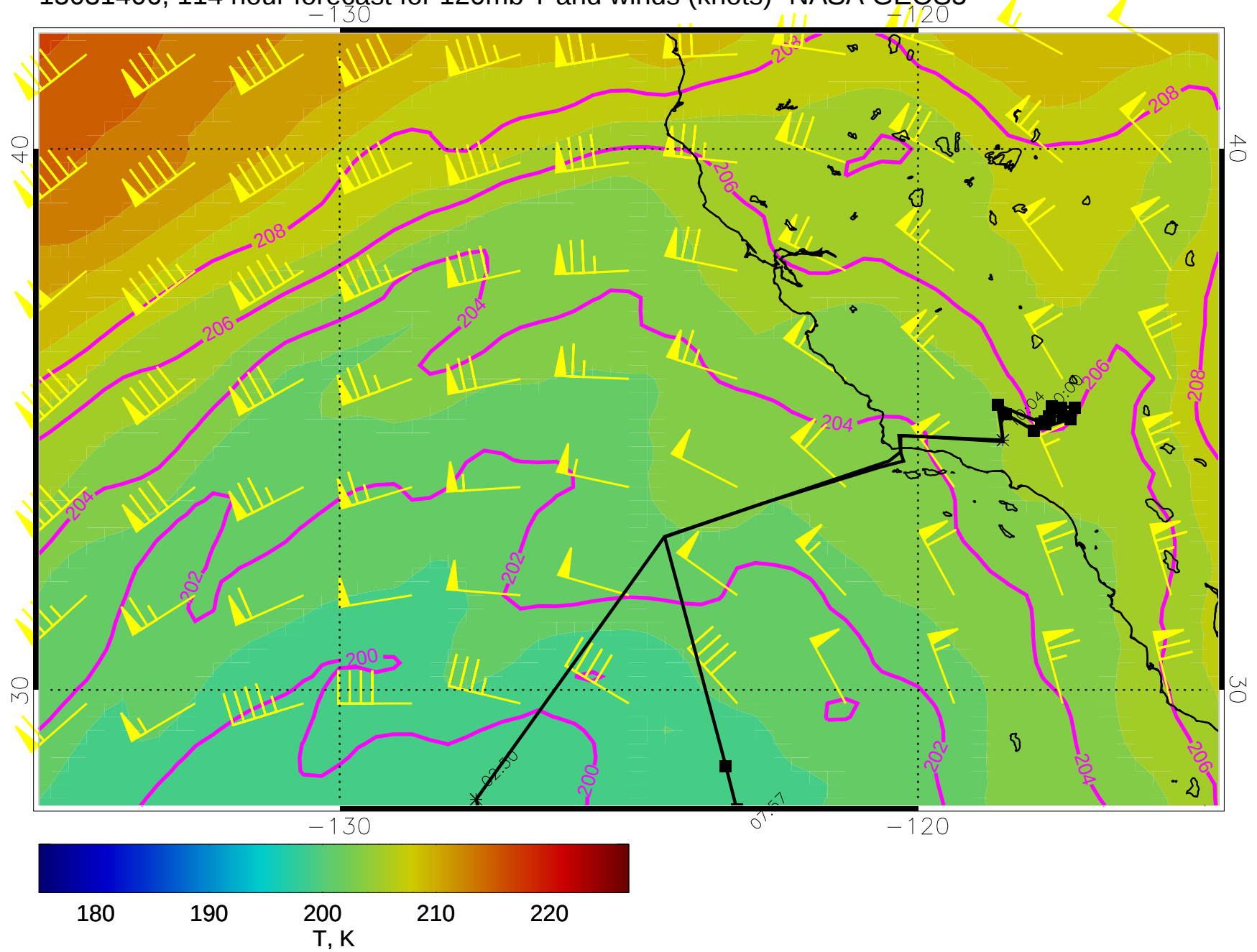
15031406, 114 hour forecast for 120mb T and winds (knots)- NASA GEOS5
