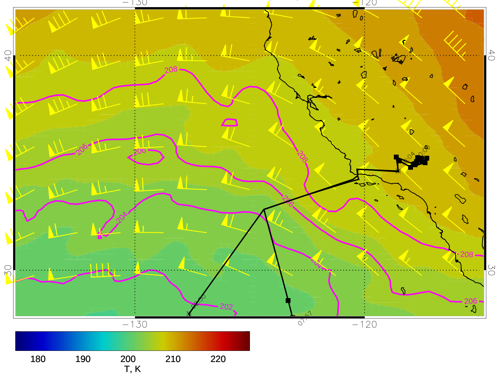
15031306, 90 hour forecast for 120mb T and winds (knots)- NASA GEOS5
