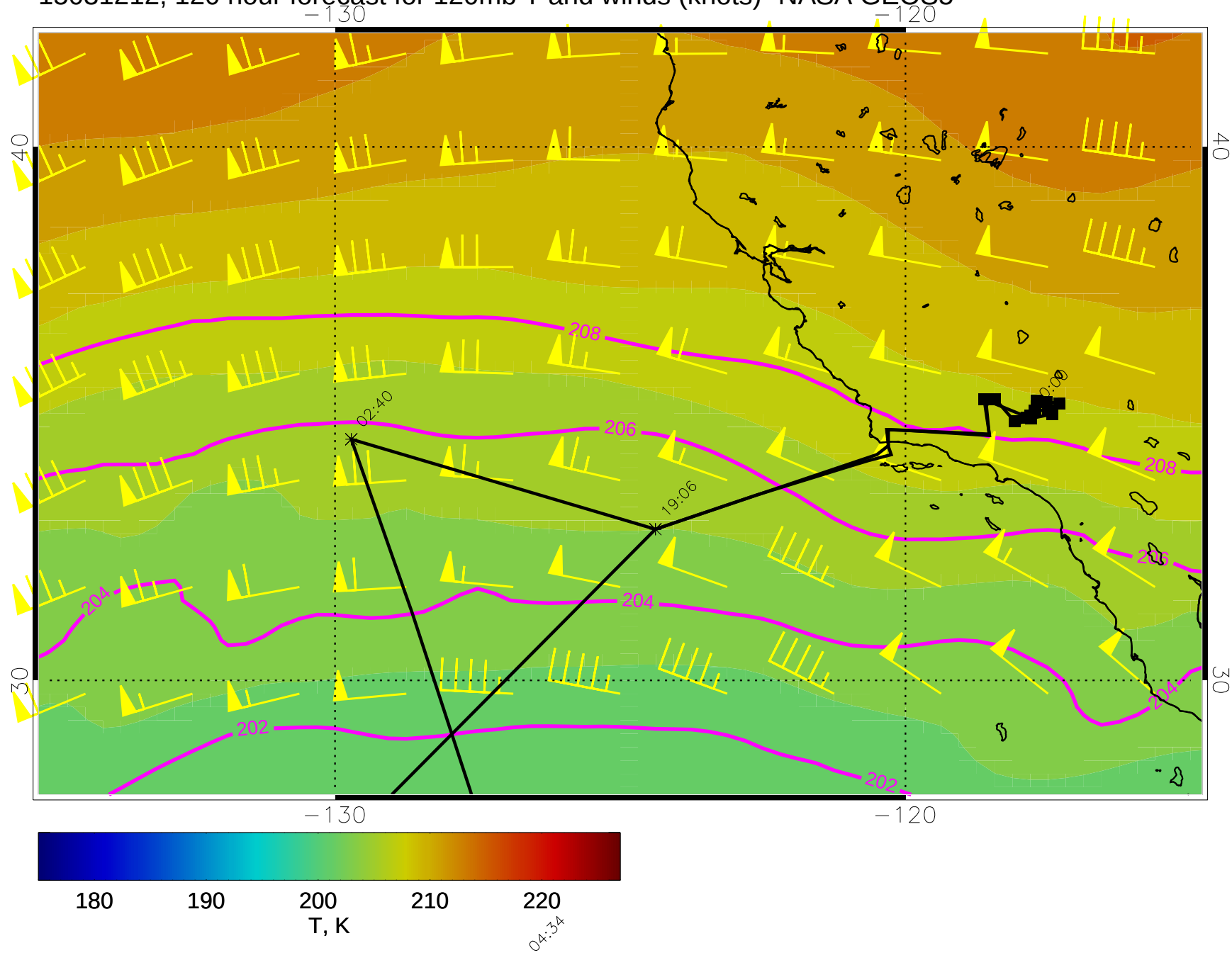
15031212, 120 hour forecast for 120mb T and winds (knots)- NASA GEOS5
