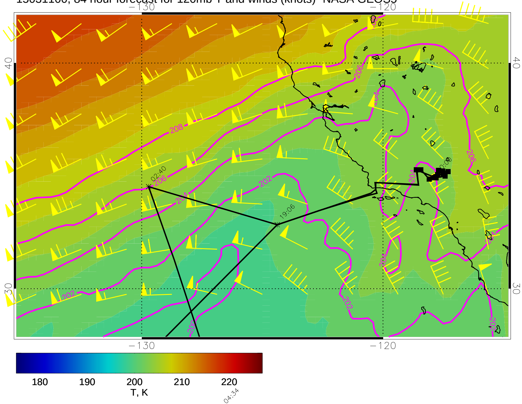
15031100, 84 hour forecast for 120mb T and winds (knots)- NASA GEOS5
