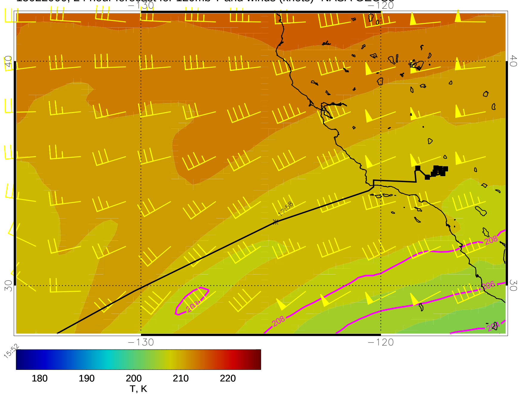
15022000, 24 hour forecast for 120mb T and winds (knots)- NASA GEOS5
