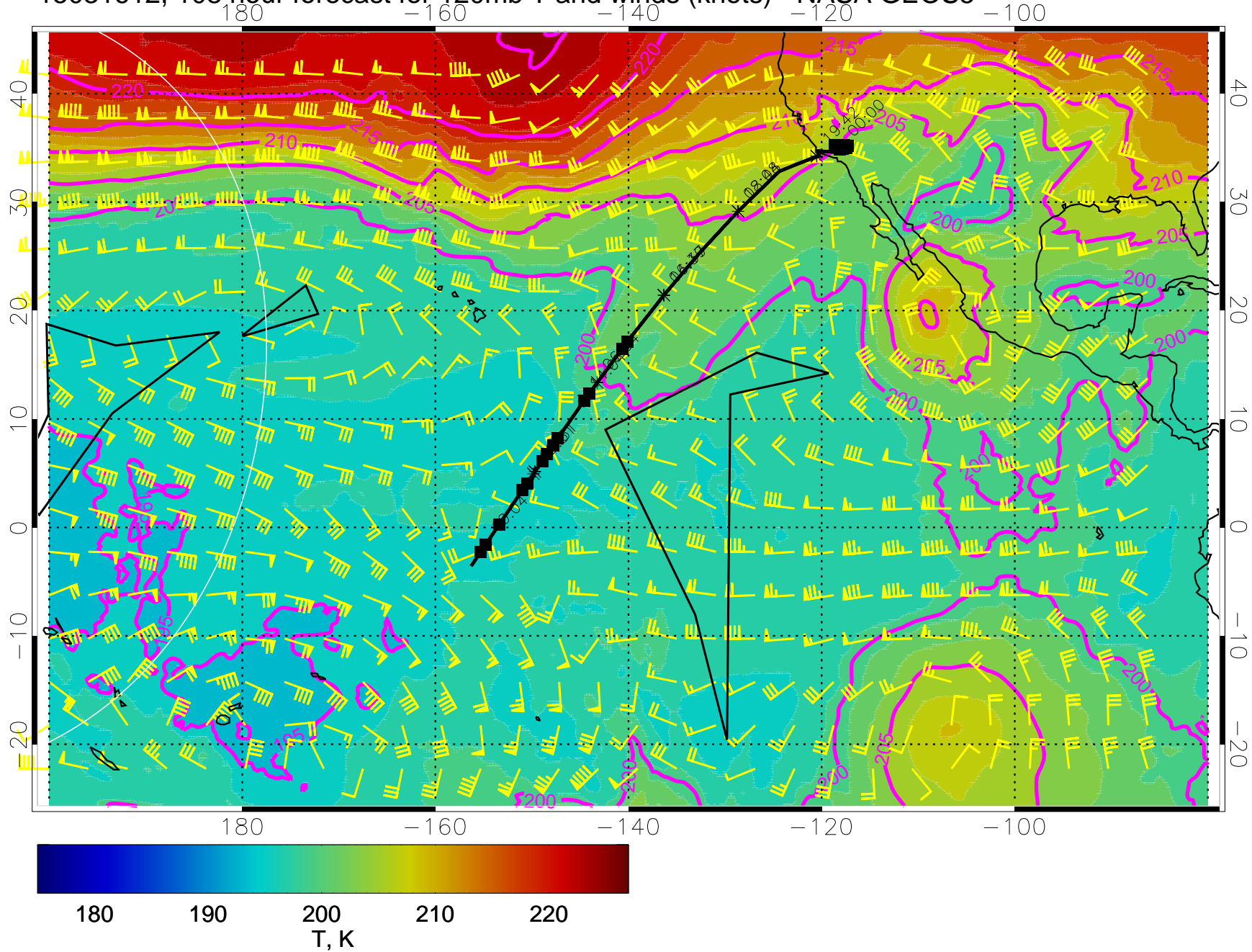
15031612, 108 hour forecast for 120mb T and winds (knots) - NASA GEOS5
