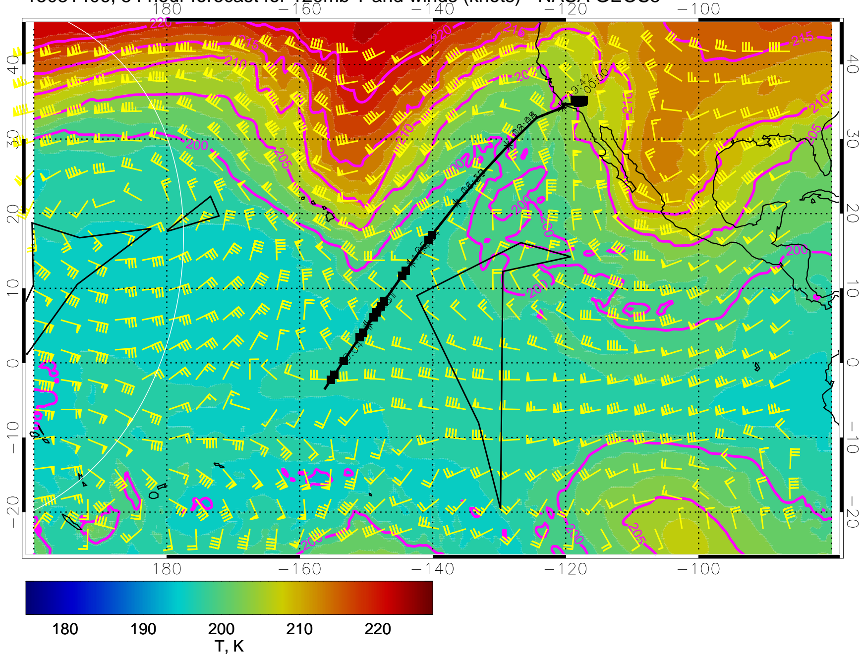
15031406, 54 hour forecast for 120mb T and winds (knots) - NASA GEOS5
