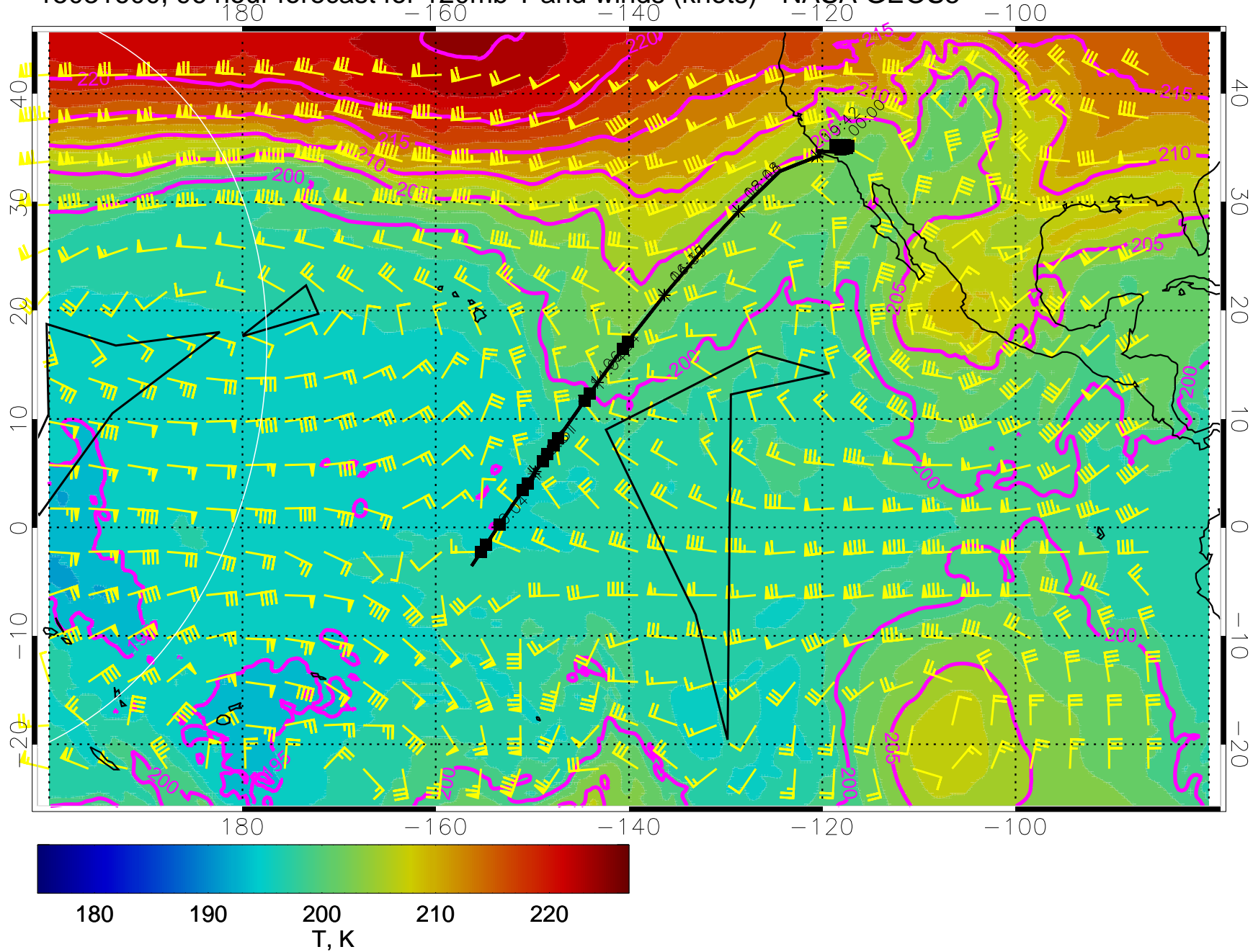
15031600, 96 hour forecast for 120mb T and winds (knots) - NASA GEOS5
