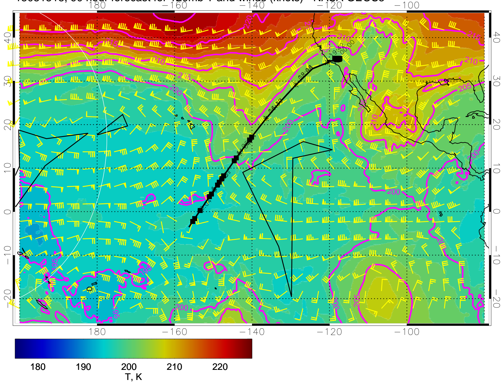
15031518, 90 hour forecast for 120mb T and winds (knots) - NASA GEOS5
