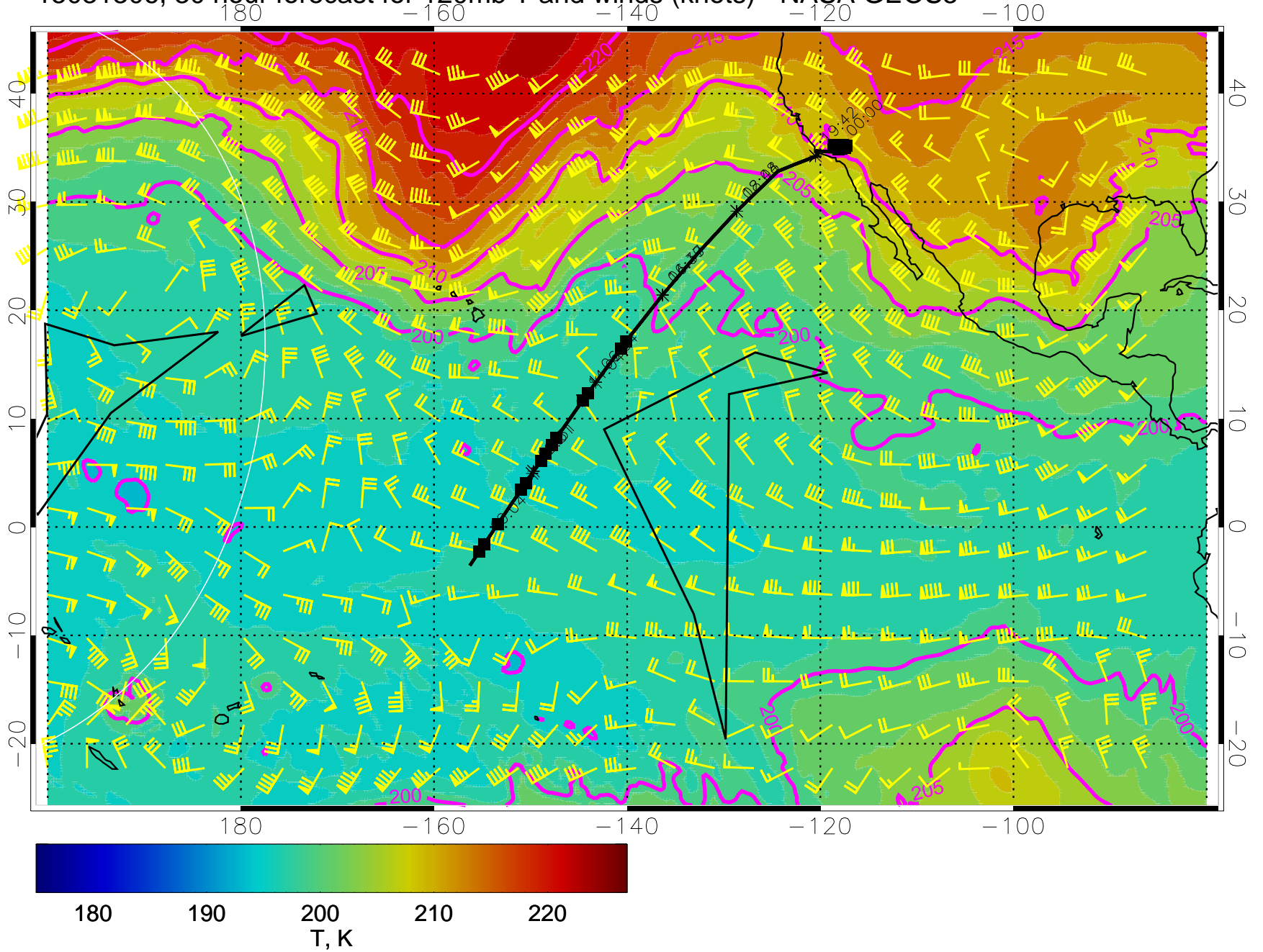
15031306, 30 hour forecast for 120mb T and winds (knots) - NASA GEOS5
