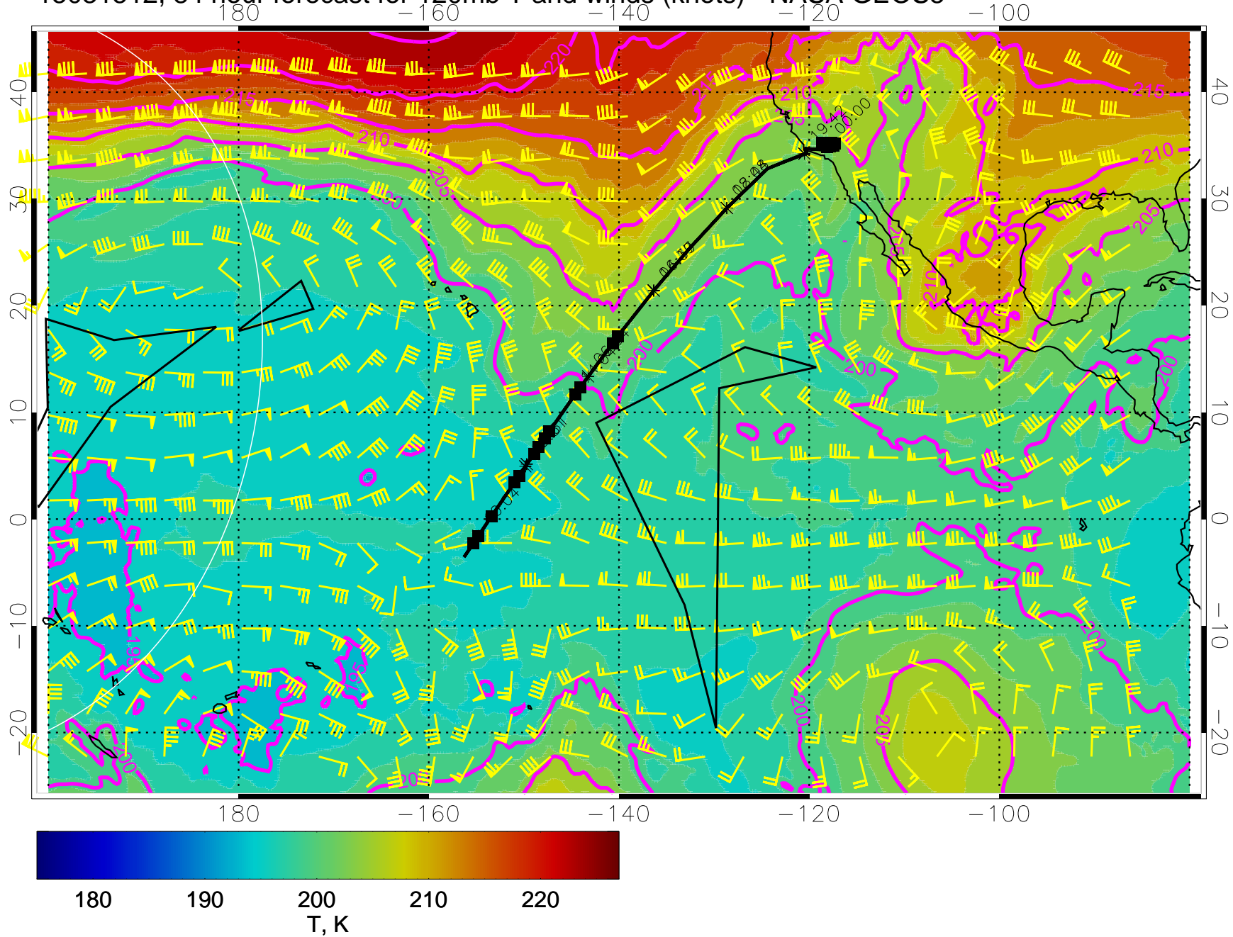
15031512, 84 hour forecast for 120mb T and winds (knots) - NASA GEOS5
