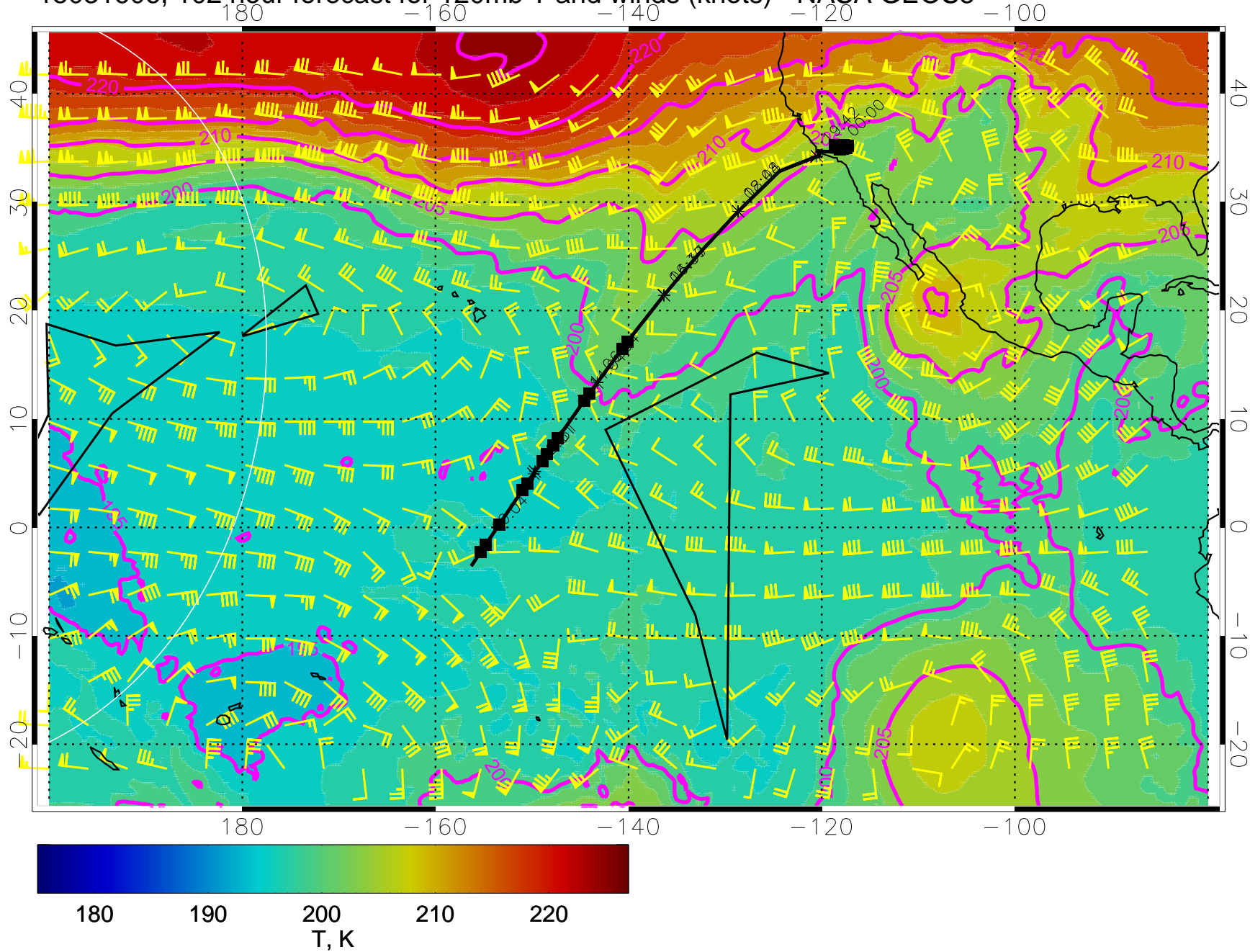
15031606, 102 hour forecast for 120mb T and winds (knots) - NASA GEOS5
