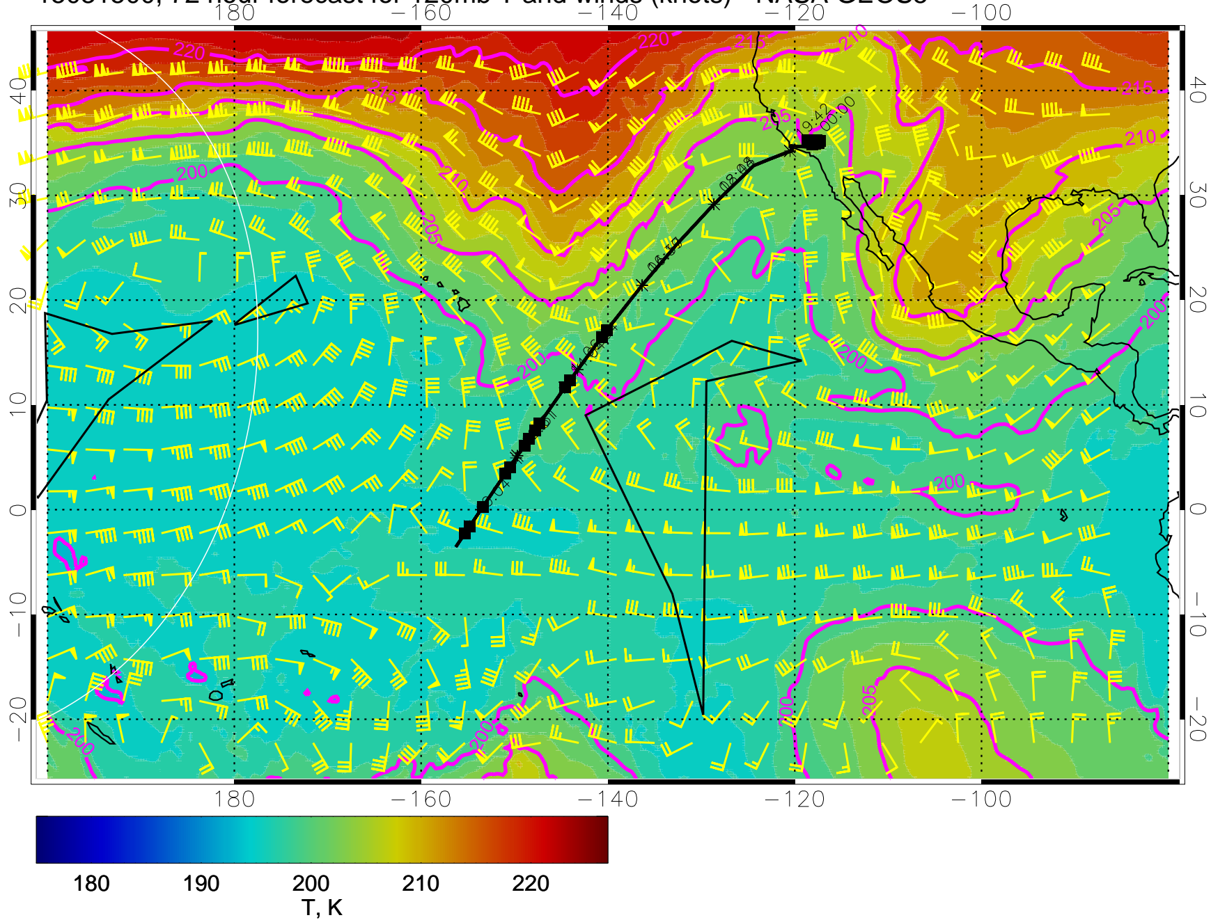
15031500, 72 hour forecast for 120mb T and winds (knots) - NASA GEOS5
