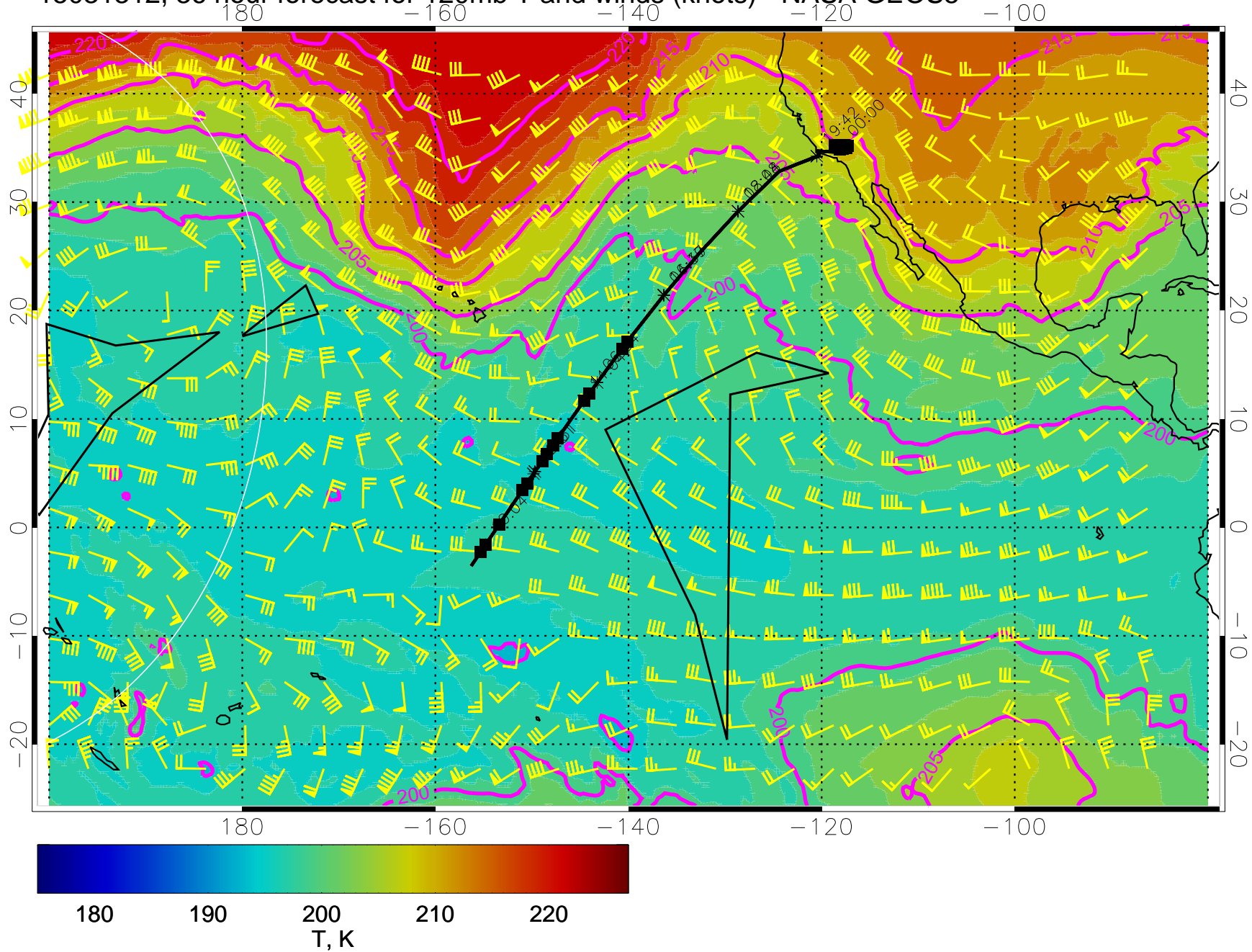
15031312, 36 hour forecast for 120mb T and winds (knots) - NASA GEOS5
