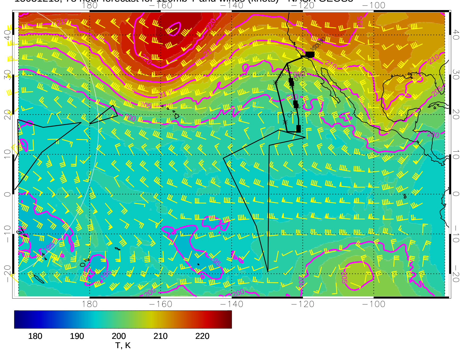
15031218, 78 hour forecast for 120mb T and winds (knots) - NASA GEOS5
