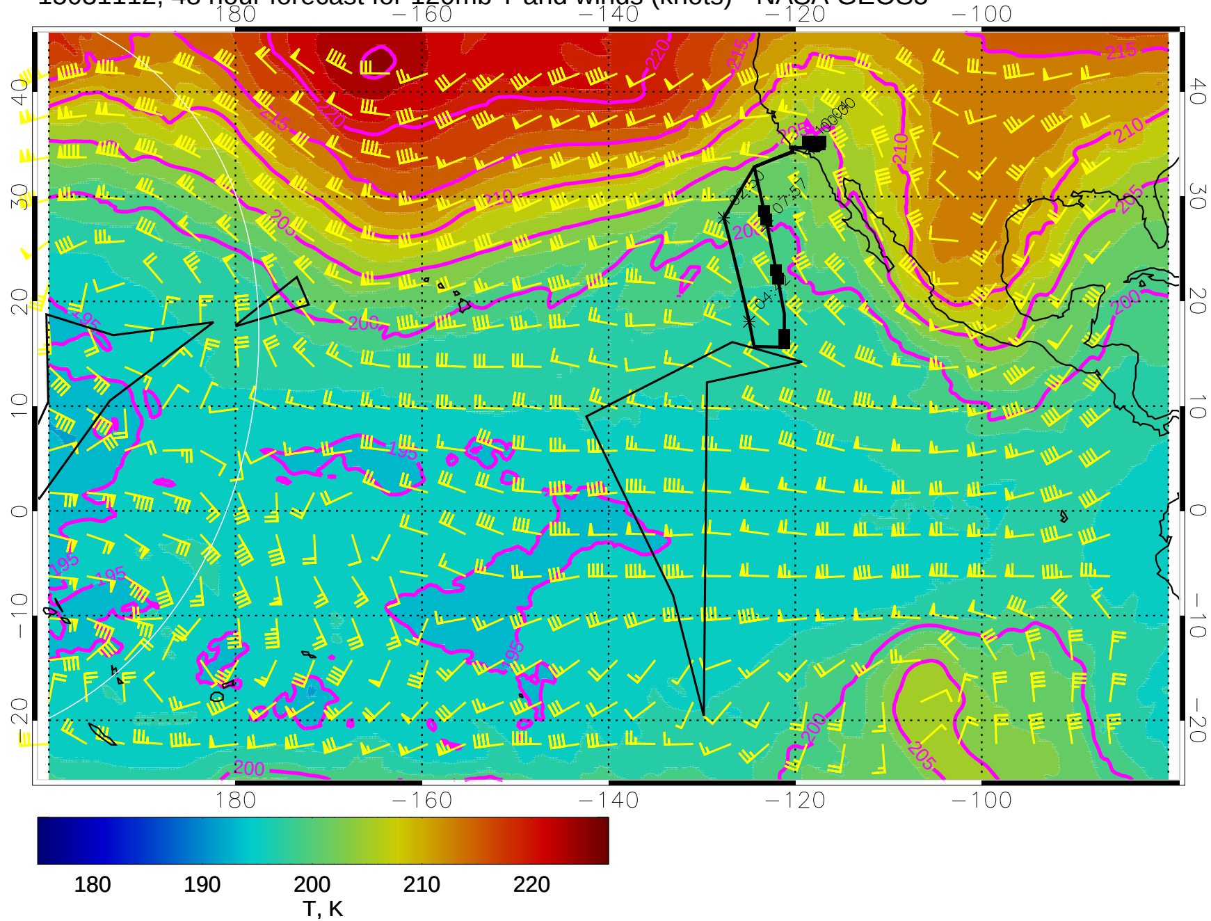
15031112, 48 hour forecast for 120mb T and winds (knots) - NASA GEOS5
