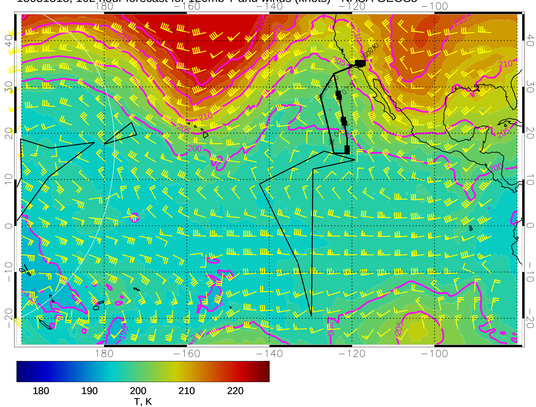
15031318, 102 hour forecast for 120mb T and winds (knots) - NASA GEOS5
