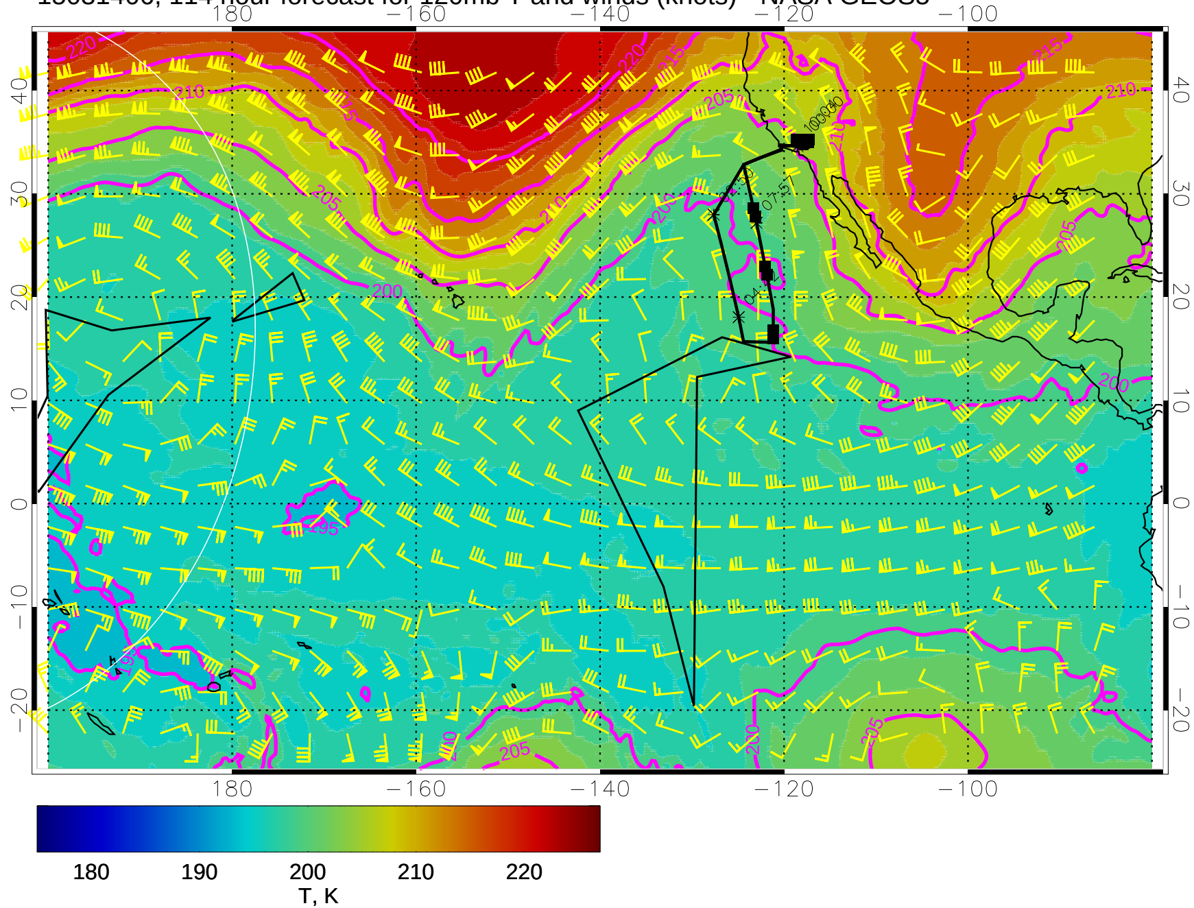
15031406, 114 hour forecast for 120mb T and winds (knots) - NASA GEOS5
