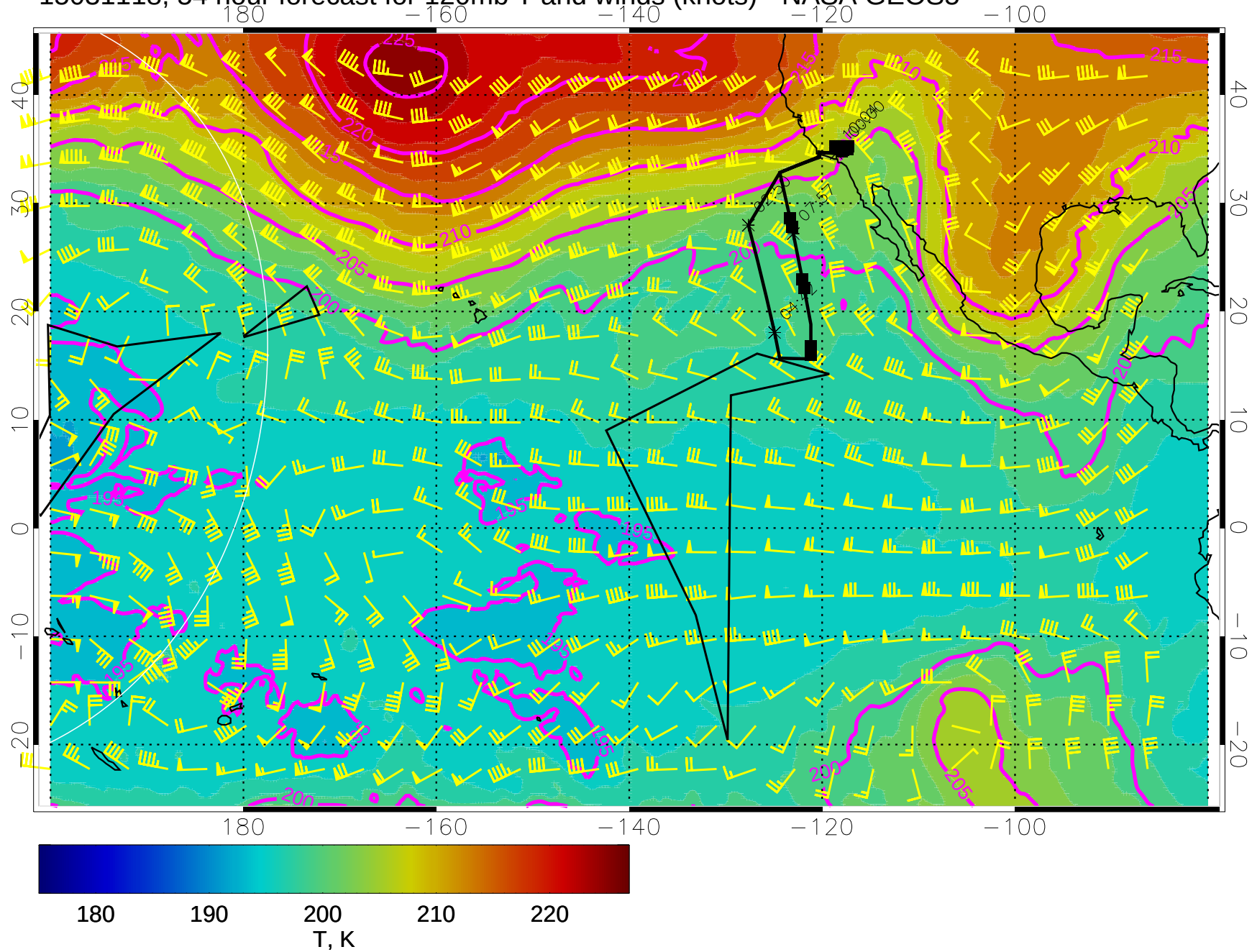
15031118, 54 hour forecast for 120mb T and winds (knots) - NASA GEOS5
