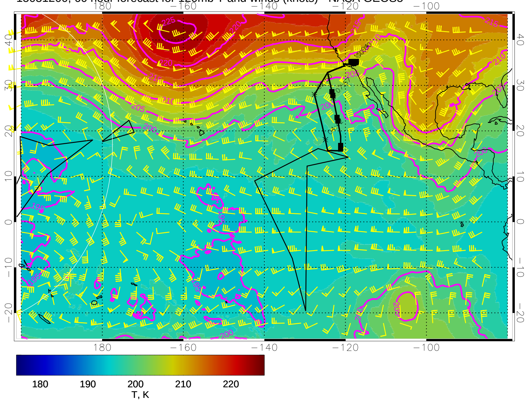
15031200, 60 hour forecast for 120mb T and winds (knots) - NASA GEOS5
