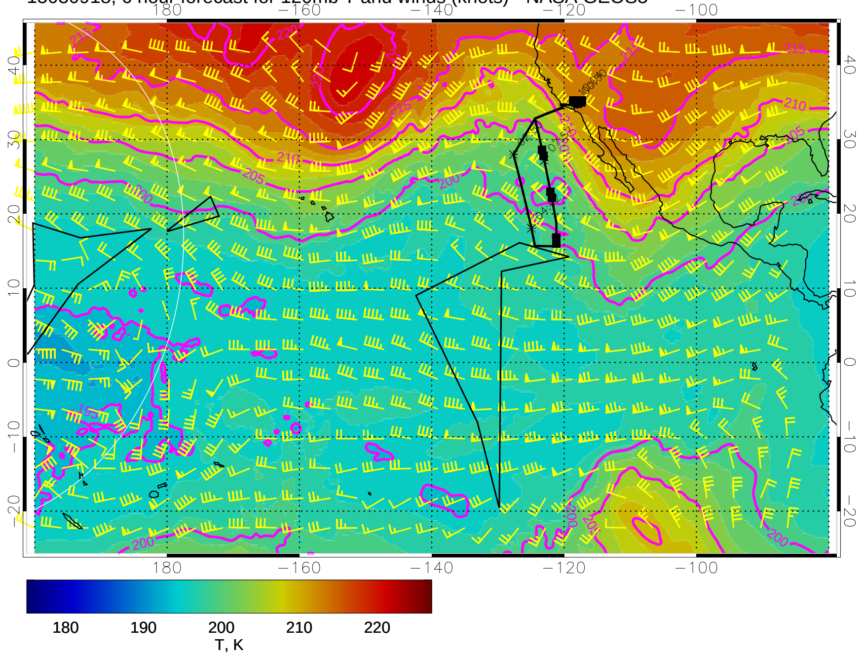
15030918, 6 hour forecast for 120mb T and winds (knots) - NASA GEOS5
