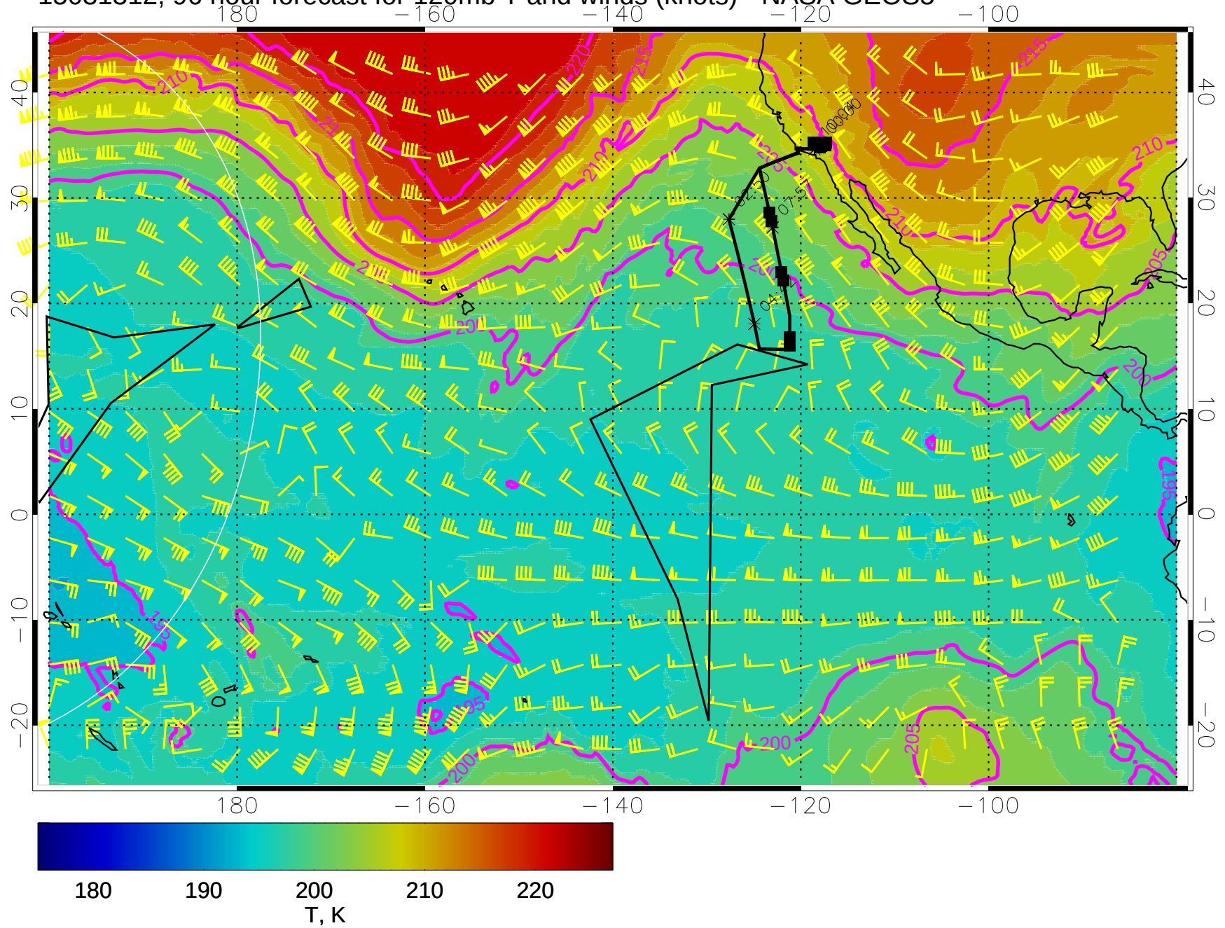
15031312, 96 hour forecast for 120mb T and winds (knots) - NASA GEOS5
