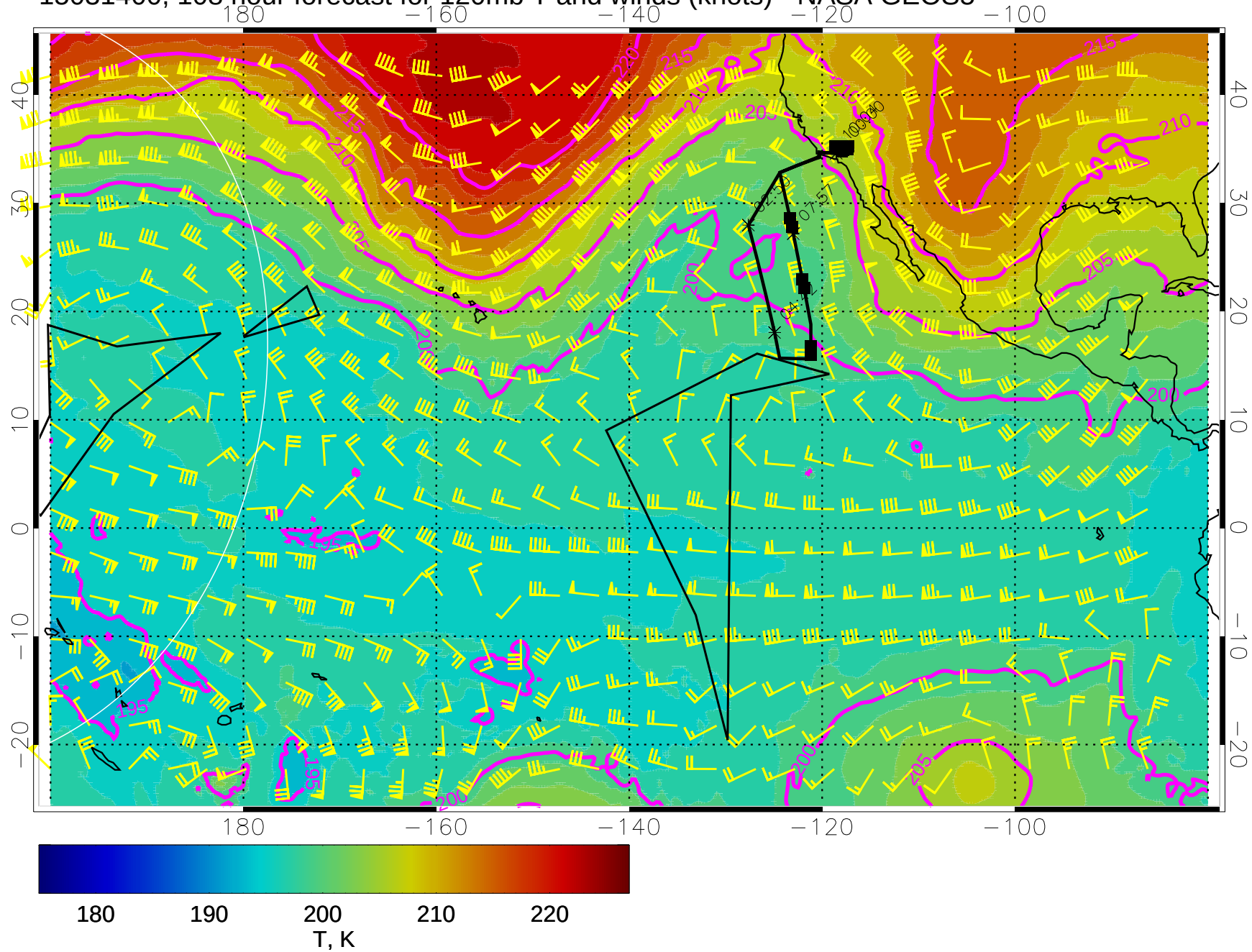
15031400, 108 hour forecast for 120mb T and winds (knots) - NASA GEOS5
