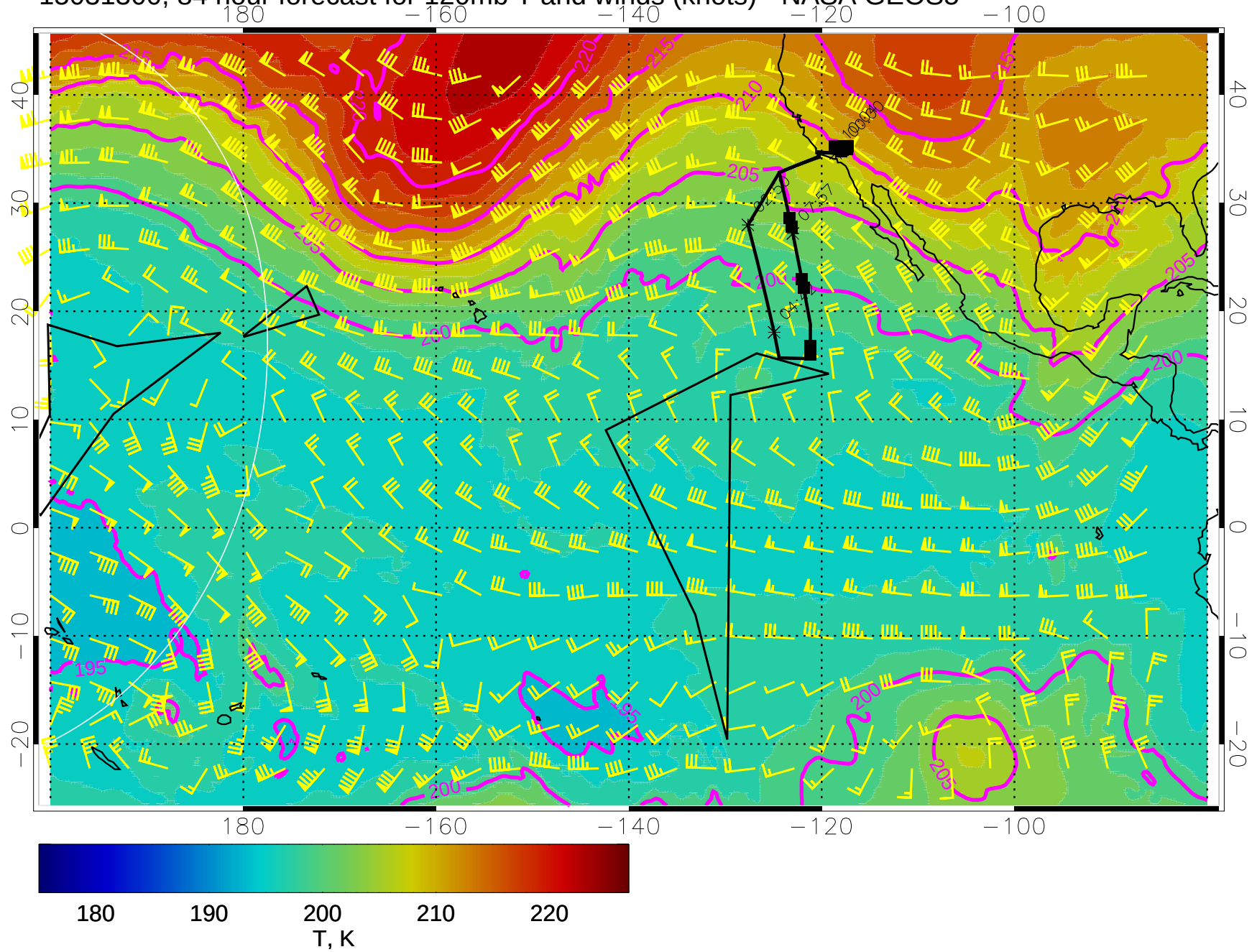
15031300, 84 hour forecast for 120mb T and winds (knots) - NASA GEOS5
