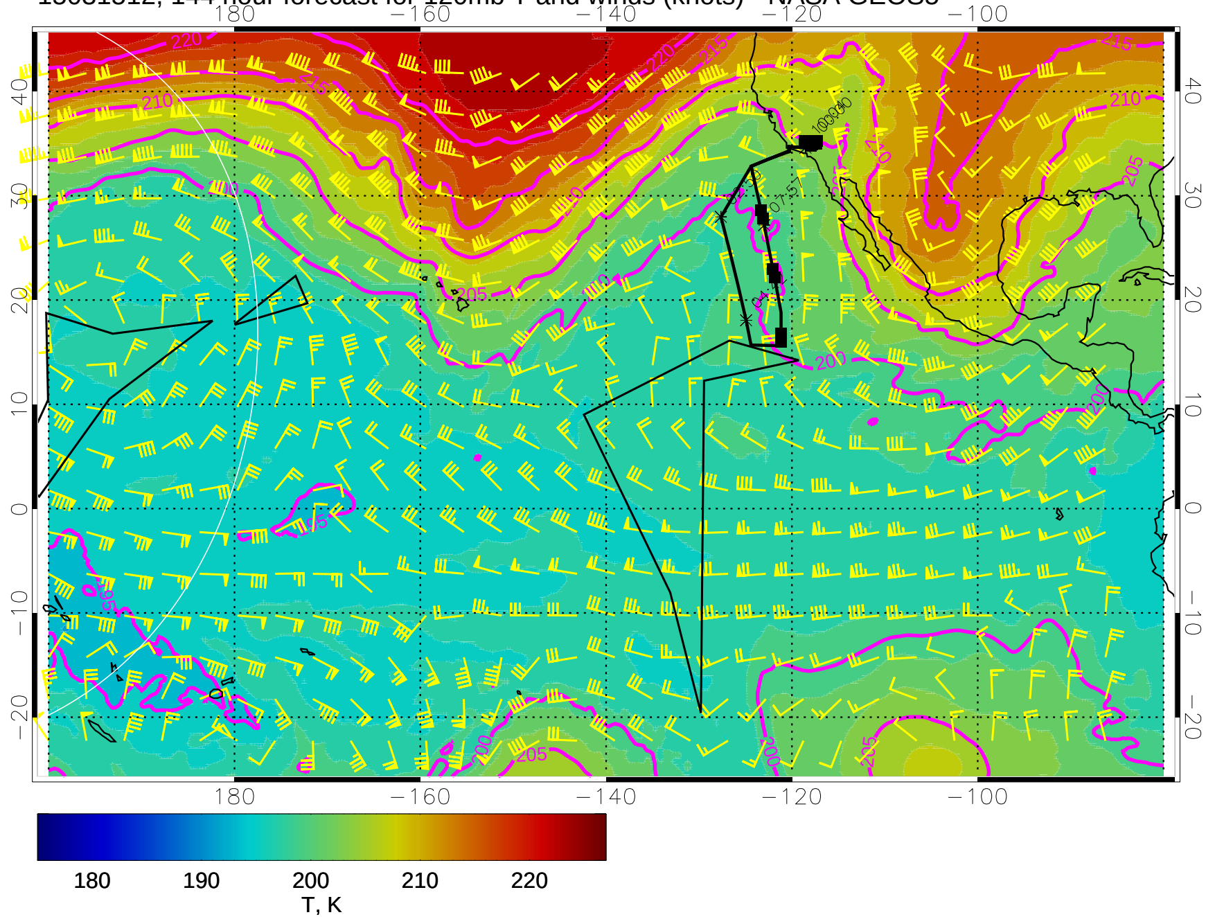
15031512, 144 hour forecast for 120mb T and winds (knots) - NASA GEOS5
