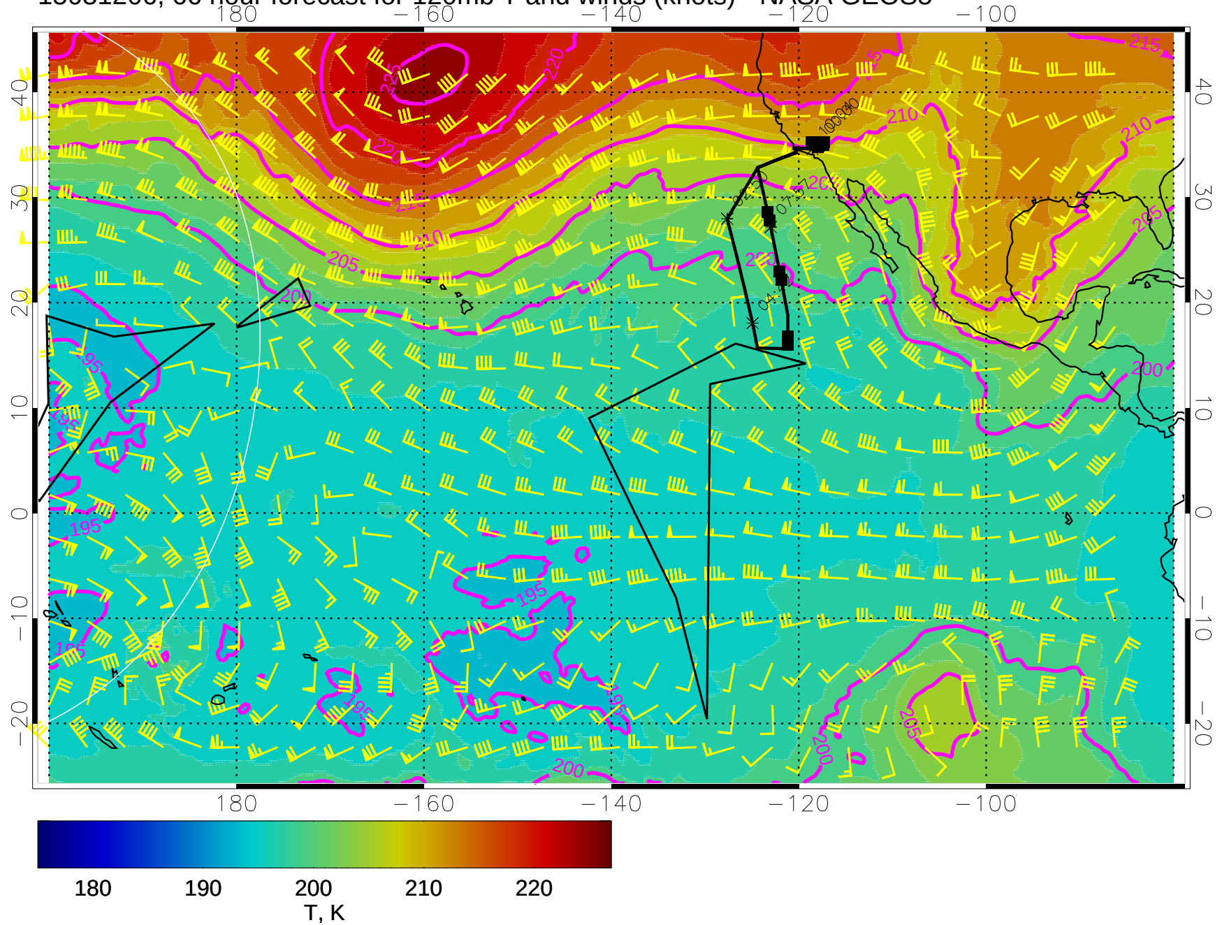
15031206, 66 hour forecast for 120mb T and winds (knots) - NASA GEOS5
