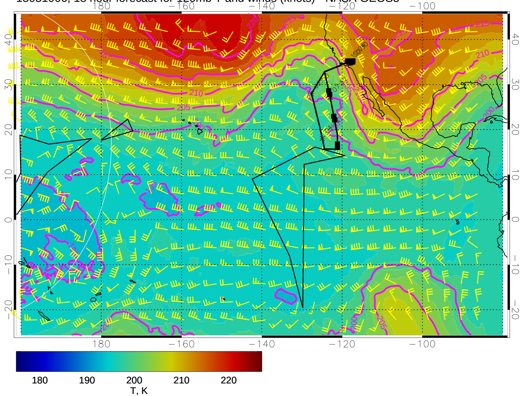
15031006, 18 hour forecast for 120mb T and winds (knots) - NASA GEOS5
