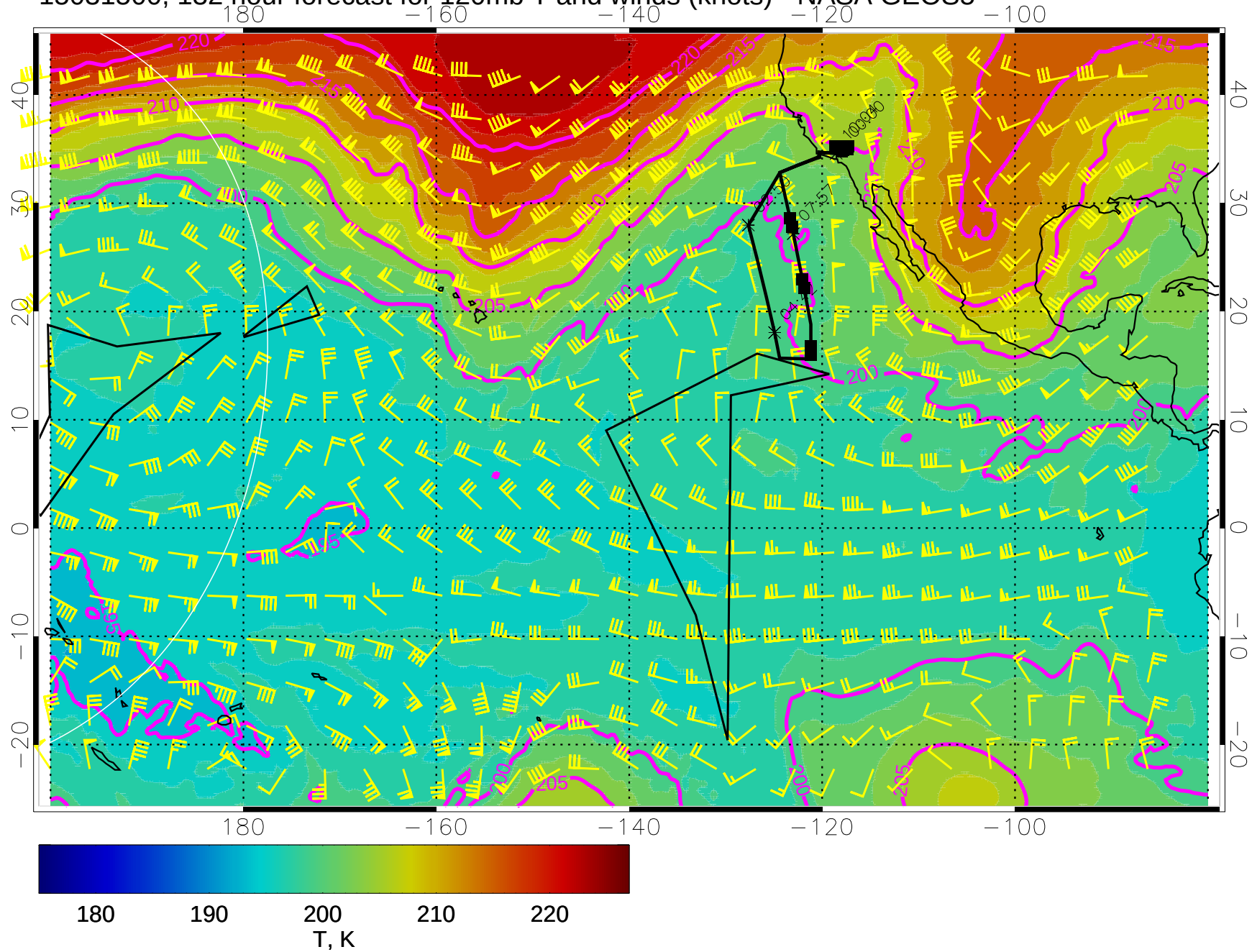
15031500, 132 hour forecast for 120mb T and winds (knots) - NASA GEOS5
