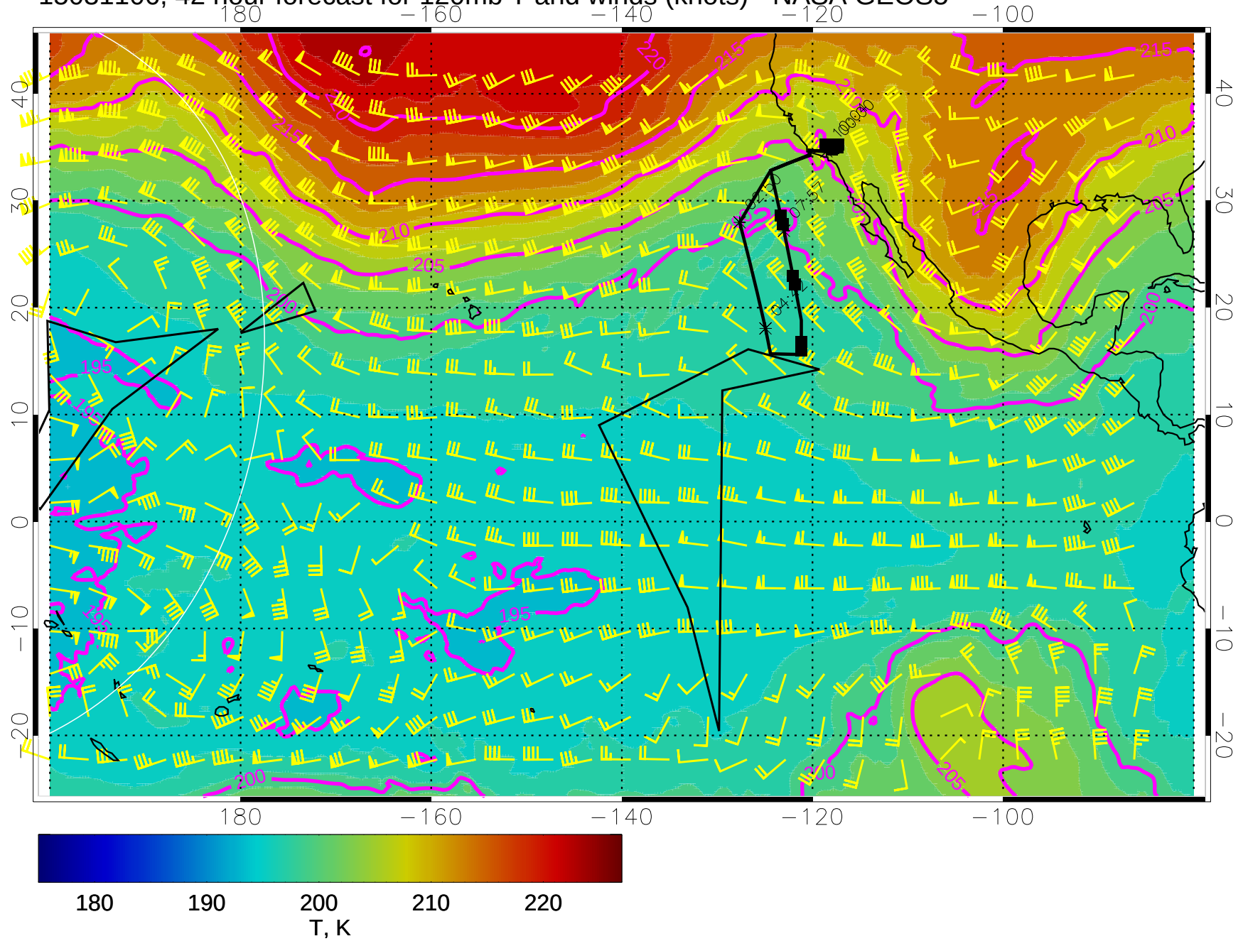
15031106, 42 hour forecast for 120mb T and winds (knots) - NASA GEOS5
