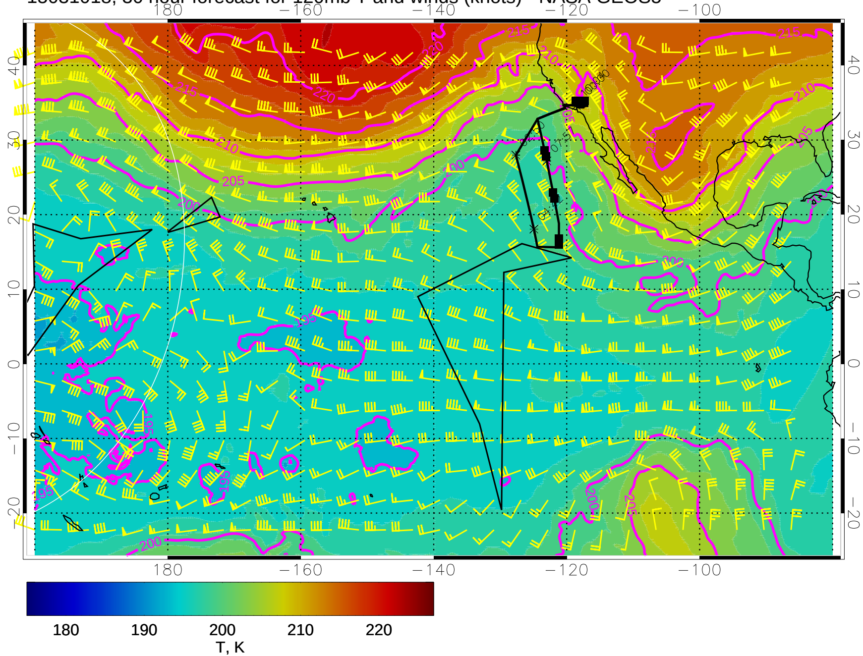
15031018, 30 hour forecast for 120mb T and winds (knots) - NASA GEOS5
