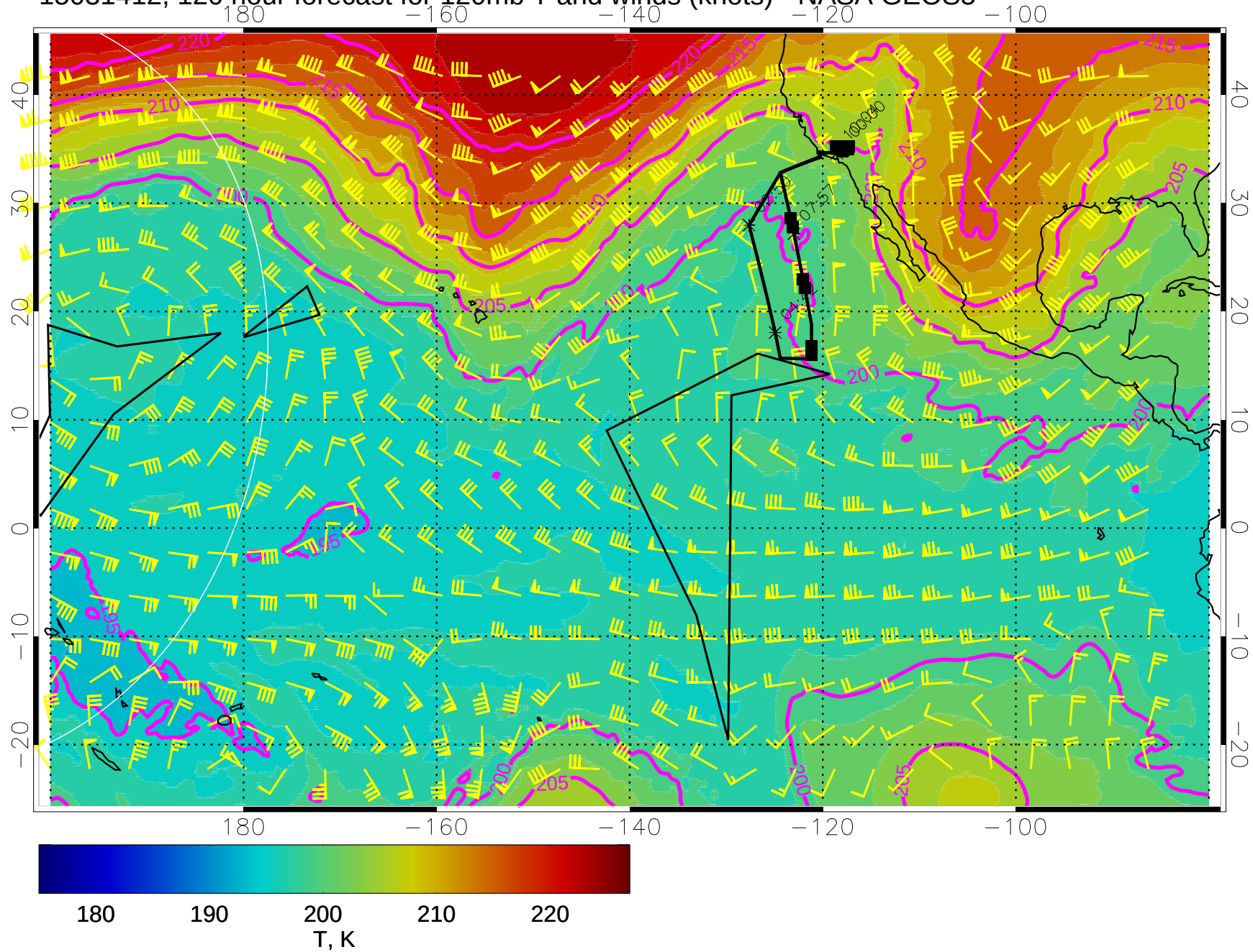
15031412, 120 hour forecast for 120mb T and winds (knots) - NASA GEOS5
