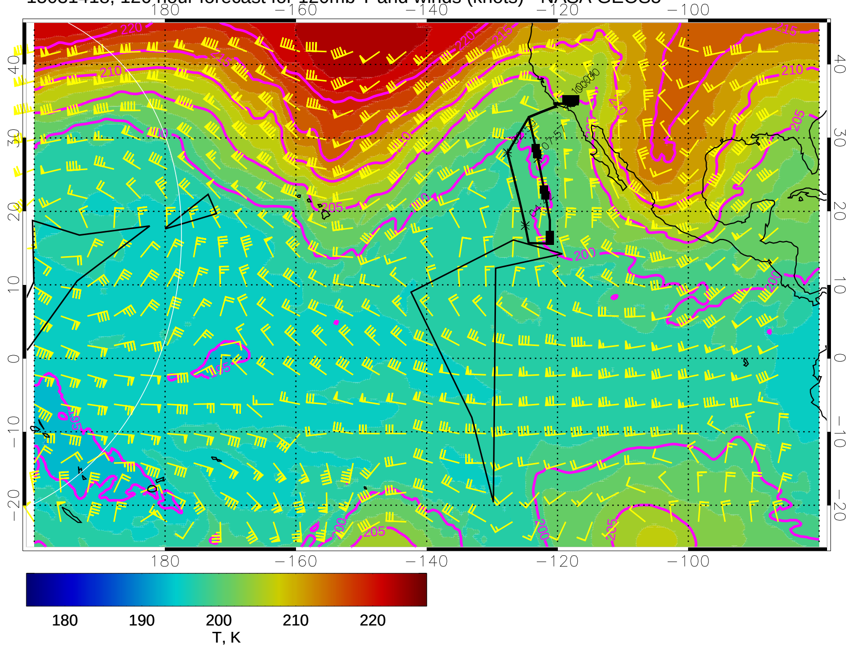
15031418, 126 hour forecast for 120mb T and winds (knots) - NASA GEOS5
