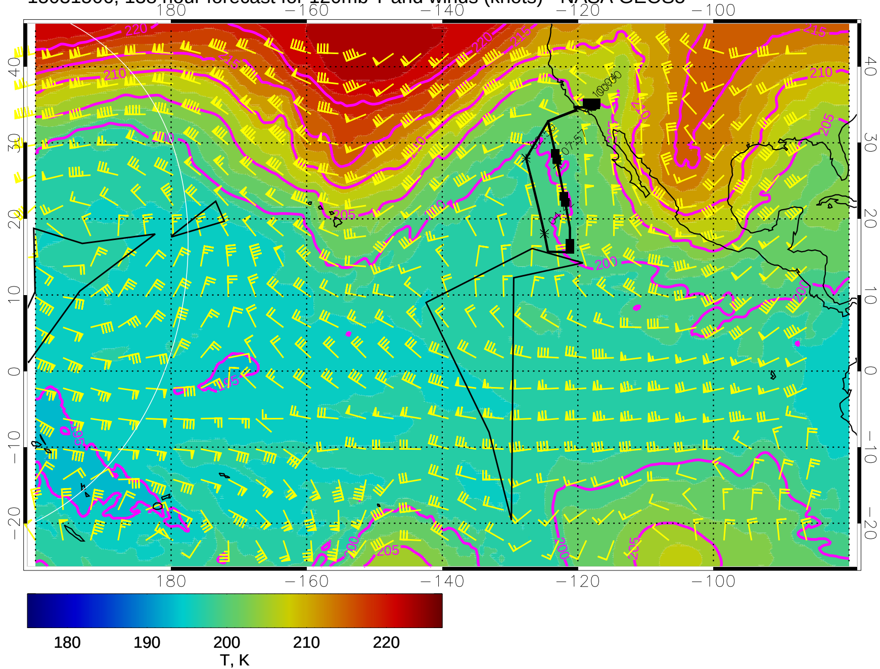
15031506, 138 hour forecast for 120mb T and winds (knots) - NASA GEOS5
