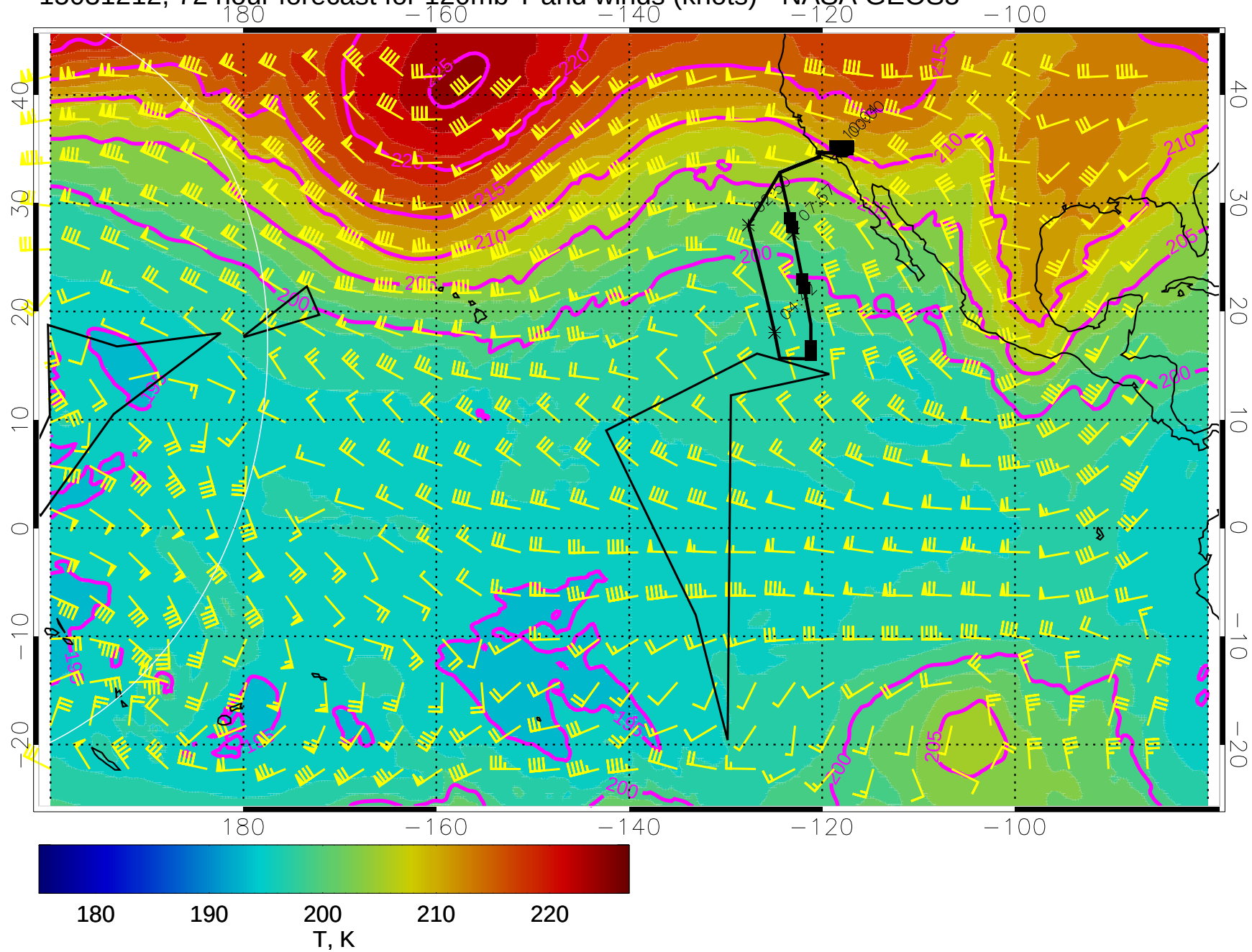
15031212, 72 hour forecast for 120mb T and winds (knots) - NASA GEOS5
