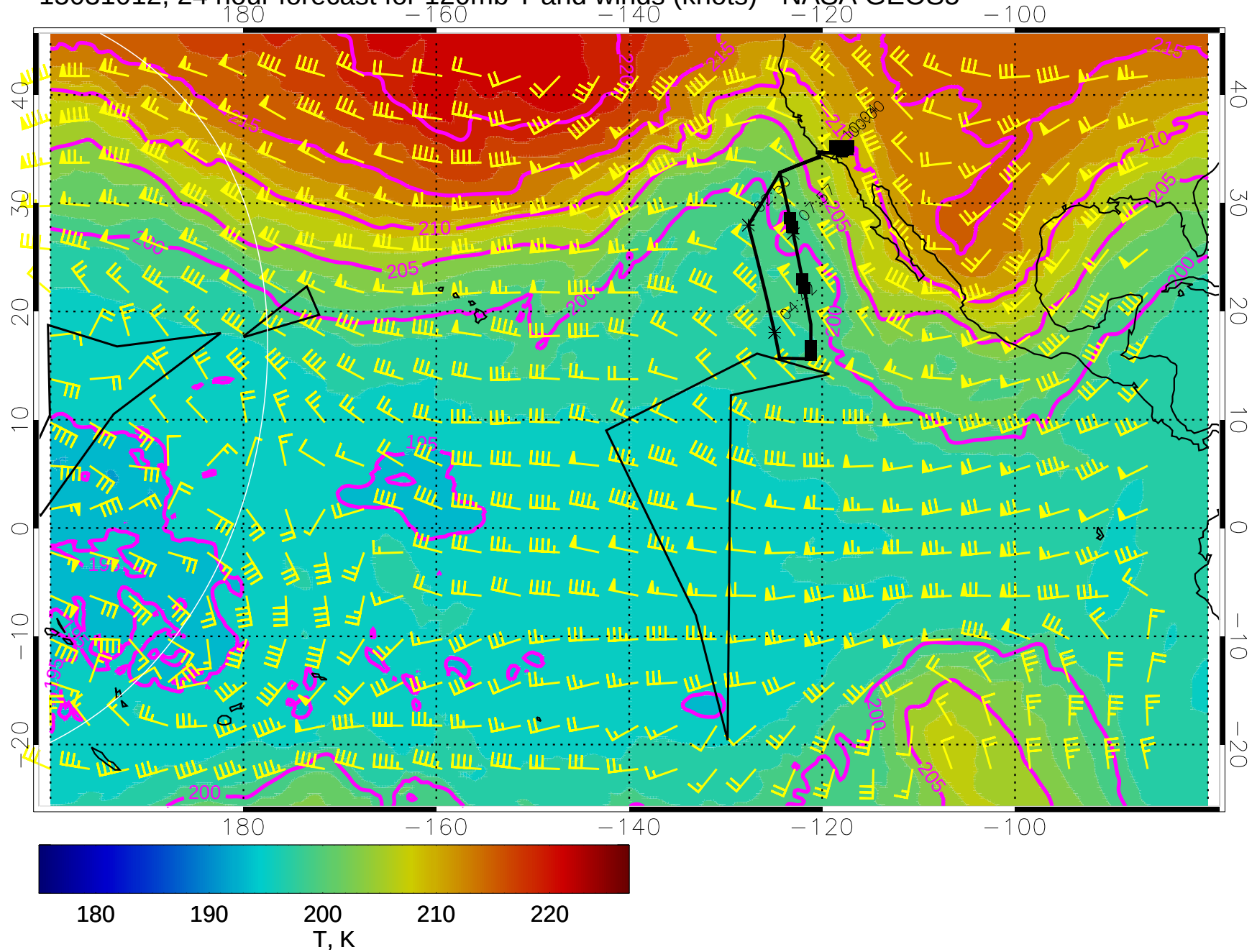
15031012, 24 hour forecast for 120mb T and winds (knots) - NASA GEOS5
