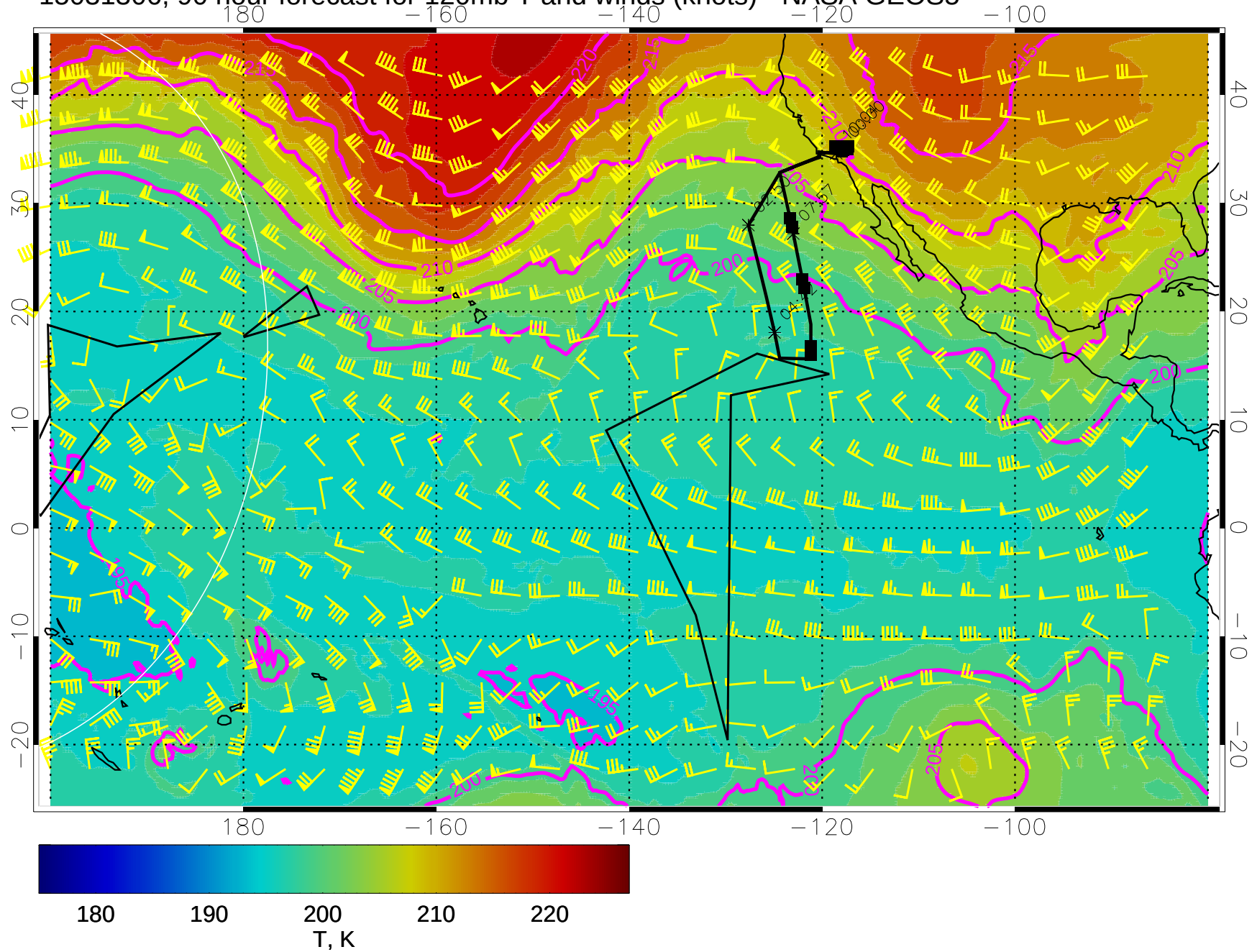
15031306, 90 hour forecast for 120mb T and winds (knots) - NASA GEOS5
