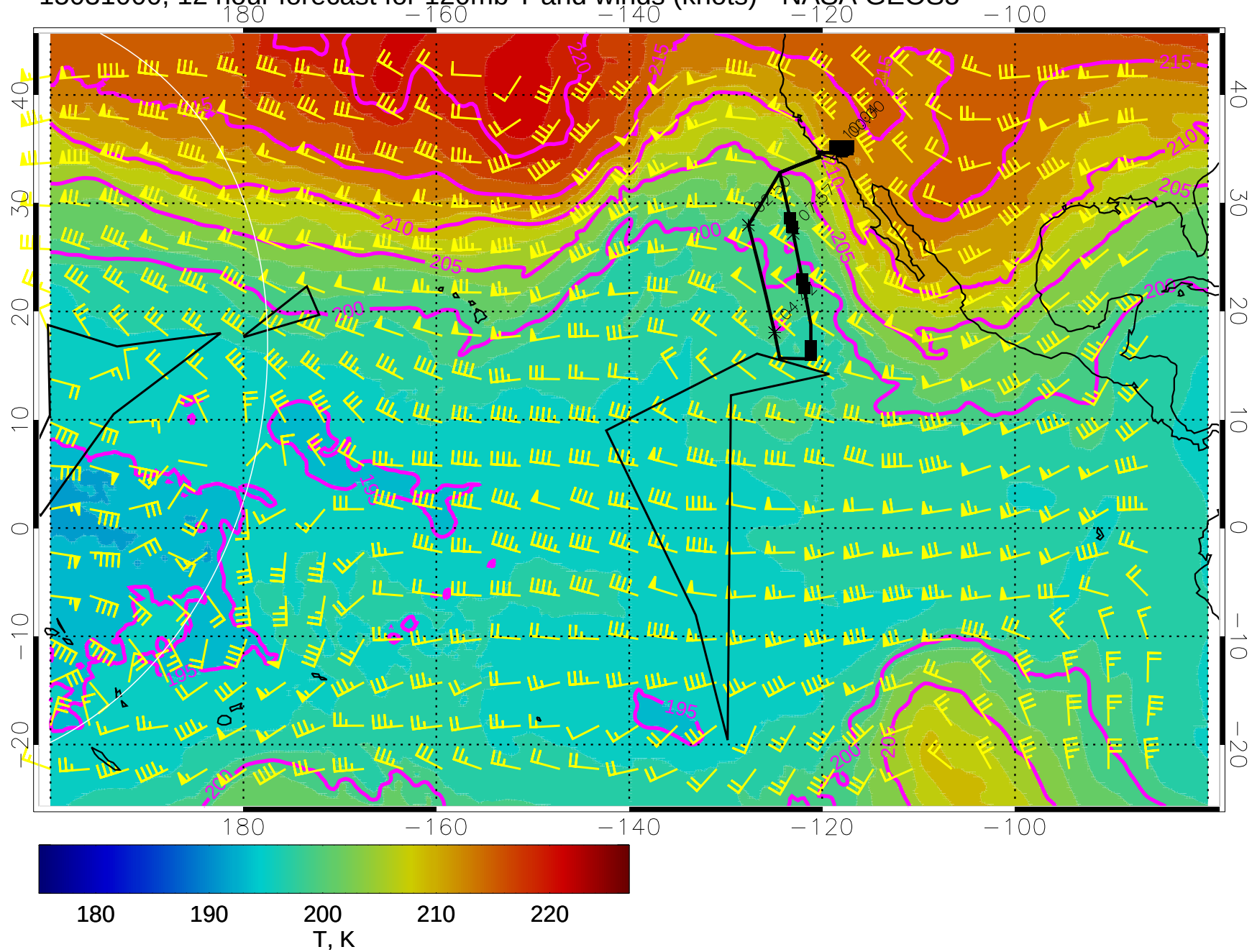
15031000, 12 hour forecast for 120mb T and winds (knots) - NASA GEOS5
