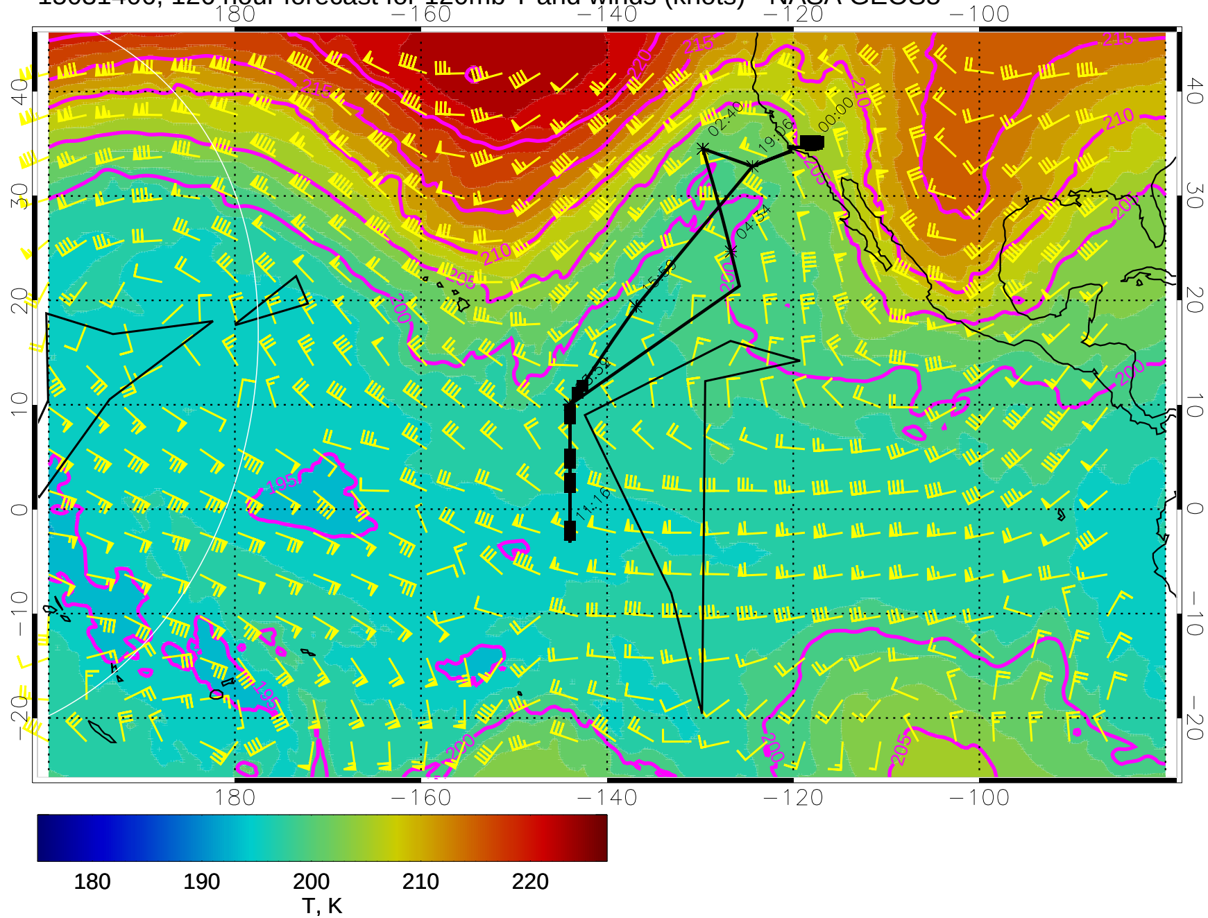
15031406, 126 hour forecast for 120mb T and winds (knots) - NASA GEOS5
