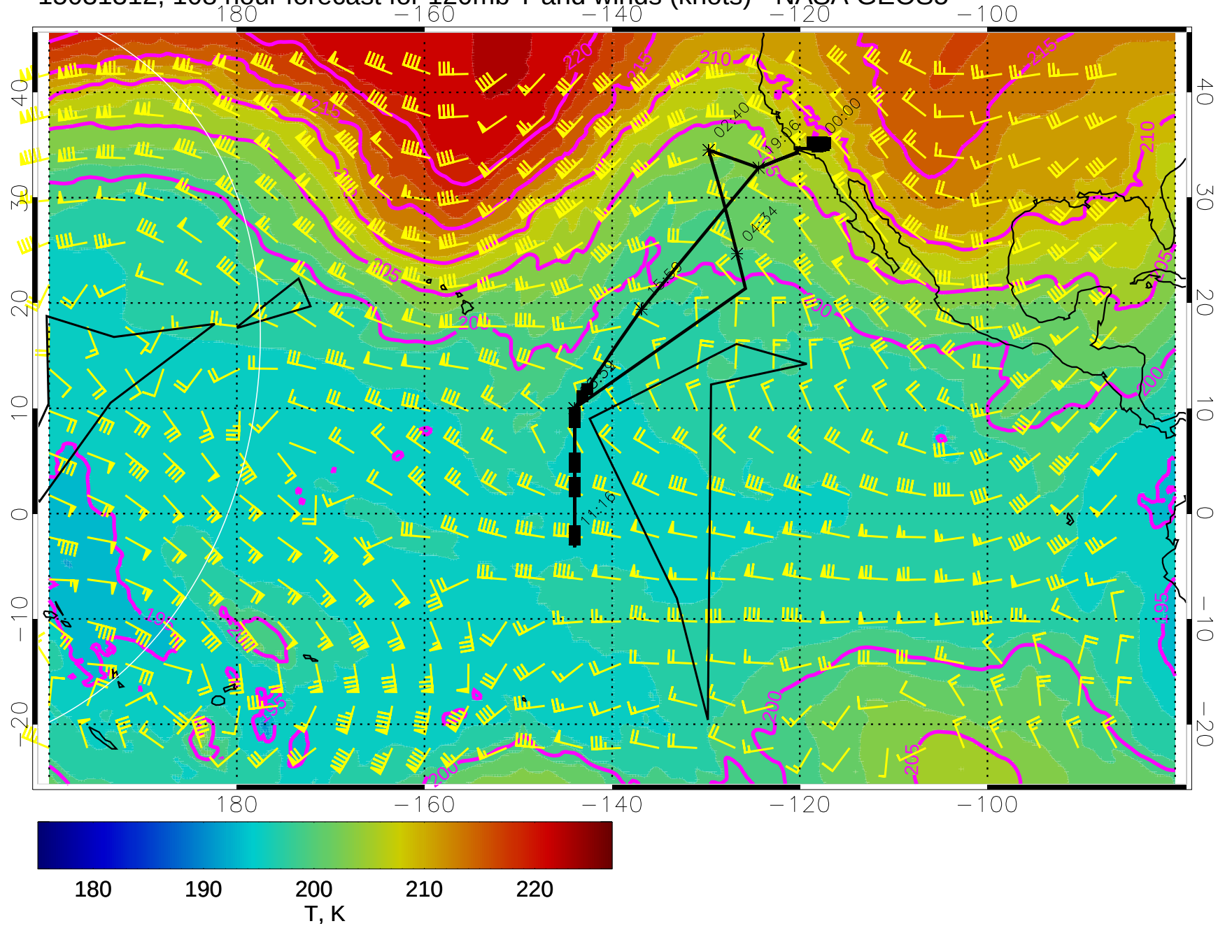
15031312, 108 hour forecast for 120mb T and winds (knots) - NASA GEOS5
