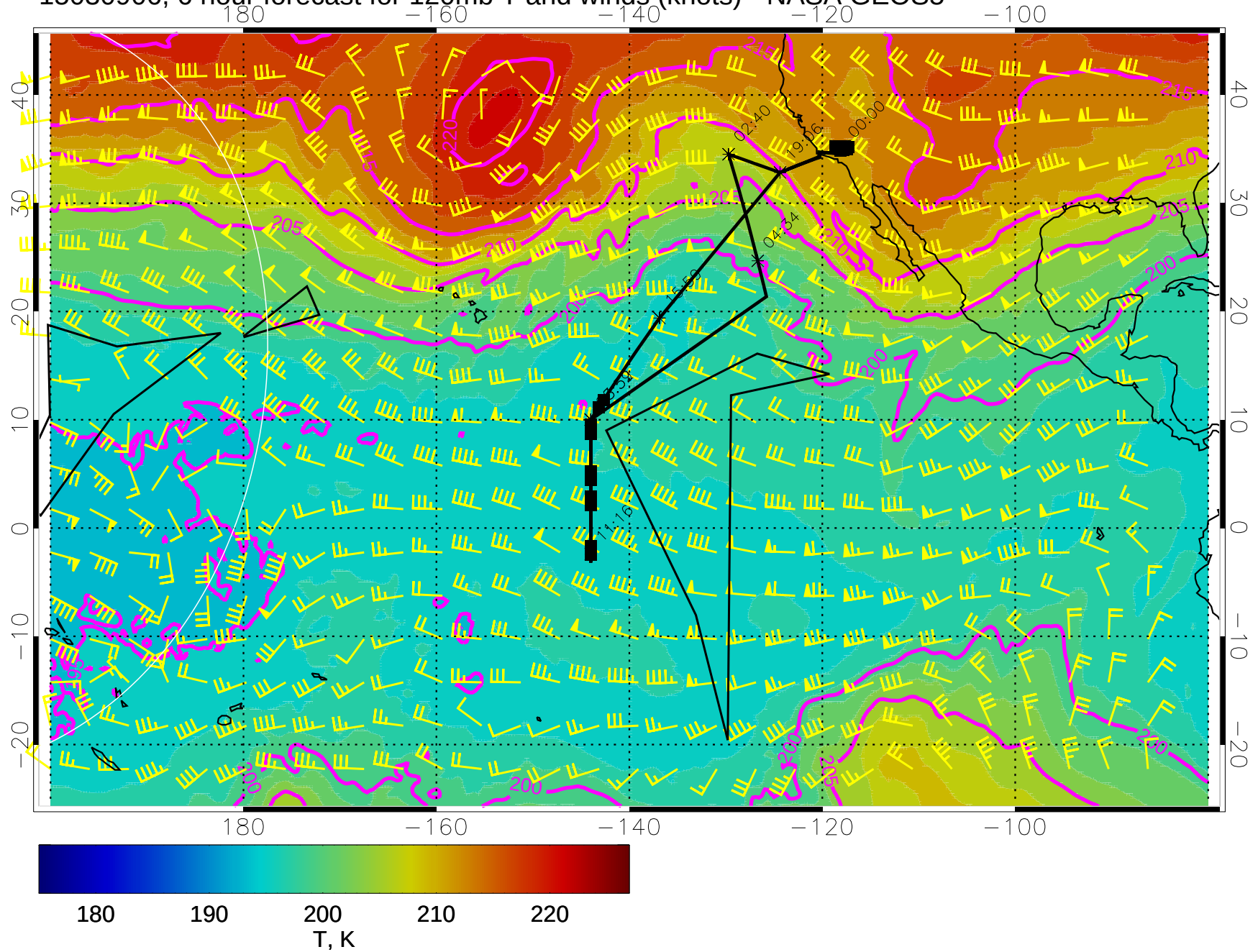
15030906, 6 hour forecast for 120mb T and winds (knots) - NASA GEOS5
