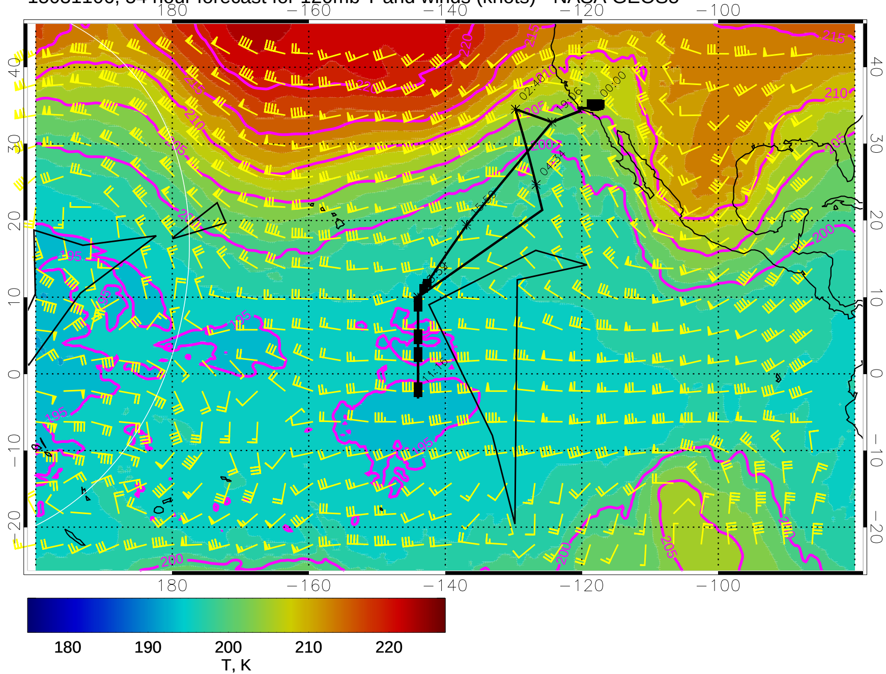
15031106, 54 hour forecast for 120mb T and winds (knots) - NASA GEOS5
