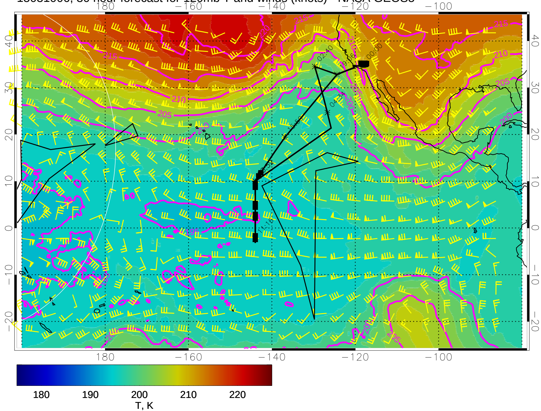
15031006, 30 hour forecast for 120mb T and winds (knots) - NASA GEOS5
