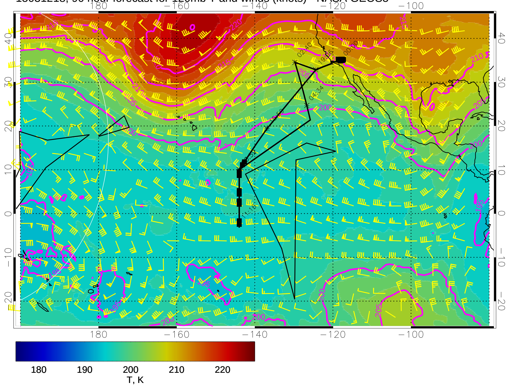
15031218, 90 hour forecast for 120mb T and winds (knots) - NASA GEOS5
