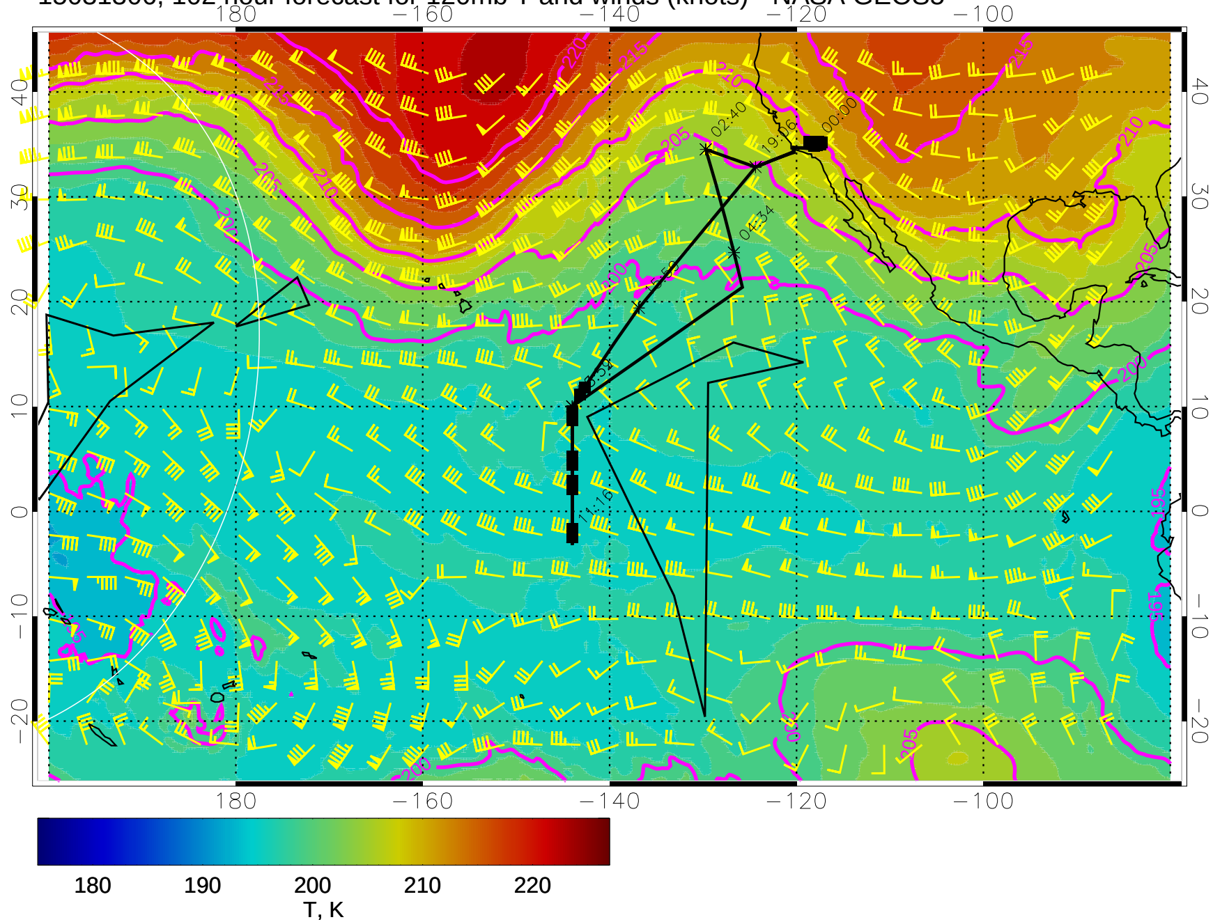
15031306, 102 hour forecast for 120mb T and winds (knots) - NASA GEOS5
