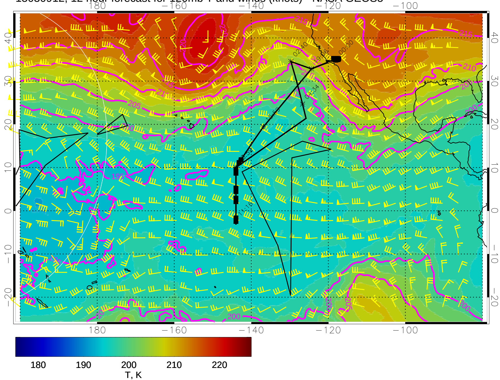
15030912, 12 hour forecast for 120mb T and winds (knots) - NASA GEOS5
