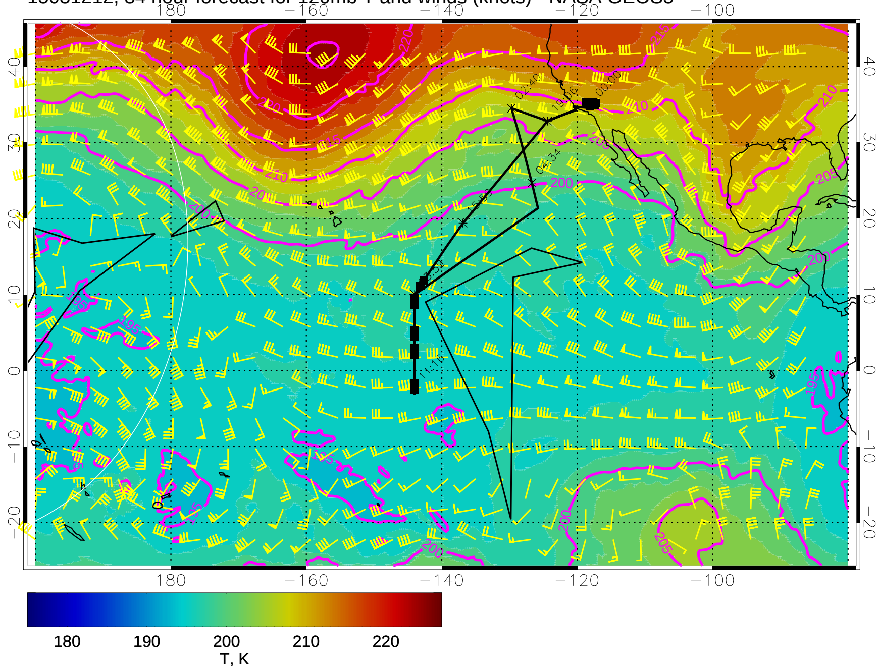
15031212, 84 hour forecast for 120mb T and winds (knots) - NASA GEOS5
