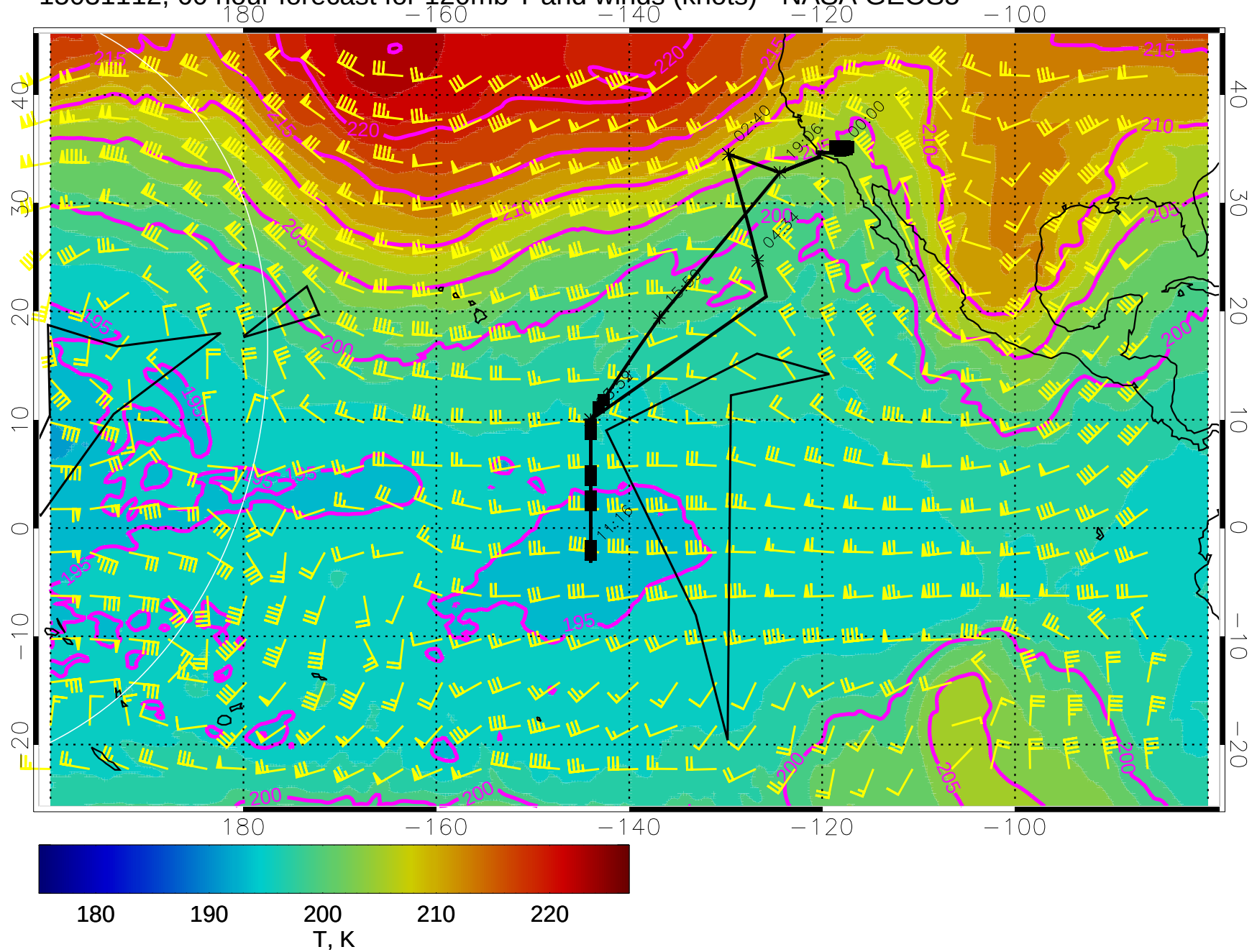
15031112, 60 hour forecast for 120mb T and winds (knots) - NASA GEOS5
