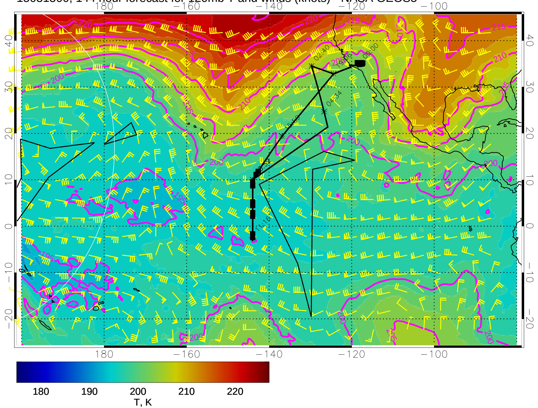
15031500, 144 hour forecast for 120mb T and winds (knots) - NASA GEOS5
