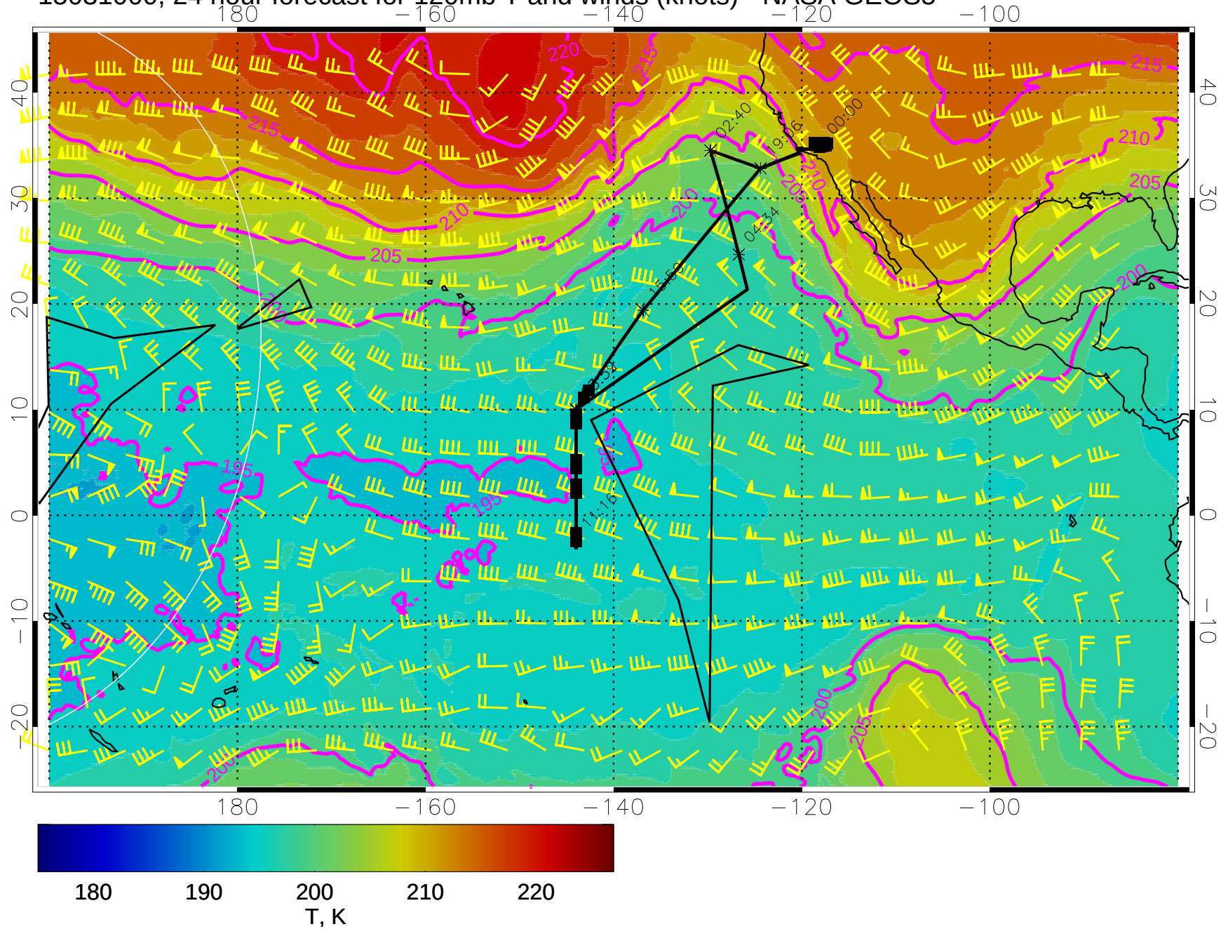
15031000, 24 hour forecast for 120mb T and winds (knots) - NASA GEOS5
