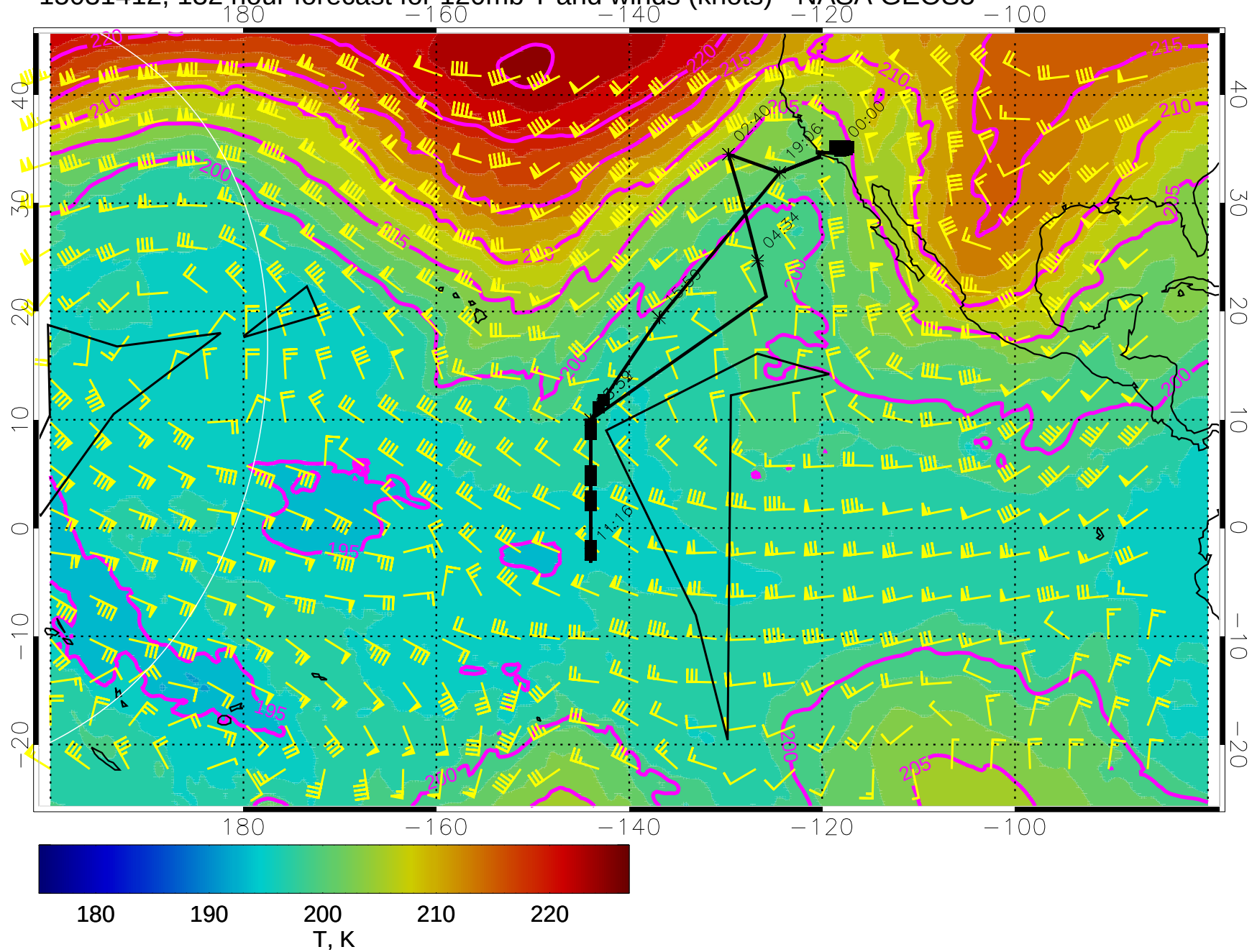
15031412, 132 hour forecast for 120mb T and winds (knots) - NASA GEOS5
