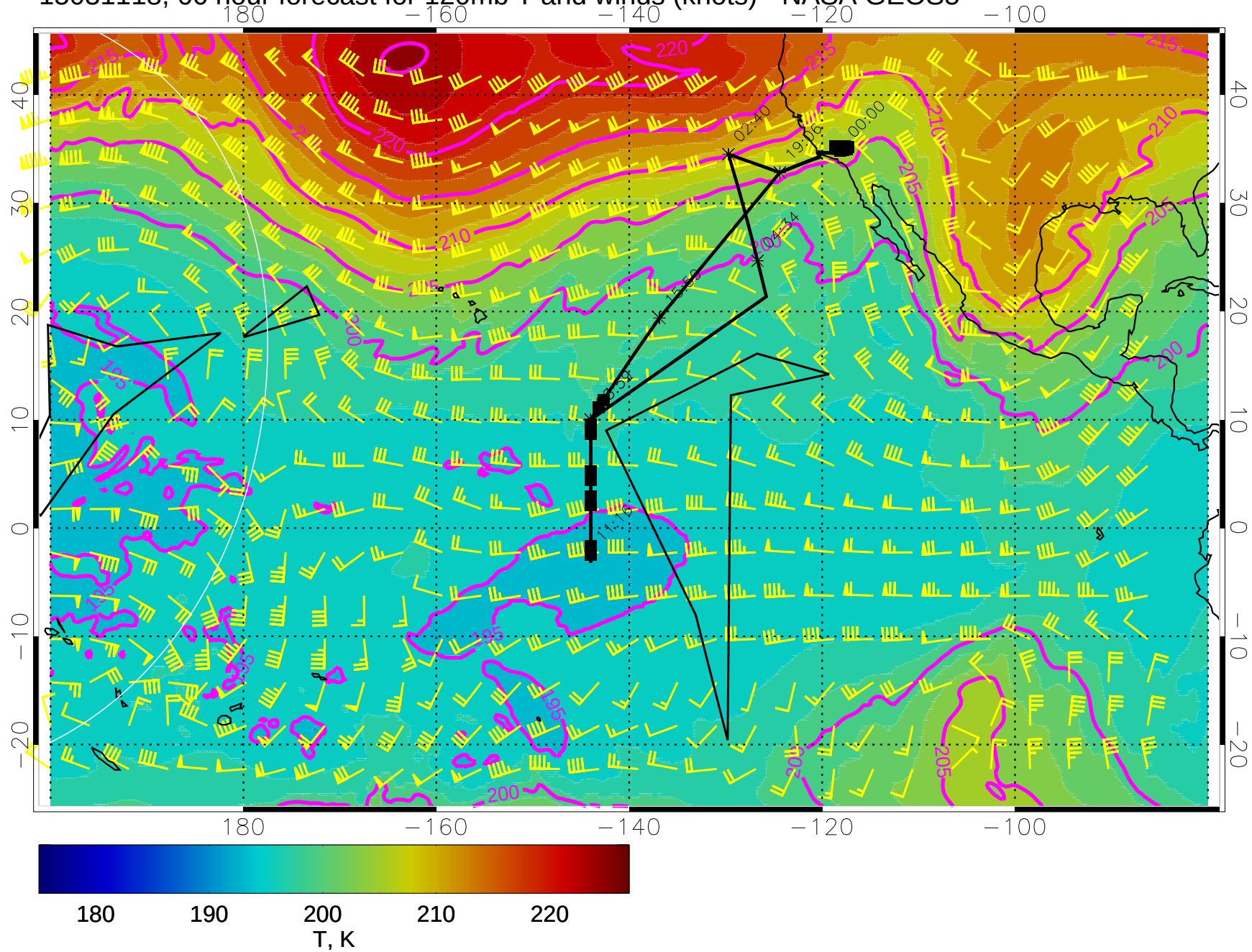
15031118, 66 hour forecast for 120mb T and winds (knots) - NASA GEOS5
