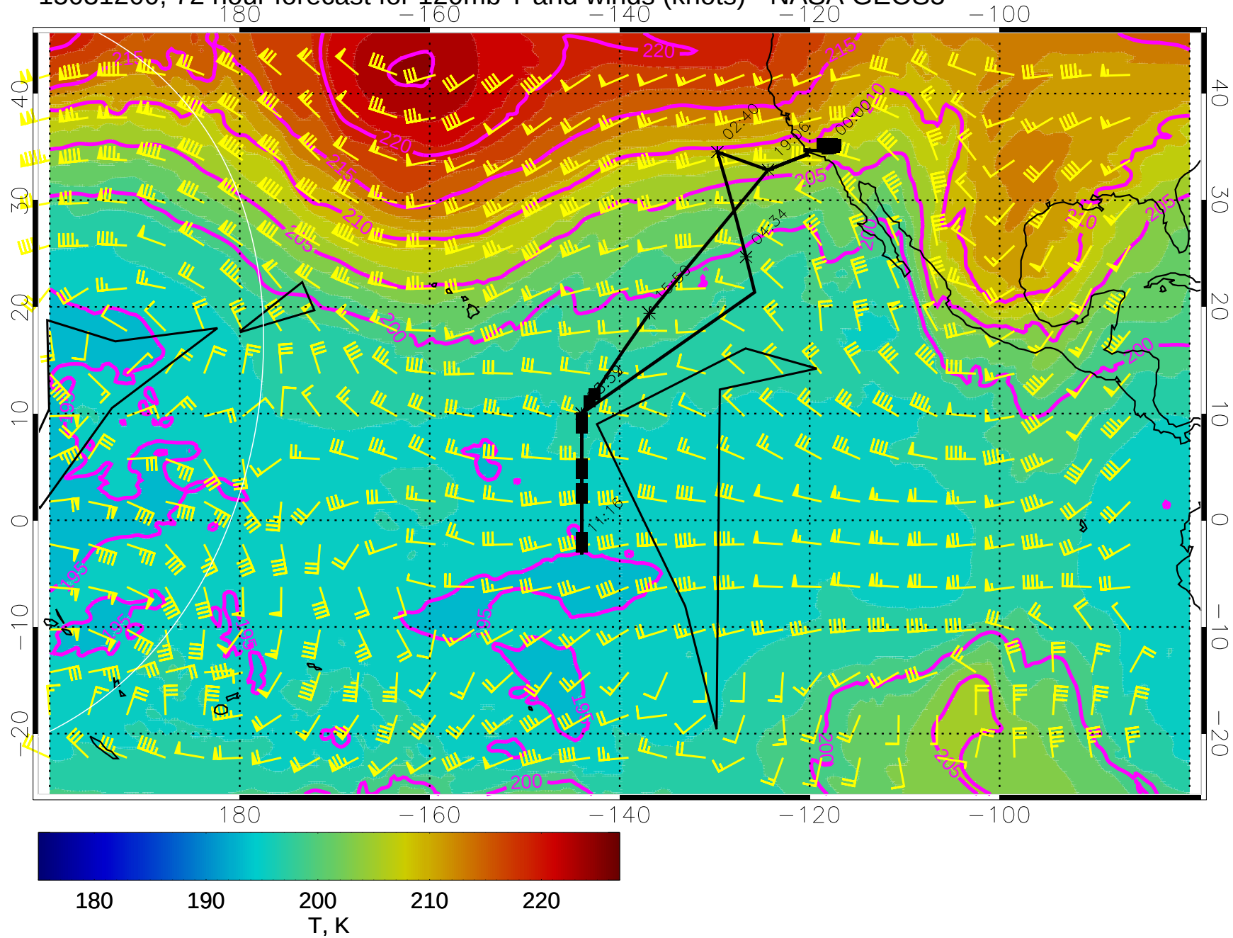
15031200, 72 hour forecast for 120mb T and winds (knots) - NASA GEOS5
