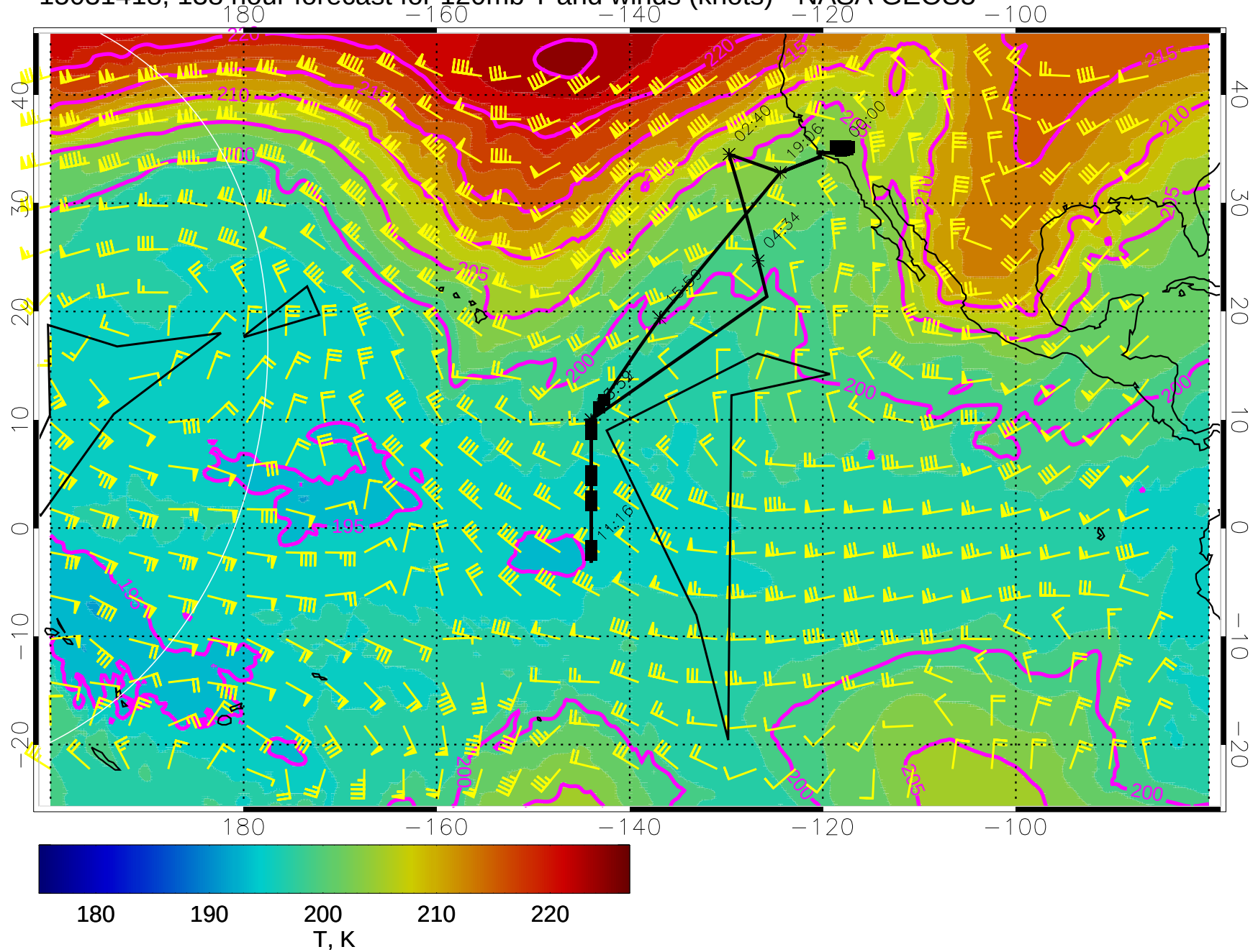
15031418, 138 hour forecast for 120mb T and winds (knots) - NASA GEOS5
