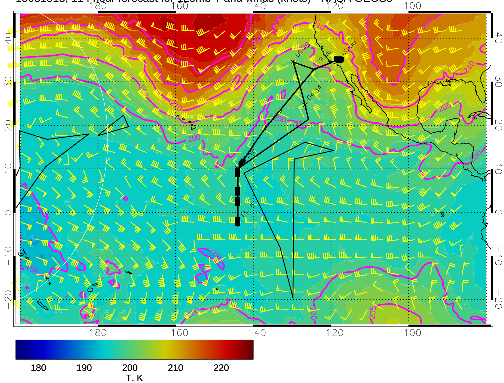
15031318, 114 hour forecast for 120mb T and winds (knots) - NASA GEOS5
