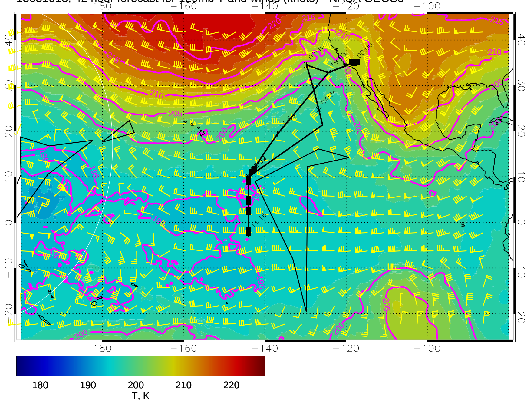
15031018, 42 hour forecast for 120mb T and winds (knots) - NASA GEOS5
