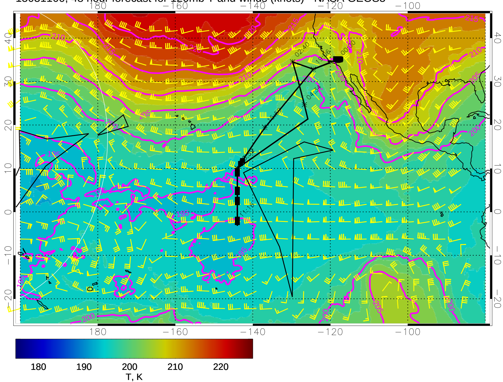
15031100, 48 hour forecast for 120mb T and winds (knots) - NASA GEOS5
