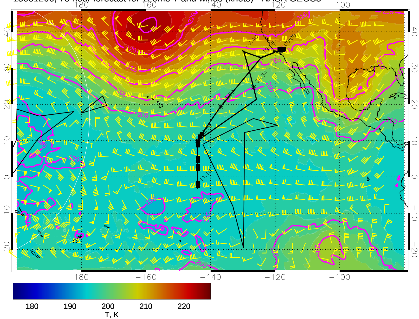
15031206, 78 hour forecast for 120mb T and winds (knots) - NASA GEOS5
