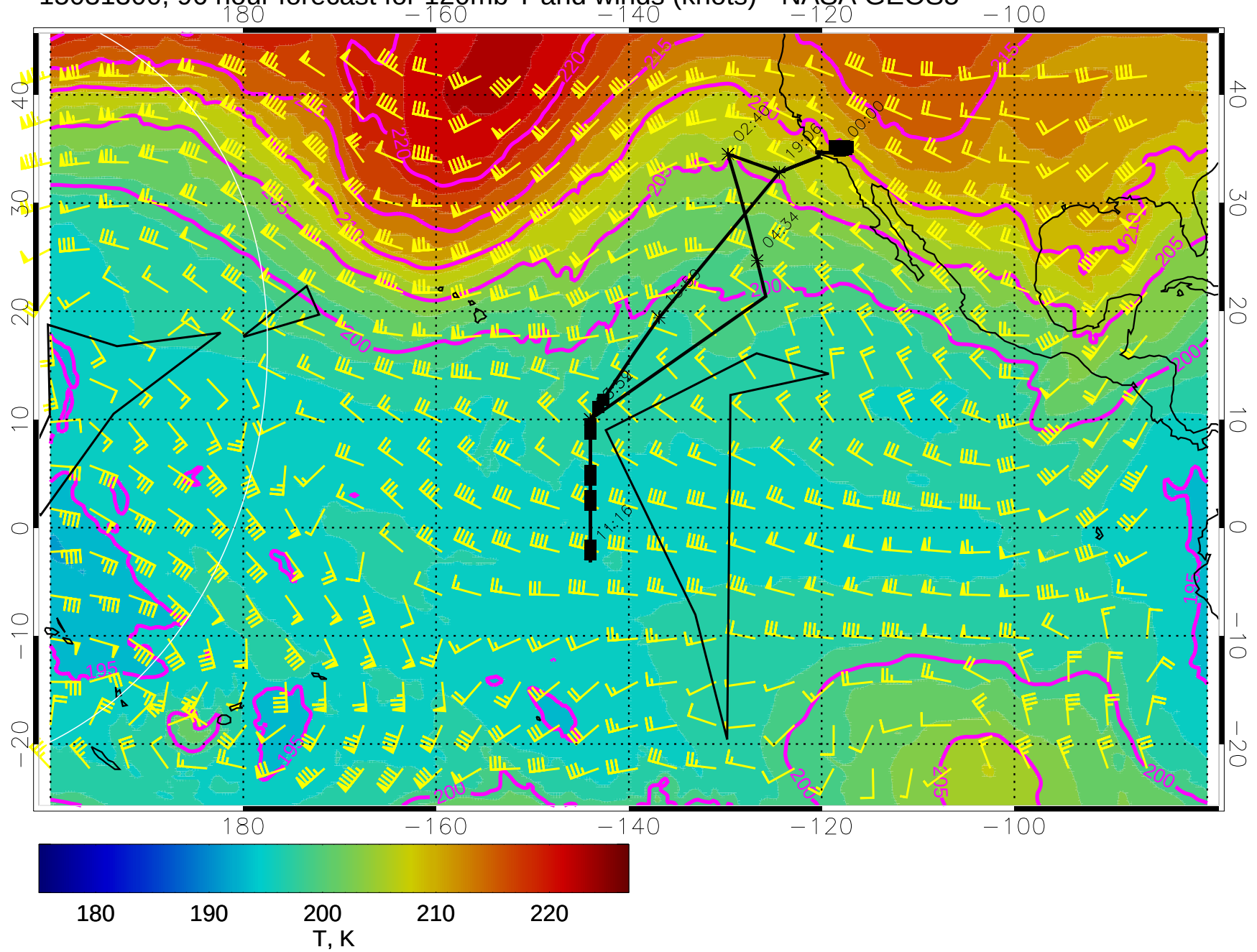
15031300, 96 hour forecast for 120mb T and winds (knots) - NASA GEOS5
