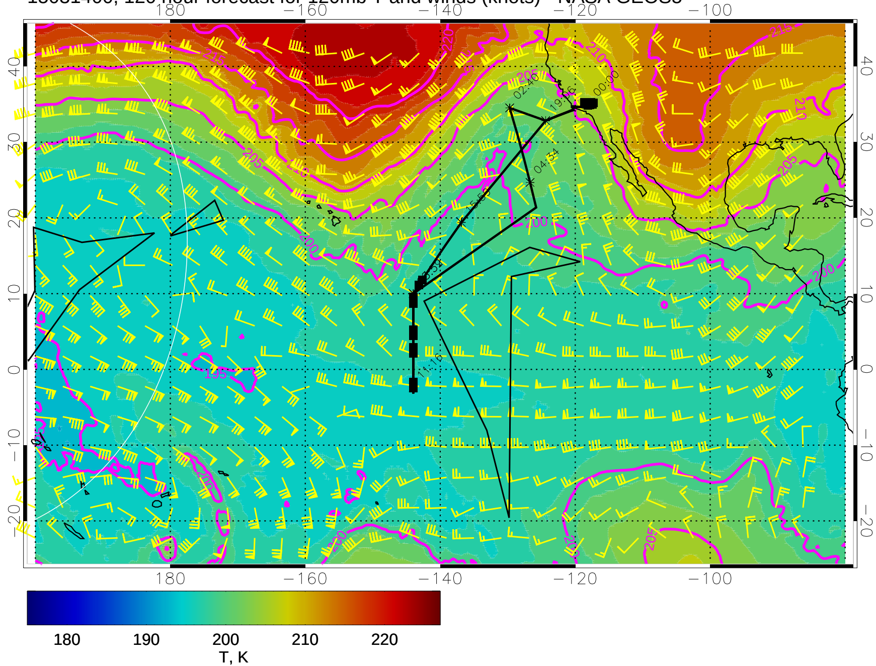
15031400, 120 hour forecast for 120mb T and winds (knots) - NASA GEOS5
