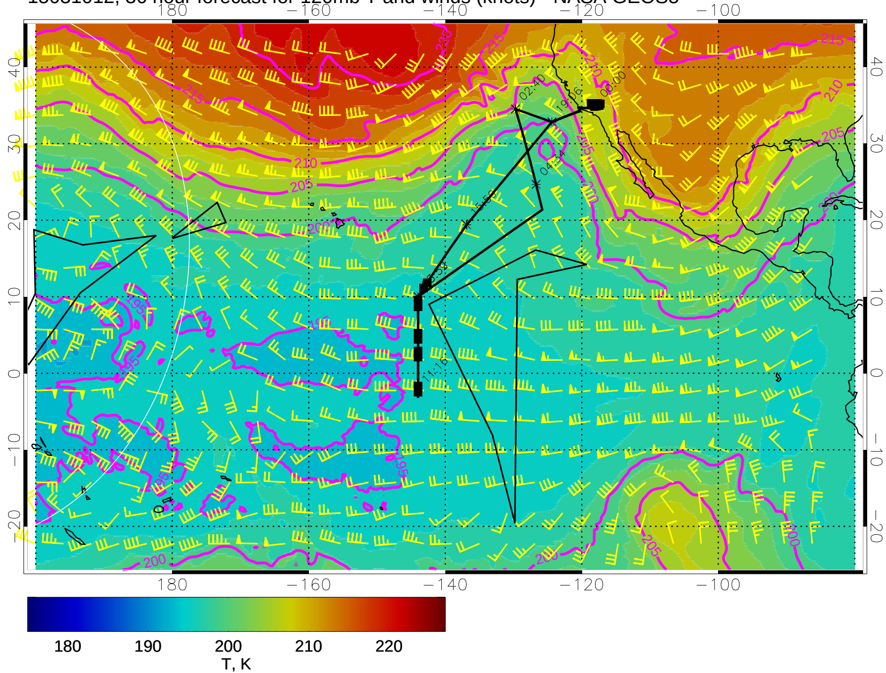
15031012, 36 hour forecast for 120mb T and winds (knots) - NASA GEOS5
