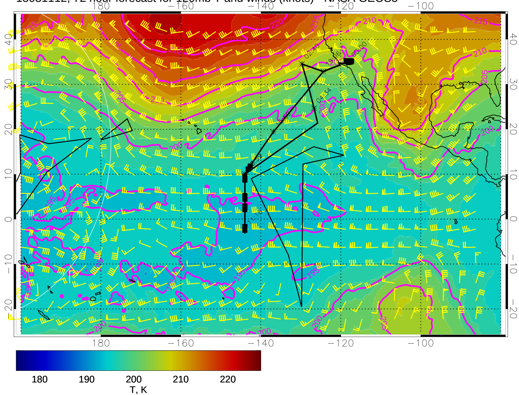
15031112, 72 hour forecast for 120mb T and winds (knots) - NASA GEOS5
