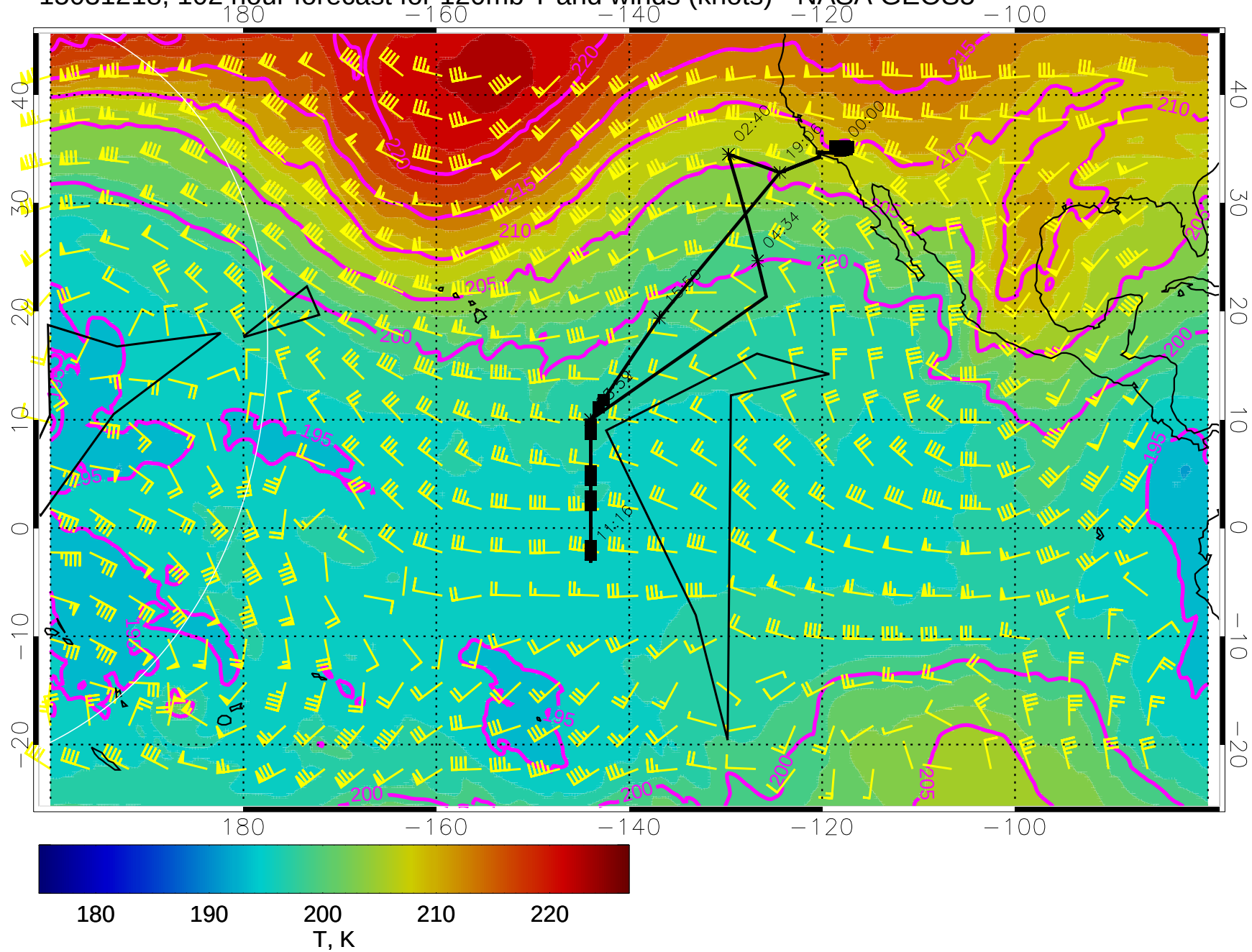
15031218, 102 hour forecast for 120mb T and winds (knots) - NASA GEOS5
