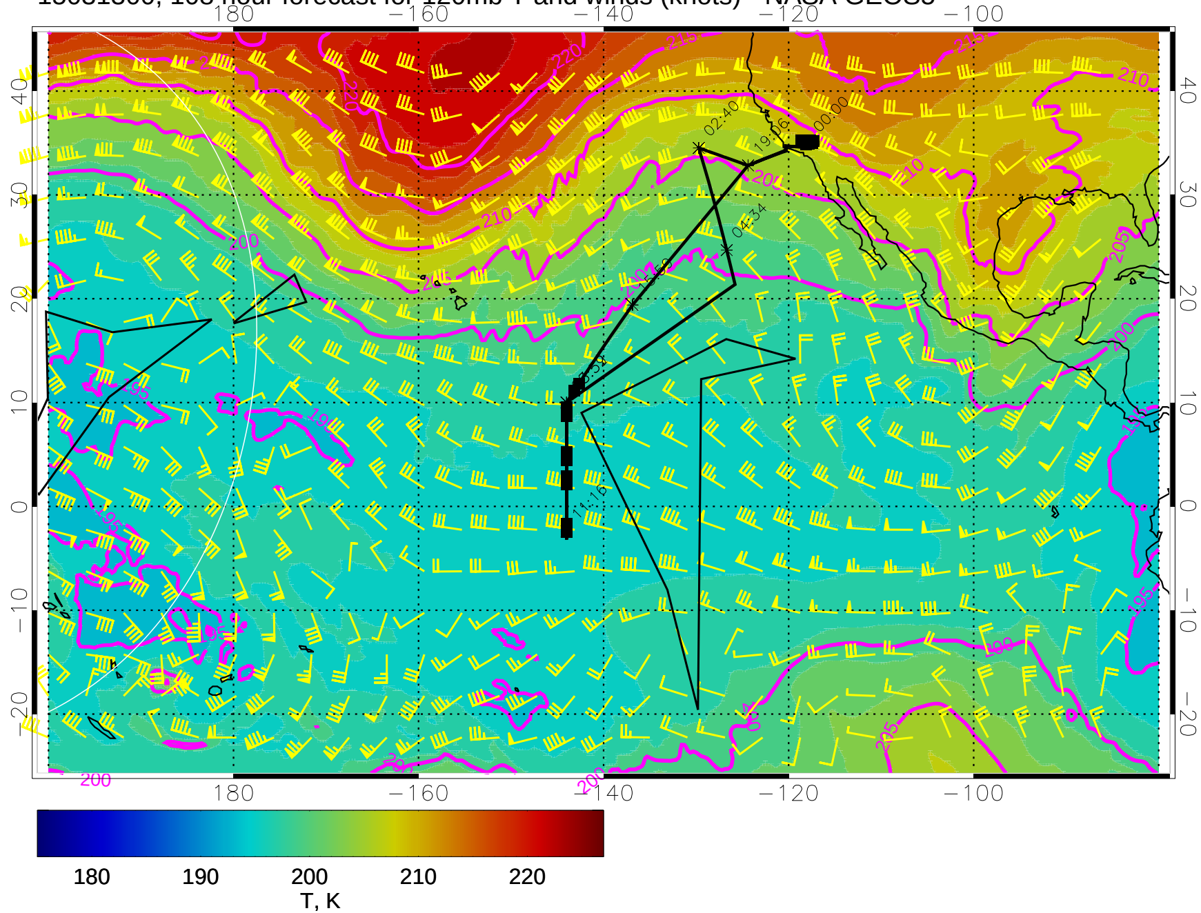
15031300, 108 hour forecast for 120mb T and winds (knots) - NASA GEOS5
