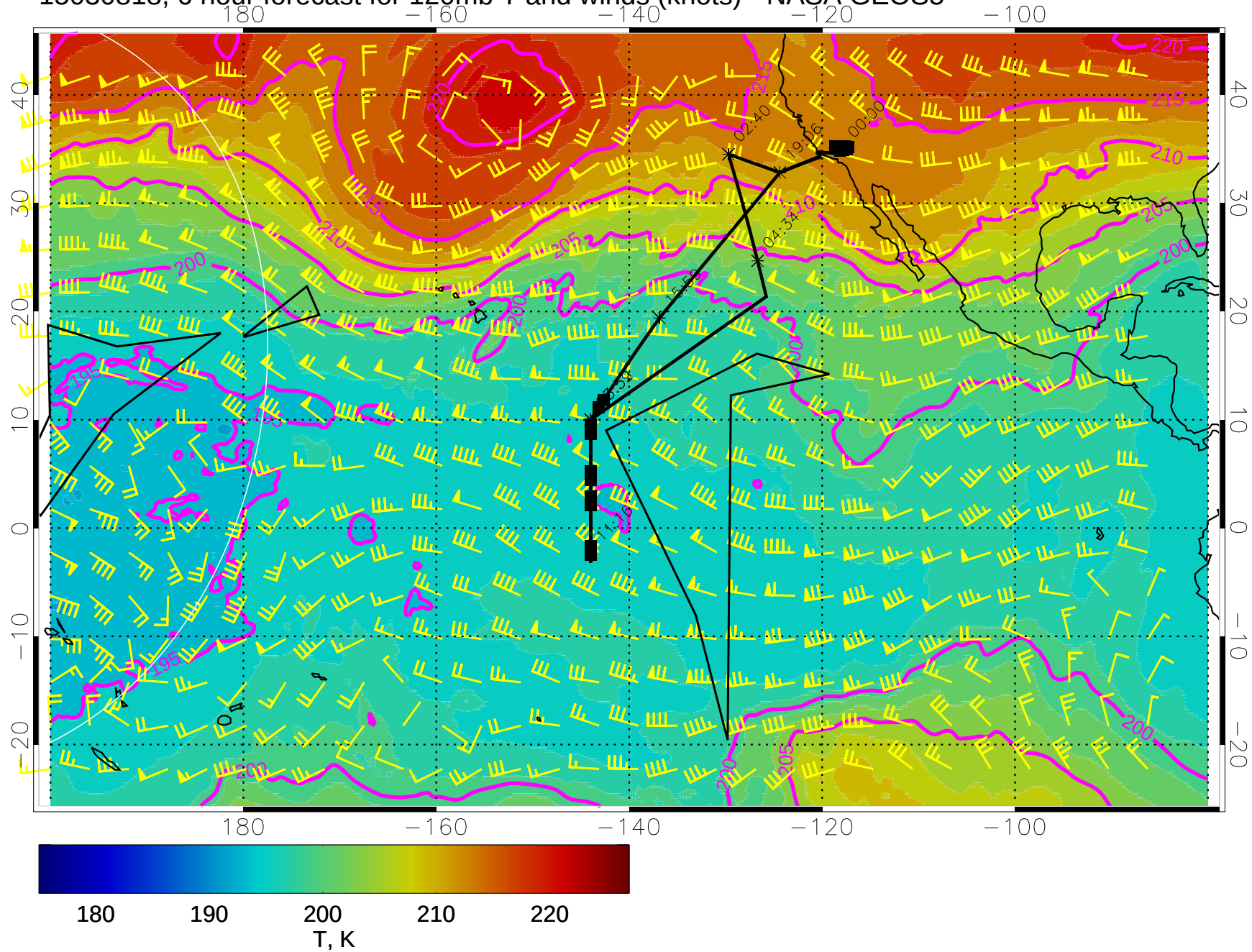
15030818, 6 hour forecast for 120mb T and winds (knots) - NASA GEOS5
