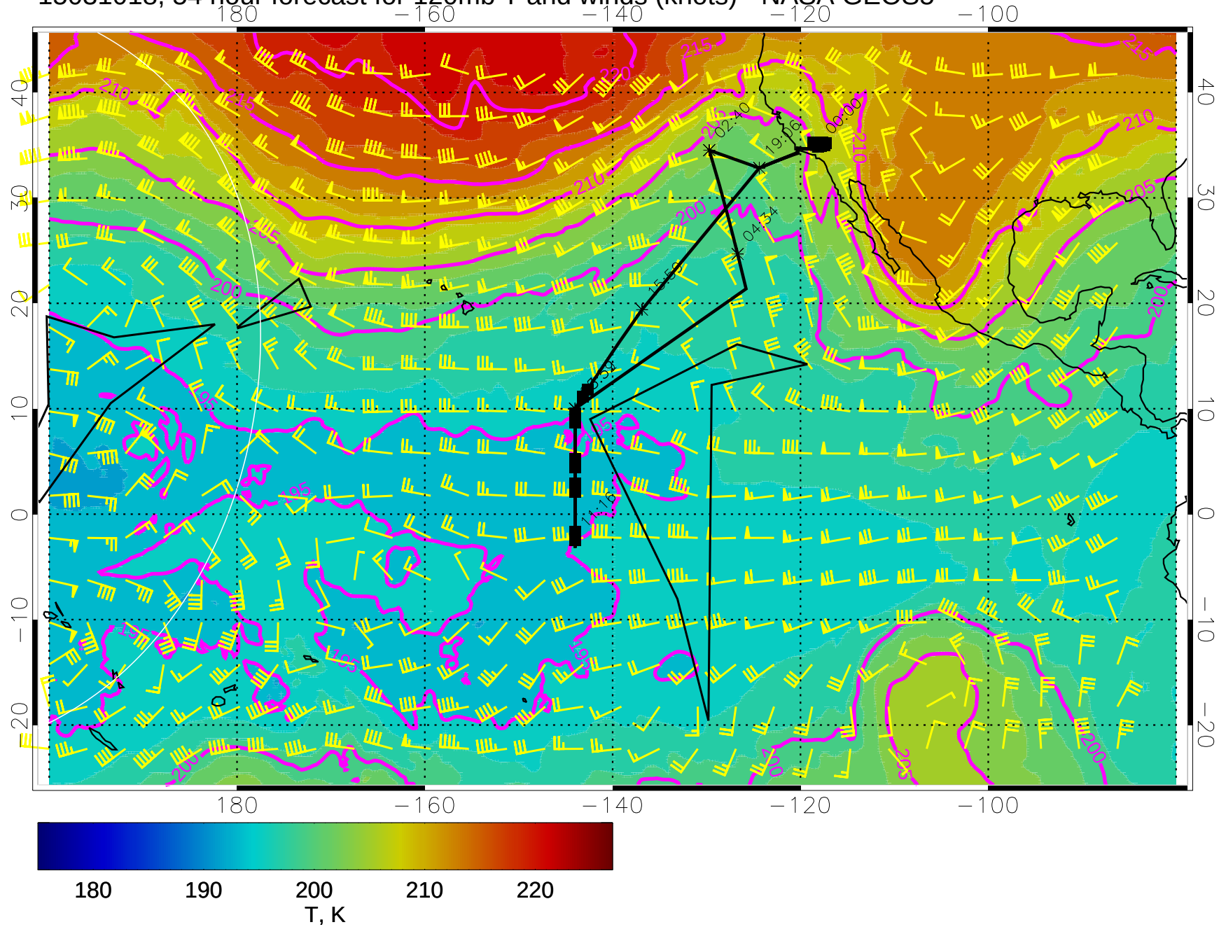
15031018, 54 hour forecast for 120mb T and winds (knots) - NASA GEOS5
