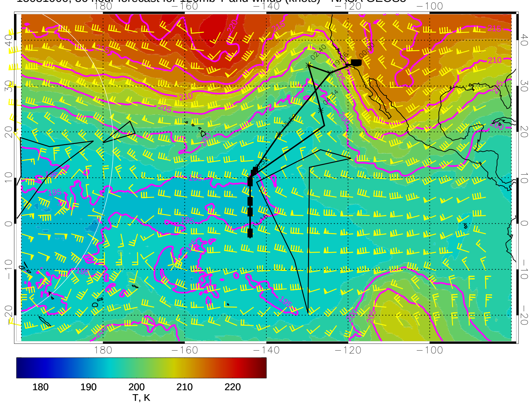
15031000, 36 hour forecast for 120mb T and winds (knots) - NASA GEOS5
