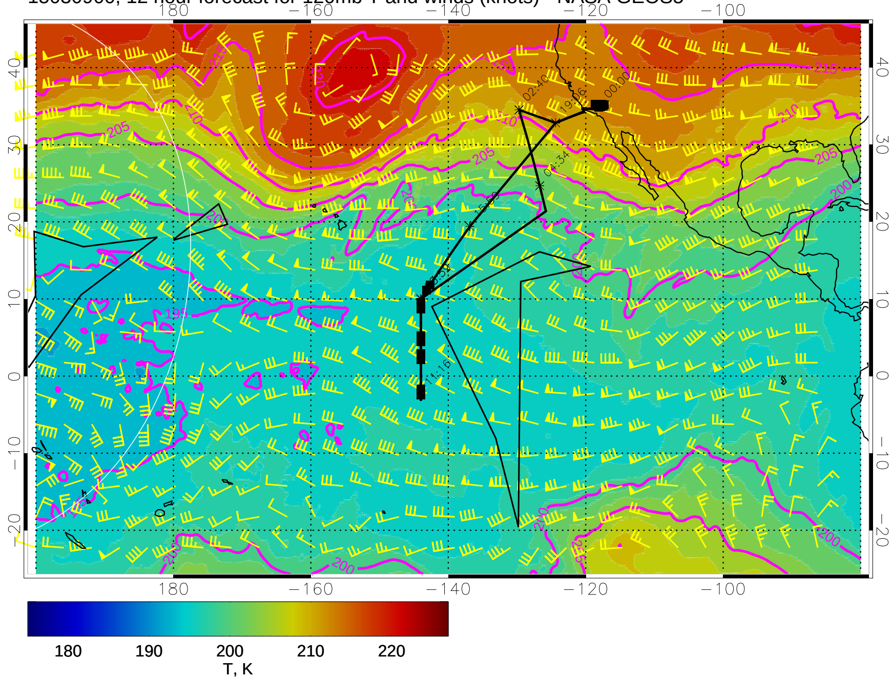
15030900, 12 hour forecast for 120mb T and winds (knots) - NASA GEOS5
