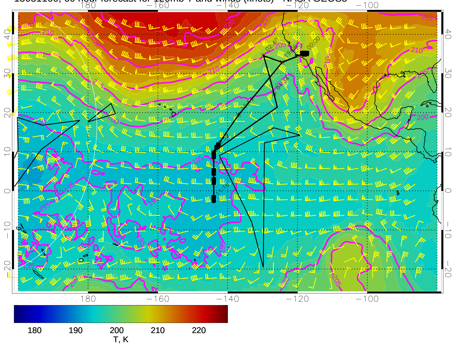
15031100, 60 hour forecast for 120mb T and winds (knots) - NASA GEOS5
