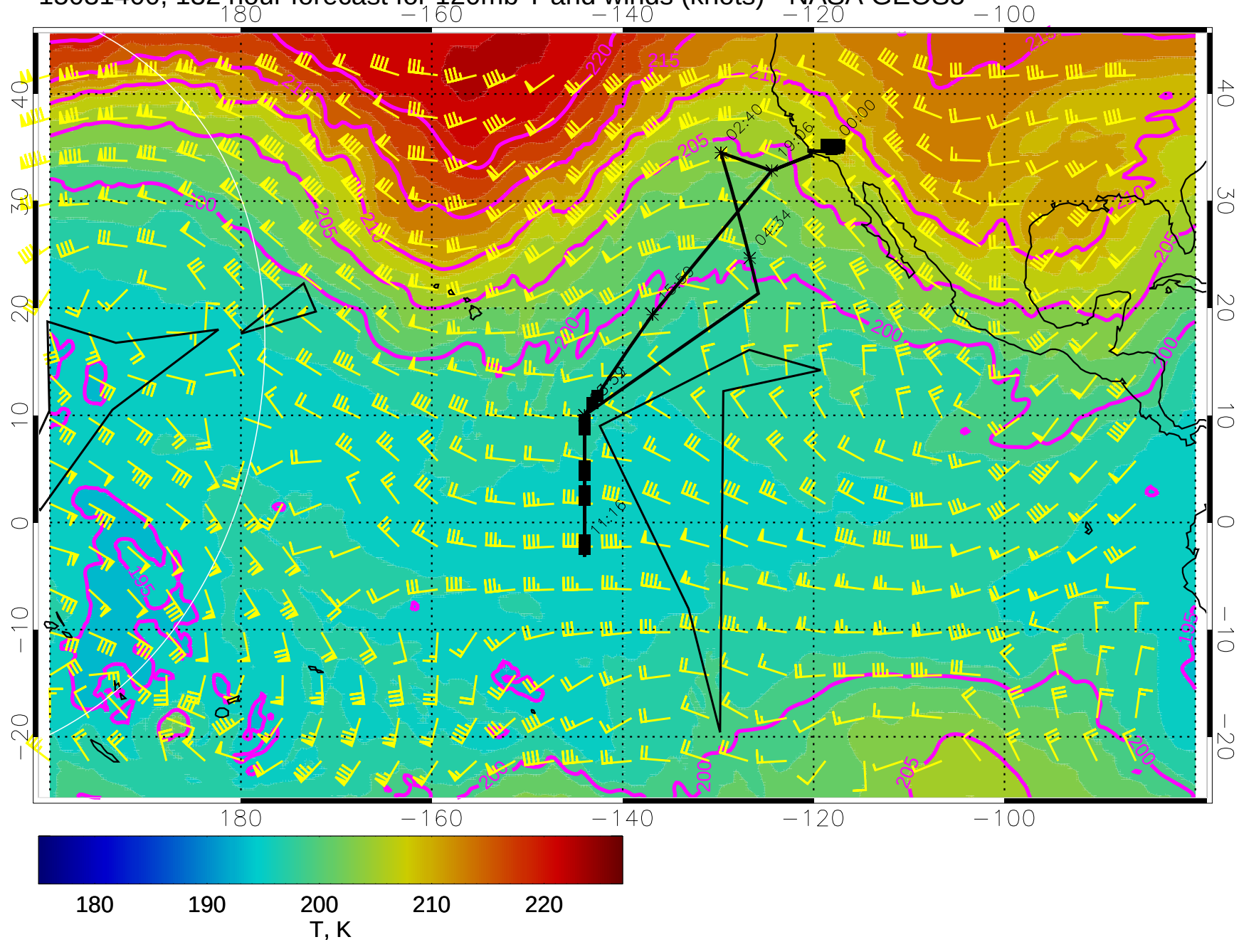
15031400, 132 hour forecast for 120mb T and winds (knots) - NASA GEOS5
