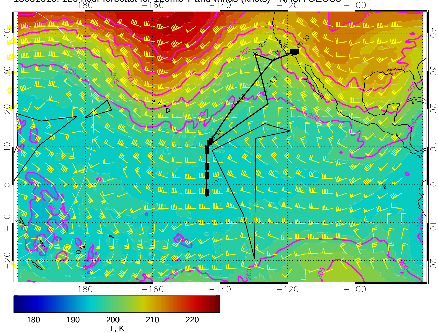
15031318, 126 hour forecast for 120mb T and winds (knots) - NASA GEOS5
