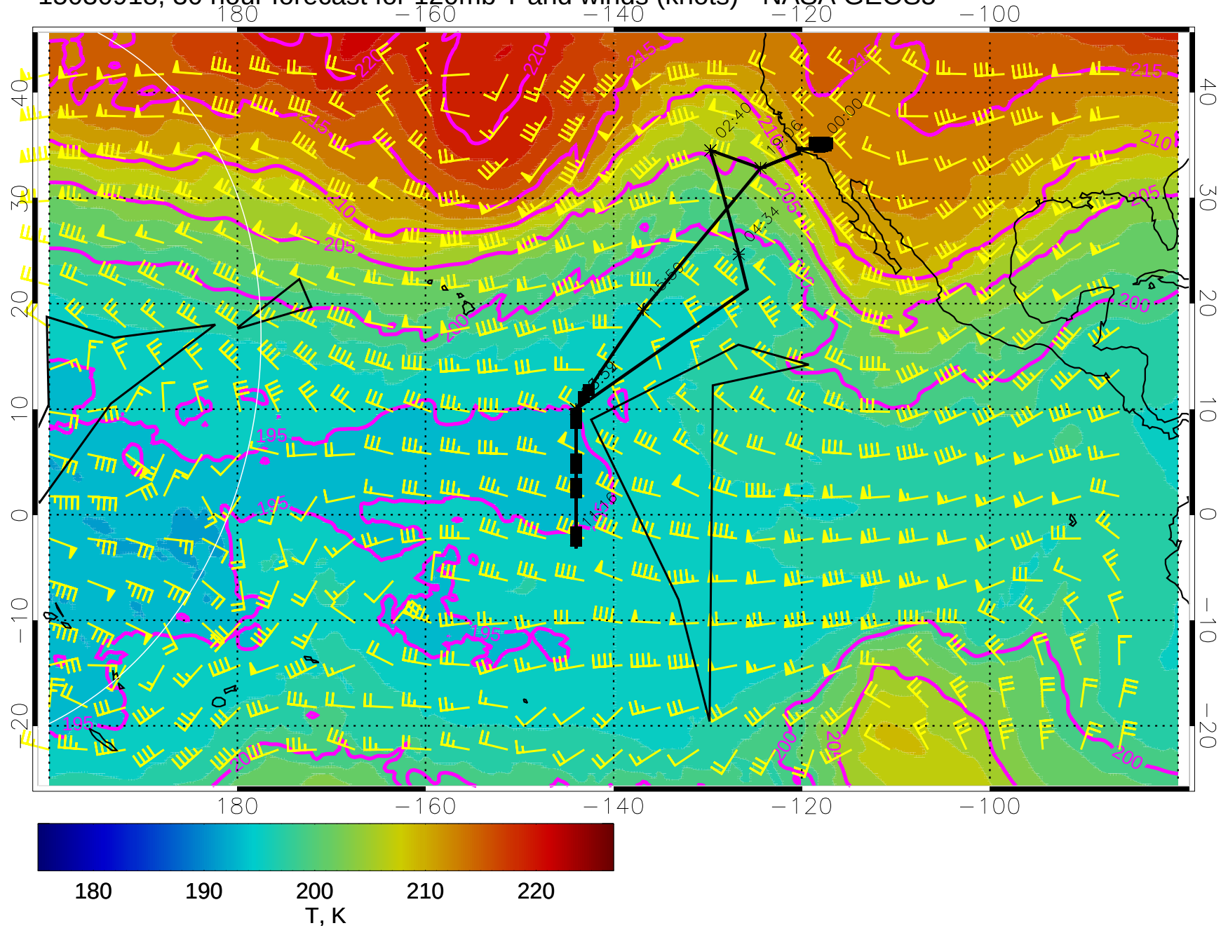
15030918, 30 hour forecast for 120mb T and winds (knots) - NASA GEOS5
