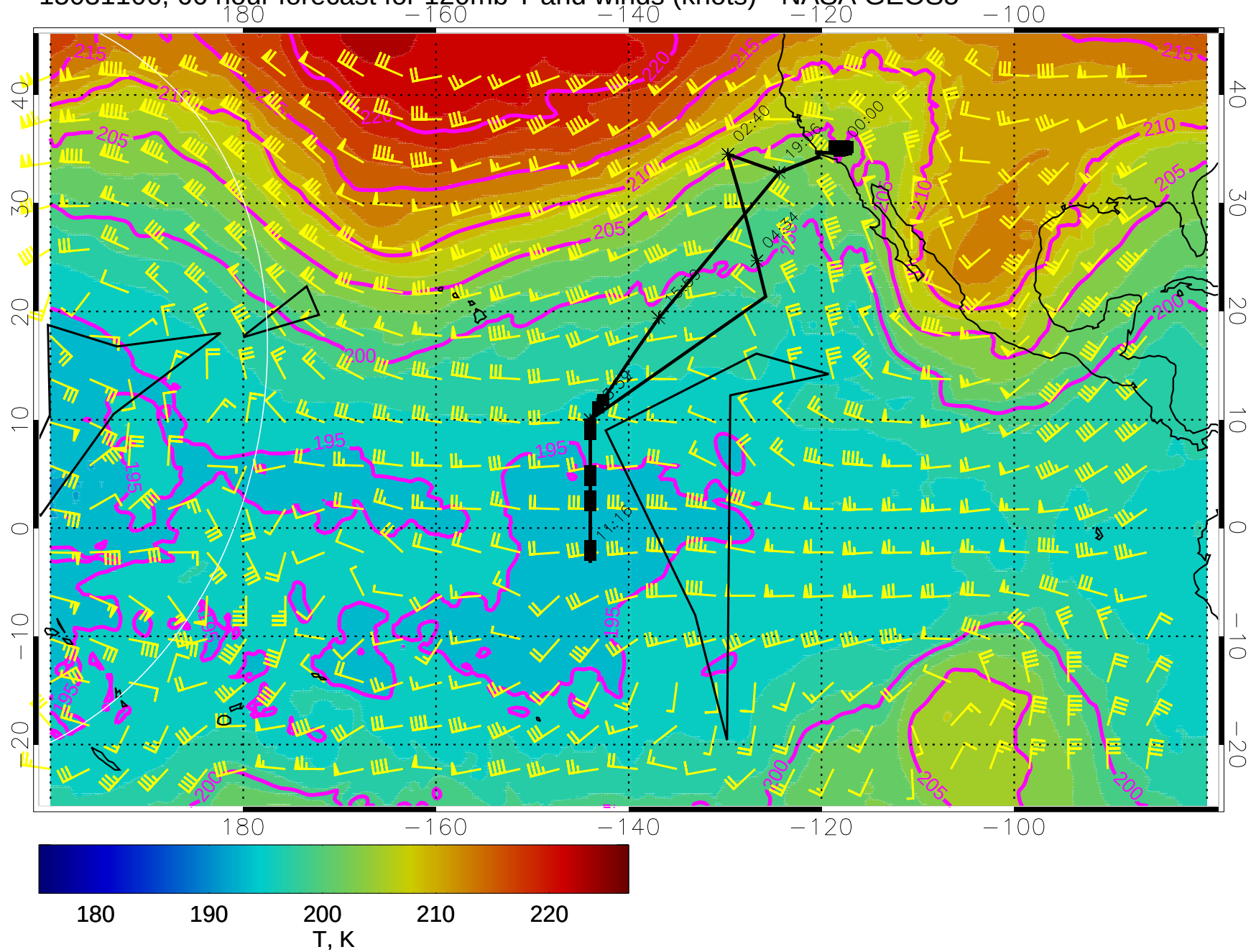
15031106, 66 hour forecast for 120mb T and winds (knots) - NASA GEOS5
