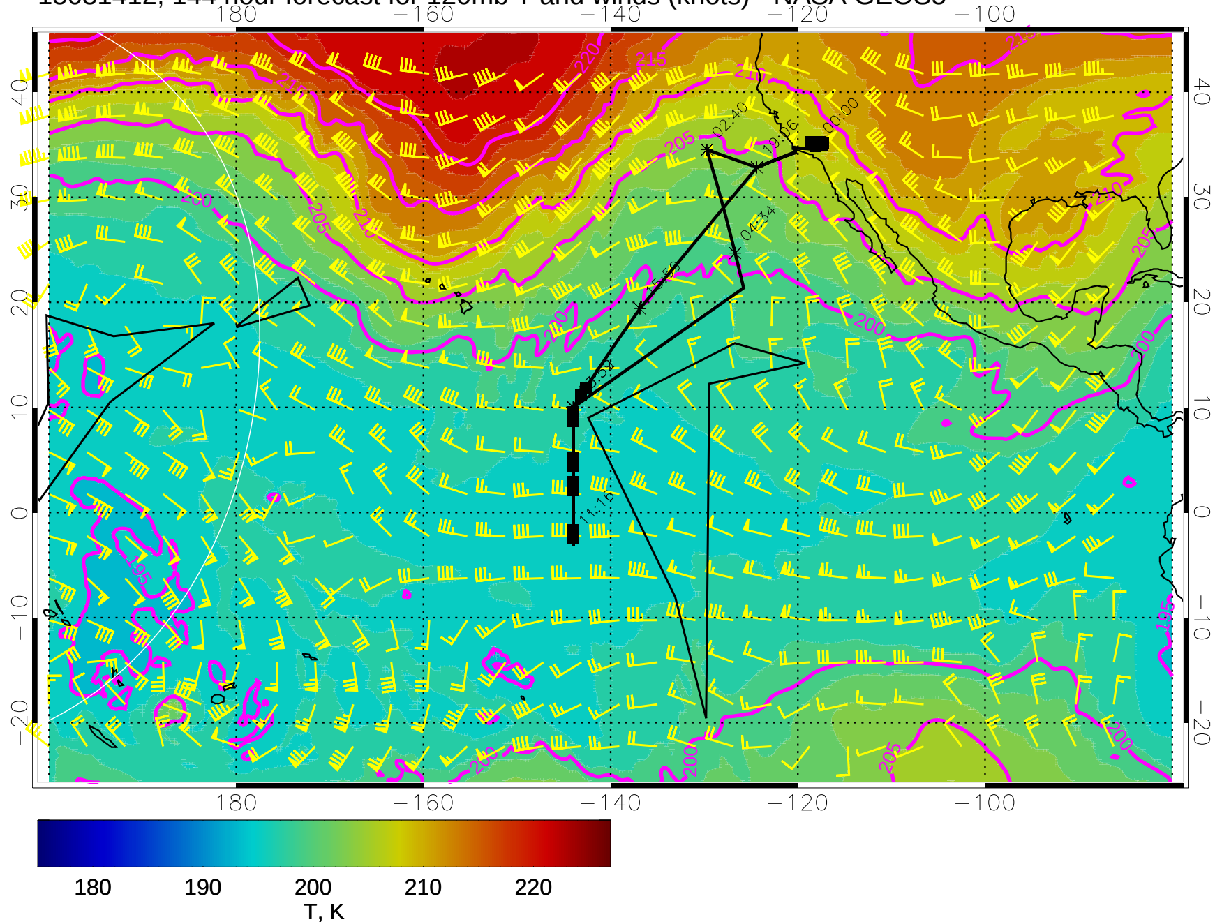
15031412, 144 hour forecast for 120mb T and winds (knots) - NASA GEOS5
