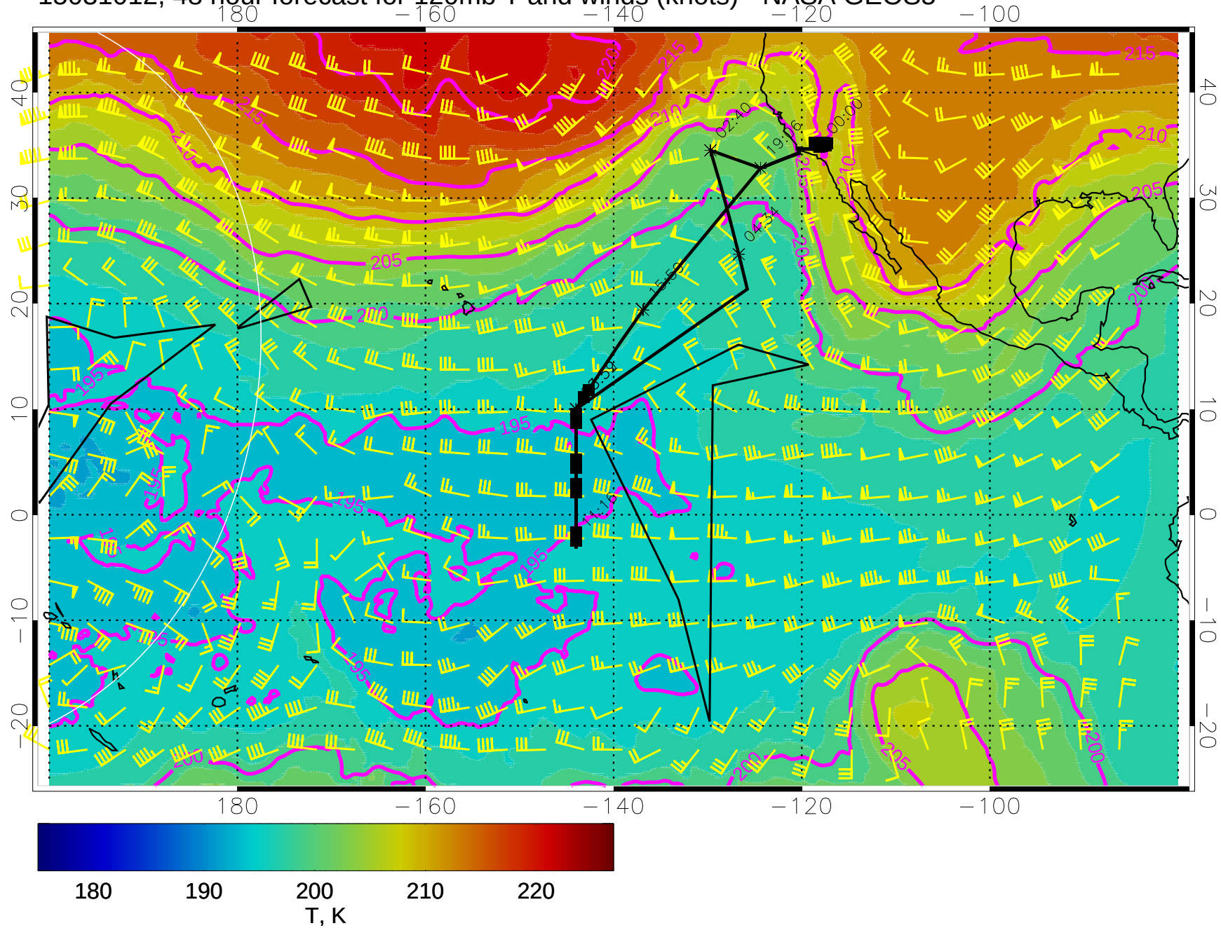
15031012, 48 hour forecast for 120mb T and winds (knots) - NASA GEOS5
