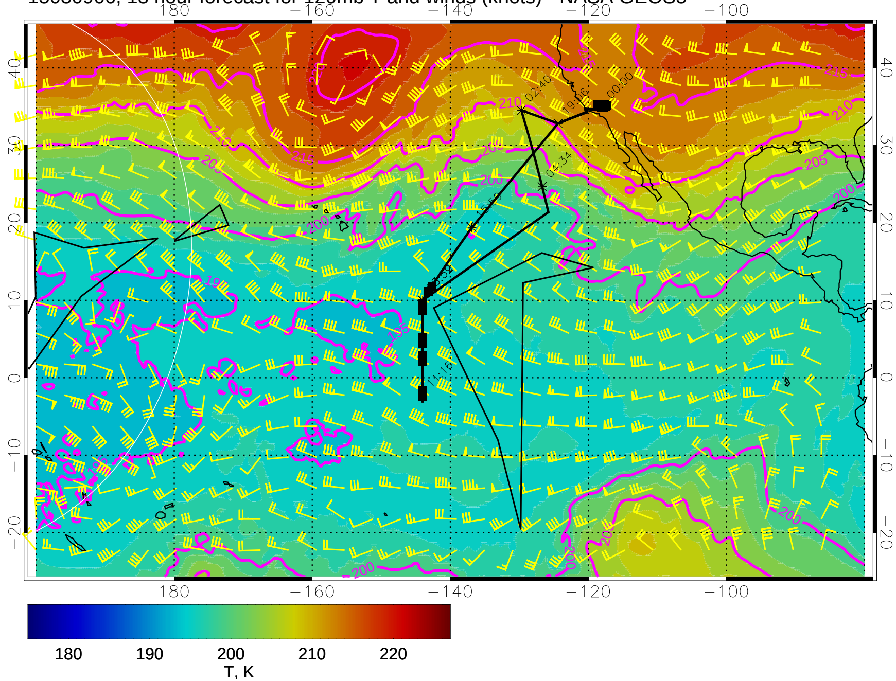
15030906, 18 hour forecast for 120mb T and winds (knots) - NASA GEOS5
