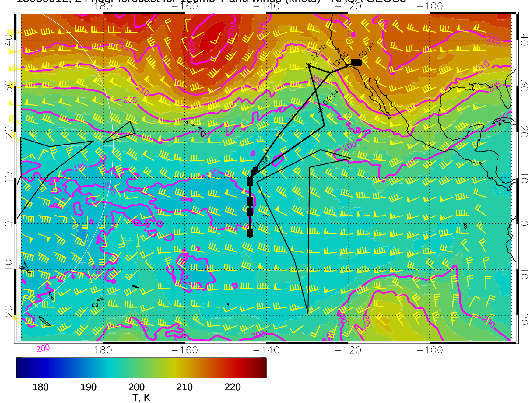
15030912, 24 hour forecast for 120mb T and winds (knots) - NASA GEOS5
