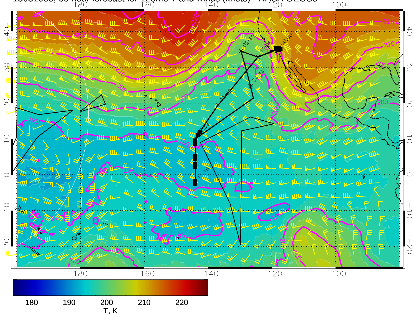
15031000, 60 hour forecast for 120mb T and winds (knots) - NASA GEOS5
