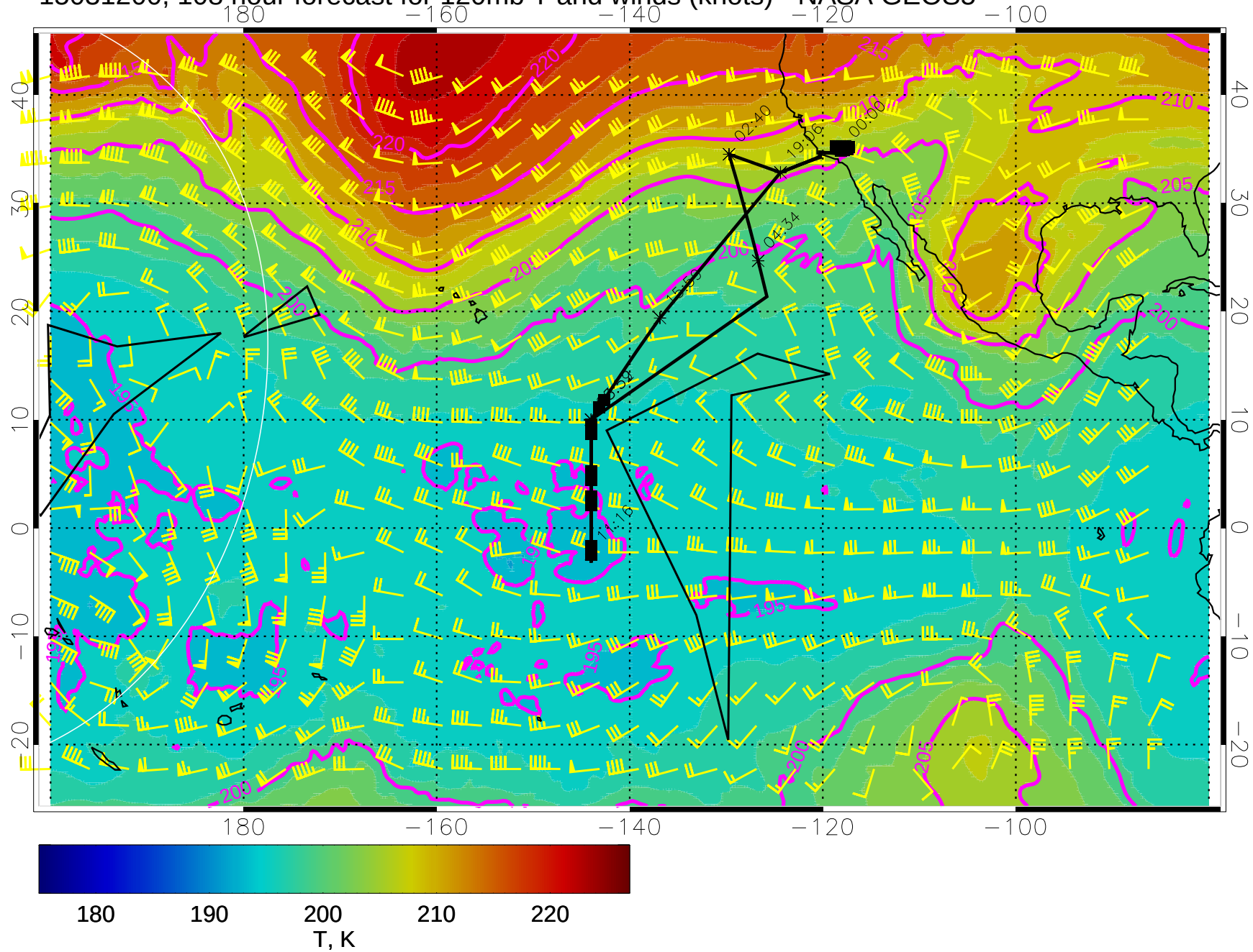
15031200, 108 hour forecast for 120mb T and winds (knots) - NASA GEOS5
