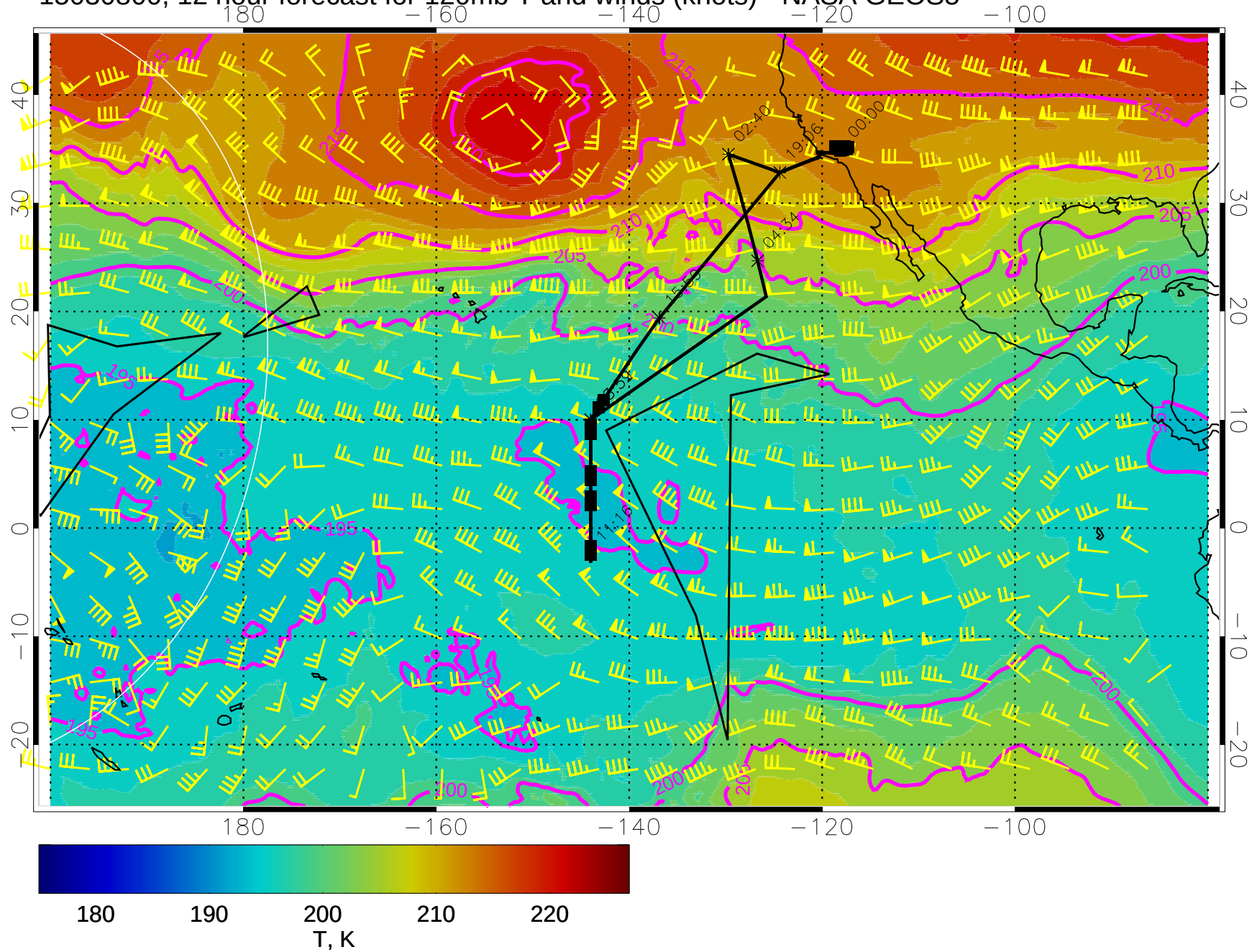
15030800, 12 hour forecast for 120mb T and winds (knots) - NASA GEOS5
