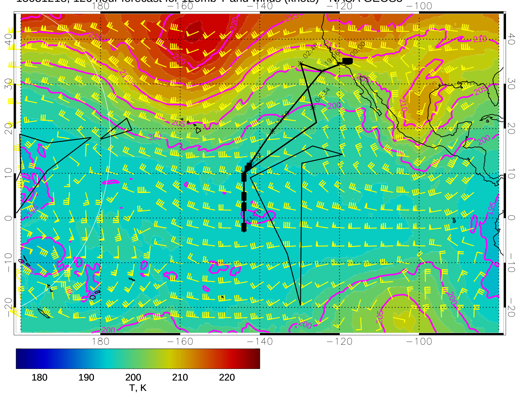
15031218, 126 hour forecast for 120mb T and winds (knots) - NASA GEOS5
