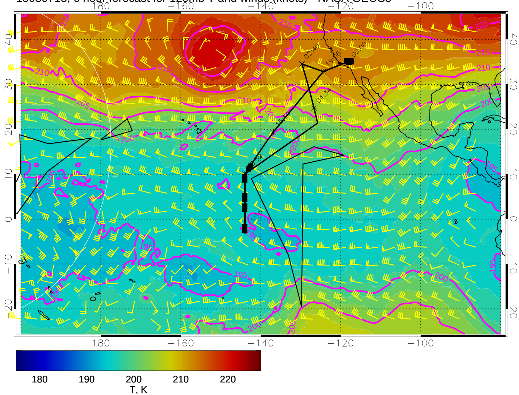
15030718, 6 hour forecast for 120mb T and winds (knots) - NASA GEOS5
