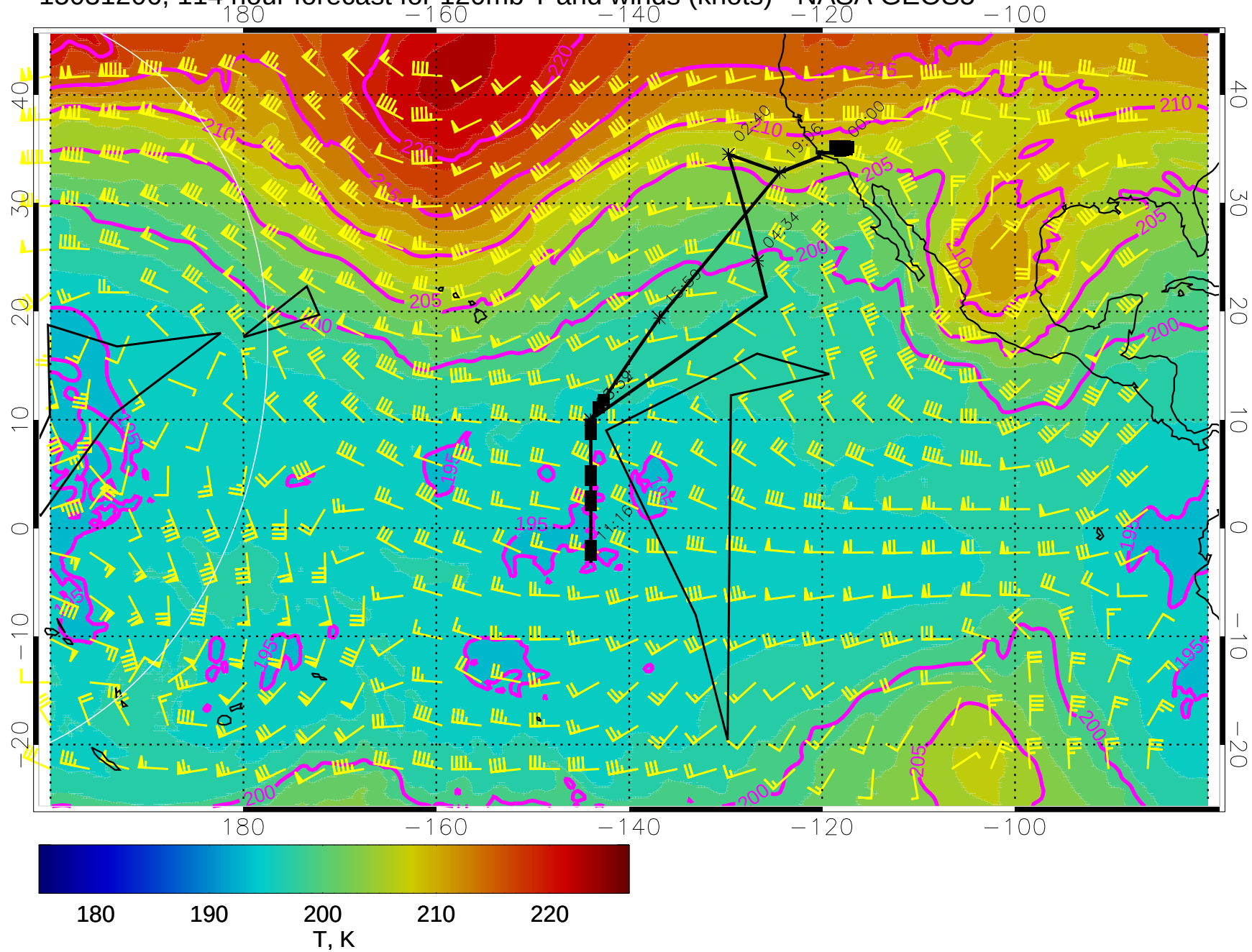
15031206, 114 hour forecast for 120mb T and winds (knots) - NASA GEOS5
