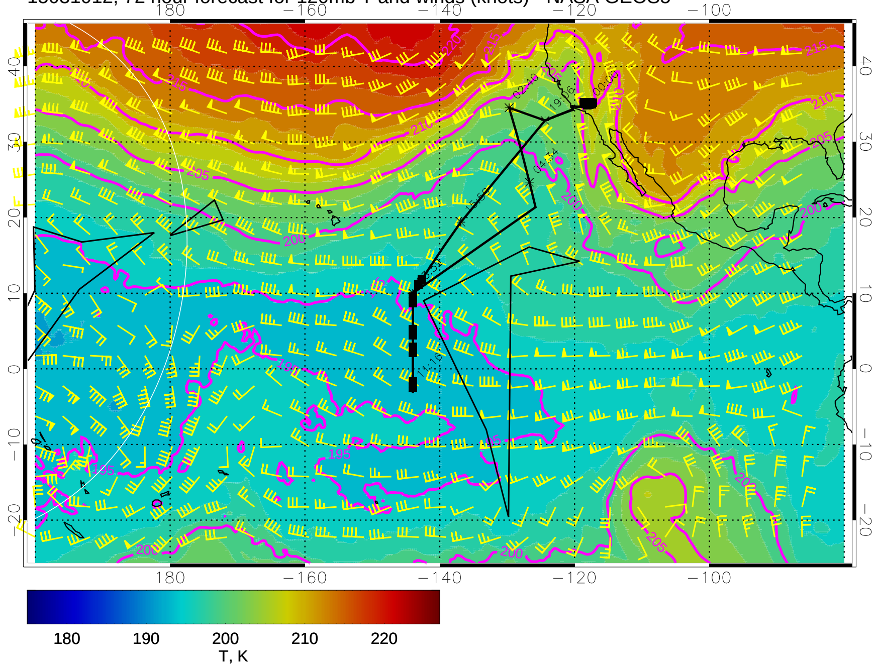
15031012, 72 hour forecast for 120mb T and winds (knots) - NASA GEOS5
