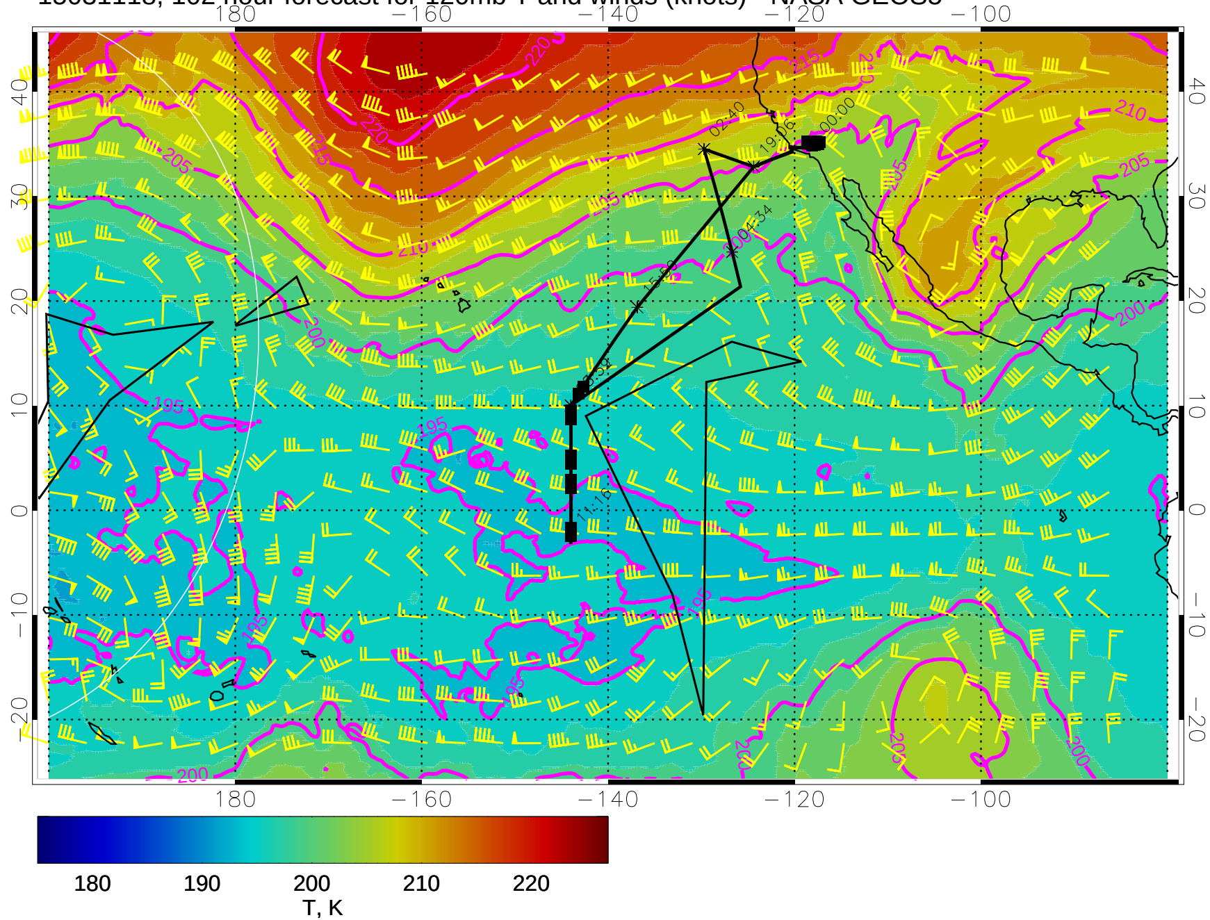
15031118, 102 hour forecast for 120mb T and winds (knots) - NASA GEOS5
