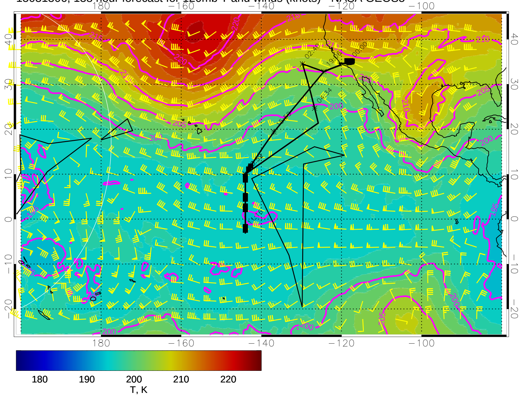
15031306, 138 hour forecast for 120mb T and winds (knots) - NASA GEOS5
