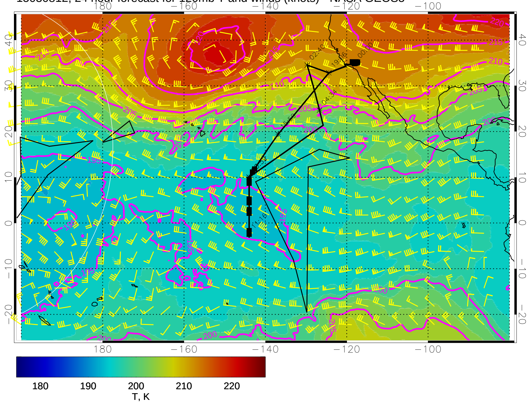
15030812, 24 hour forecast for 120mb T and winds (knots) - NASA GEOS5
