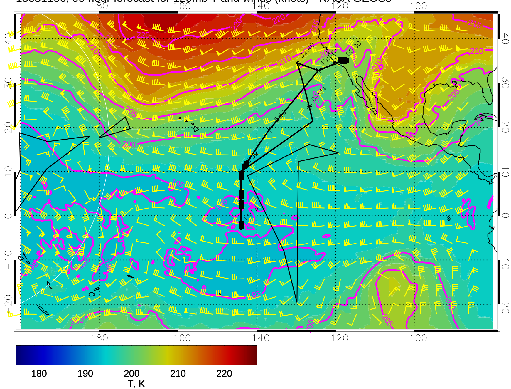
15031106, 90 hour forecast for 120mb T and winds (knots) - NASA GEOS5
