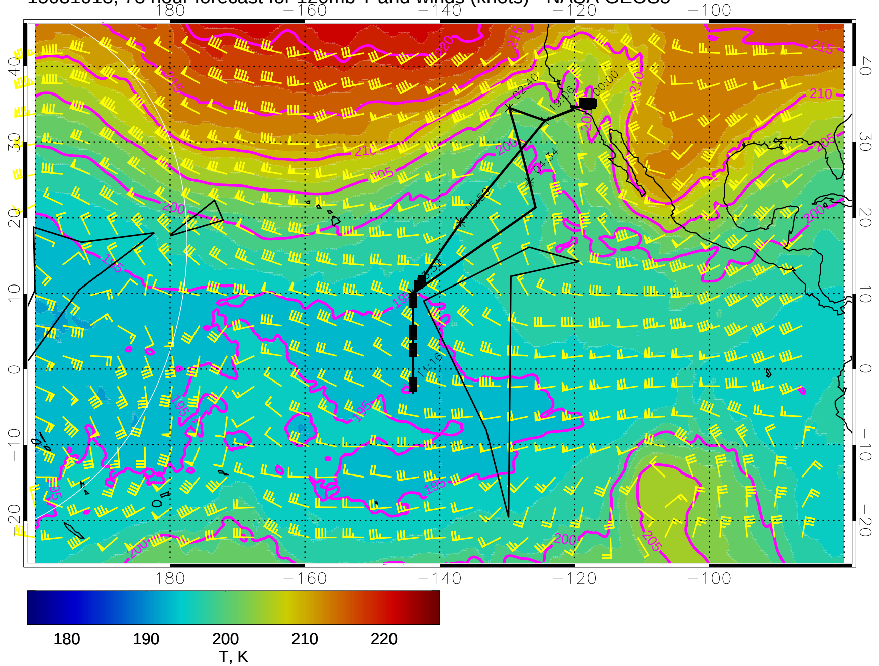
15031018, 78 hour forecast for 120mb T and winds (knots) - NASA GEOS5
