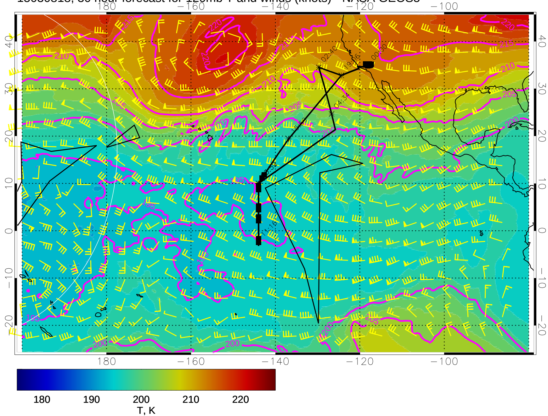
15030818, 30 hour forecast for 120mb T and winds (knots) - NASA GEOS5
