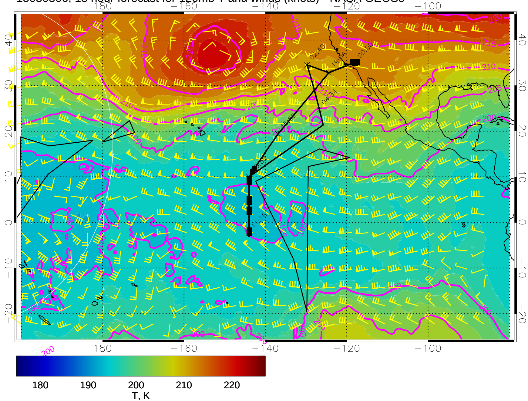
15030806, 18 hour forecast for 120mb T and winds (knots) - NASA GEOS5
