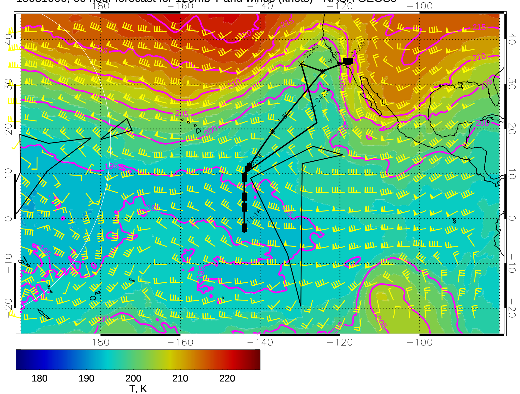
15031006, 66 hour forecast for 120mb T and winds (knots) - NASA GEOS5
