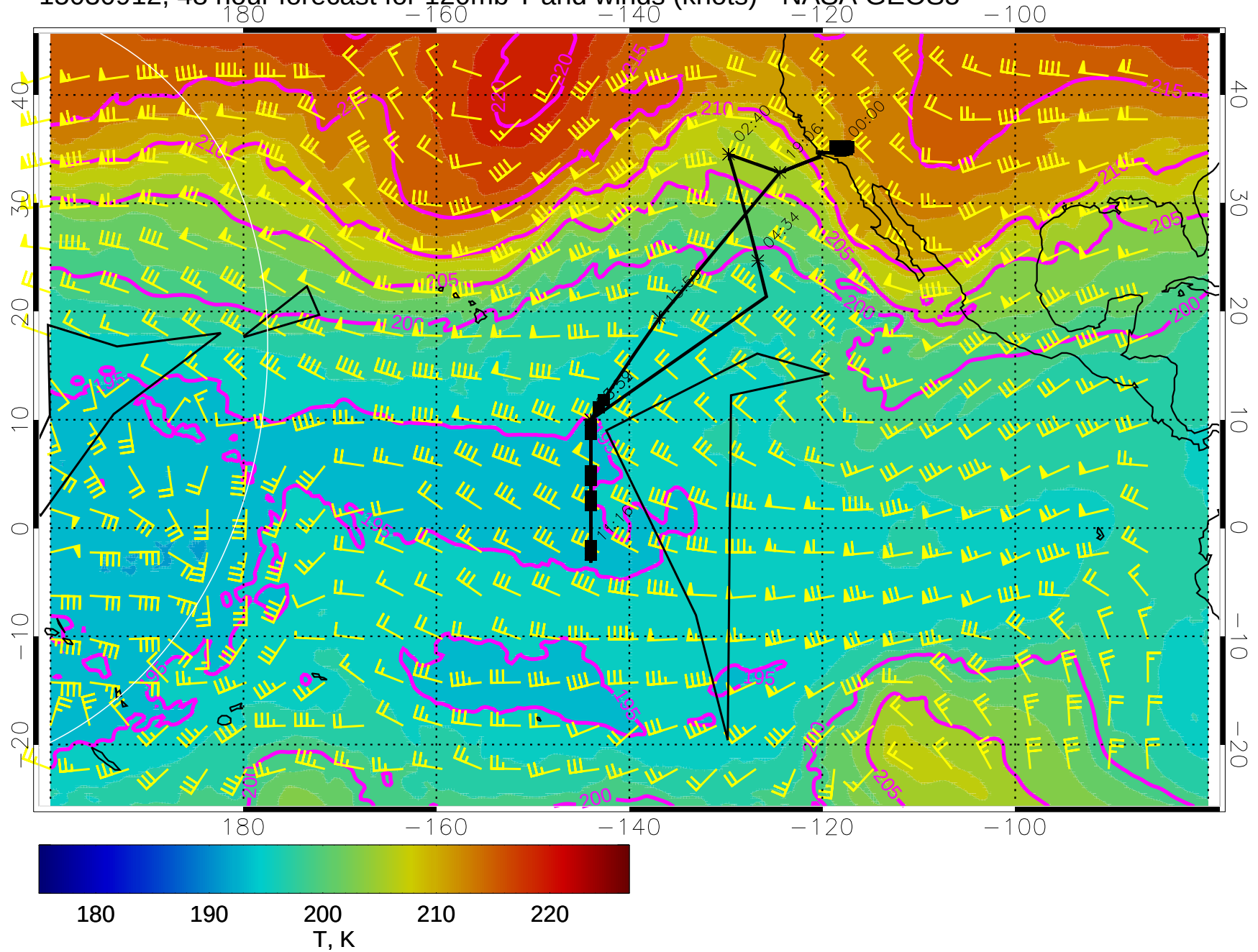
15030912, 48 hour forecast for 120mb T and winds (knots) - NASA GEOS5
