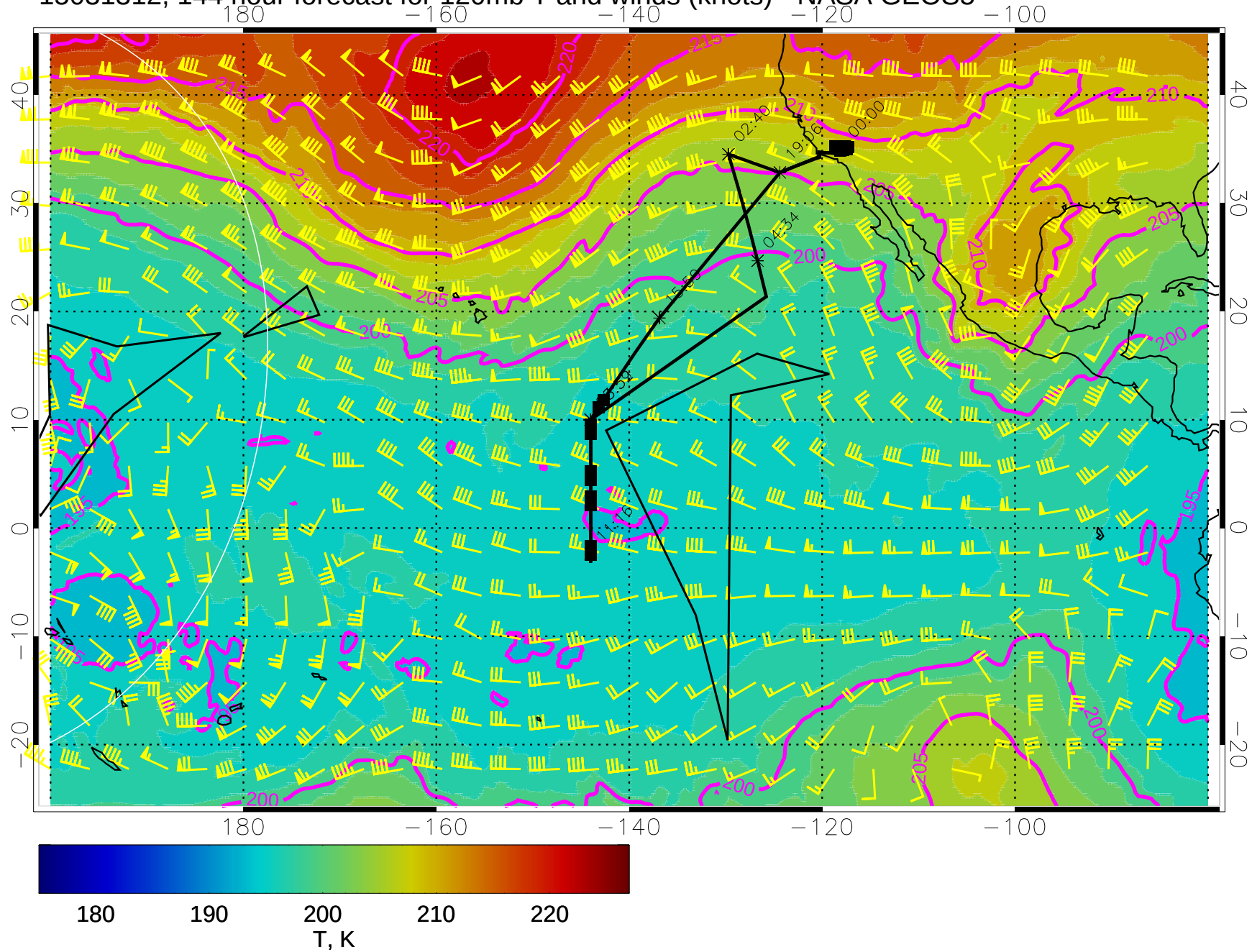
15031312, 144 hour forecast for 120mb T and winds (knots) - NASA GEOS5
