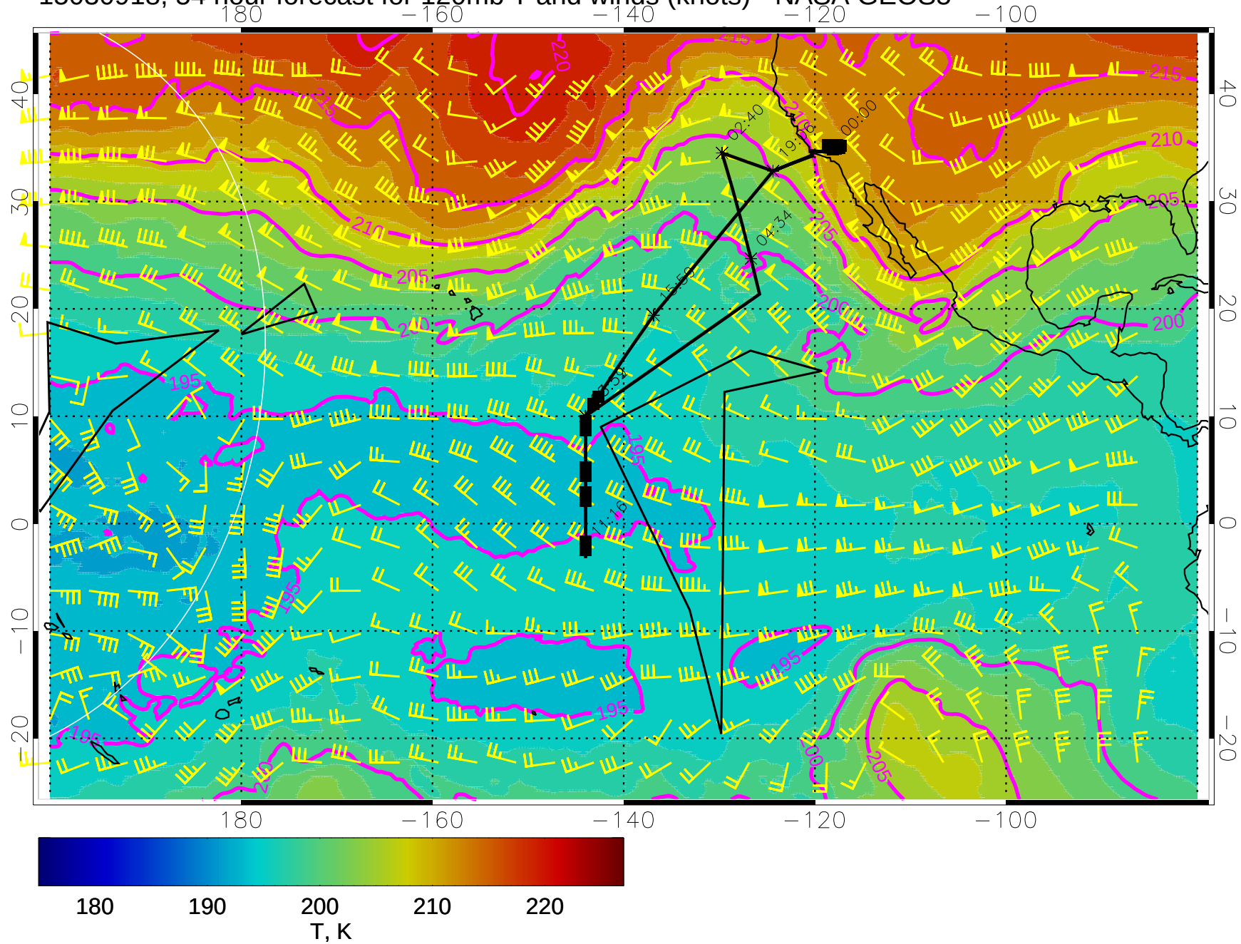
15030918, 54 hour forecast for 120mb T and winds (knots) - NASA GEOS5
