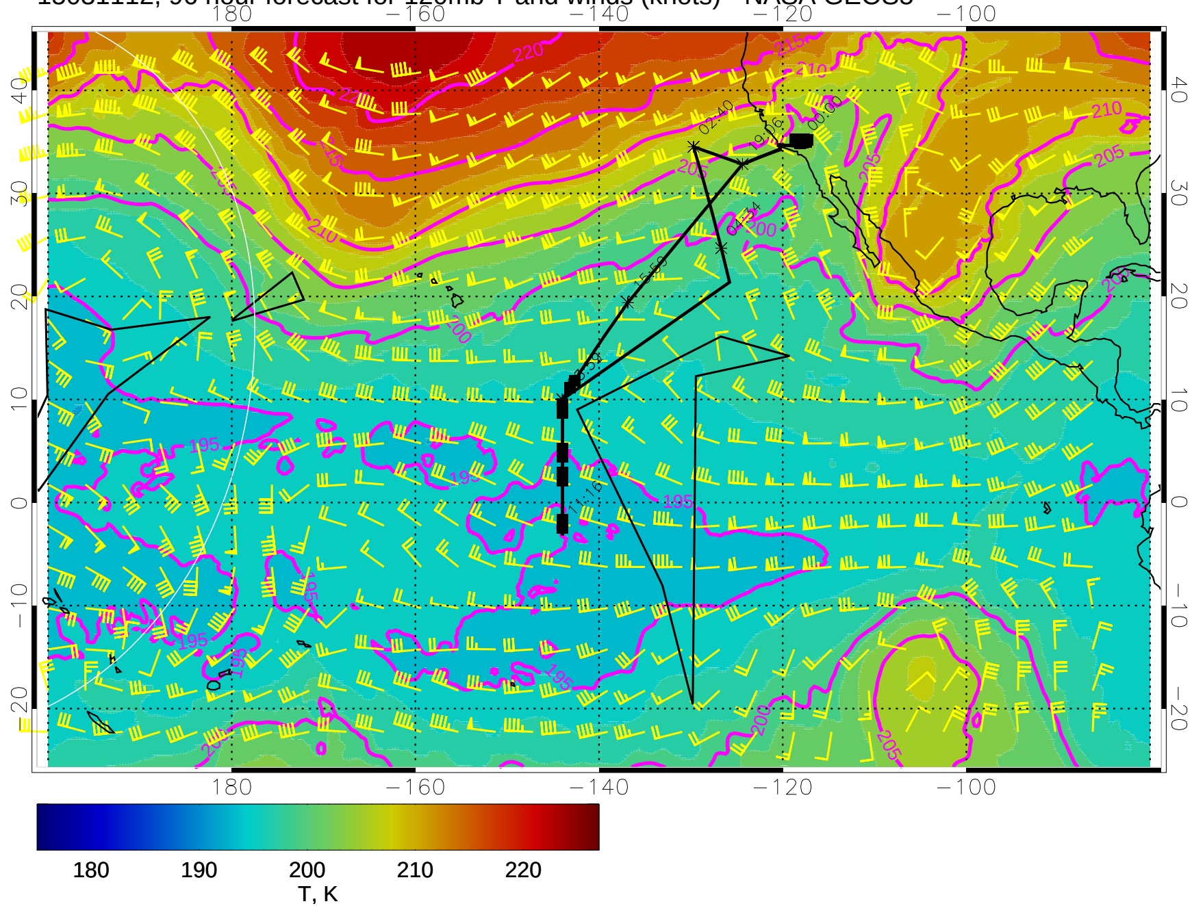
15031112, 96 hour forecast for 120mb T and winds (knots) - NASA GEOS5
