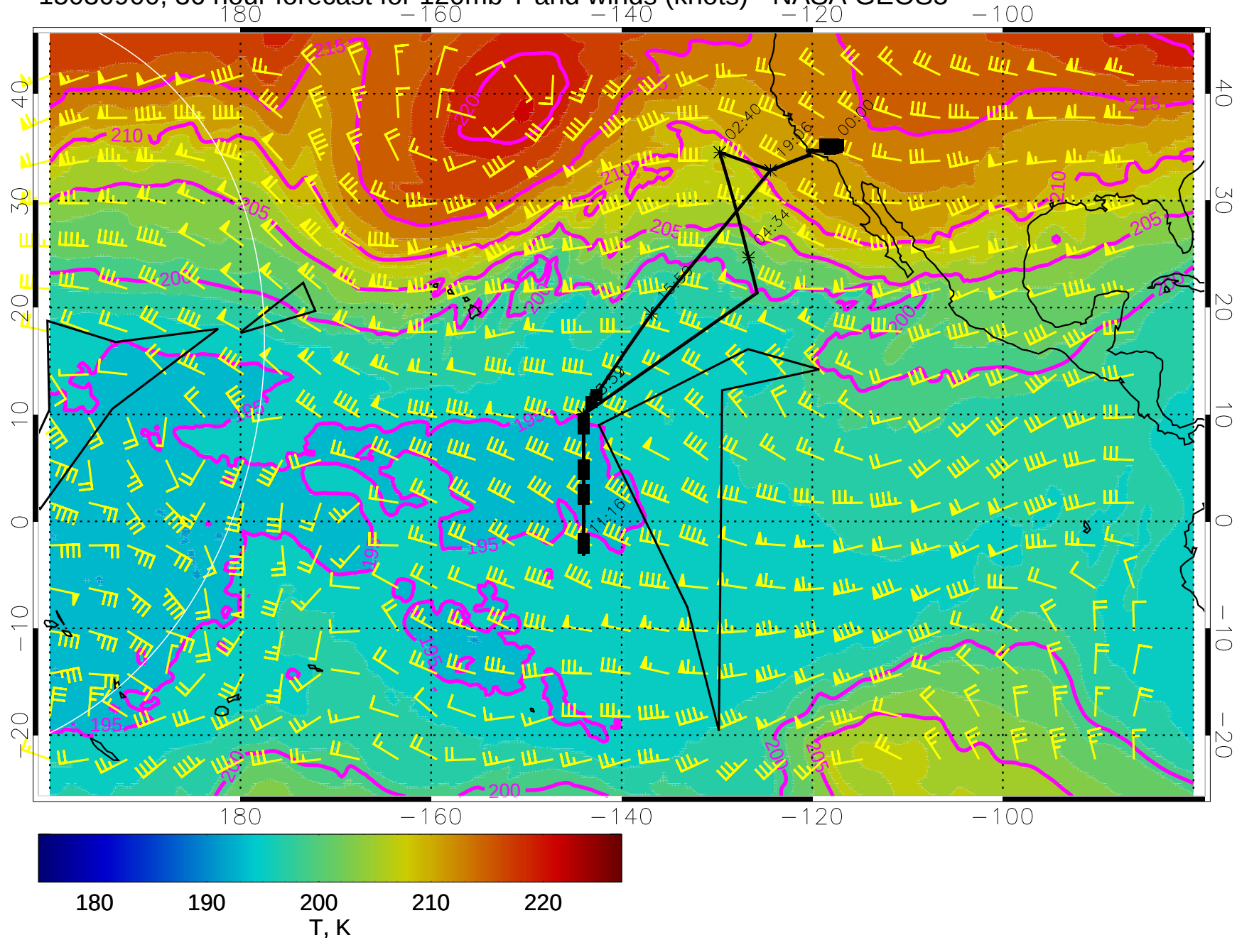
15030900, 36 hour forecast for 120mb T and winds (knots) - NASA GEOS5
