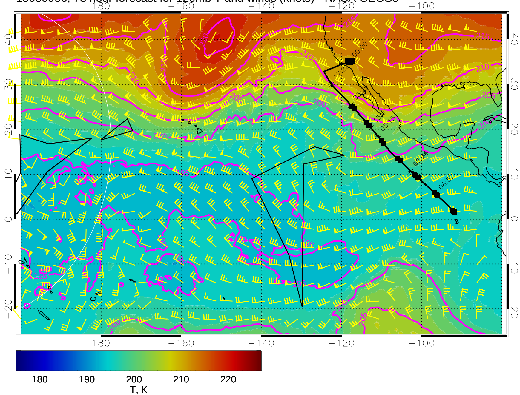
15030906, 78 hour forecast for 120mb T and winds (knots) - NASA GEOS5
