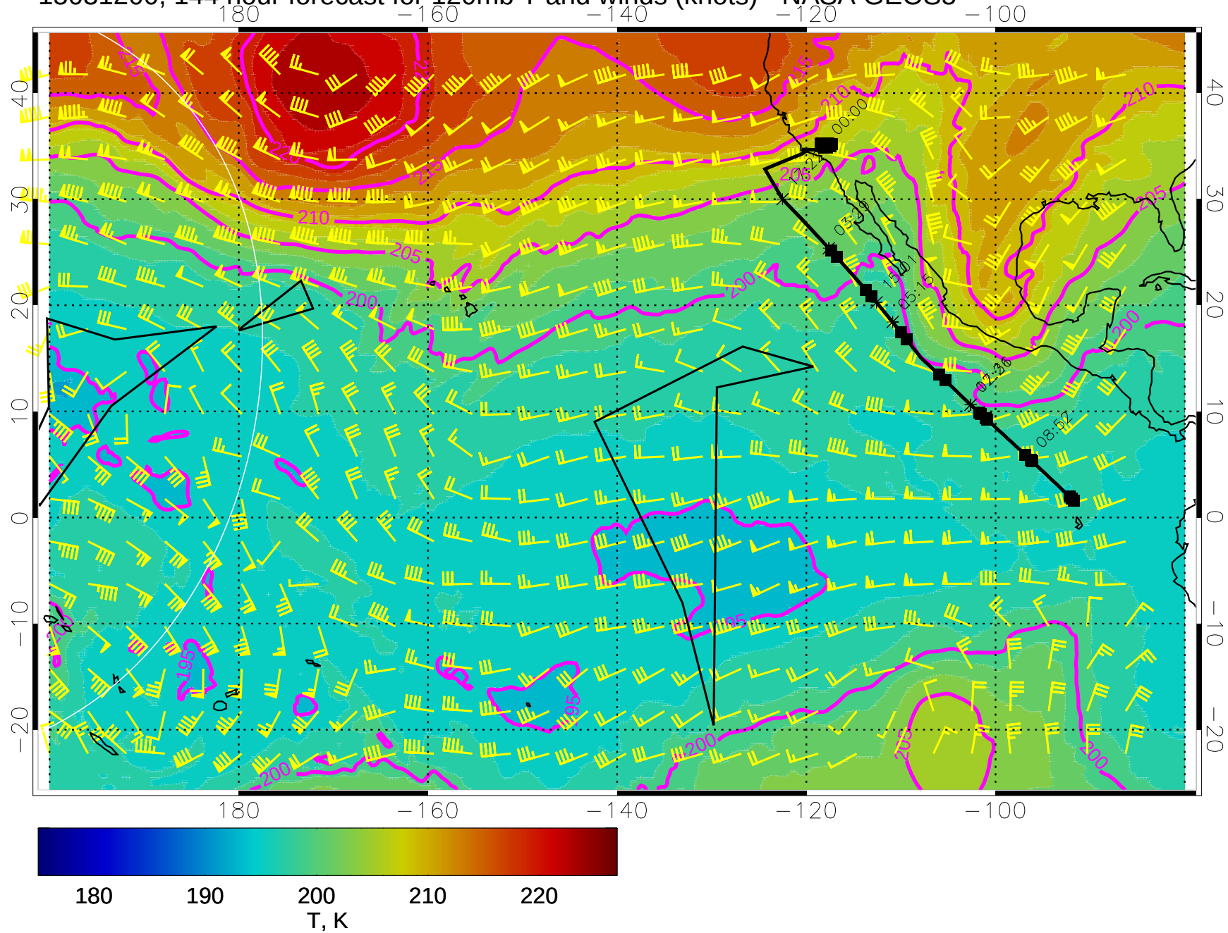
15031200, 144 hour forecast for 120mb T and winds (knots) - NASA GEOS5
