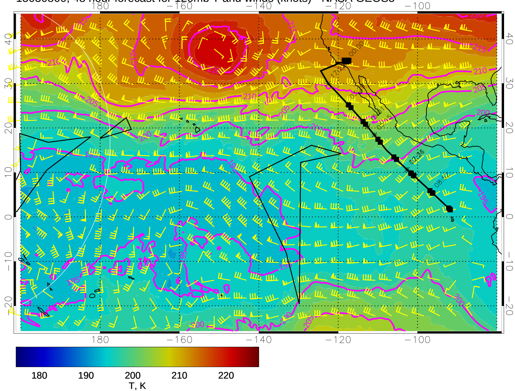
15030800, 48 hour forecast for 120mb T and winds (knots) - NASA GEOS5
