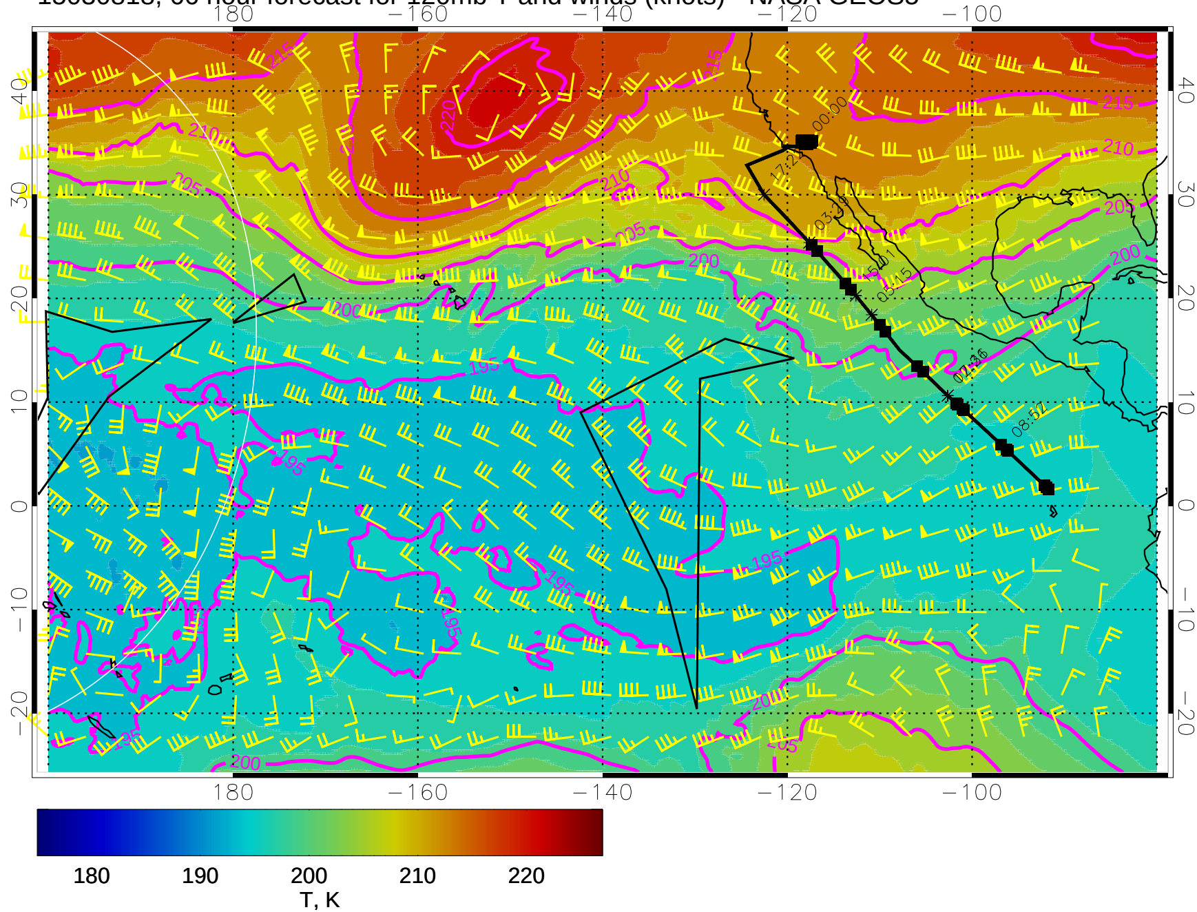
15030818, 66 hour forecast for 120mb T and winds (knots) - NASA GEOS5
