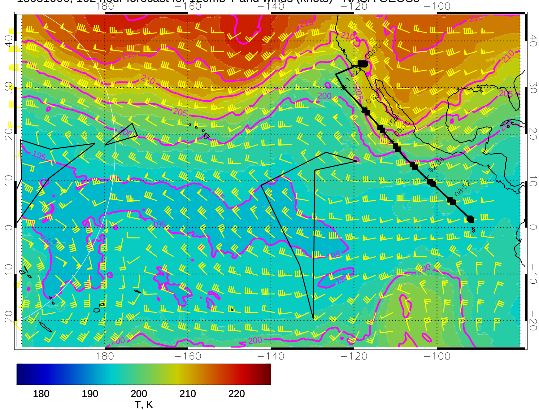
15031006, 102 hour forecast for 120mb T and winds (knots) - NASA GEOS5
