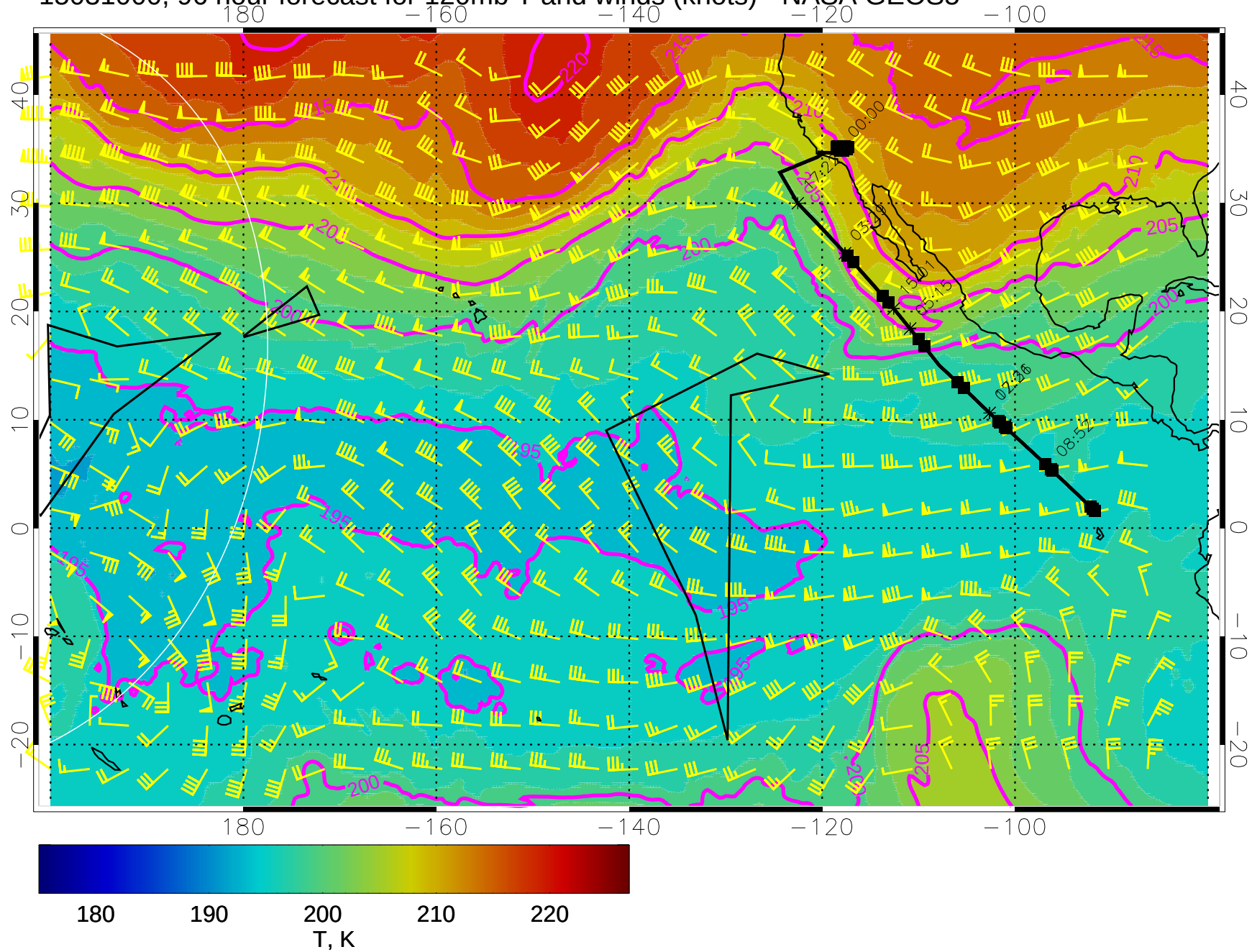
15031000, 96 hour forecast for 120mb T and winds (knots) - NASA GEOS5
