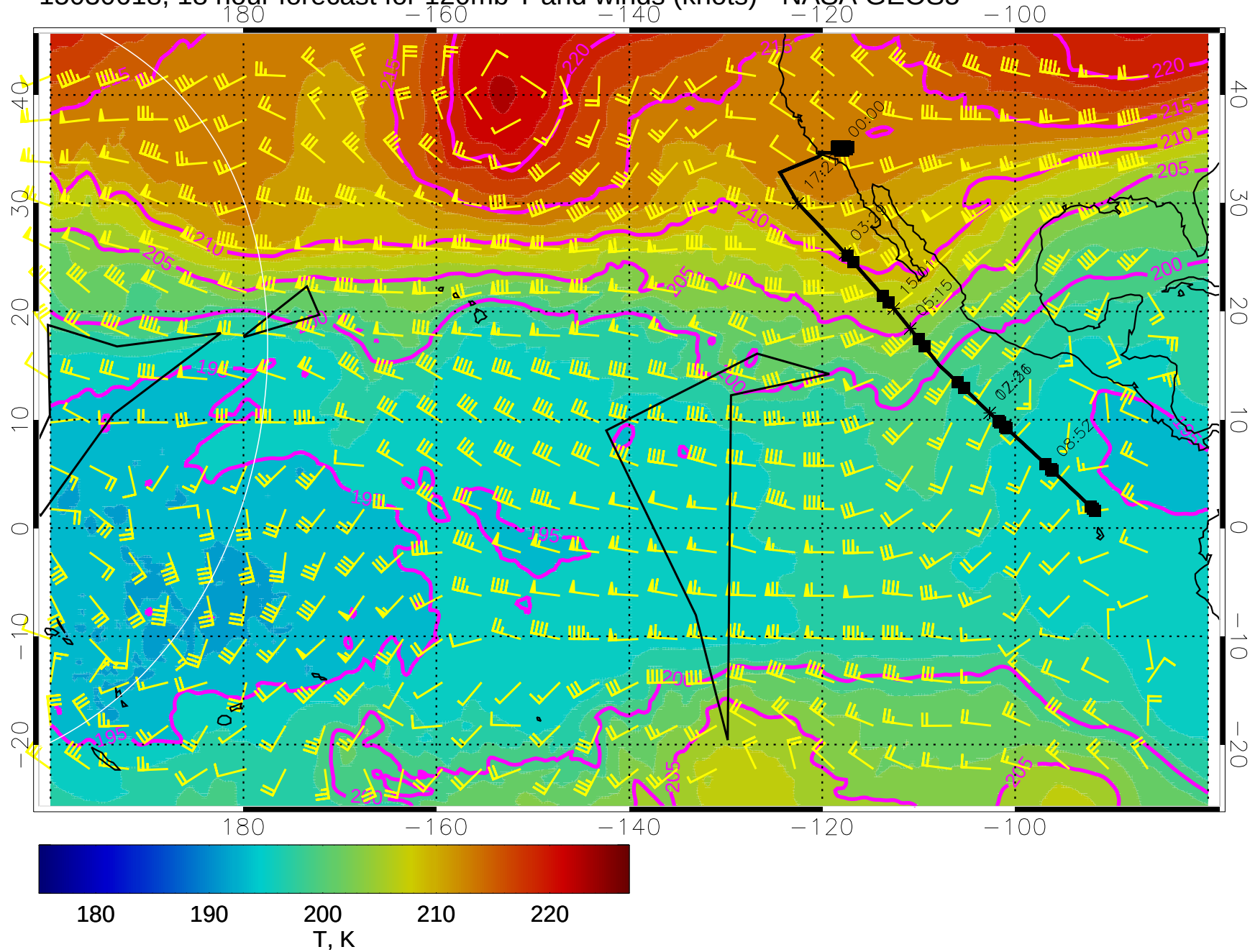
15030618, 18 hour forecast for 120mb T and winds (knots) - NASA GEOS5
