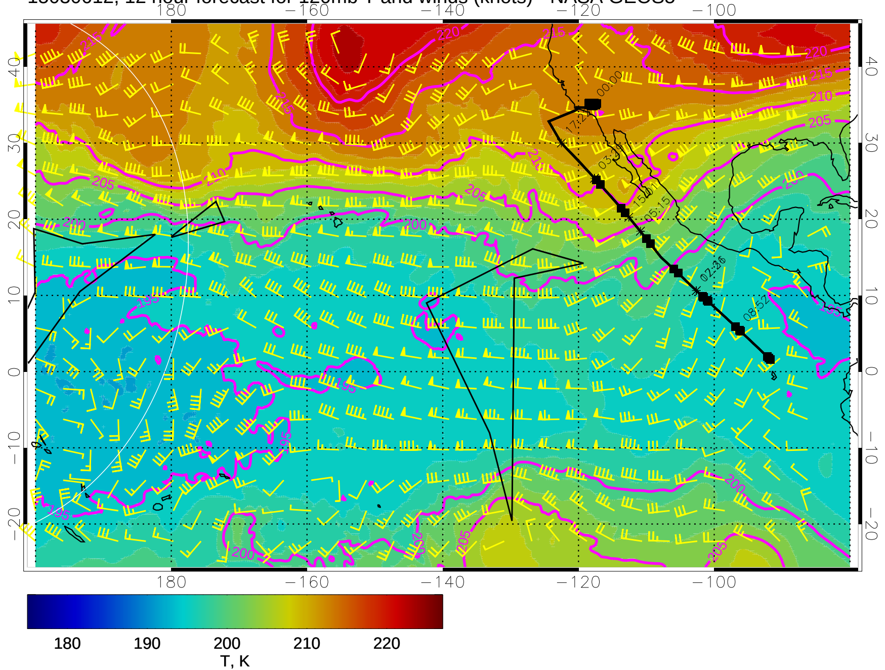
15030612, 12 hour forecast for 120mb T and winds (knots) - NASA GEOS5
