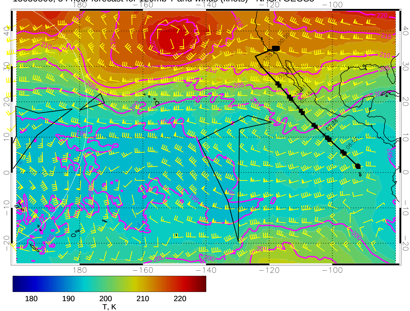
15030806, 54 hour forecast for 120mb T and winds (knots) - NASA GEOS5
