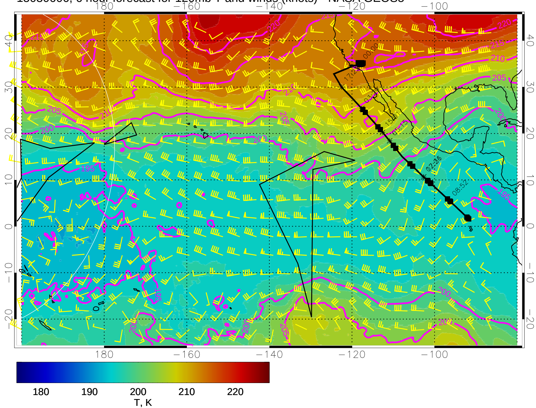
15030606, 6 hour forecast for 120mb T and winds (knots) - NASA GEOS5
