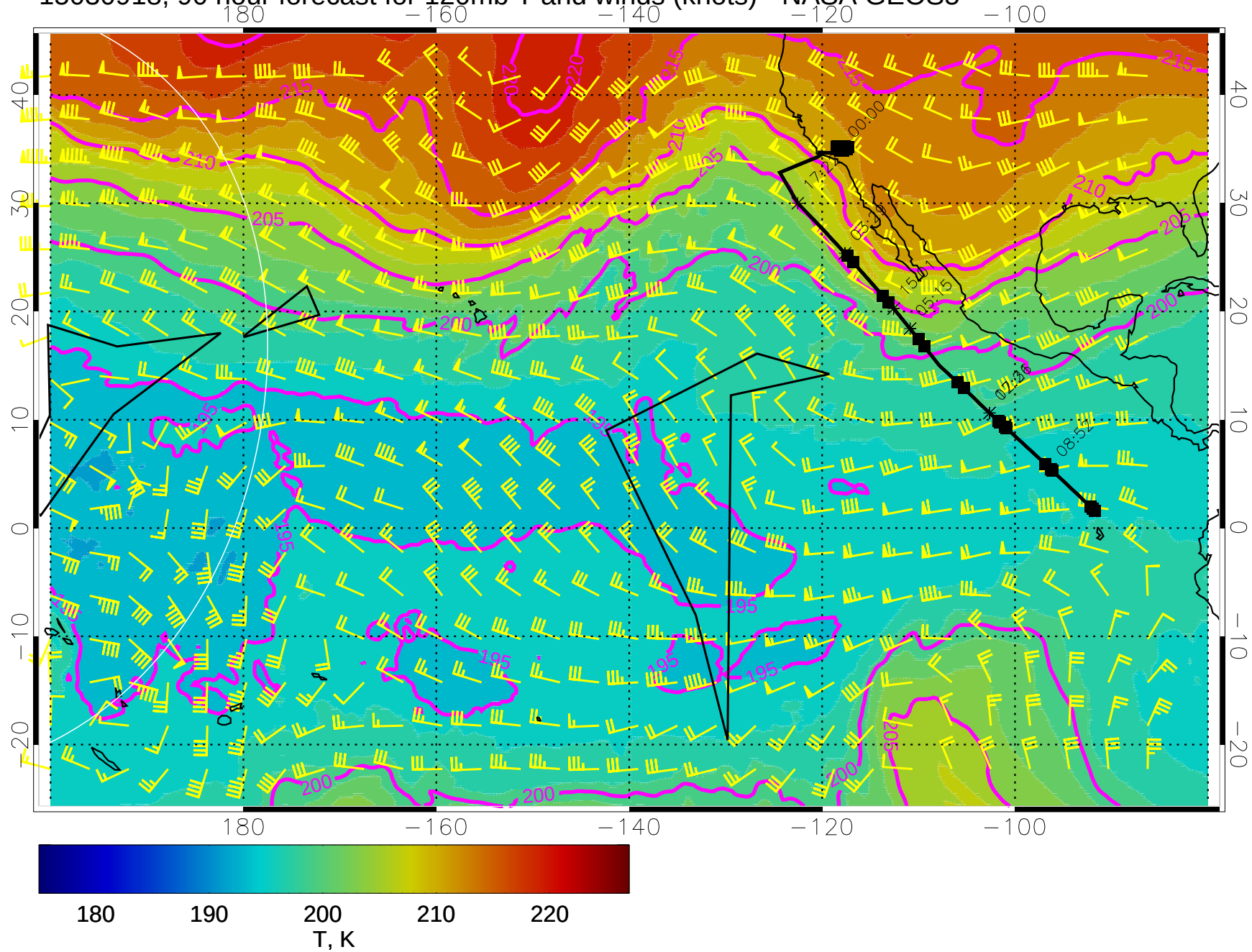
15030918, 90 hour forecast for 120mb T and winds (knots) - NASA GEOS5
