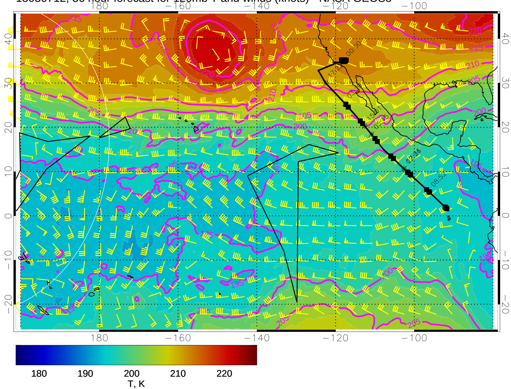
15030712, 36 hour forecast for 120mb T and winds (knots) - NASA GEOS5
