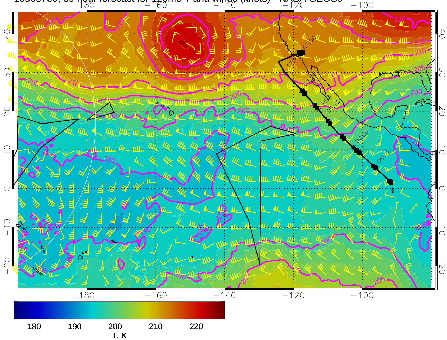
15030706, 30 hour forecast for 120mb T and winds (knots) - NASA GEOS5
