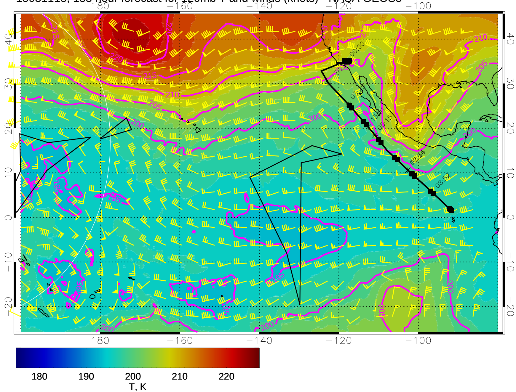
15031118, 138 hour forecast for 120mb T and winds (knots) - NASA GEOS5
