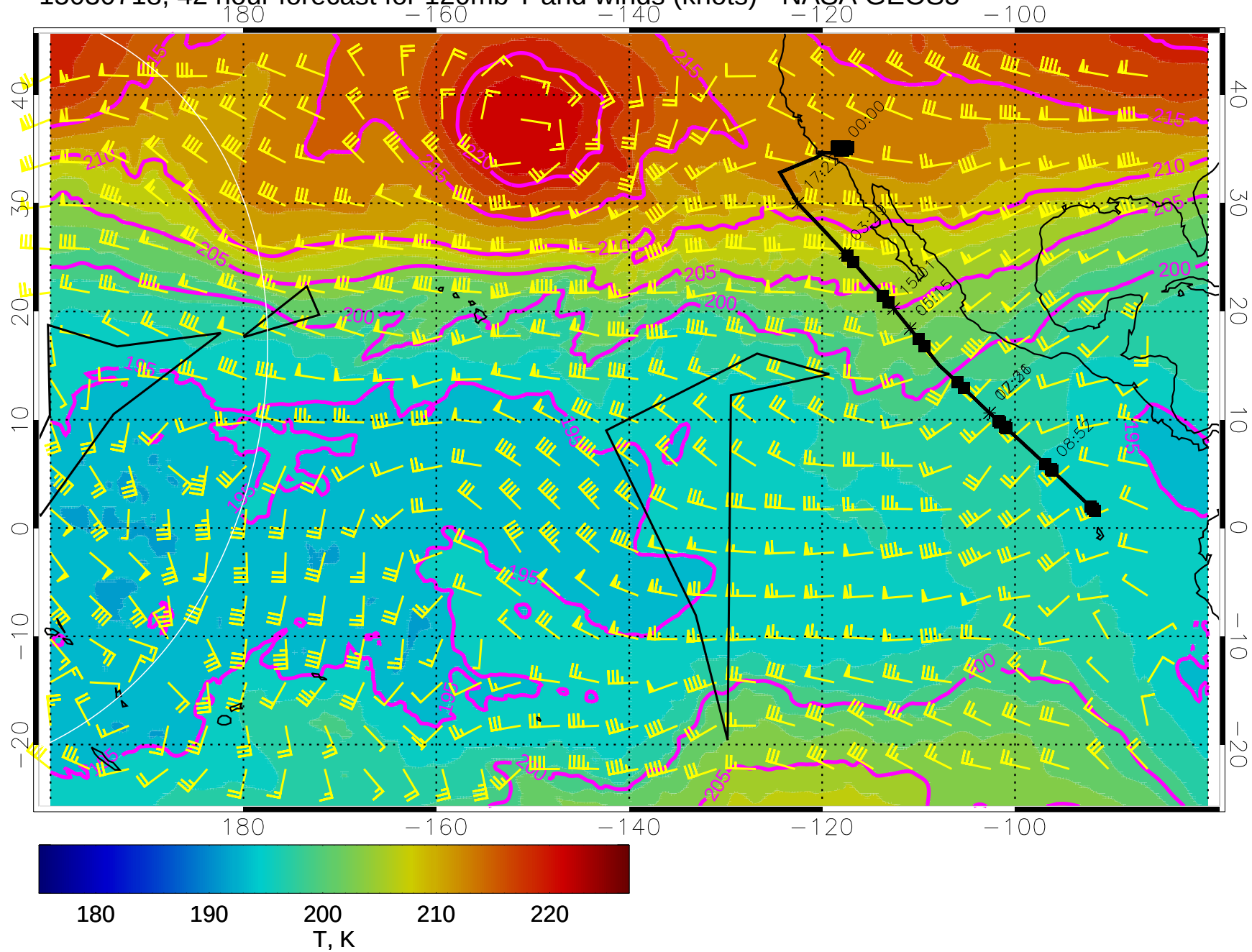
15030718, 42 hour forecast for 120mb T and winds (knots) - NASA GEOS5
