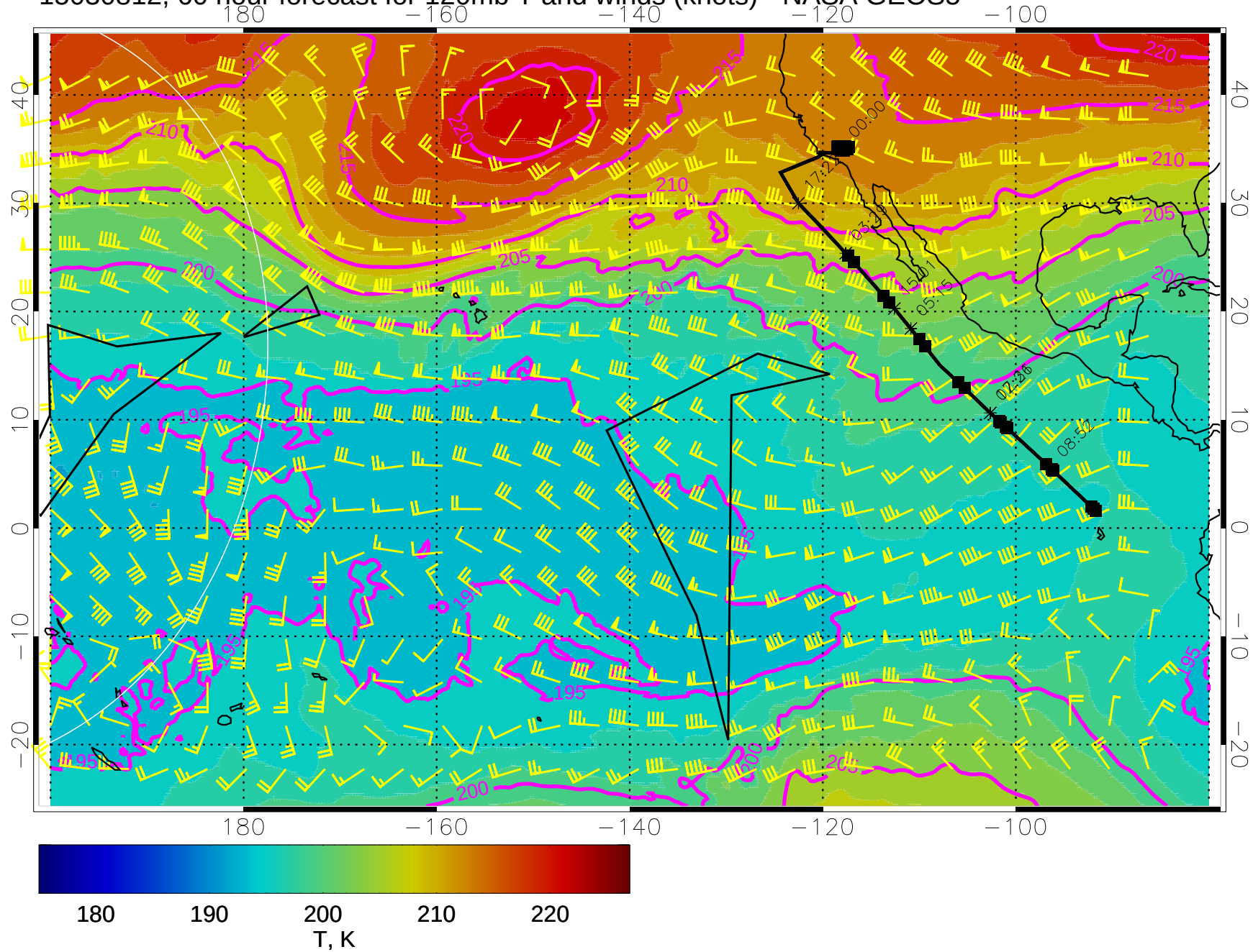
15030812, 60 hour forecast for 120mb T and winds (knots) - NASA GEOS5
