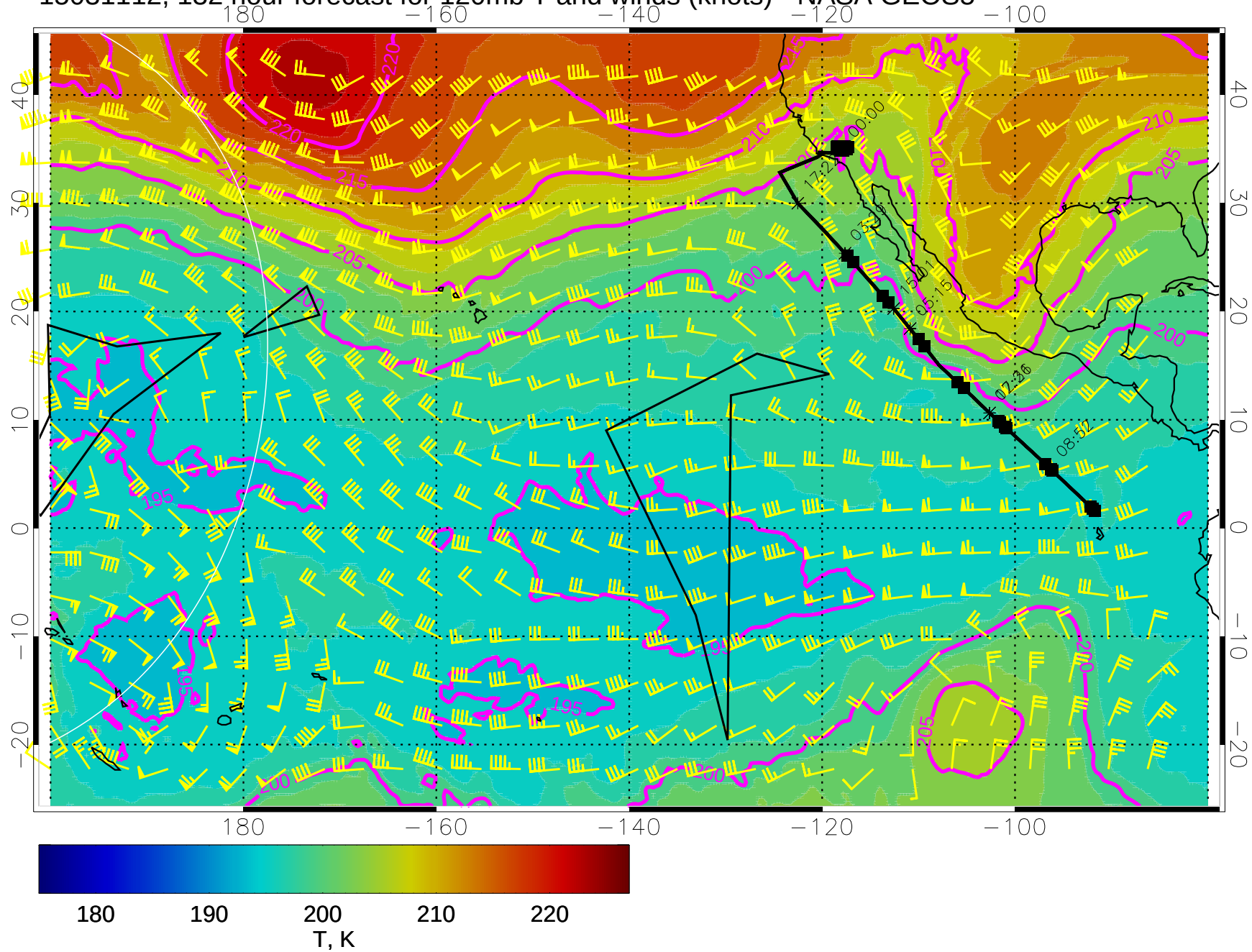
15031112, 132 hour forecast for 120mb T and winds (knots) - NASA GEOS5
