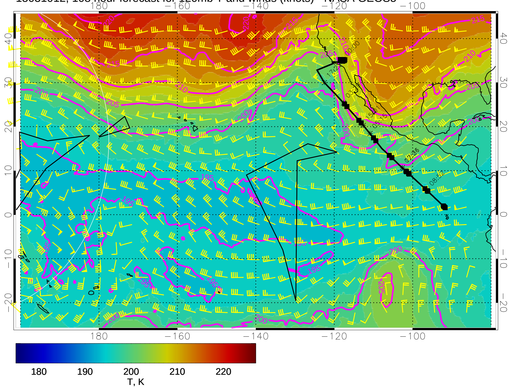
15031012, 108 hour forecast for 120mb T and winds (knots) - NASA GEOS5
