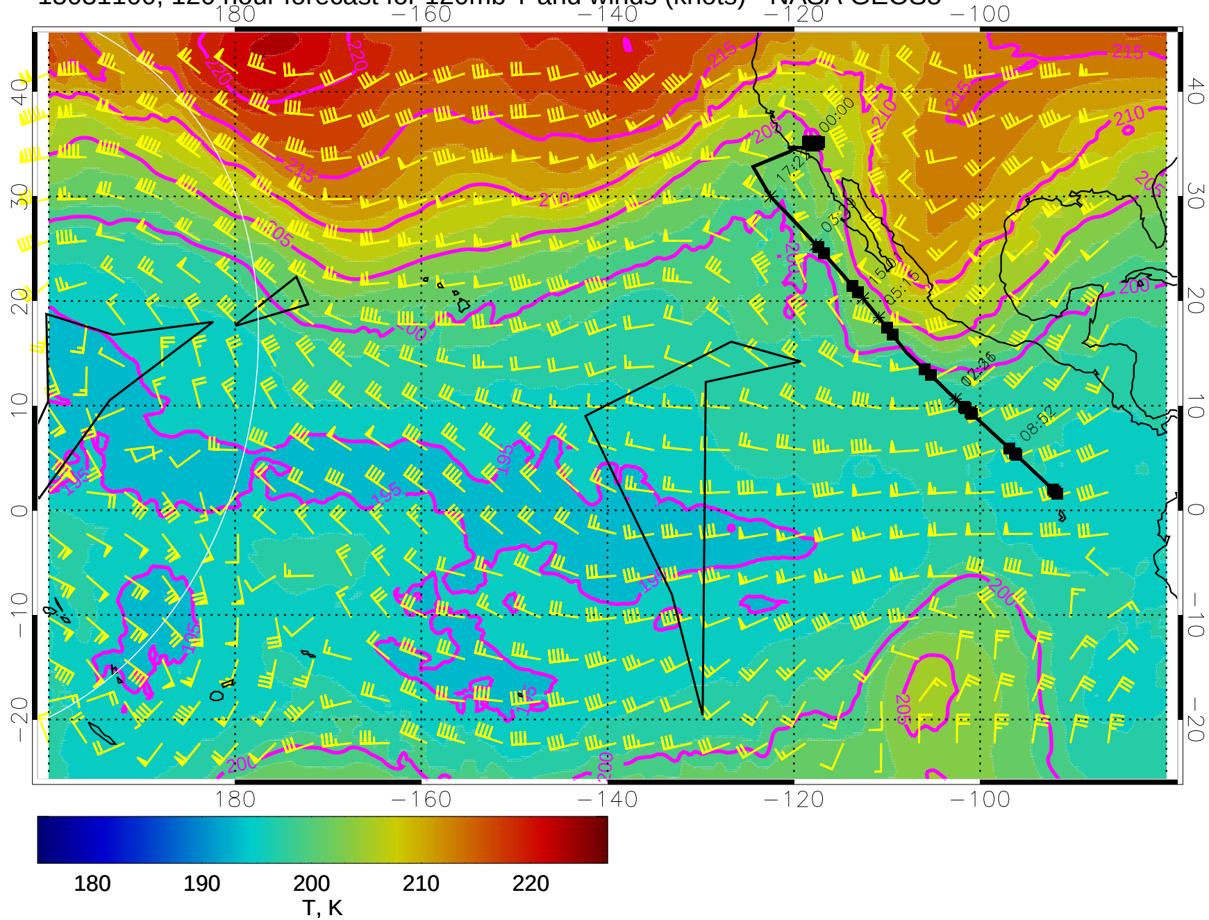
15031100, 120 hour forecast for 120mb T and winds (knots) - NASA GEOS5
