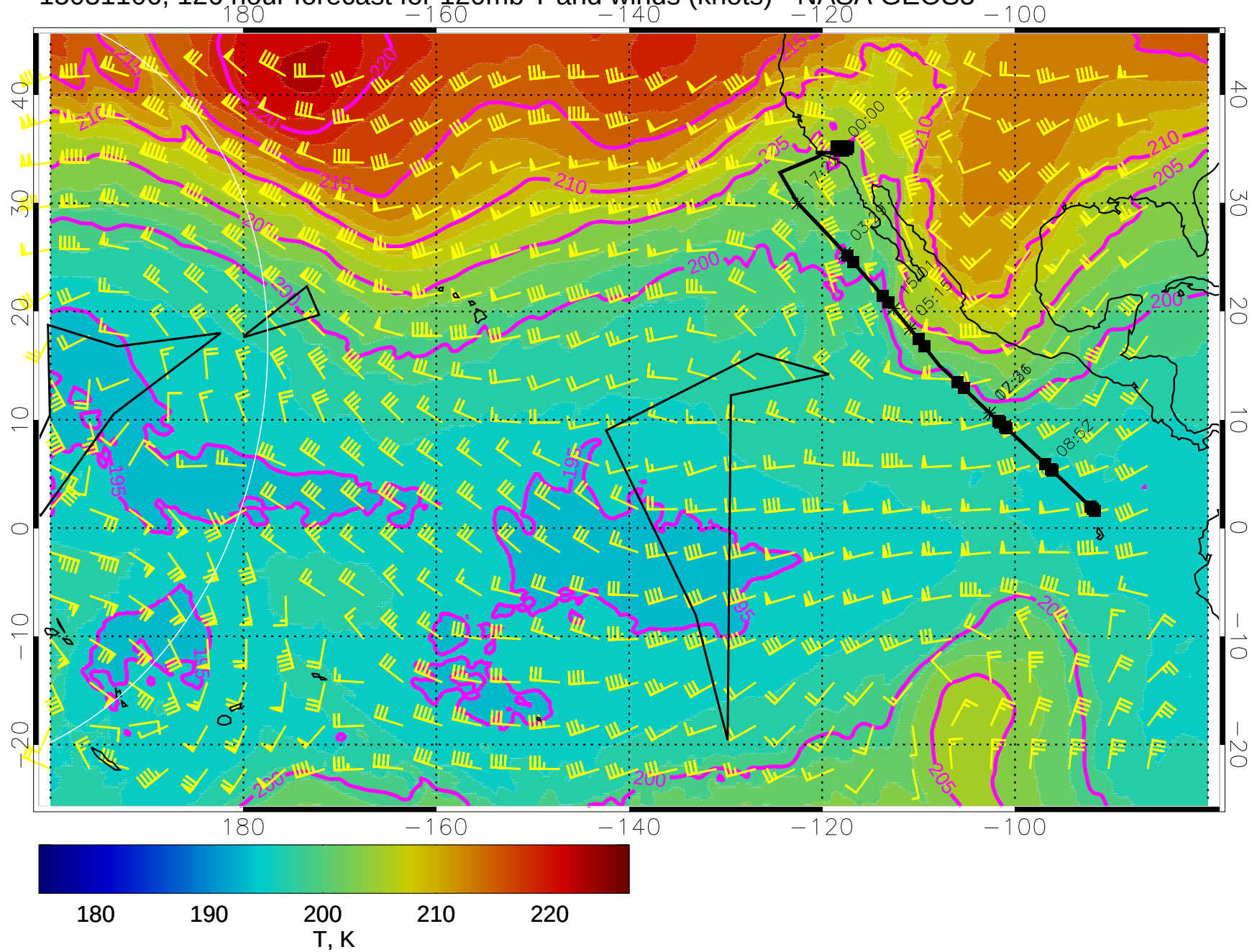
15031106, 126 hour forecast for 120mb T and winds (knots) - NASA GEOS5
