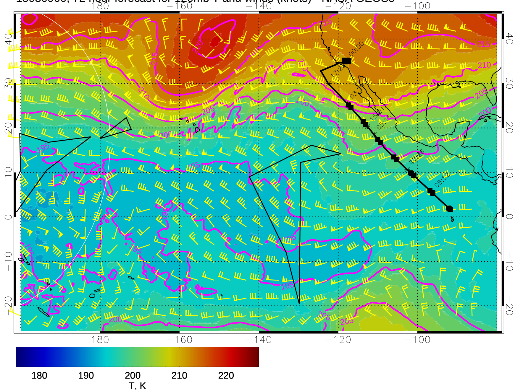
15030900, 72 hour forecast for 120mb T and winds (knots) - NASA GEOS5
