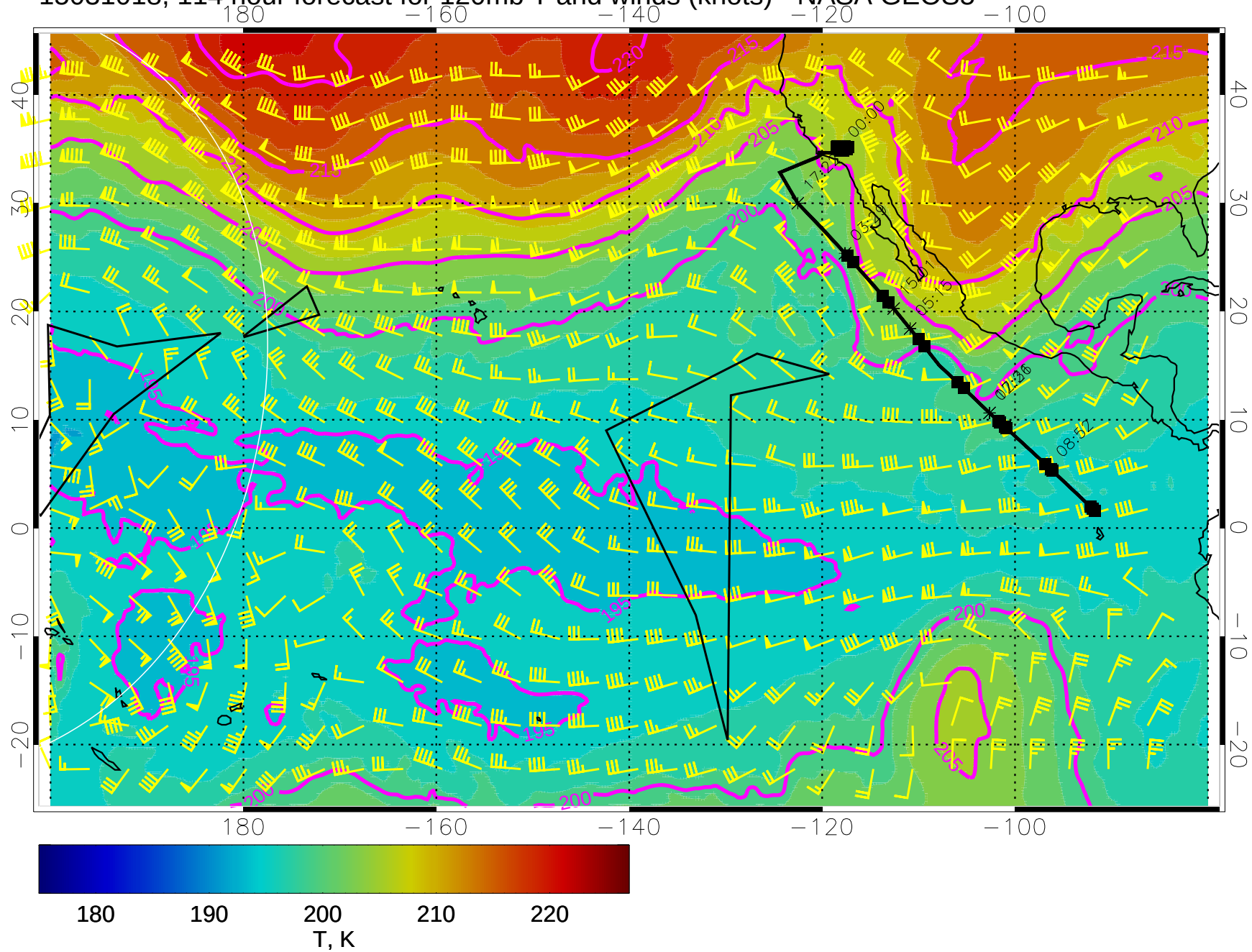
15031018, 114 hour forecast for 120mb T and winds (knots) - NASA GEOS5
