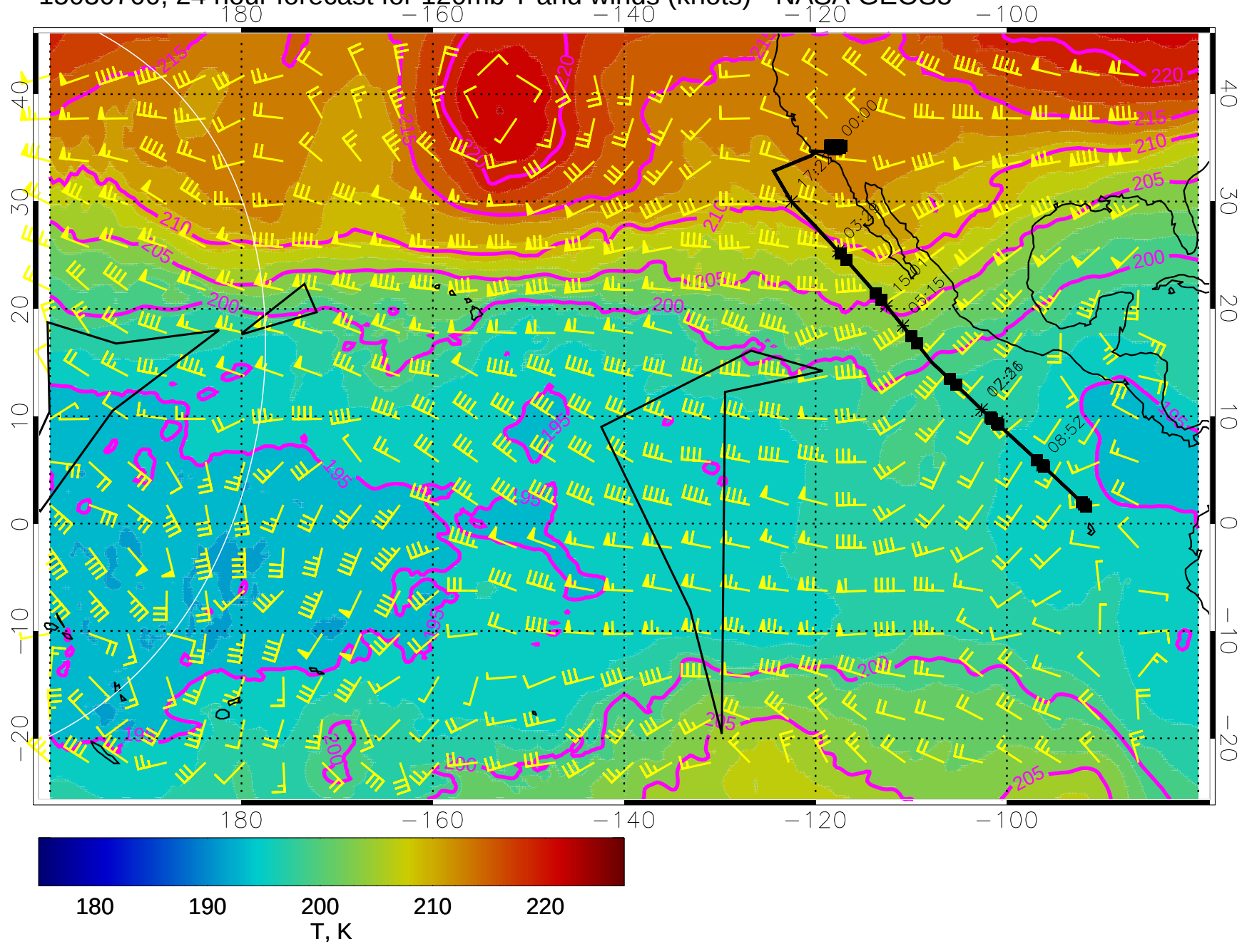
15030700, 24 hour forecast for 120mb T and winds (knots) - NASA GEOS5
