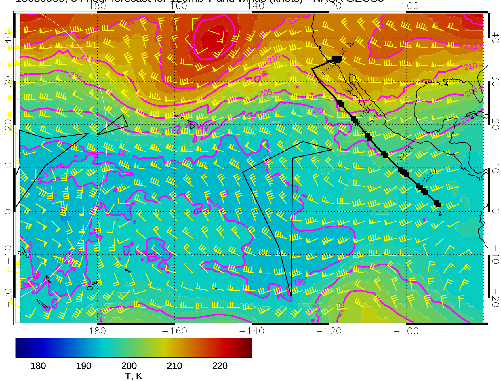
15030900, 84 hour forecast for 120mb T and winds (knots) - NASA GEOS5
