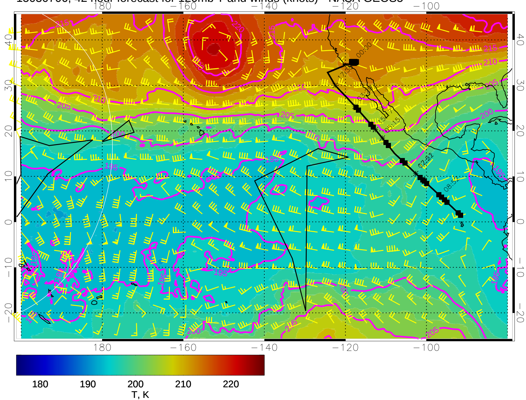
15030706, 42 hour forecast for 120mb T and winds (knots) - NASA GEOS5
