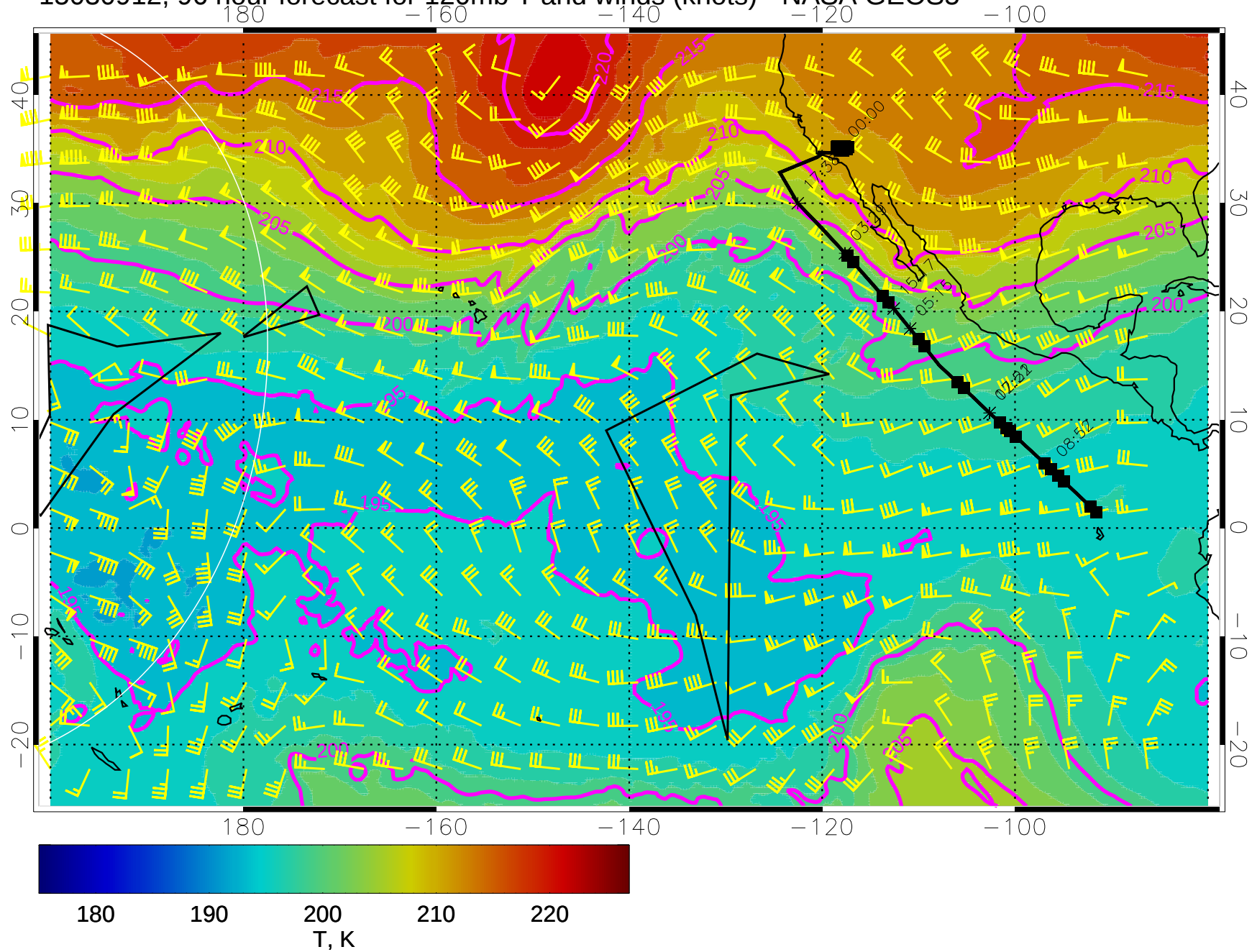
15030912, 96 hour forecast for 120mb T and winds (knots) - NASA GEOS5
