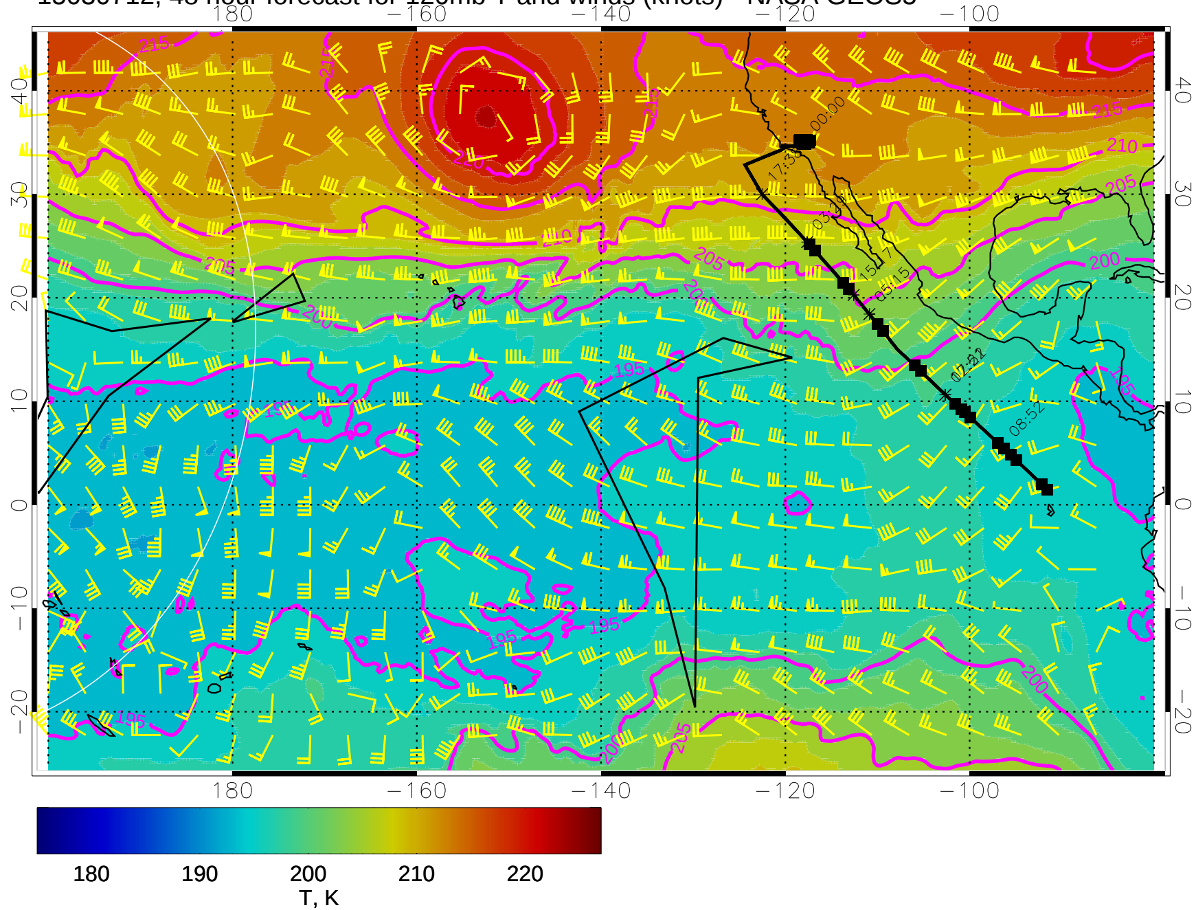
15030712, 48 hour forecast for 120mb T and winds (knots) - NASA GEOS5
