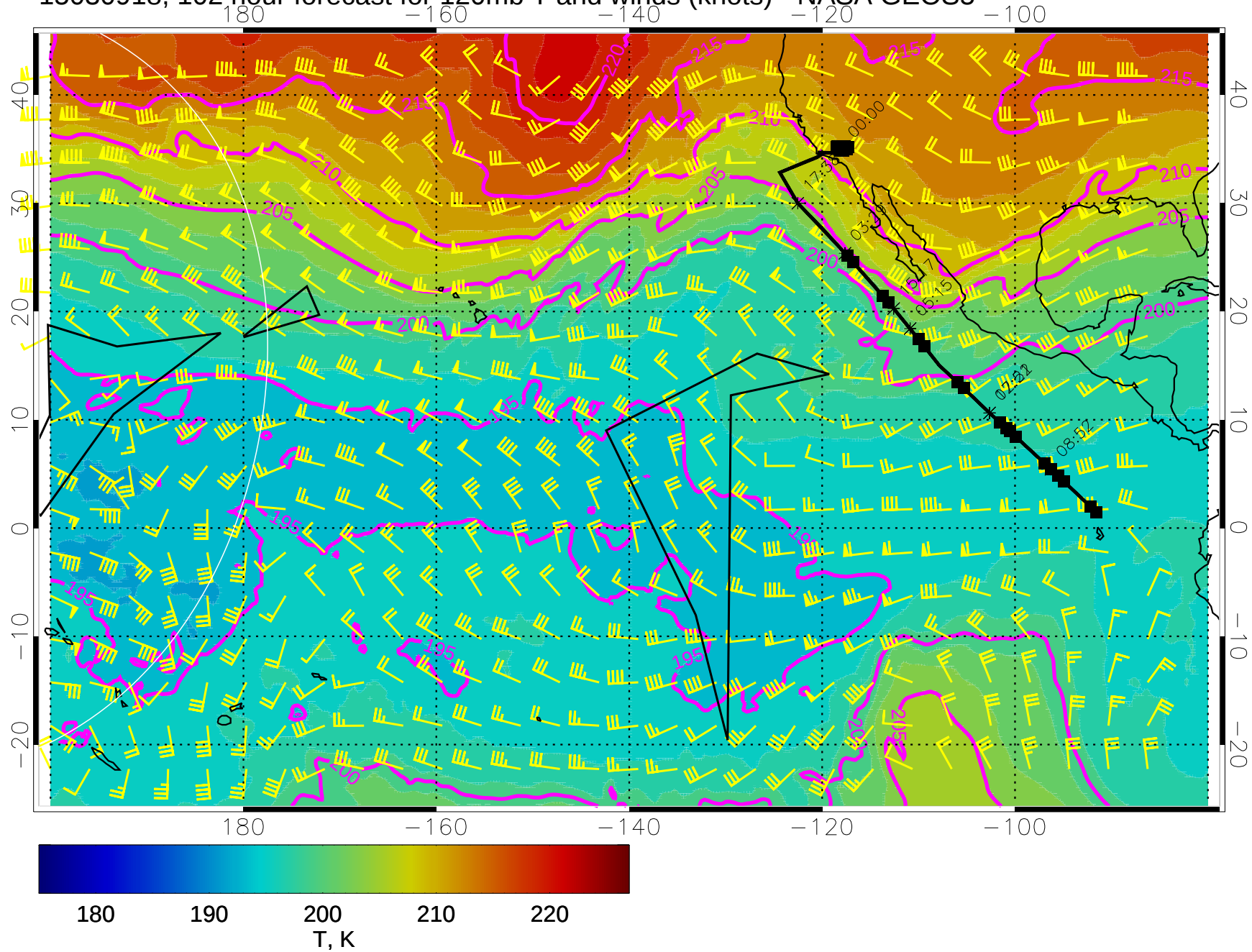
15030918, 102 hour forecast for 120mb T and winds (knots) - NASA GEOS5
