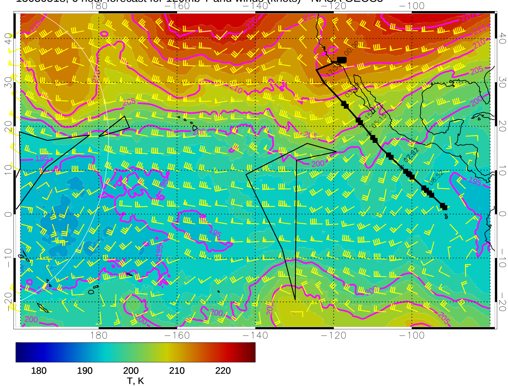
15030518, 6 hour forecast for 120mb T and winds (knots) - NASA GEOS5
