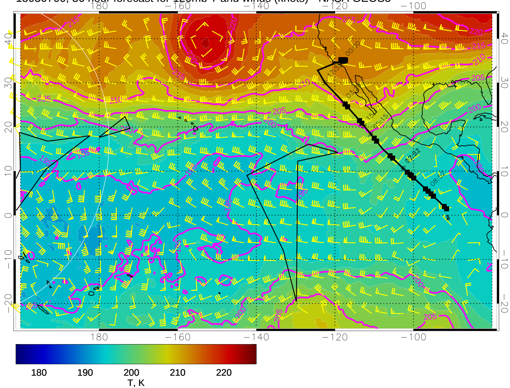
15030700, 36 hour forecast for 120mb T and winds (knots) - NASA GEOS5
