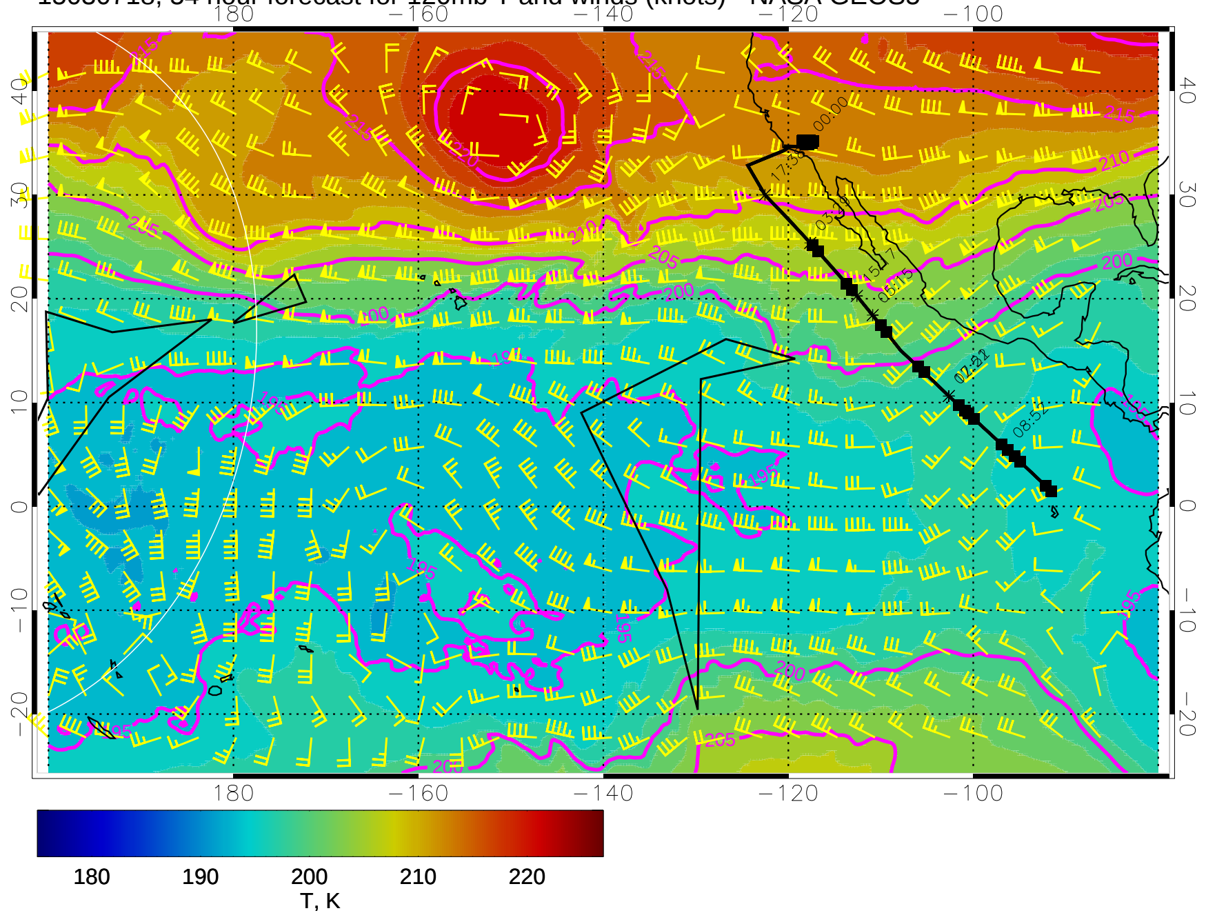
15030718, 54 hour forecast for 120mb T and winds (knots) - NASA GEOS5
