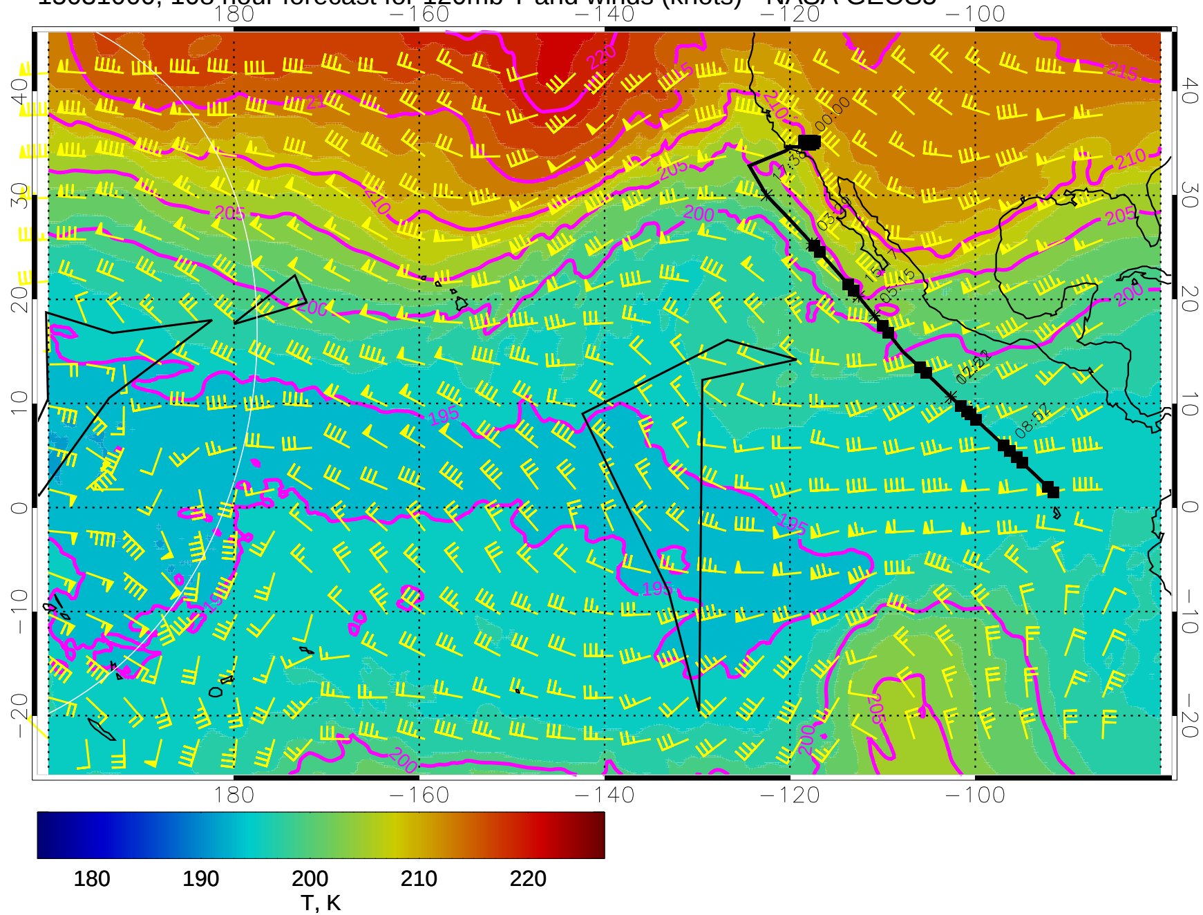
15031000, 108 hour forecast for 120mb T and winds (knots) - NASA GEOS5
