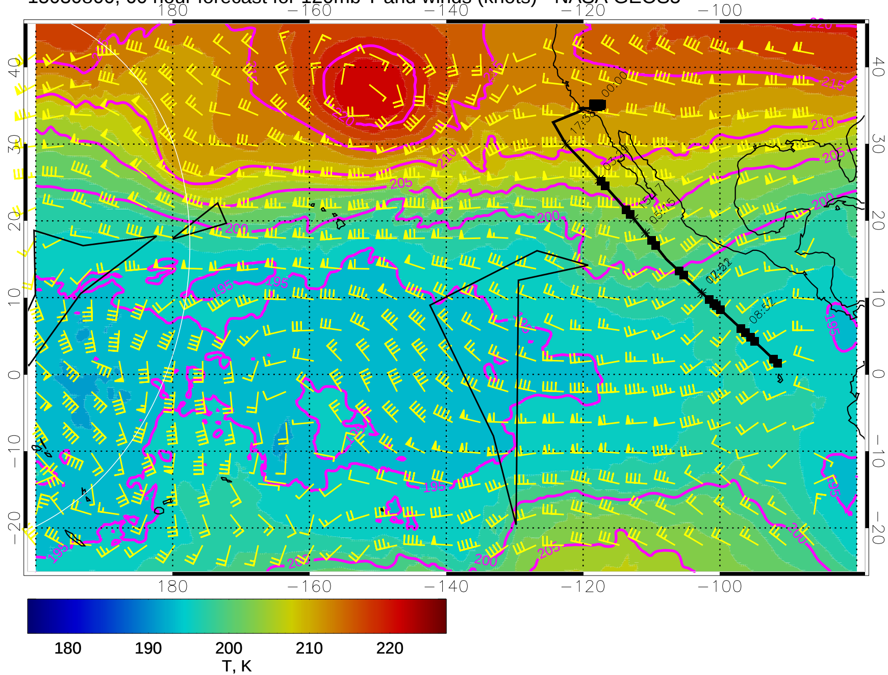
15030800, 60 hour forecast for 120mb T and winds (knots) - NASA GEOS5
