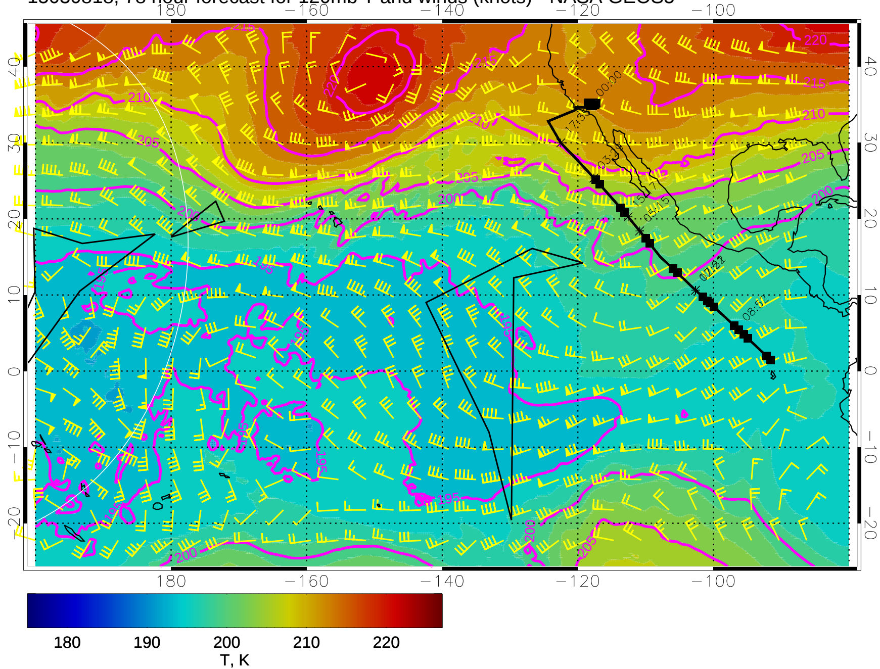
15030818, 78 hour forecast for 120mb T and winds (knots) - NASA GEOS5
