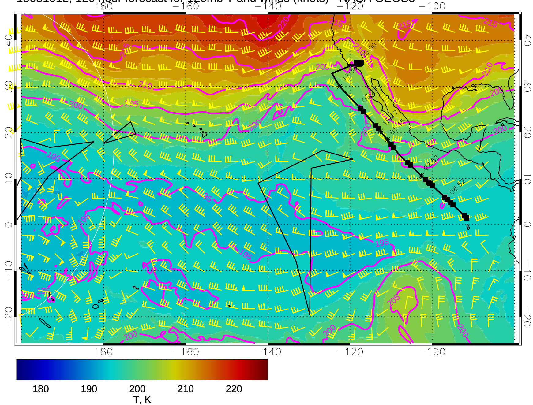
15031012, 120 hour forecast for 120mb T and winds (knots) - NASA GEOS5
