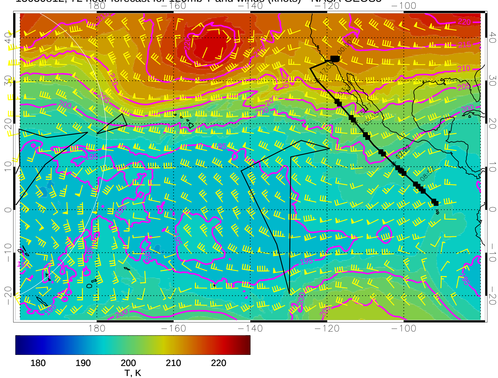
15030812, 72 hour forecast for 120mb T and winds (knots) - NASA GEOS5
