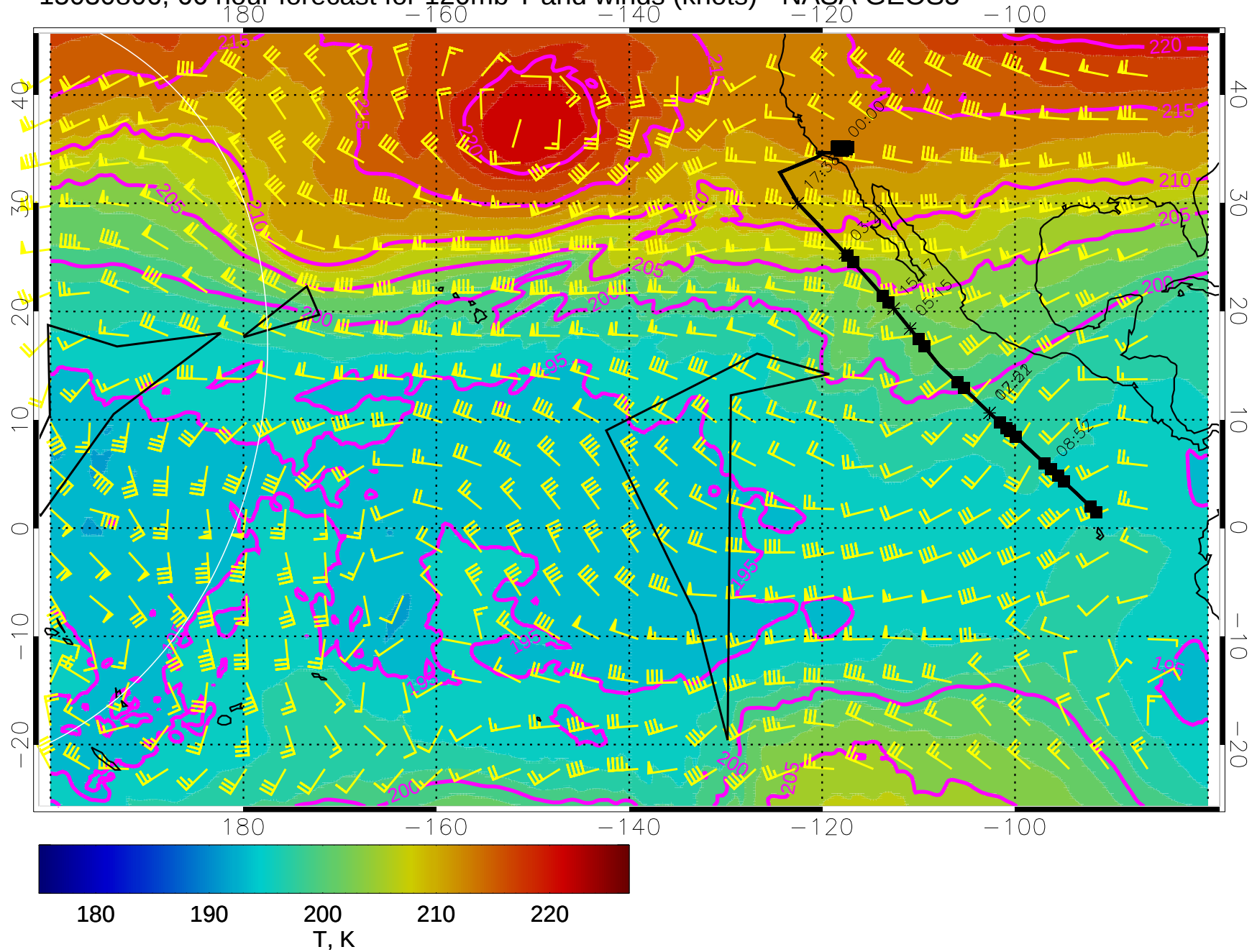
15030806, 66 hour forecast for 120mb T and winds (knots) - NASA GEOS5
