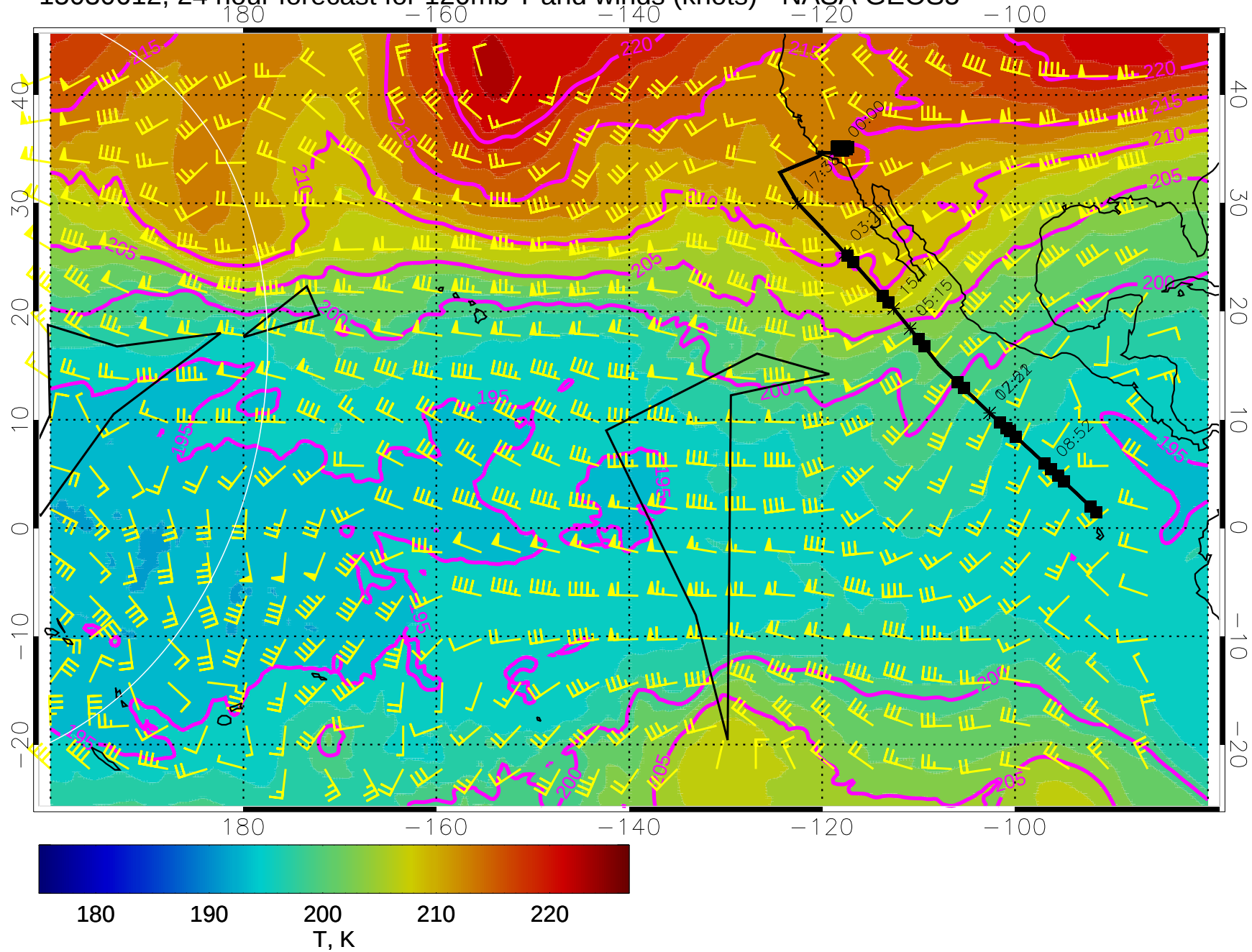
15030612, 24 hour forecast for 120mb T and winds (knots) - NASA GEOS5
