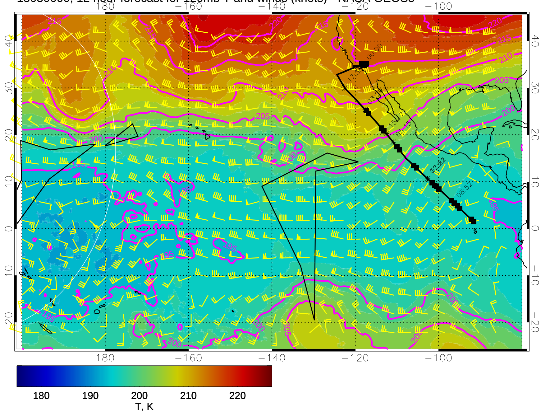
15030600, 12 hour forecast for 120mb T and winds (knots) - NASA GEOS5
