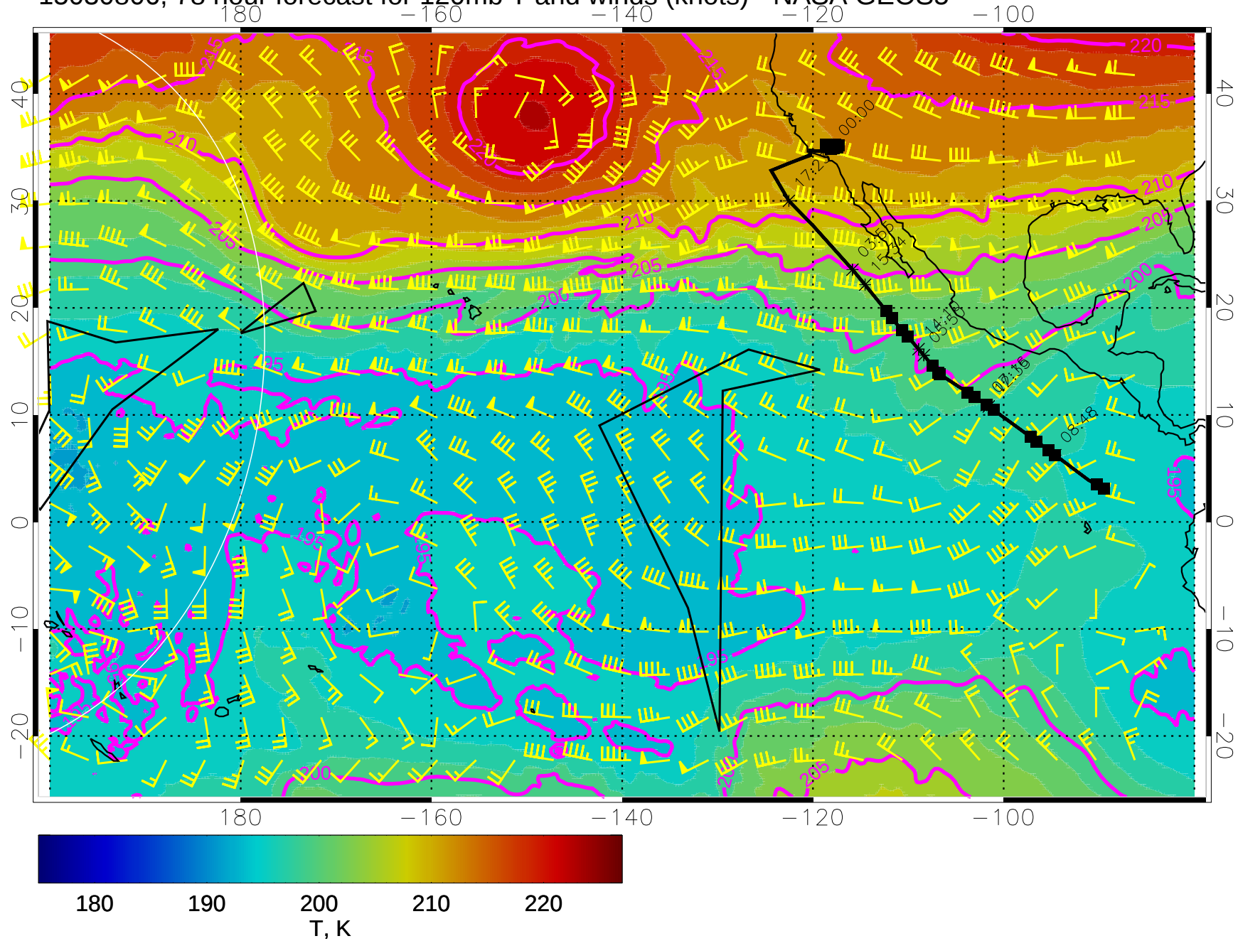
15030806, 78 hour forecast for 120mb T and winds (knots) - NASA GEOS5
