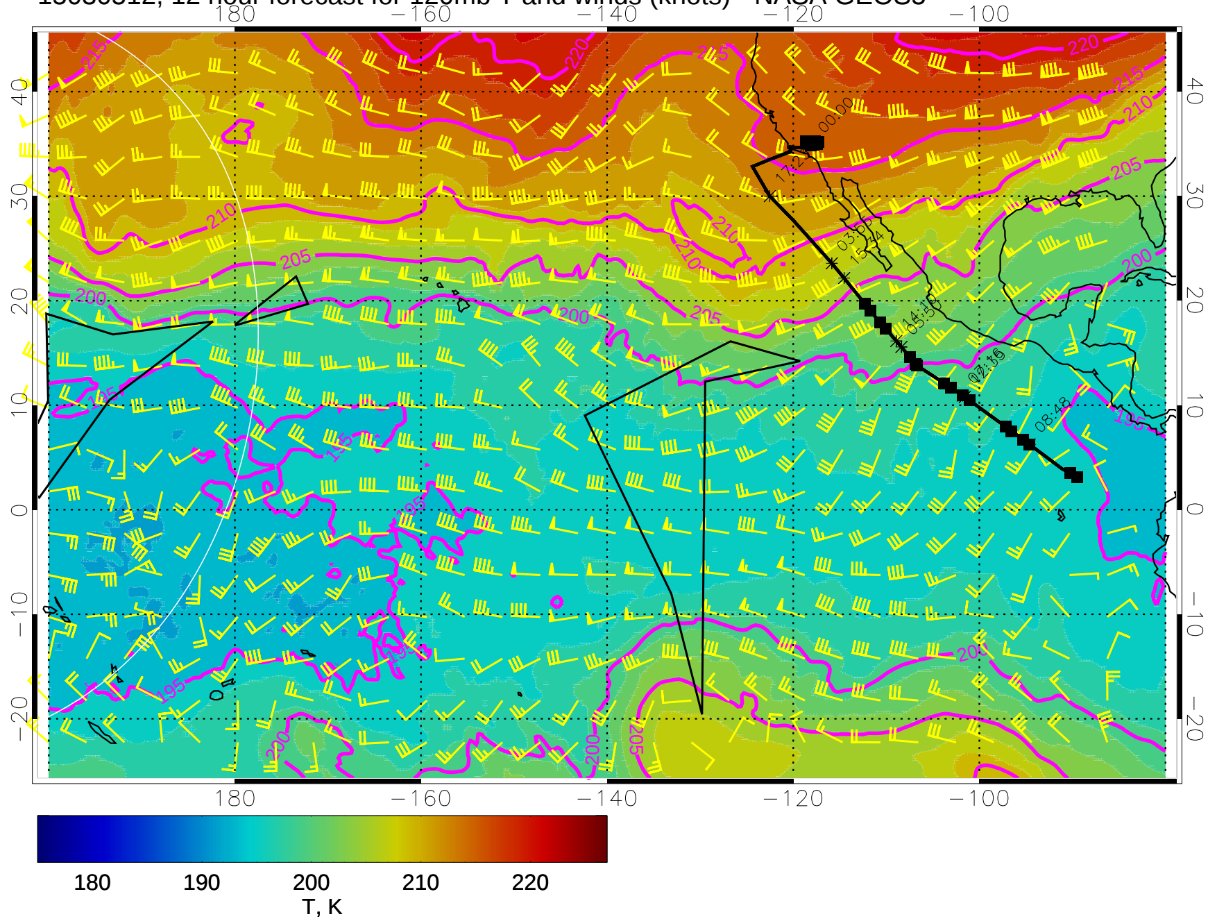
15030512, 12 hour forecast for 120mb T and winds (knots) - NASA GEOS5
