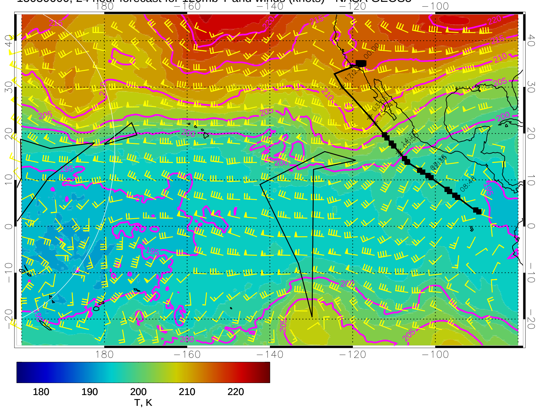
15030600, 24 hour forecast for 120mb T and winds (knots) - NASA GEOS5
