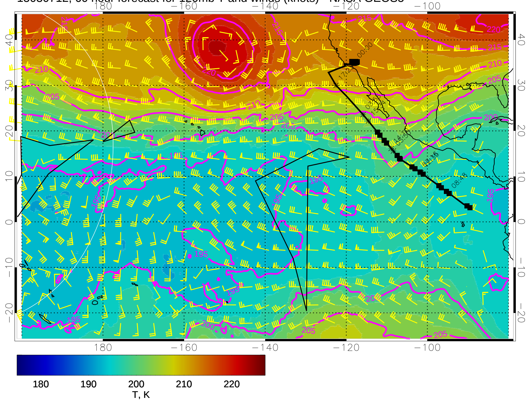
15030712, 60 hour forecast for 120mb T and winds (knots) - NASA GEOS5
