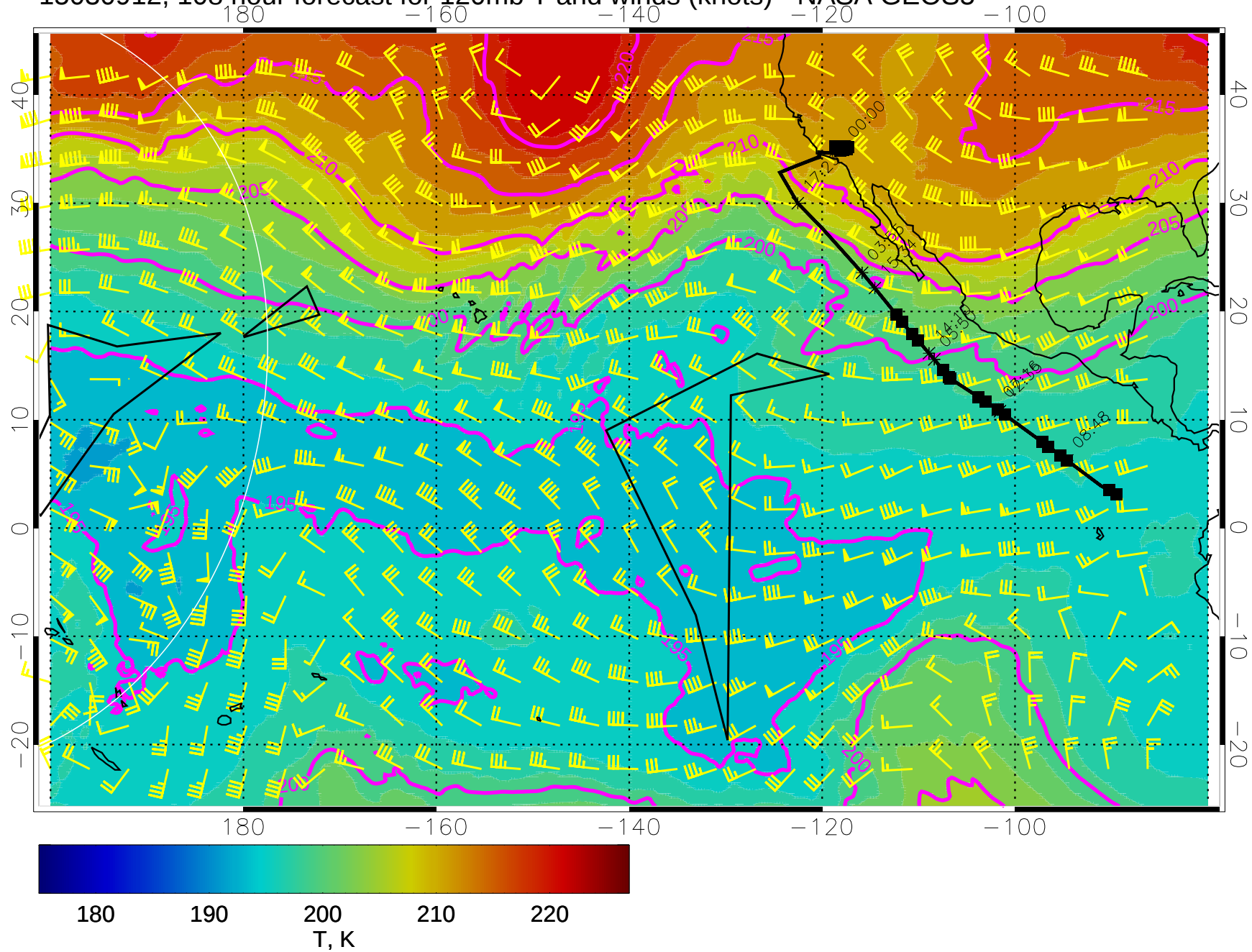
15030912, 108 hour forecast for 120mb T and winds (knots) - NASA GEOS5
