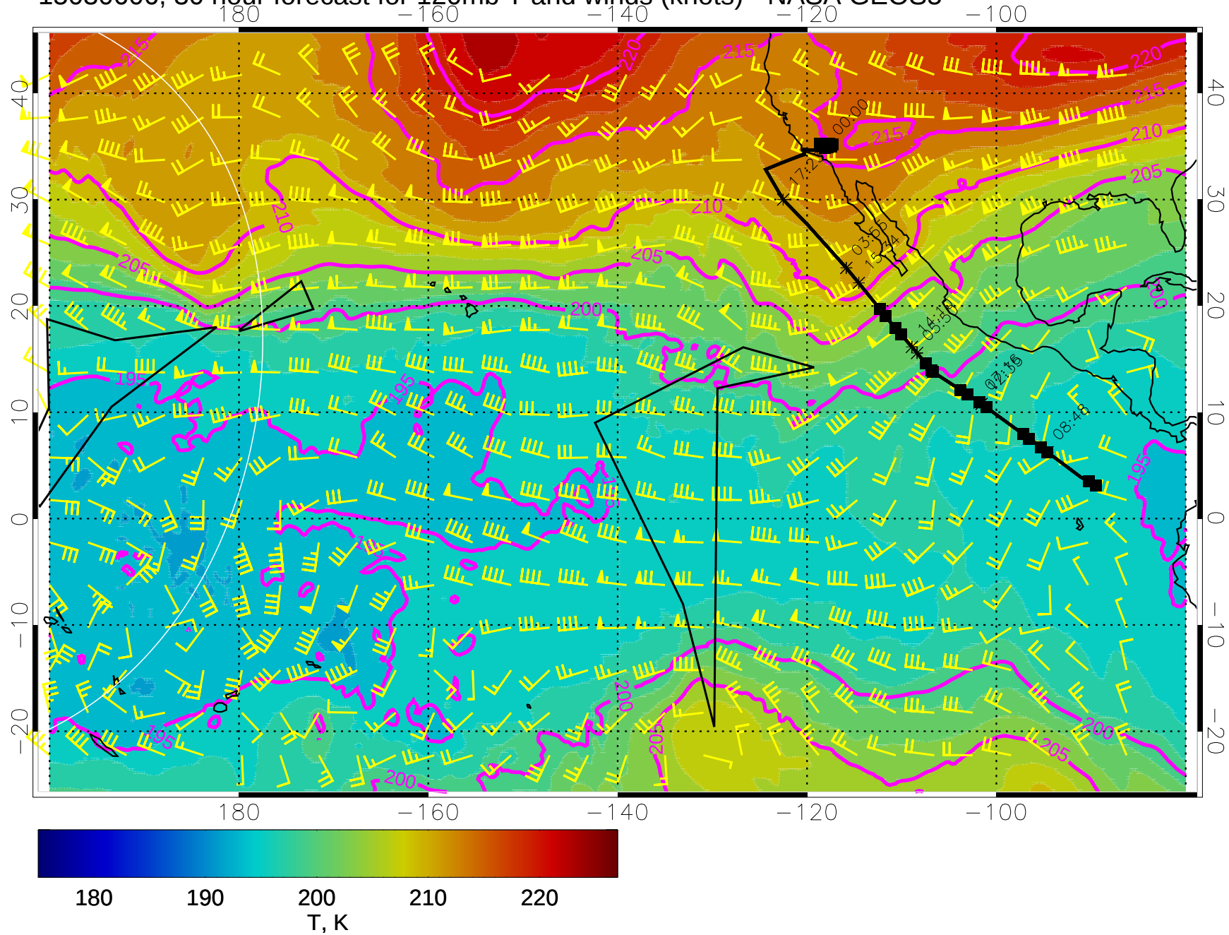
15030606, 30 hour forecast for 120mb T and winds (knots) - NASA GEOS5
