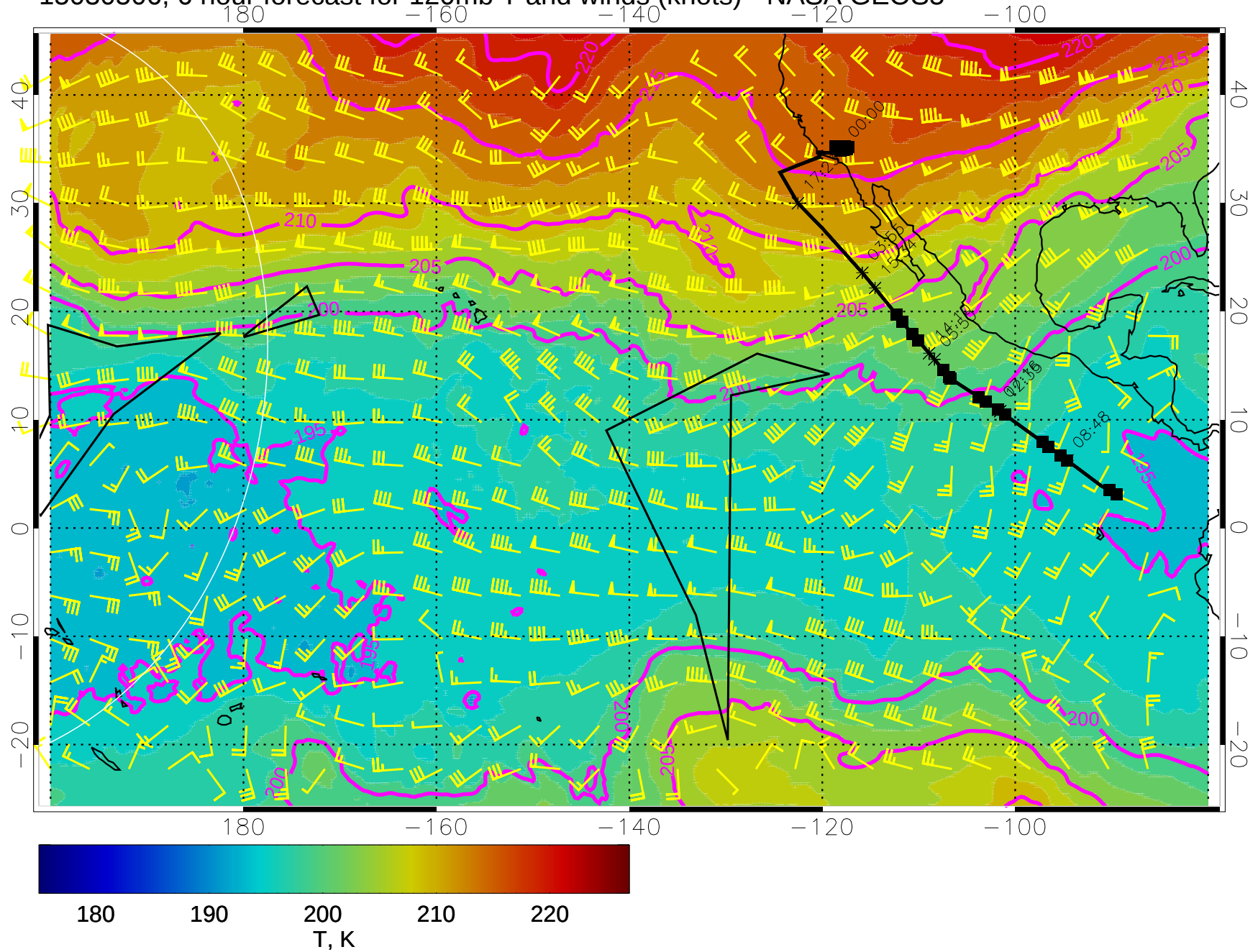
15030506, 6 hour forecast for 120mb T and winds (knots) - NASA GEOS5
