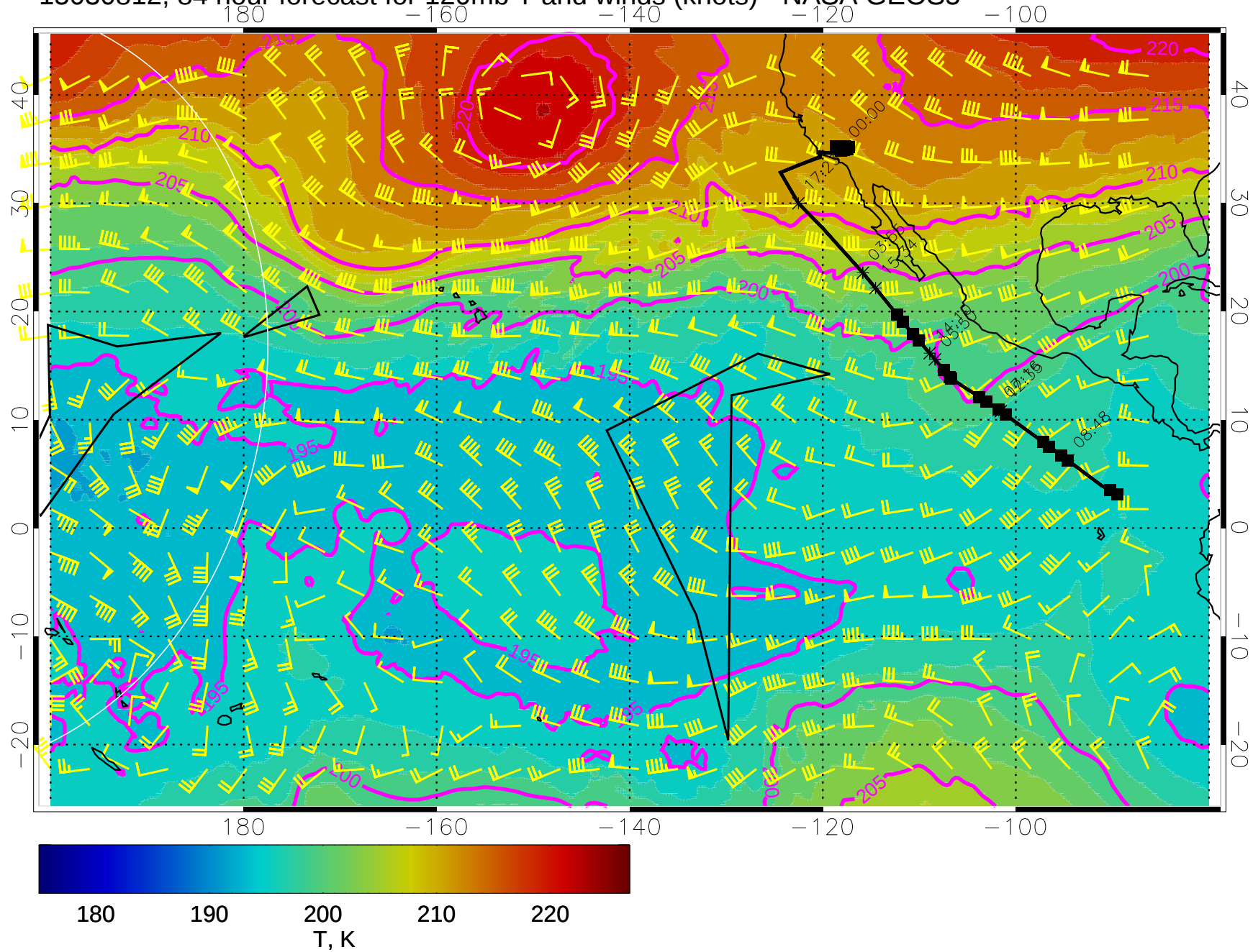
15030812, 84 hour forecast for 120mb T and winds (knots) - NASA GEOS5
