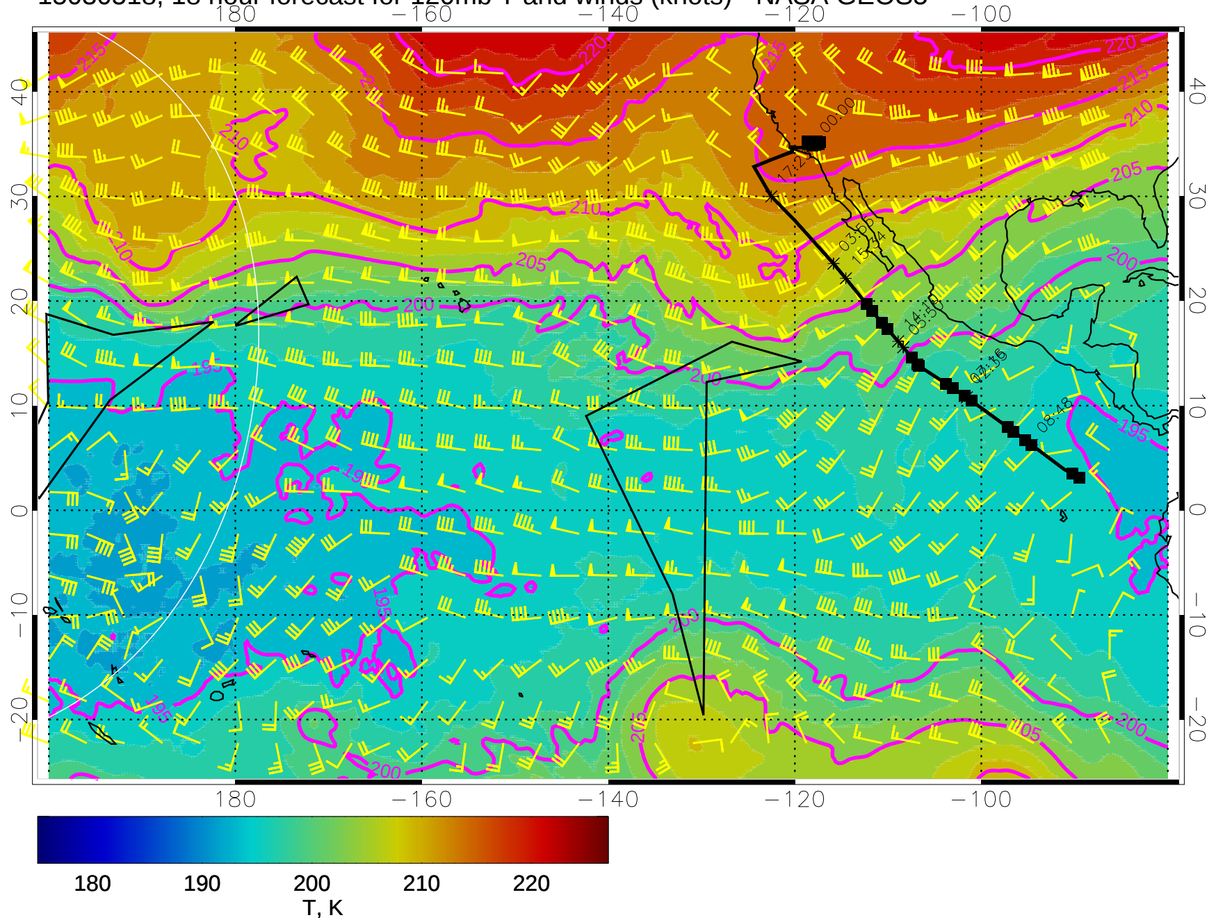
15030518, 18 hour forecast for 120mb T and winds (knots) - NASA GEOS5
