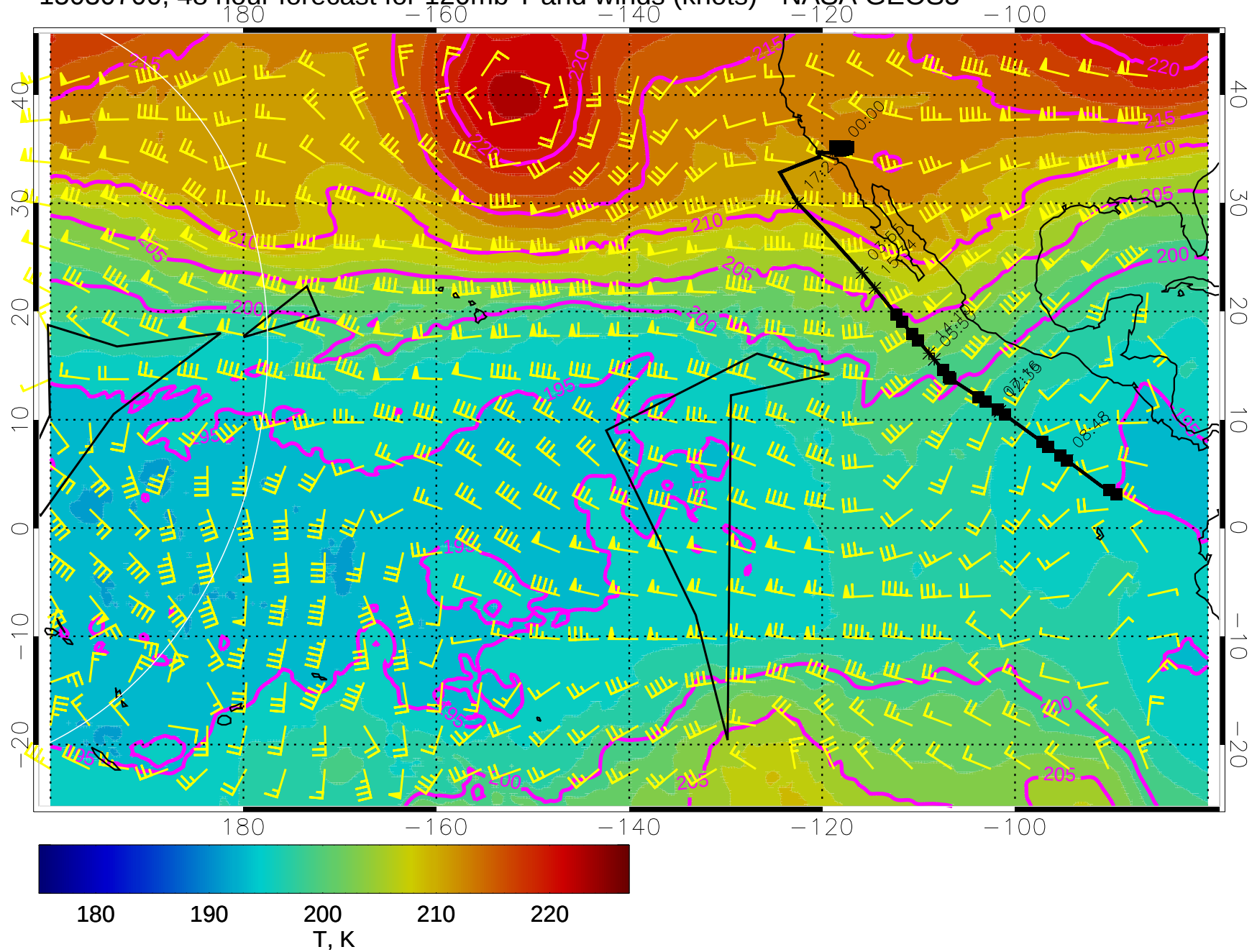
15030700, 48 hour forecast for 120mb T and winds (knots) - NASA GEOS5
