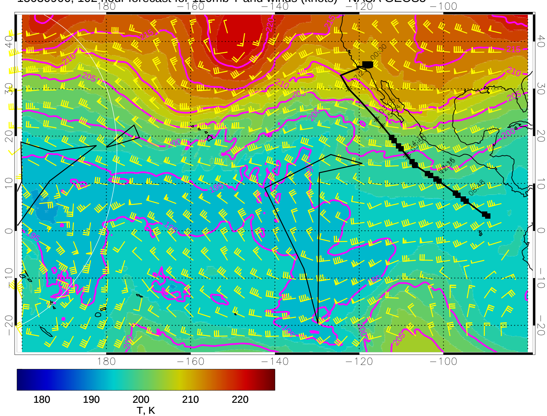
15030906, 102 hour forecast for 120mb T and winds (knots) - NASA GEOS5
