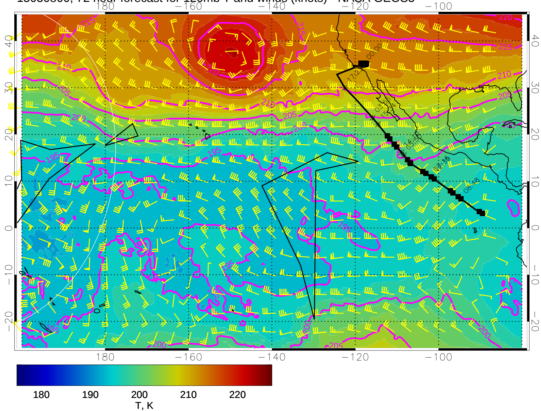
15030800, 72 hour forecast for 120mb T and winds (knots) - NASA GEOS5
