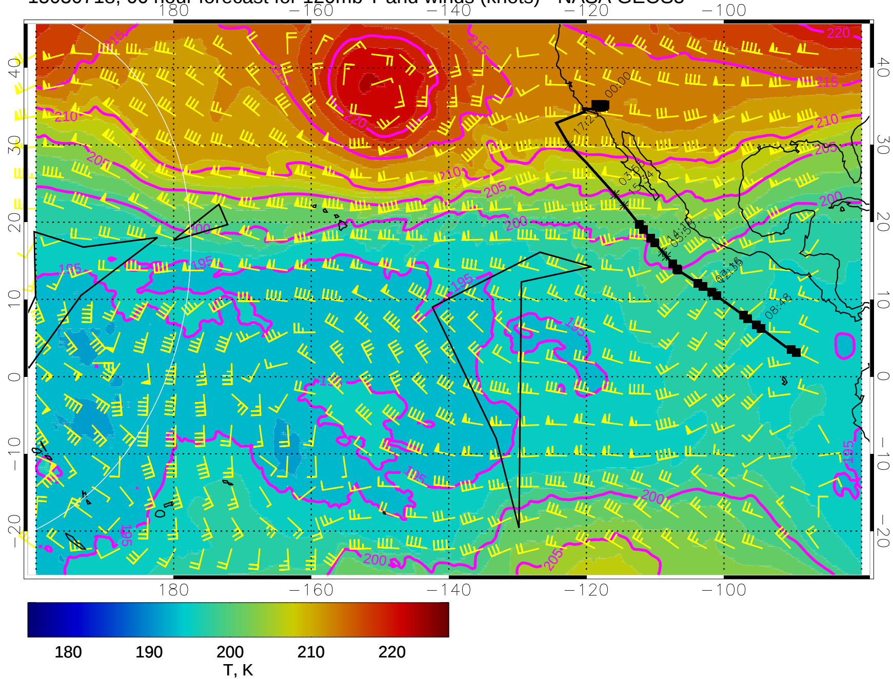
15030718, 66 hour forecast for 120mb T and winds (knots) - NASA GEOS5
