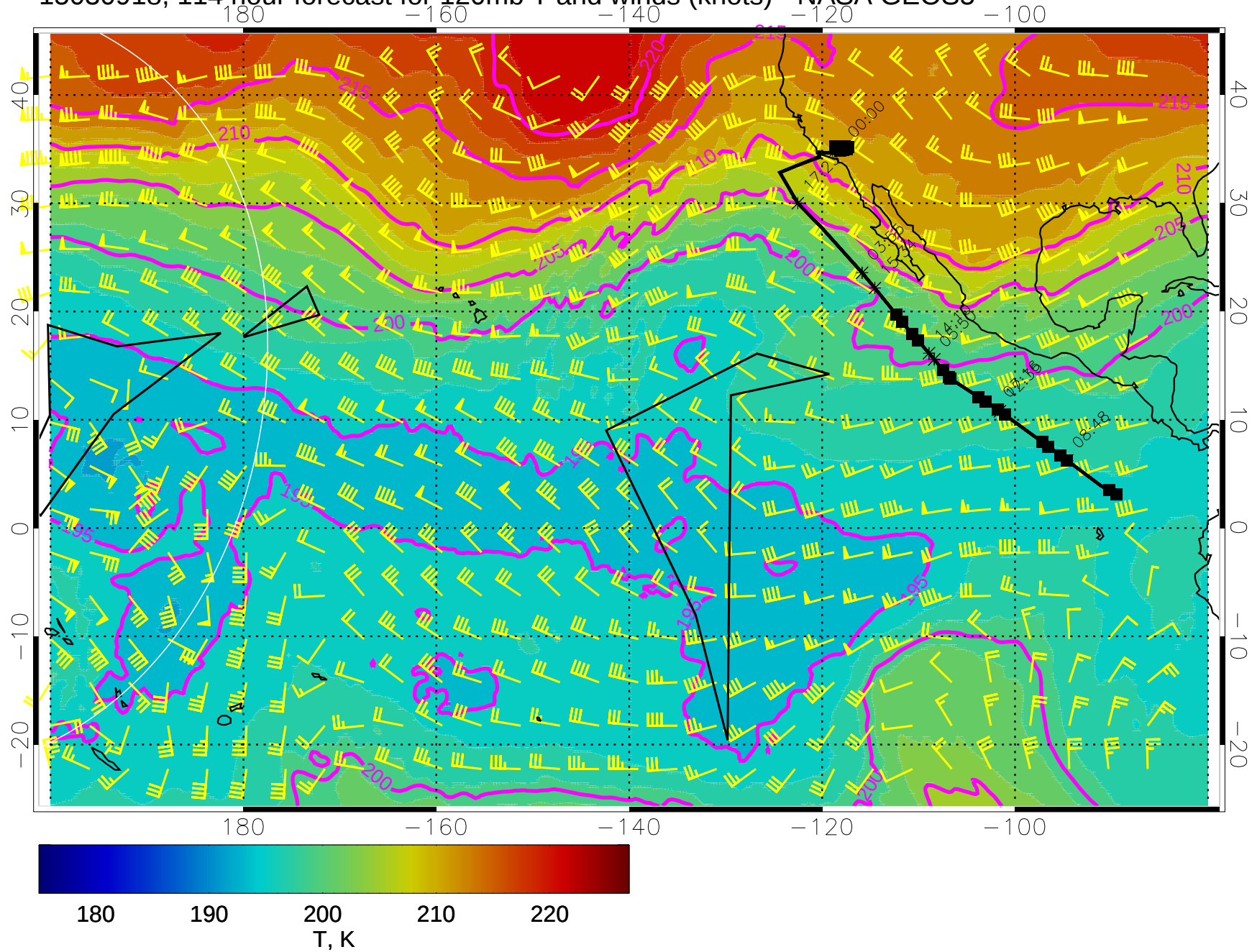
15030918, 114 hour forecast for 120mb T and winds (knots) - NASA GEOS5
