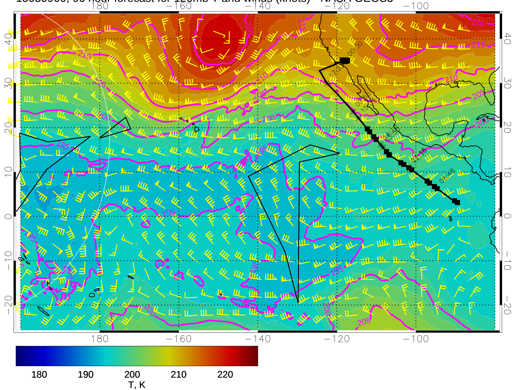
15030900, 96 hour forecast for 120mb T and winds (knots) - NASA GEOS5
