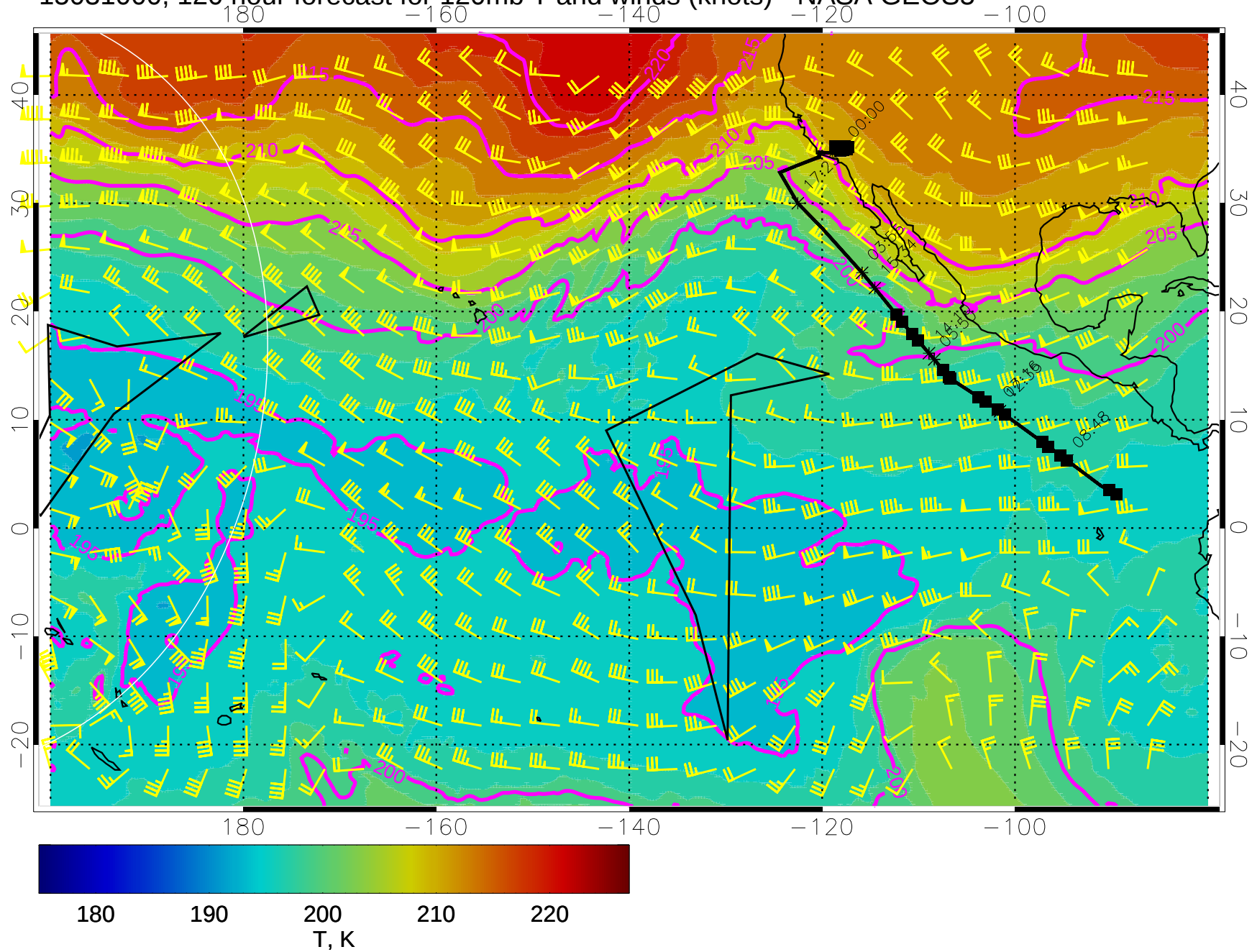
15031000, 120 hour forecast for 120mb T and winds (knots) - NASA GEOS5
