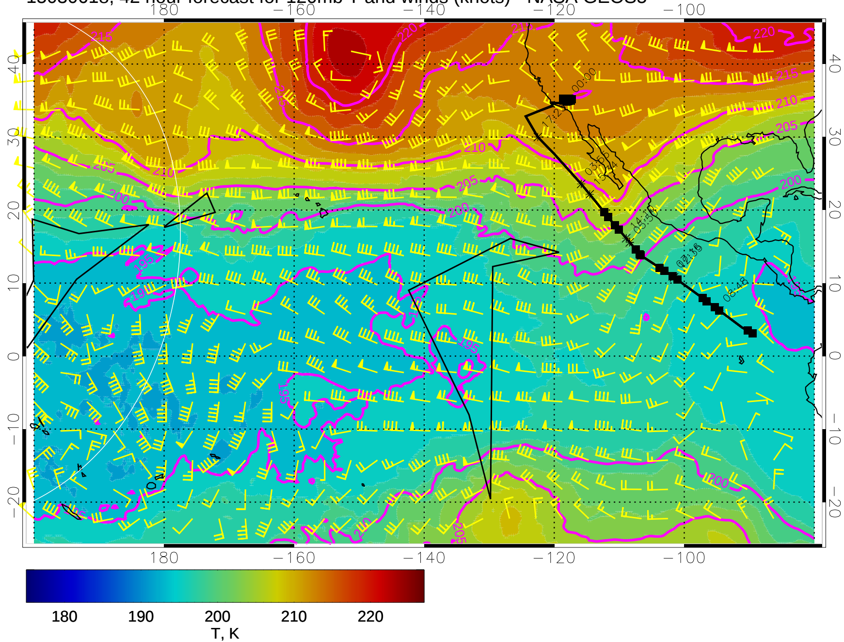
15030618, 42 hour forecast for 120mb T and winds (knots) - NASA GEOS5
