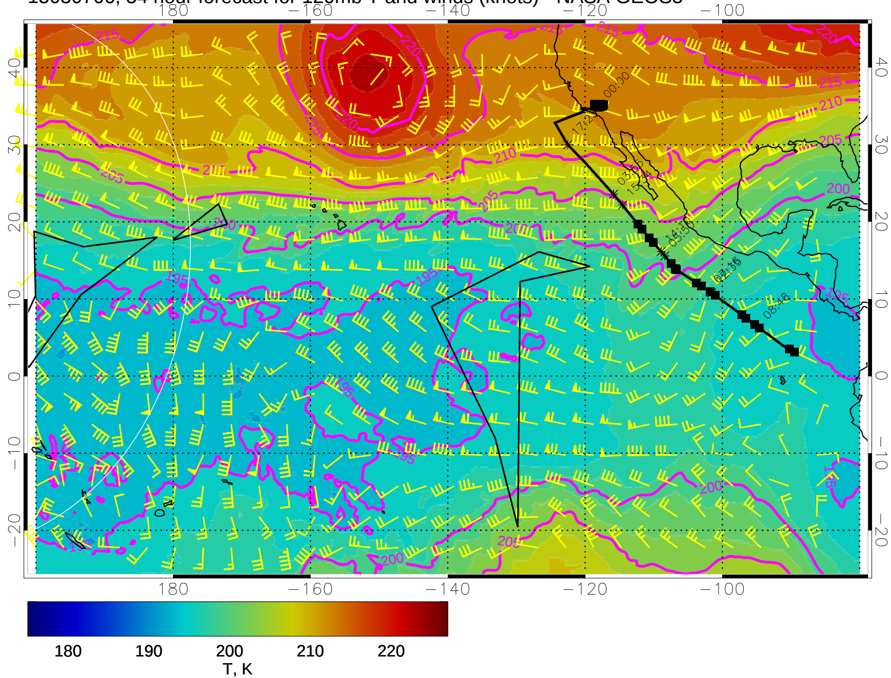
15030706, 54 hour forecast for 120mb T and winds (knots) - NASA GEOS5
