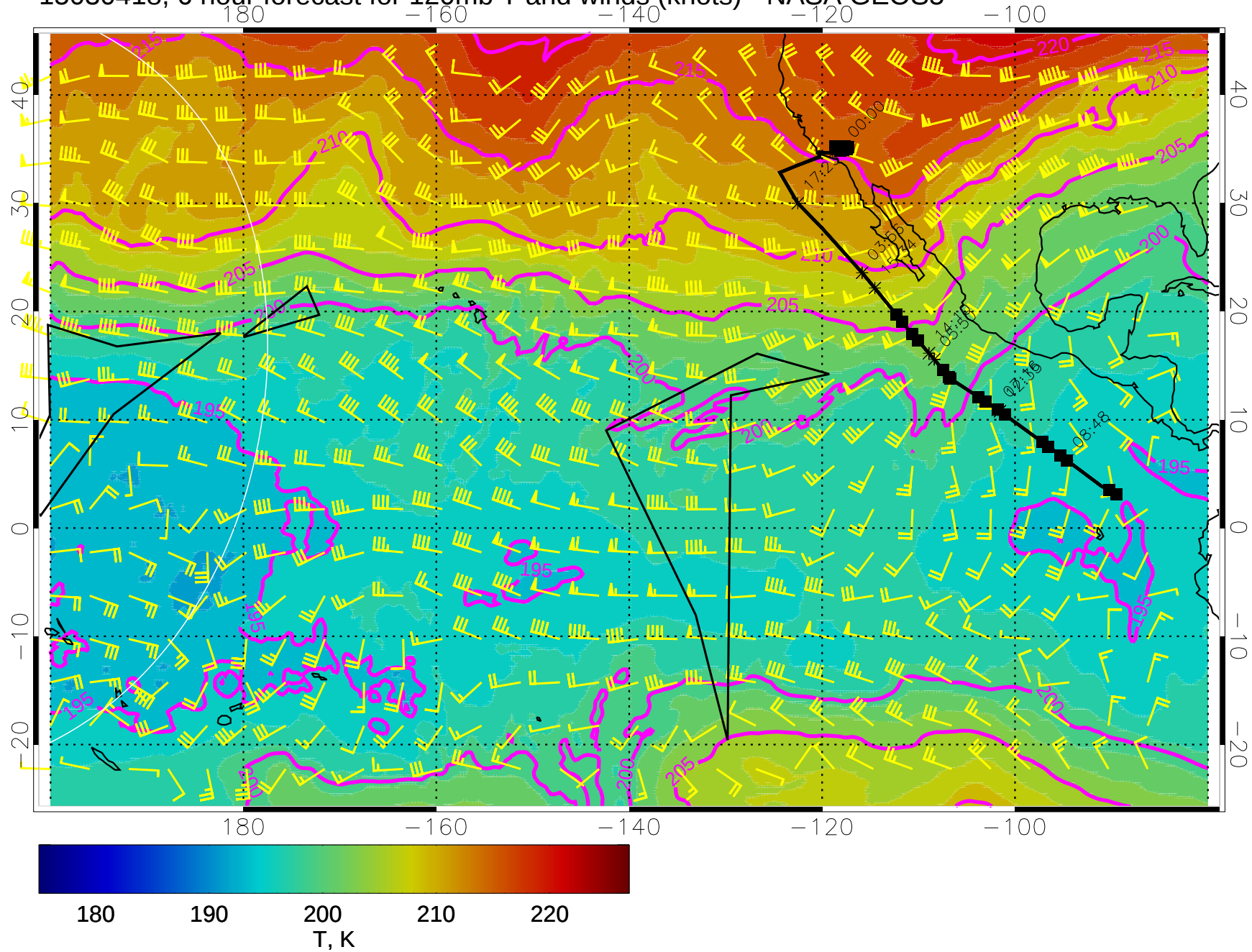
15030418, 6 hour forecast for 120mb T and winds (knots) - NASA GEOS5
