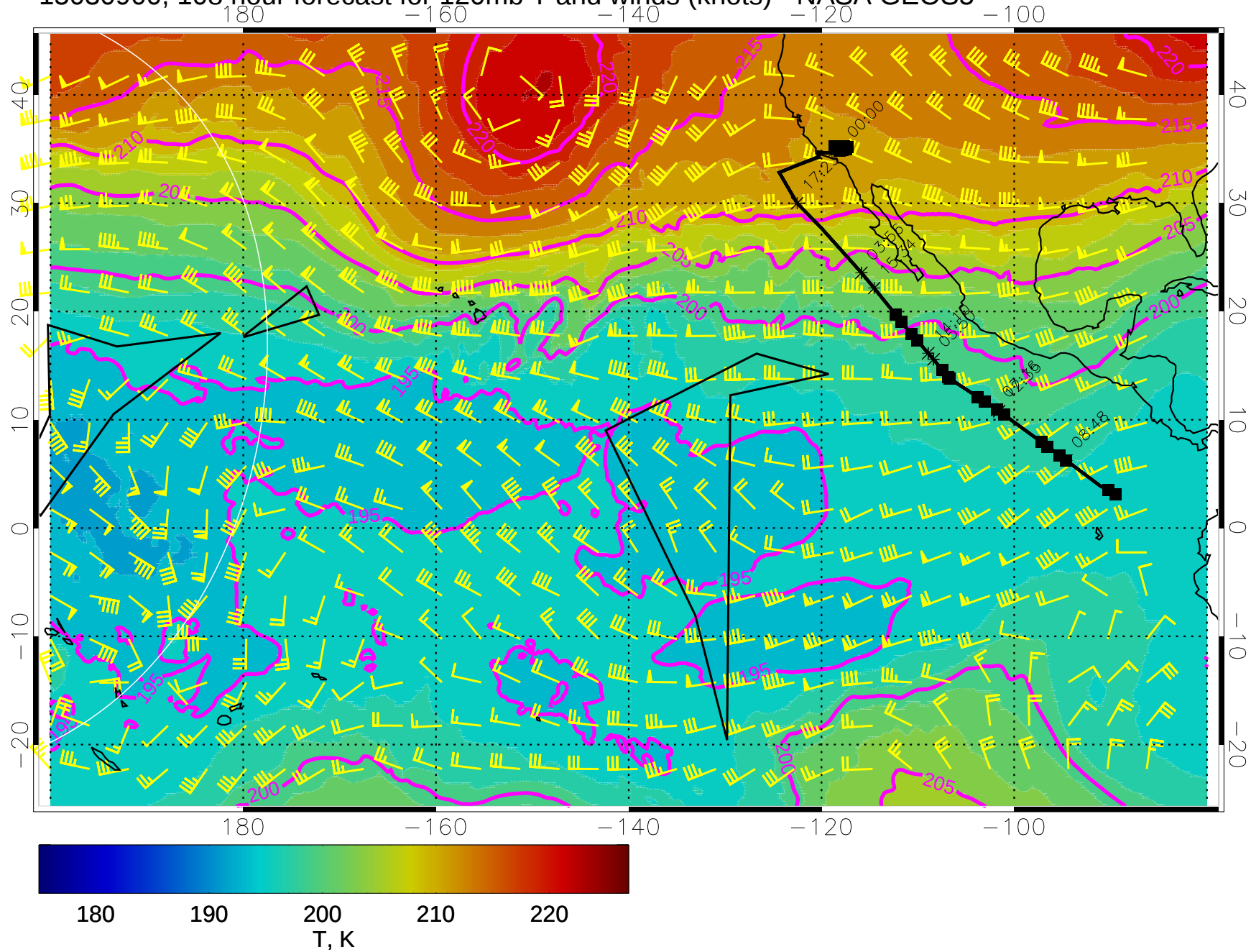
15030900, 108 hour forecast for 120mb T and winds (knots) - NASA GEOS5
