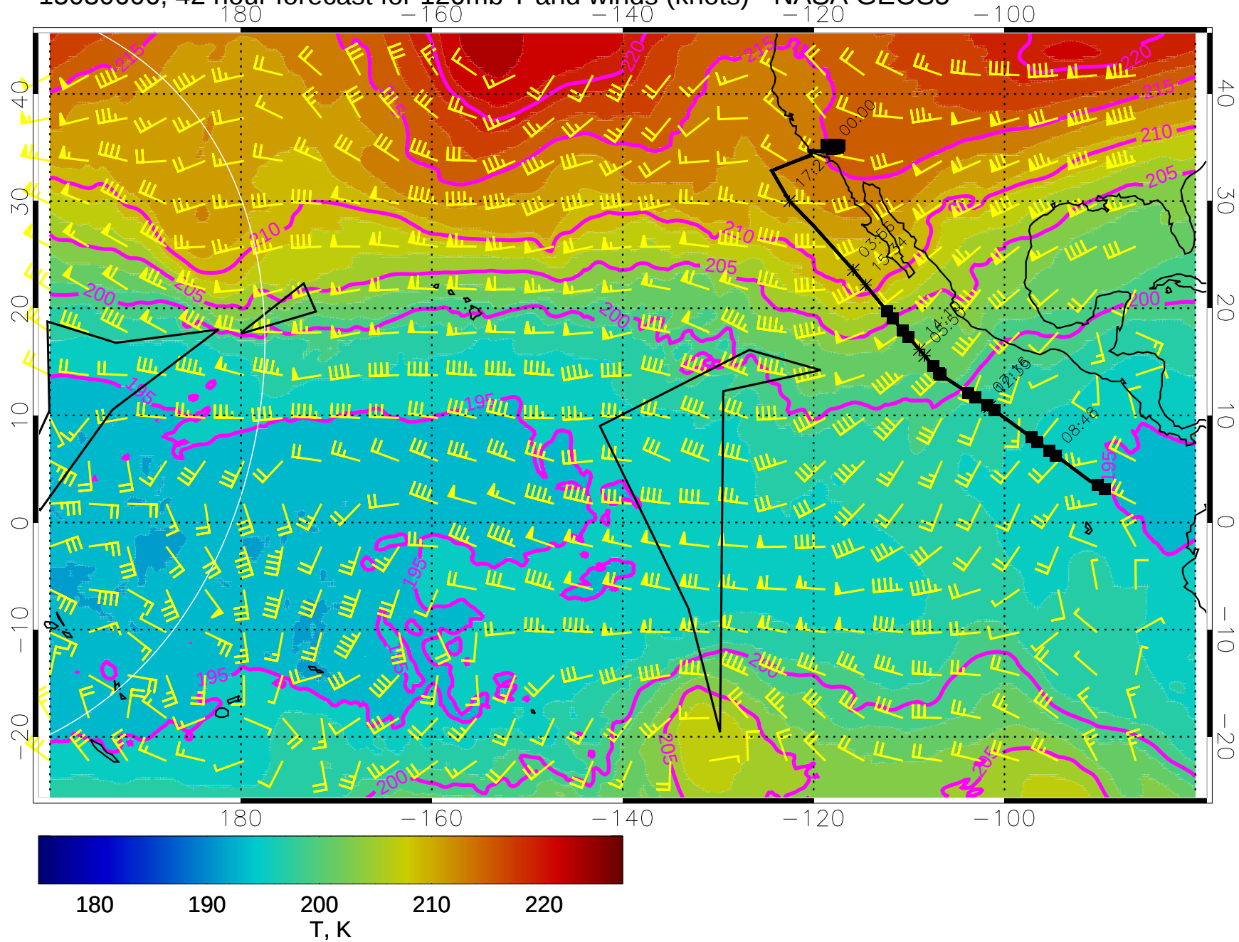
15030606, 42 hour forecast for 120mb T and winds (knots) - NASA GEOS5
