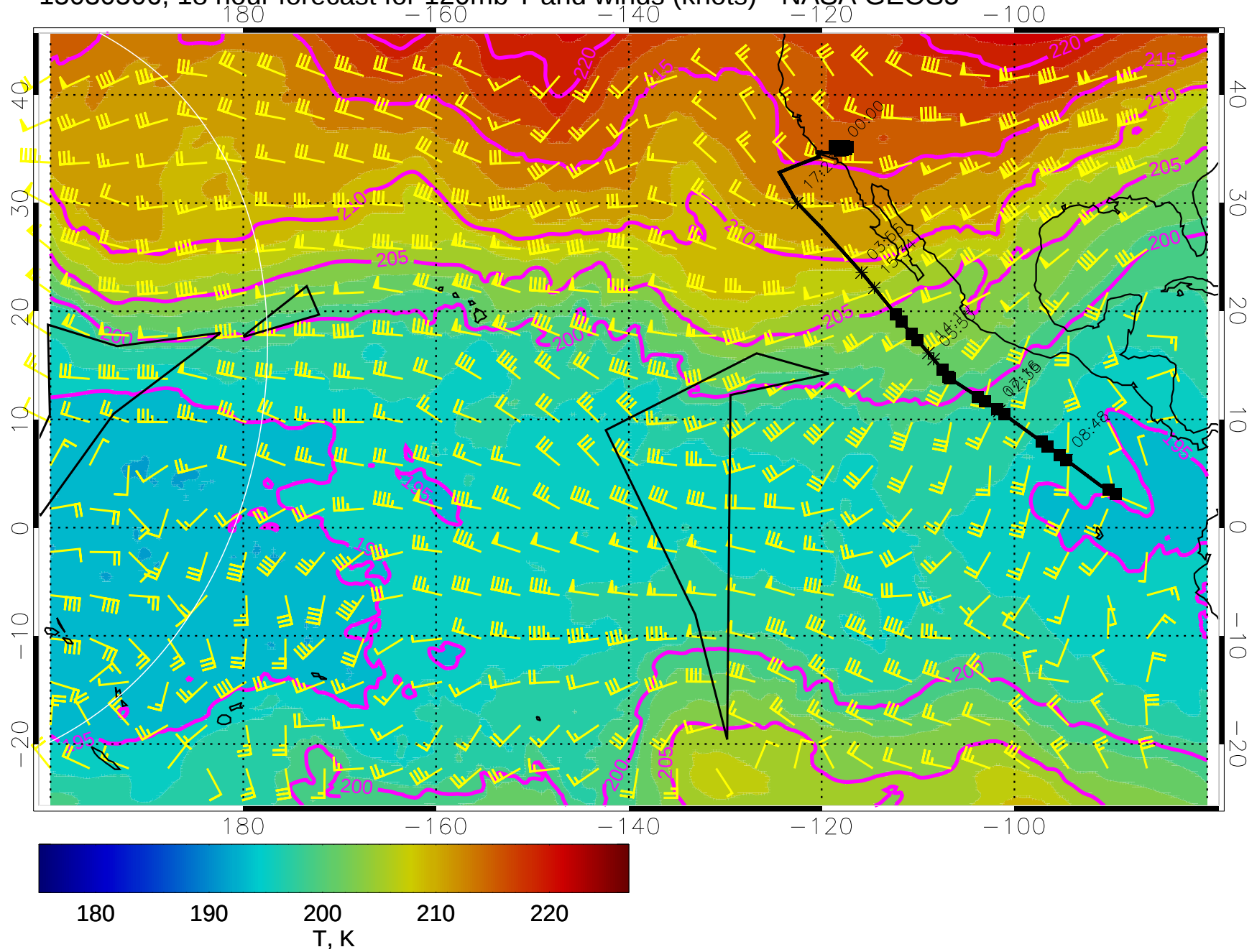
15030506, 18 hour forecast for 120mb T and winds (knots) - NASA GEOS5
