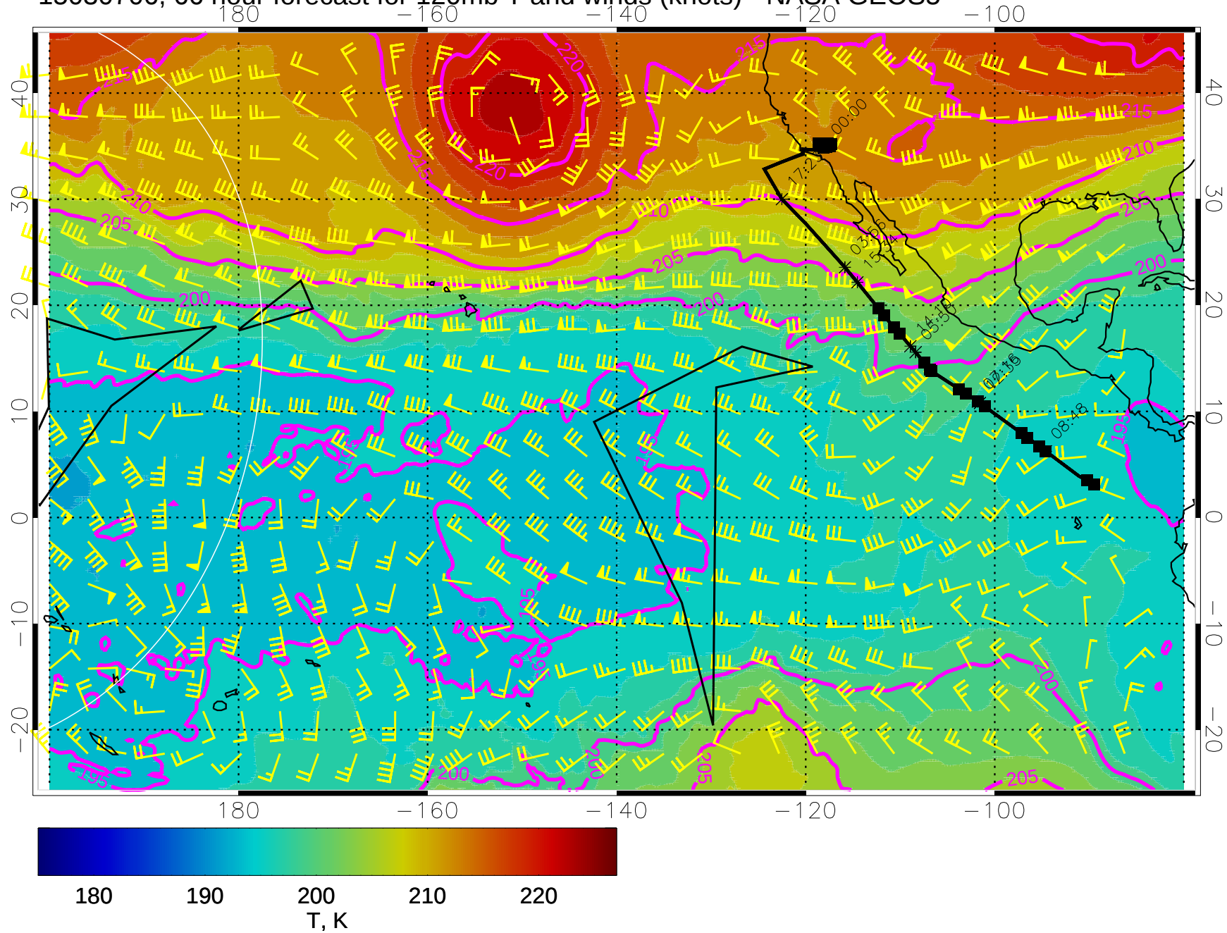
15030706, 66 hour forecast for 120mb T and winds (knots) - NASA GEOS5
