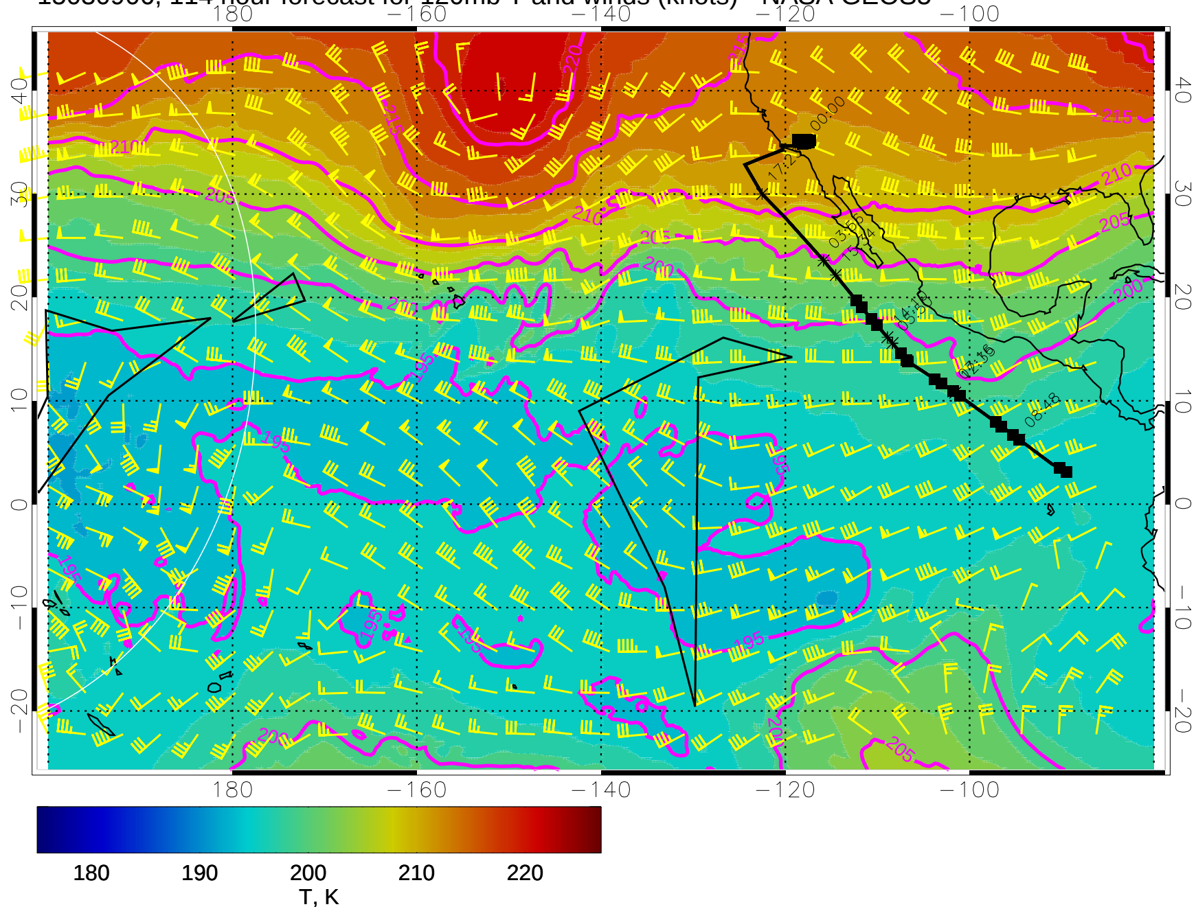
15030906, 114 hour forecast for 120mb T and winds (knots) - NASA GEOS5
