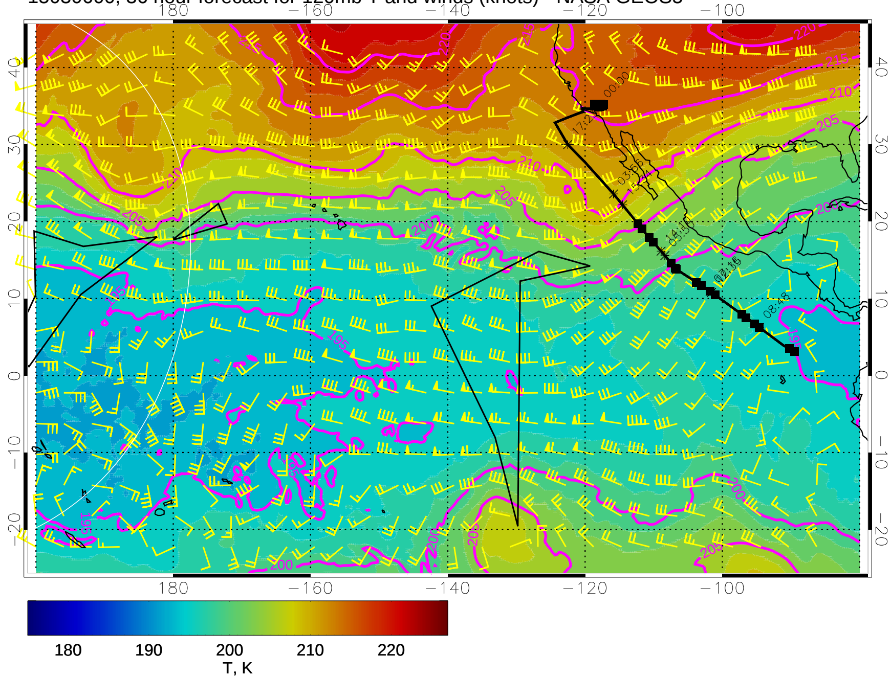
15030600, 36 hour forecast for 120mb T and winds (knots) - NASA GEOS5
