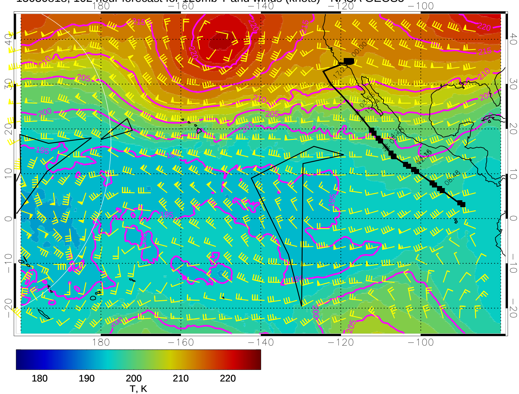
15030818, 102 hour forecast for 120mb T and winds (knots) - NASA GEOS5
