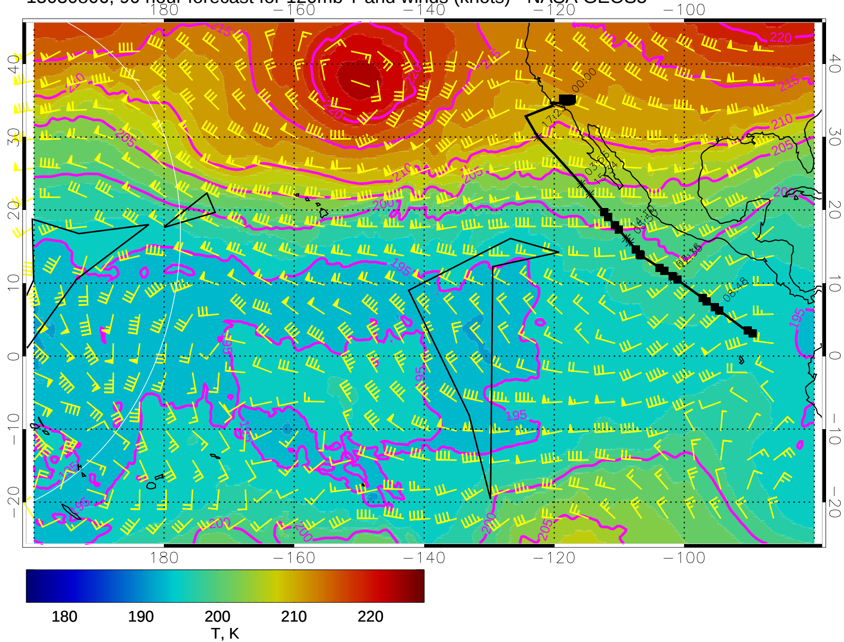
15030806, 90 hour forecast for 120mb T and winds (knots) - NASA GEOS5
