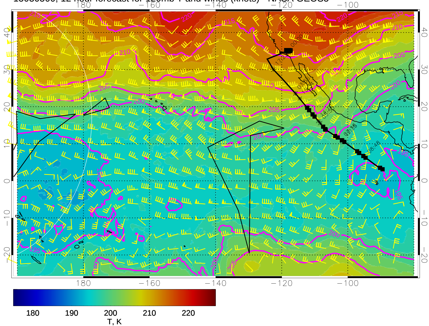
15030500, 12 hour forecast for 120mb T and winds (knots) - NASA GEOS5
