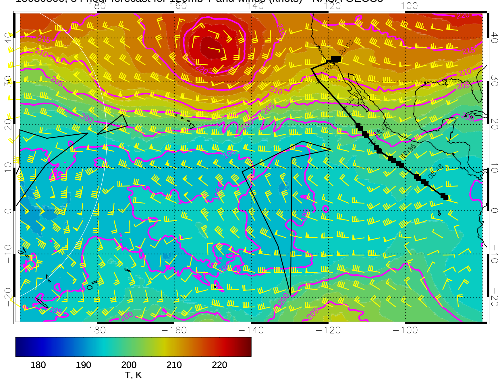
15030800, 84 hour forecast for 120mb T and winds (knots) - NASA GEOS5
