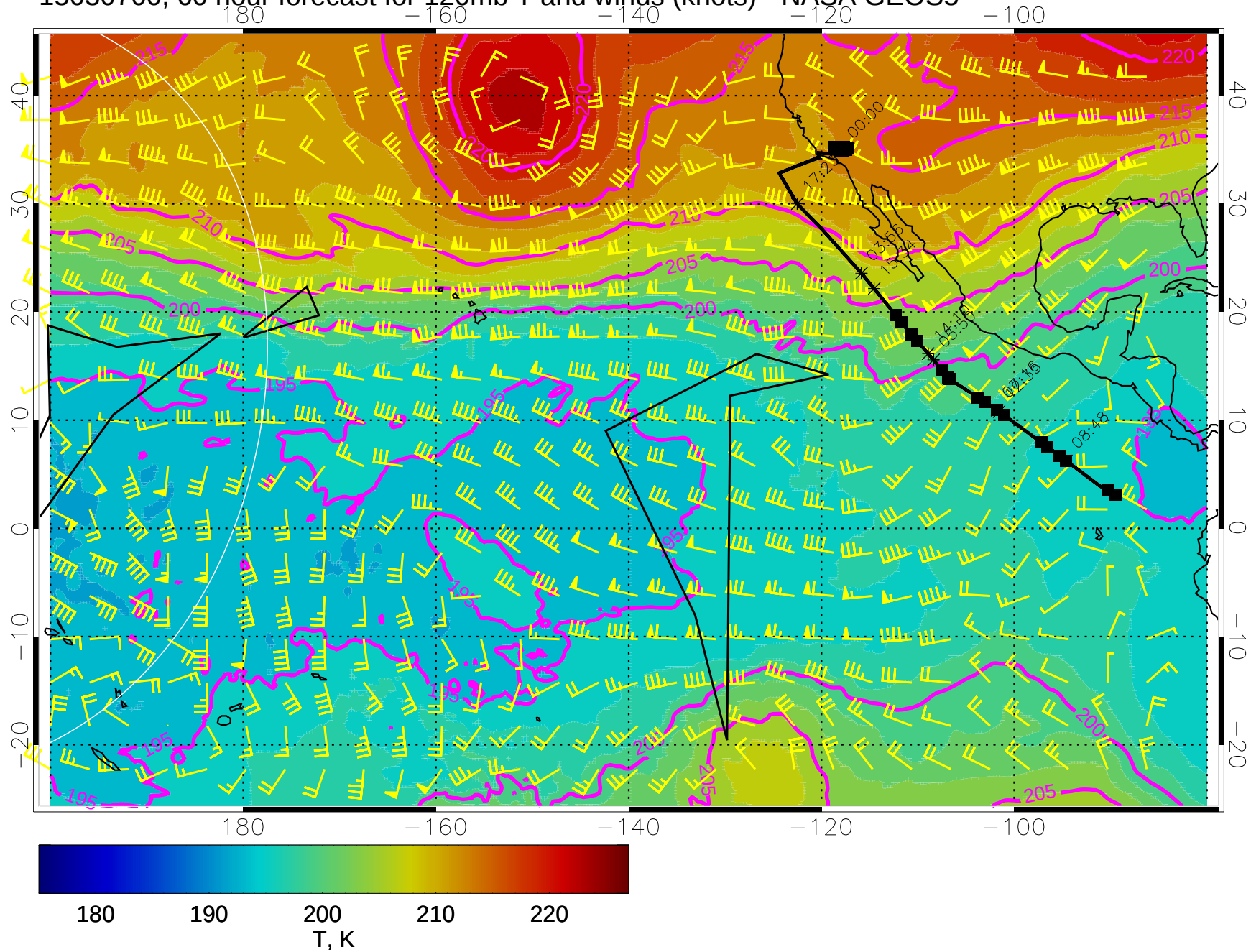
15030700, 60 hour forecast for 120mb T and winds (knots) - NASA GEOS5
