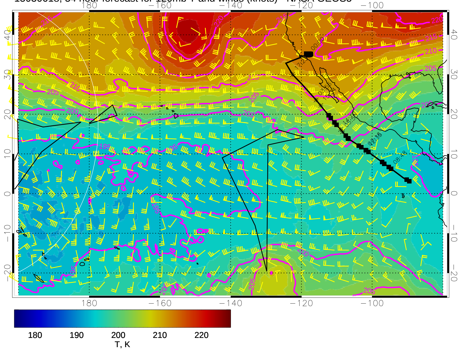
15030618, 54 hour forecast for 120mb T and winds (knots) - NASA GEOS5
