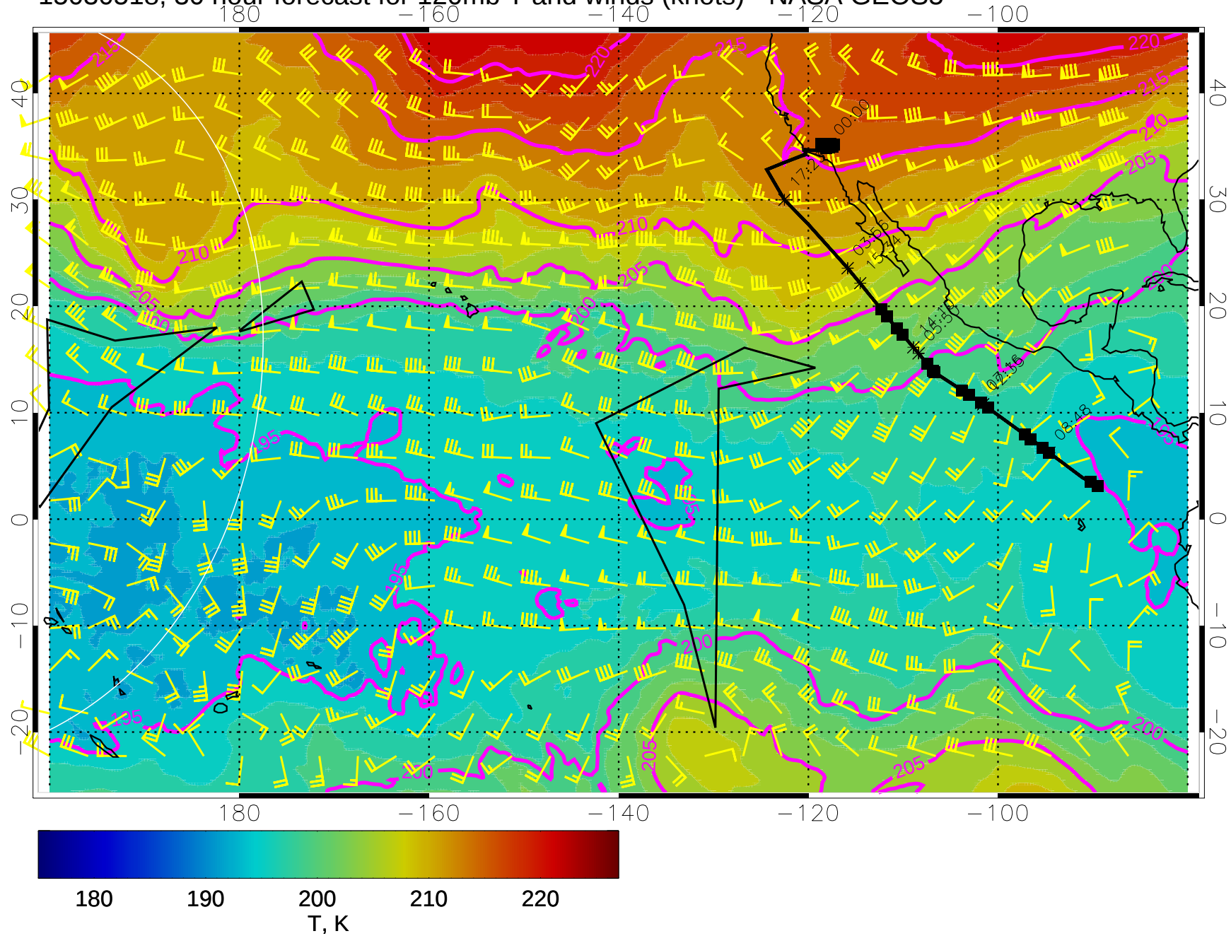
15030518, 30 hour forecast for 120mb T and winds (knots) - NASA GEOS5
