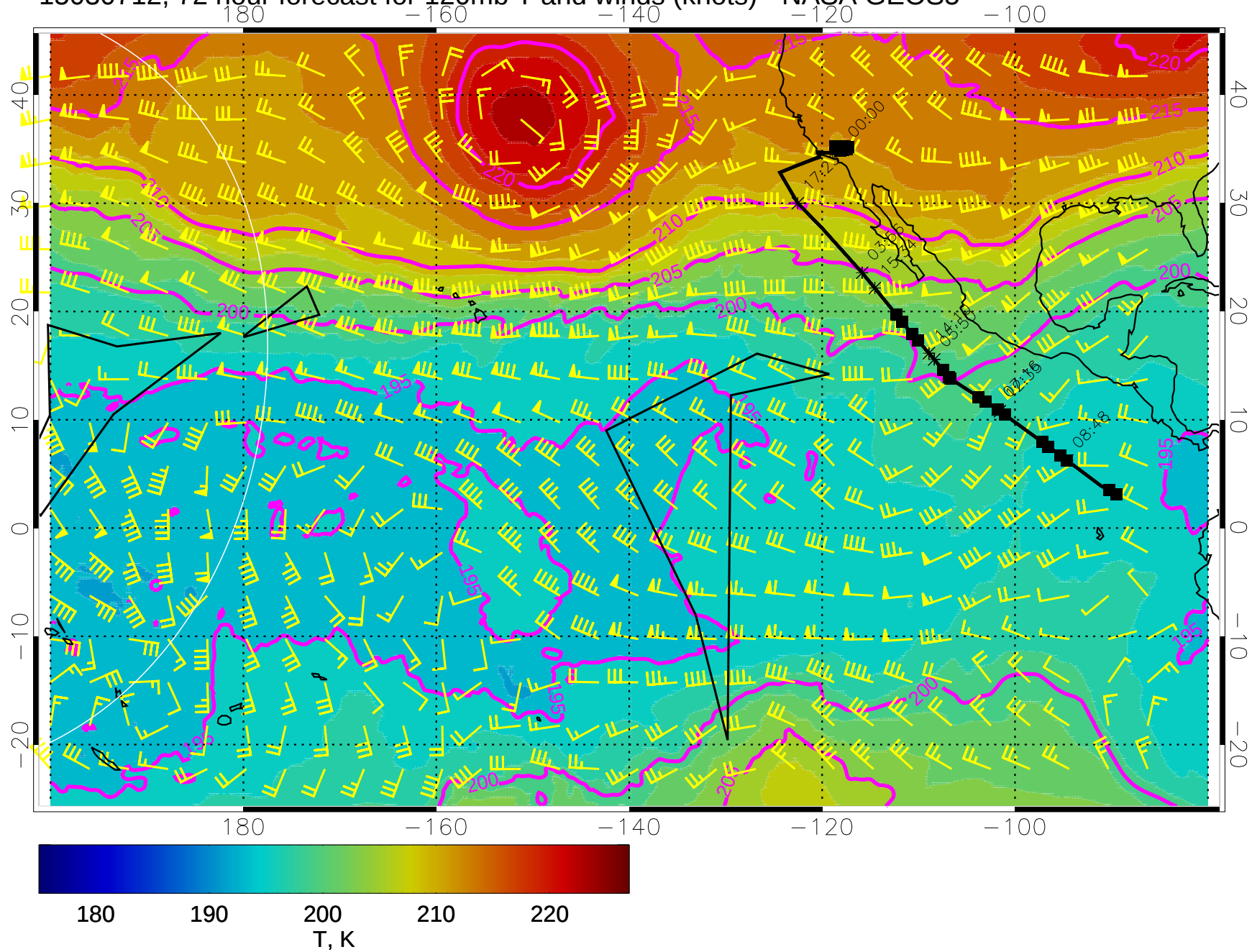
15030712, 72 hour forecast for 120mb T and winds (knots) - NASA GEOS5
