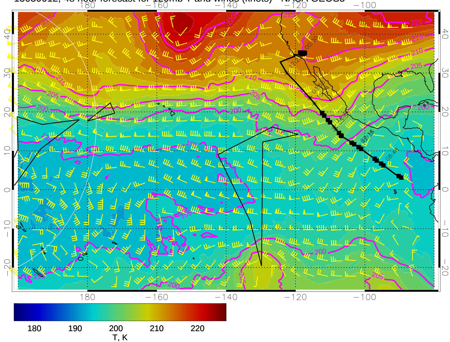
15030612, 48 hour forecast for 120mb T and winds (knots) - NASA GEOS5
