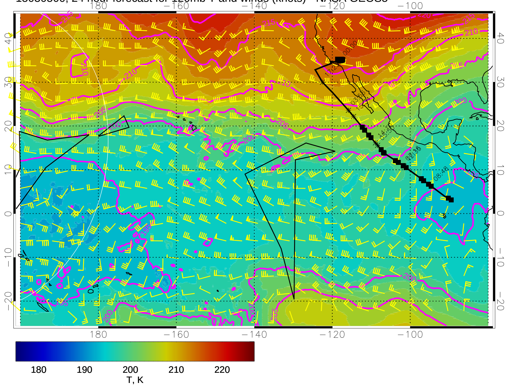
15030500, 24 hour forecast for 120mb T and winds (knots) - NASA GEOS5
