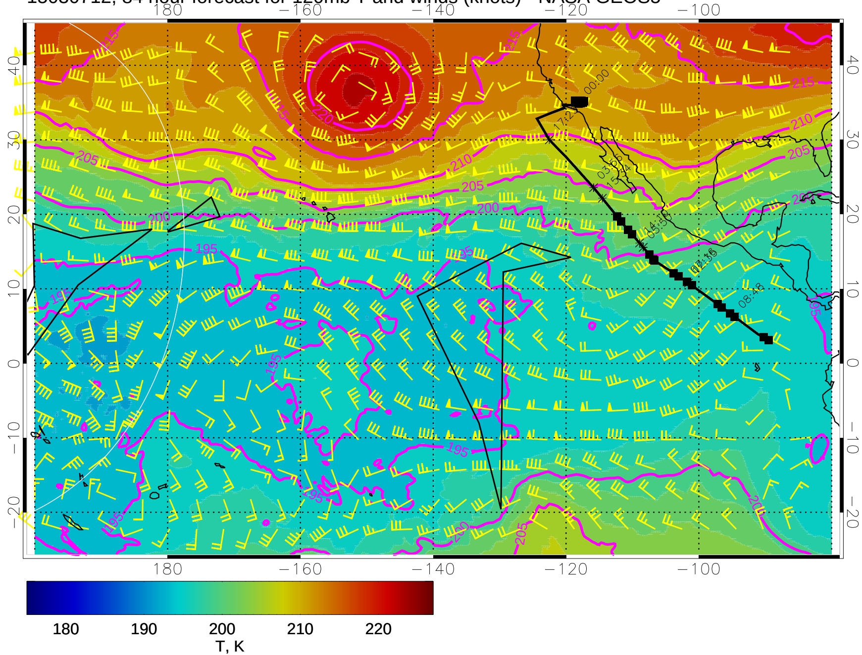
15030712, 84 hour forecast for 120mb T and winds (knots) - NASA GEOS5
