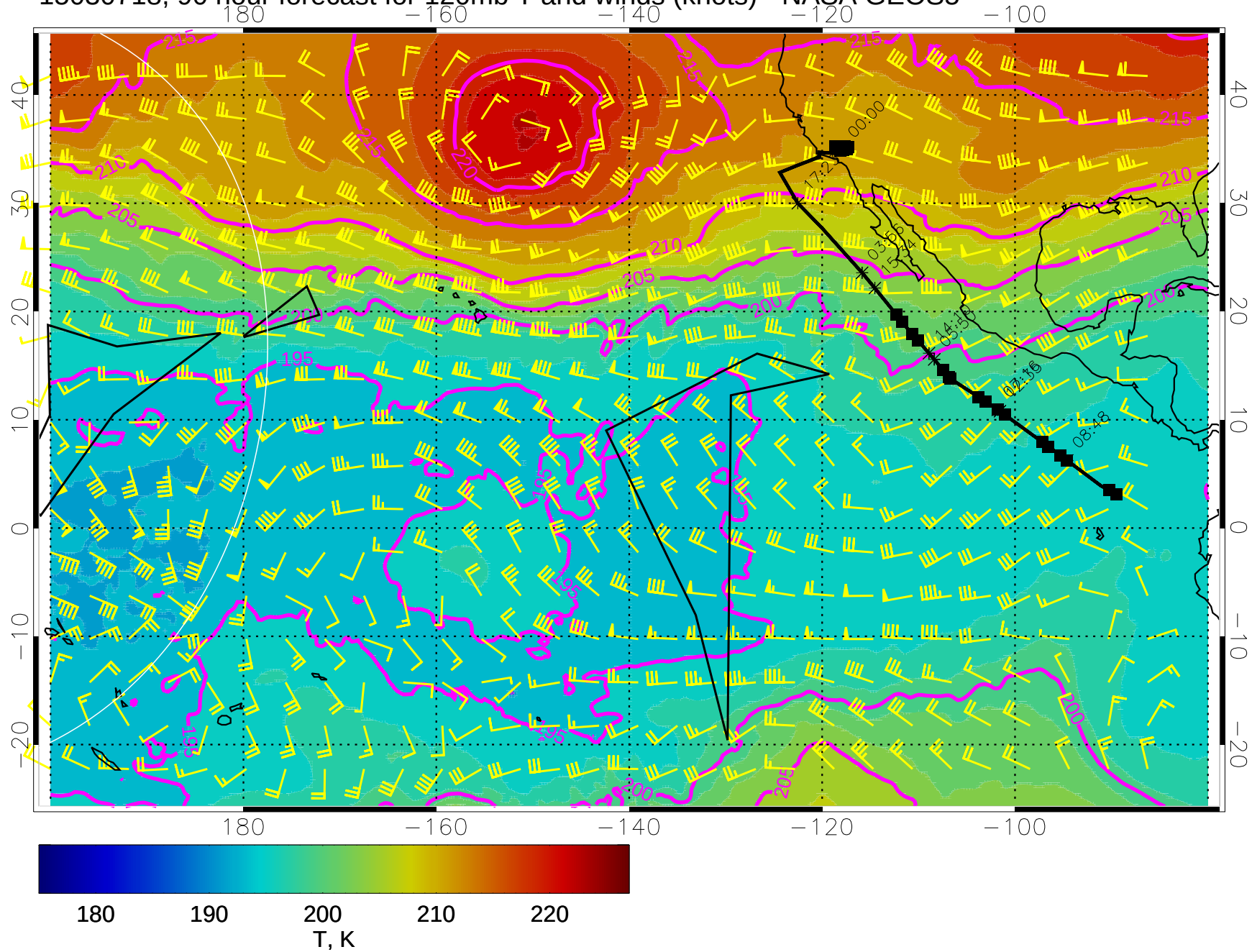
15030718, 90 hour forecast for 120mb T and winds (knots) - NASA GEOS5
