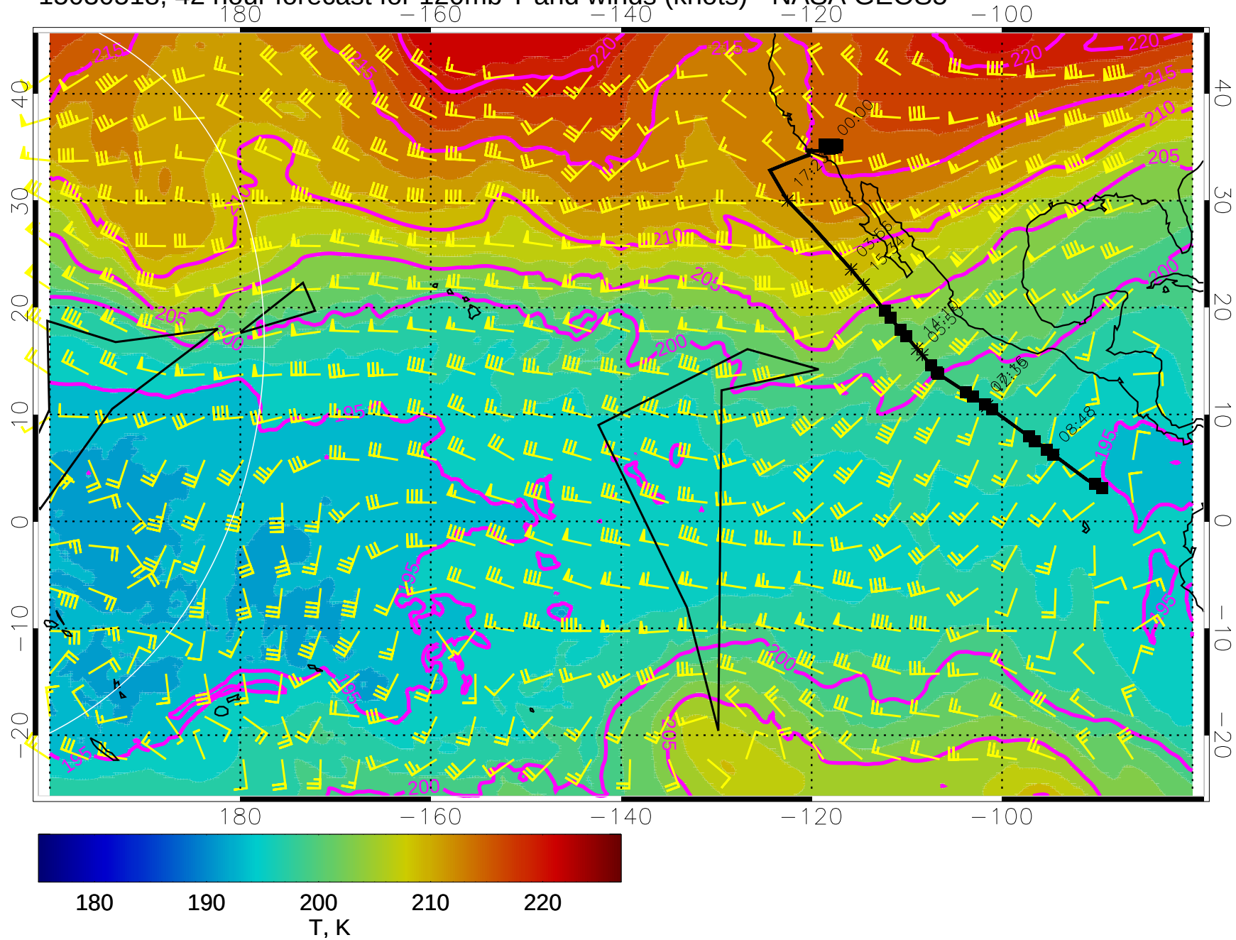
15030518, 42 hour forecast for 120mb T and winds (knots) - NASA GEOS5
