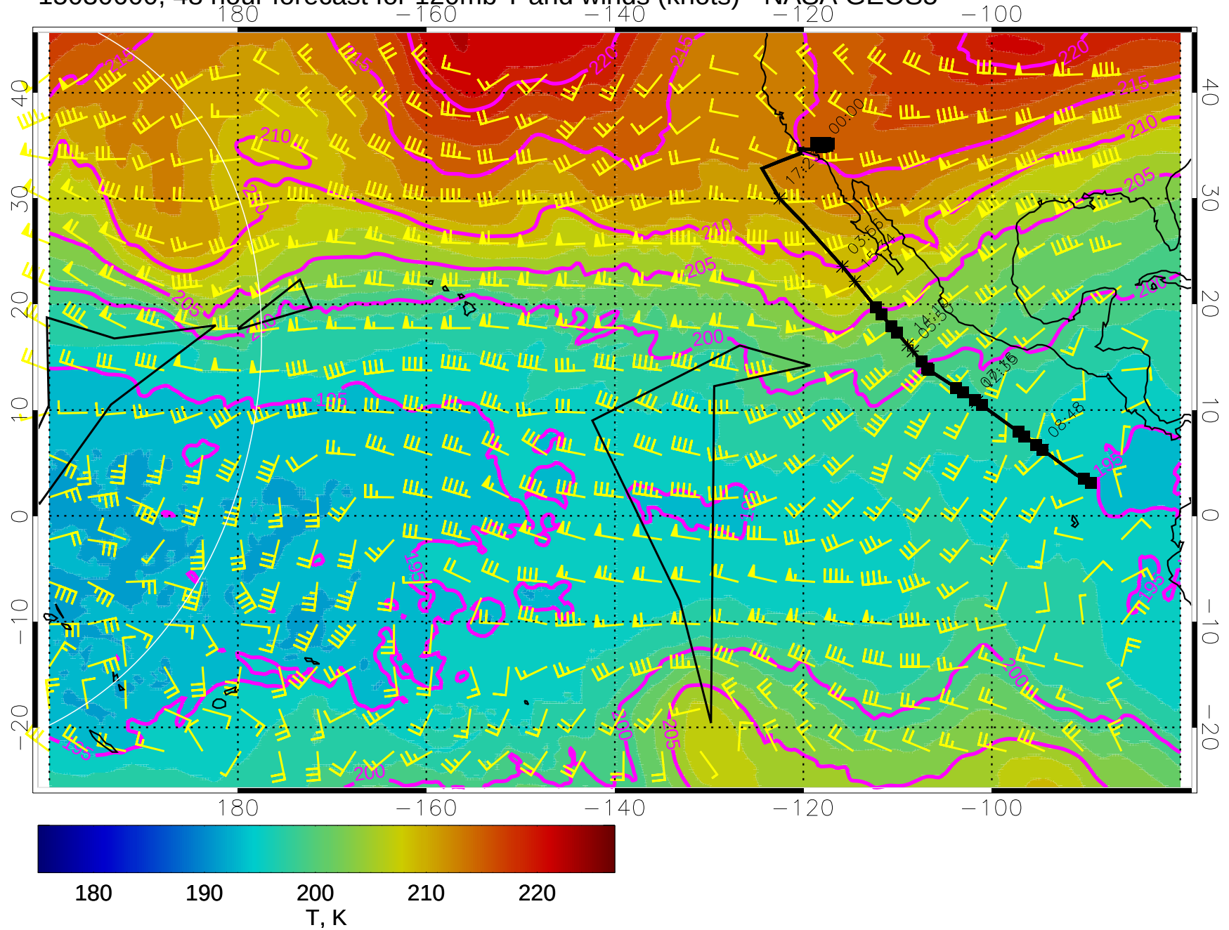
15030600, 48 hour forecast for 120mb T and winds (knots) - NASA GEOS5
