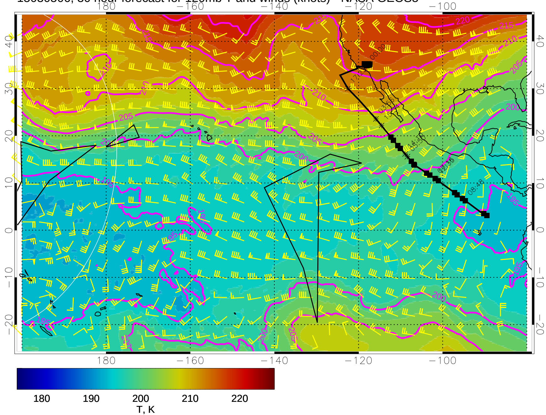
15030506, 30 hour forecast for 120mb T and winds (knots) - NASA GEOS5
