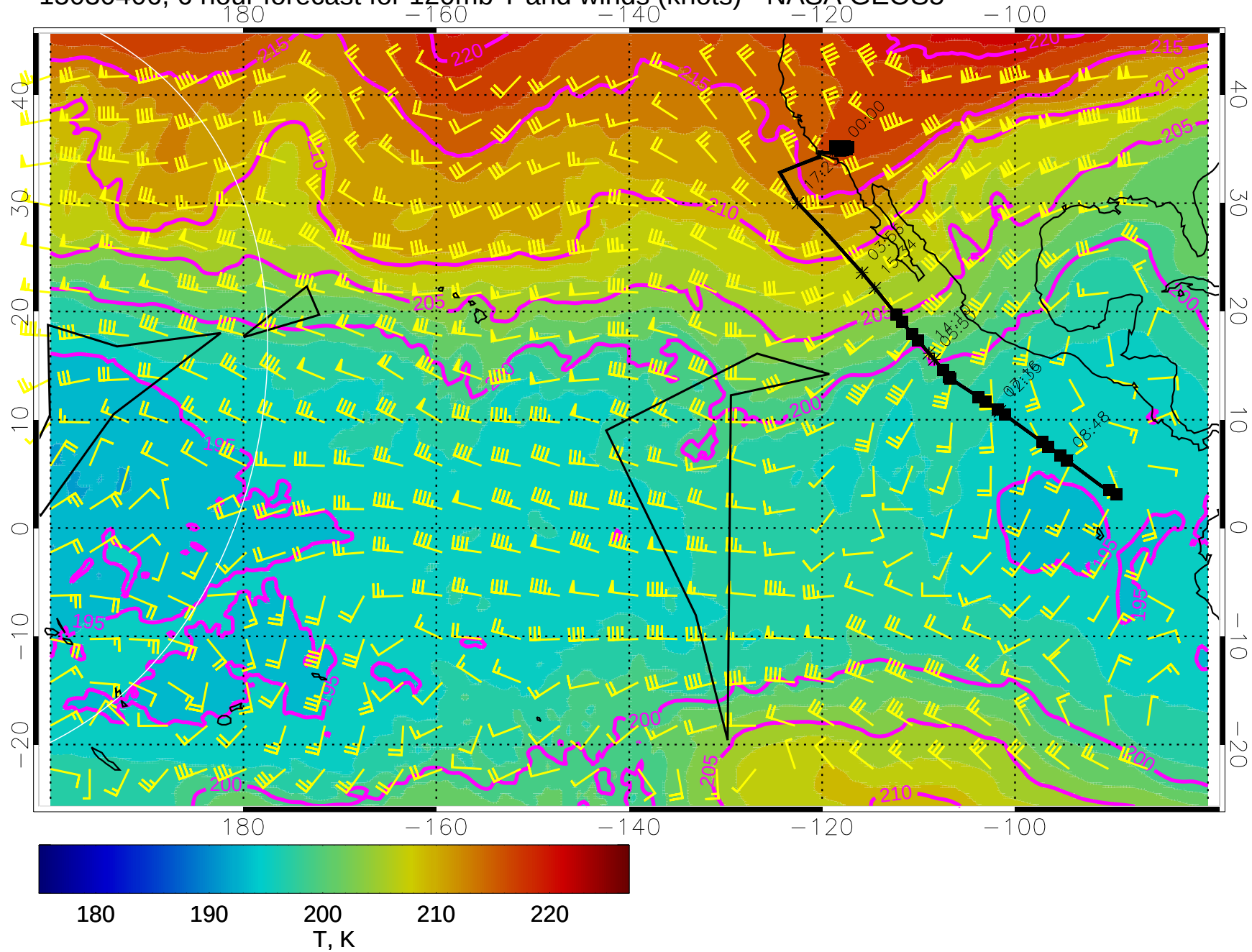
15030406, 6 hour forecast for 120mb T and winds (knots) - NASA GEOS5
