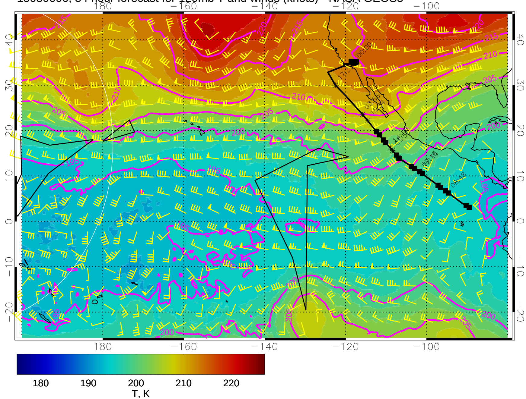
15030606, 54 hour forecast for 120mb T and winds (knots) - NASA GEOS5
