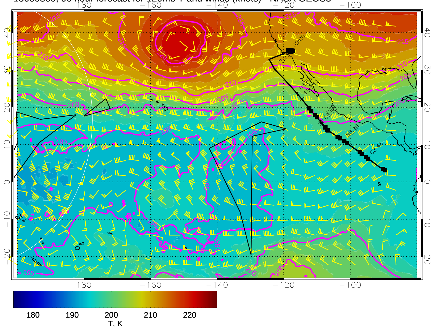
15030800, 96 hour forecast for 120mb T and winds (knots) - NASA GEOS5
