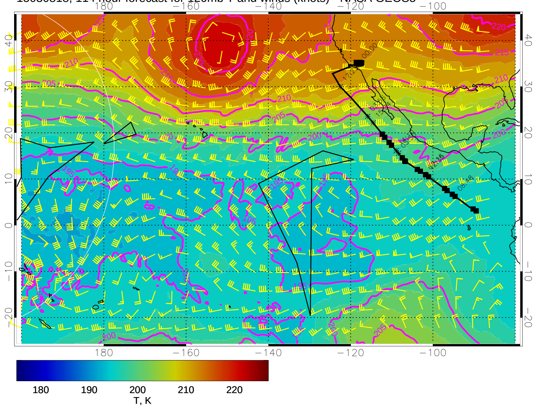
15030818, 114 hour forecast for 120mb T and winds (knots) - NASA GEOS5
