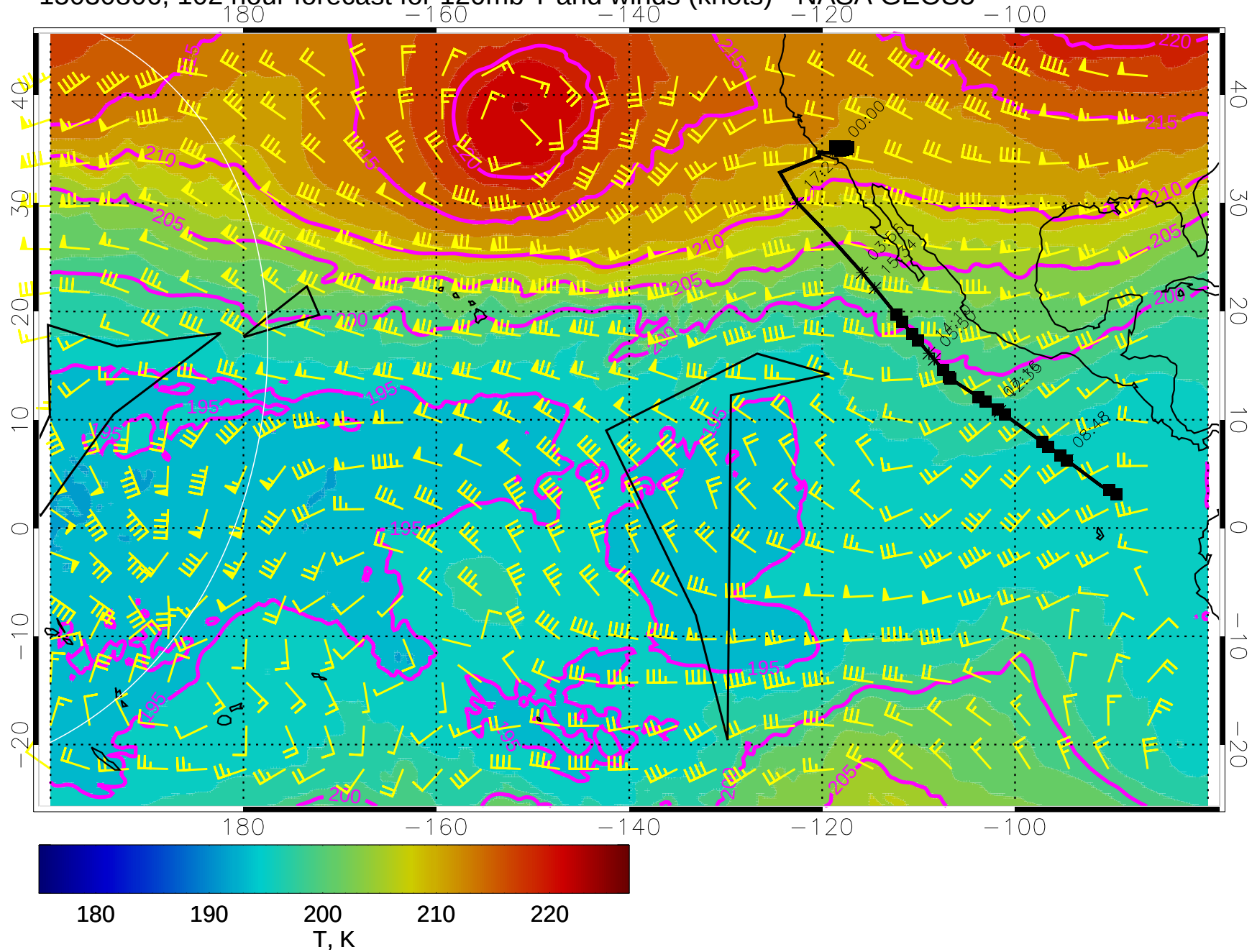
15030806, 102 hour forecast for 120mb T and winds (knots) - NASA GEOS5
