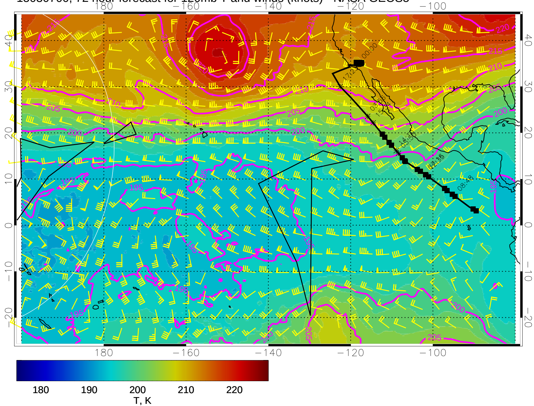
15030700, 72 hour forecast for 120mb T and winds (knots) - NASA GEOS5
