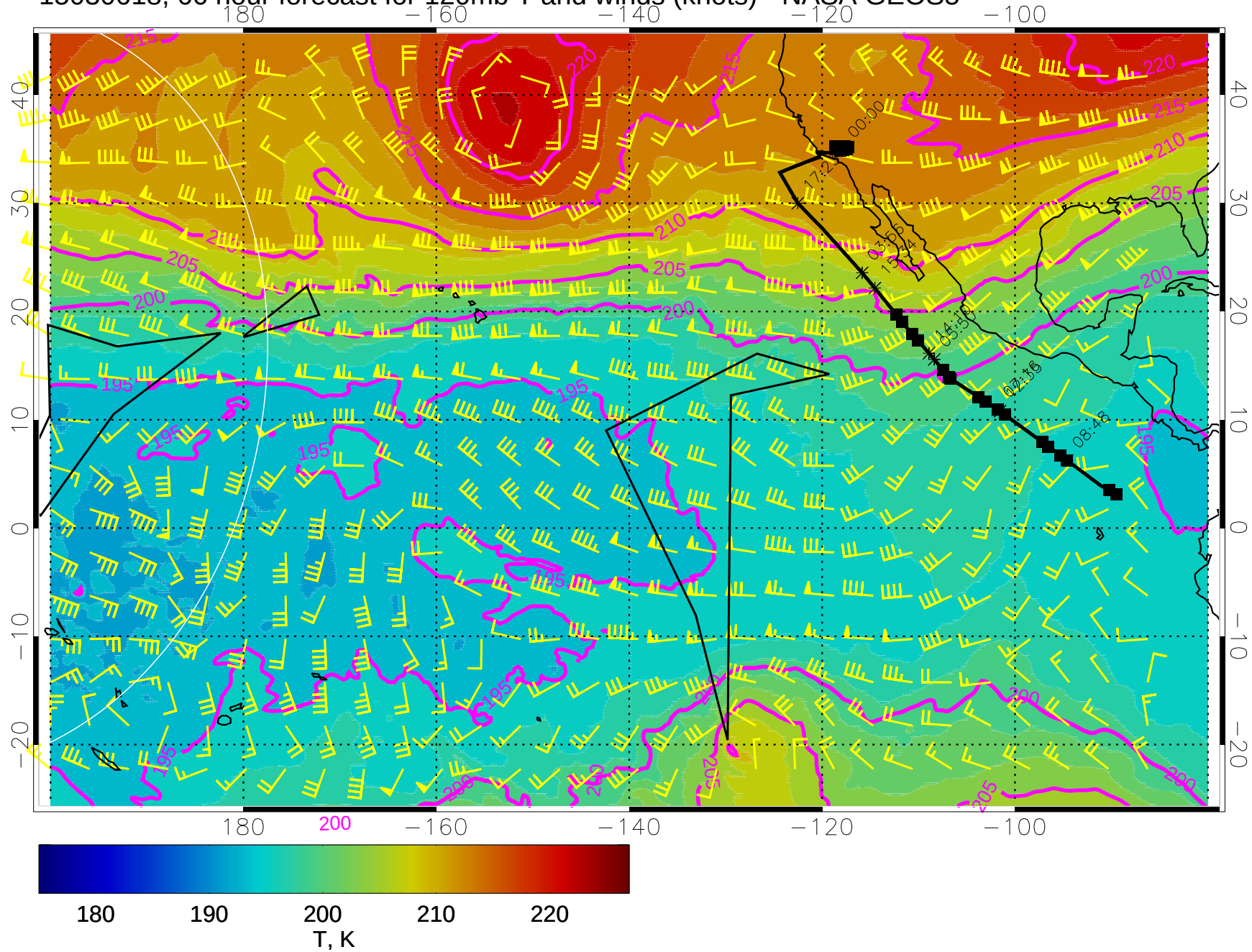
15030618, 66 hour forecast for 120mb T and winds (knots) - NASA GEOS5
