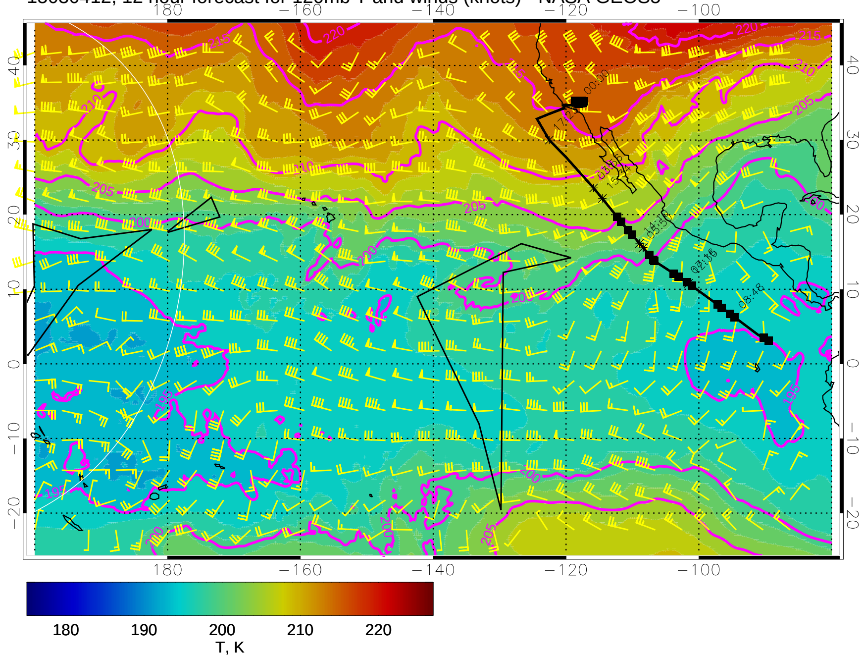
15030412, 12 hour forecast for 120mb T and winds (knots) - NASA GEOS5
