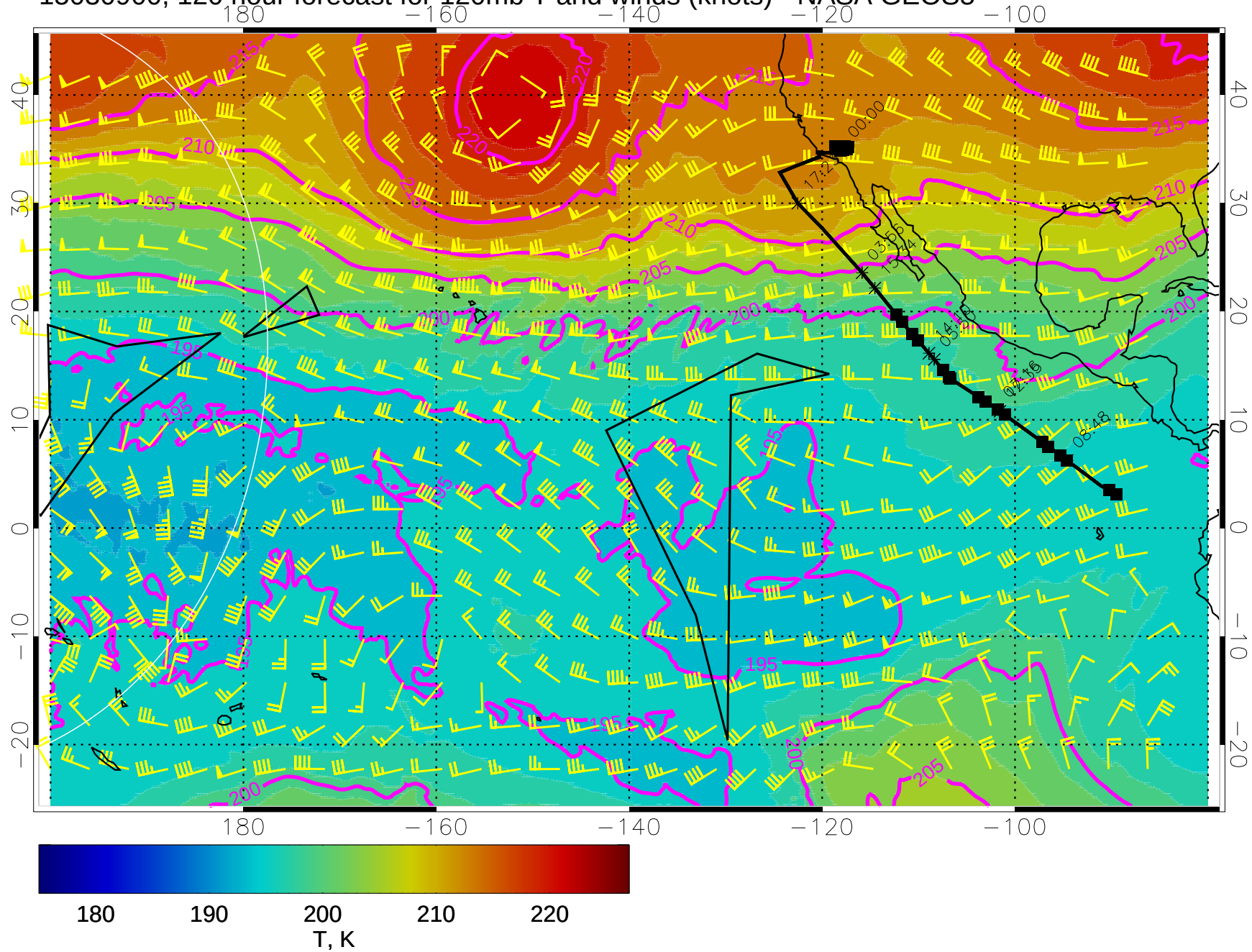
15030900, 120 hour forecast for 120mb T and winds (knots) - NASA GEOS5
