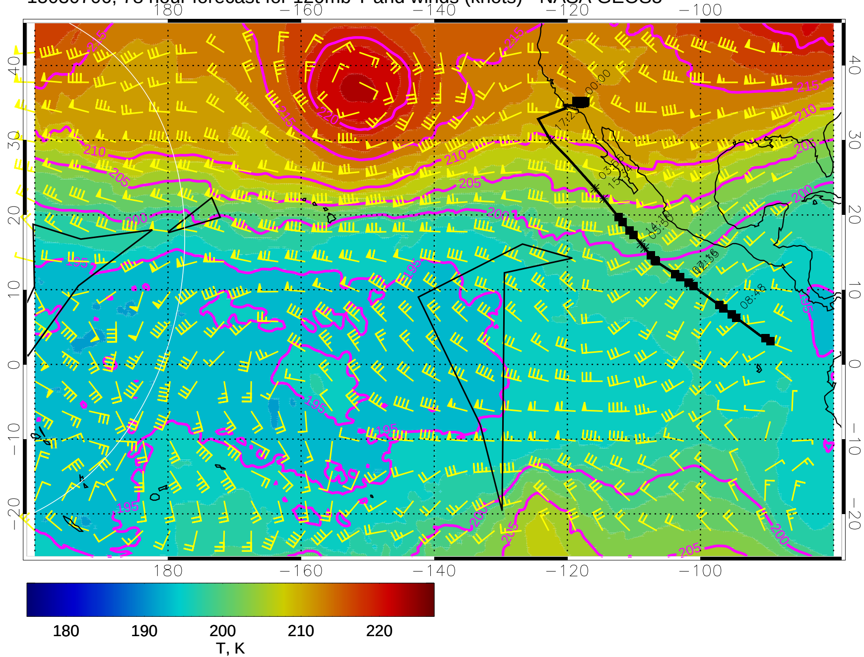
15030706, 78 hour forecast for 120mb T and winds (knots) - NASA GEOS5
