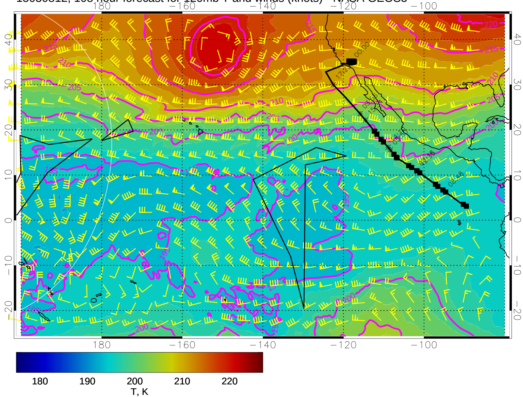
15030812, 108 hour forecast for 120mb T and winds (knots) - NASA GEOS5
