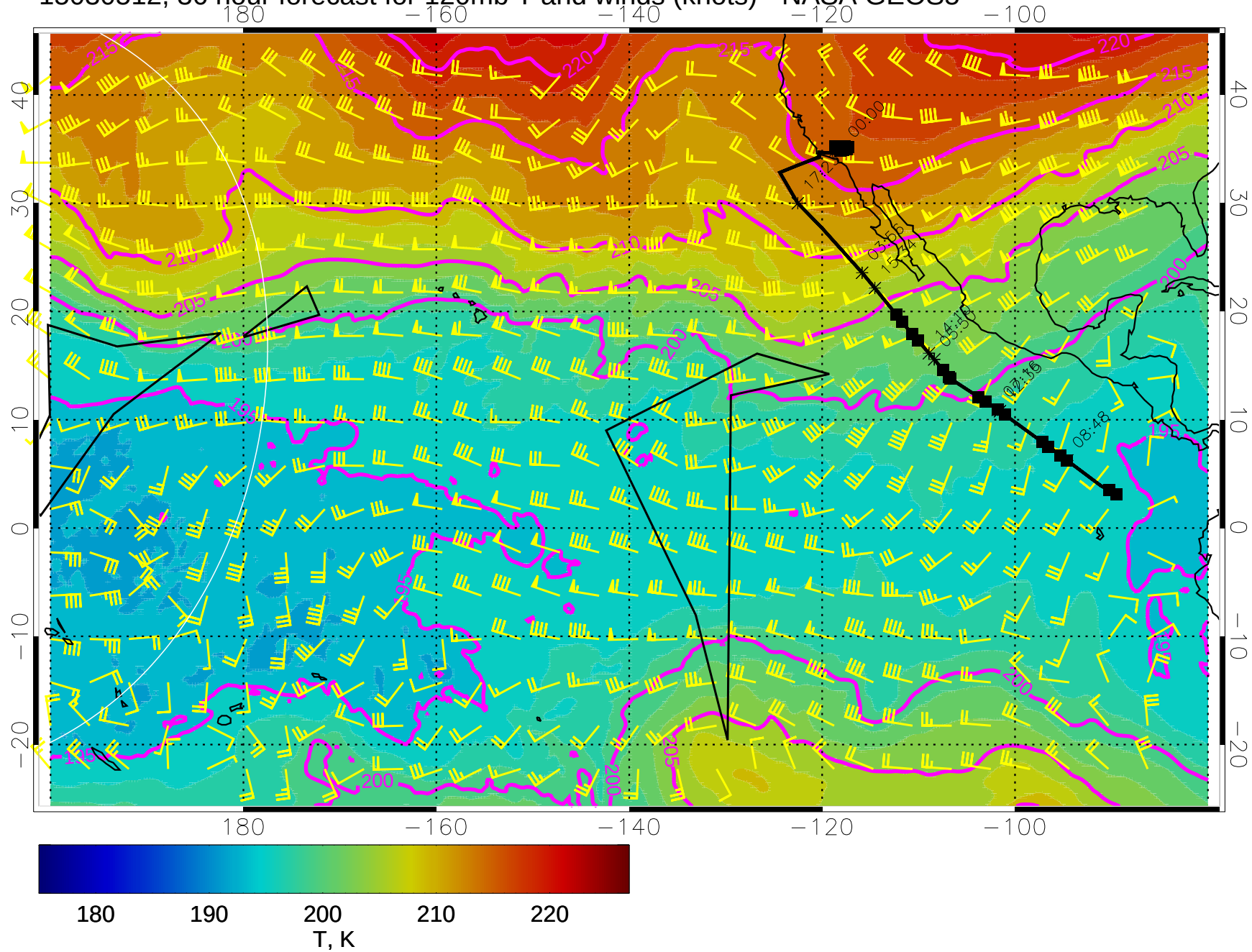
15030512, 36 hour forecast for 120mb T and winds (knots) - NASA GEOS5
