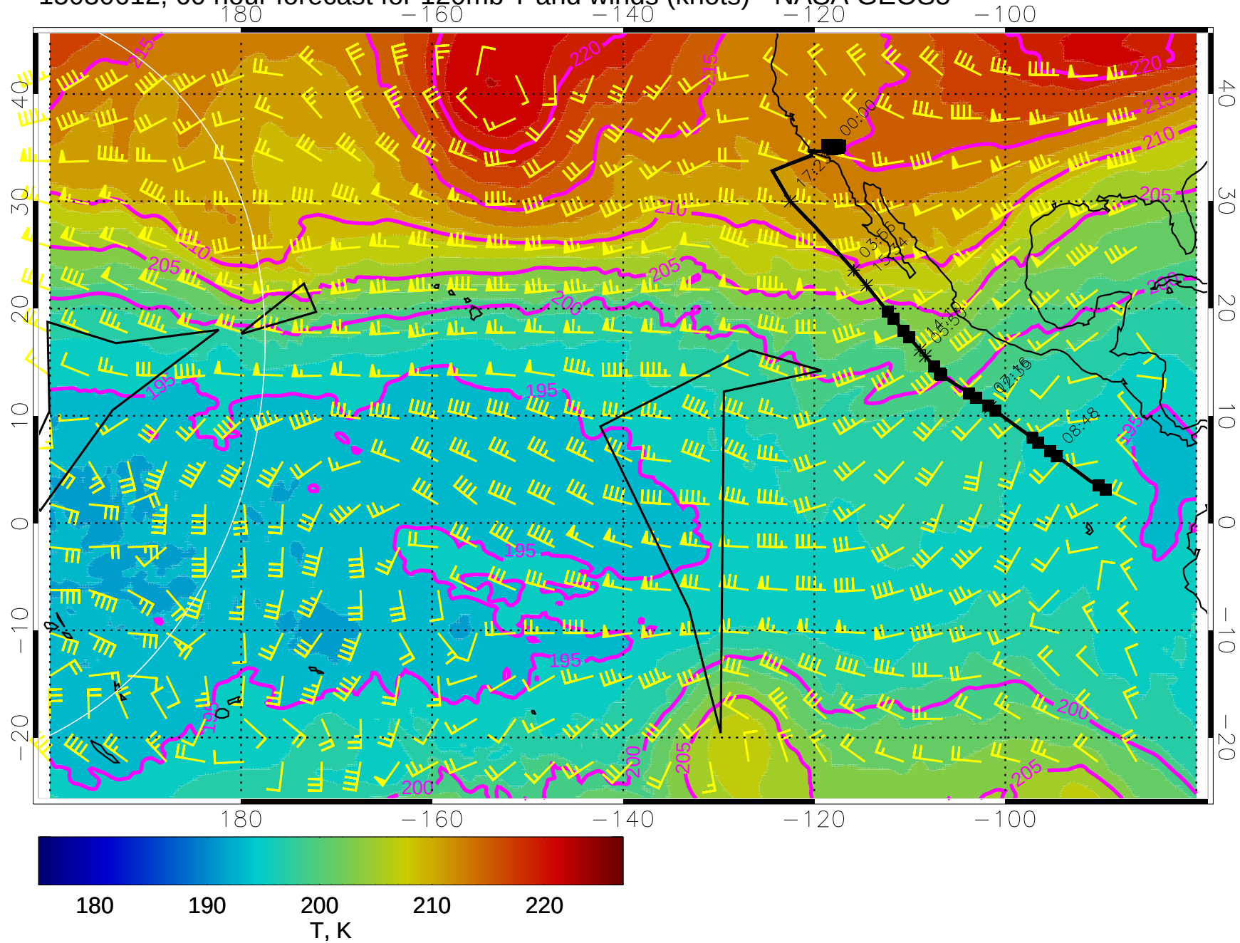
15030612, 60 hour forecast for 120mb T and winds (knots) - NASA GEOS5
