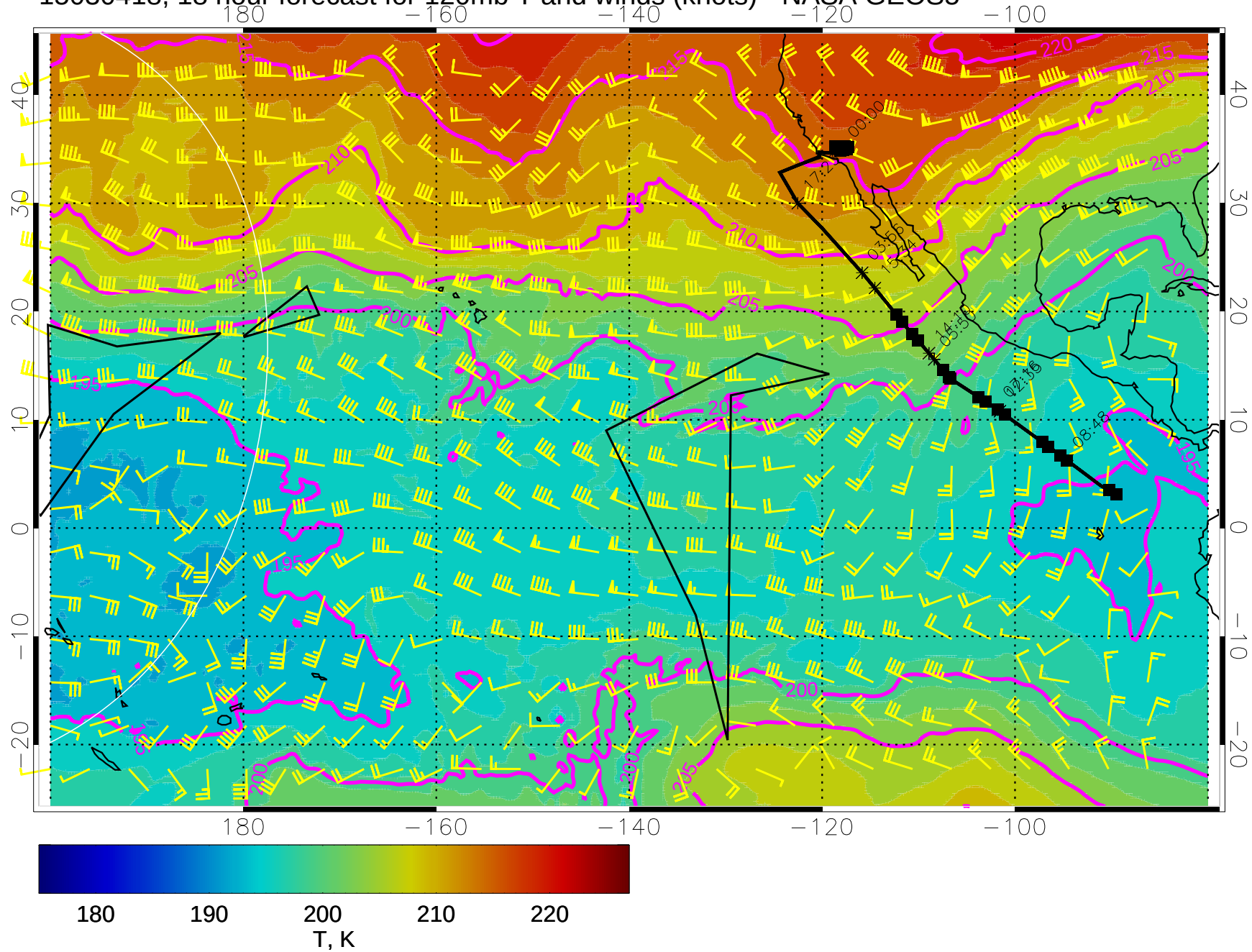
15030418, 18 hour forecast for 120mb T and winds (knots) - NASA GEOS5
