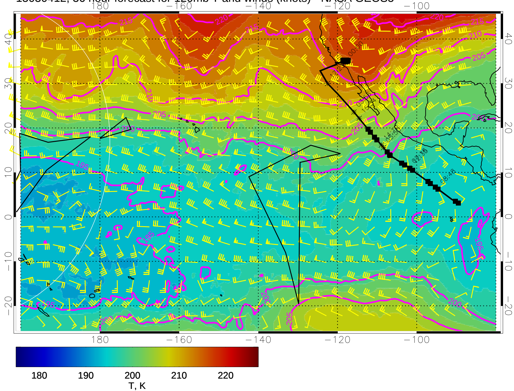
15030412, 36 hour forecast for 120mb T and winds (knots) - NASA GEOS5
