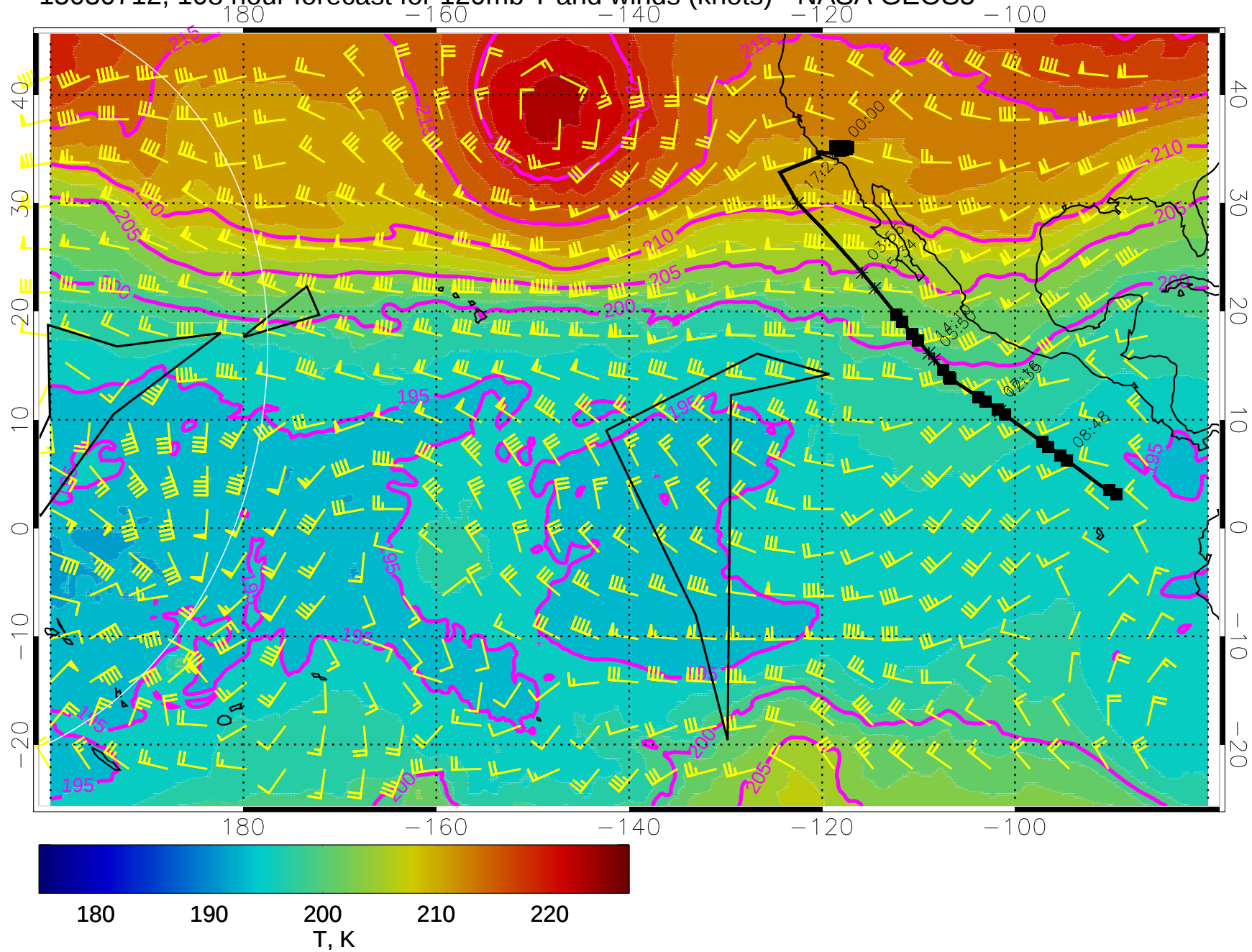
15030712, 108 hour forecast for 120mb T and winds (knots) - NASA GEOS5
