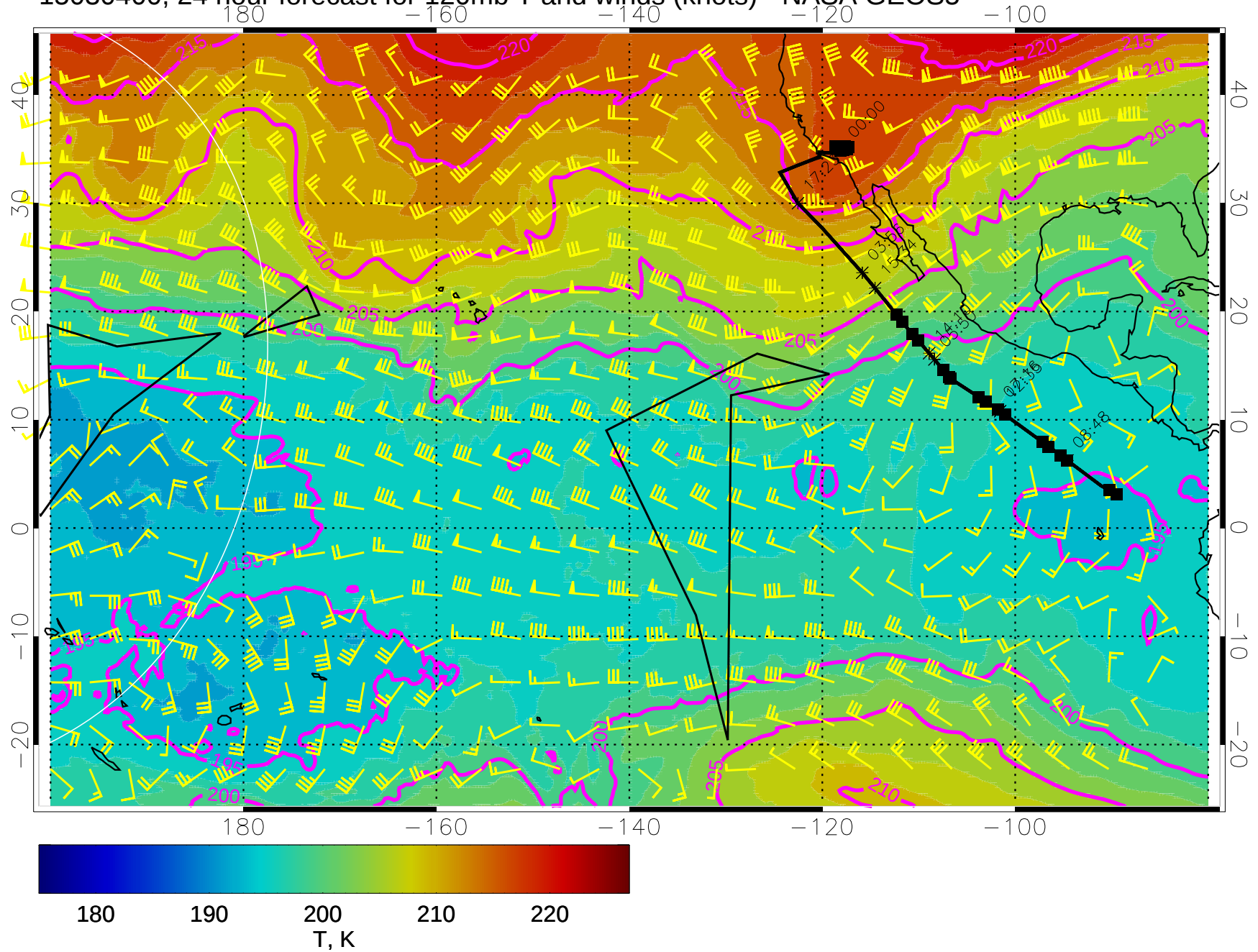
15030400, 24 hour forecast for 120mb T and winds (knots) - NASA GEOS5
