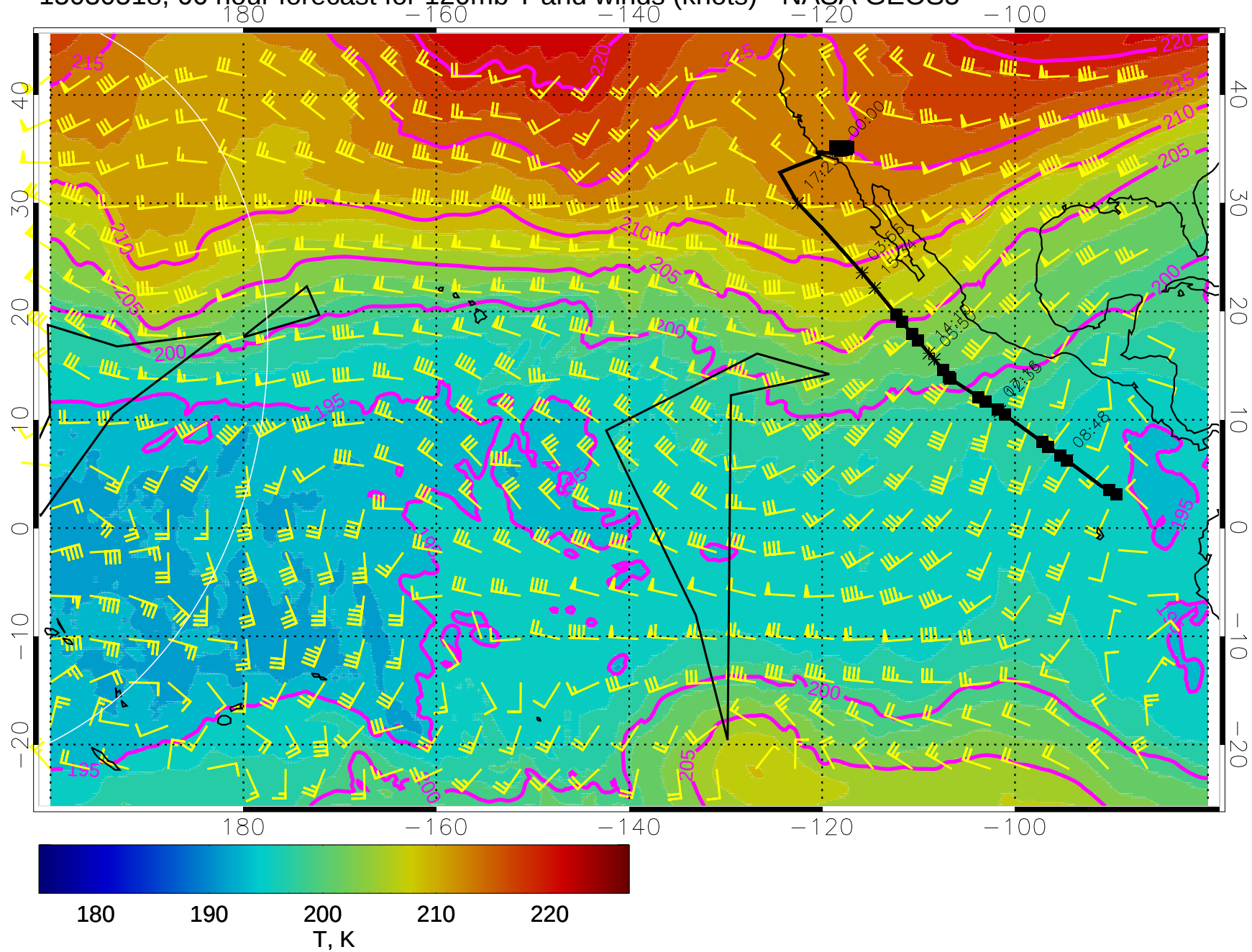
15030518, 66 hour forecast for 120mb T and winds (knots) - NASA GEOS5
