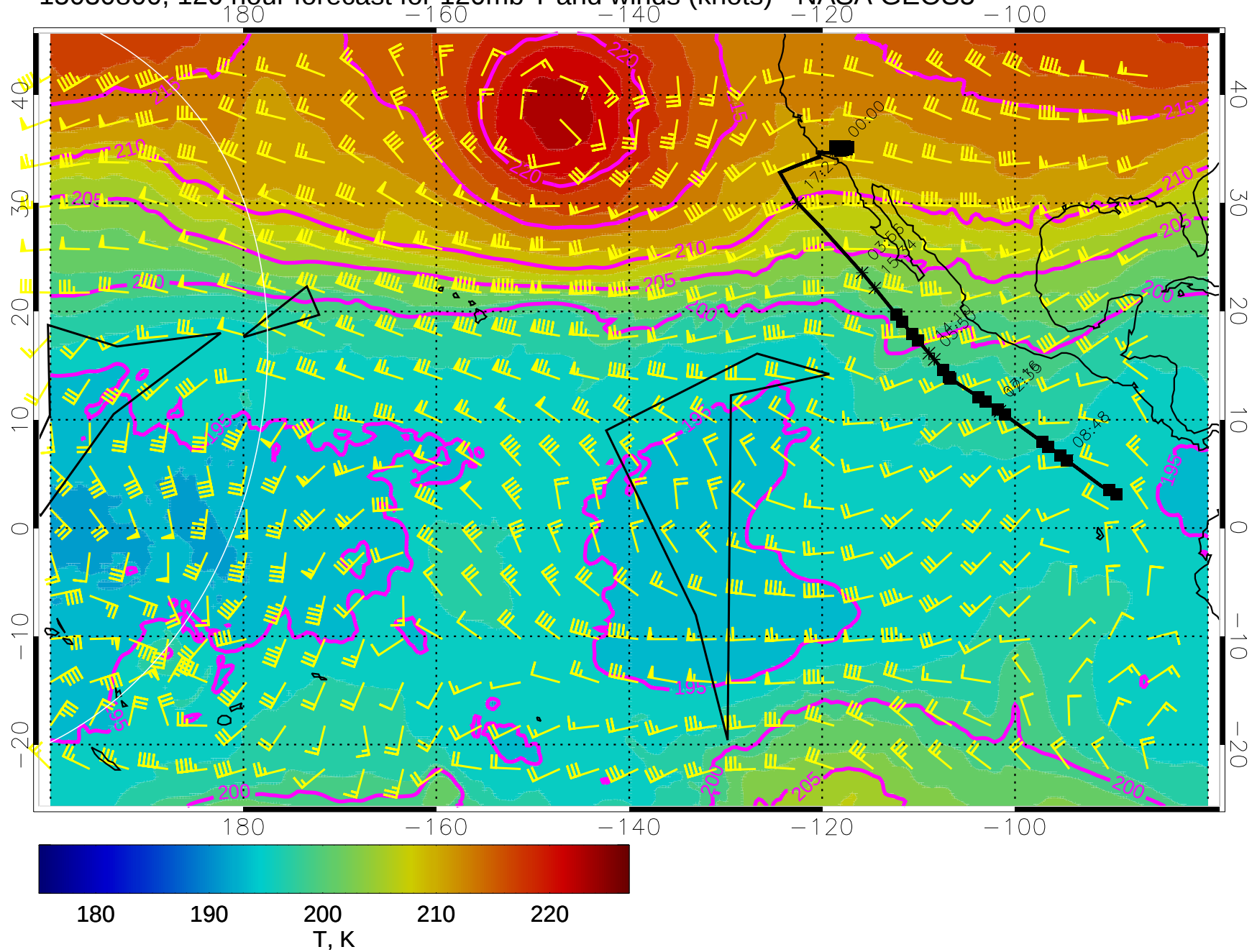
15030800, 120 hour forecast for 120mb T and winds (knots) - NASA GEOS5
