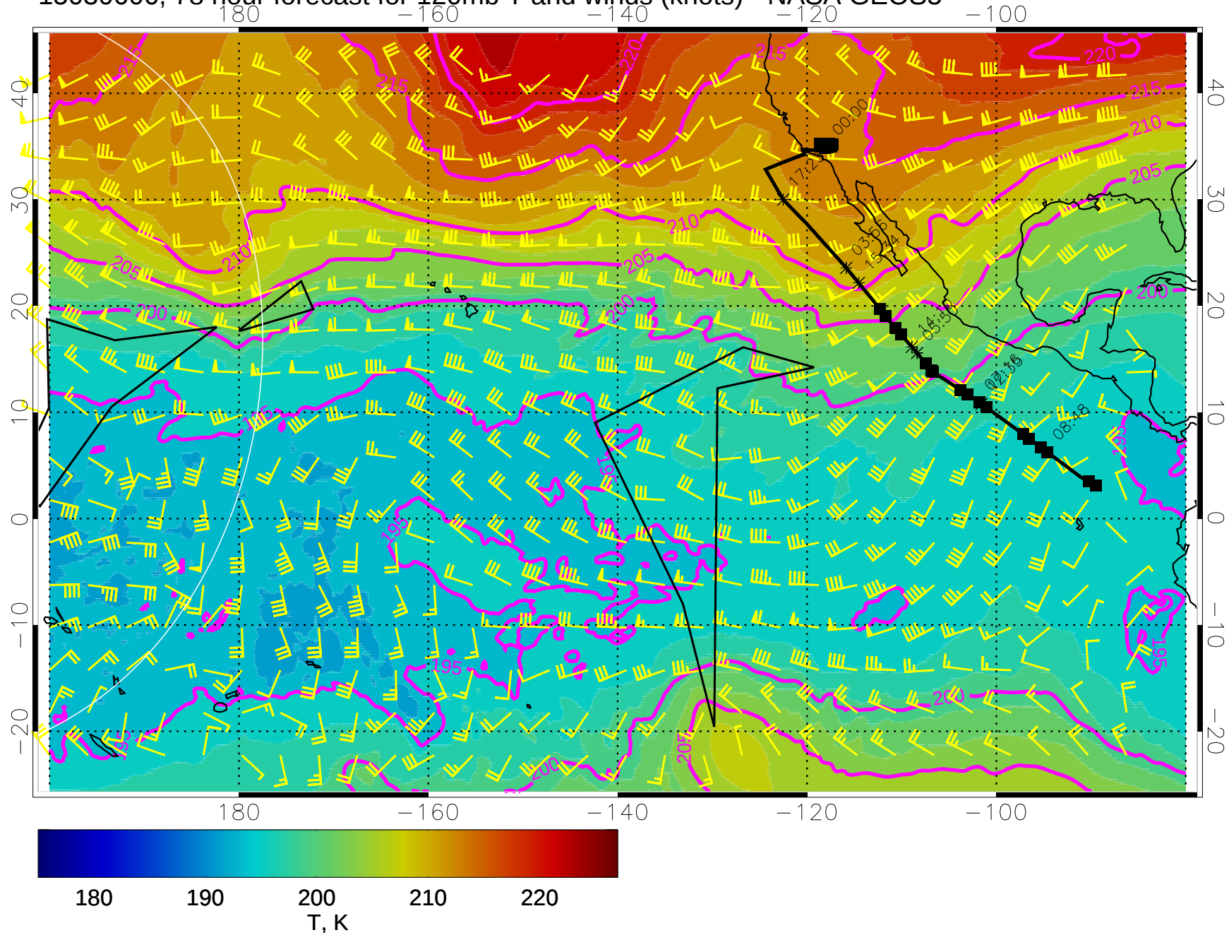
15030606, 78 hour forecast for 120mb T and winds (knots) - NASA GEOS5
