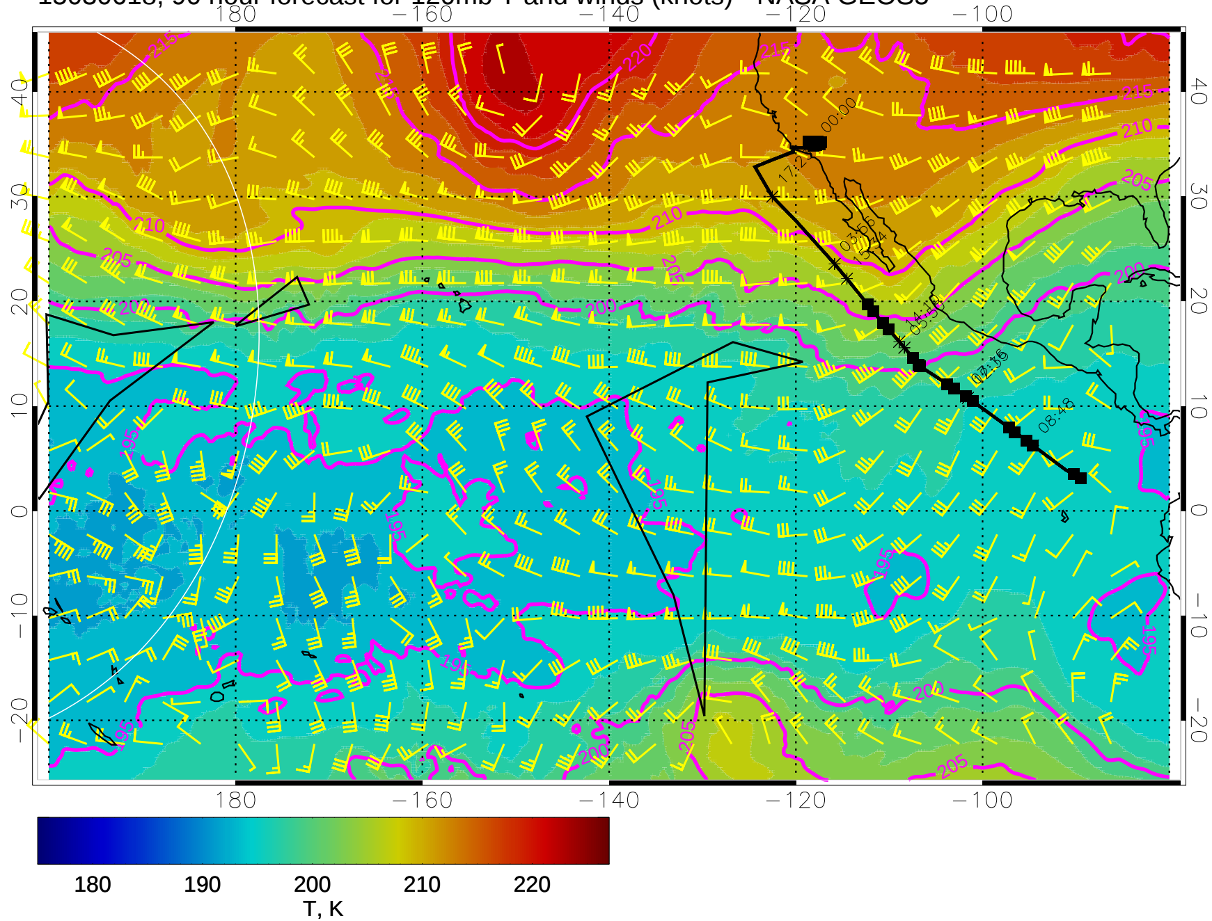
15030618, 90 hour forecast for 120mb T and winds (knots) - NASA GEOS5
