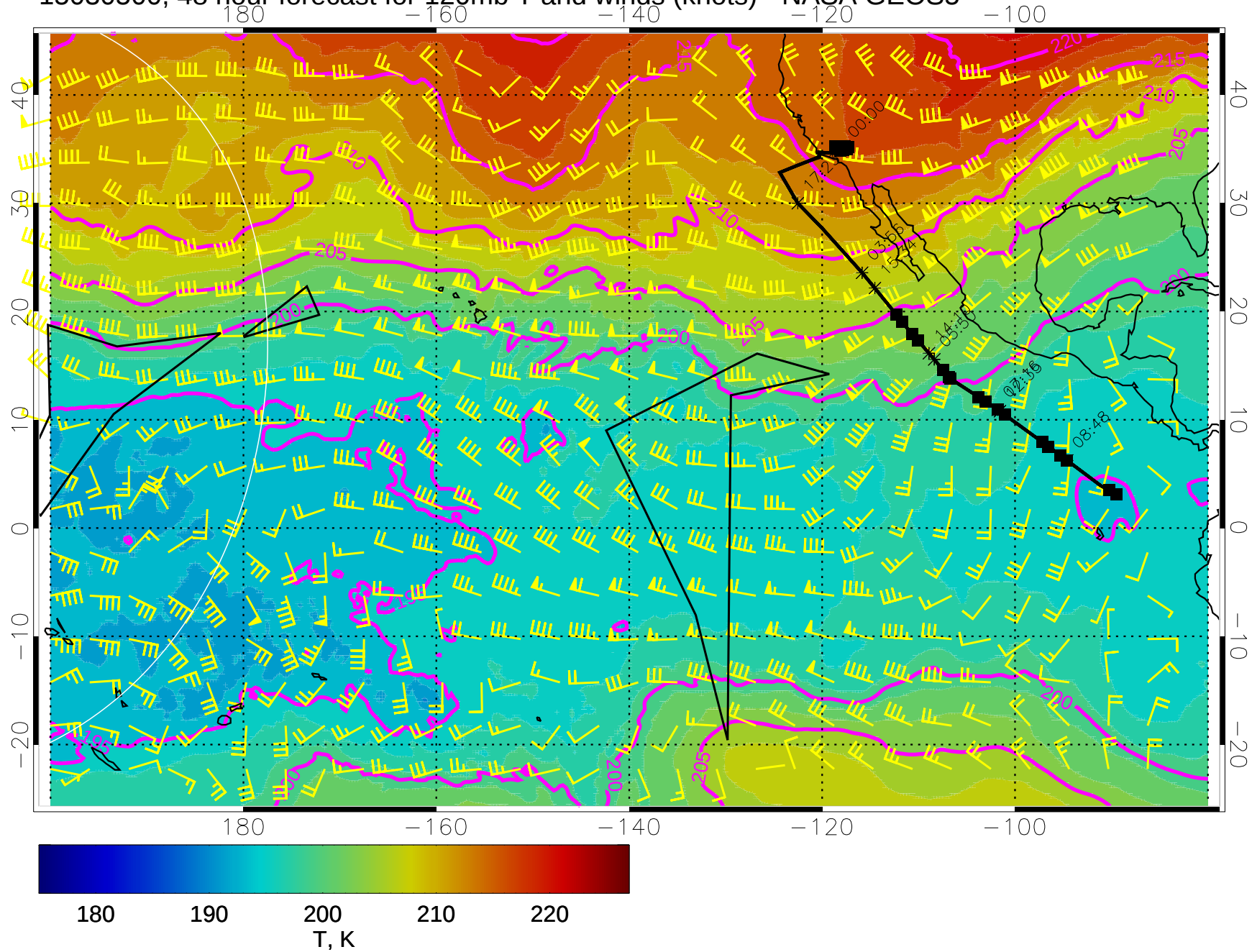
15030500, 48 hour forecast for 120mb T and winds (knots) - NASA GEOS5
