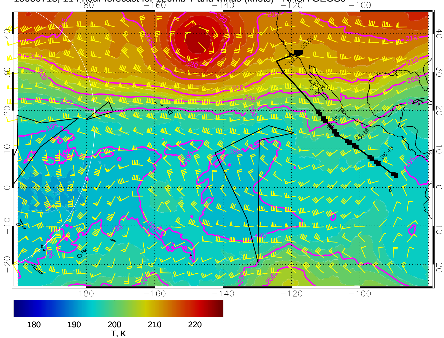
15030718, 114 hour forecast for 120mb T and winds (knots) - NASA GEOS5
