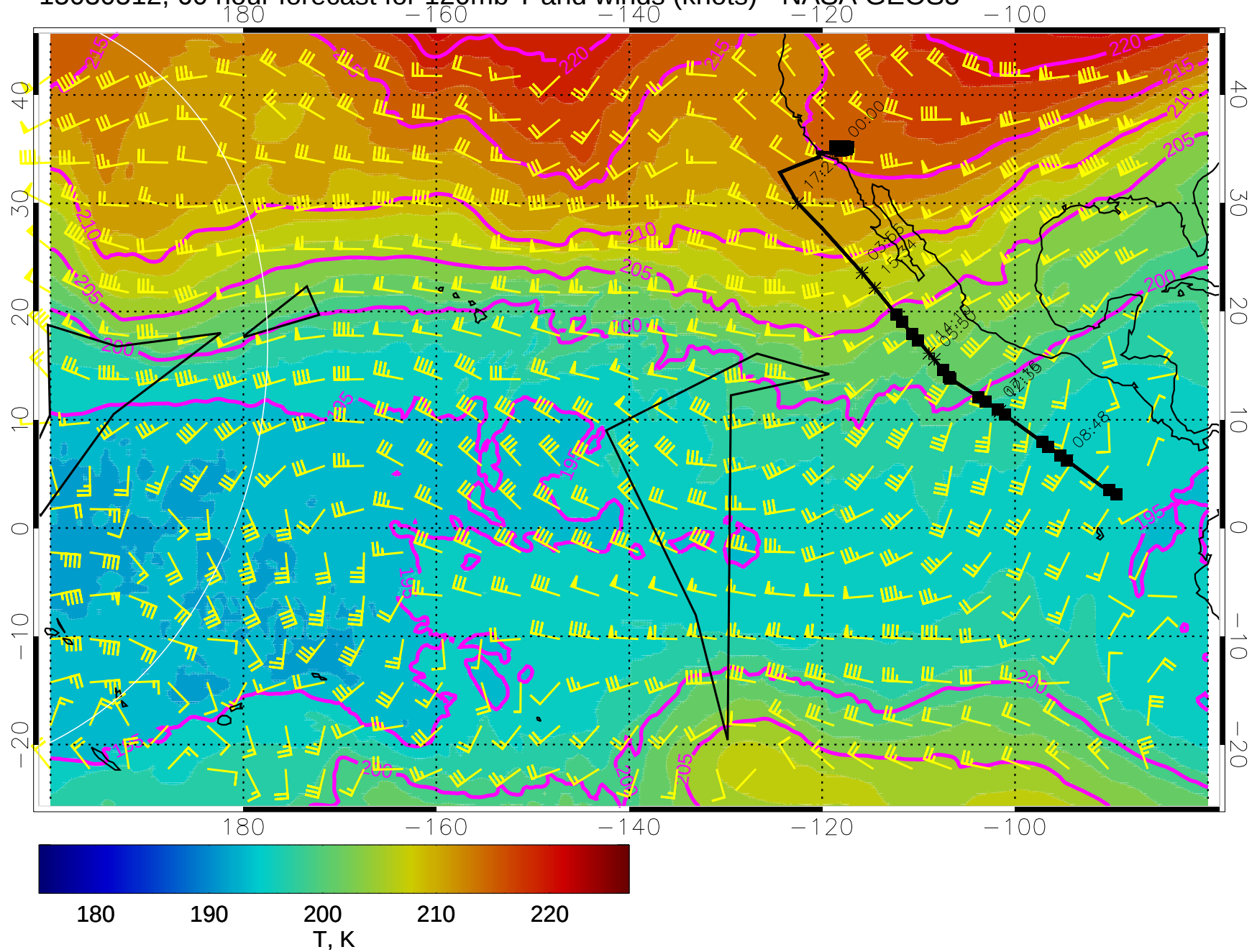
15030512, 60 hour forecast for 120mb T and winds (knots) - NASA GEOS5
