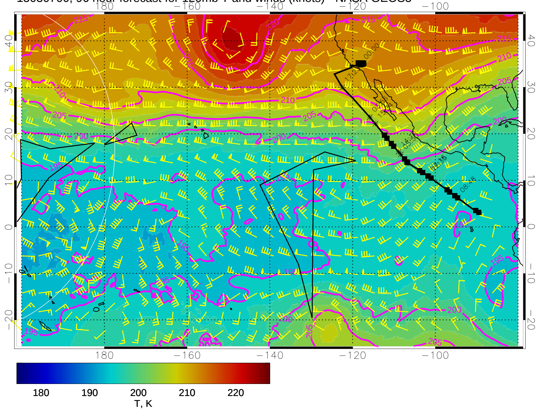
15030700, 96 hour forecast for 120mb T and winds (knots) - NASA GEOS5
