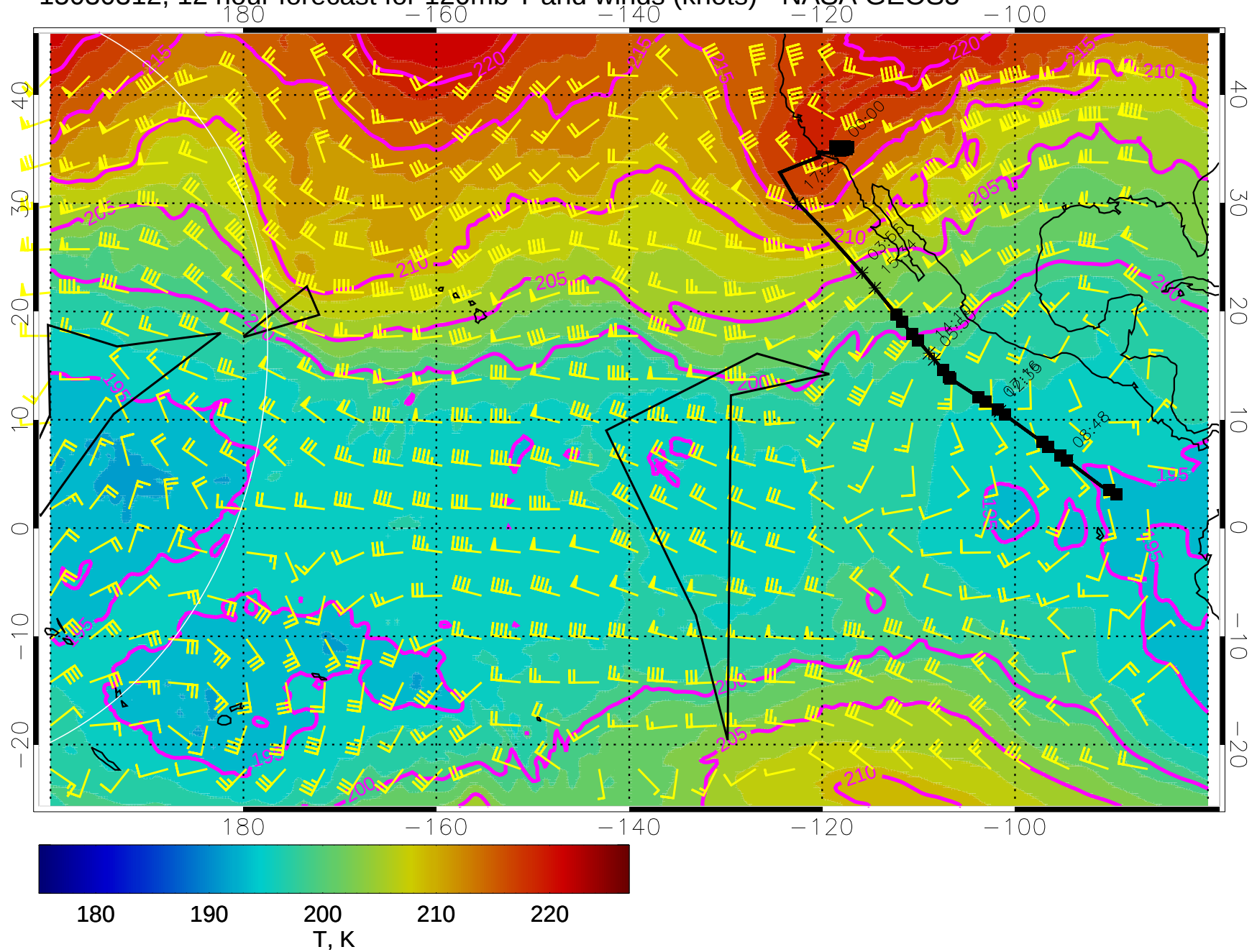
15030312, 12 hour forecast for 120mb T and winds (knots) - NASA GEOS5
