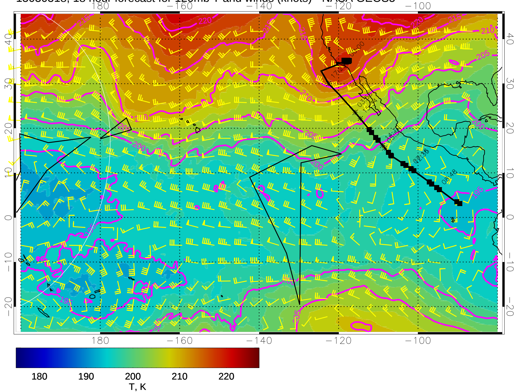
15030318, 18 hour forecast for 120mb T and winds (knots) - NASA GEOS5
