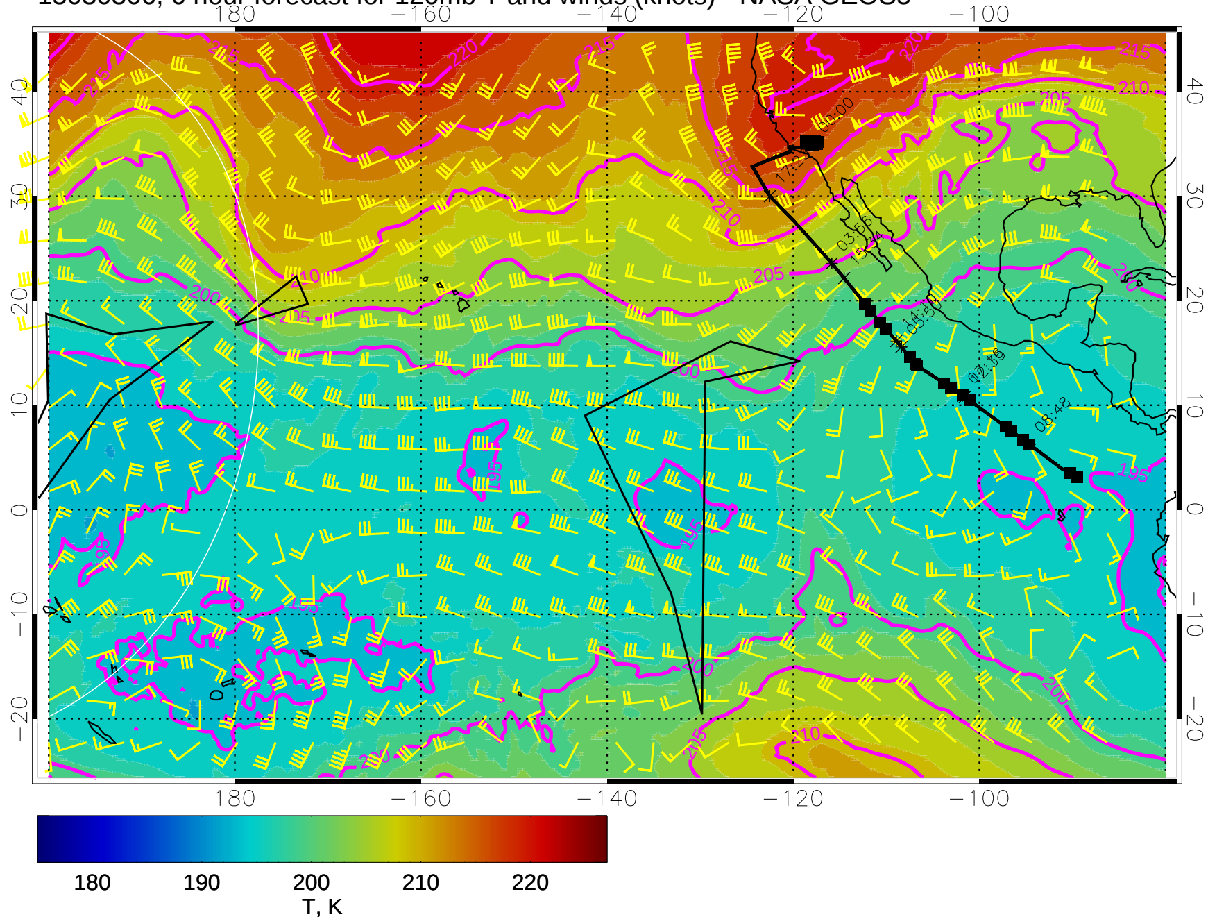
15030306, 6 hour forecast for 120mb T and winds (knots) - NASA GEOS5
