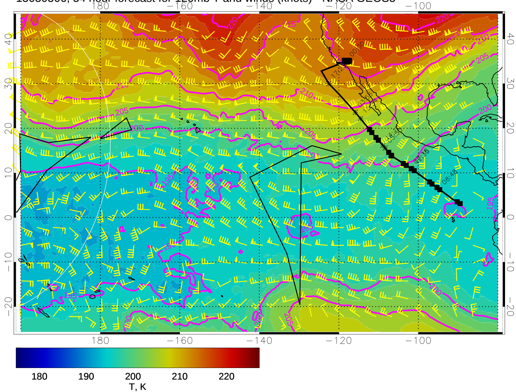
15030506, 54 hour forecast for 120mb T and winds (knots) - NASA GEOS5
