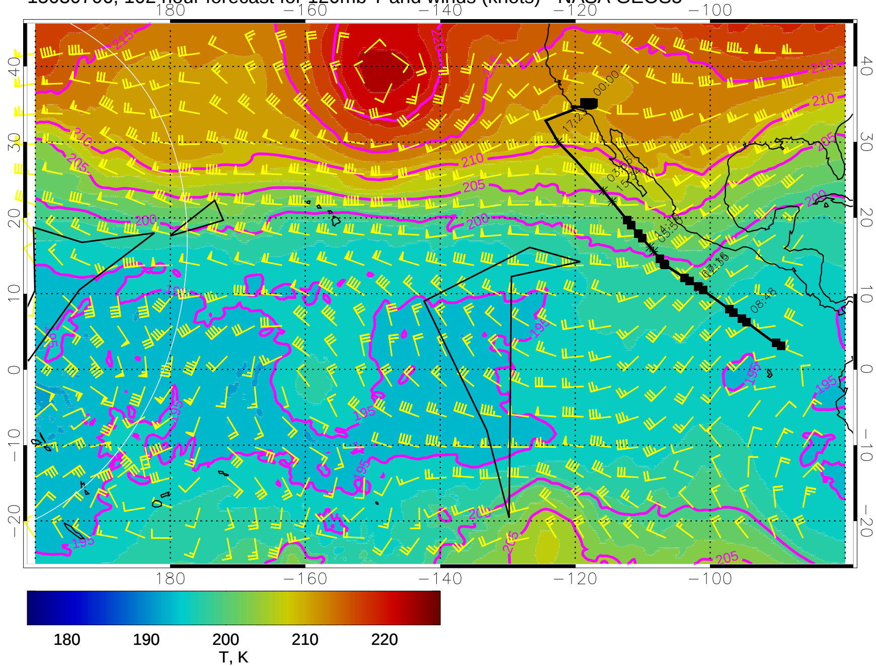
15030706, 102 hour forecast for 120mb T and winds (knots) - NASA GEOS5
