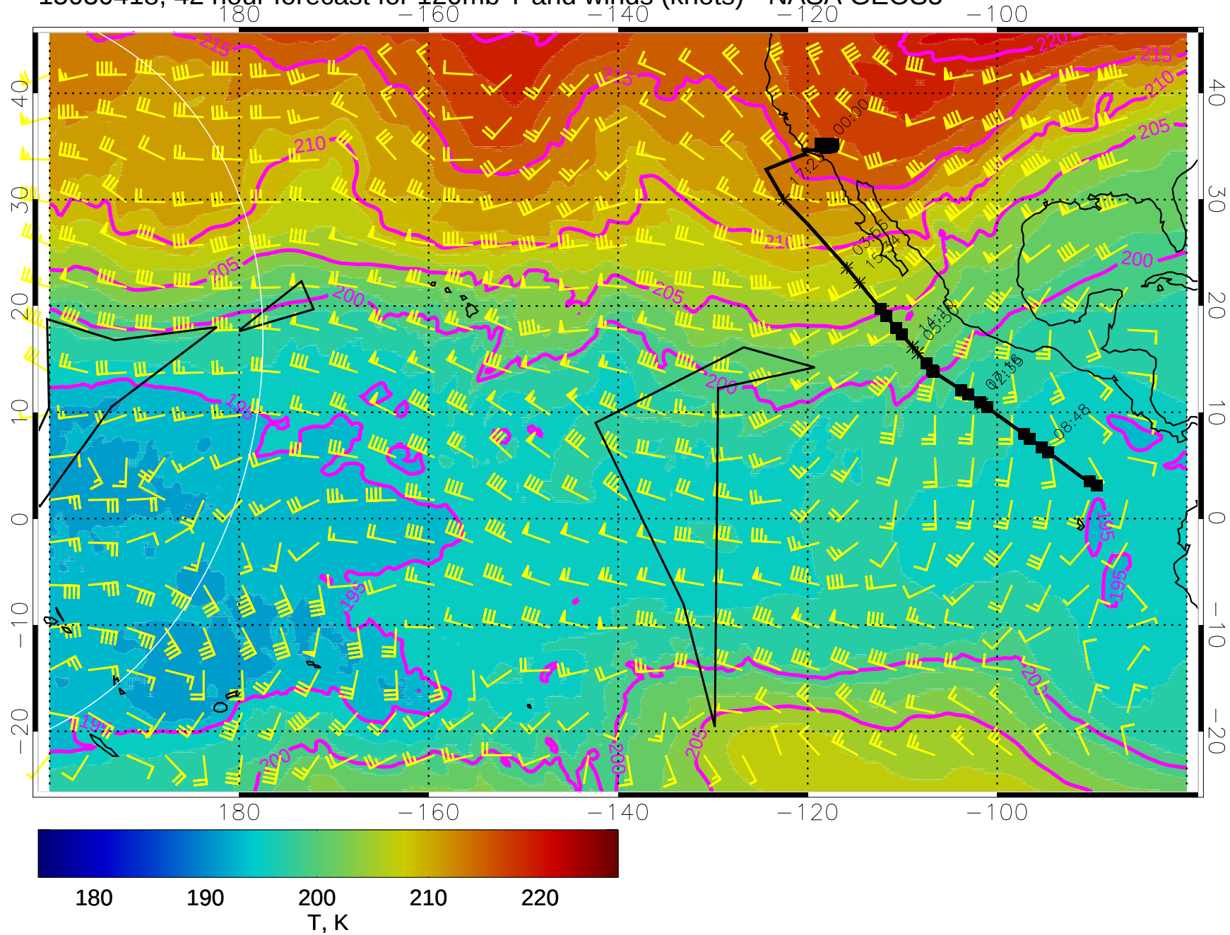
15030418, 42 hour forecast for 120mb T and winds (knots) - NASA GEOS5
