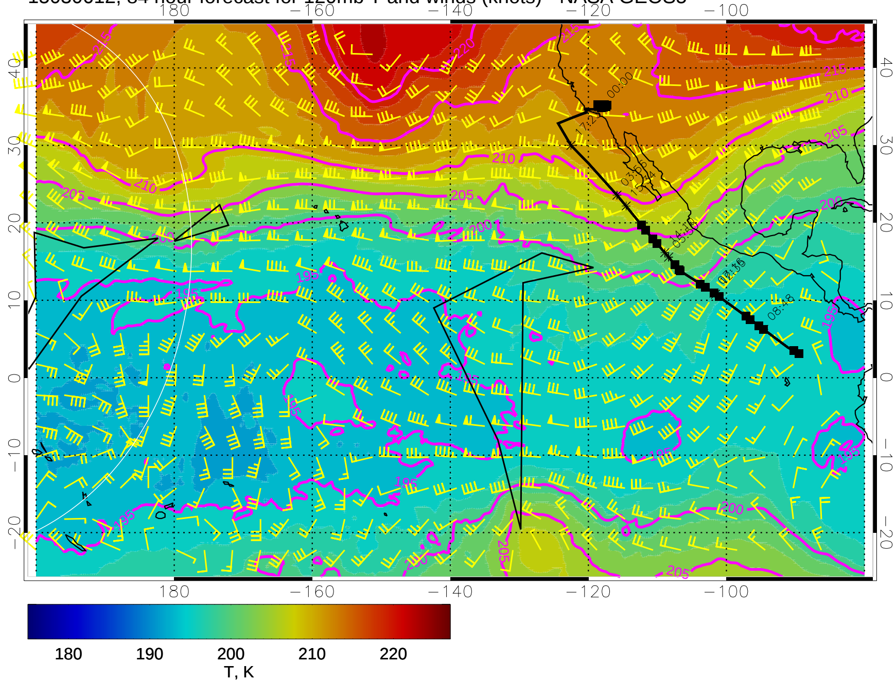
15030612, 84 hour forecast for 120mb T and winds (knots) - NASA GEOS5
