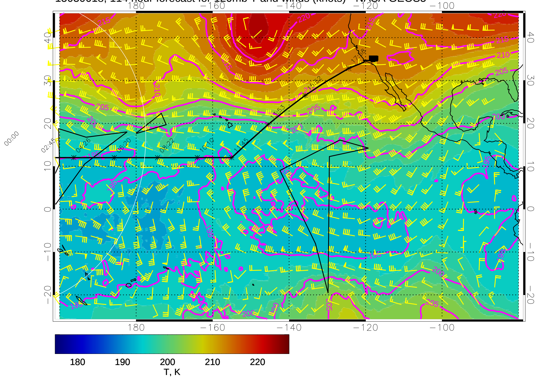
15030618, 114 hour forecast for 120mb T and winds (knots) - NASA GEOS5
