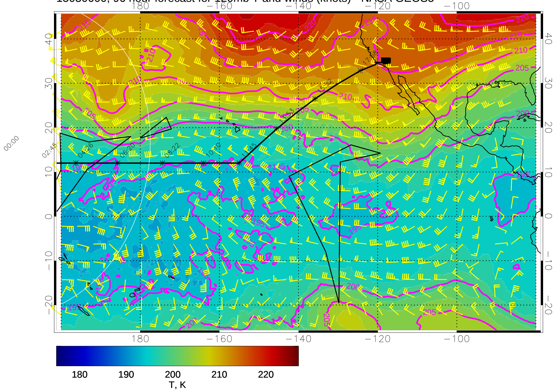
15030600, 96 hour forecast for 120mb T and winds (knots) - NASA GEOS5
