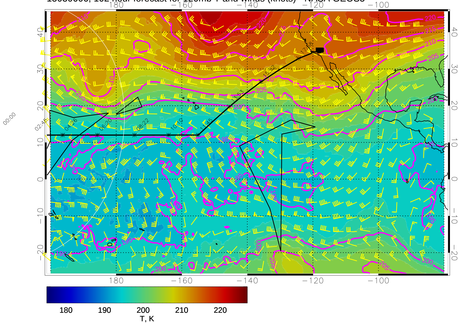
15030606, 102 hour forecast for 120mb T and winds (knots) - NASA GEOS5
