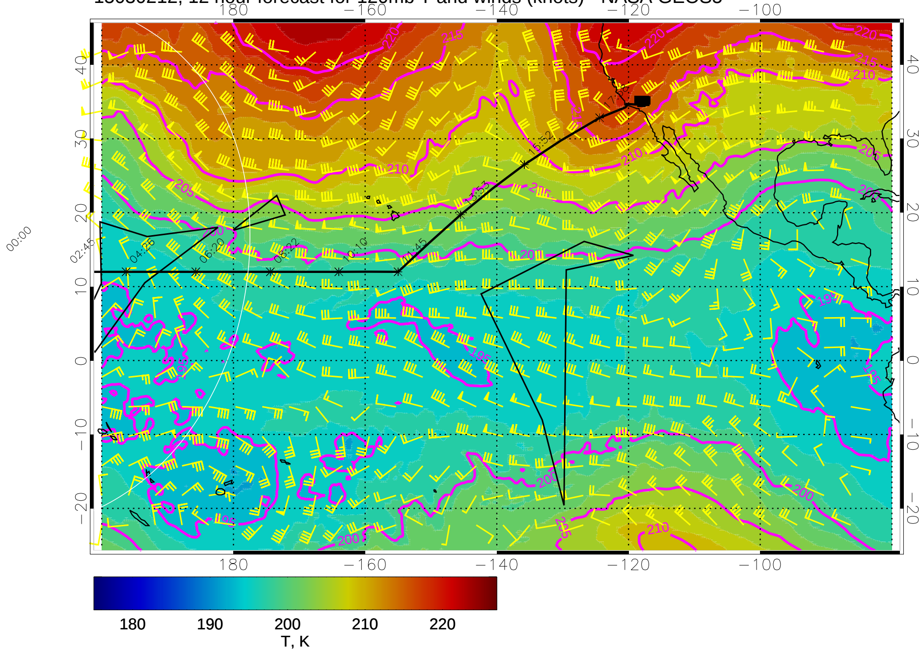
15030212, 12 hour forecast for 120mb T and winds (knots) - NASA GEOS5
