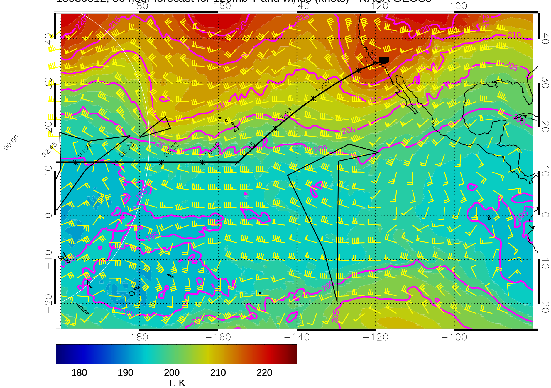
15030312, 36 hour forecast for 120mb T and winds (knots) - NASA GEOS5
