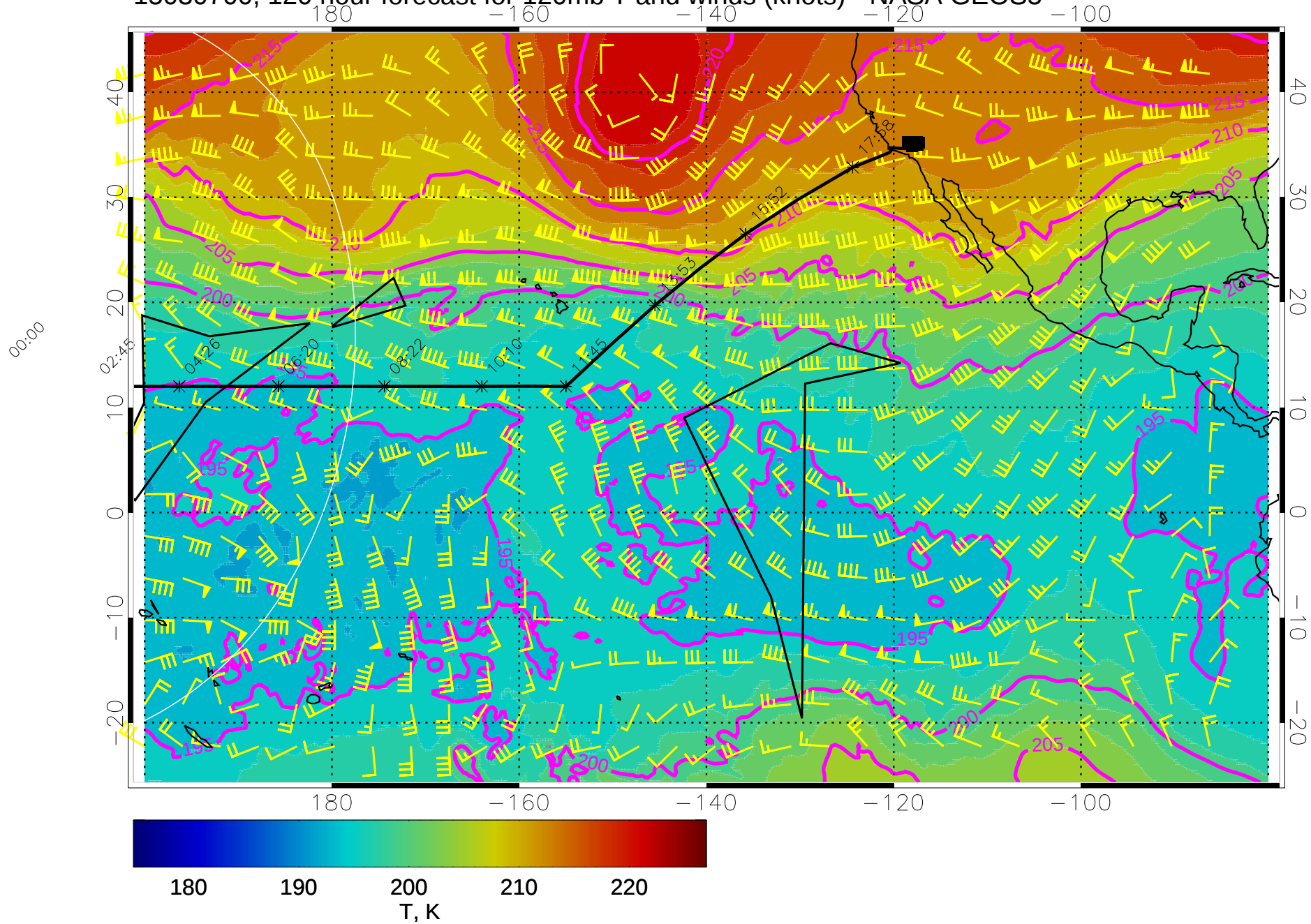
15030700, 120 hour forecast for 120mb T and winds (knots) - NASA GEOS5
