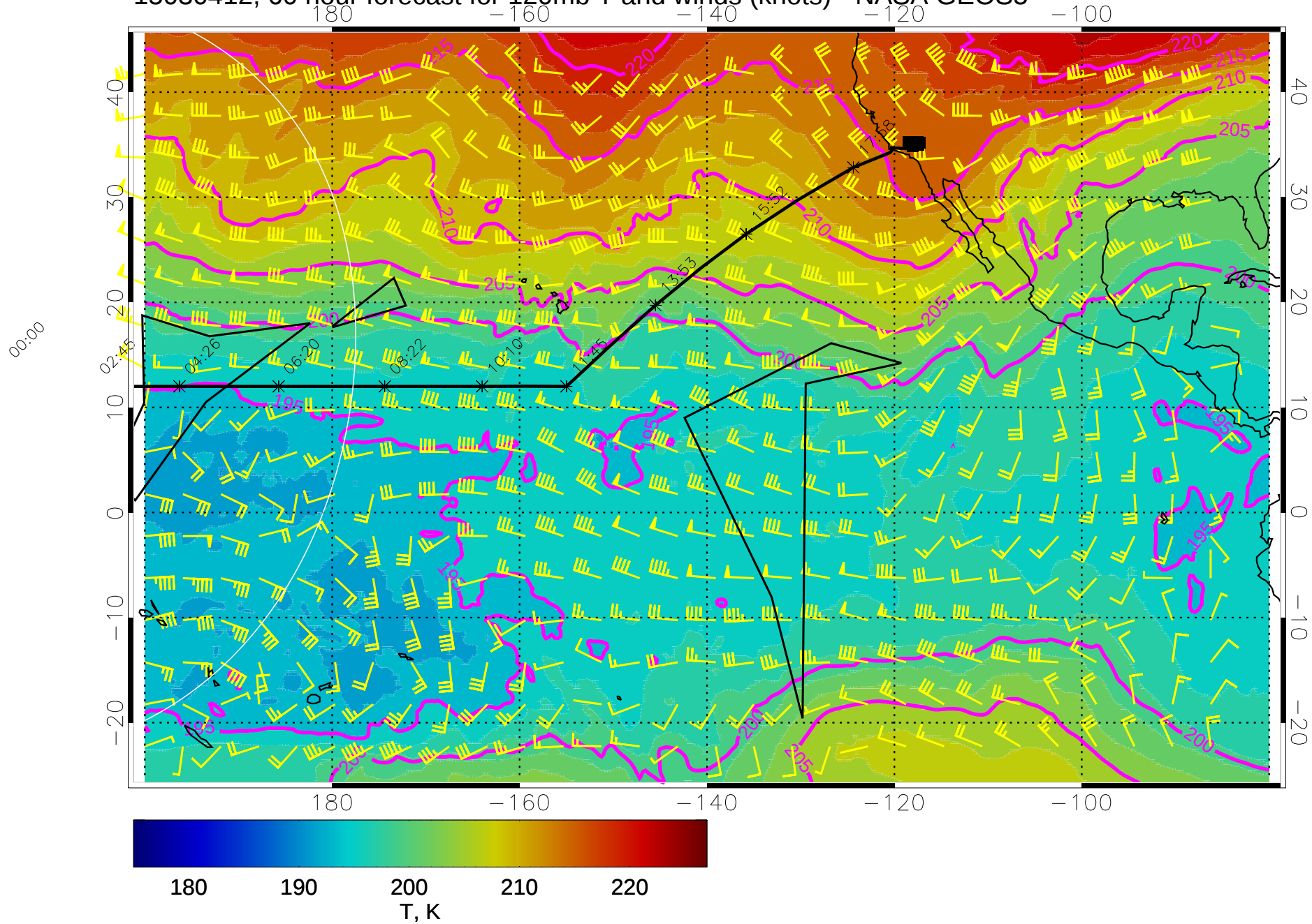
15030412, 60 hour forecast for 120mb T and winds (knots) - NASA GEOS5
