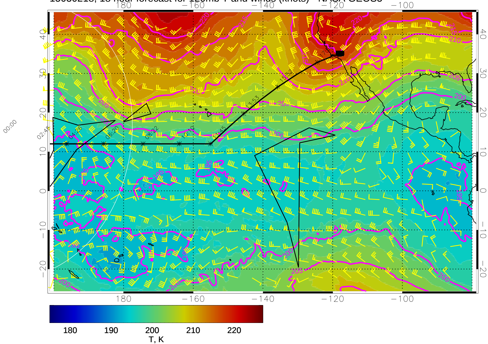
15030218, 18 hour forecast for 120mb T and winds (knots) - NASA GEOS5
