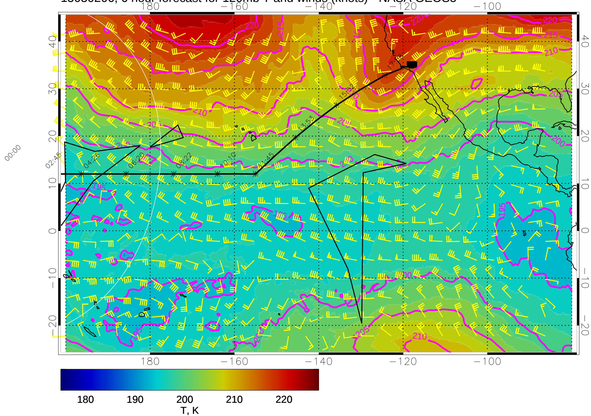
15030206, 6 hour forecast for 120mb T and winds (knots) - NASA GEOS5
