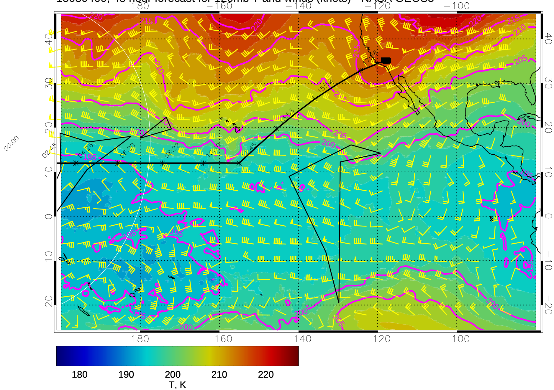
15030400, 48 hour forecast for 120mb T and winds (knots) - NASA GEOS5
