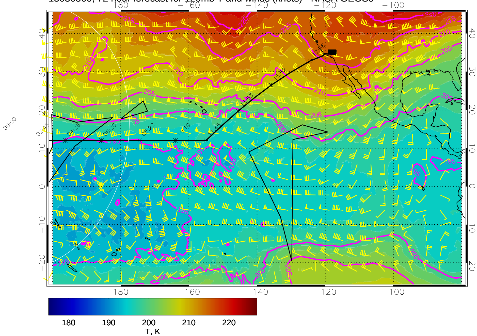
15030500, 72 hour forecast for 120mb T and winds (knots) - NASA GEOS5
