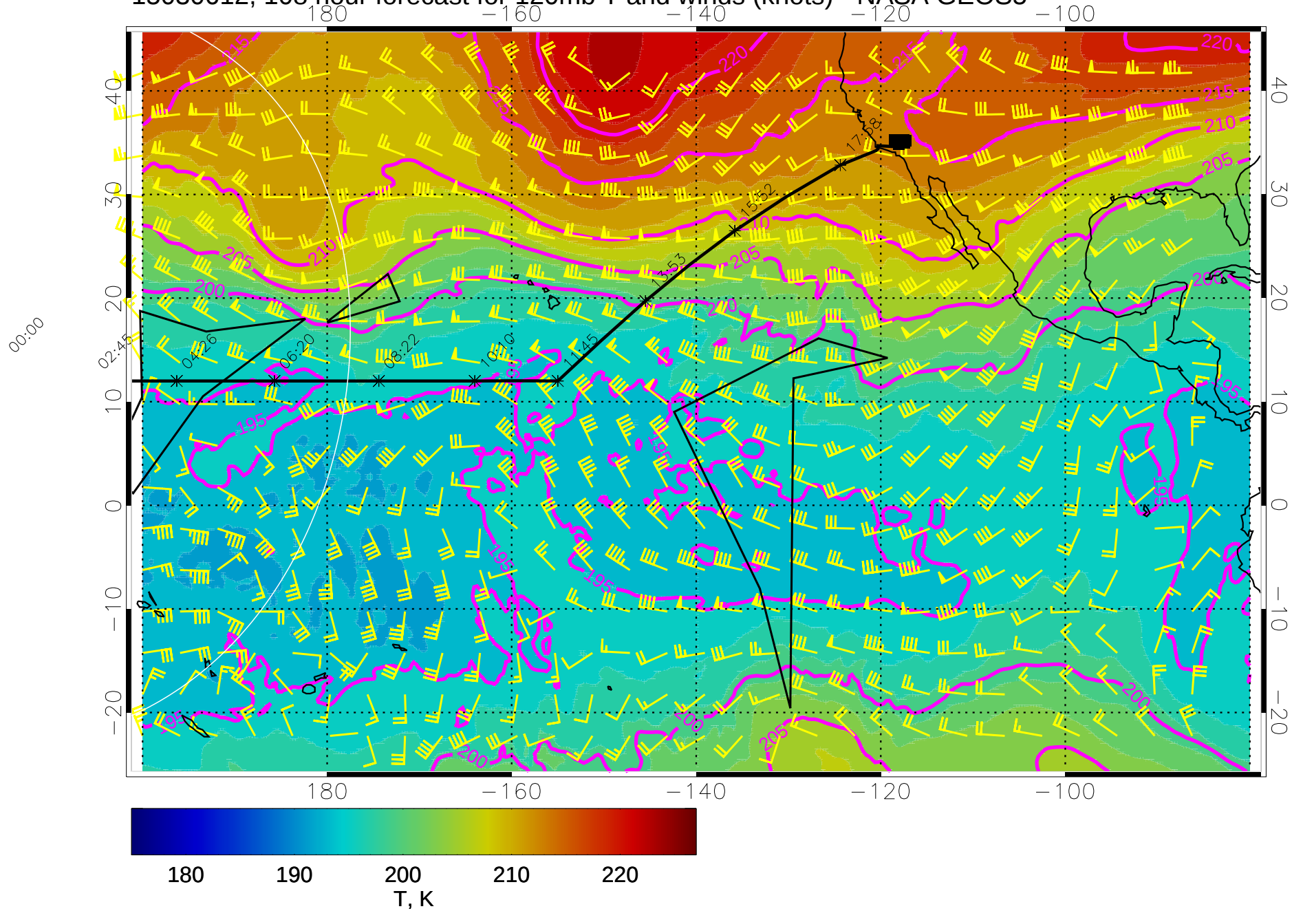
15030612, 108 hour forecast for 120mb T and winds (knots) - NASA GEOS5
