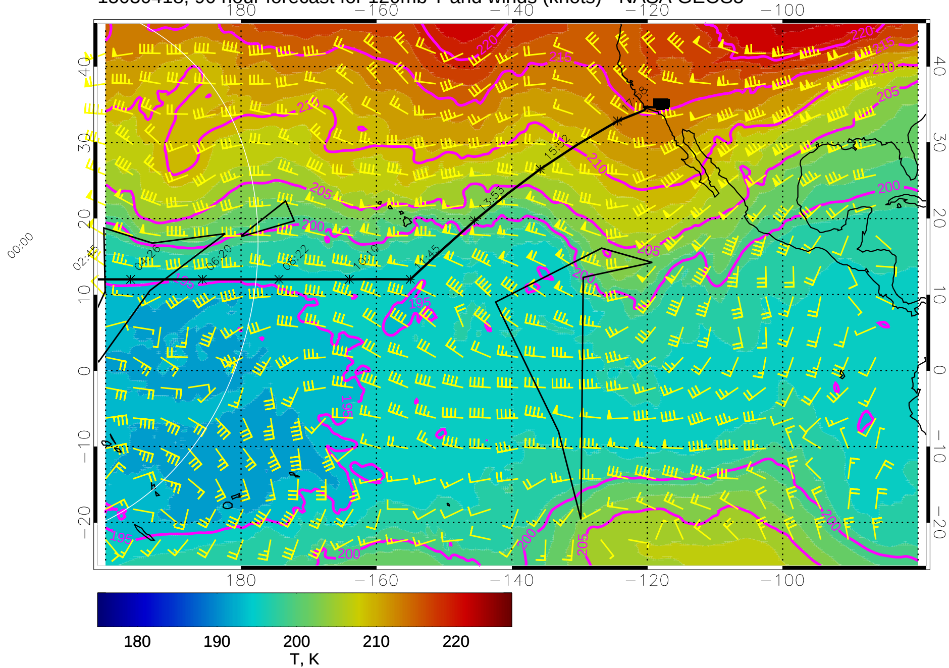
15030418, 90 hour forecast for 120mb T and winds (knots) - NASA GEOS5
