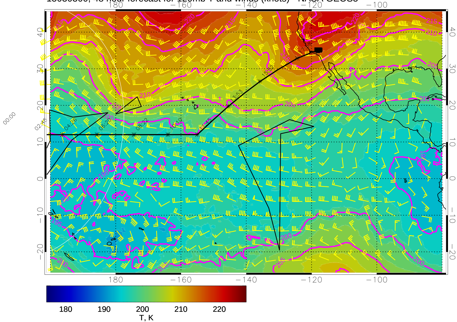
15030300, 48 hour forecast for 120mb T and winds (knots) - NASA GEOS5
