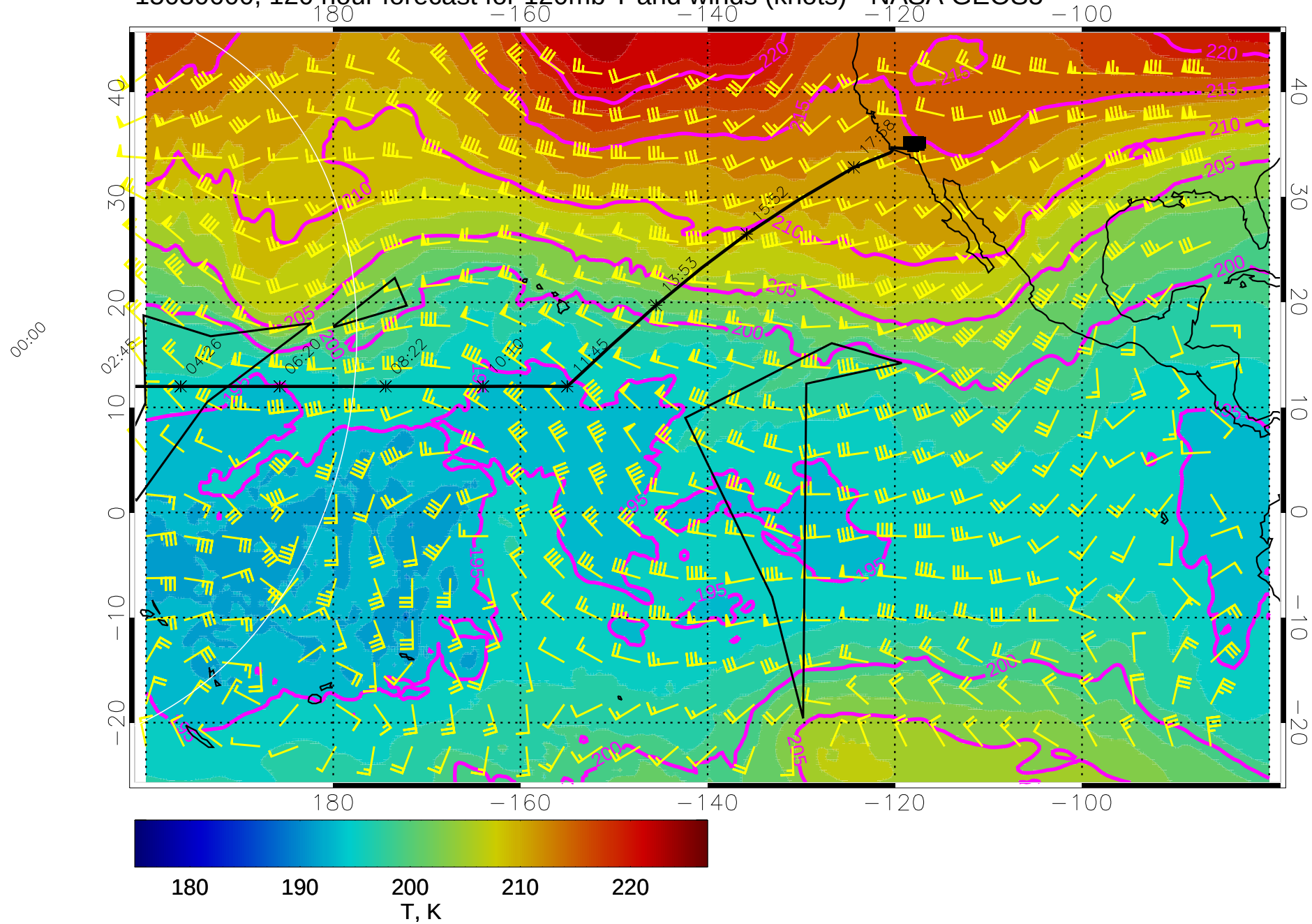
15030600, 120 hour forecast for 120mb T and winds (knots) - NASA GEOS5
