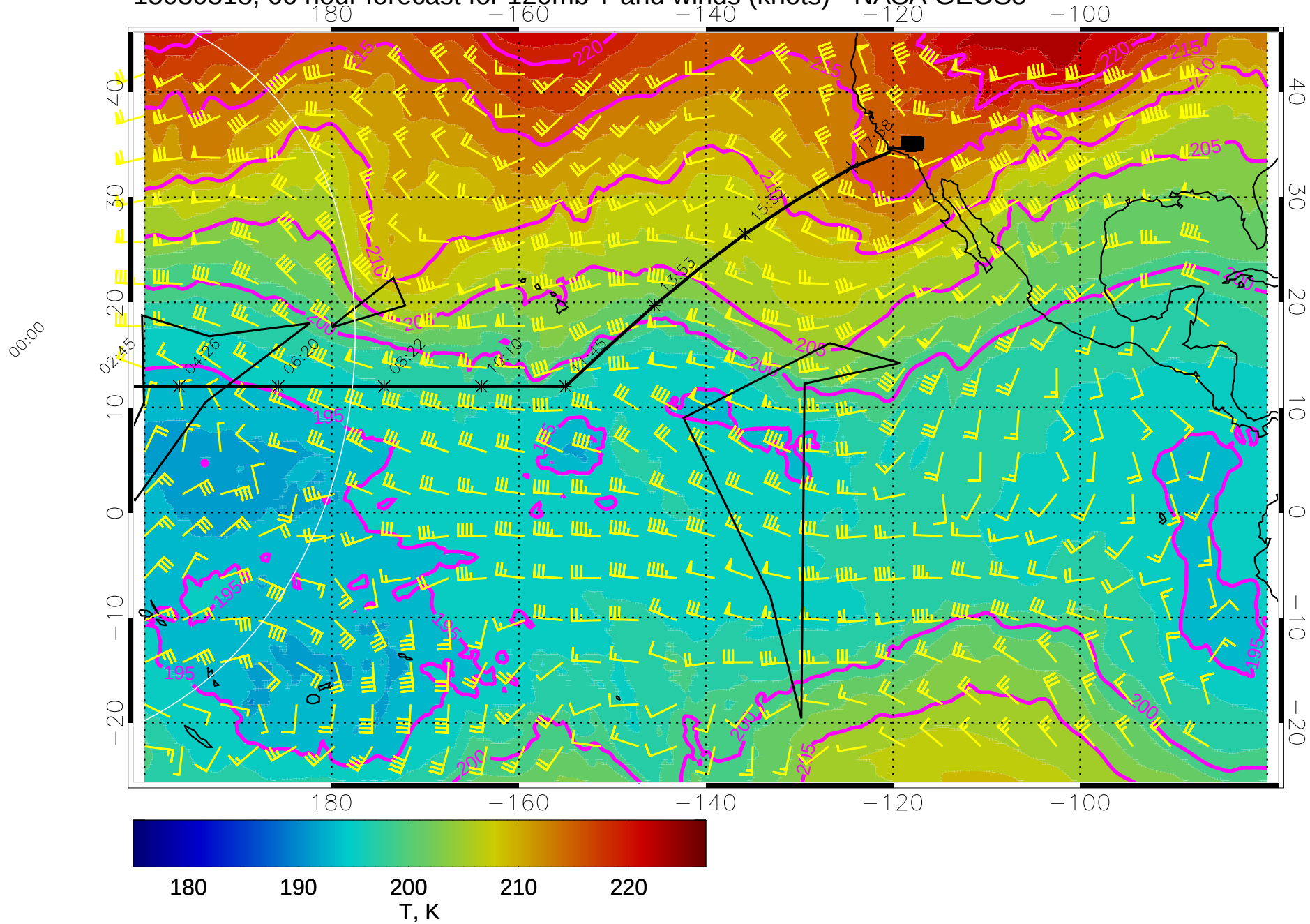
15030318, 66 hour forecast for 120mb T and winds (knots) - NASA GEOS5
