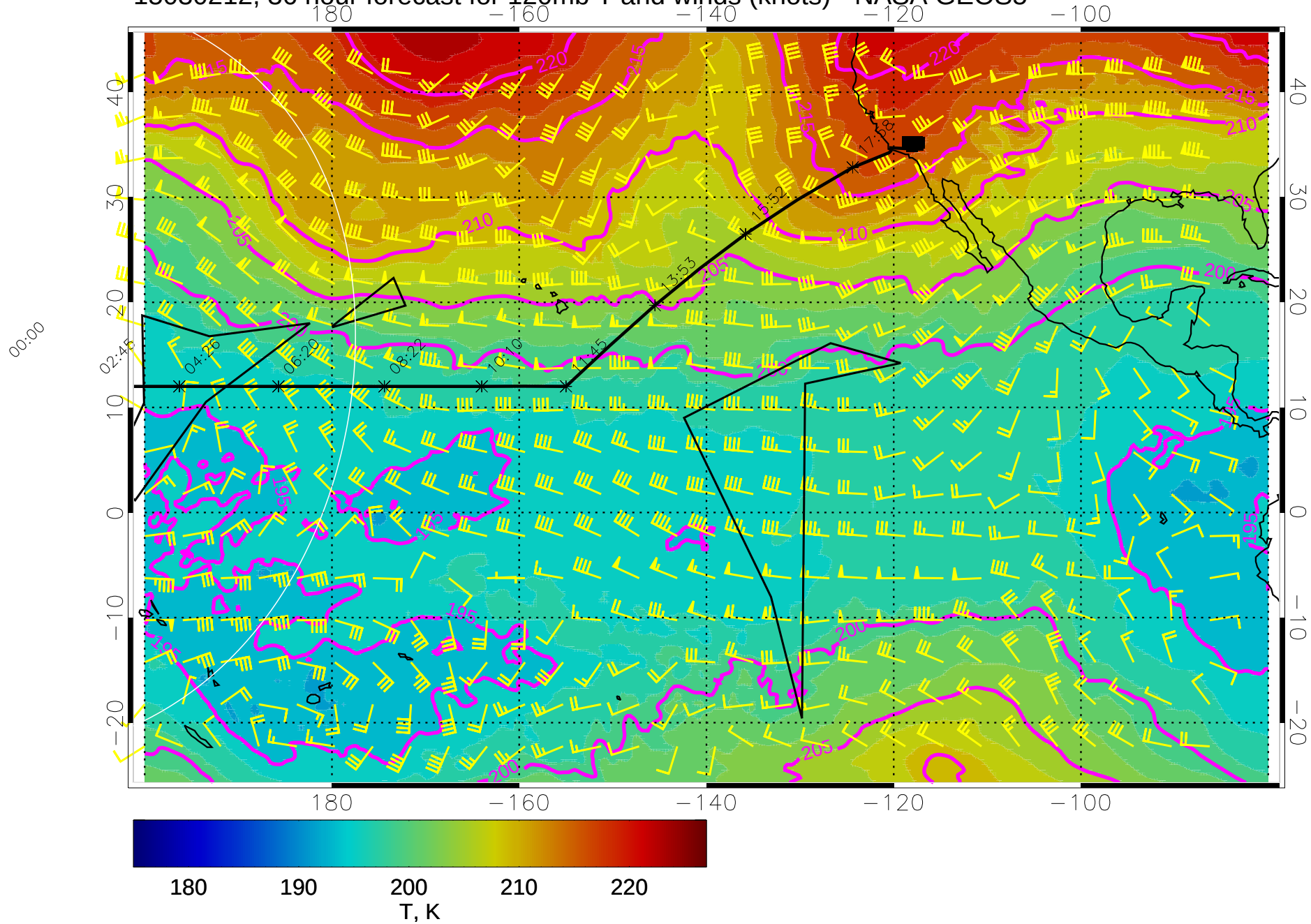
15030212, 36 hour forecast for 120mb T and winds (knots) - NASA GEOS5
