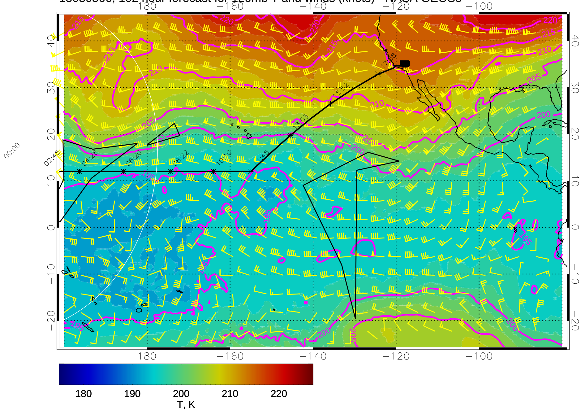
15030506, 102 hour forecast for 120mb T and winds (knots) - NASA GEOS5
