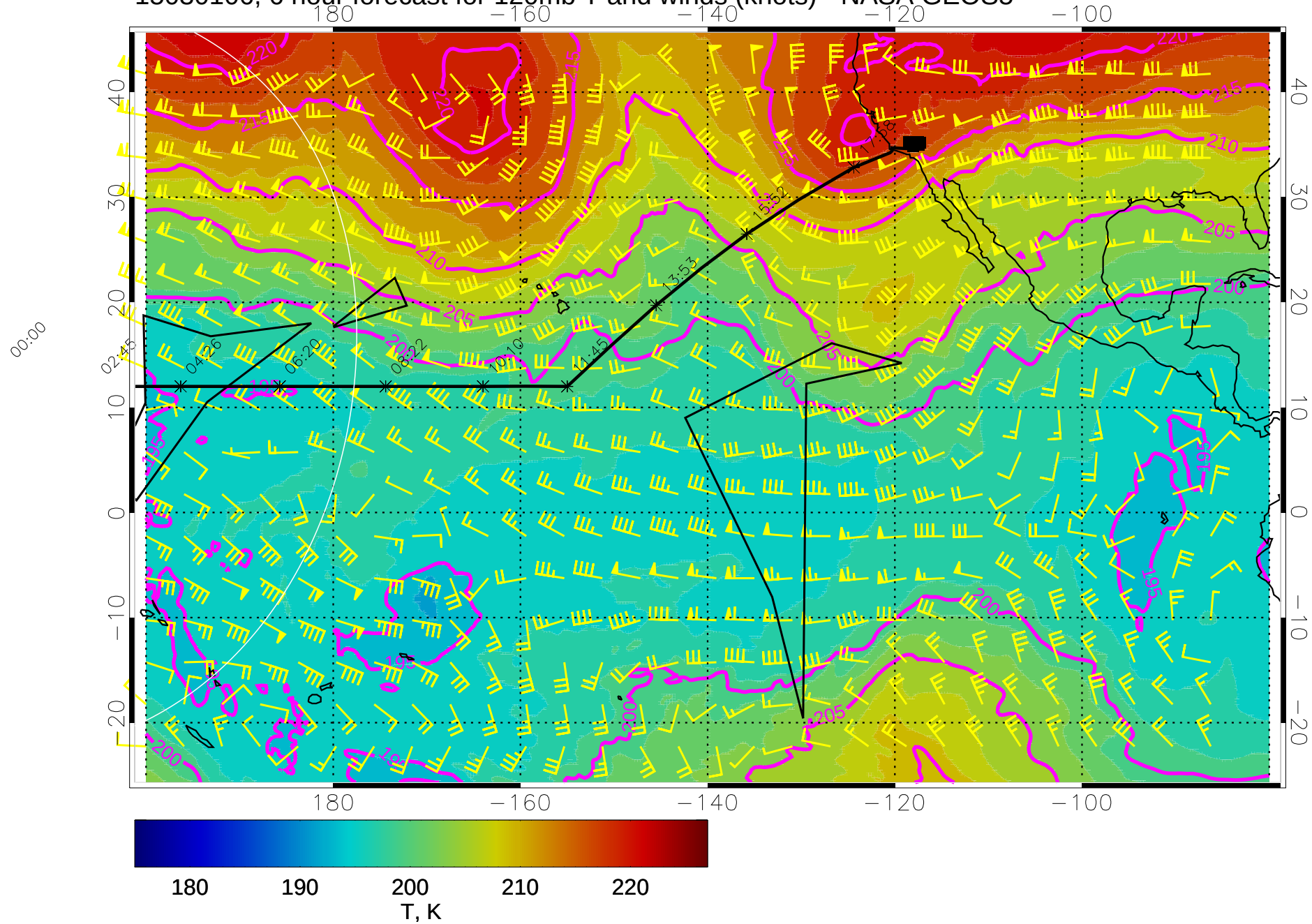
15030106, 6 hour forecast for 120mb T and winds (knots) - NASA GEOS5
