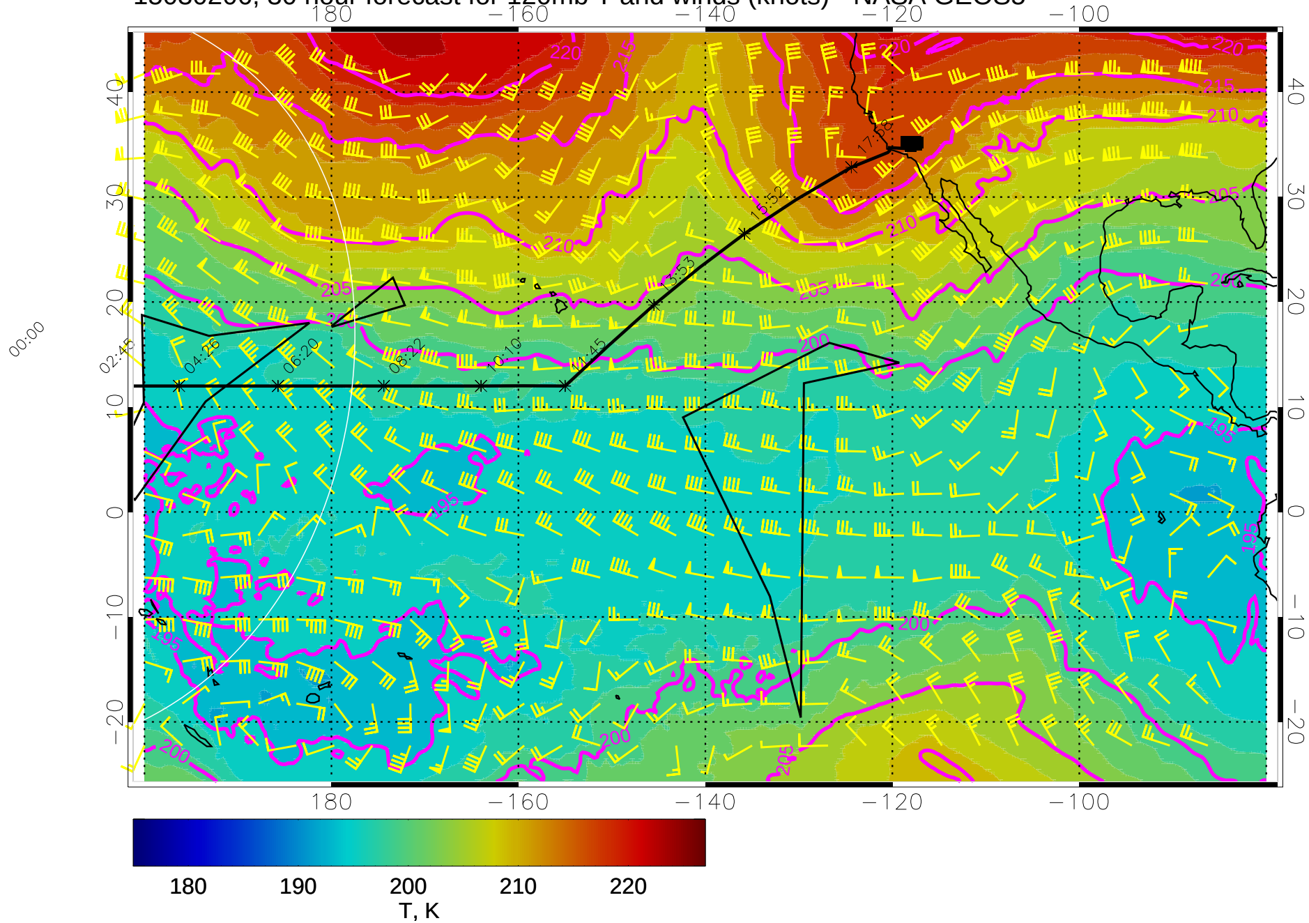
15030206, 30 hour forecast for 120mb T and winds (knots) - NASA GEOS5
