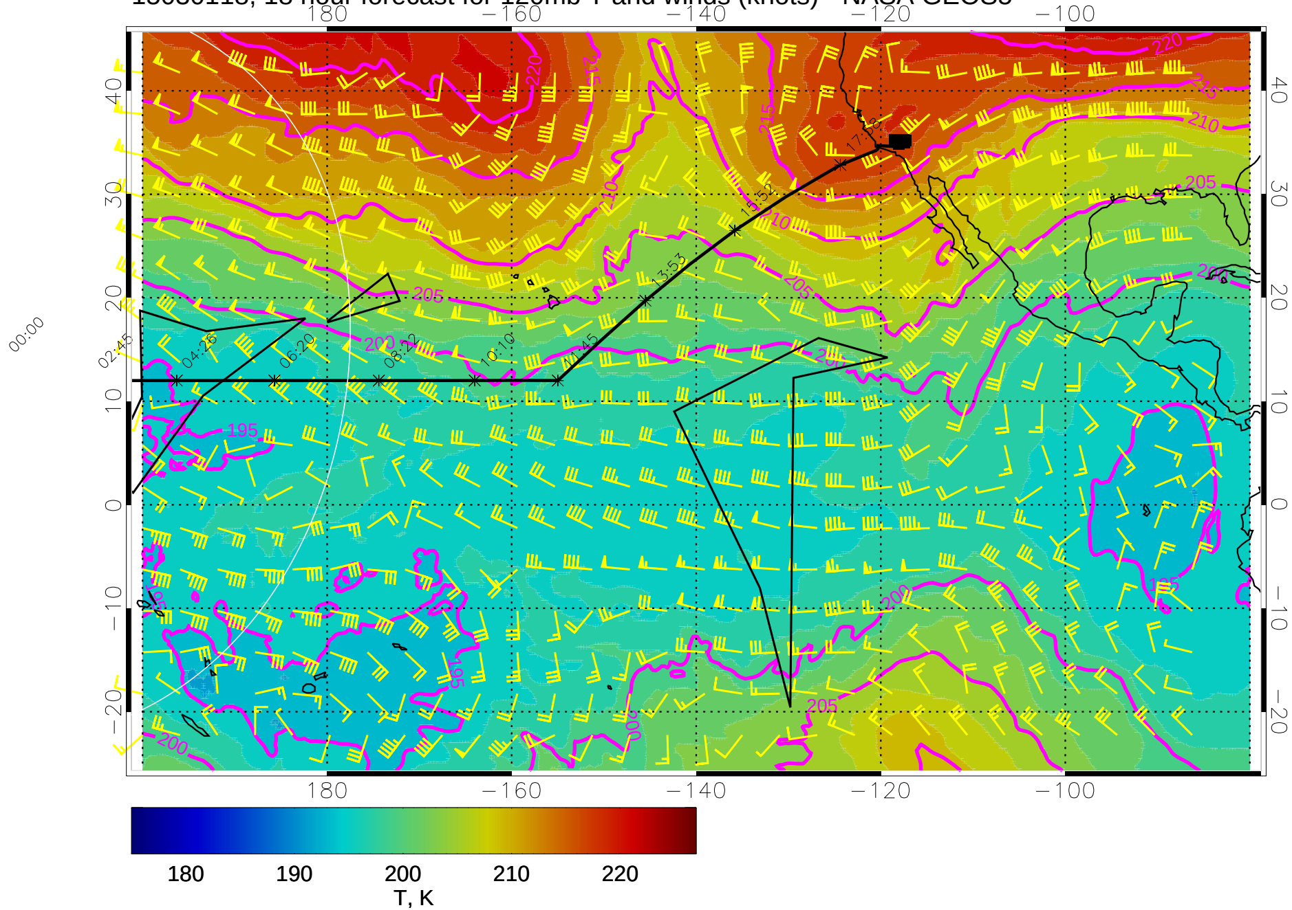
15030118, 18 hour forecast for 120mb T and winds (knots) - NASA GEOS5
