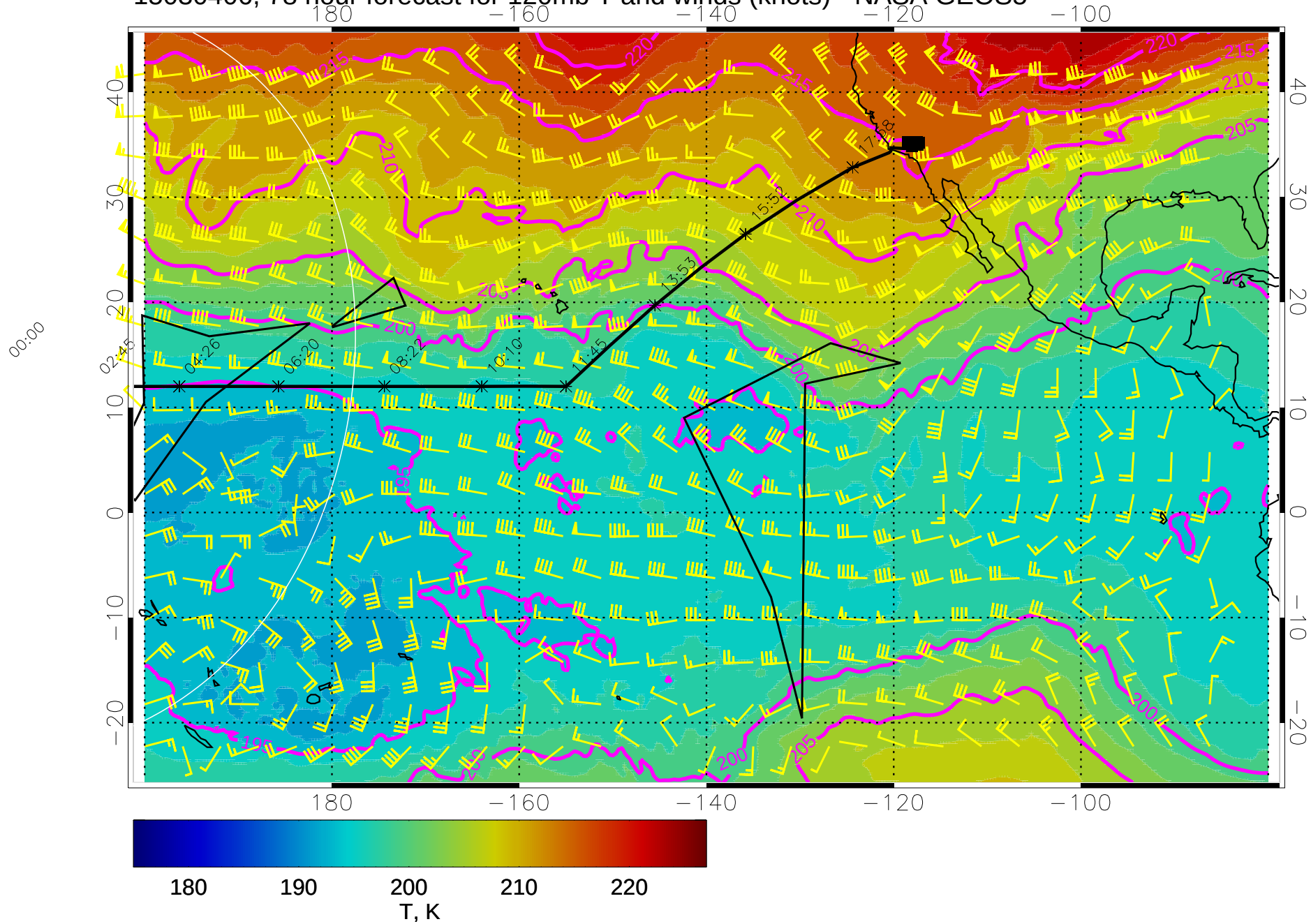
15030406, 78 hour forecast for 120mb T and winds (knots) - NASA GEOS5
