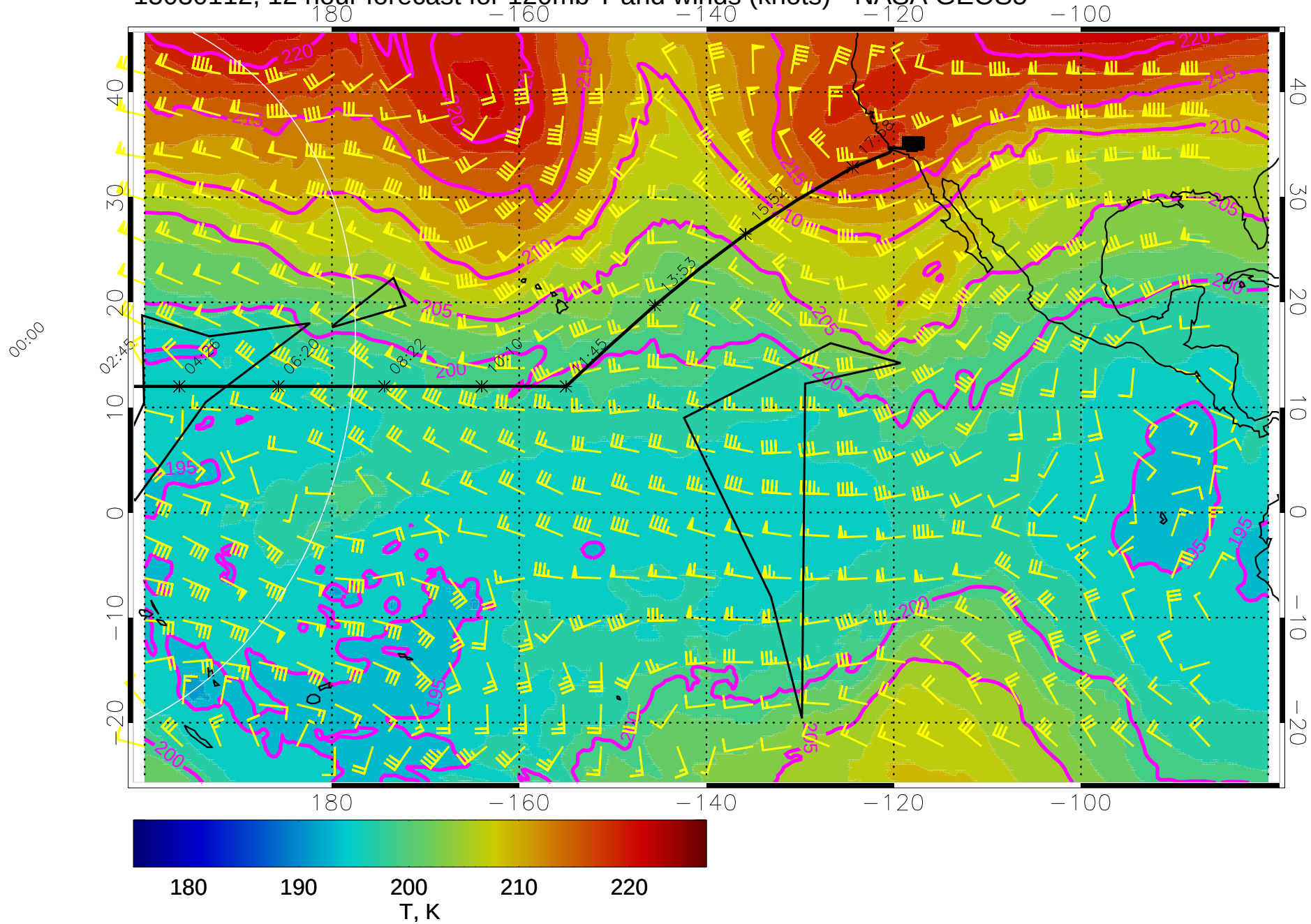
15030112, 12 hour forecast for 120mb T and winds (knots) - NASA GEOS5
