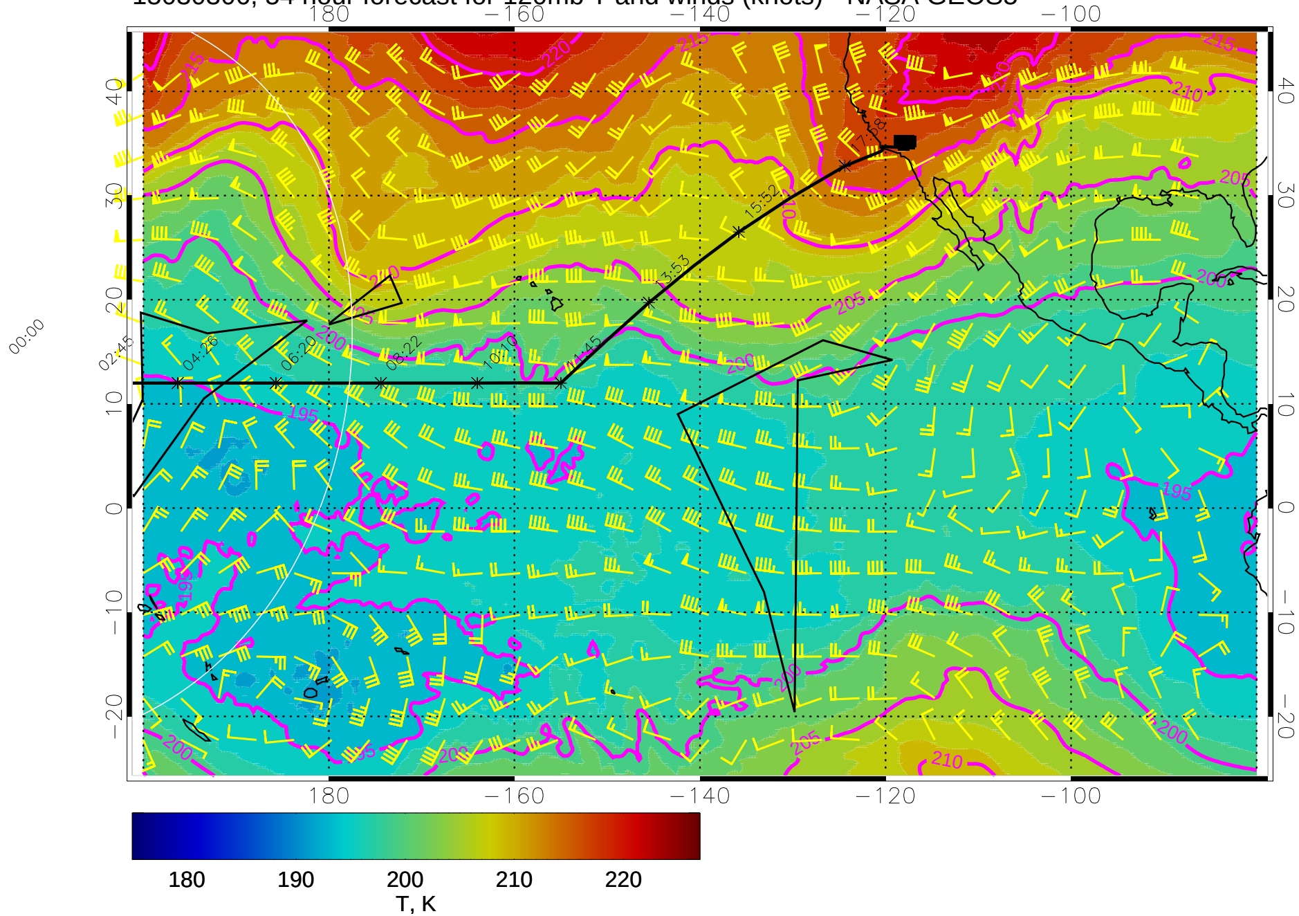
15030306, 54 hour forecast for 120mb T and winds (knots) - NASA GEOS5
