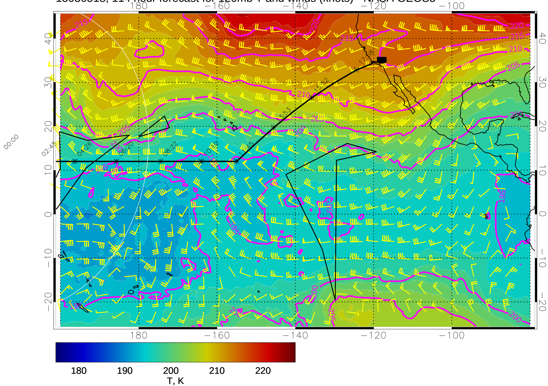
15030518, 114 hour forecast for 120mb T and winds (knots) - NASA GEOS5
