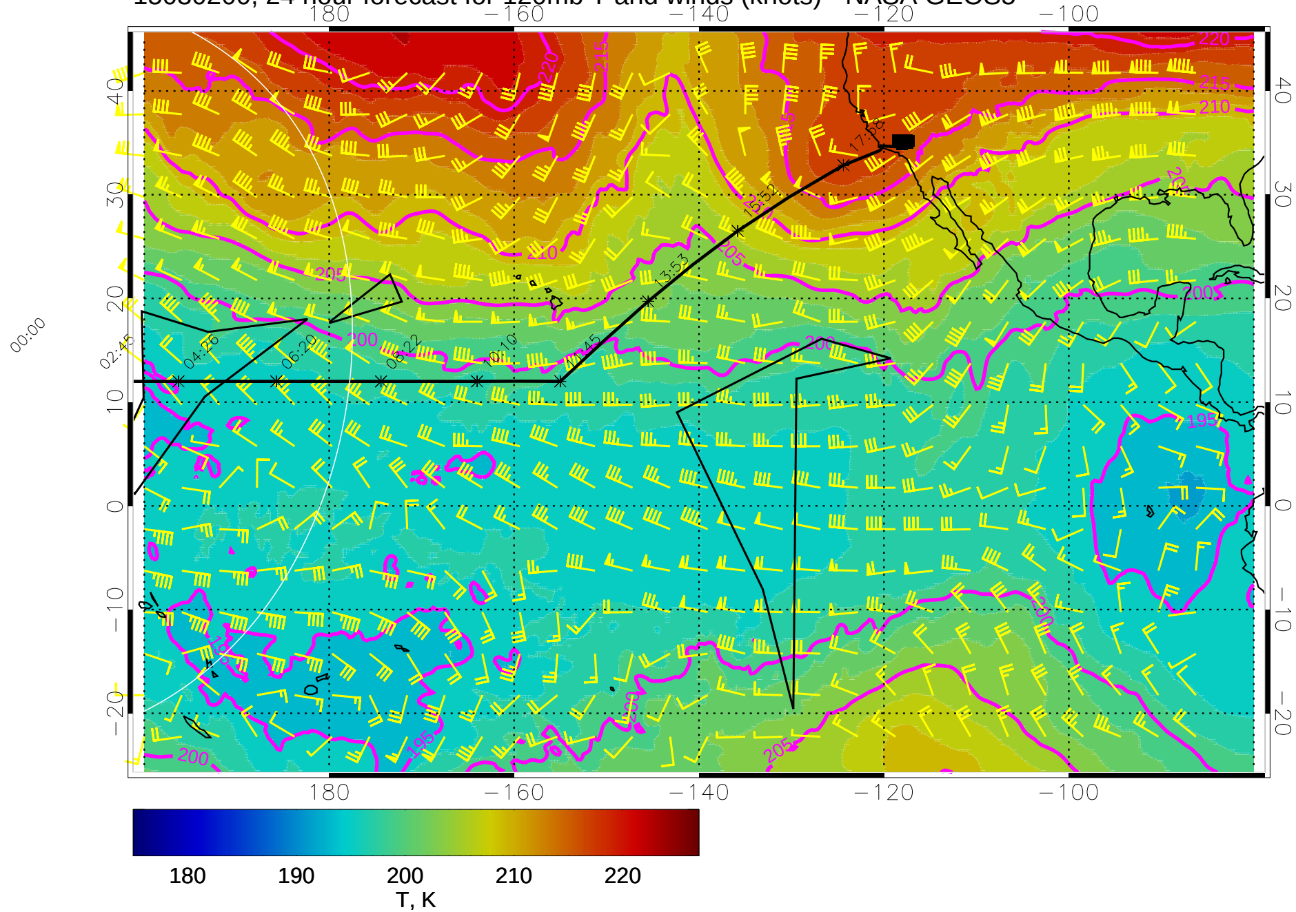
15030200, 24 hour forecast for 120mb T and winds (knots) - NASA GEOS5
