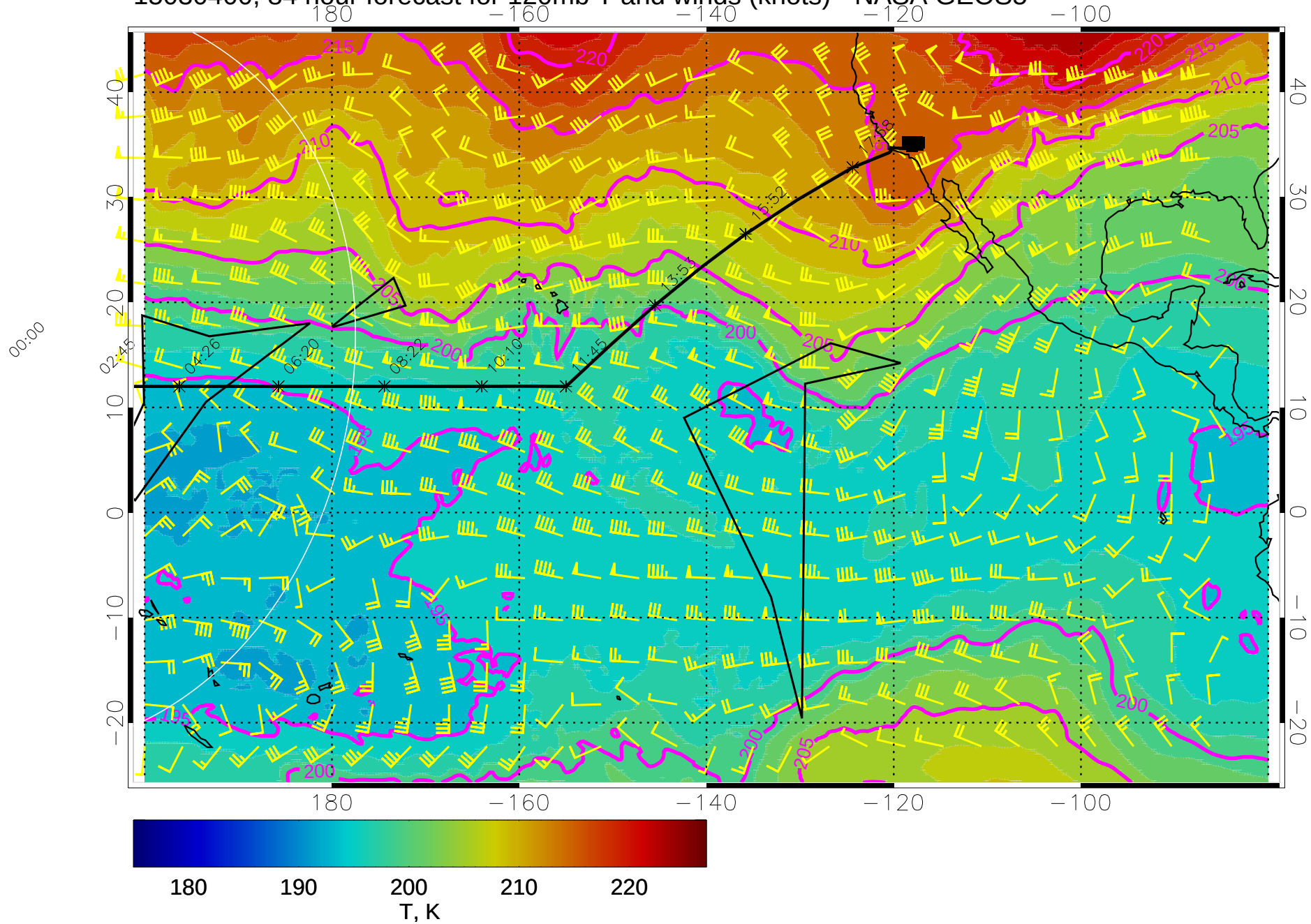
15030400, 84 hour forecast for 120mb T and winds (knots) - NASA GEOS5
