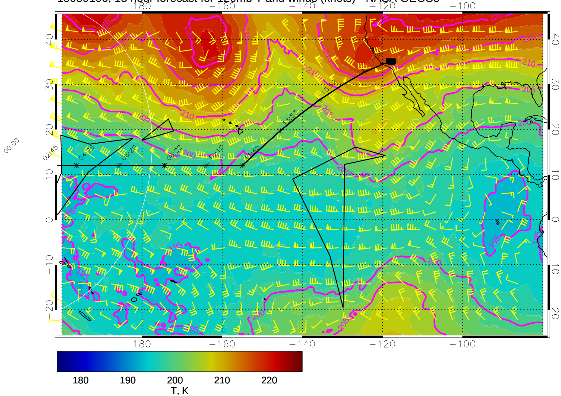
15030106, 18 hour forecast for 120mb T and winds (knots) - NASA GEOS5
