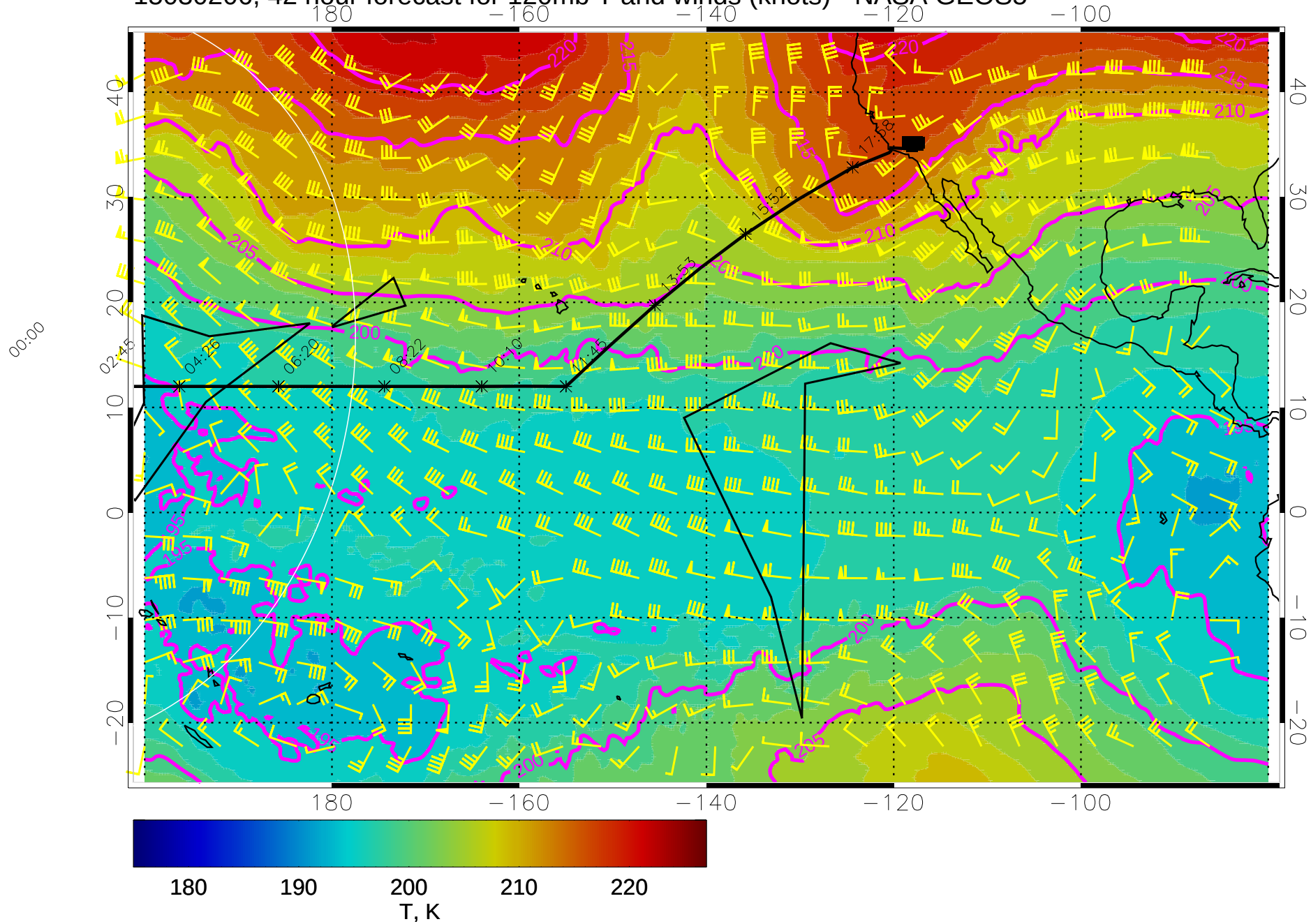
15030206, 42 hour forecast for 120mb T and winds (knots) - NASA GEOS5
