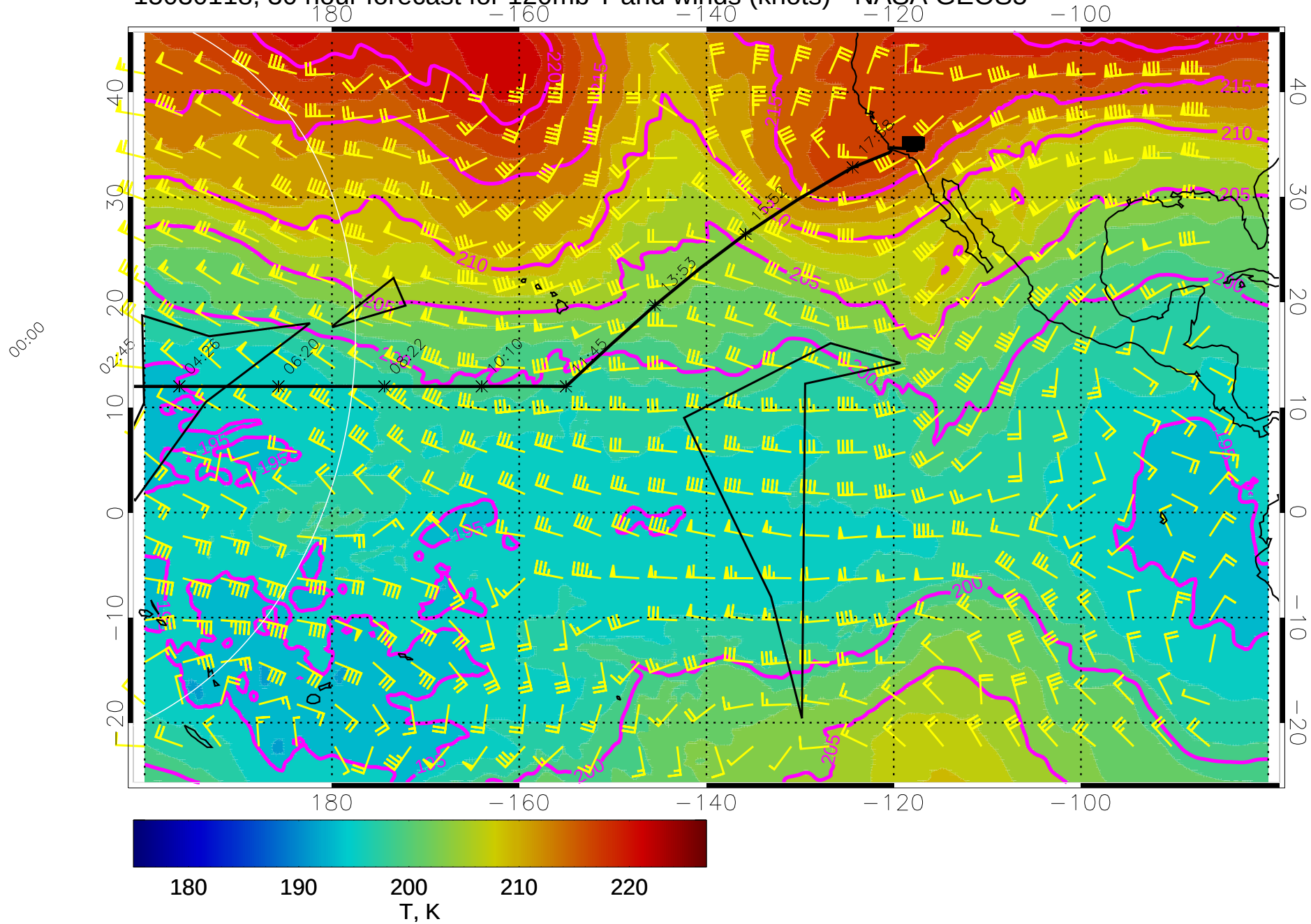
15030118, 30 hour forecast for 120mb T and winds (knots) - NASA GEOS5
