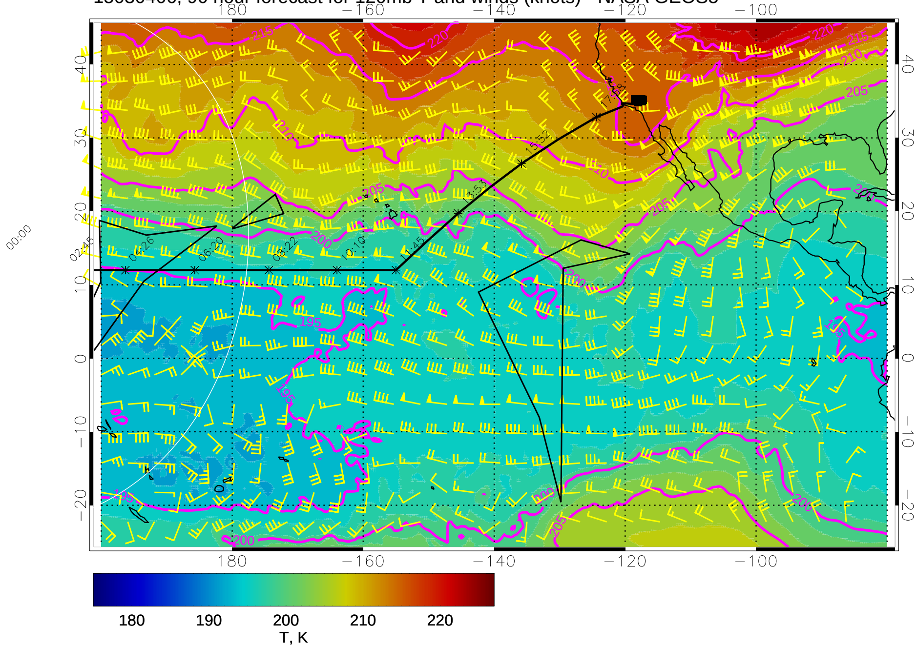
15030406, 90 hour forecast for 120mb T and winds (knots) - NASA GEOS5
