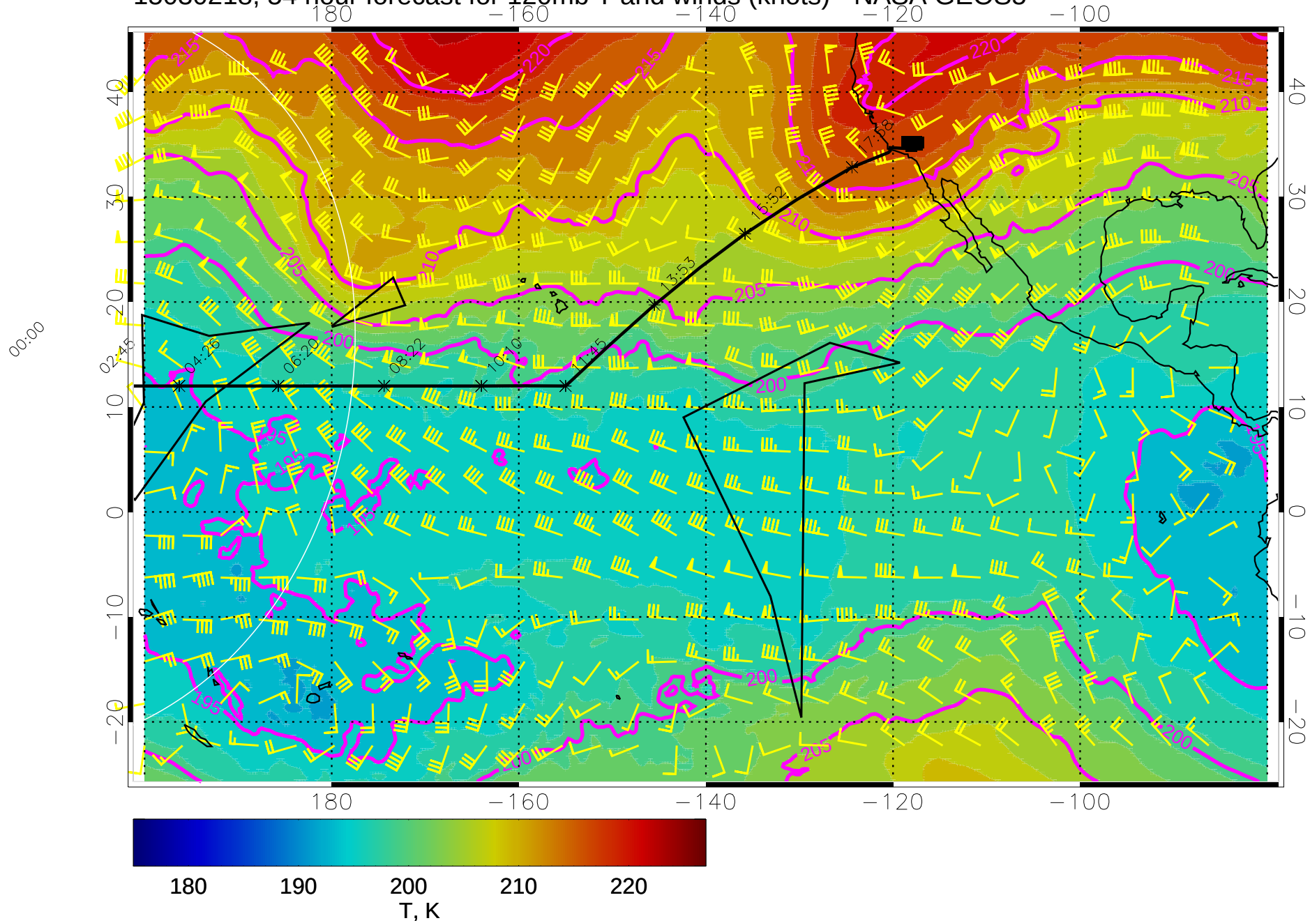
15030218, 54 hour forecast for 120mb T and winds (knots) - NASA GEOS5
