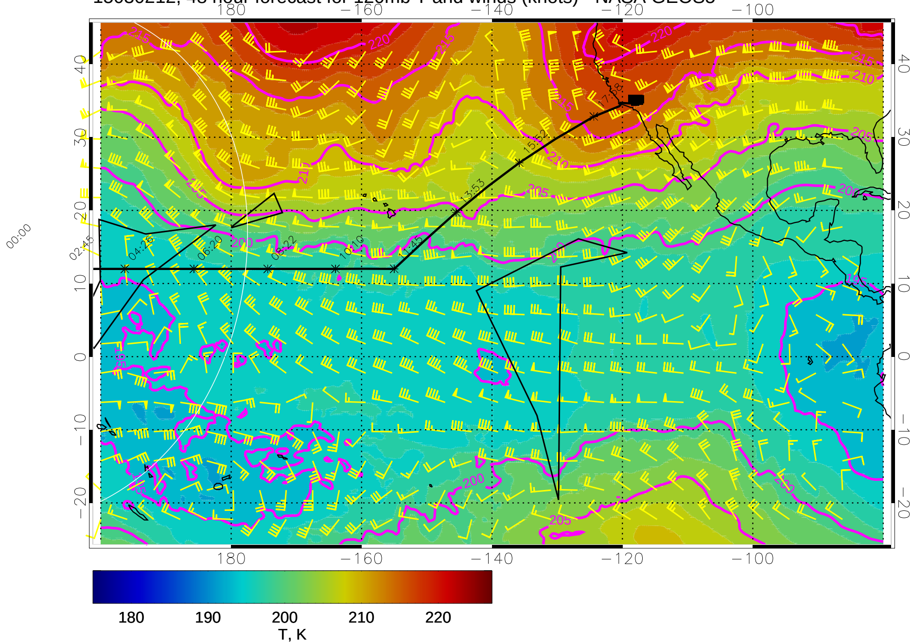
15030212, 48 hour forecast for 120mb T and winds (knots) - NASA GEOS5
