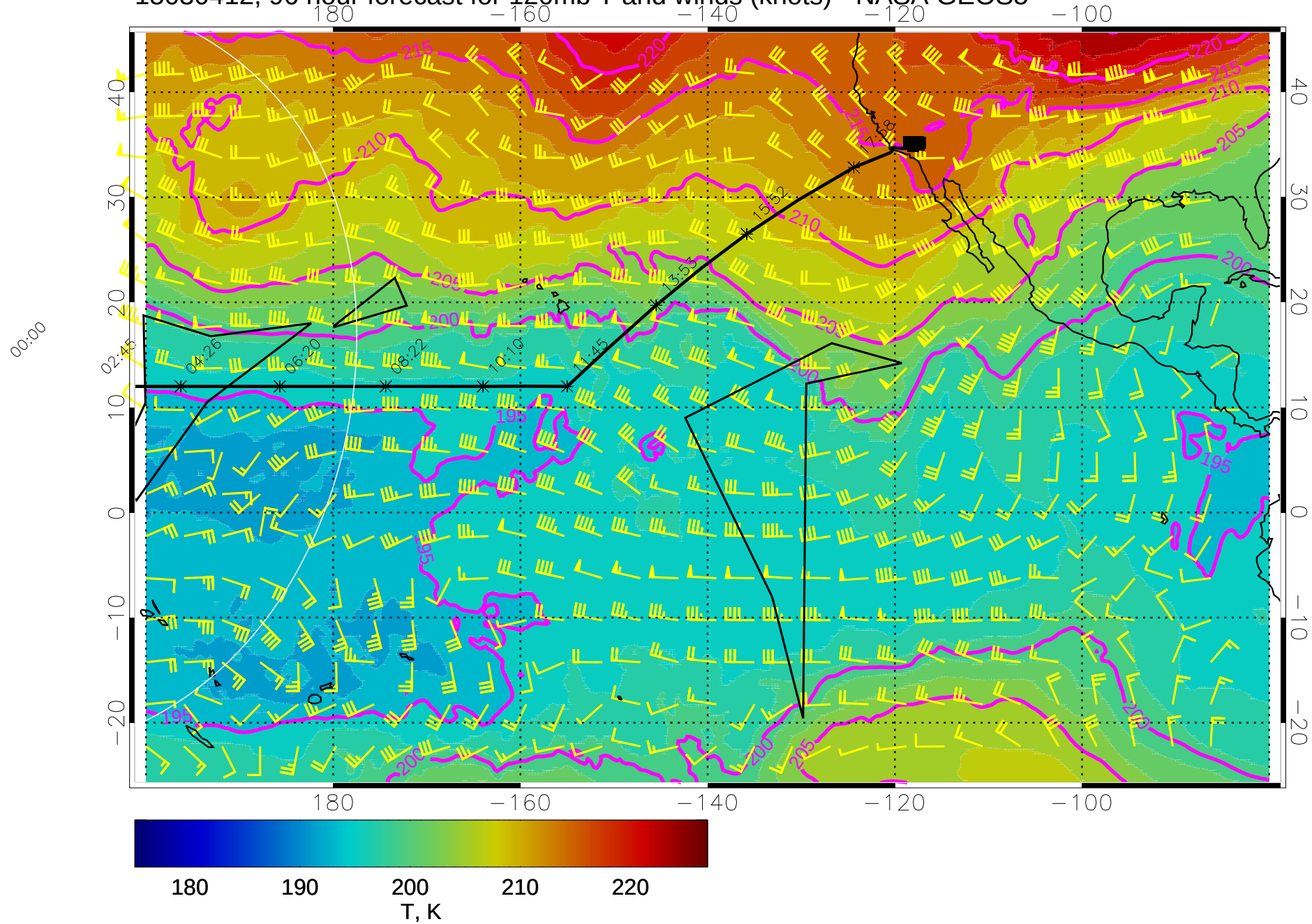
15030412, 96 hour forecast for 120mb T and winds (knots) - NASA GEOS5
