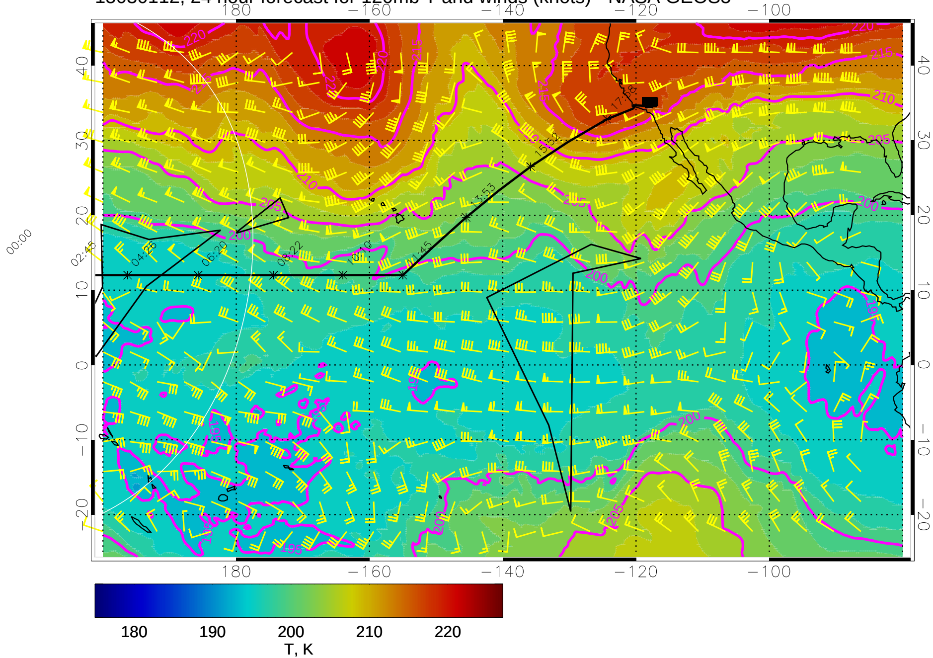
15030112, 24 hour forecast for 120mb T and winds (knots) - NASA GEOS5
