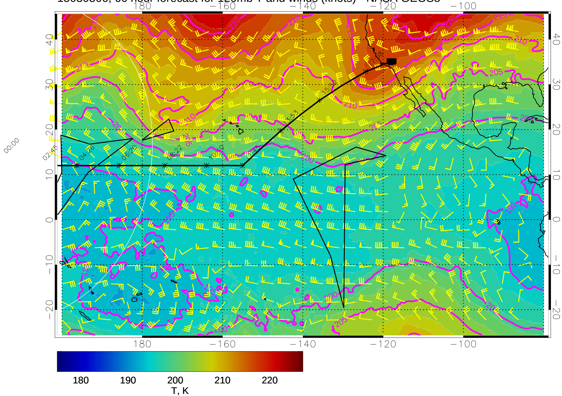
15030306, 66 hour forecast for 120mb T and winds (knots) - NASA GEOS5
