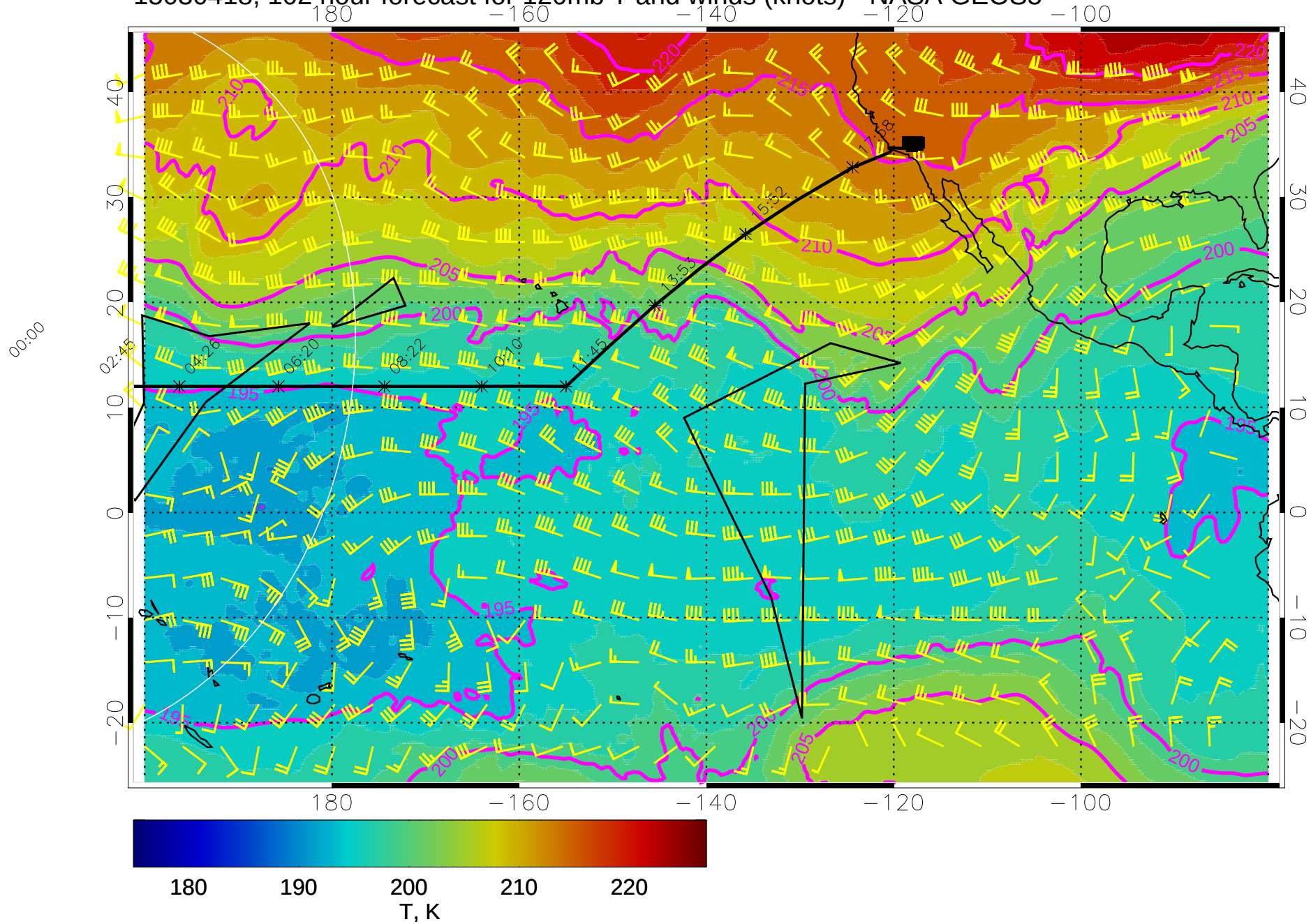
15030418, 102 hour forecast for 120mb T and winds (knots) - NASA GEOS5
