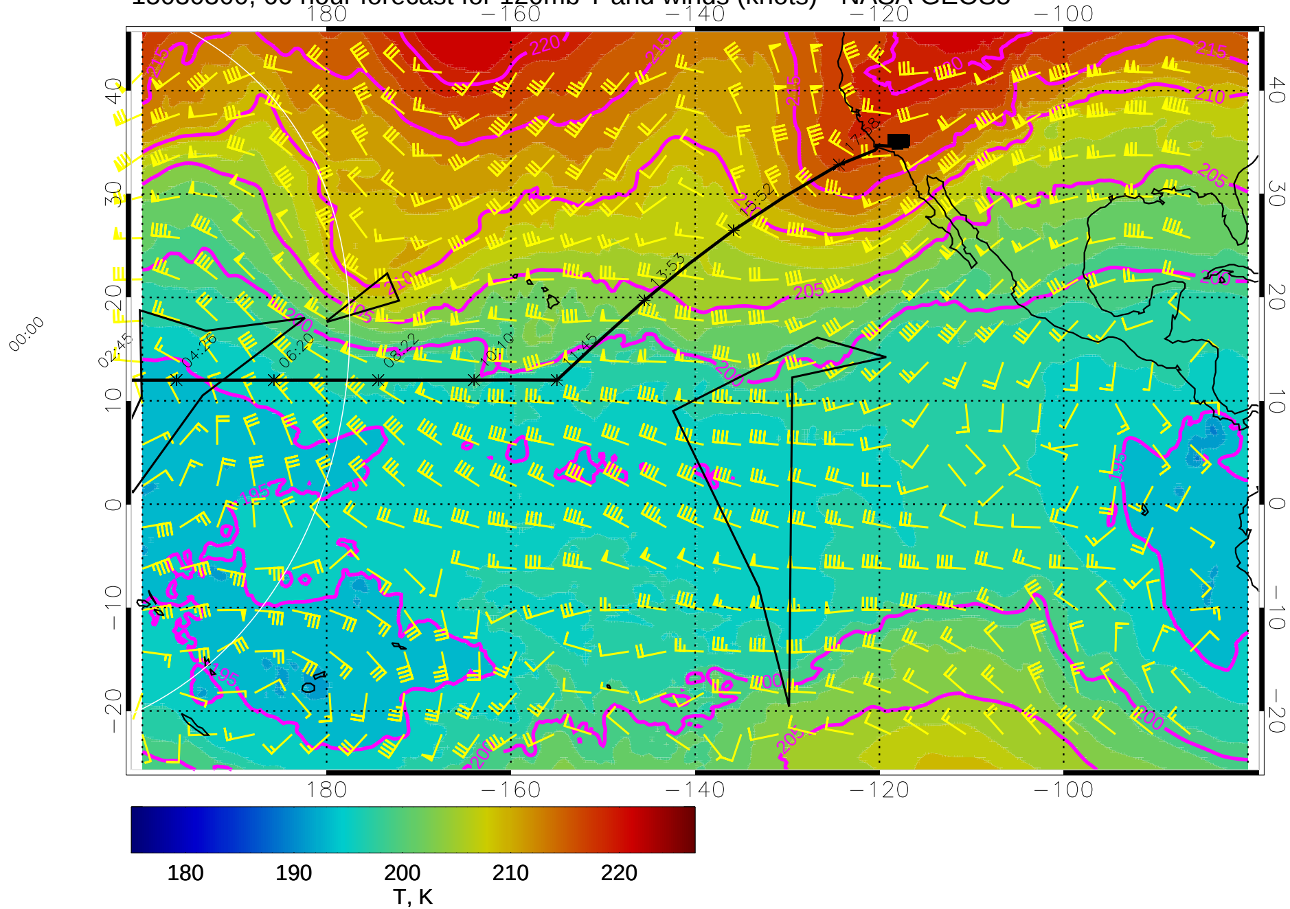
15030300, 60 hour forecast for 120mb T and winds (knots) - NASA GEOS5
