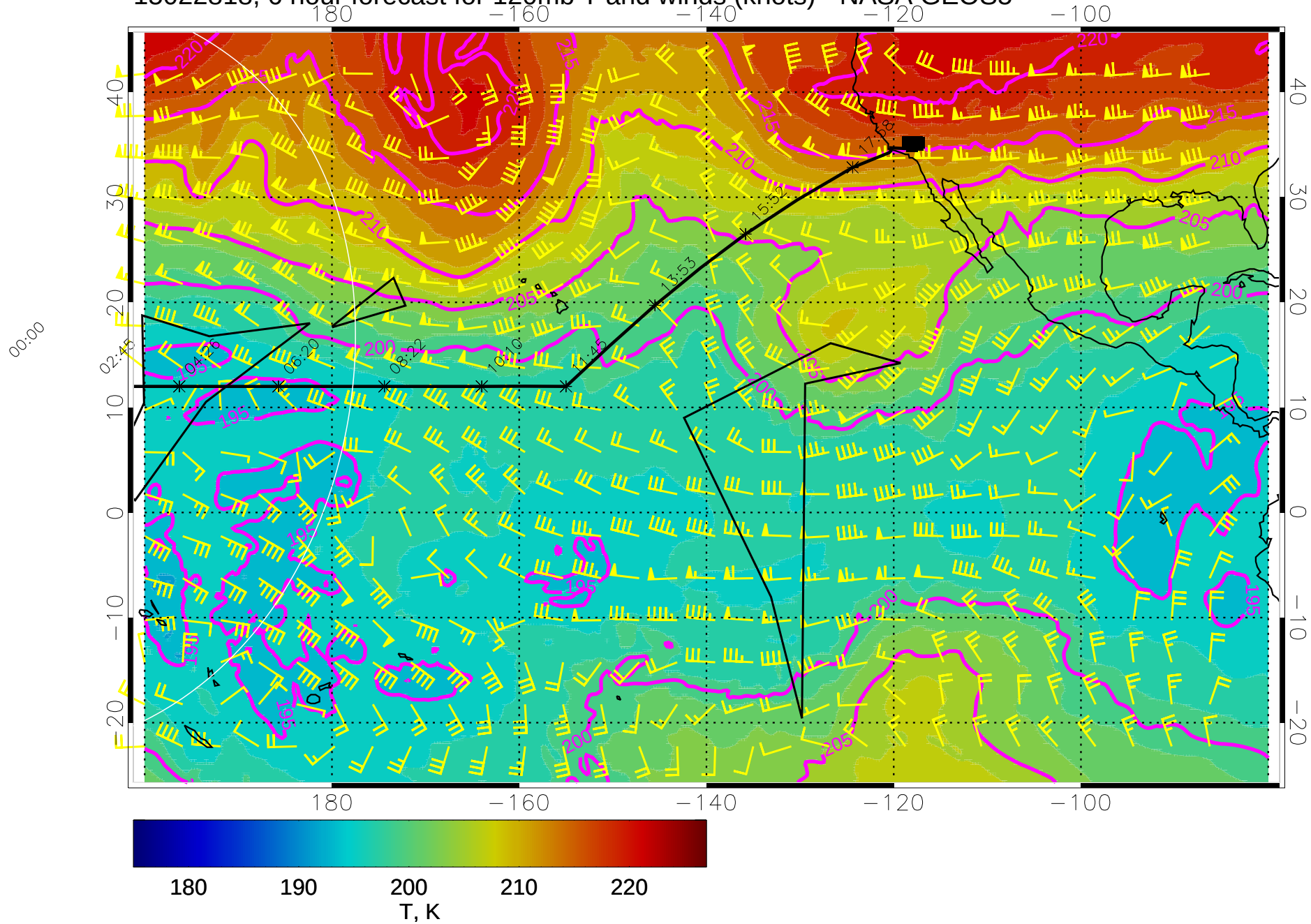
15022818, 6 hour forecast for 120mb T and winds (knots) - NASA GEOS5
