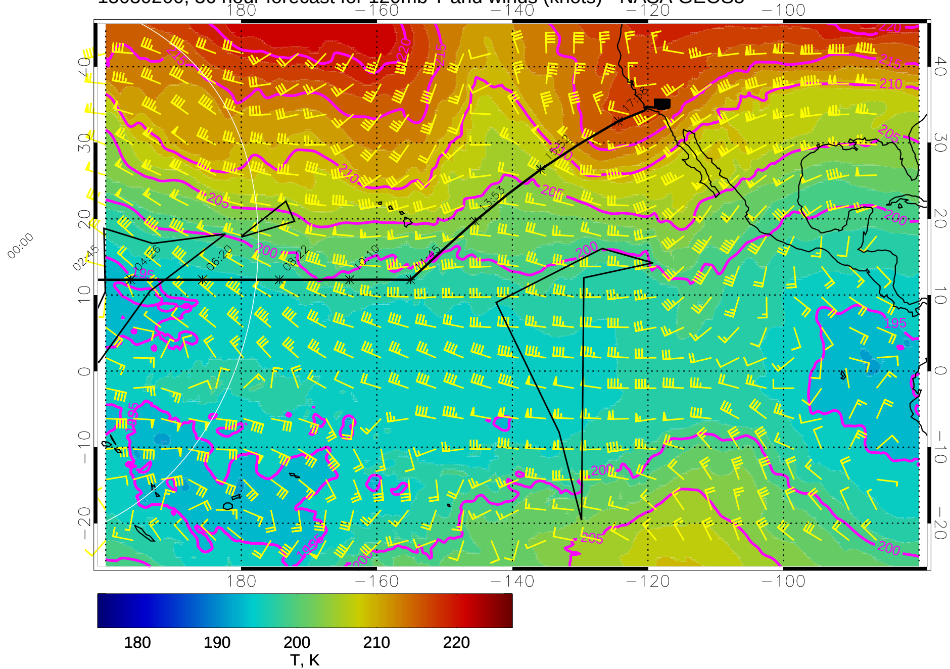
15030200, 36 hour forecast for 120mb T and winds (knots) - NASA GEOS5
