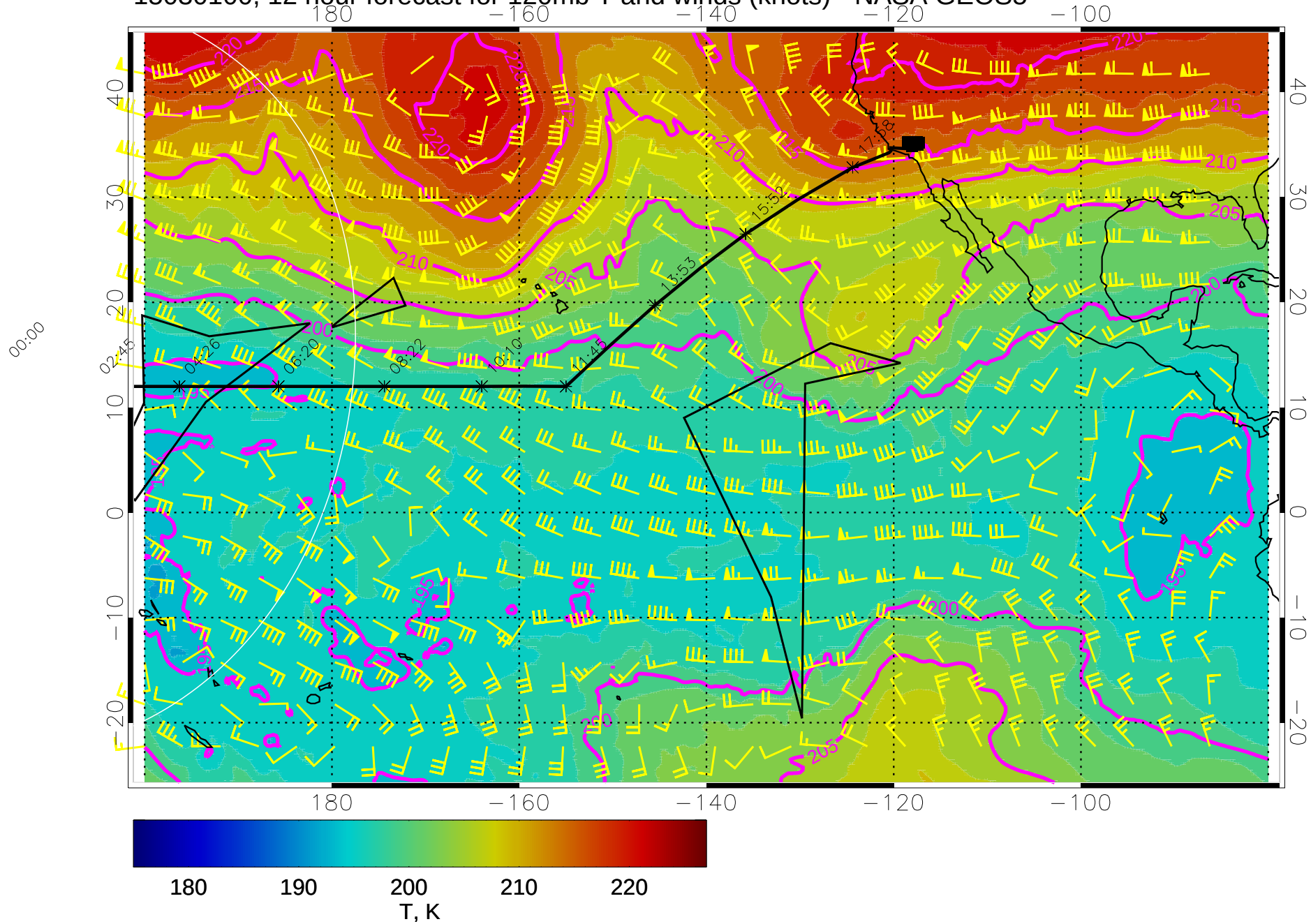
15030100, 12 hour forecast for 120mb T and winds (knots) - NASA GEOS5
