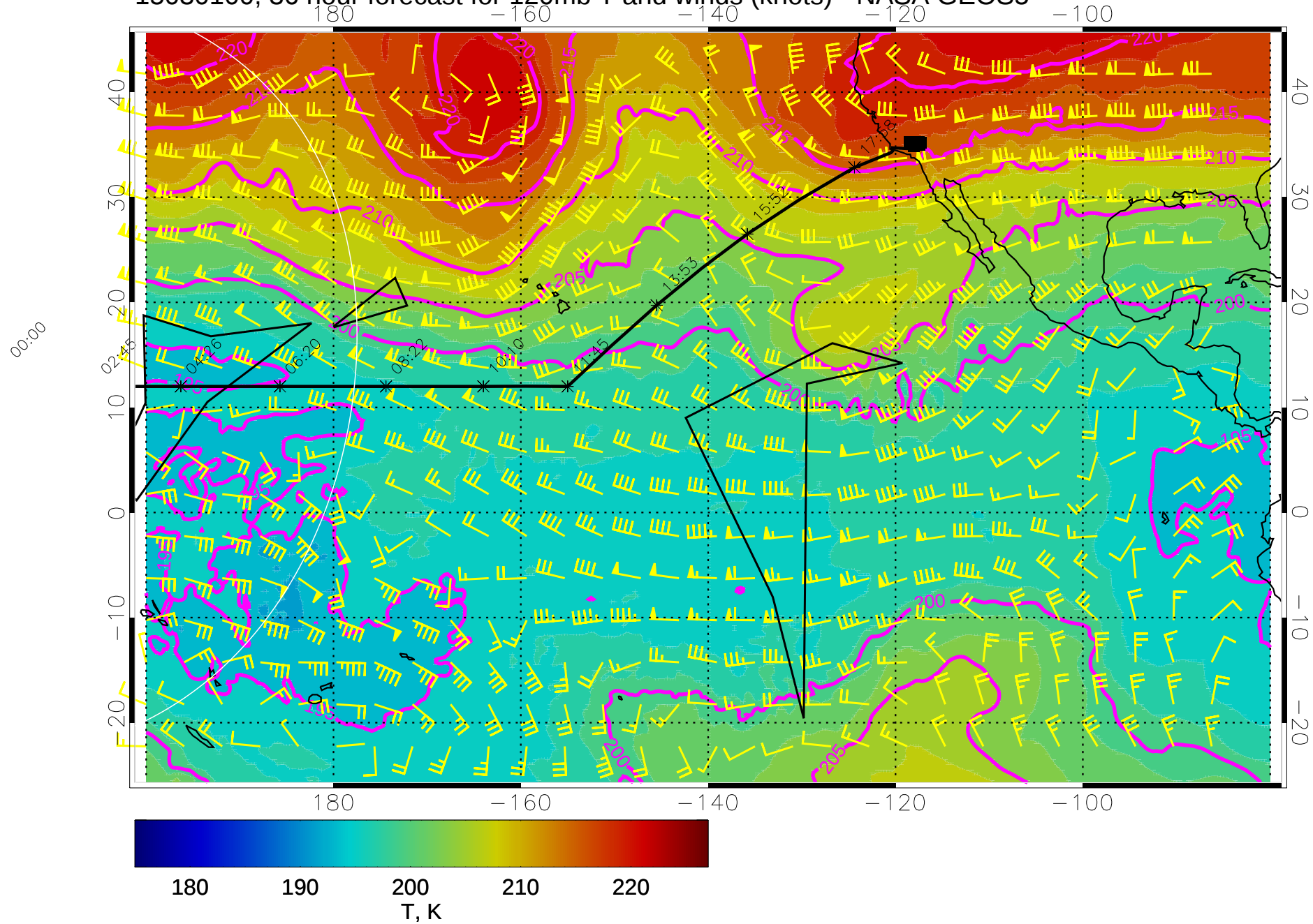
15030100, 36 hour forecast for 120mb T and winds (knots) - NASA GEOS5
