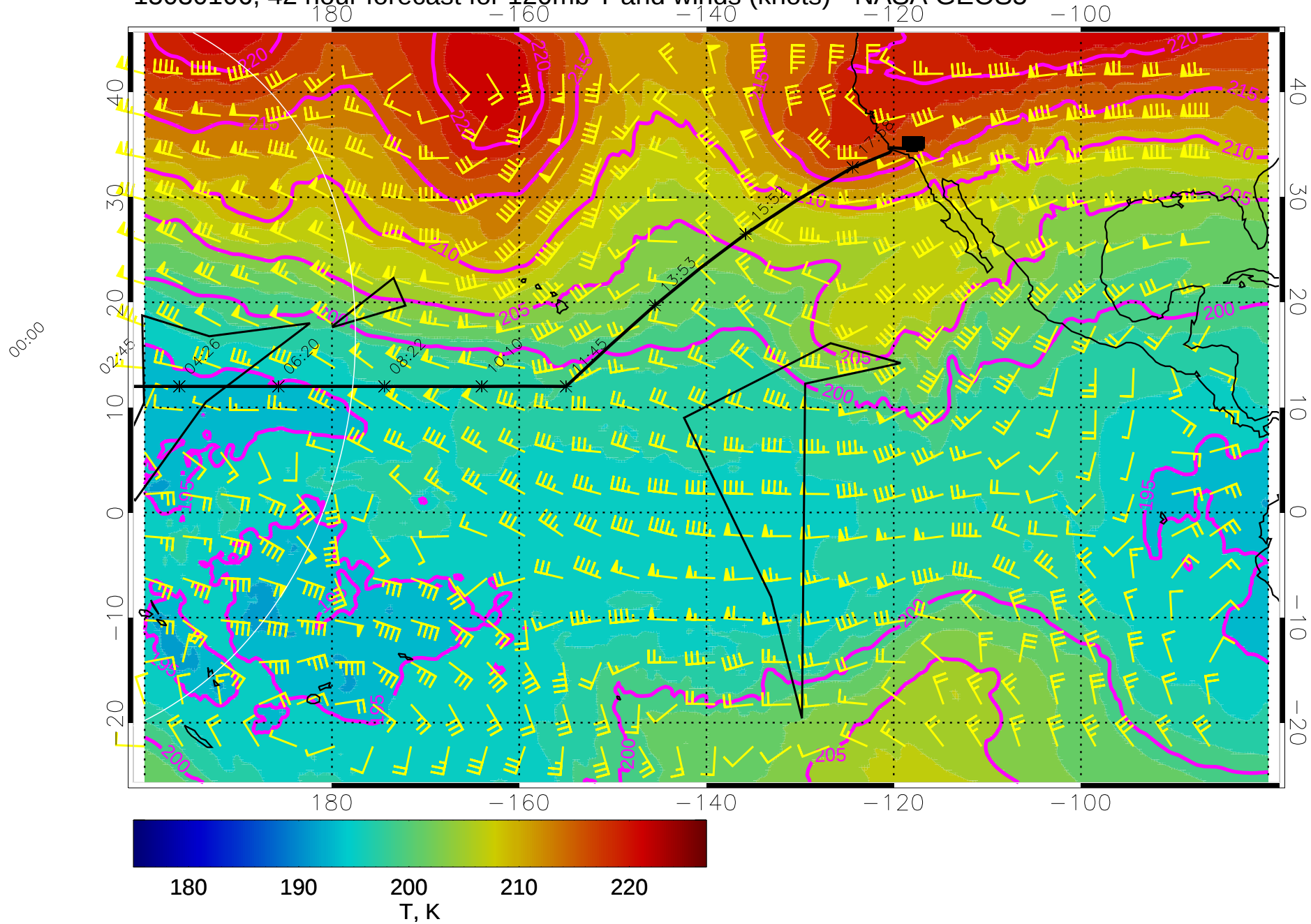
15030106, 42 hour forecast for 120mb T and winds (knots) - NASA GEOS5
