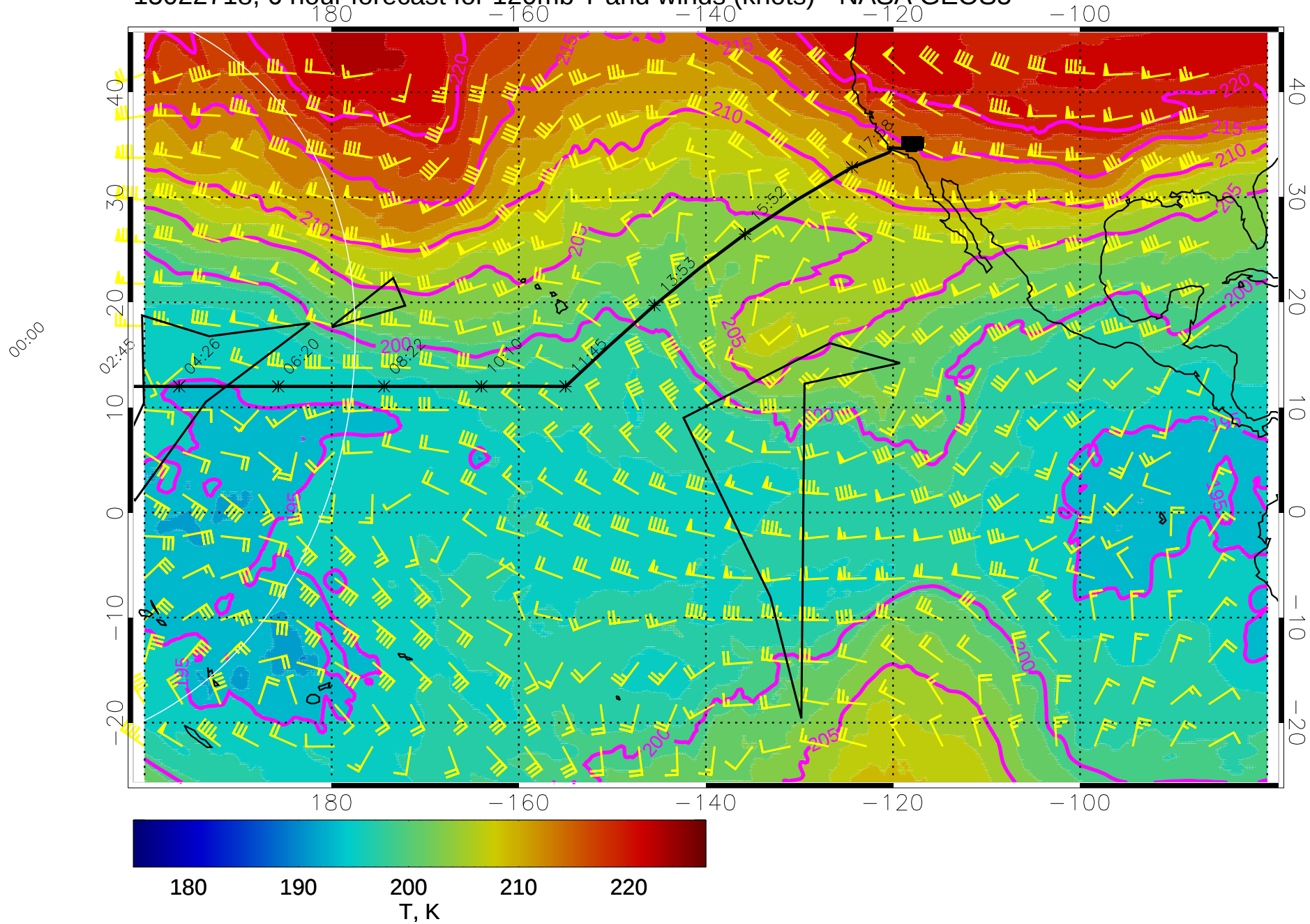
15022718, 6 hour forecast for 120mb T and winds (knots) - NASA GEOS5
