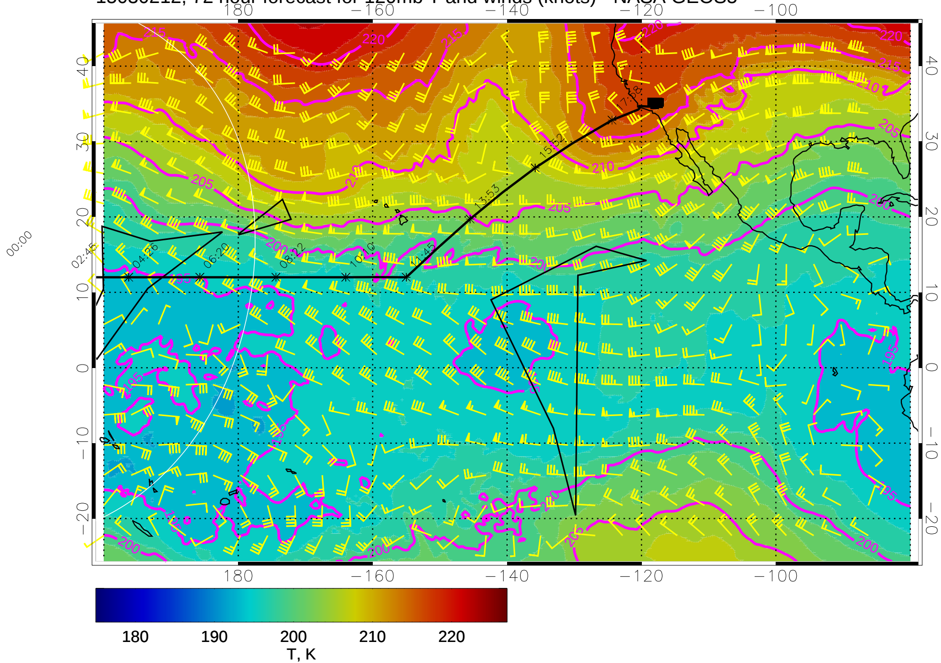
15030212, 72 hour forecast for 120mb T and winds (knots) - NASA GEOS5
