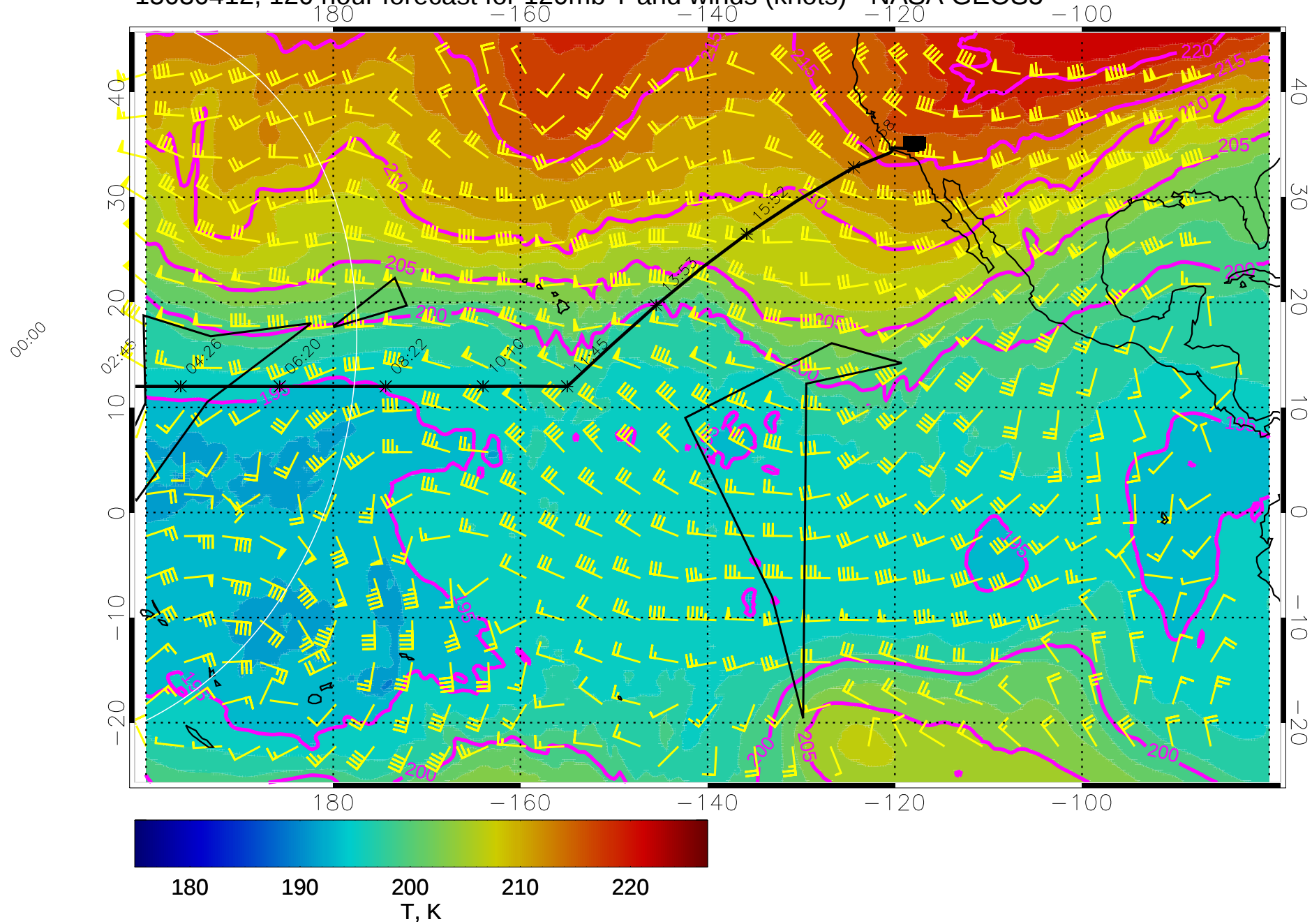
15030412, 120 hour forecast for 120mb T and winds (knots) - NASA GEOS5
