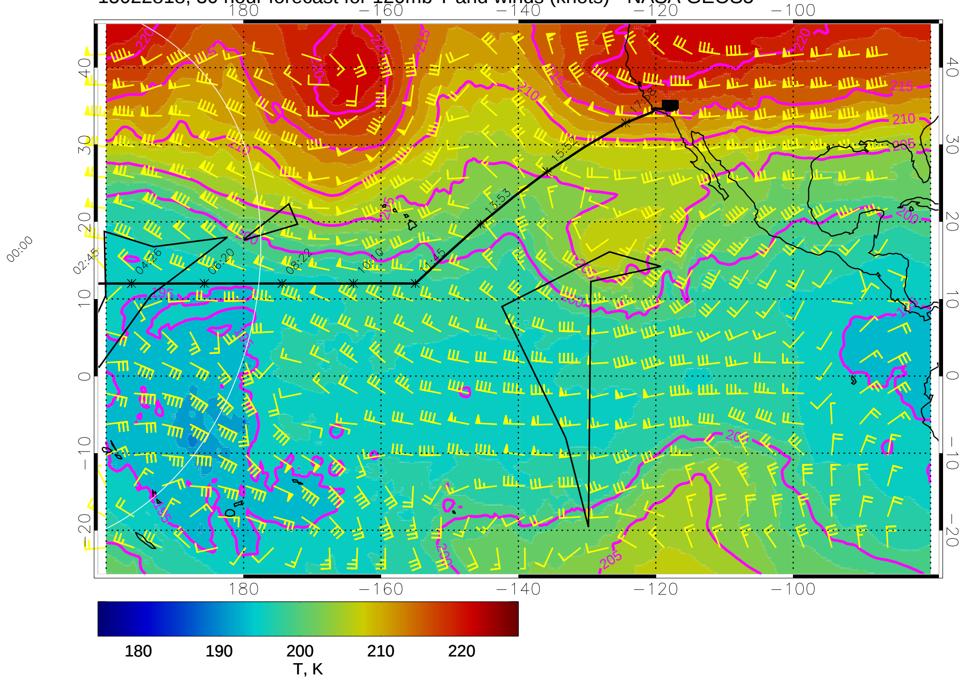
15022818, 30 hour forecast for 120mb T and winds (knots) - NASA GEOS5
