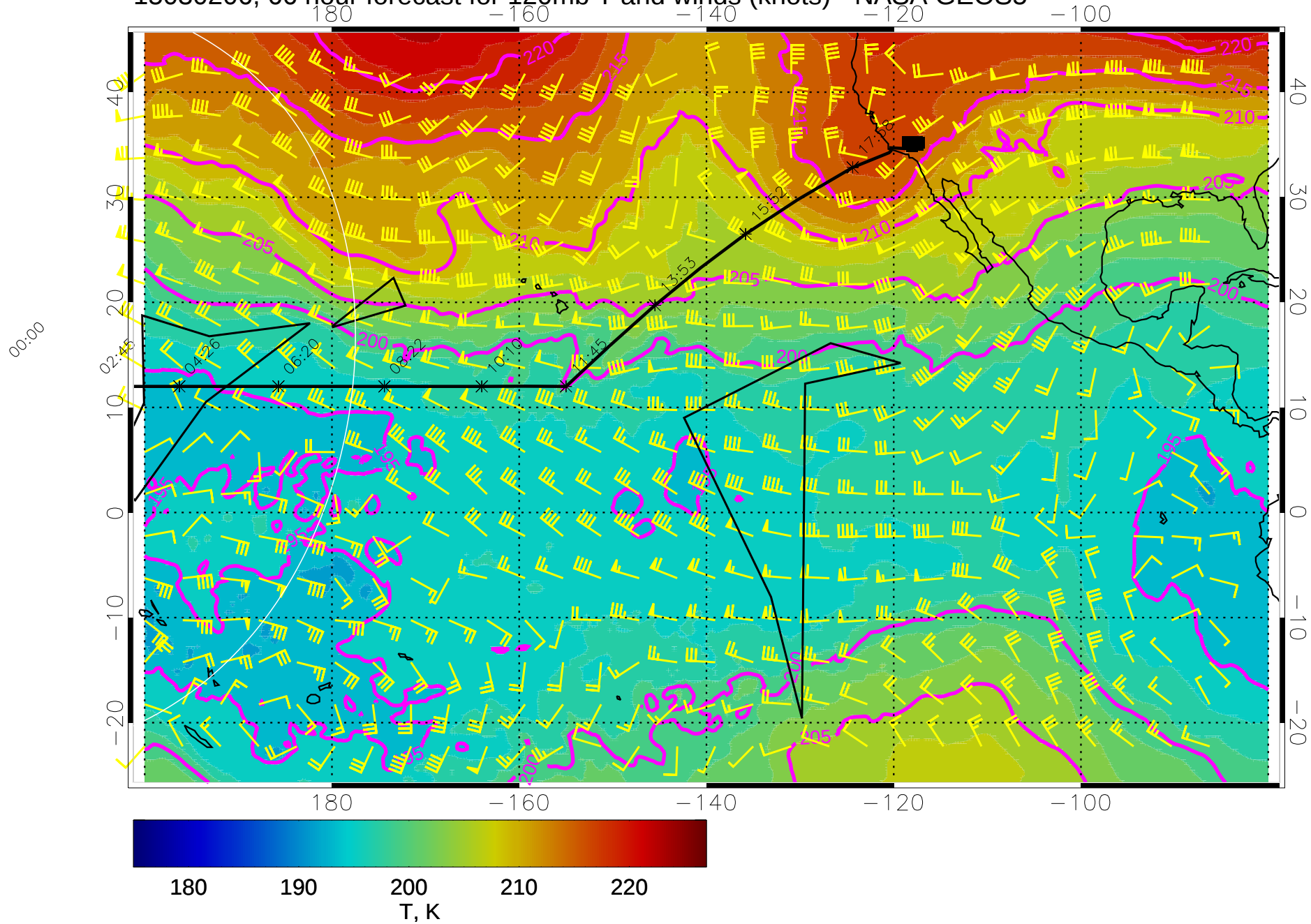
15030206, 66 hour forecast for 120mb T and winds (knots) - NASA GEOS5
