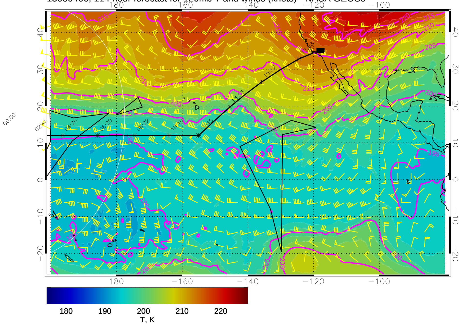
15030406, 114 hour forecast for 120mb T and winds (knots) - NASA GEOS5
