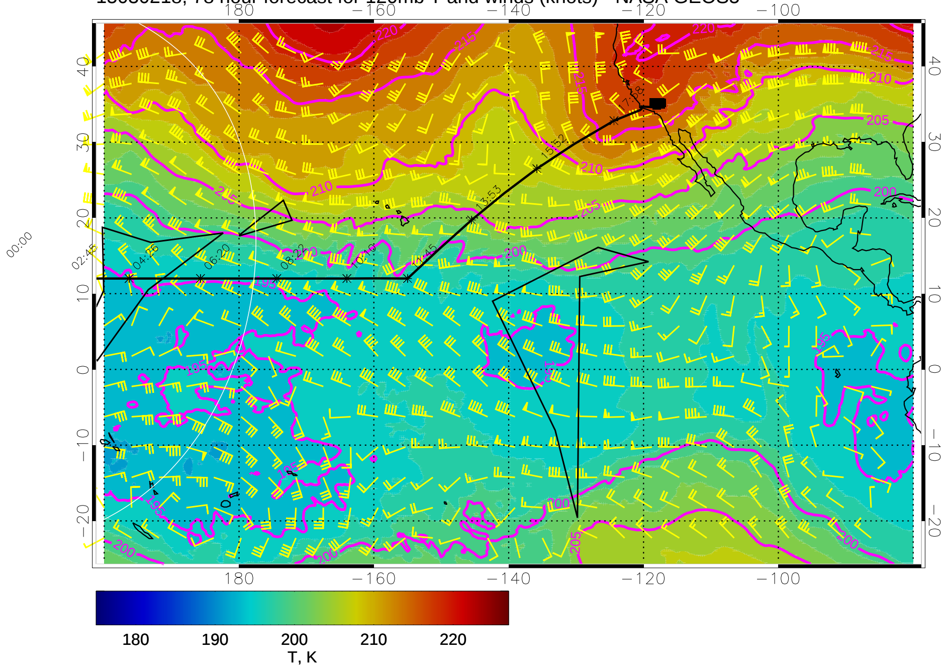
15030218, 78 hour forecast for 120mb T and winds (knots) - NASA GEOS5
