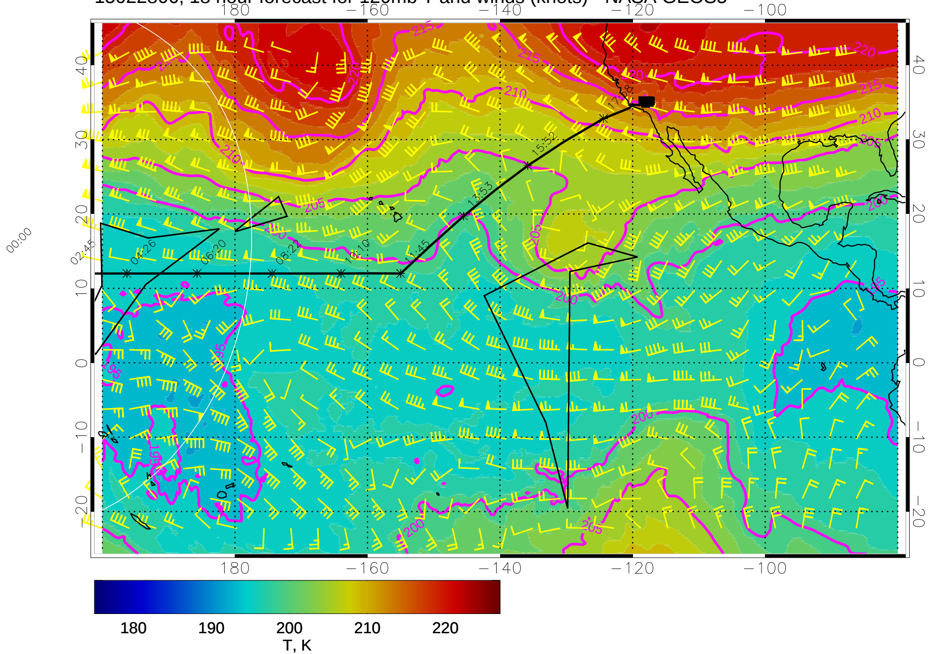
15022806, 18 hour forecast for 120mb T and winds (knots) - NASA GEOS5
