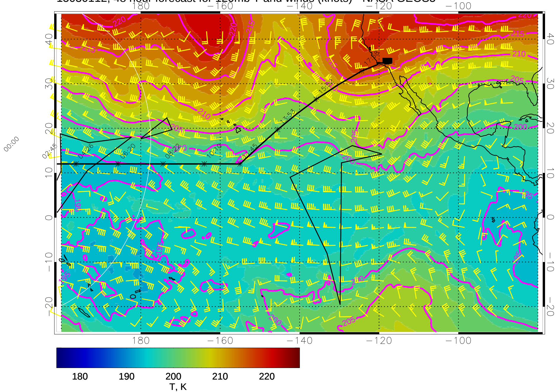
15030112, 48 hour forecast for 120mb T and winds (knots) - NASA GEOS5
