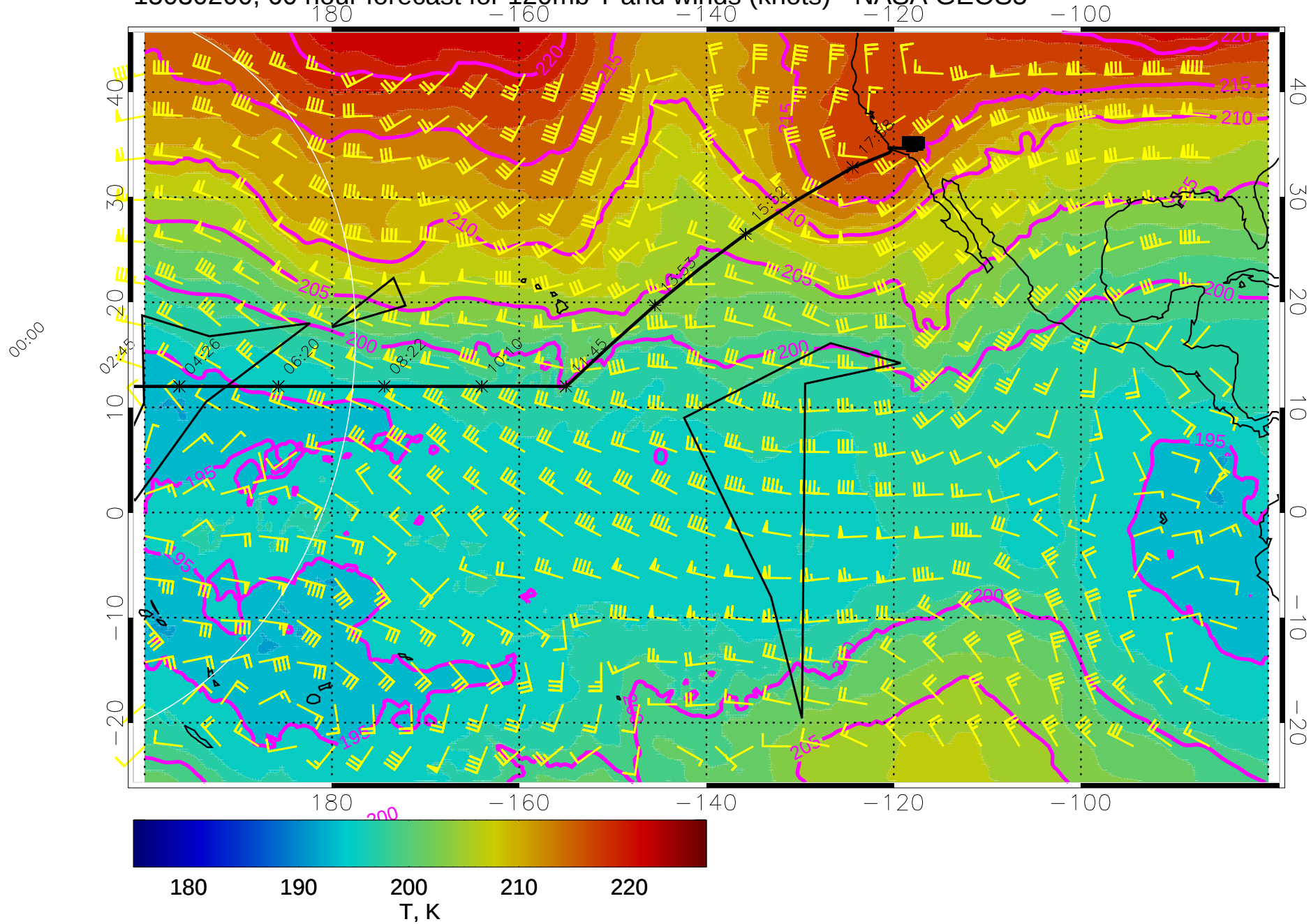
15030200, 60 hour forecast for 120mb T and winds (knots) - NASA GEOS5
