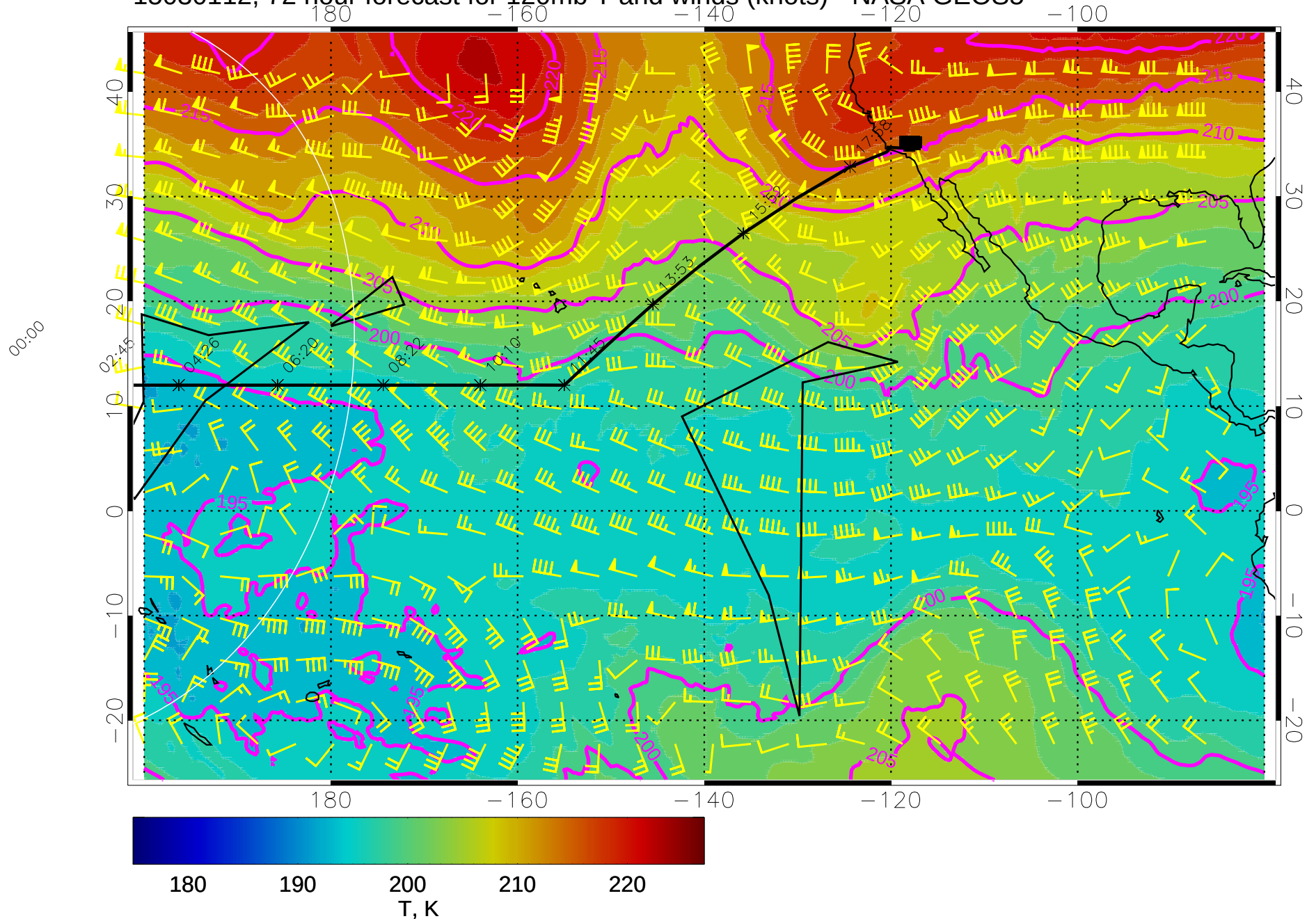
15030112, 72 hour forecast for 120mb T and winds (knots) - NASA GEOS5
