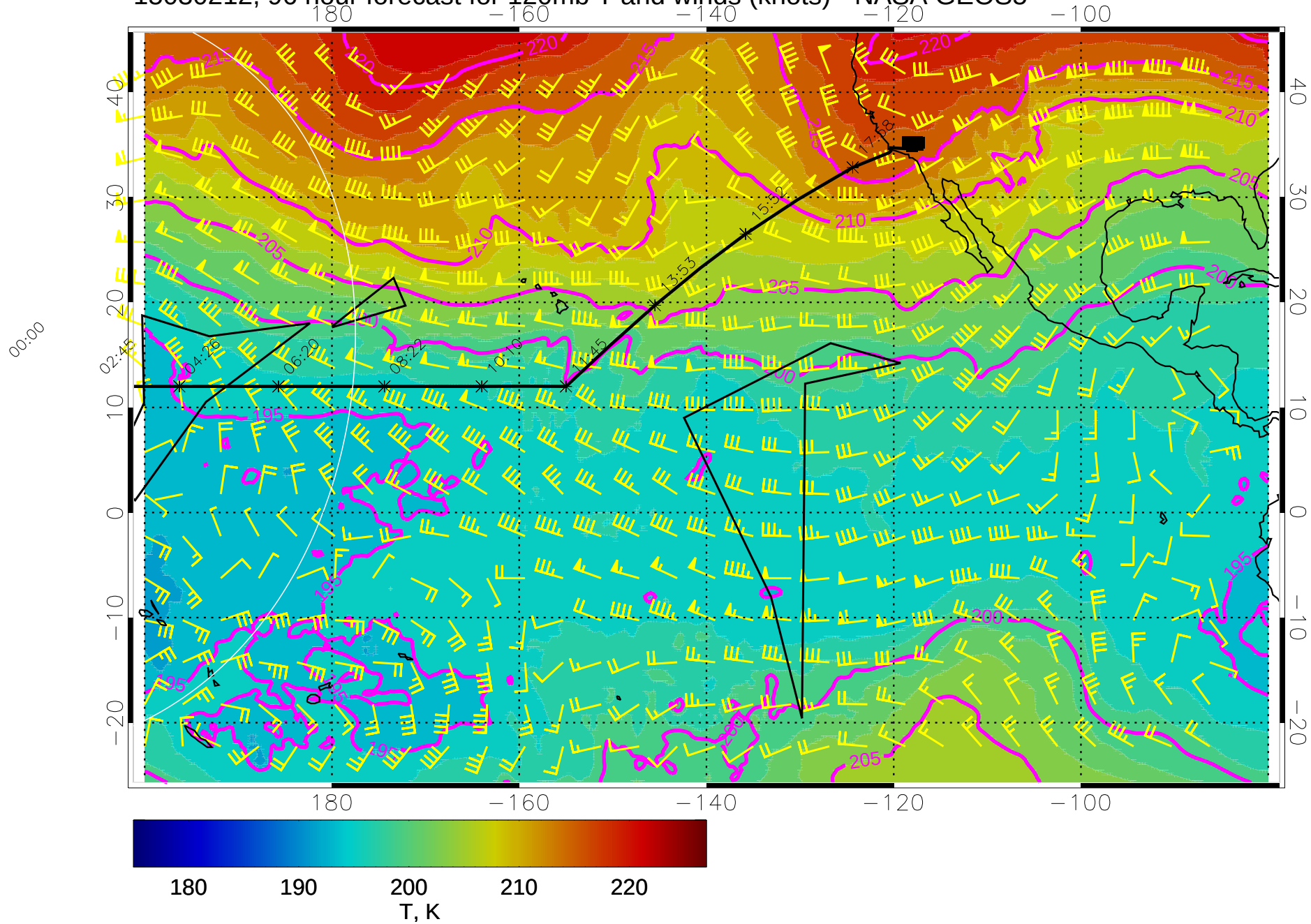
15030212, 96 hour forecast for 120mb T and winds (knots) - NASA GEOS5
