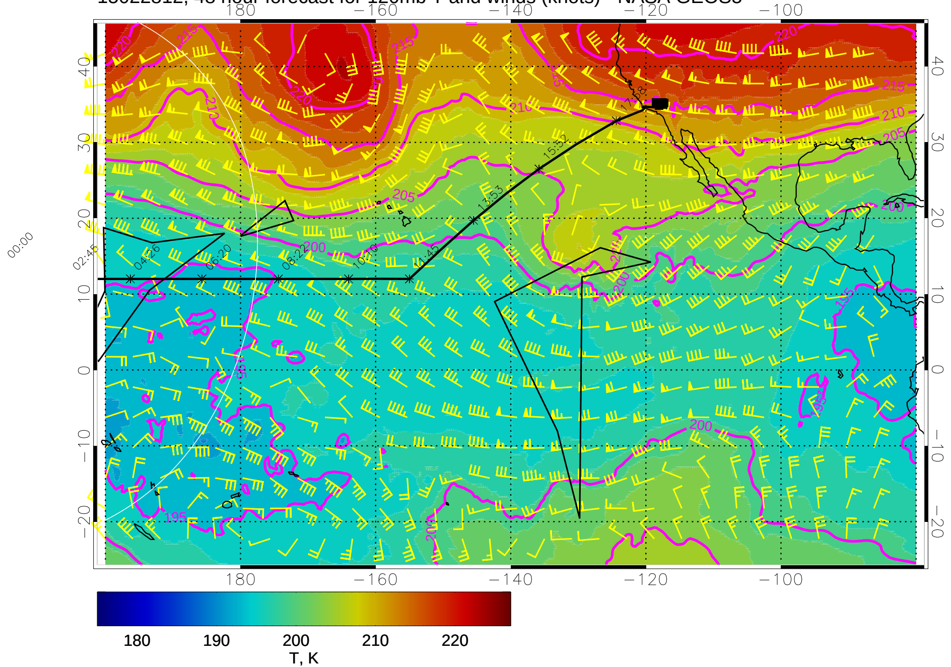
15022812, 48 hour forecast for 120mb T and winds (knots) - NASA GEOS5
