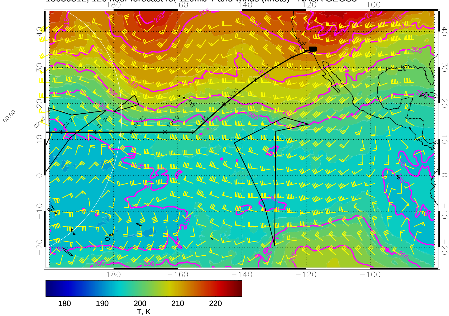
15030312, 120 hour forecast for 120mb T and winds (knots) - NASA GEOS5
