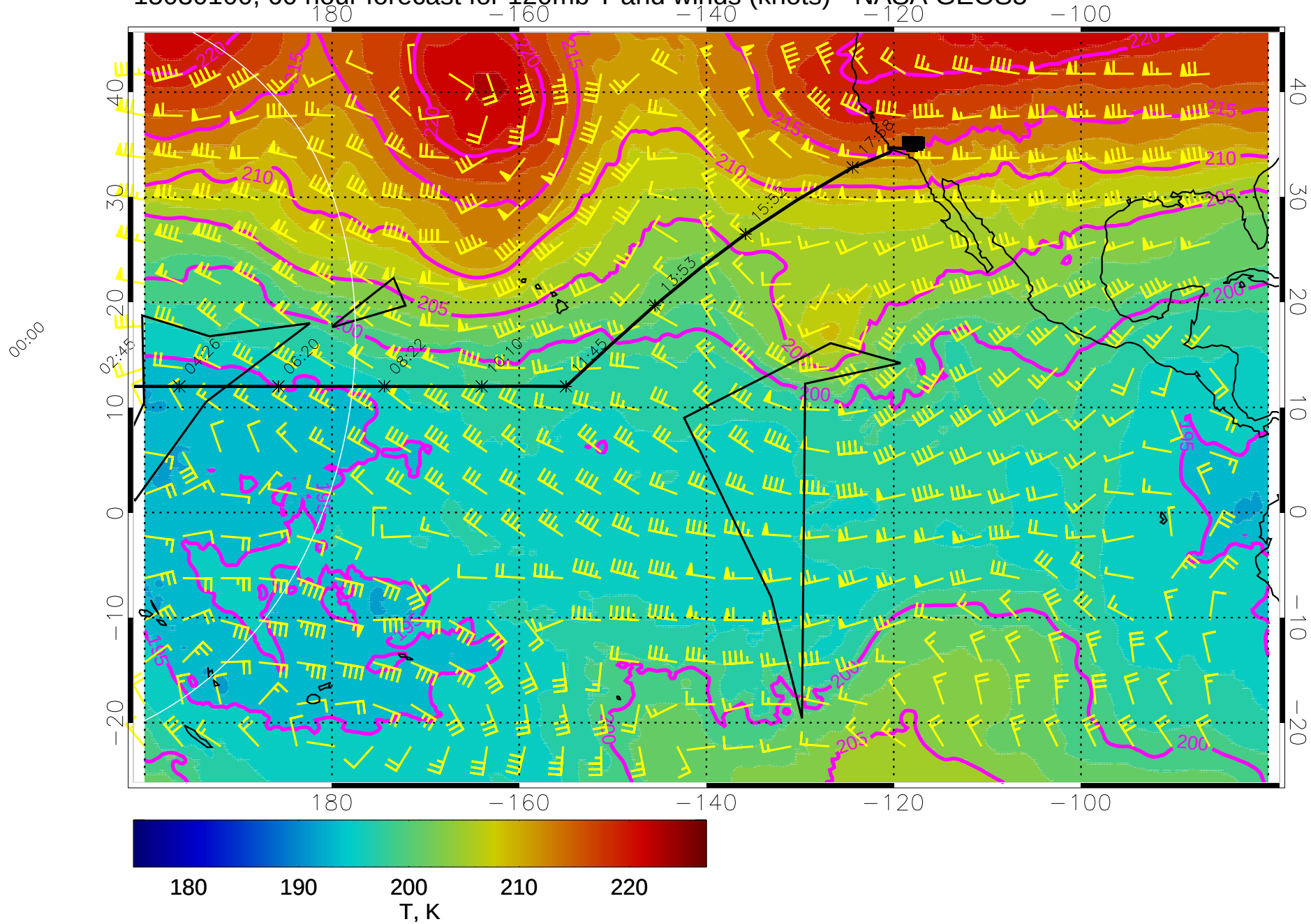
15030100, 60 hour forecast for 120mb T and winds (knots) - NASA GEOS5
