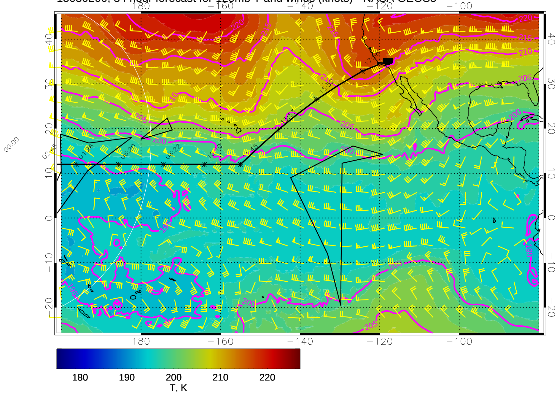
15030200, 84 hour forecast for 120mb T and winds (knots) - NASA GEOS5
