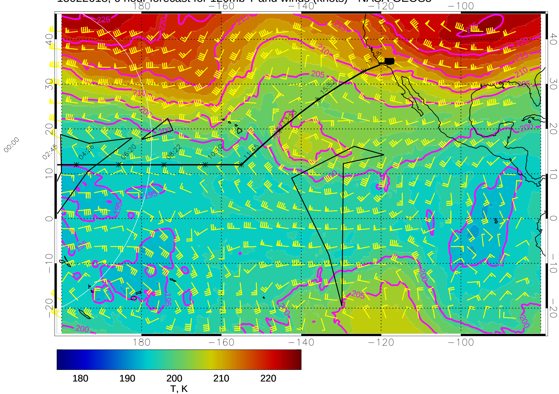
15022618, 6 hour forecast for 120mb T and winds (knots) - NASA GEOS5
