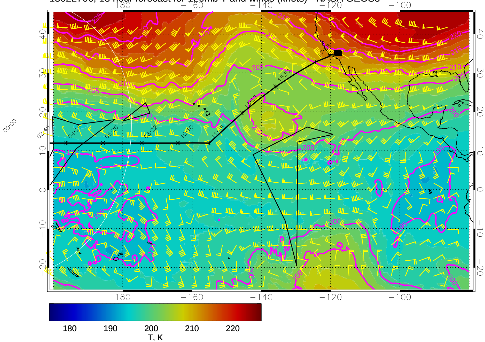
15022706, 18 hour forecast for 120mb T and winds (knots) - NASA GEOS5
