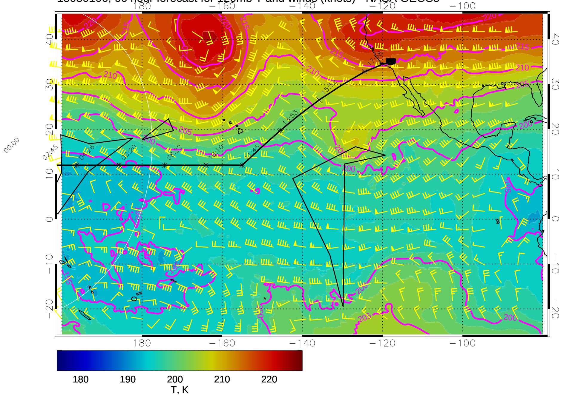
15030106, 66 hour forecast for 120mb T and winds (knots) - NASA GEOS5
