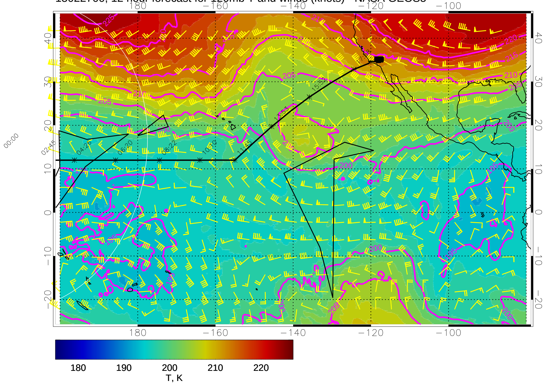
15022700, 12 hour forecast for 120mb T and winds (knots) - NASA GEOS5
