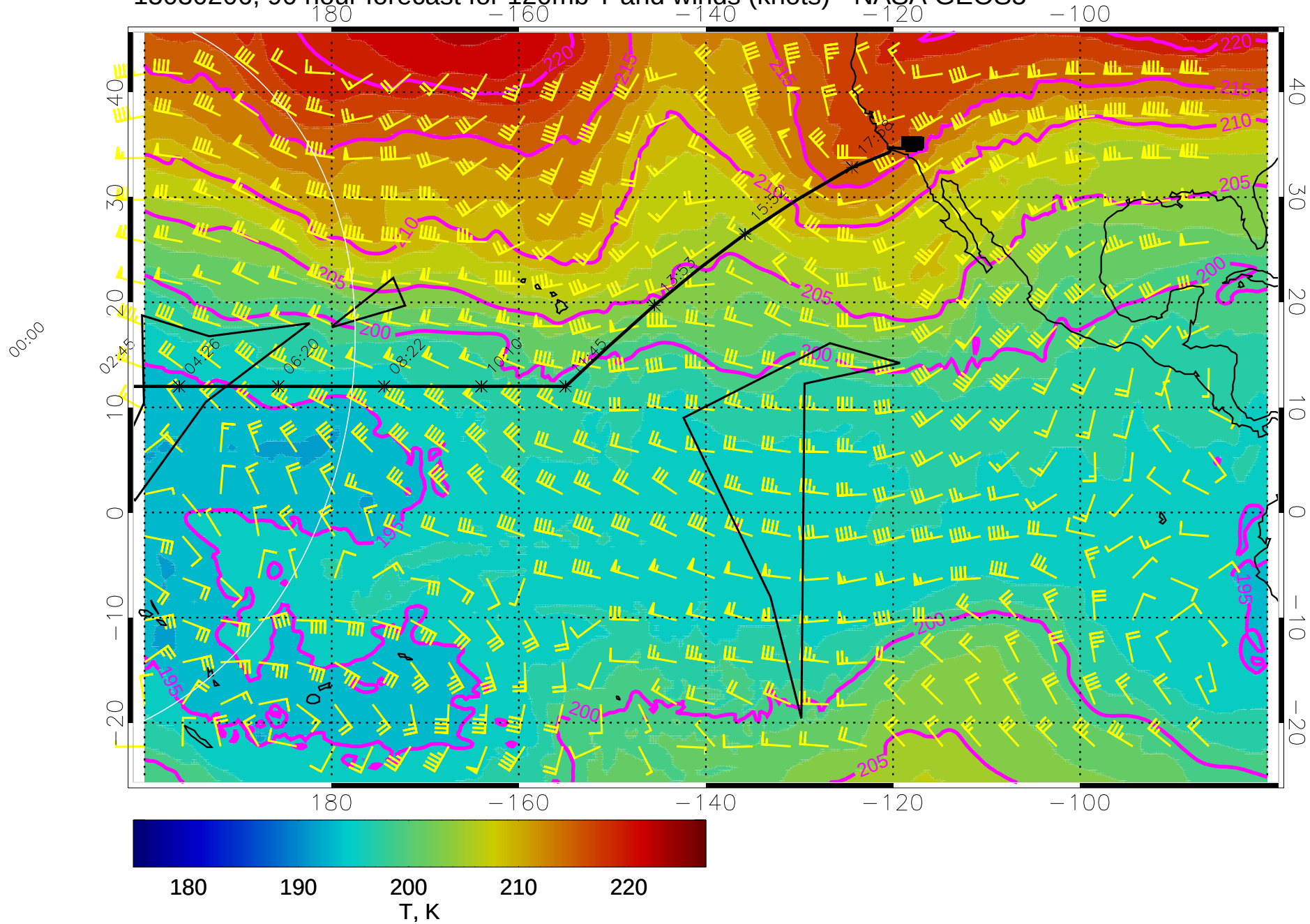
15030206, 90 hour forecast for 120mb T and winds (knots) - NASA GEOS5
