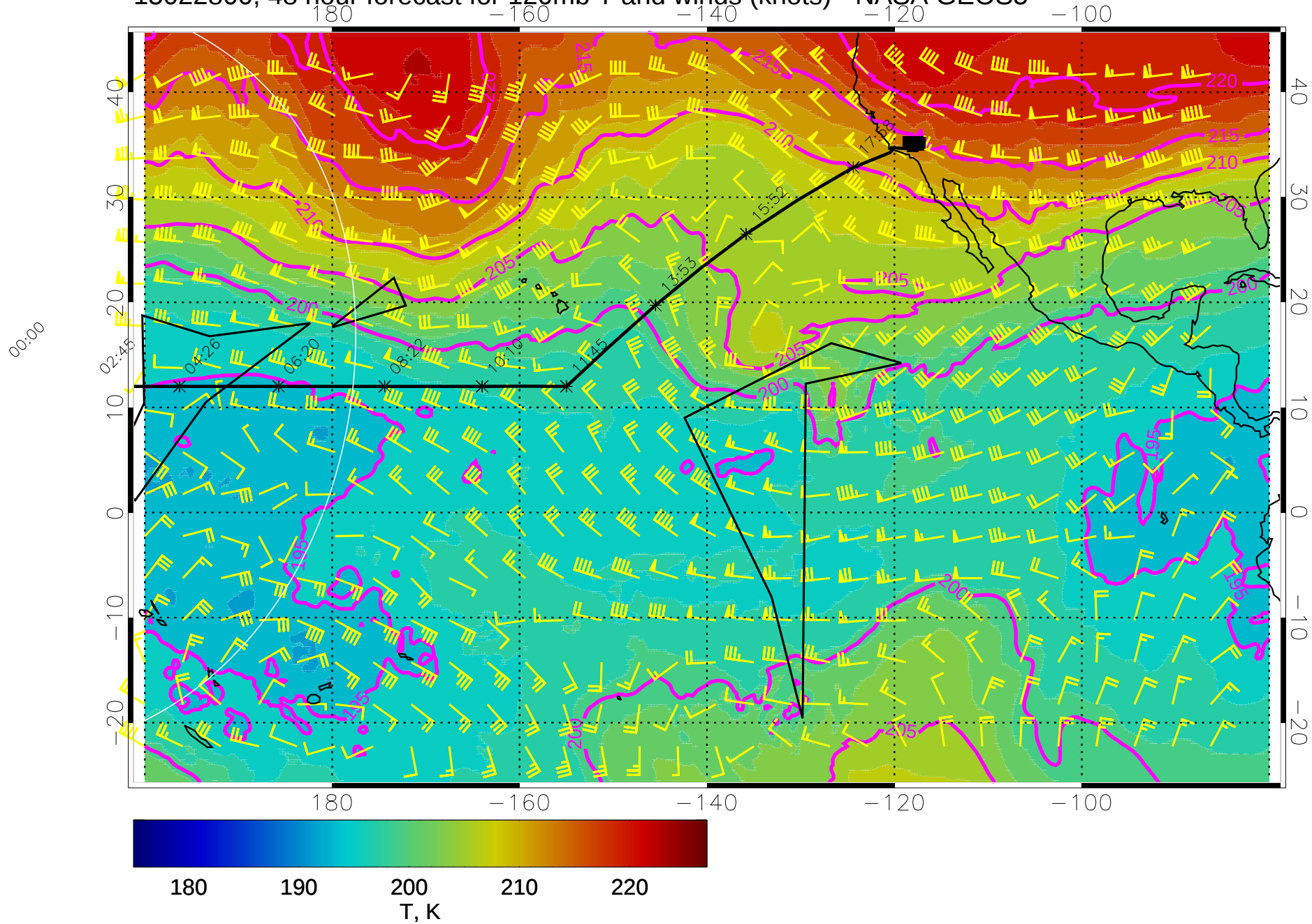
15022800, 48 hour forecast for 120mb T and winds (knots) - NASA GEOS5
