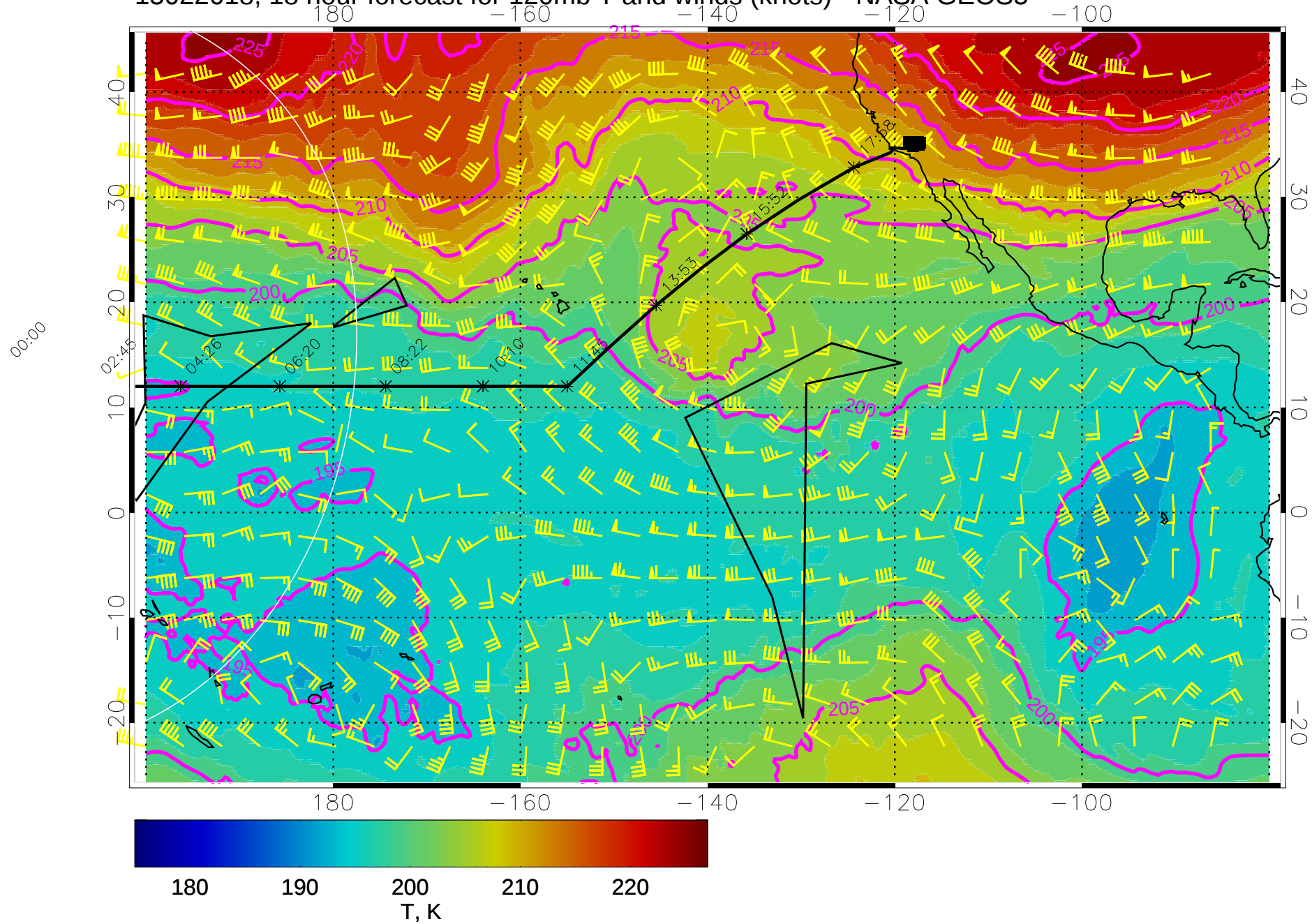
15022618, 18 hour forecast for 120mb T and winds (knots) - NASA GEOS5
