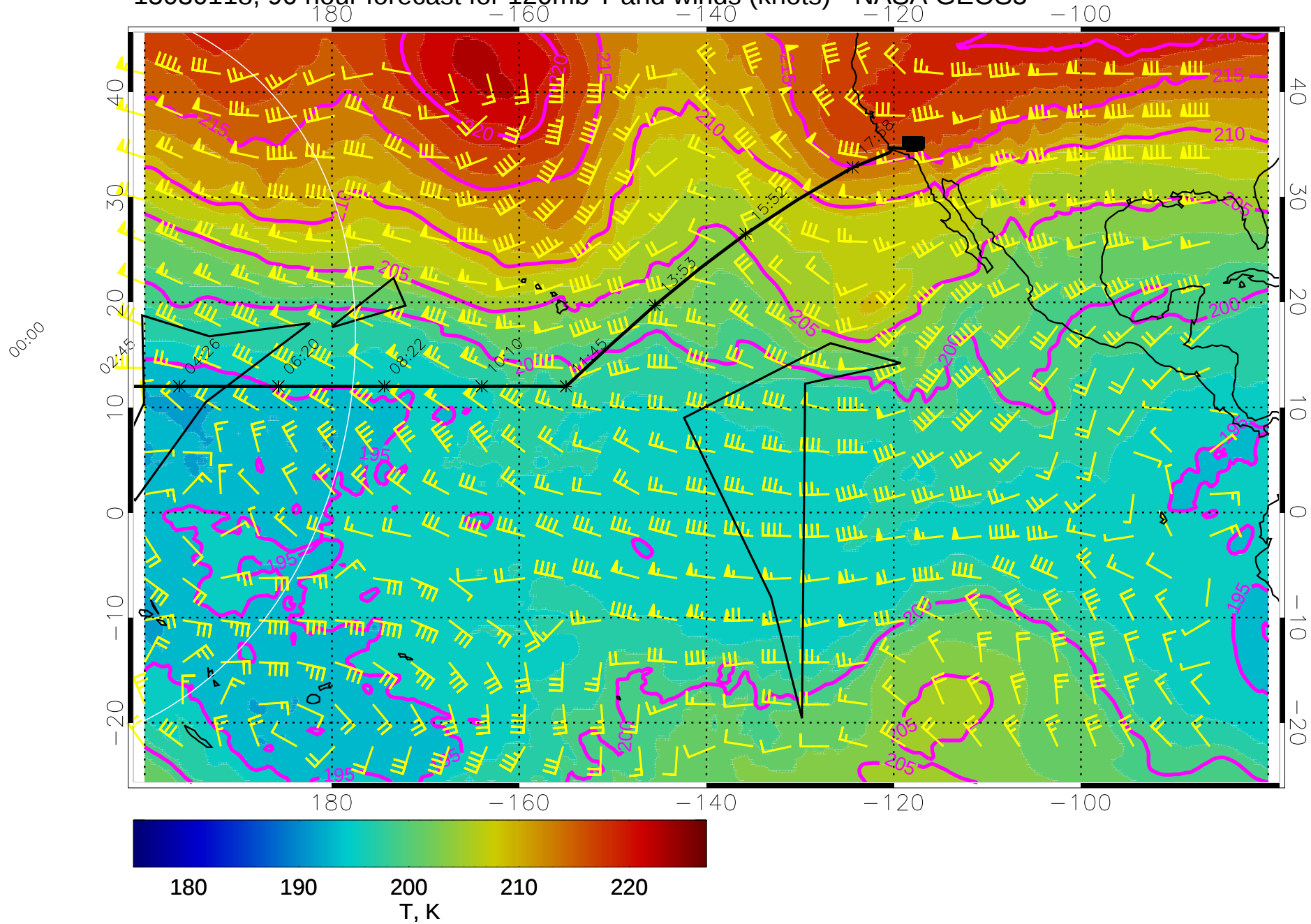
15030118, 90 hour forecast for 120mb T and winds (knots) - NASA GEOS5
