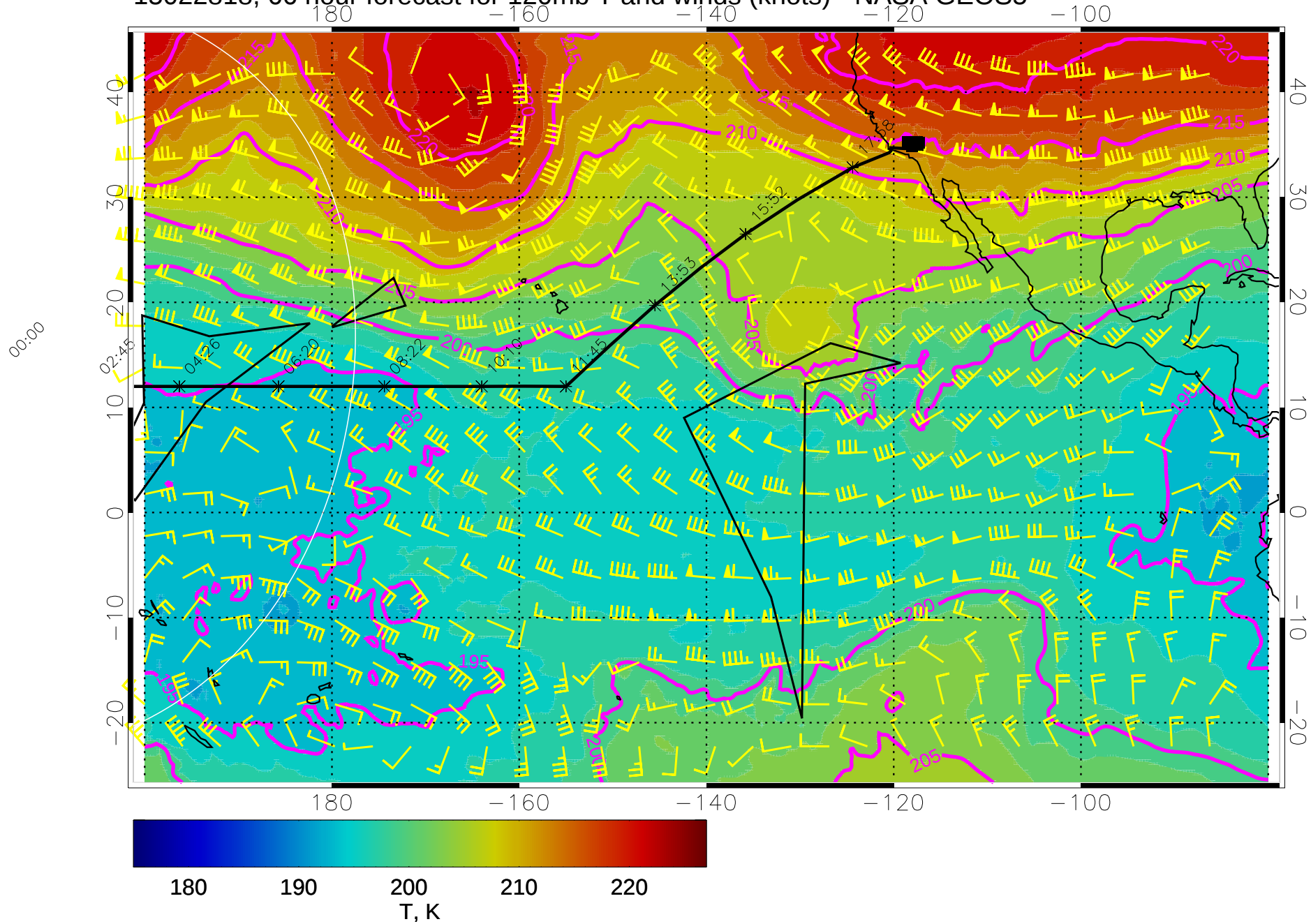
15022818, 66 hour forecast for 120mb T and winds (knots) - NASA GEOS5
