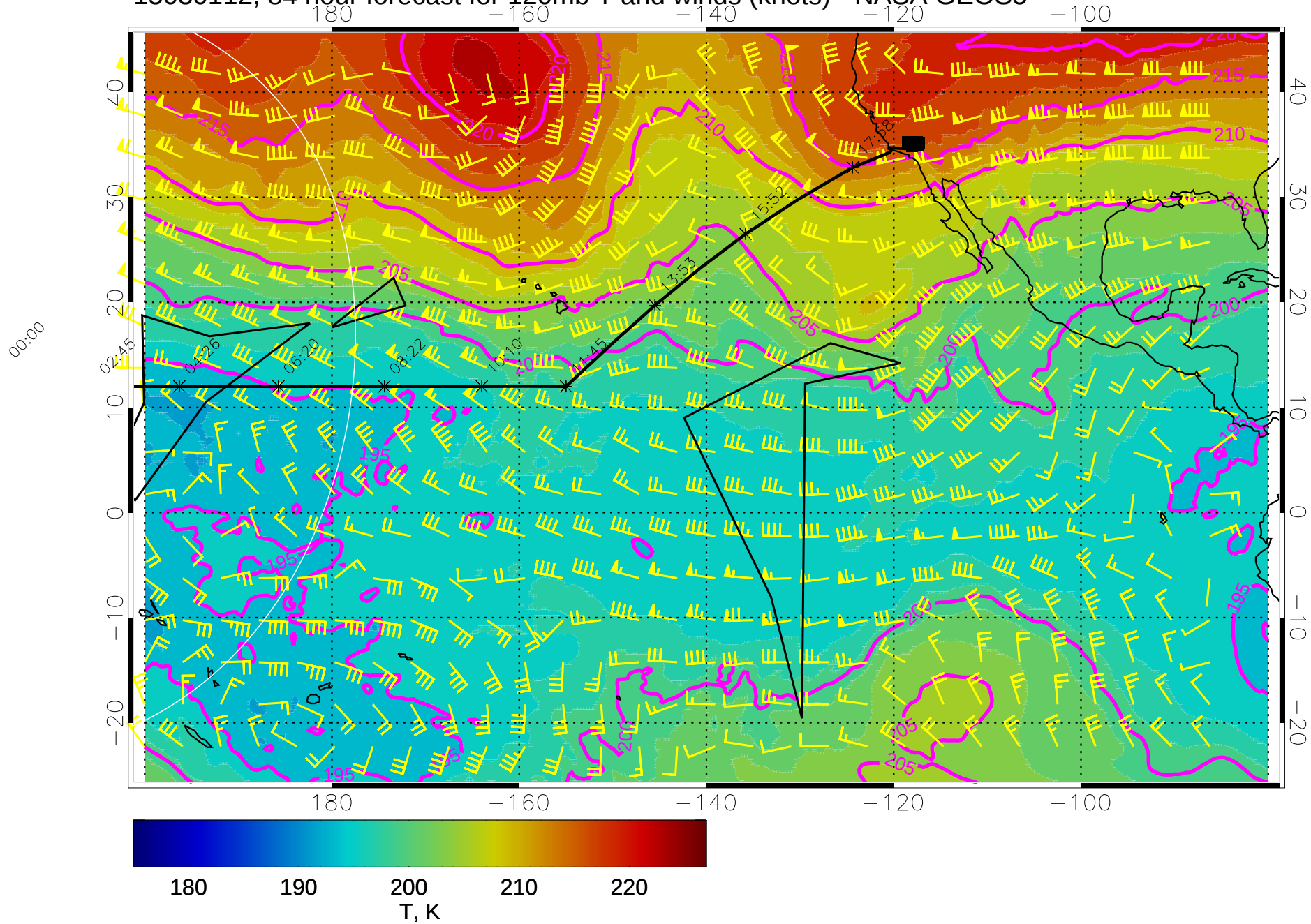
15030112, 84 hour forecast for 120mb T and winds (knots) - NASA GEOS5
