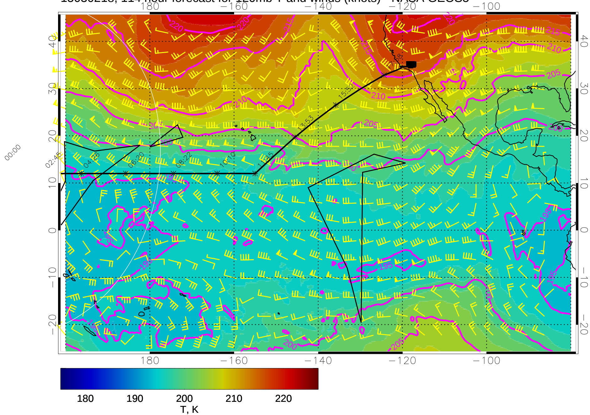
15030218, 114 hour forecast for 120mb T and winds (knots) - NASA GEOS5
