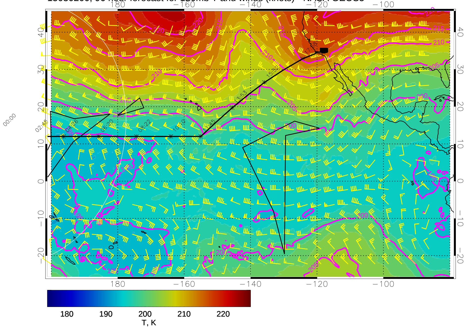
15030200, 96 hour forecast for 120mb T and winds (knots) - NASA GEOS5
