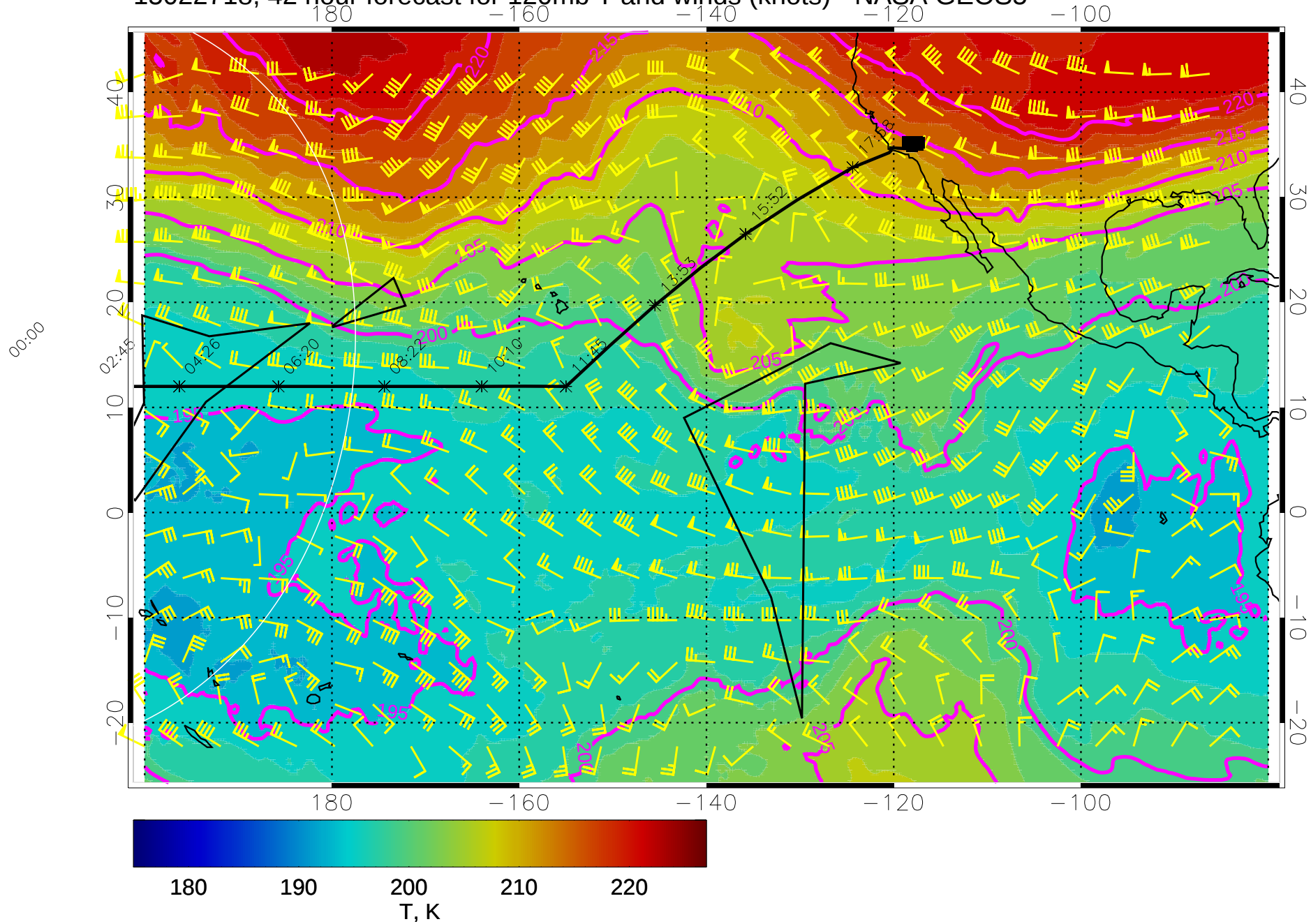
15022718, 42 hour forecast for 120mb T and winds (knots) - NASA GEOS5
