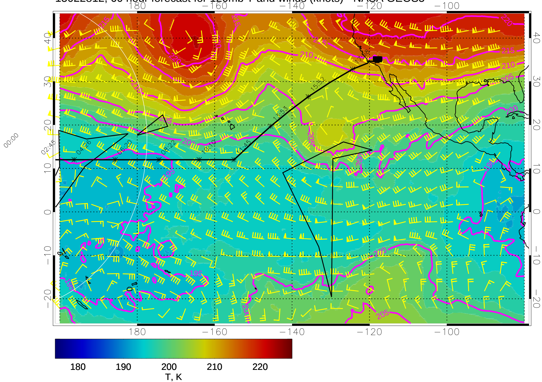
15022812, 60 hour forecast for 120mb T and winds (knots) - NASA GEOS5
