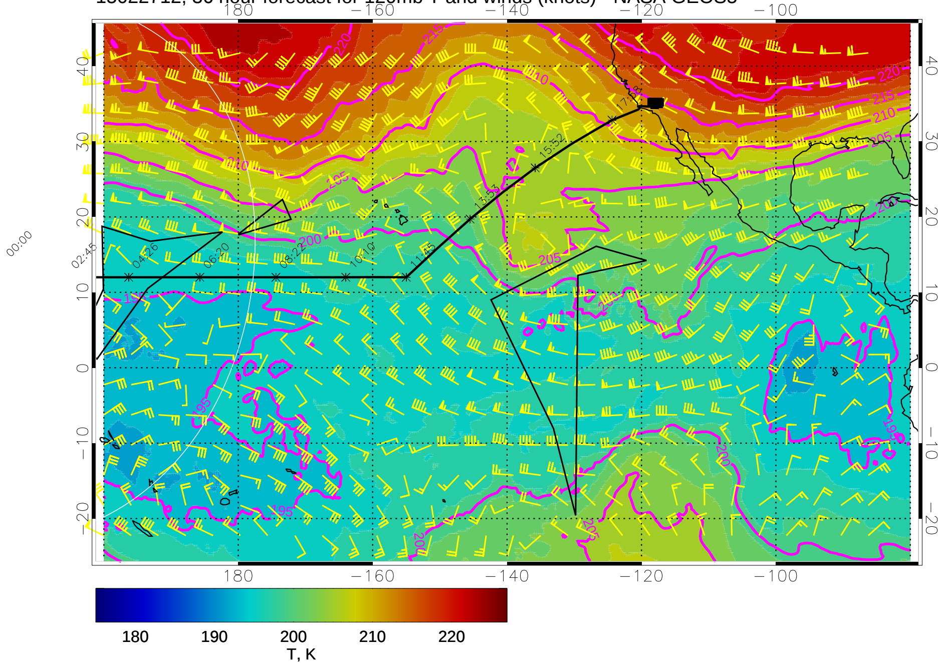
15022712, 36 hour forecast for 120mb T and winds (knots) - NASA GEOS5
