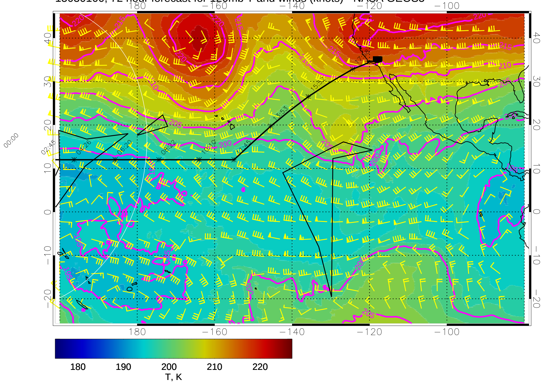
15030100, 72 hour forecast for 120mb T and winds (knots) - NASA GEOS5
