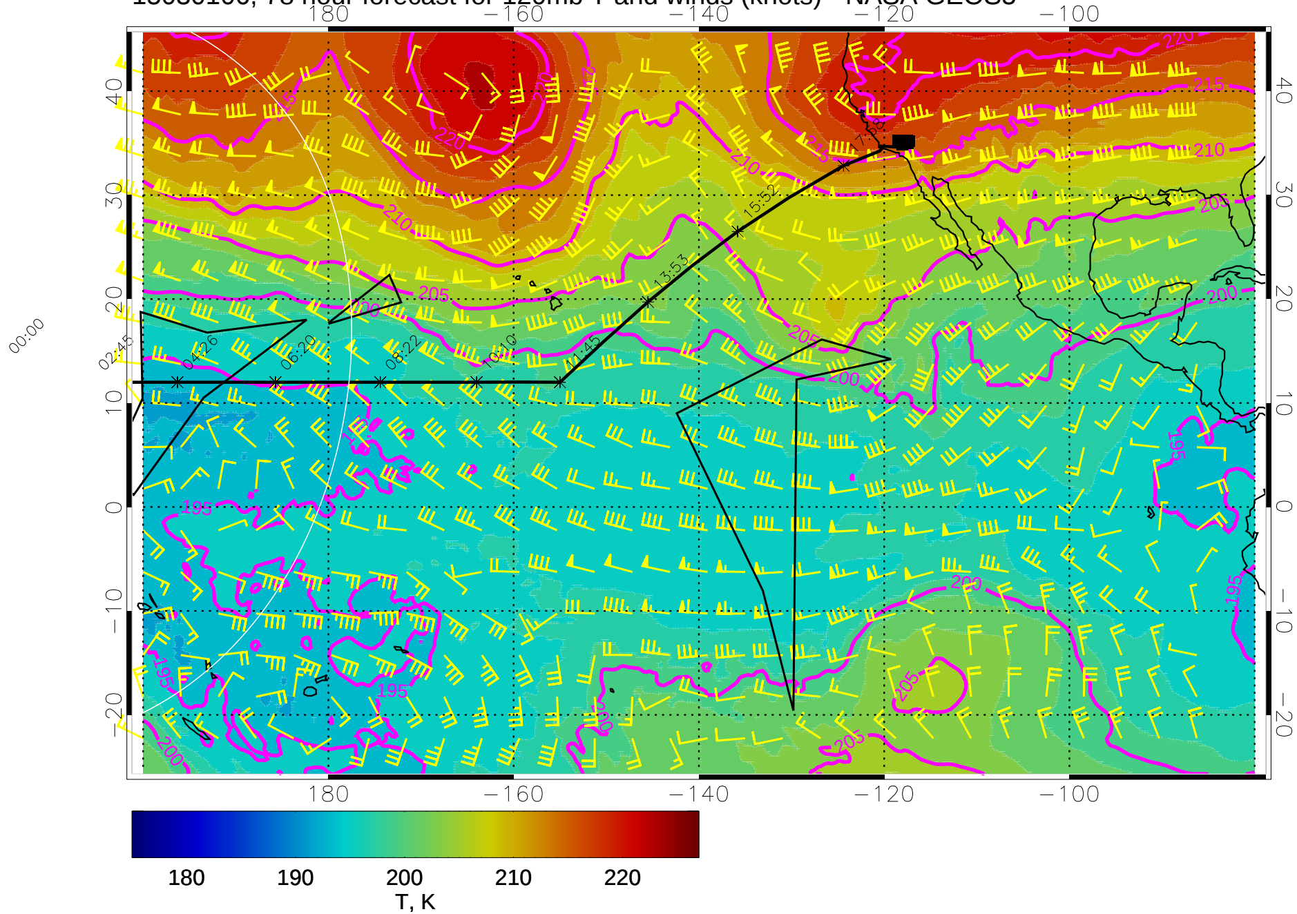
15030106, 78 hour forecast for 120mb T and winds (knots) - NASA GEOS5
