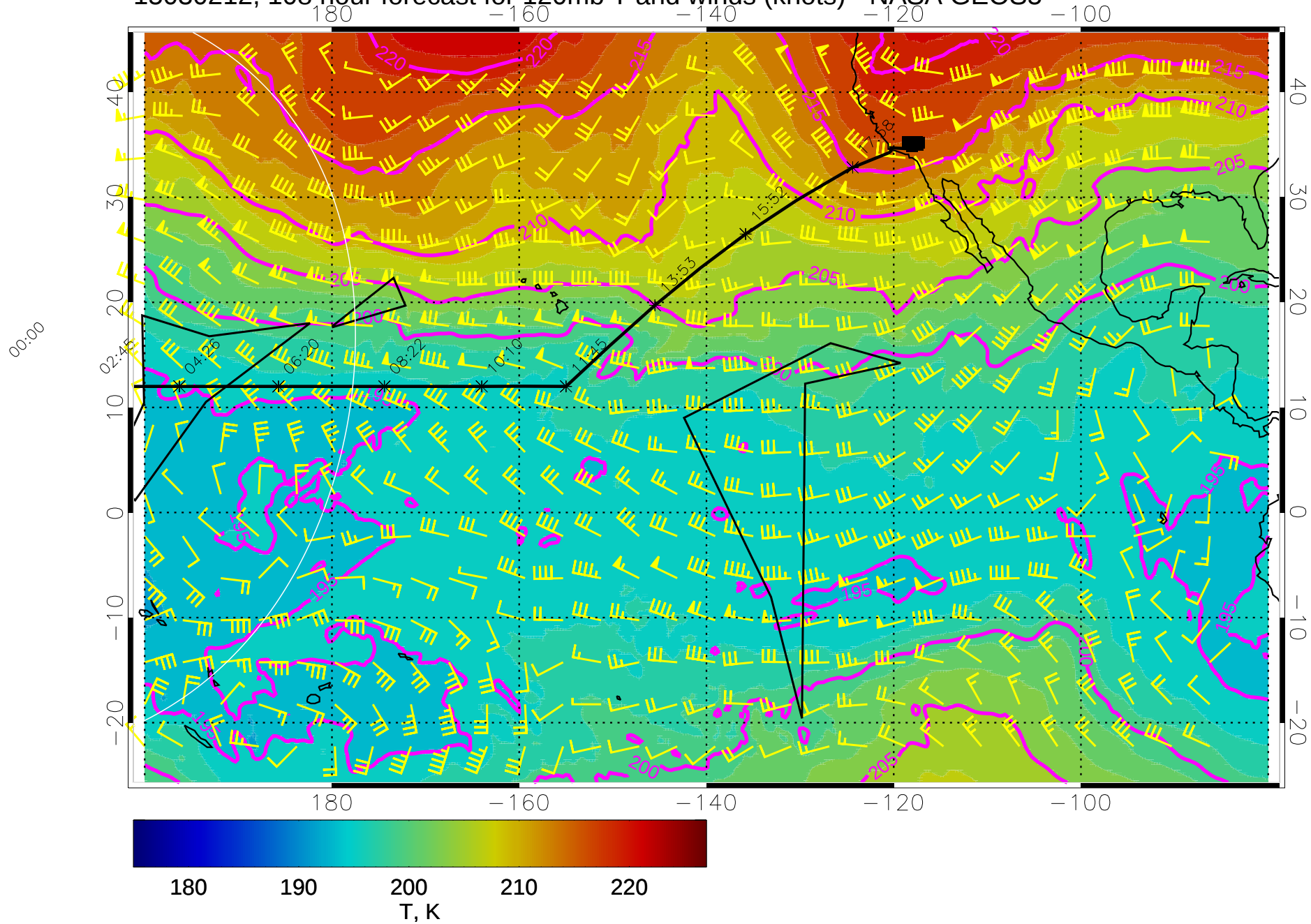
15030212, 108 hour forecast for 120mb T and winds (knots) - NASA GEOS5
