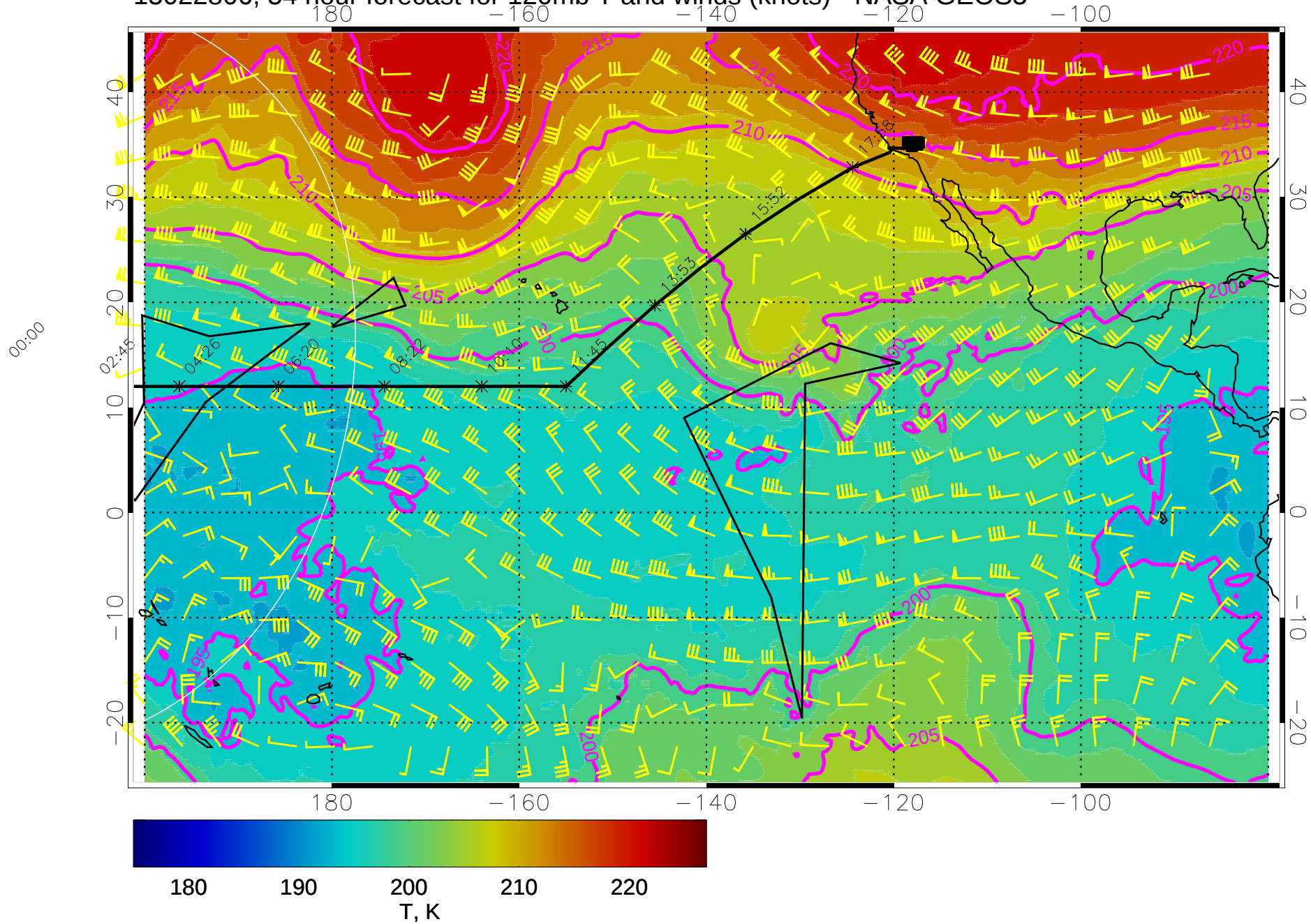
15022806, 54 hour forecast for 120mb T and winds (knots) - NASA GEOS5
