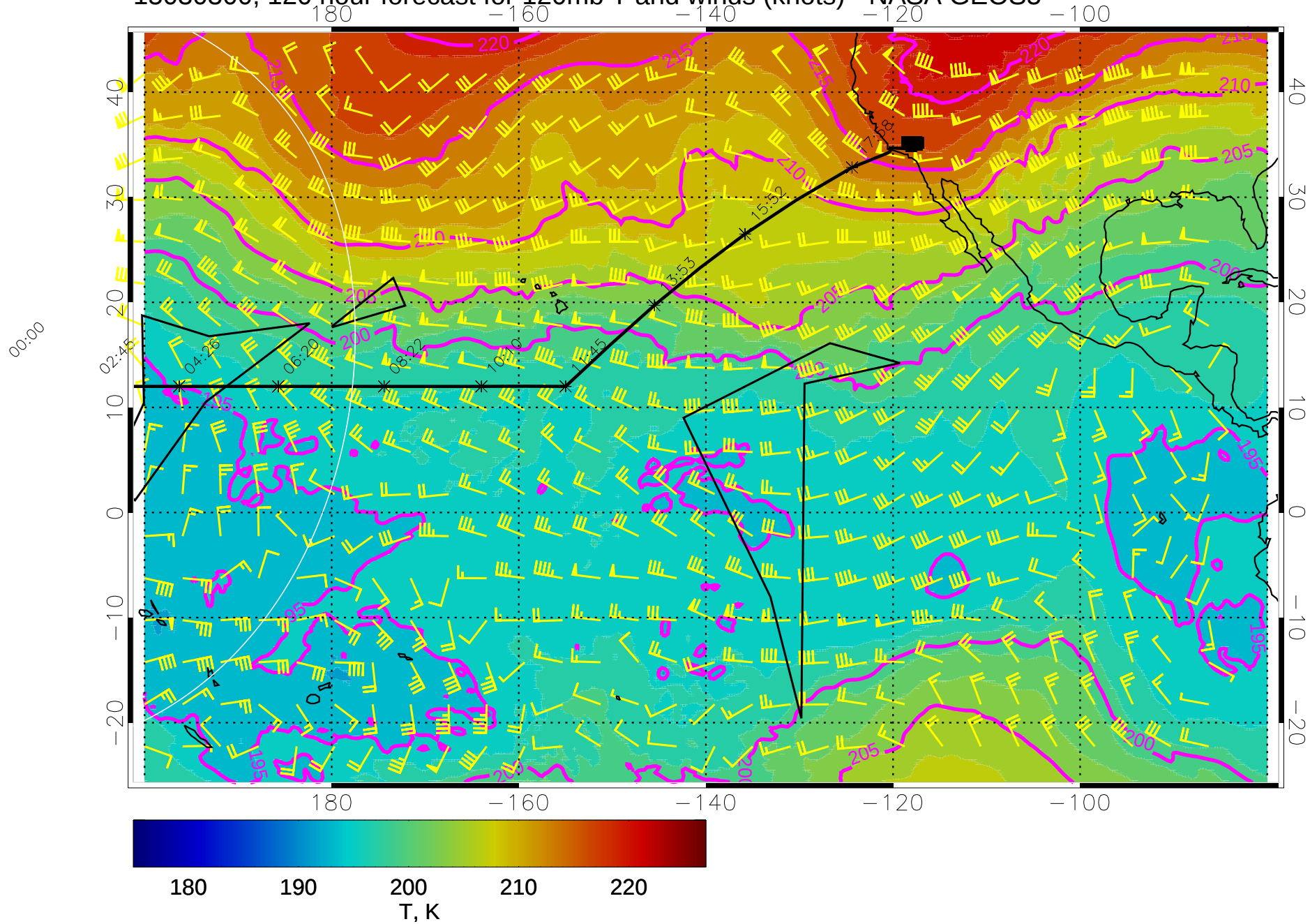
15030300, 120 hour forecast for 120mb T and winds (knots) - NASA GEOS5
