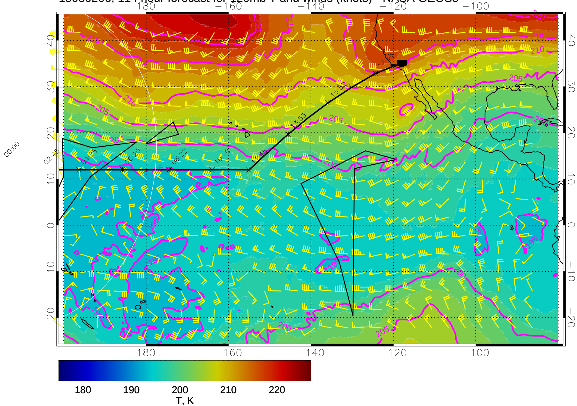
15030206, 114 hour forecast for 120mb T and winds (knots) - NASA GEOS5
