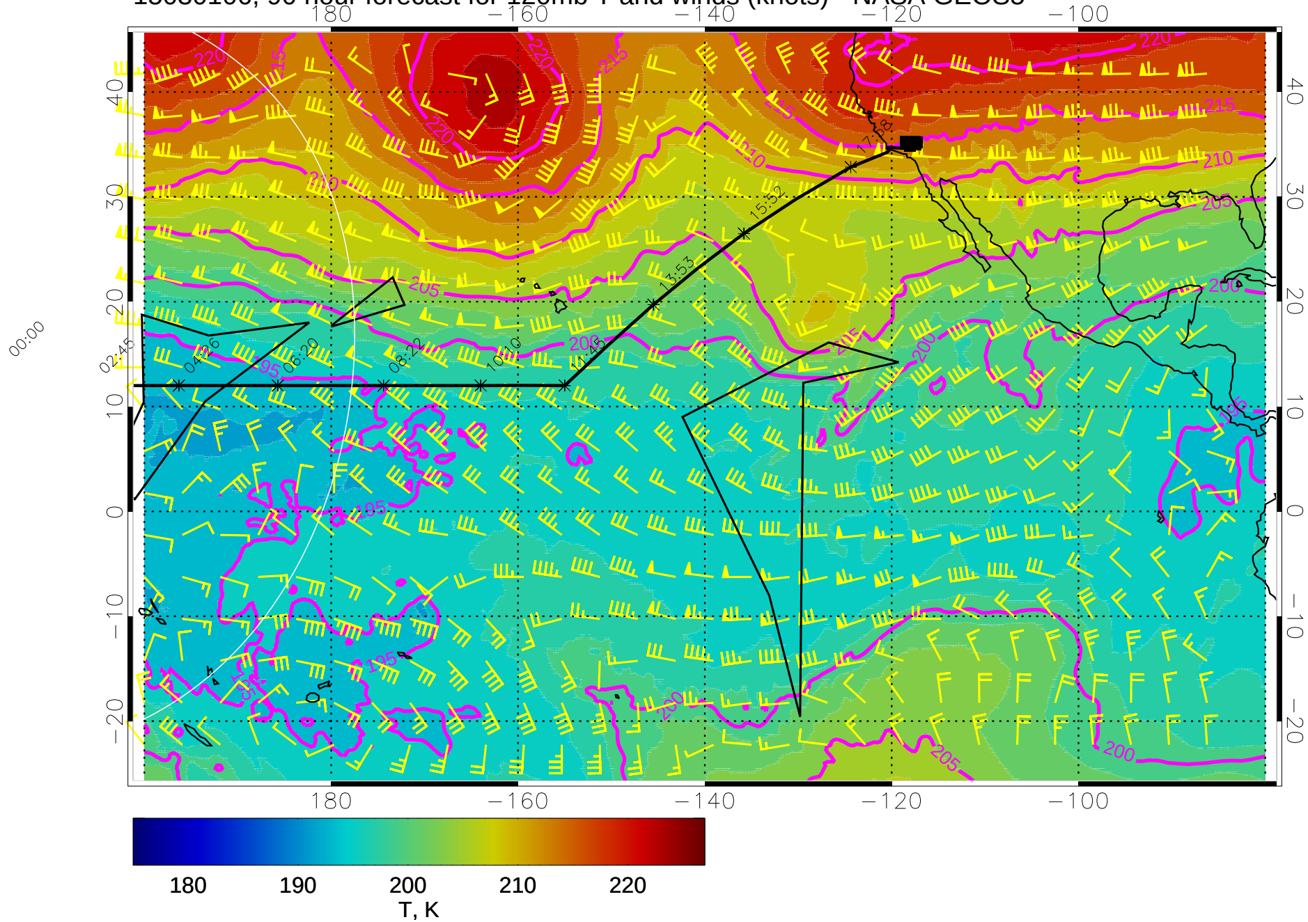
15030106, 90 hour forecast for 120mb T and winds (knots) - NASA GEOS5
