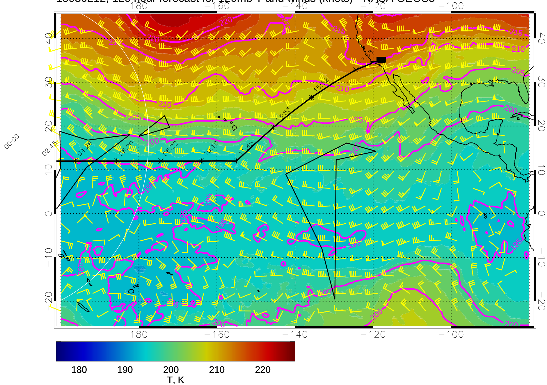
15030212, 120 hour forecast for 120mb T and winds (knots) - NASA GEOS5
