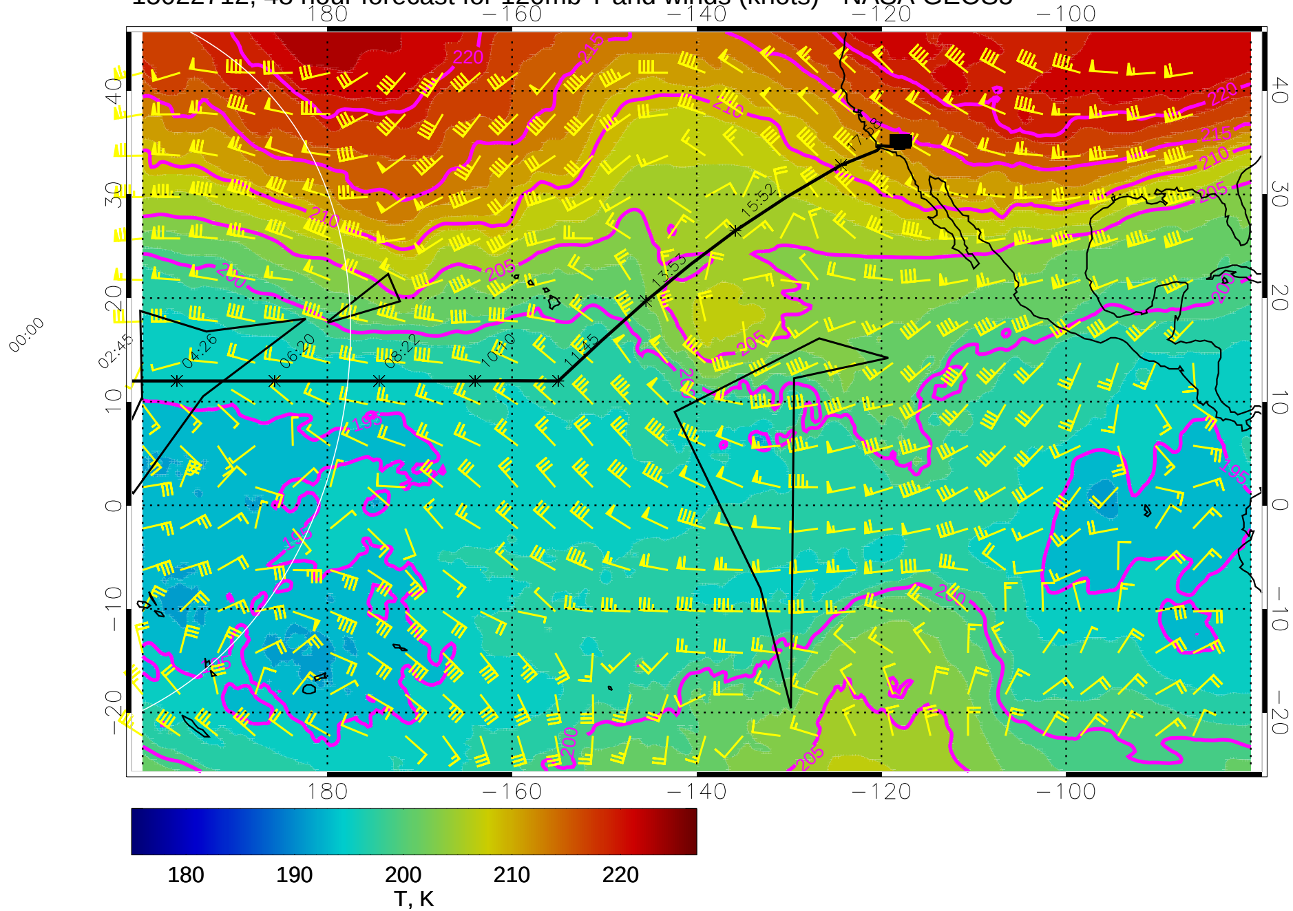
15022712, 48 hour forecast for 120mb T and winds (knots) - NASA GEOS5
