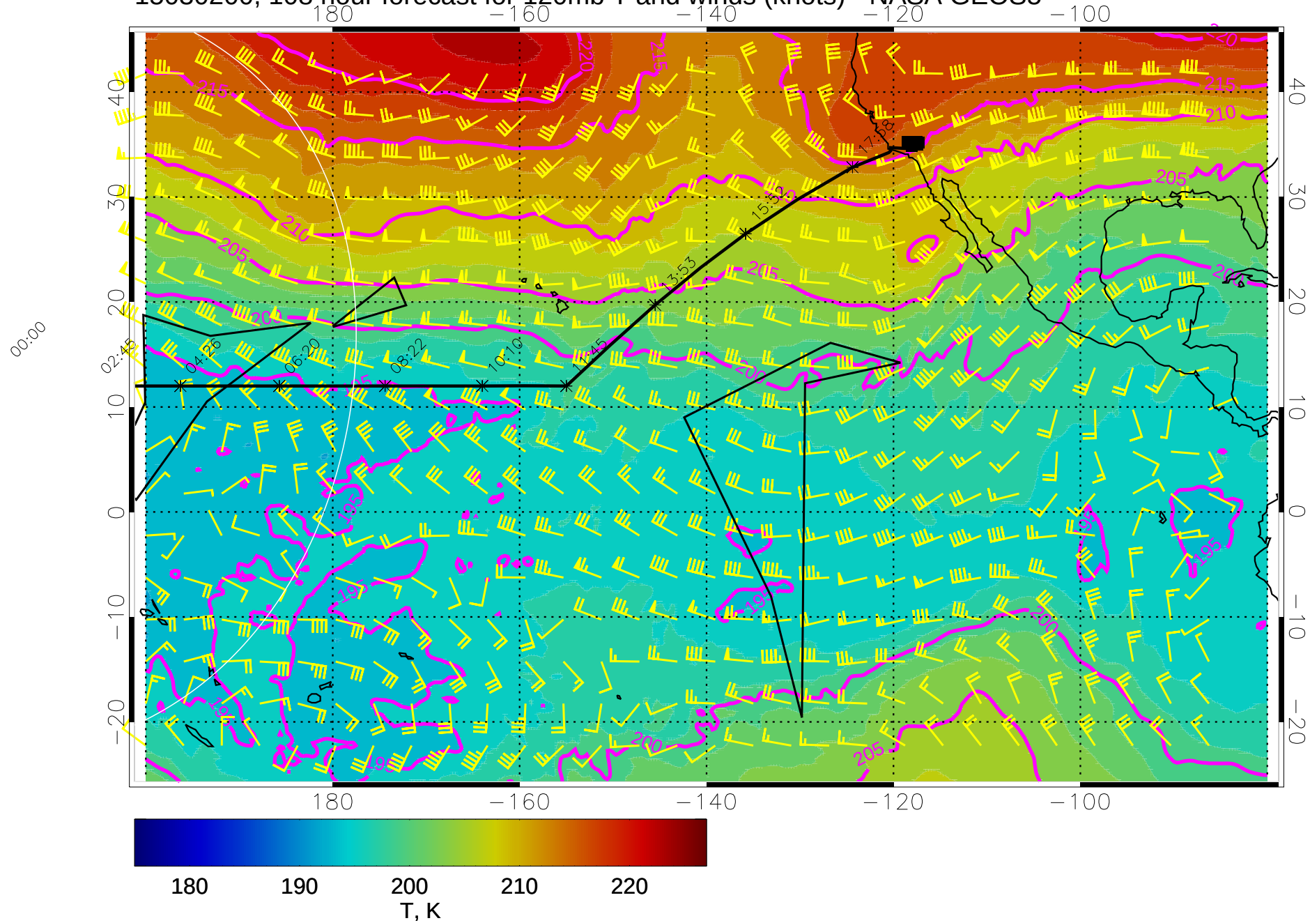
15030200, 108 hour forecast for 120mb T and winds (knots) - NASA GEOS5
