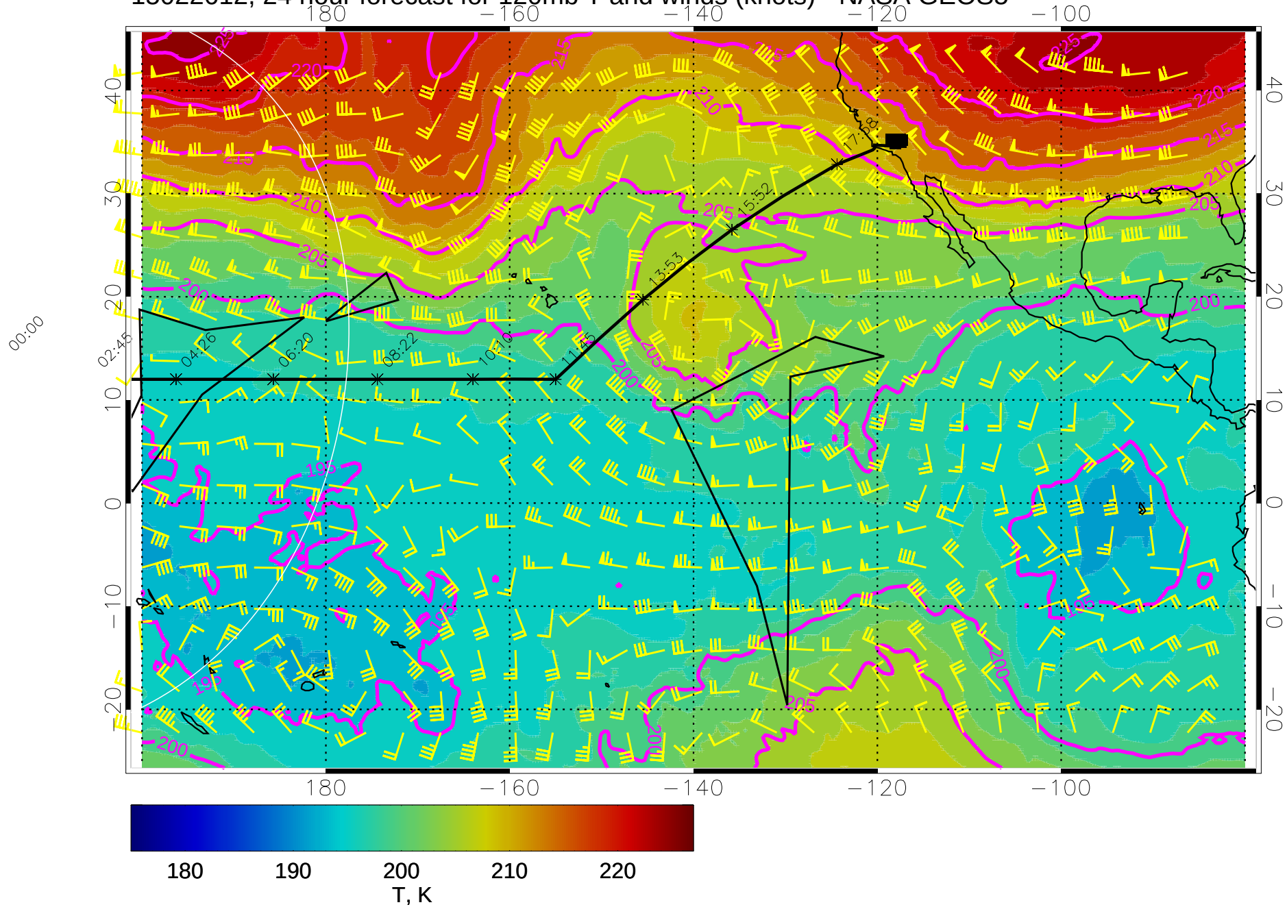
15022612, 24 hour forecast for 120mb T and winds (knots) - NASA GEOS5
