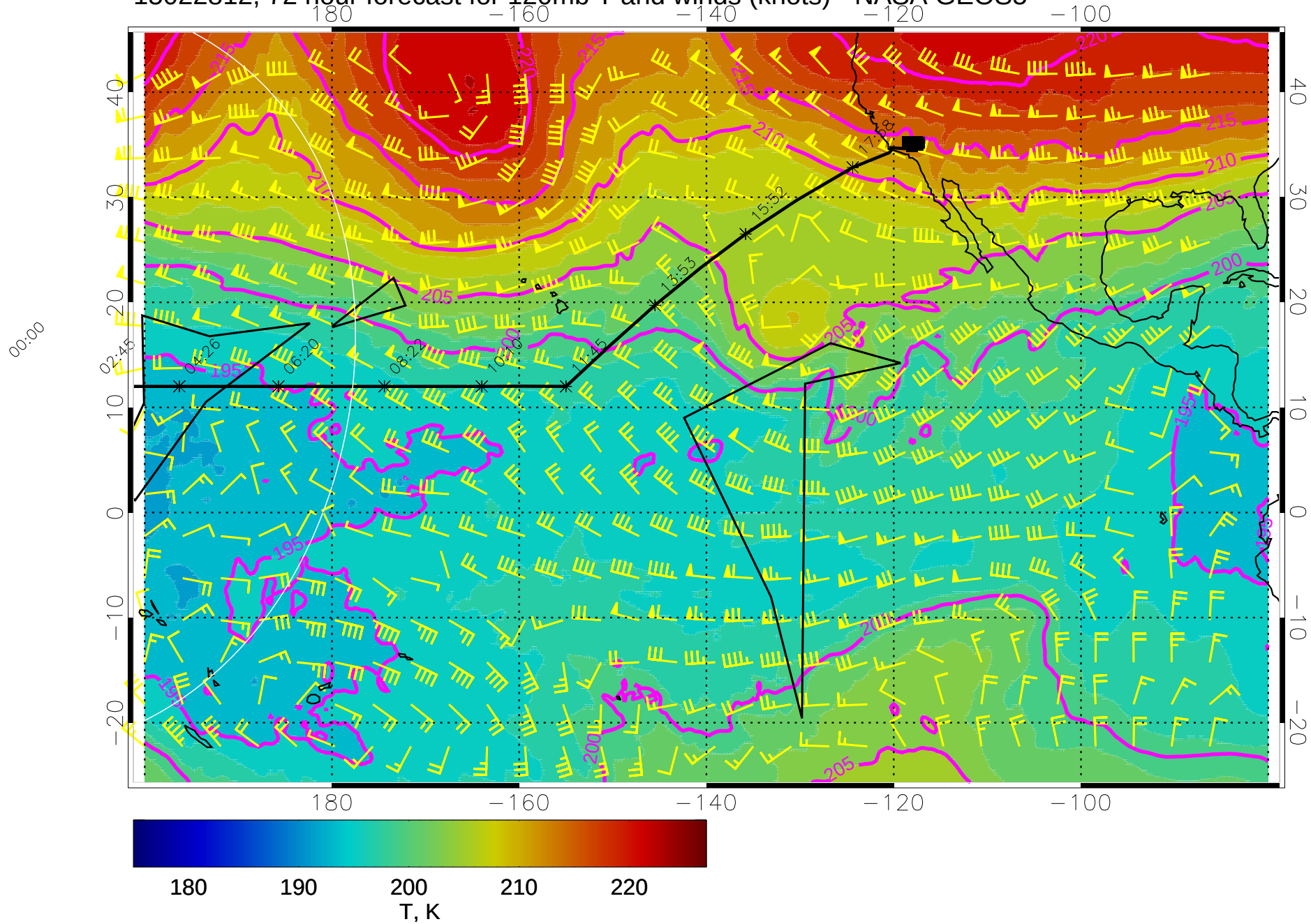
15022812, 72 hour forecast for 120mb T and winds (knots) - NASA GEOS5
