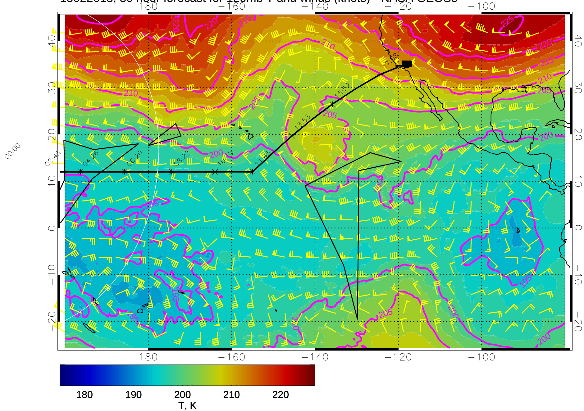
15022618, 30 hour forecast for 120mb T and winds (knots) - NASA GEOS5
