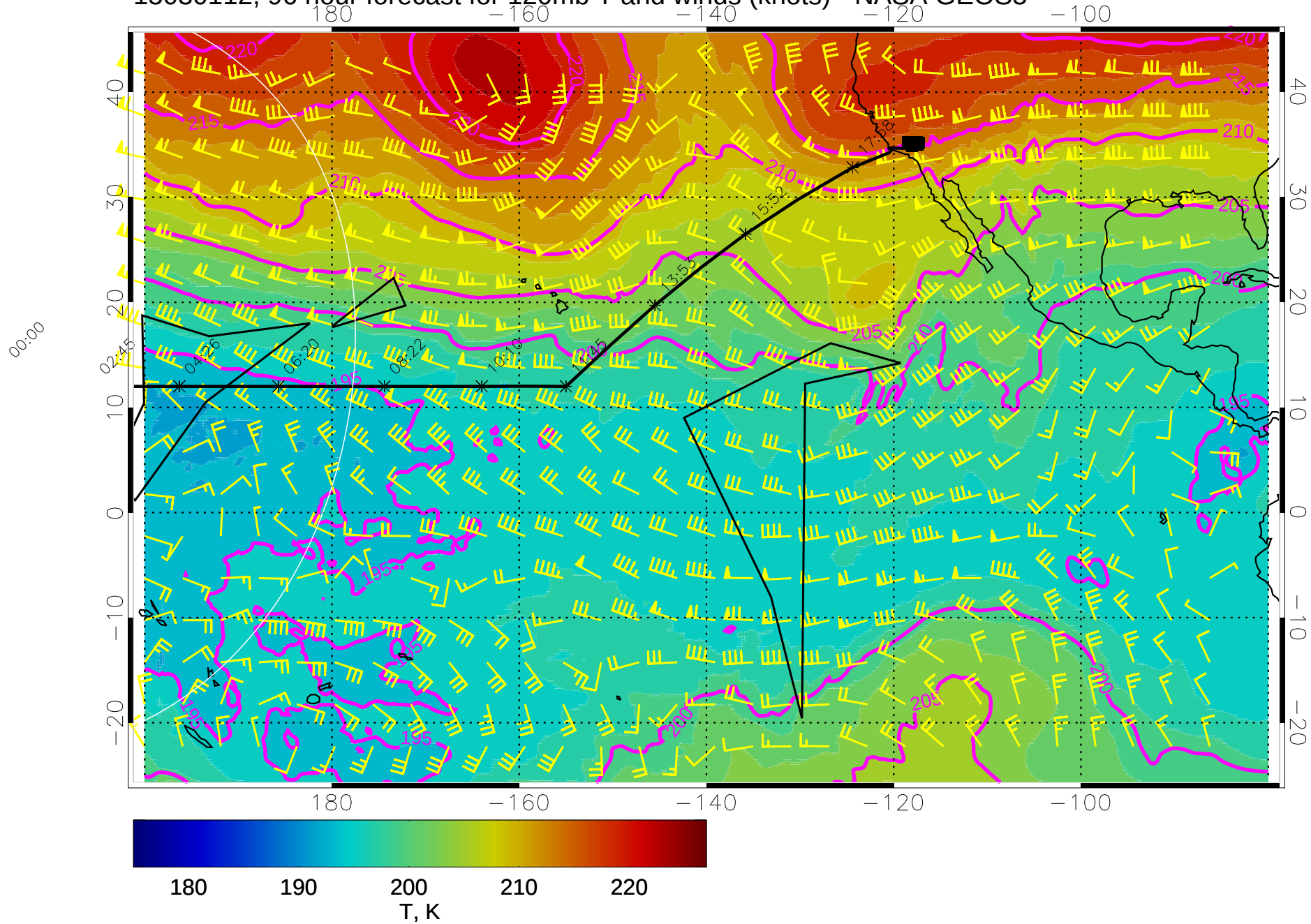
15030112, 96 hour forecast for 120mb T and winds (knots) - NASA GEOS5
