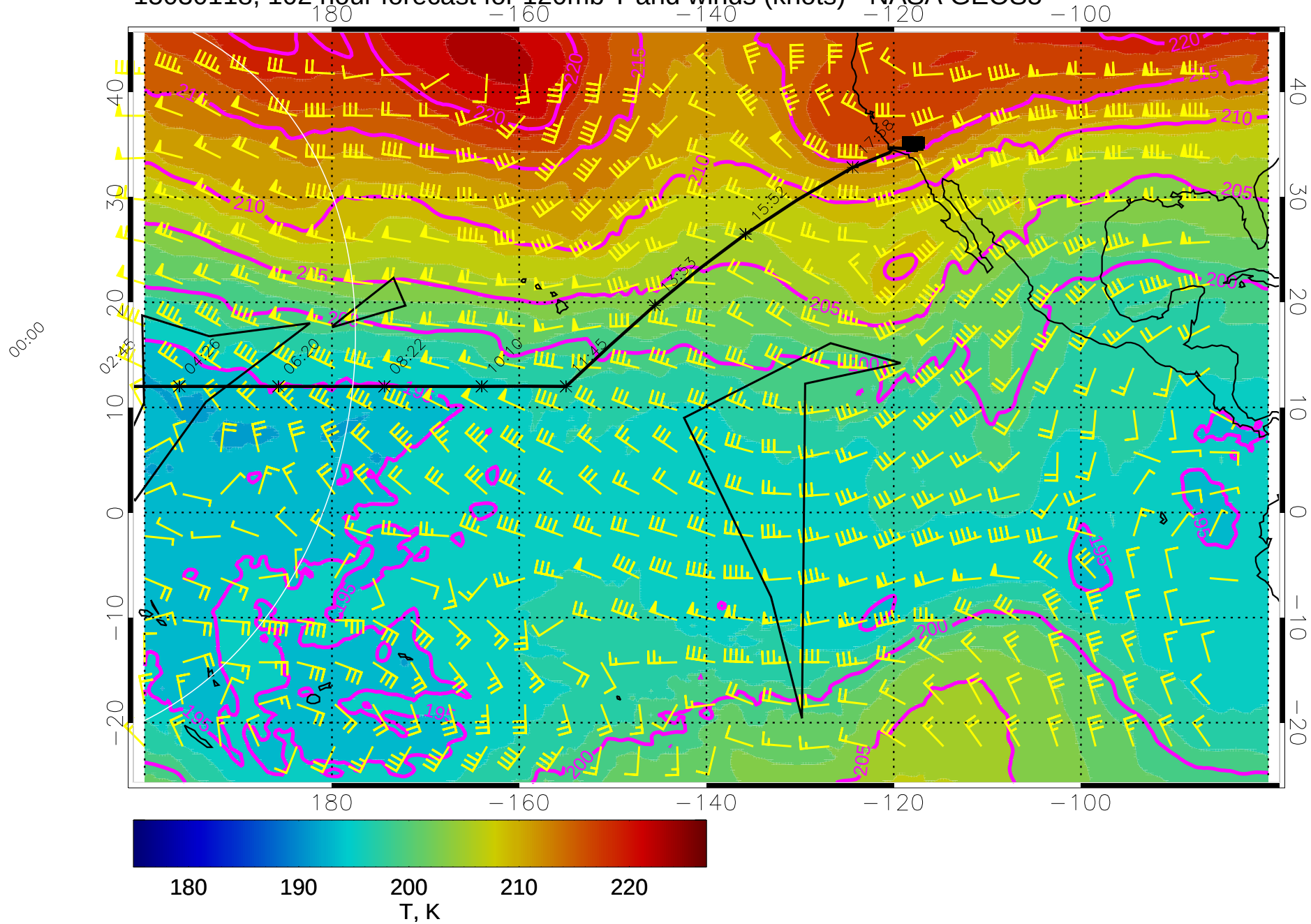
15030118, 102 hour forecast for 120mb T and winds (knots) - NASA GEOS5
