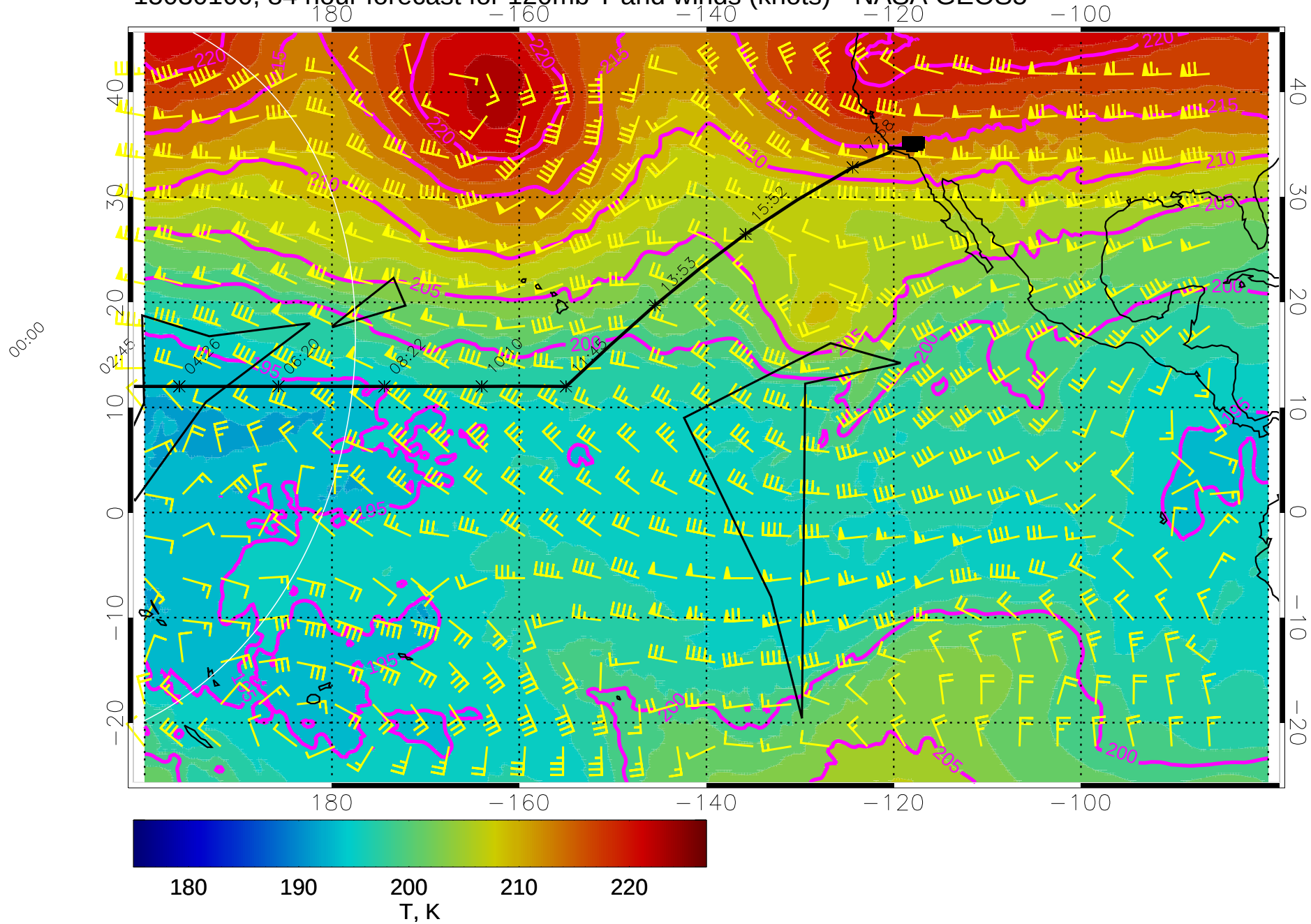
15030100, 84 hour forecast for 120mb T and winds (knots) - NASA GEOS5
