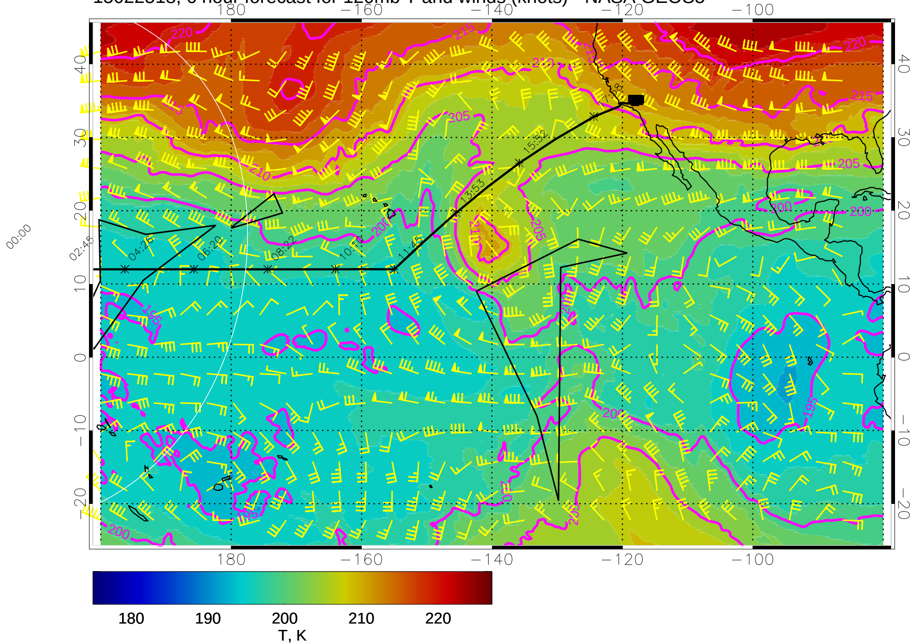
15022518, 6 hour forecast for 120mb T and winds (knots) - NASA GEOS5
