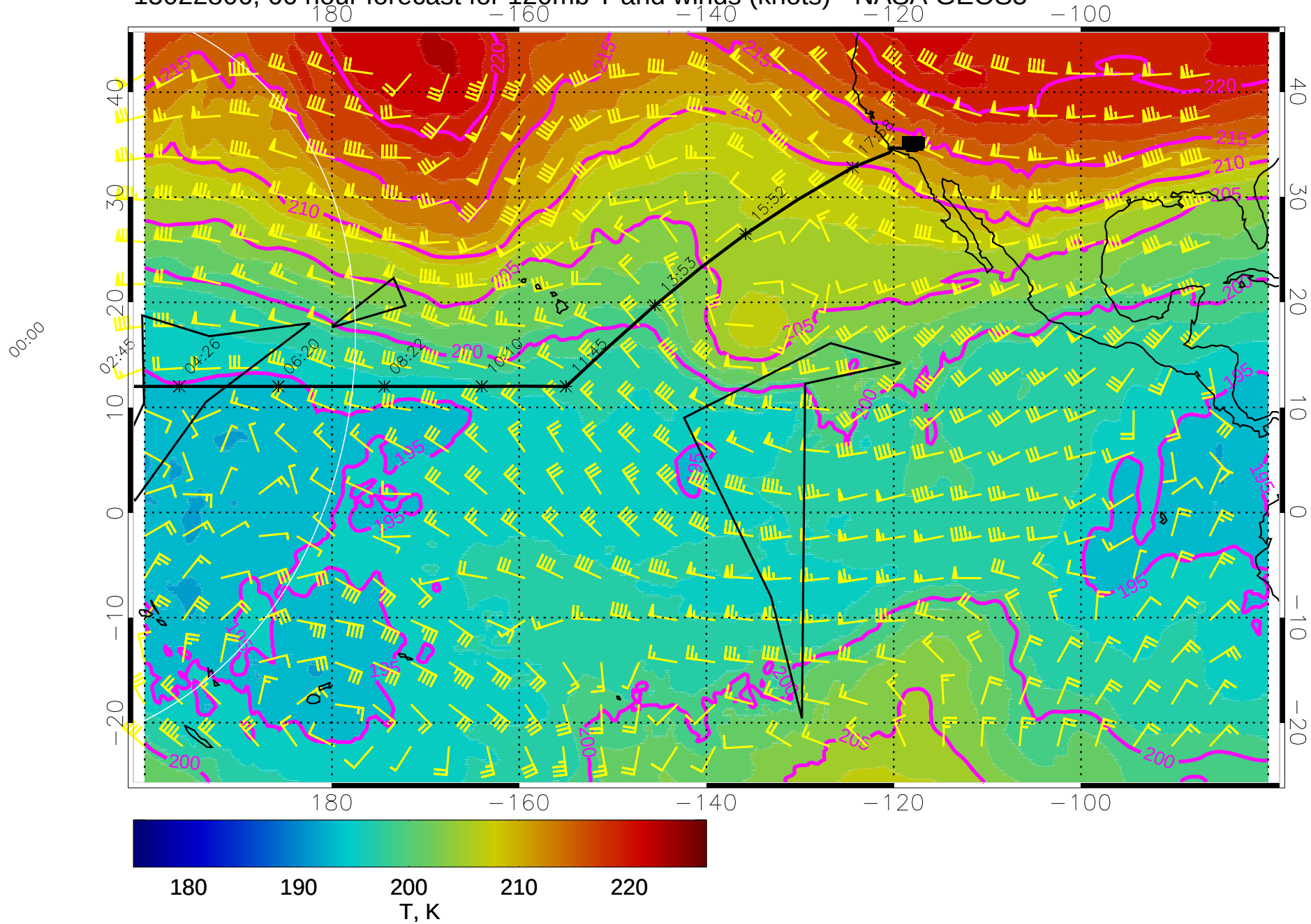
15022806, 66 hour forecast for 120mb T and winds (knots) - NASA GEOS5
