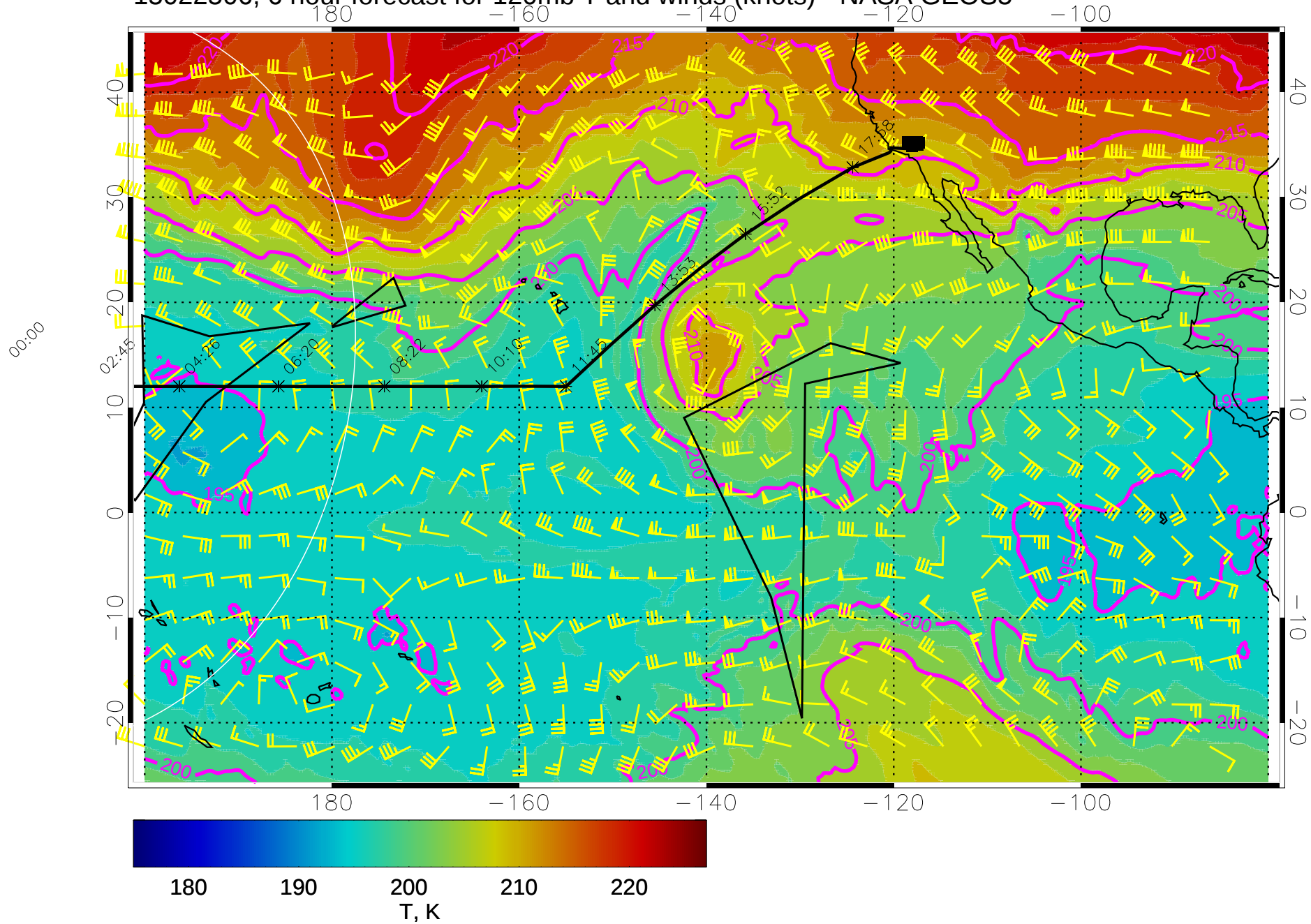
15022506, 6 hour forecast for 120mb T and winds (knots) - NASA GEOS5
