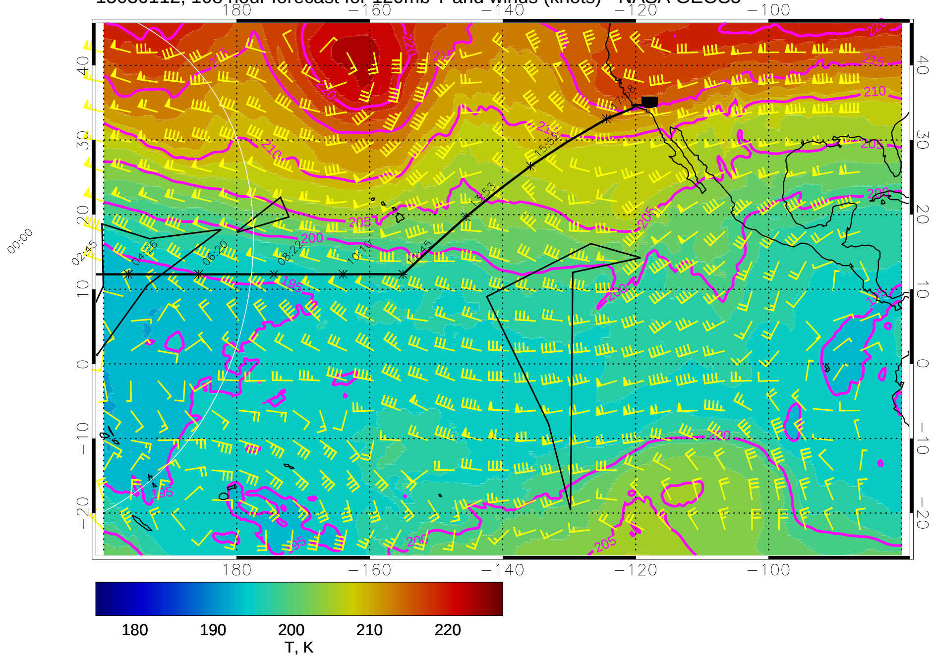
15030112, 108 hour forecast for 120mb T and winds (knots) - NASA GEOS5
