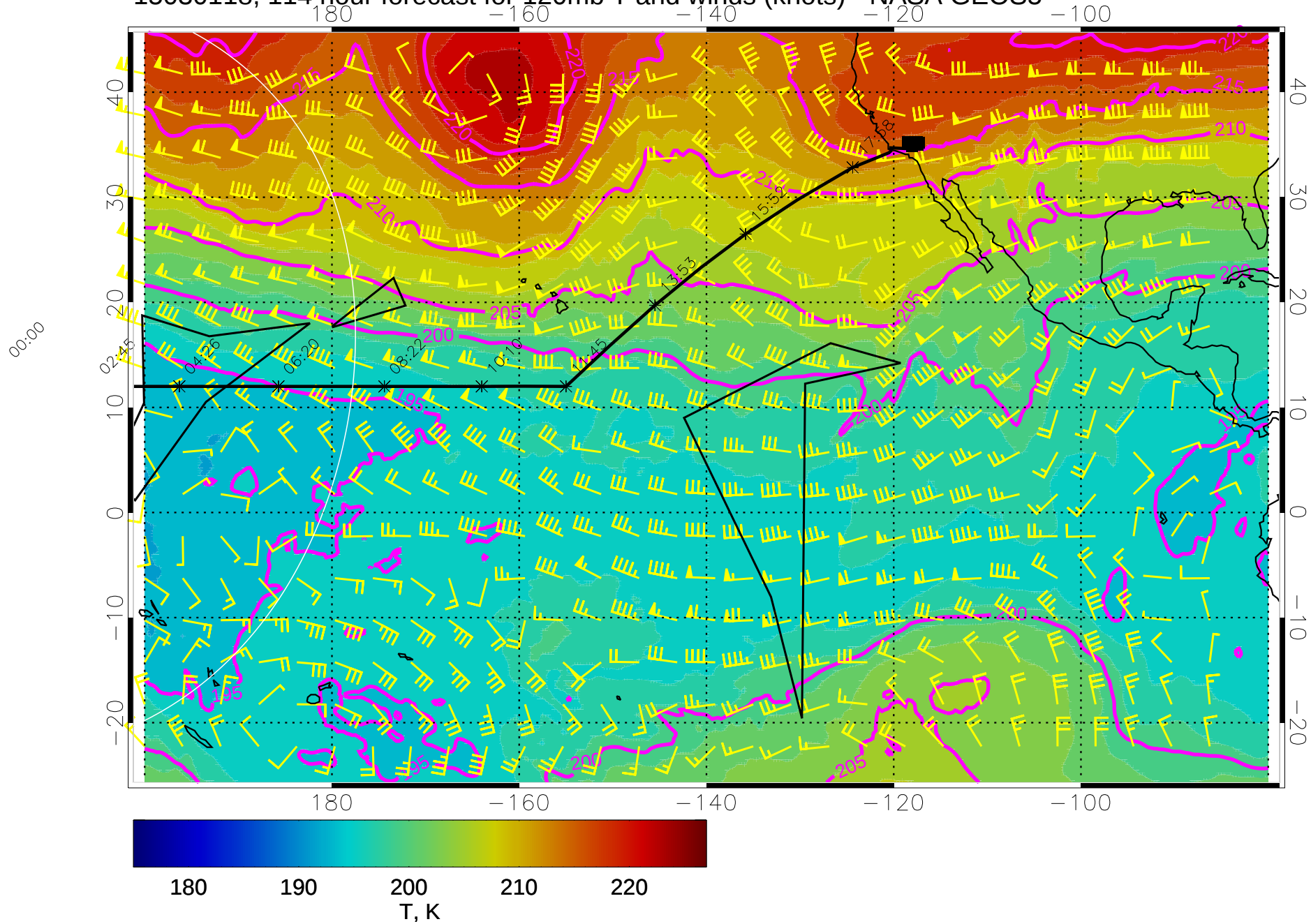
15030118, 114 hour forecast for 120mb T and winds (knots) - NASA GEOS5
