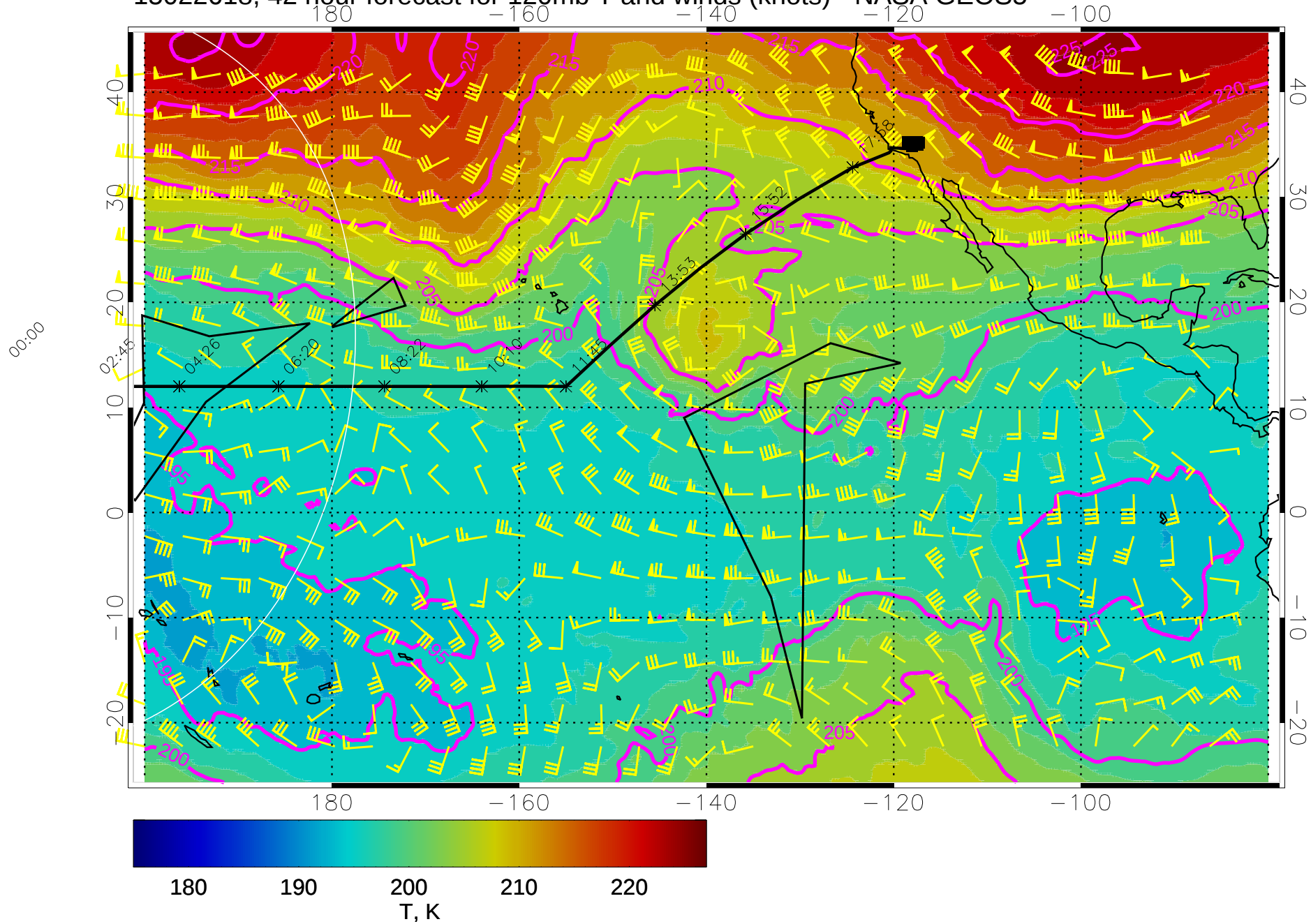
15022618, 42 hour forecast for 120mb T and winds (knots) - NASA GEOS5
