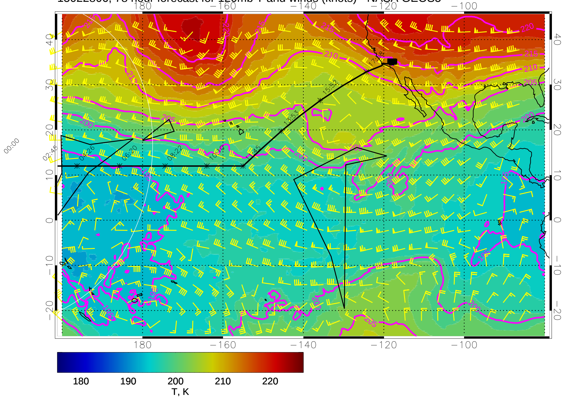
15022806, 78 hour forecast for 120mb T and winds (knots) - NASA GEOS5
