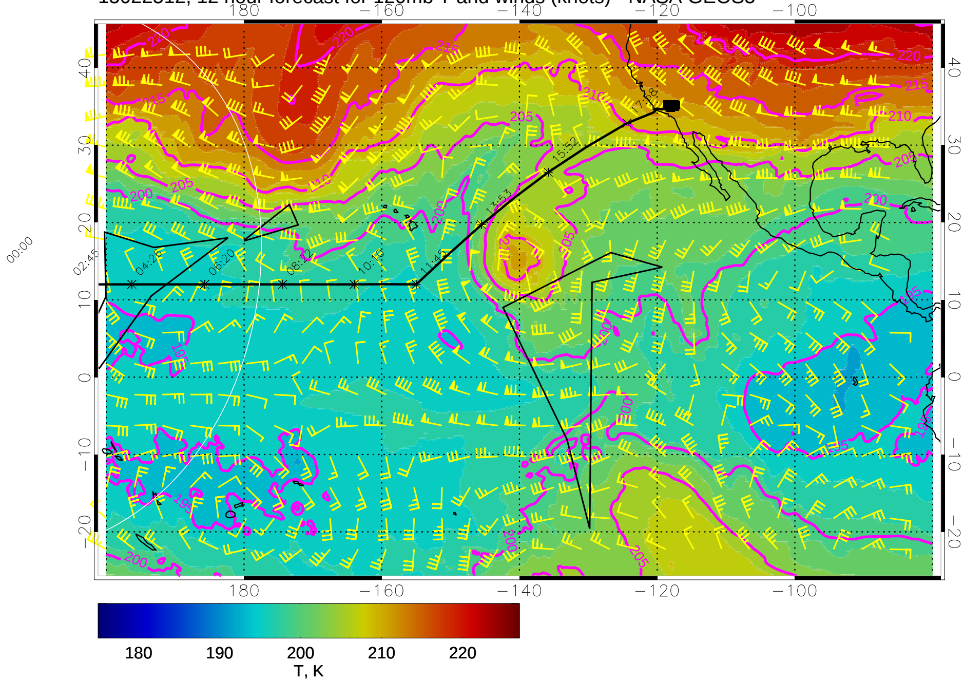
15022512, 12 hour forecast for 120mb T and winds (knots) - NASA GEOS5
