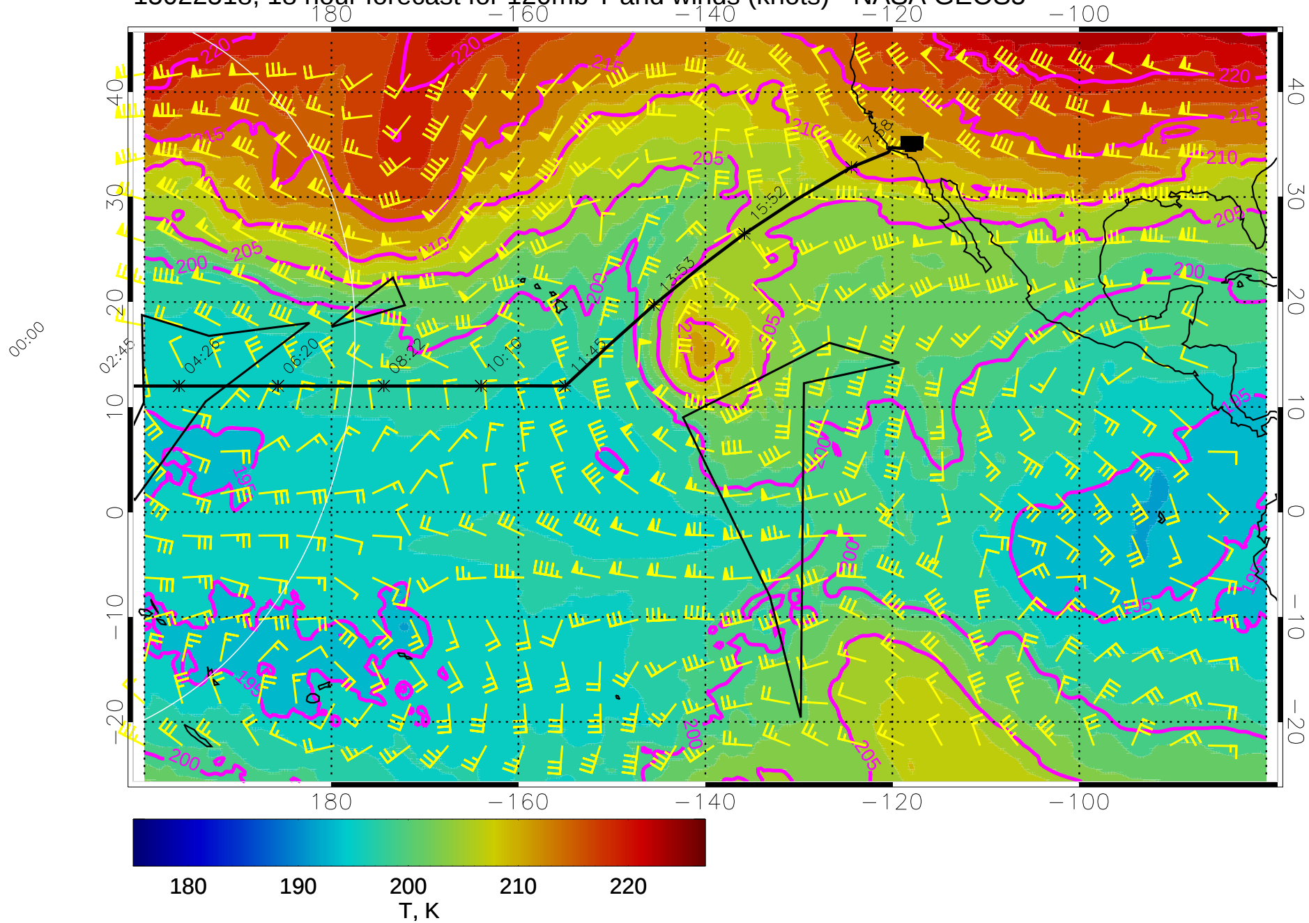
15022518, 18 hour forecast for 120mb T and winds (knots) - NASA GEOS5
