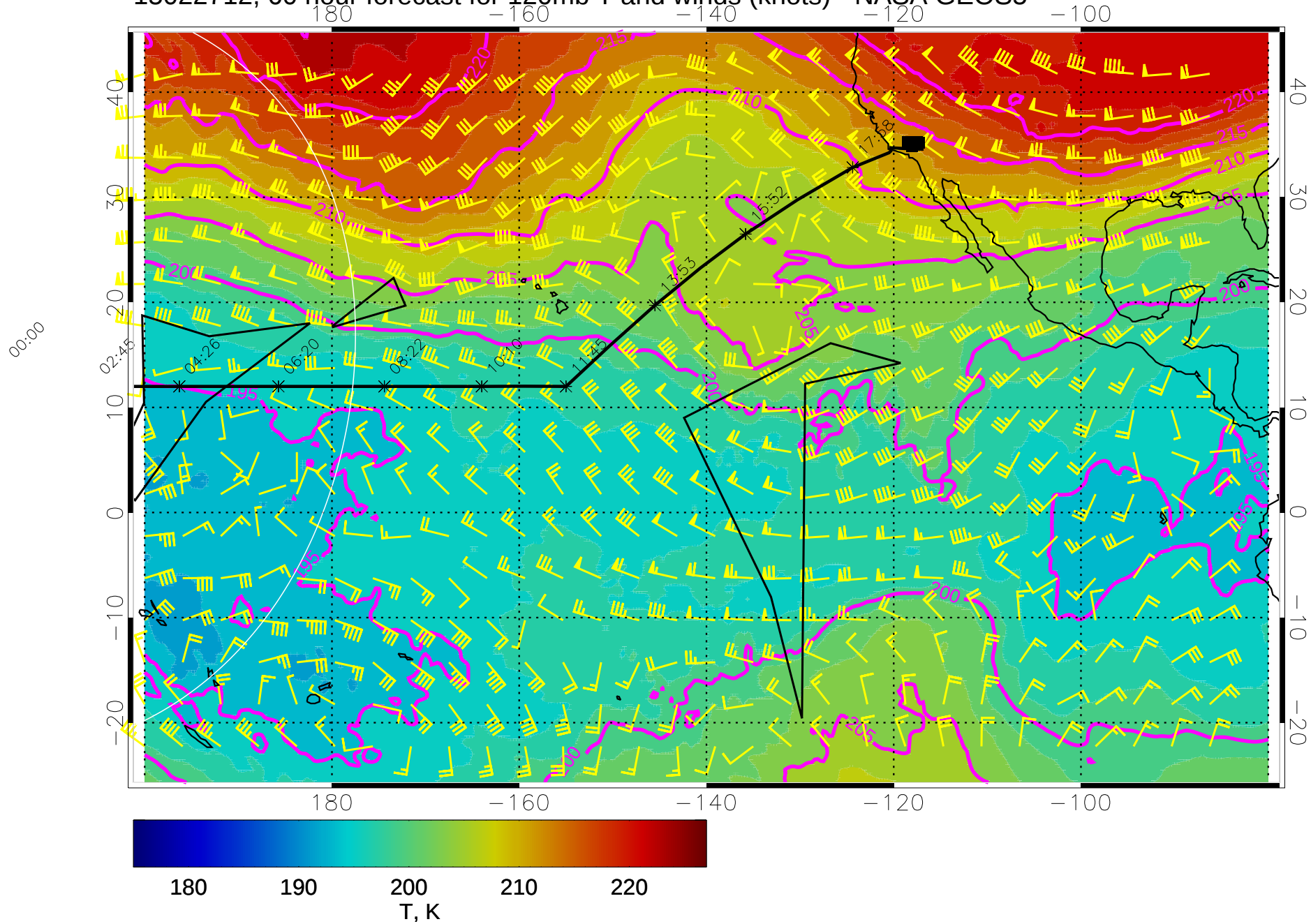
15022712, 60 hour forecast for 120mb T and winds (knots) - NASA GEOS5
