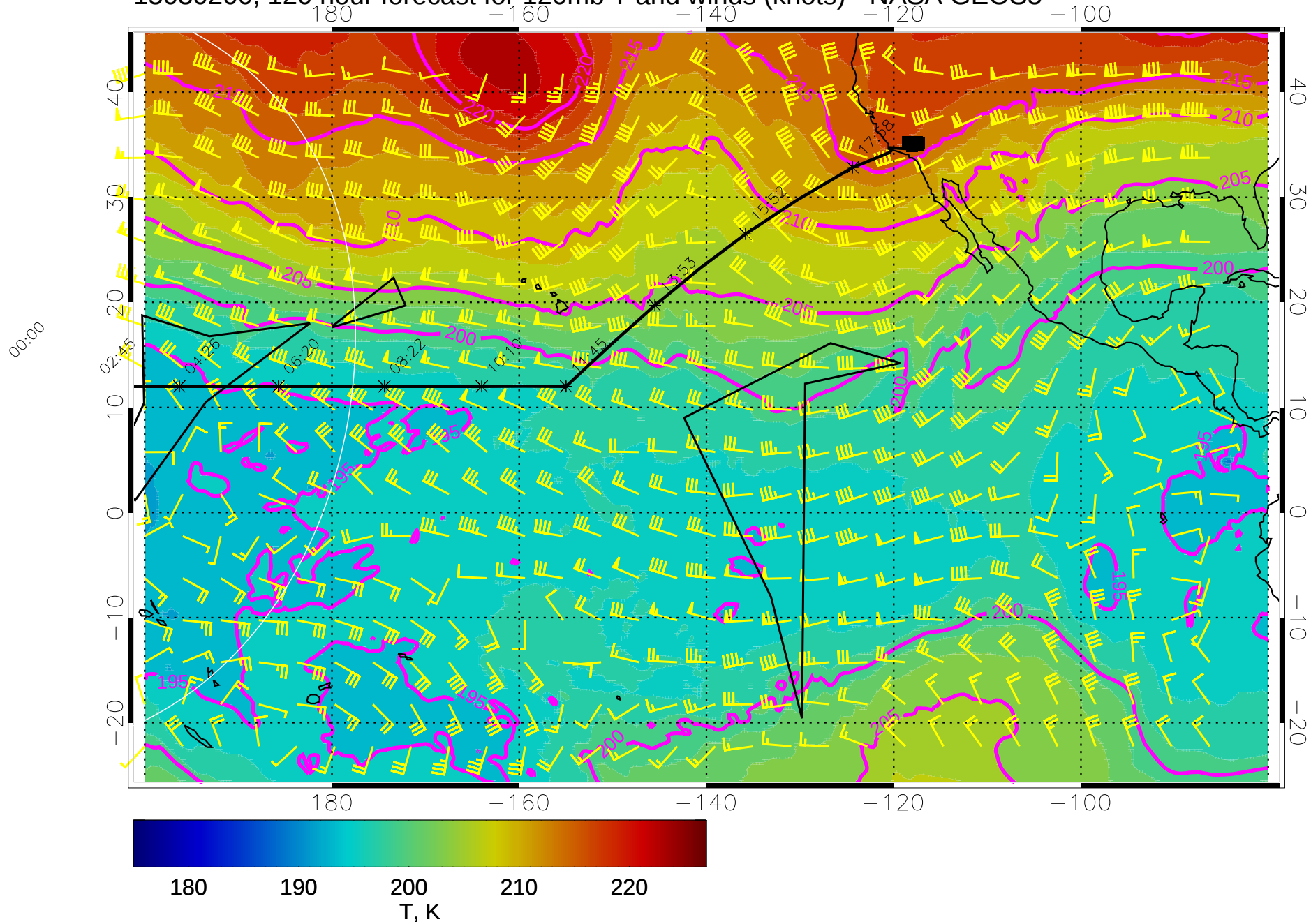
15030200, 120 hour forecast for 120mb T and winds (knots) - NASA GEOS5
