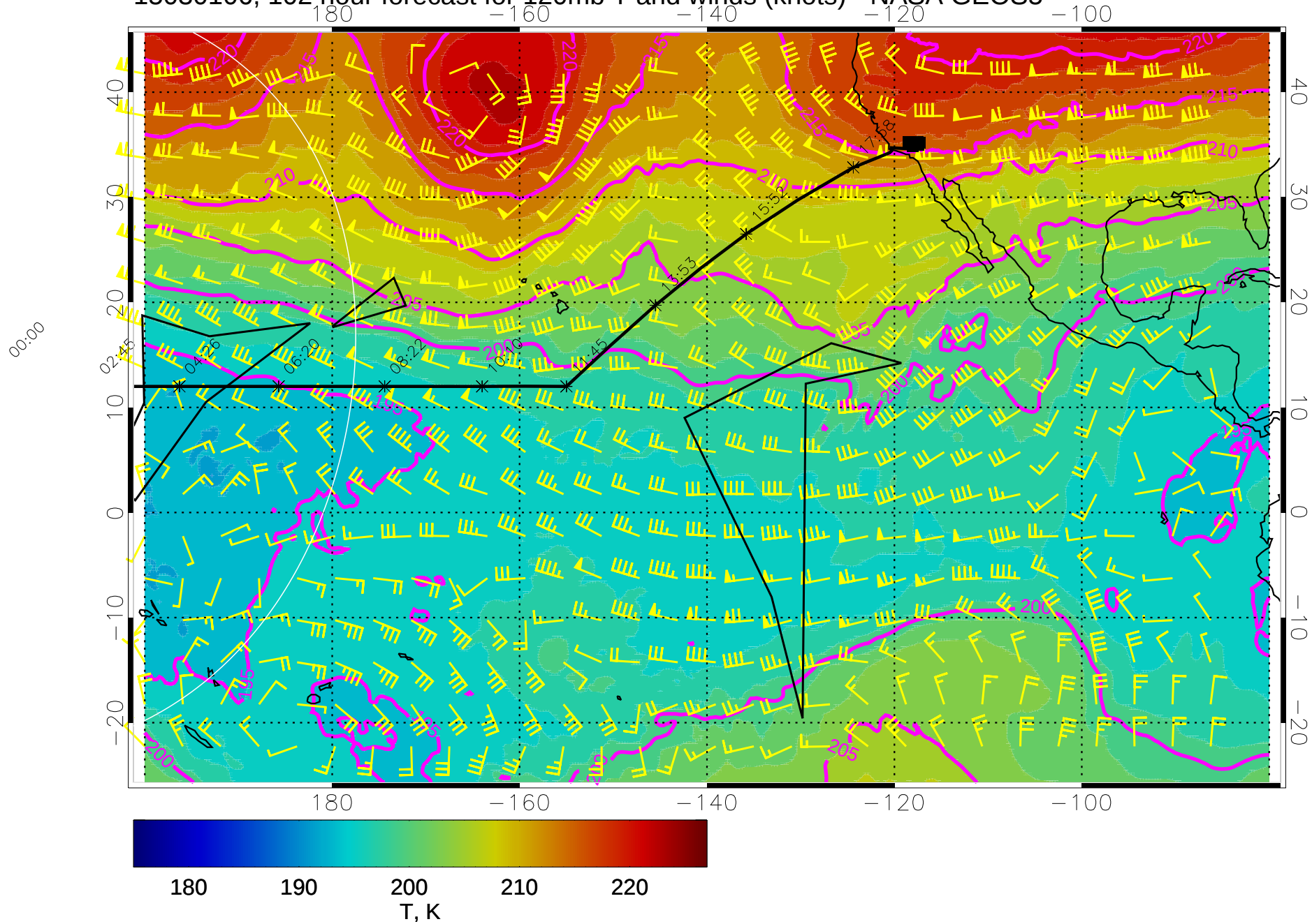
15030106, 102 hour forecast for 120mb T and winds (knots) - NASA GEOS5
