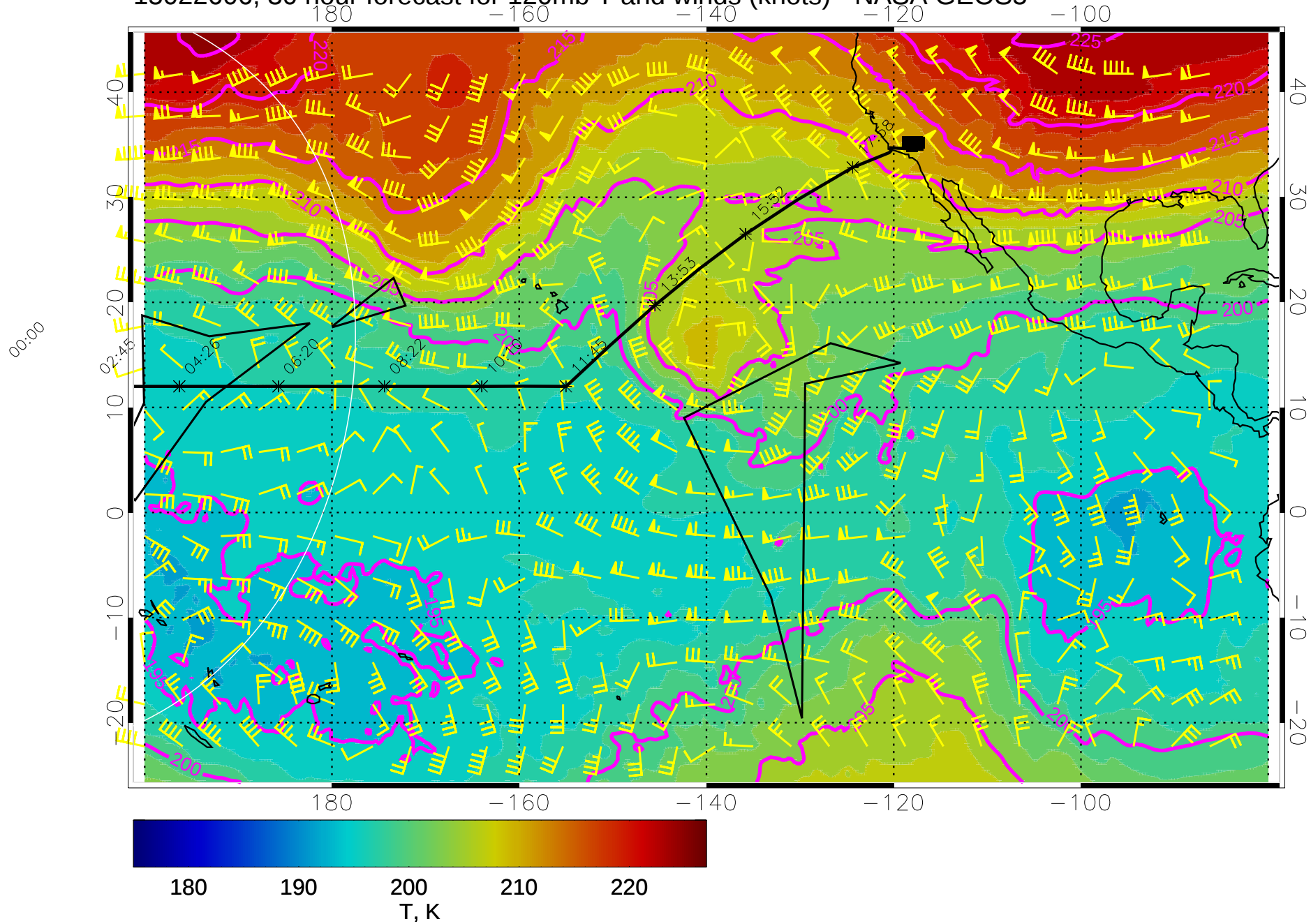
15022606, 30 hour forecast for 120mb T and winds (knots) - NASA GEOS5
