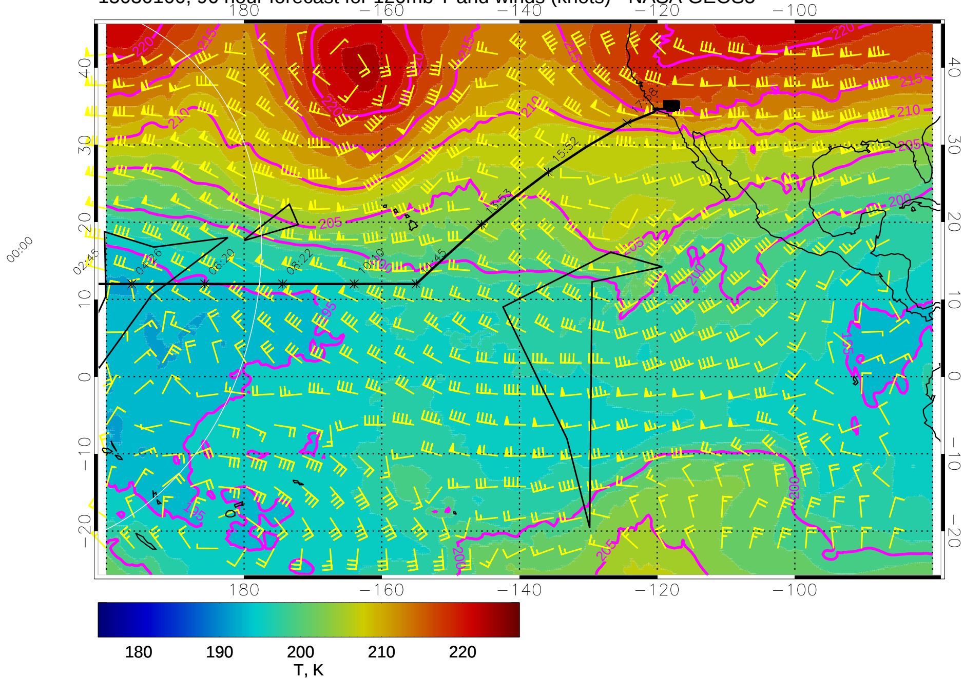
15030100, 96 hour forecast for 120mb T and winds (knots) - NASA GEOS5
