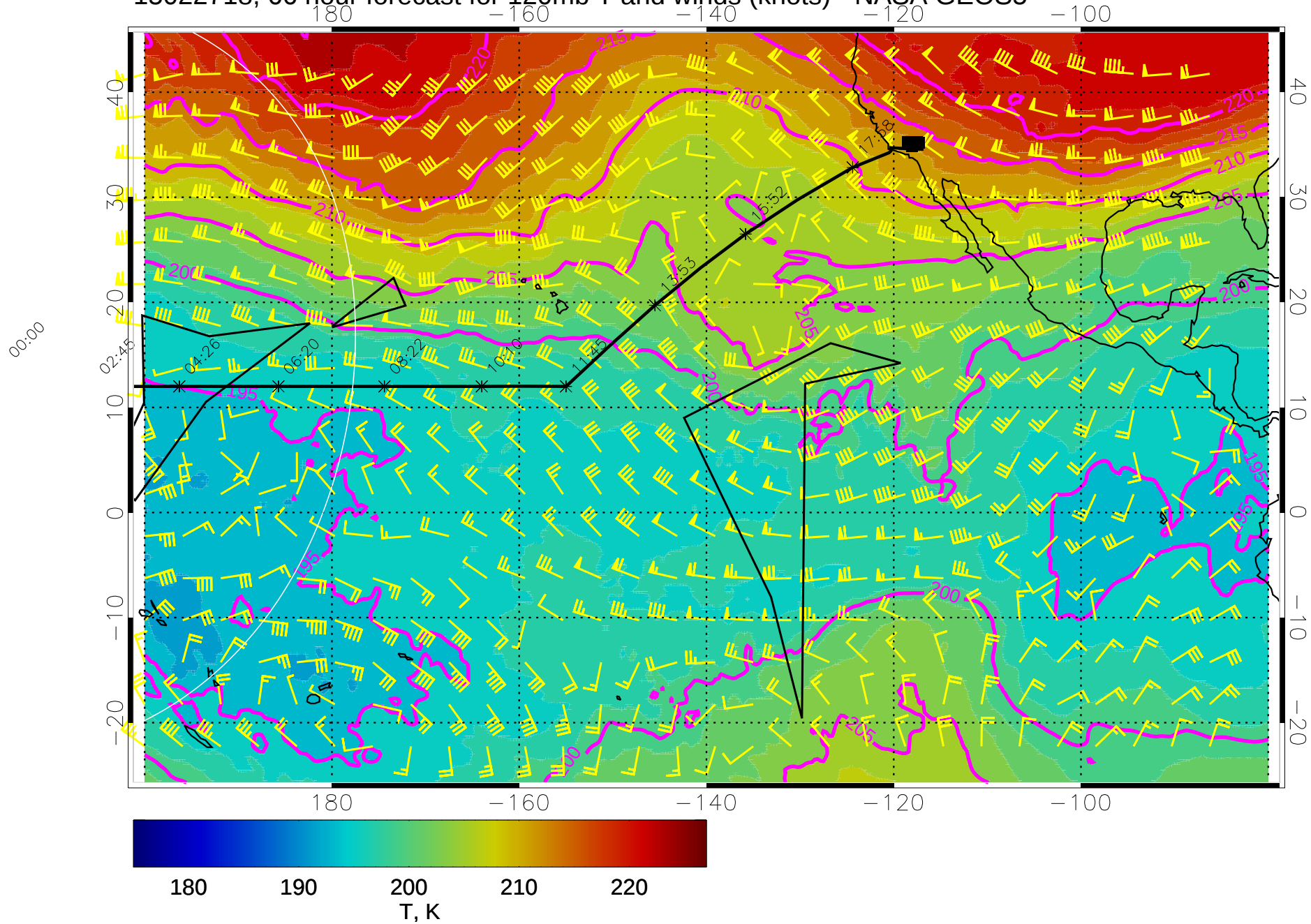
15022718, 66 hour forecast for 120mb T and winds (knots) - NASA GEOS5
