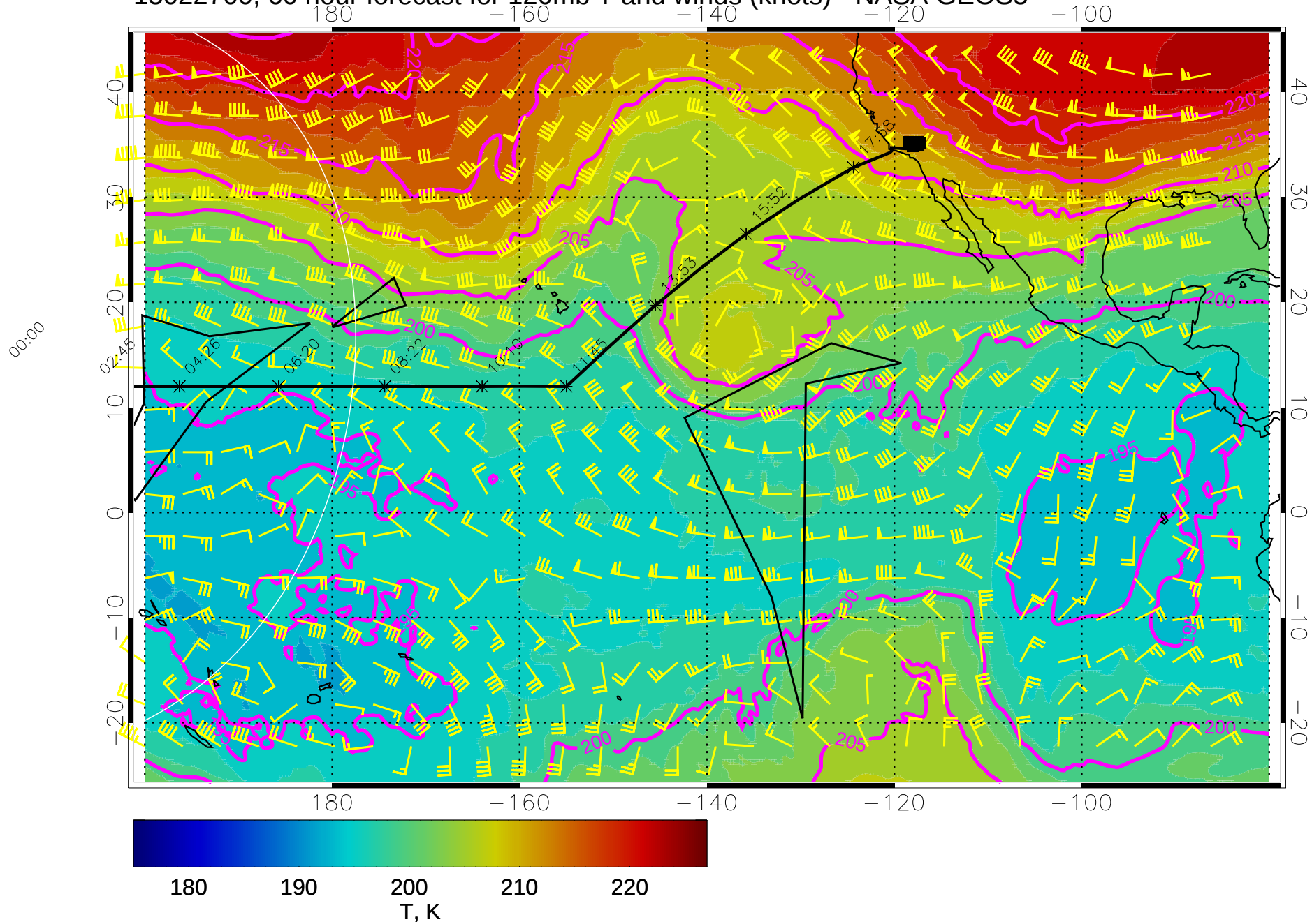
15022700, 60 hour forecast for 120mb T and winds (knots) - NASA GEOS5
