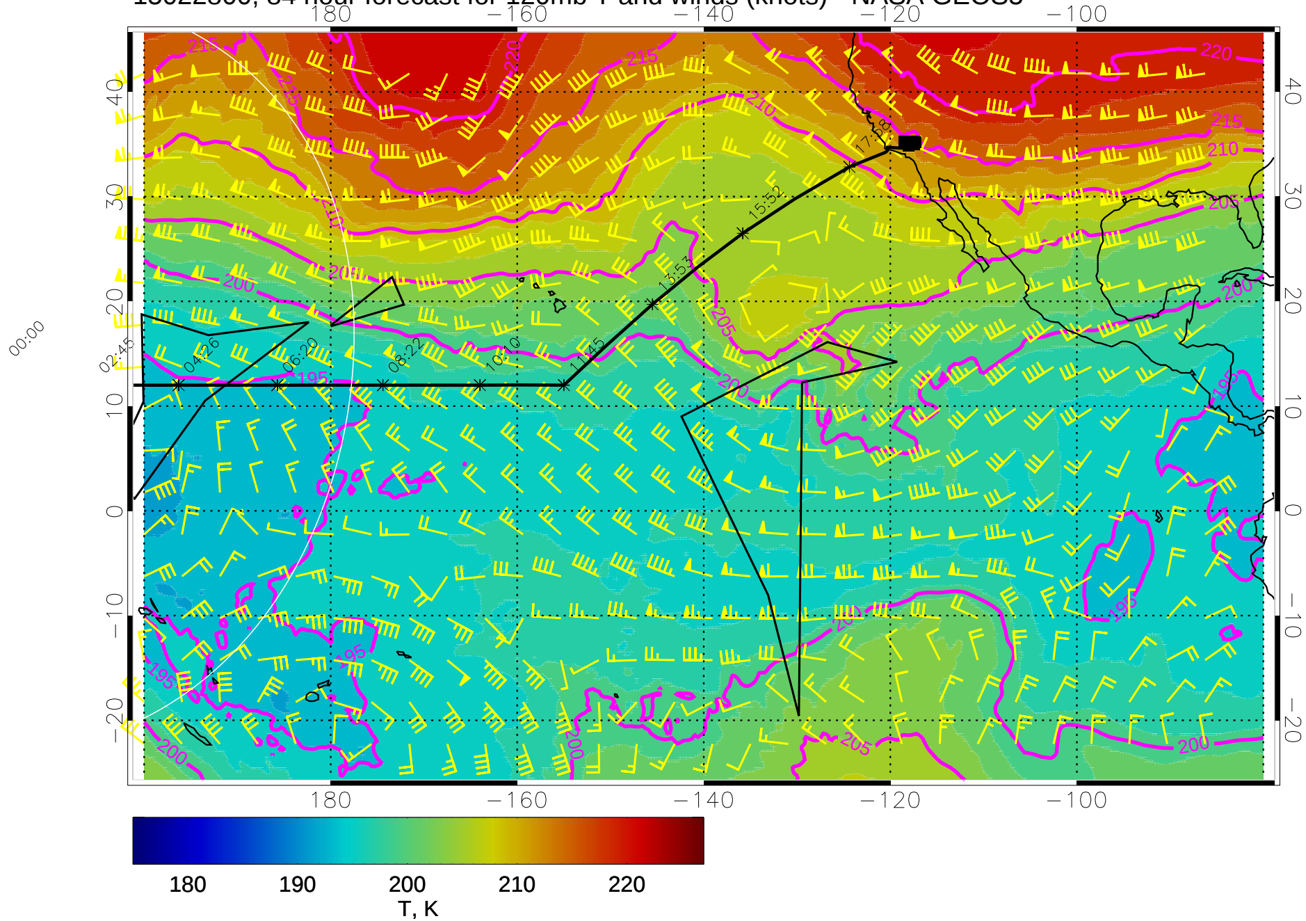
15022800, 84 hour forecast for 120mb T and winds (knots) - NASA GEOS5
