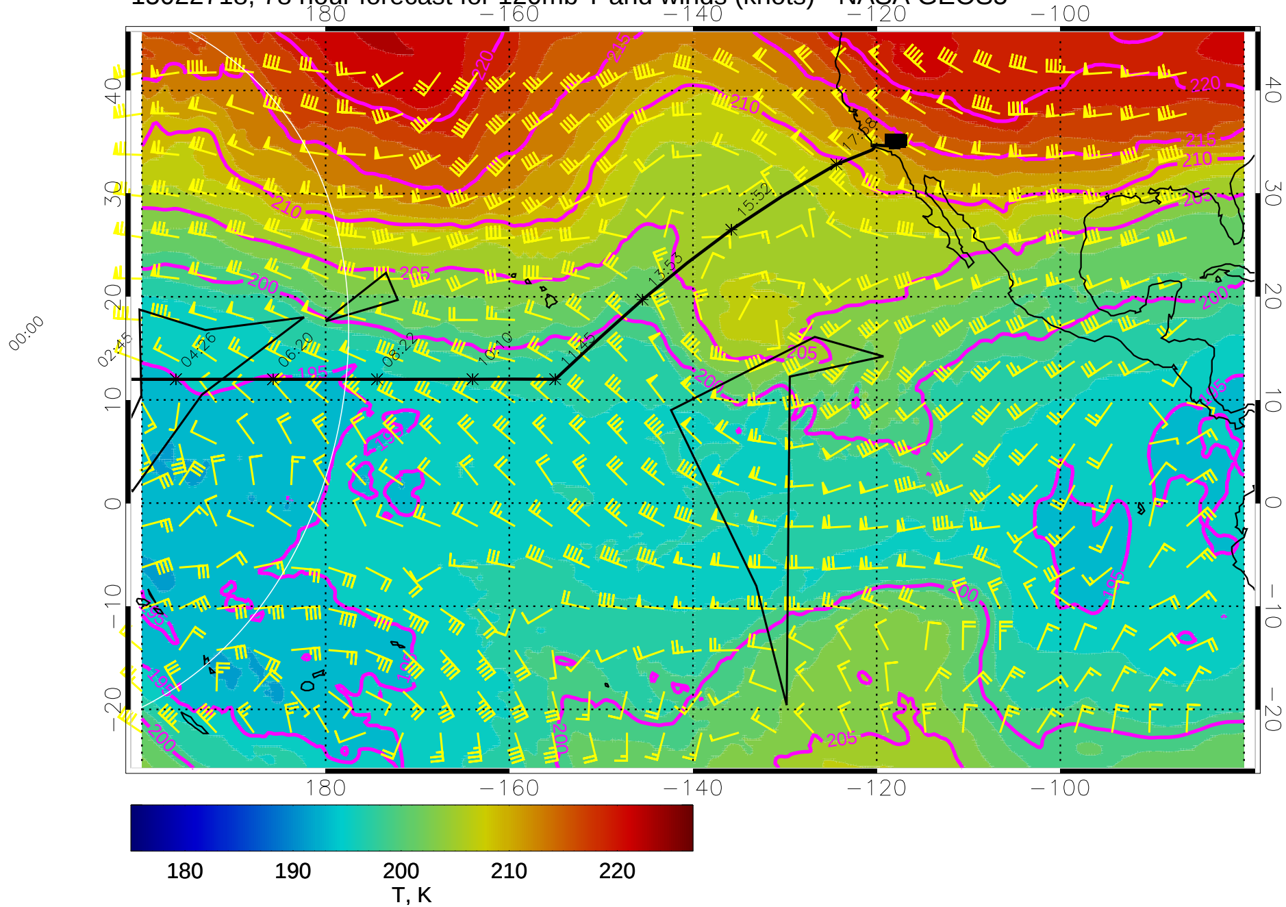
15022718, 78 hour forecast for 120mb T and winds (knots) - NASA GEOS5
