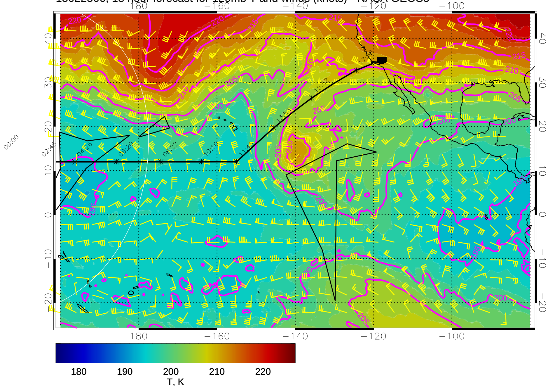
15022506, 18 hour forecast for 120mb T and winds (knots) - NASA GEOS5
