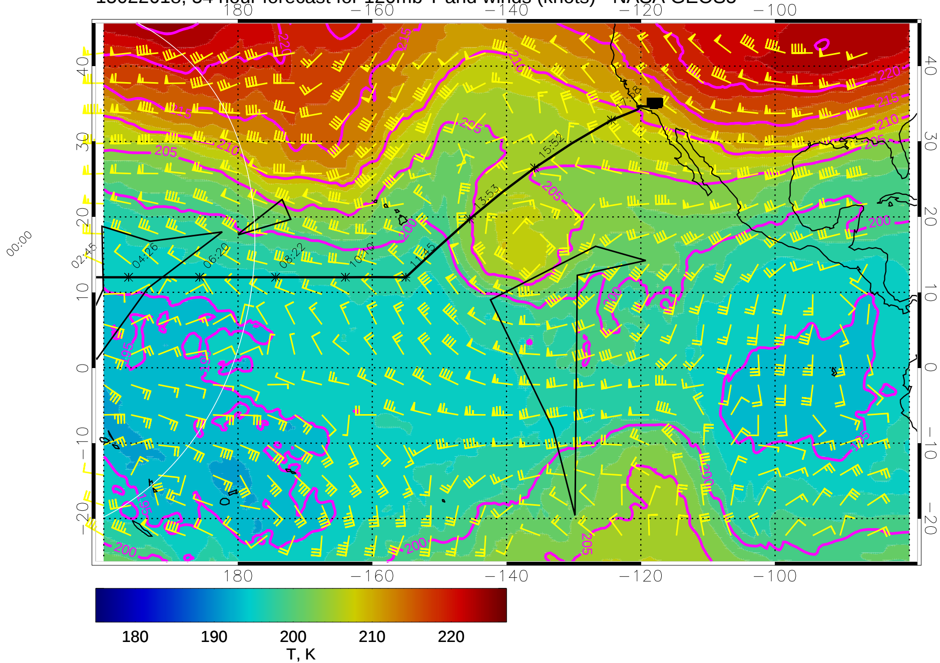
15022618, 54 hour forecast for 120mb T and winds (knots) - NASA GEOS5
