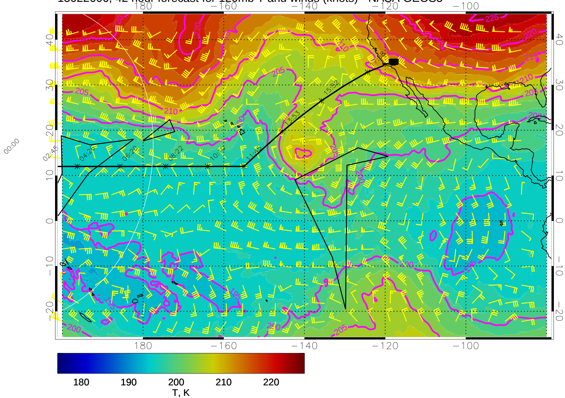
15022606, 42 hour forecast for 120mb T and winds (knots) - NASA GEOS5
