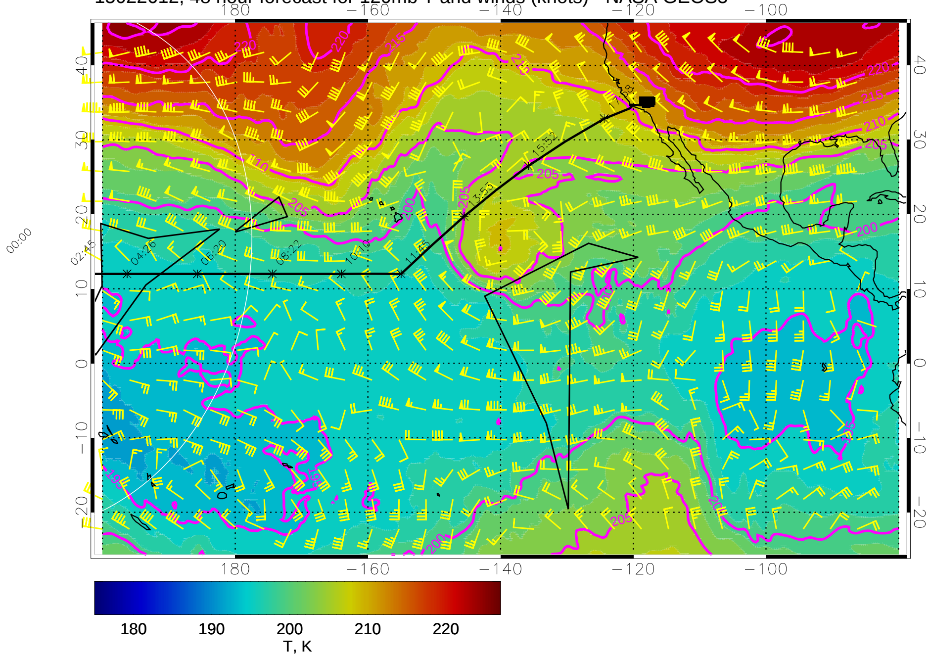
15022612, 48 hour forecast for 120mb T and winds (knots) - NASA GEOS5
