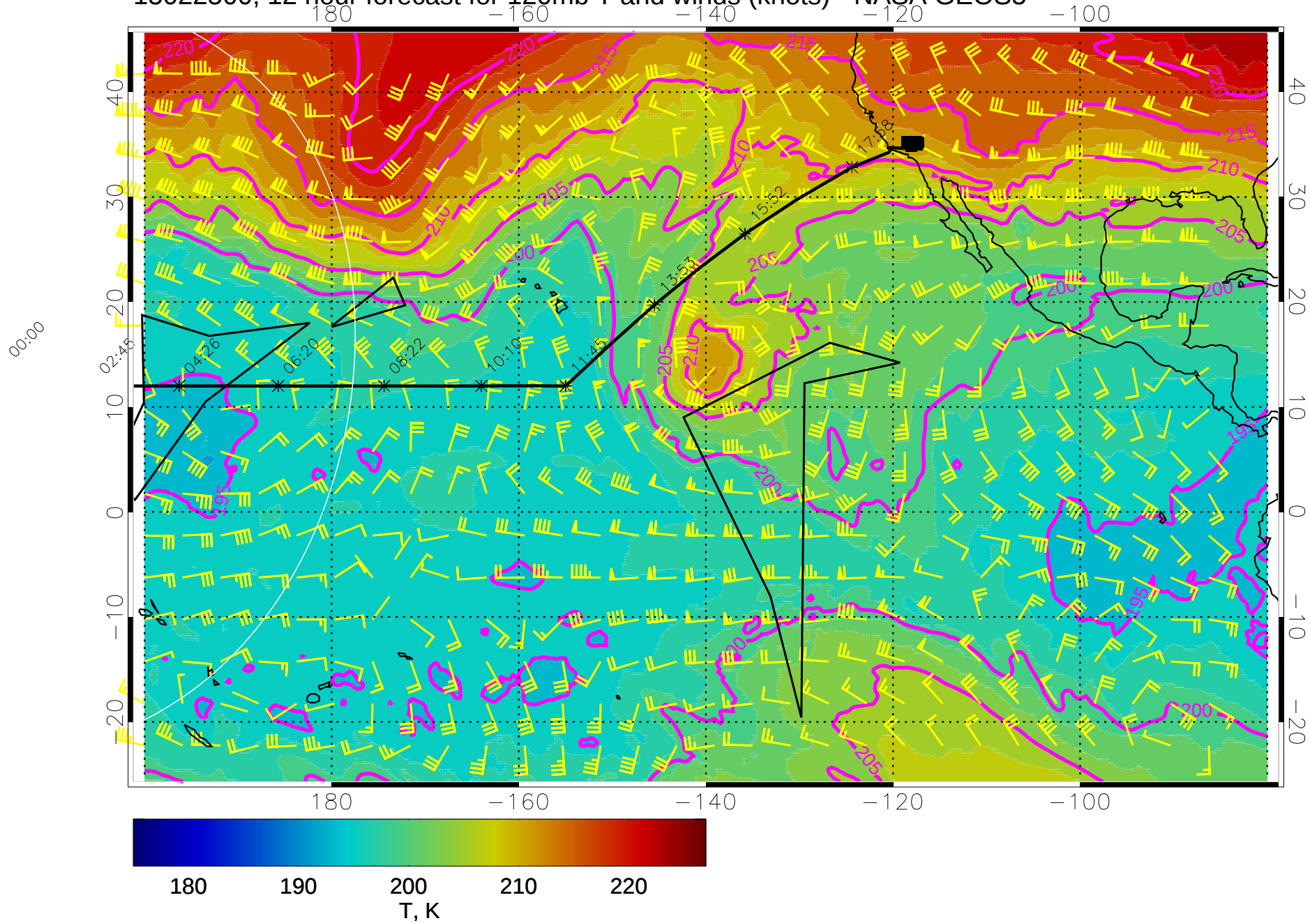
15022500, 12 hour forecast for 120mb T and winds (knots) - NASA GEOS5
