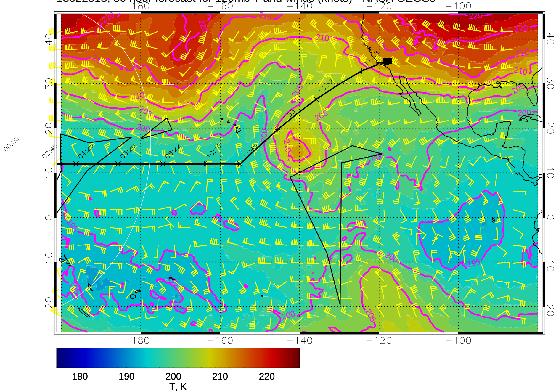
15022518, 30 hour forecast for 120mb T and winds (knots) - NASA GEOS5
