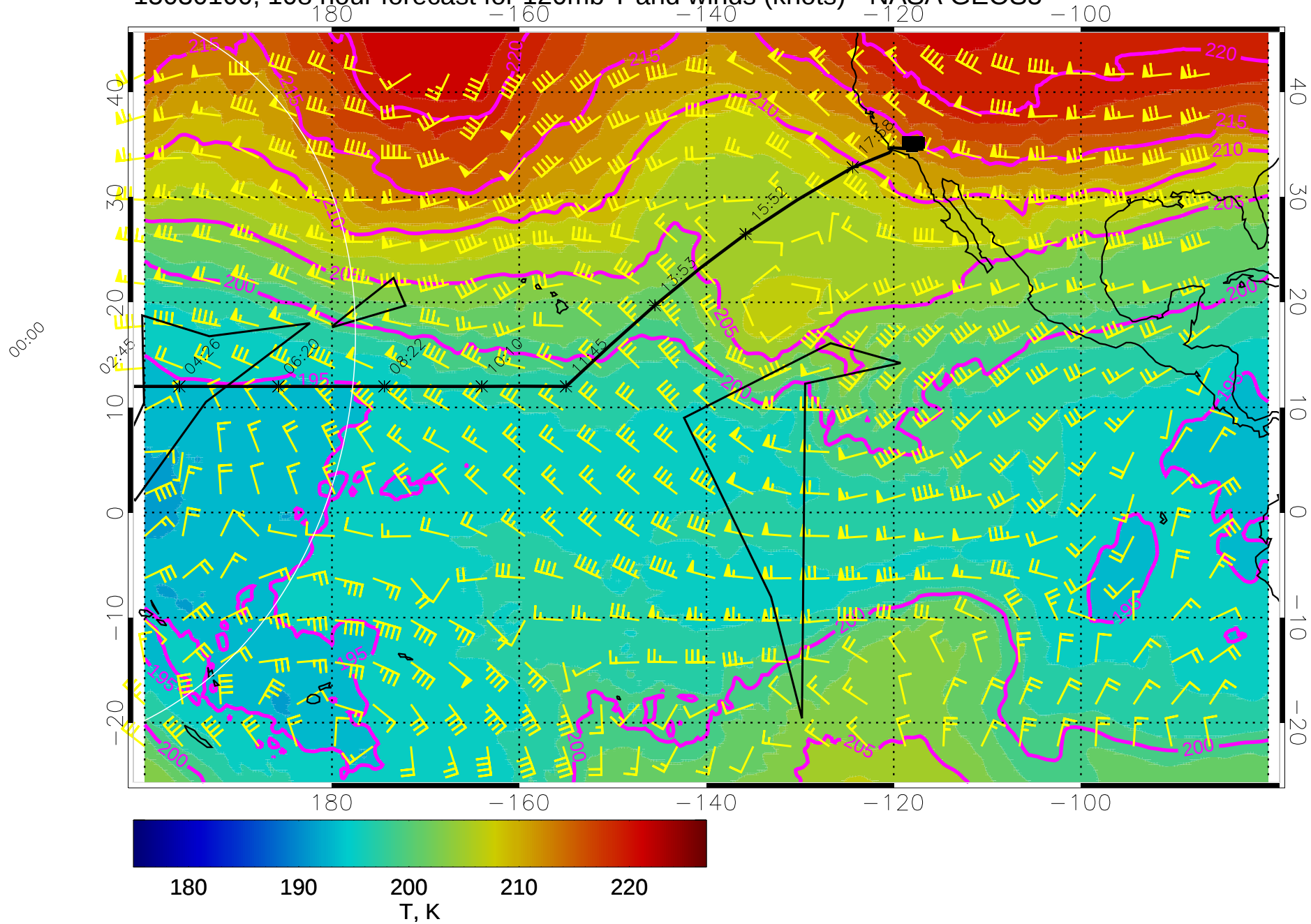
15030100, 108 hour forecast for 120mb T and winds (knots) - NASA GEOS5
