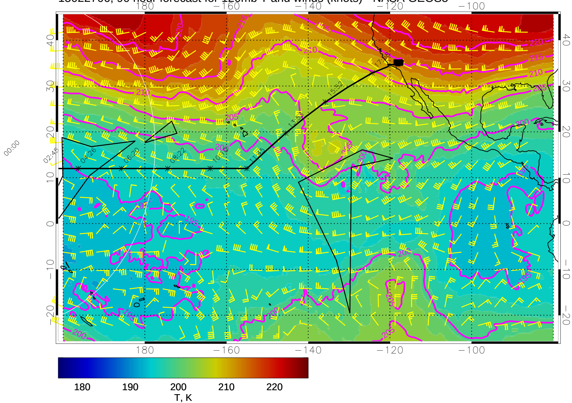
15022706, 90 hour forecast for 120mb T and winds (knots) - NASA GEOS5
