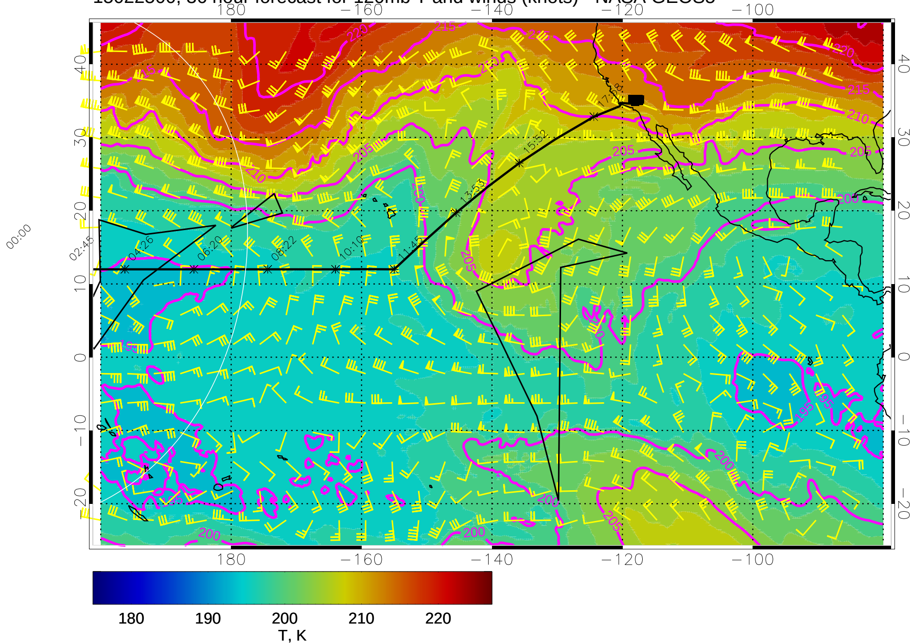
15022500, 36 hour forecast for 120mb T and winds (knots) - NASA GEOS5
