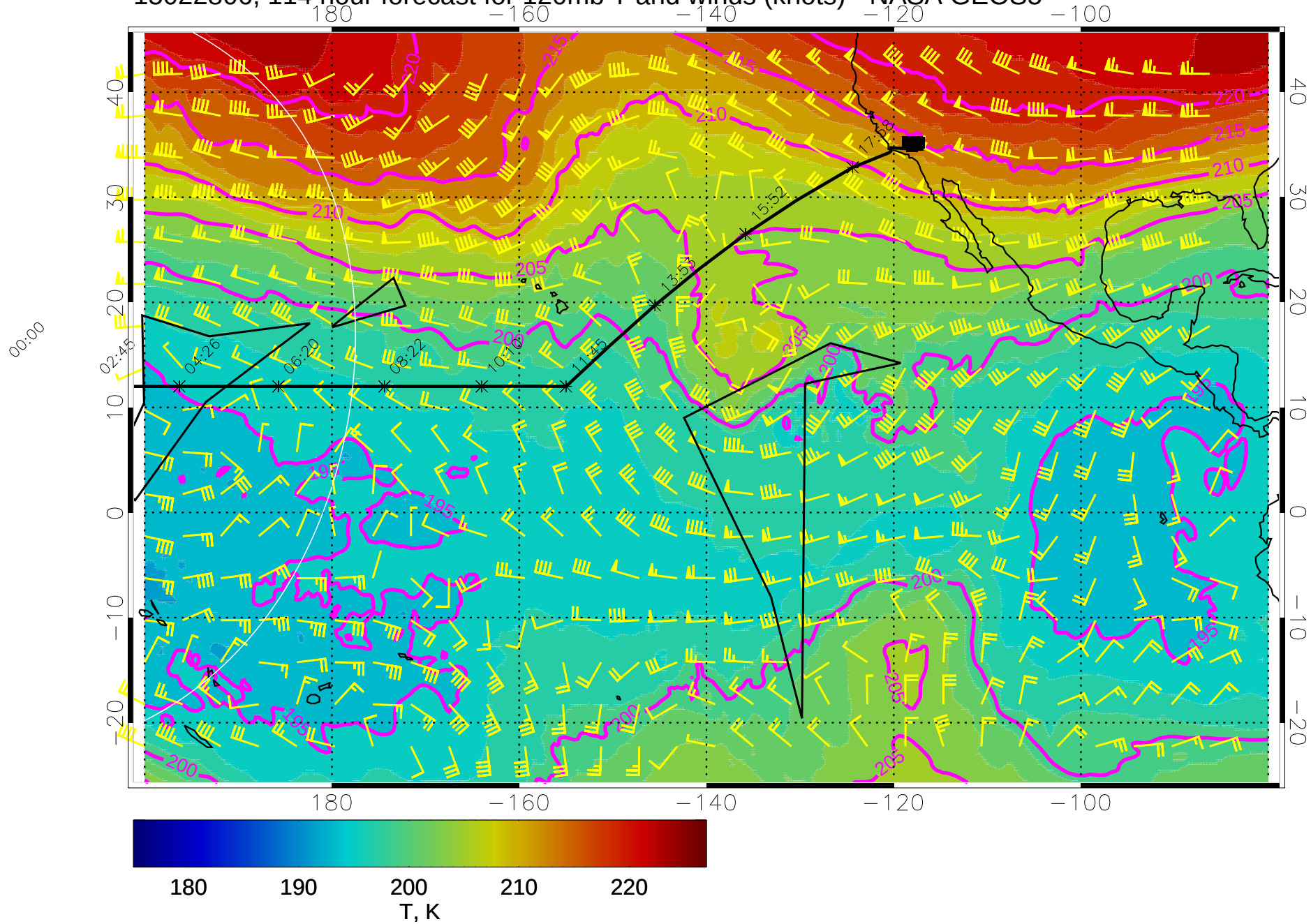
15022806, 114 hour forecast for 120mb T and winds (knots) - NASA GEOS5
