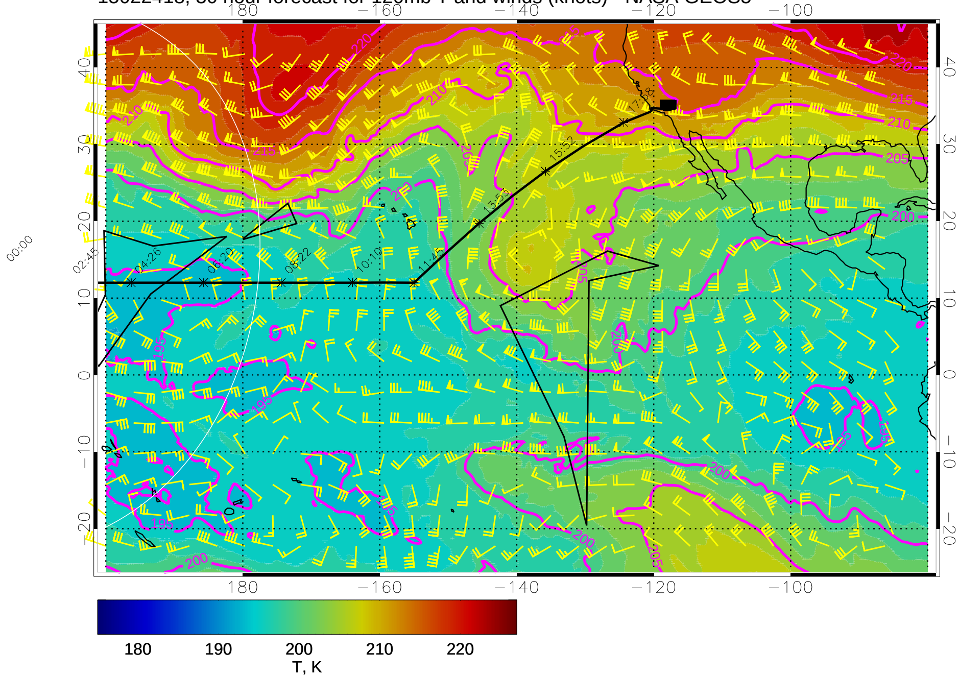
15022418, 30 hour forecast for 120mb T and winds (knots) - NASA GEOS5
