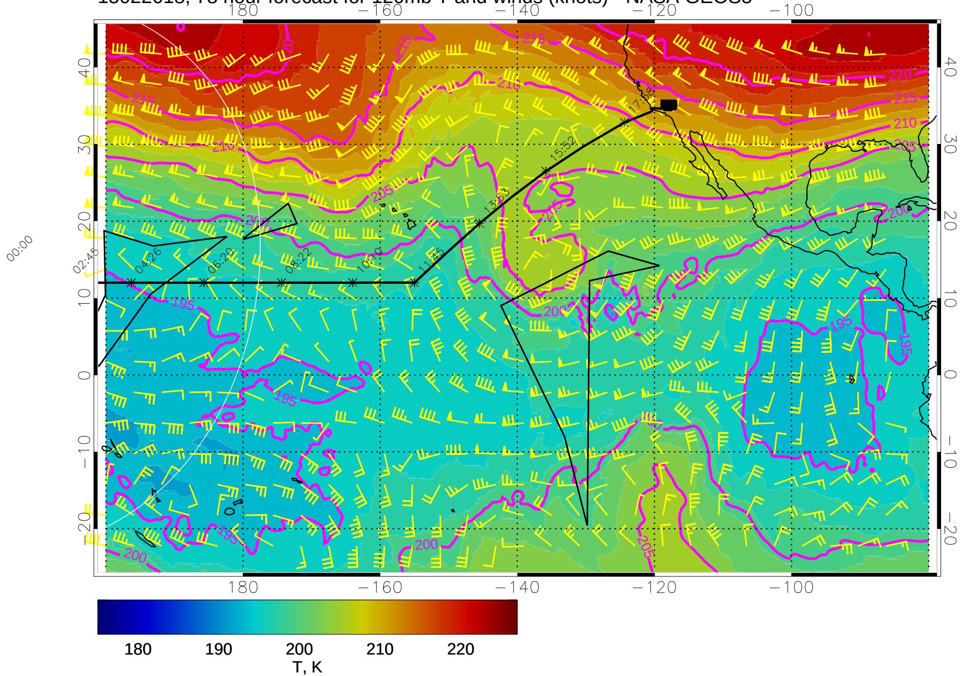
15022618, 78 hour forecast for 120mb T and winds (knots) - NASA GEOS5
