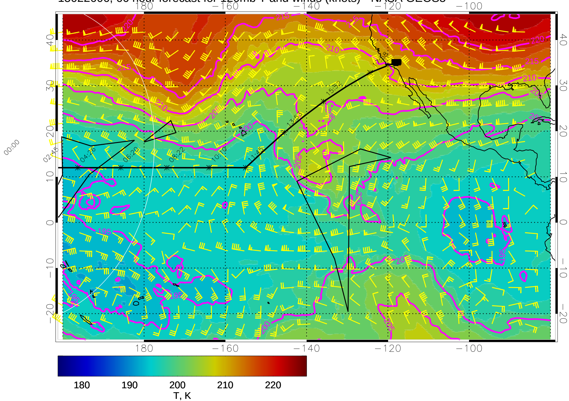
15022606, 66 hour forecast for 120mb T and winds (knots) - NASA GEOS5
