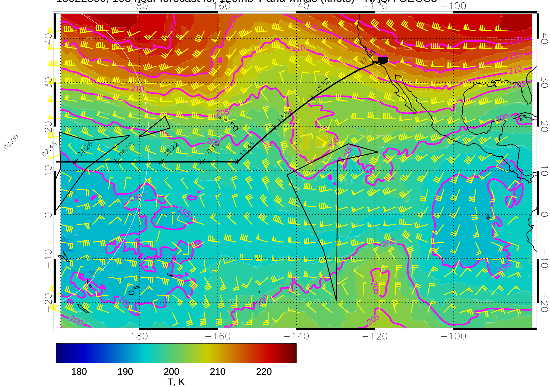
15022800, 108 hour forecast for 120mb T and winds (knots) - NASA GEOS5
