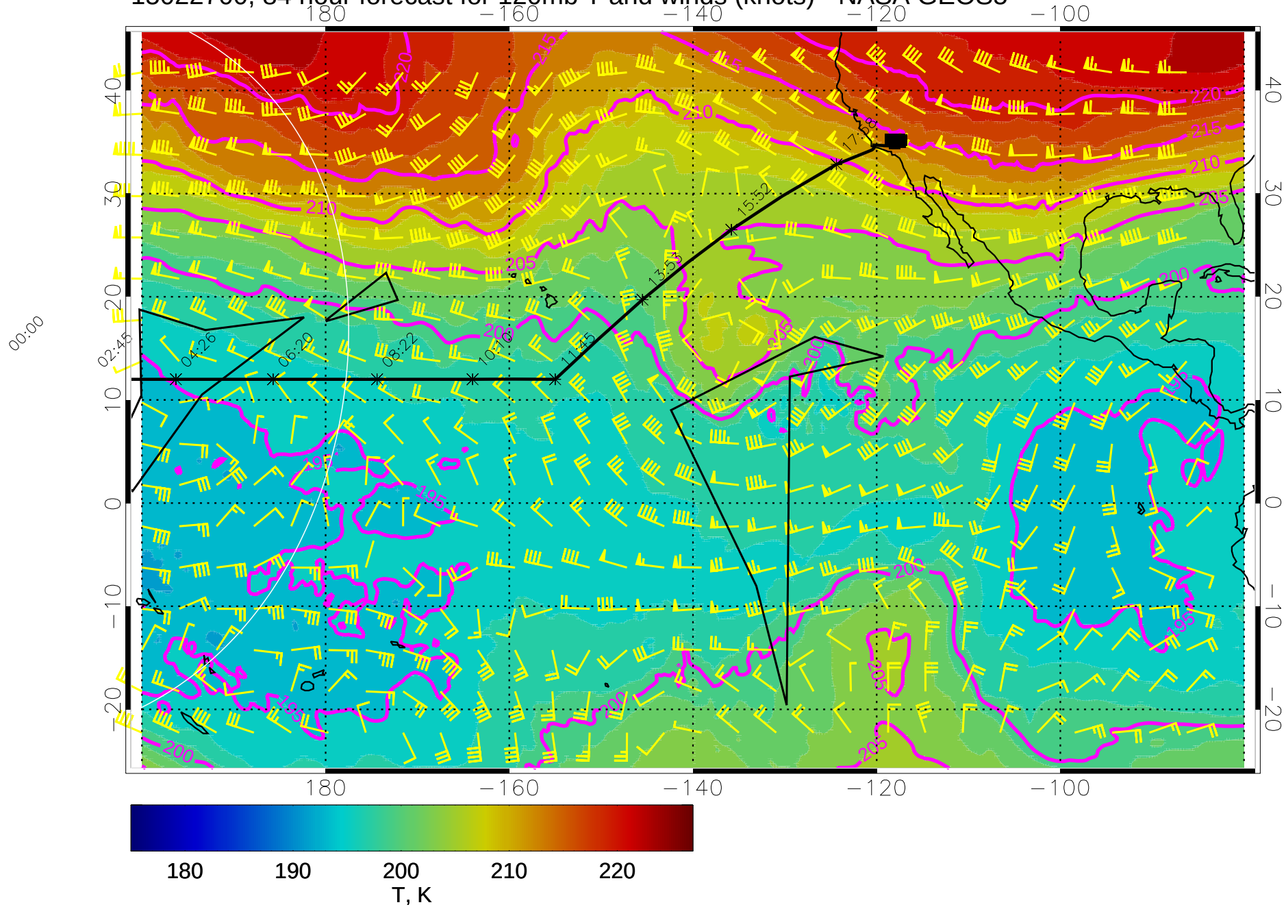
15022700, 84 hour forecast for 120mb T and winds (knots) - NASA GEOS5
