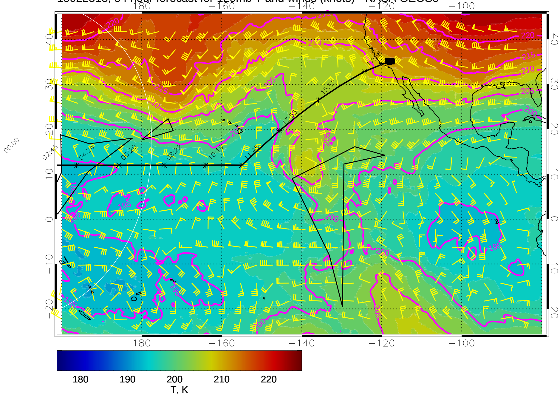
15022518, 54 hour forecast for 120mb T and winds (knots) - NASA GEOS5
