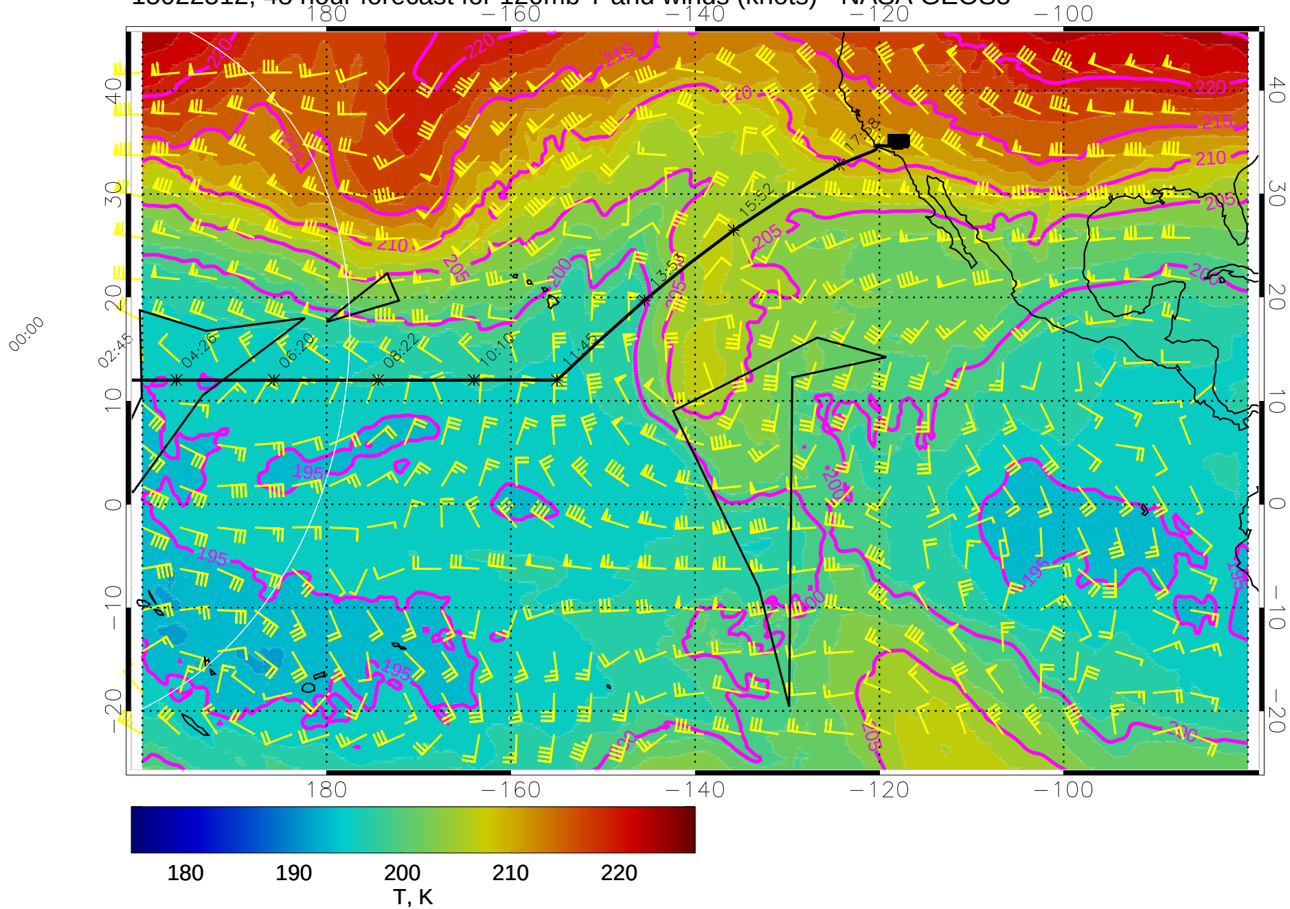
15022512, 48 hour forecast for 120mb T and winds (knots) - NASA GEOS5
