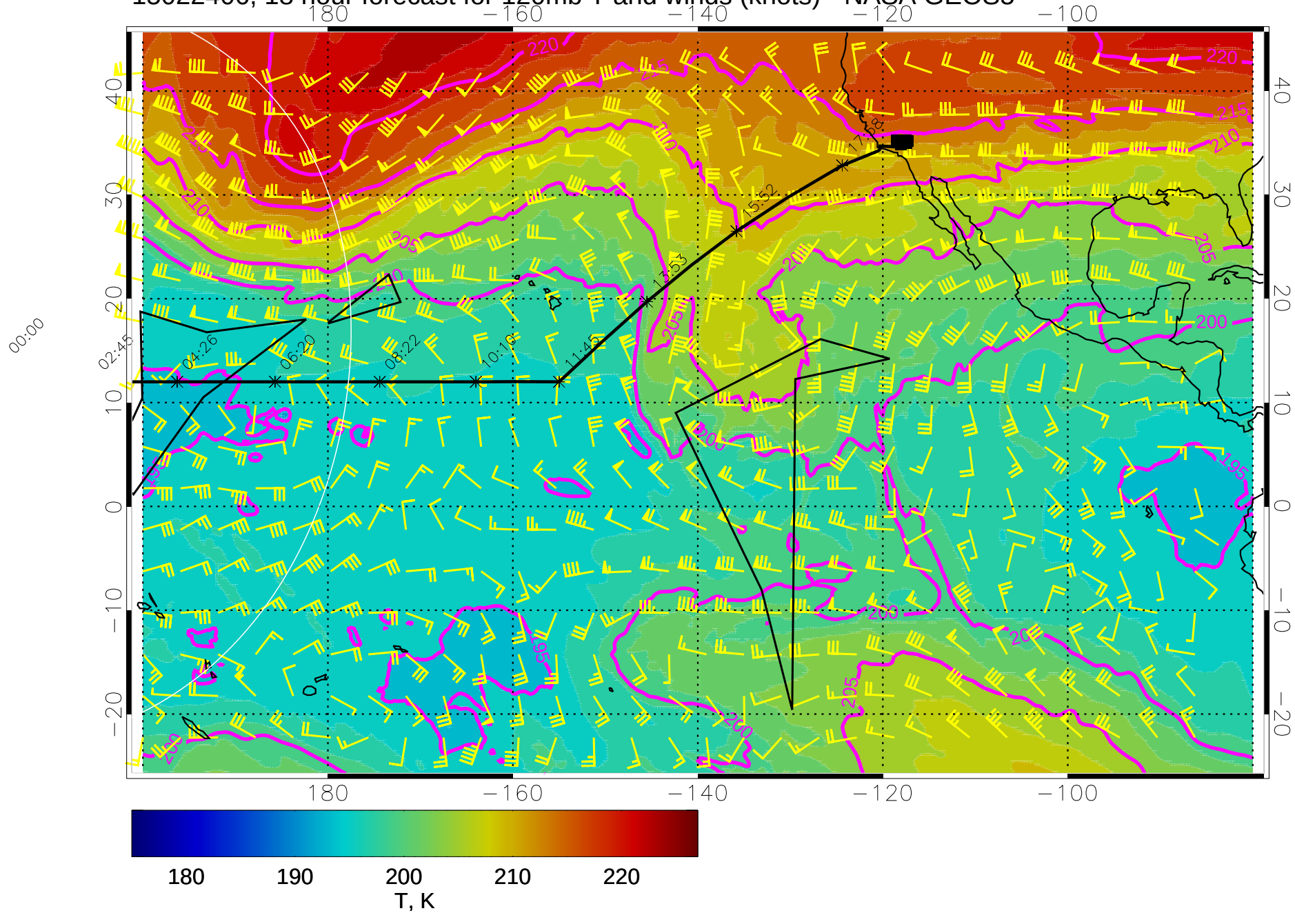
15022406, 18 hour forecast for 120mb T and winds (knots) - NASA GEOS5
