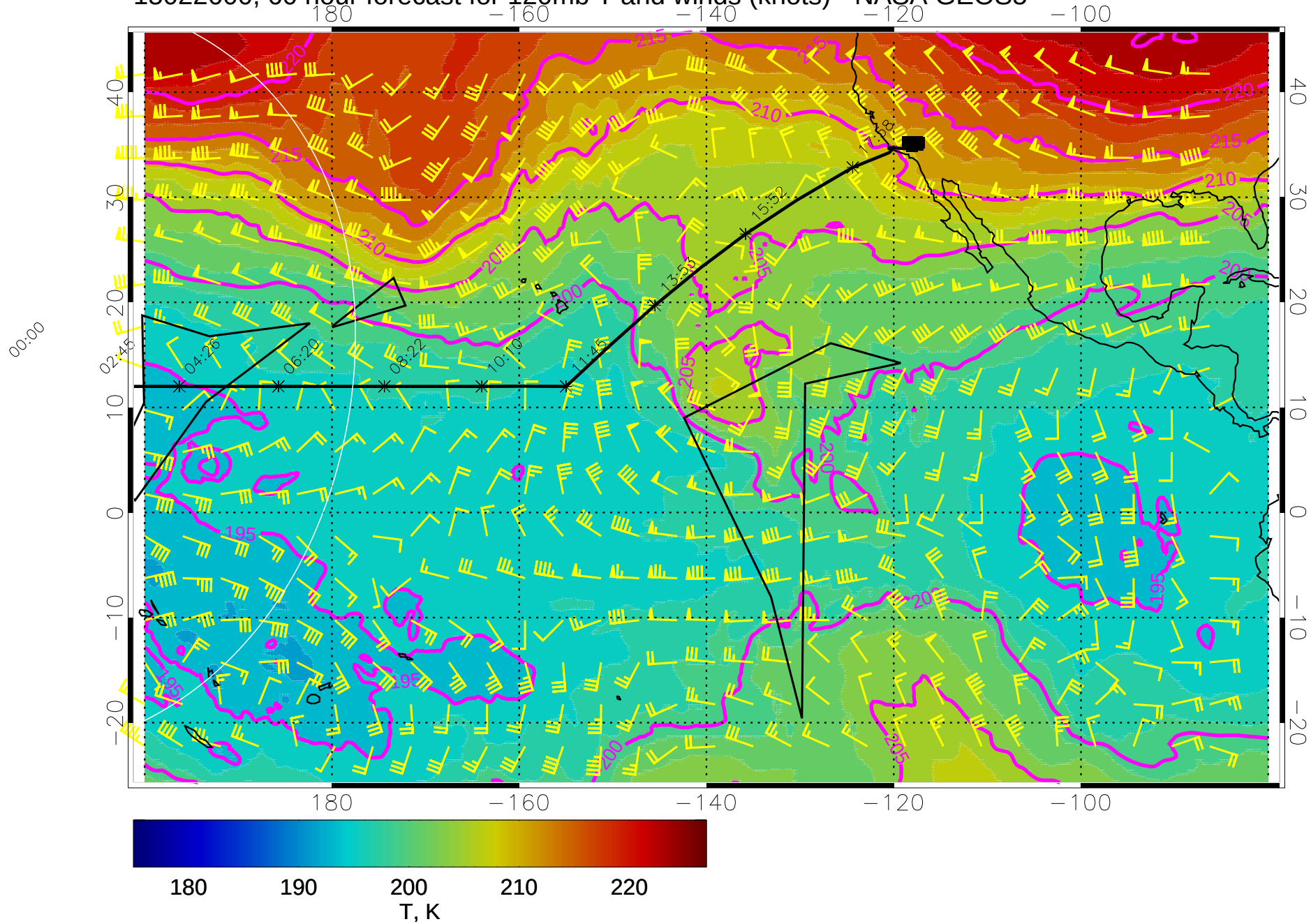
15022600, 60 hour forecast for 120mb T and winds (knots) - NASA GEOS5
