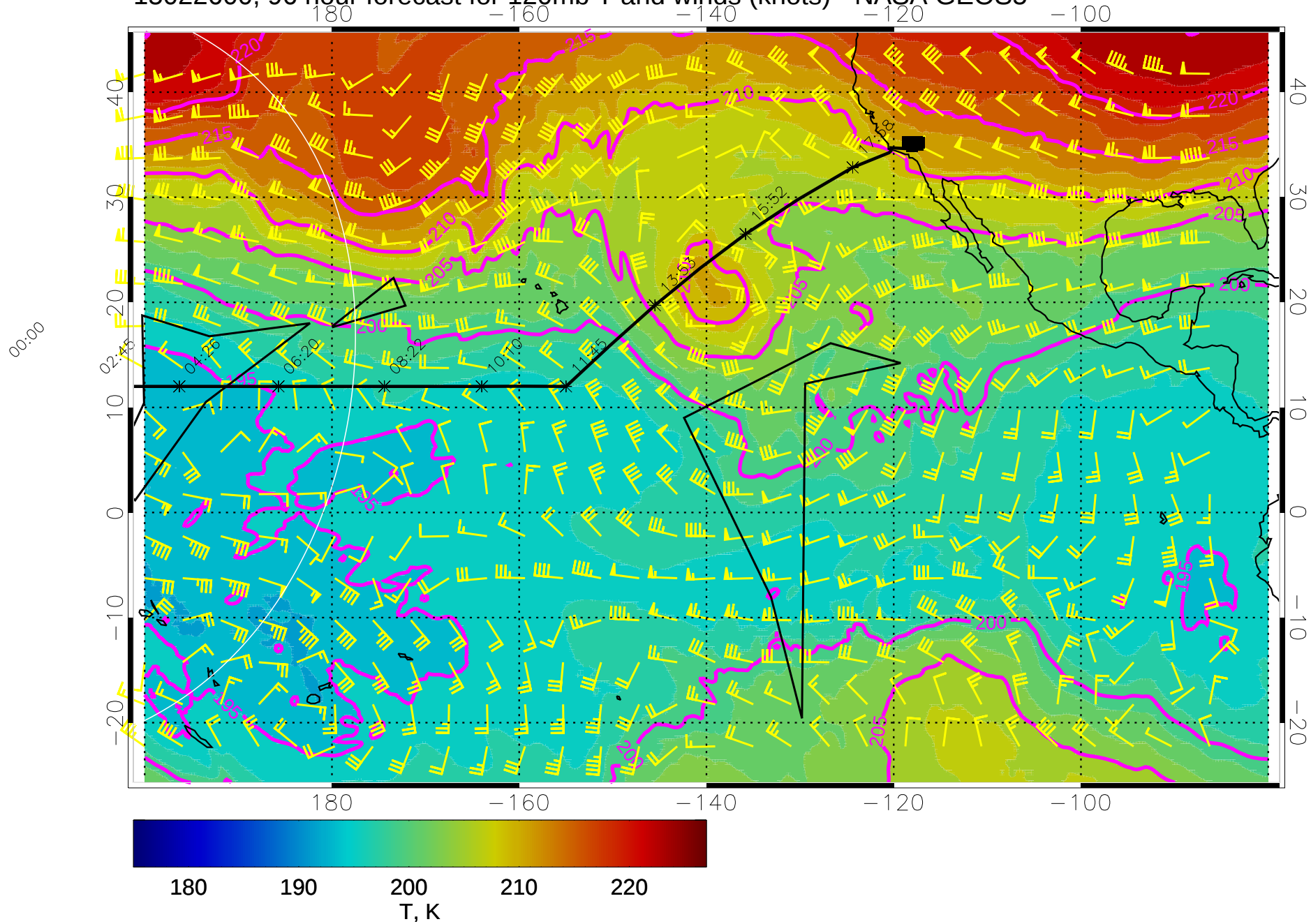
15022600, 96 hour forecast for 120mb T and winds (knots) - NASA GEOS5
