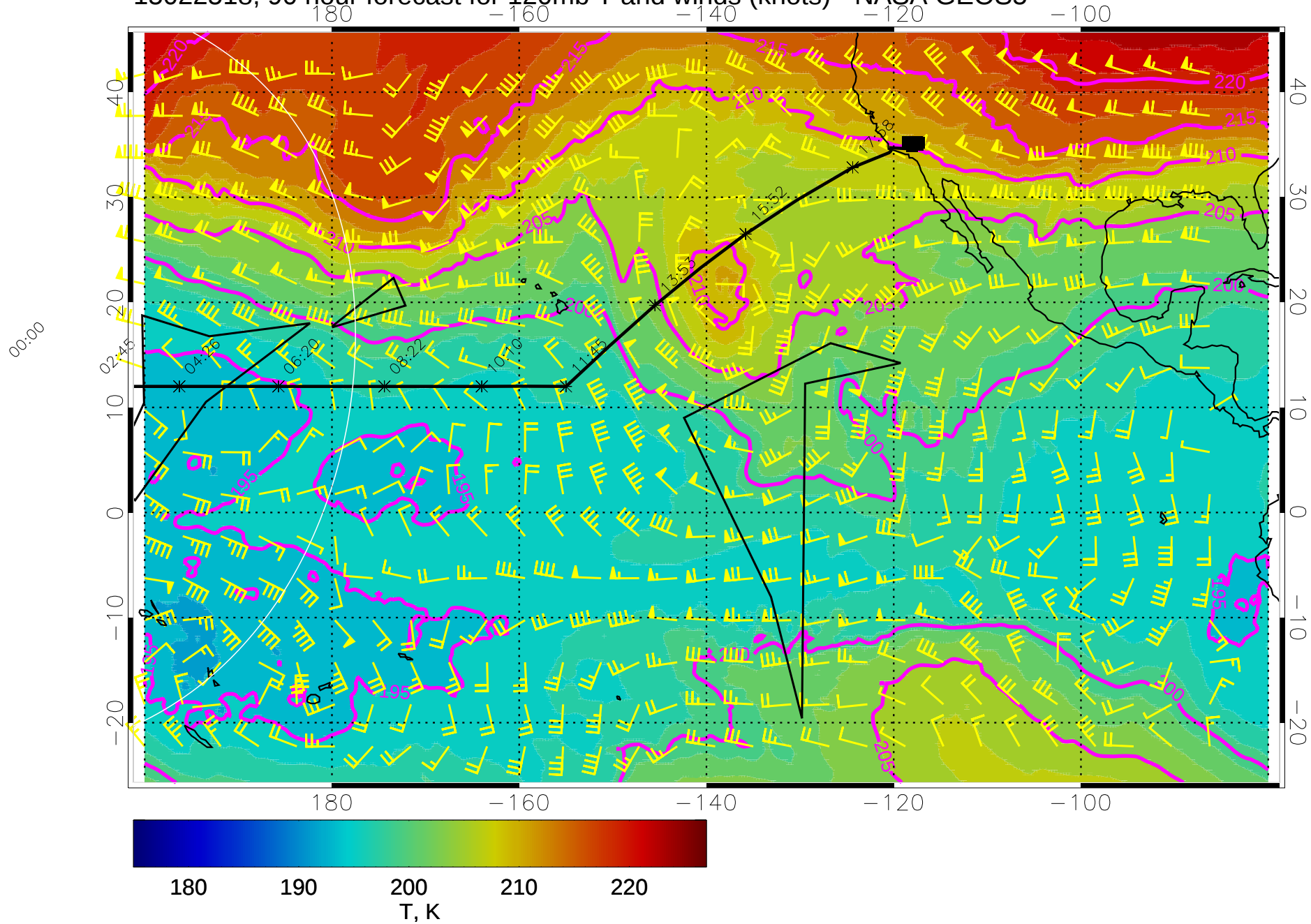
15022518, 90 hour forecast for 120mb T and winds (knots) - NASA GEOS5
