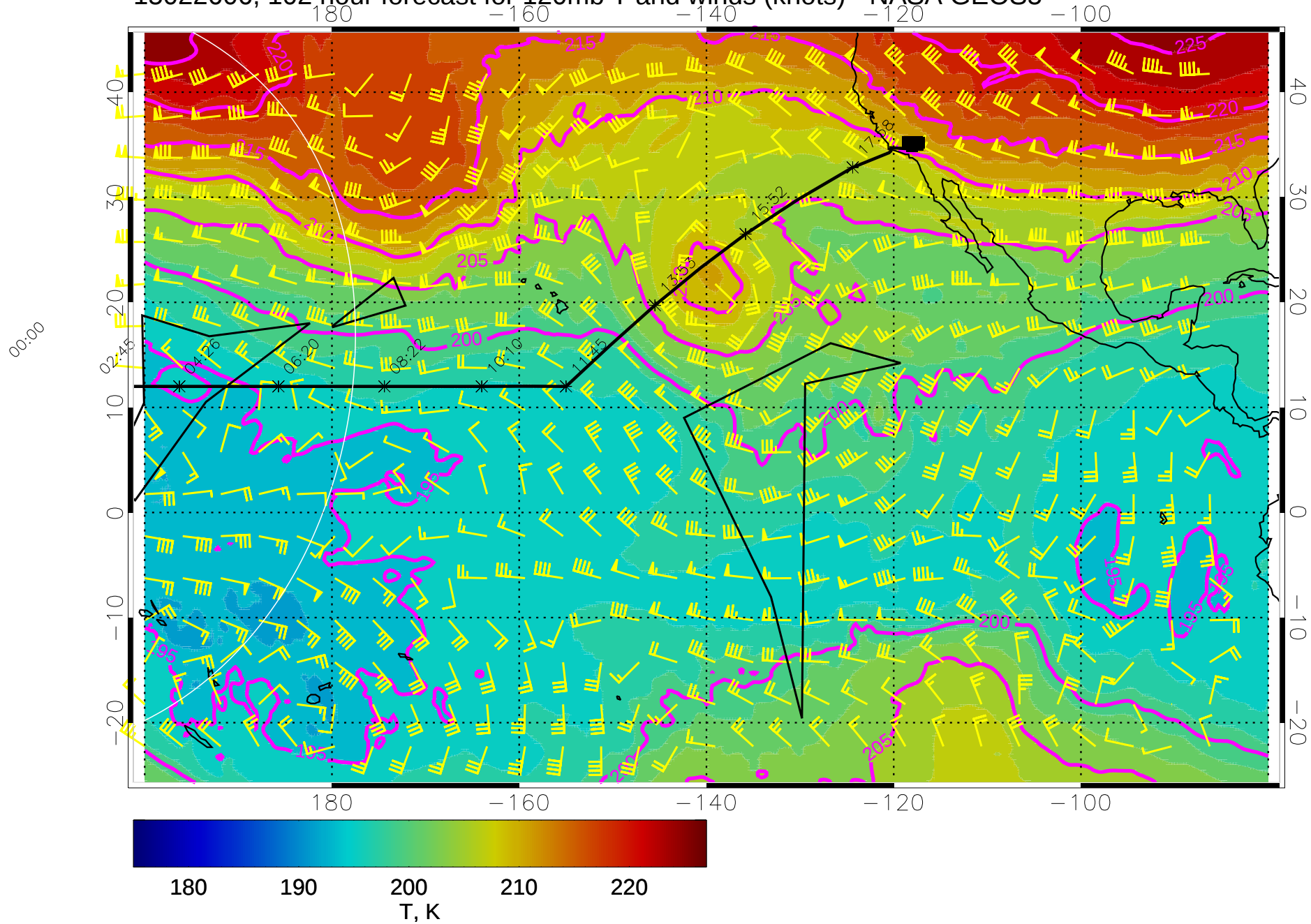
15022606, 102 hour forecast for 120mb T and winds (knots) - NASA GEOS5
