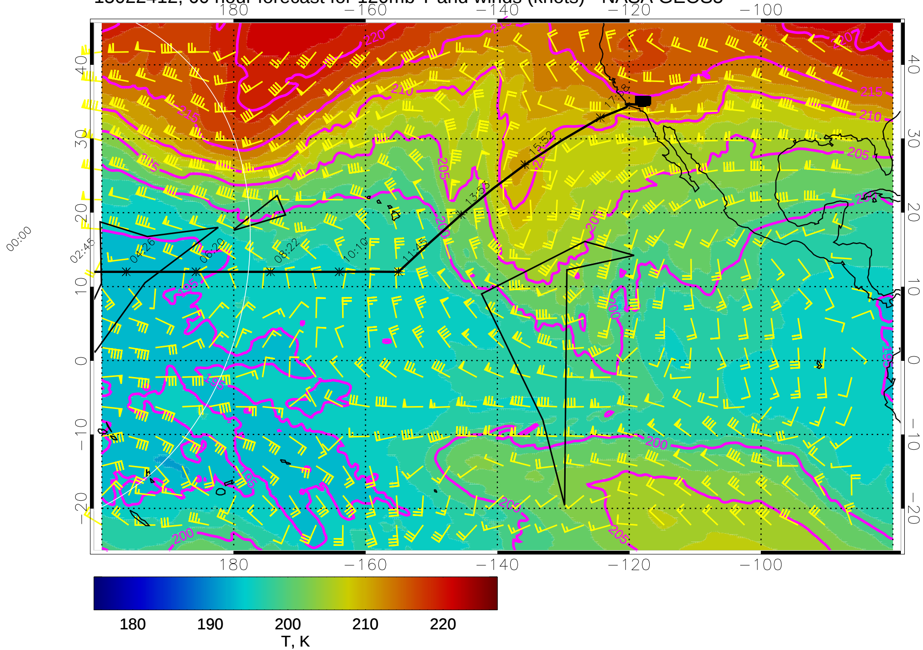
15022412, 60 hour forecast for 120mb T and winds (knots) - NASA GEOS5
