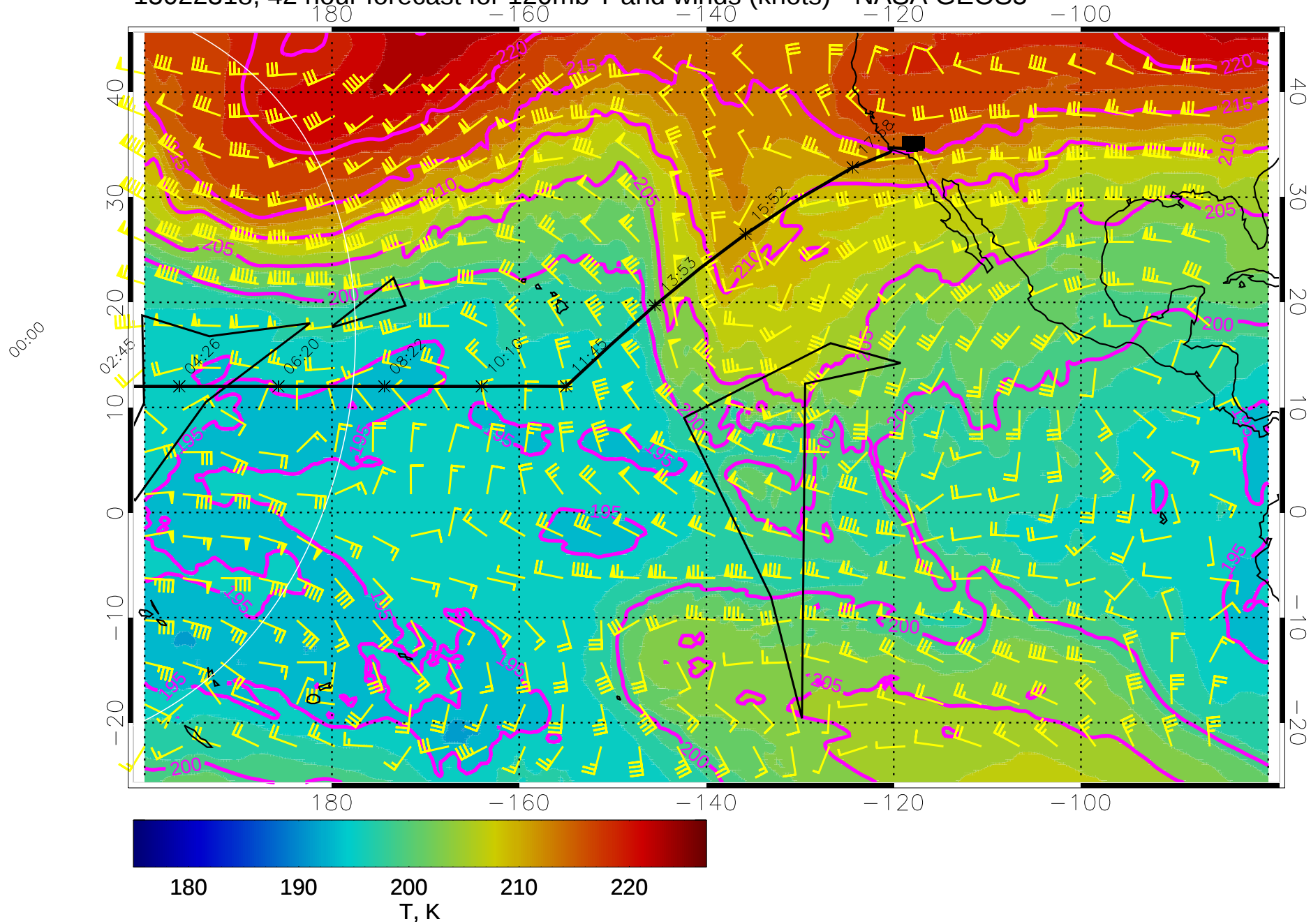
15022318, 42 hour forecast for 120mb T and winds (knots) - NASA GEOS5
