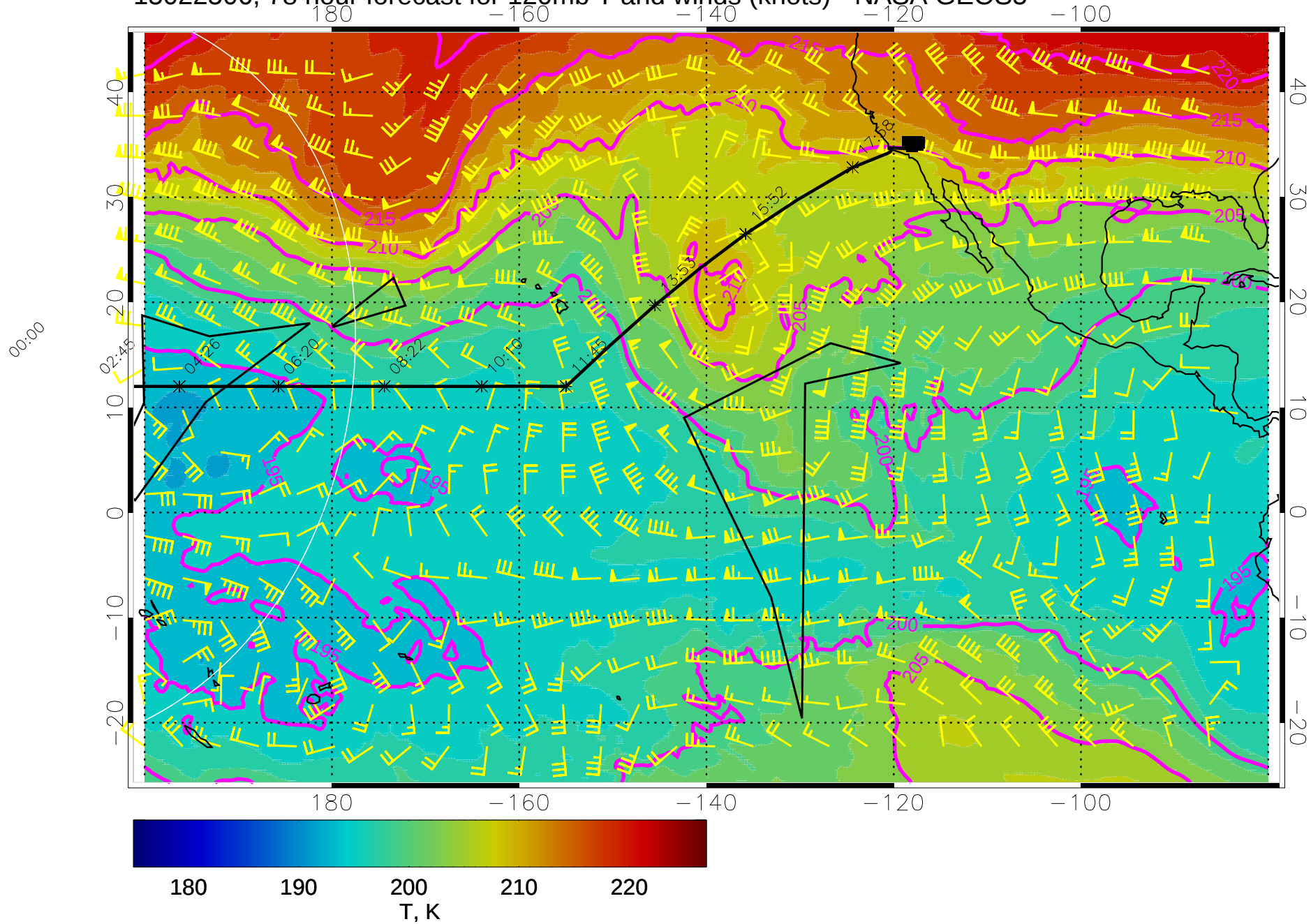
15022506, 78 hour forecast for 120mb T and winds (knots) - NASA GEOS5
