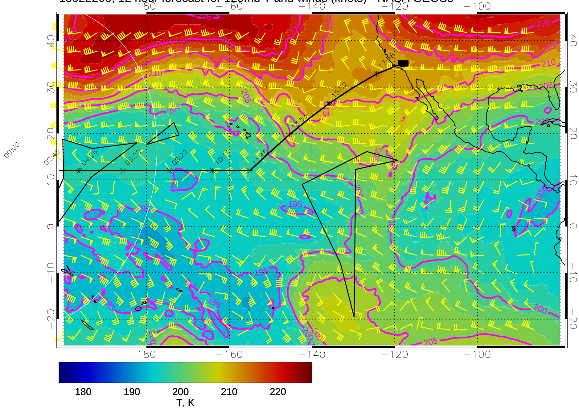
15022200, 12 hour forecast for 120mb T and winds (knots) - NASA GEOS5
