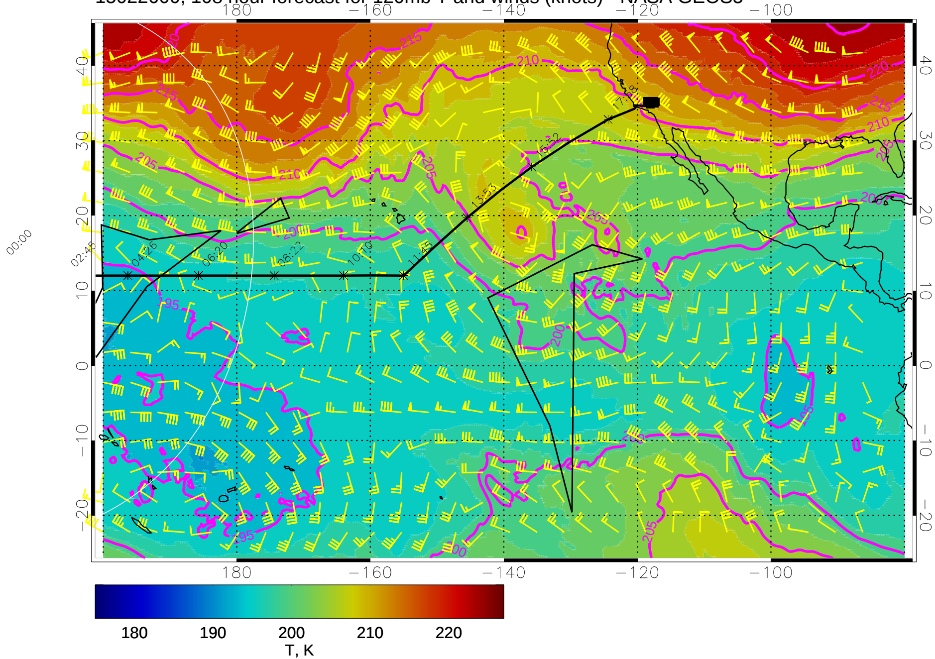
15022600, 108 hour forecast for 120mb T and winds (knots) - NASA GEOS5
