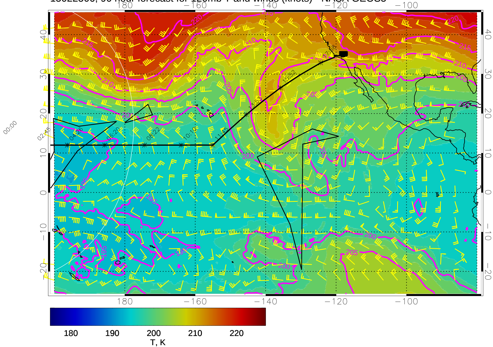
15022506, 90 hour forecast for 120mb T and winds (knots) - NASA GEOS5
