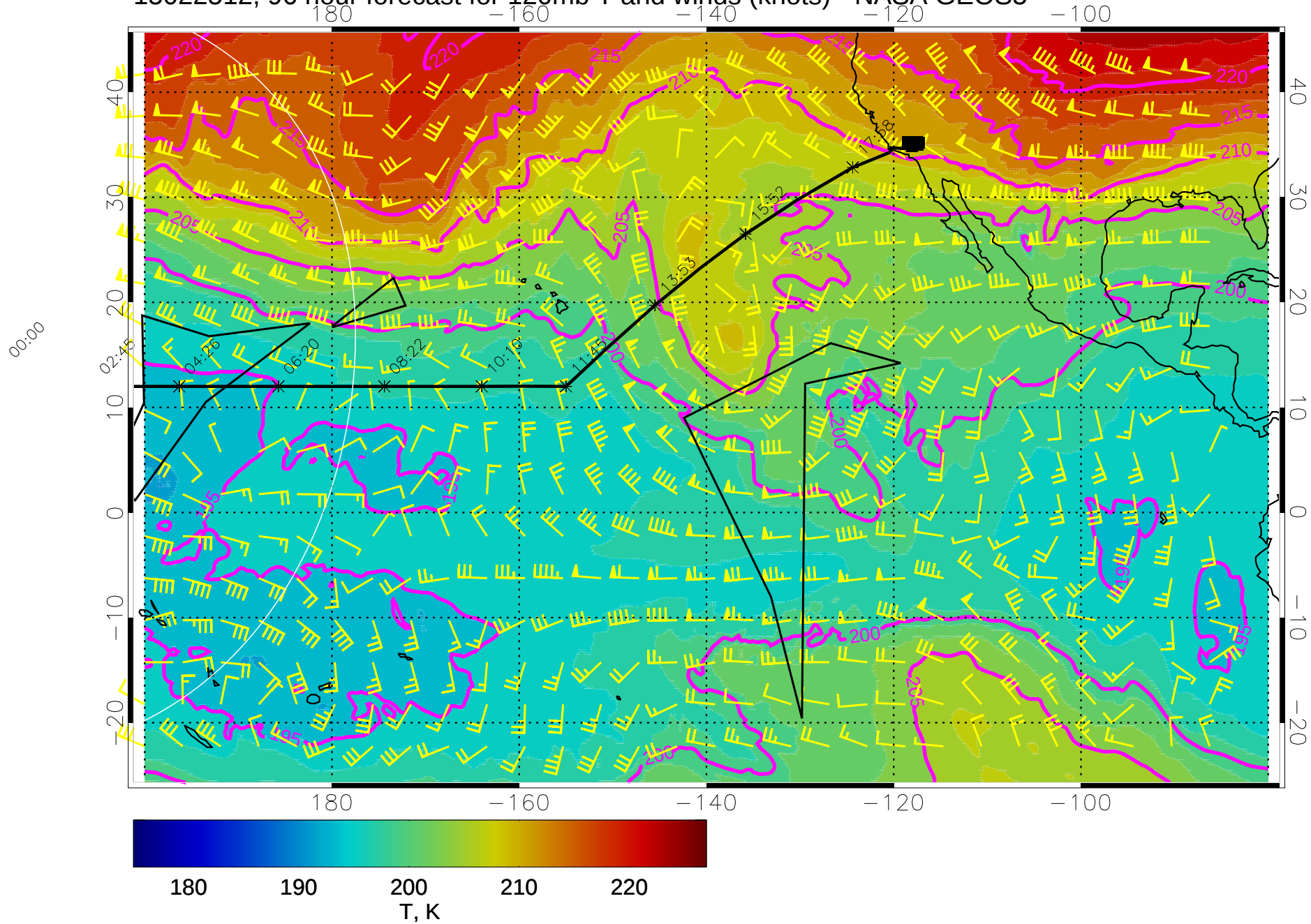
15022512, 96 hour forecast for 120mb T and winds (knots) - NASA GEOS5
