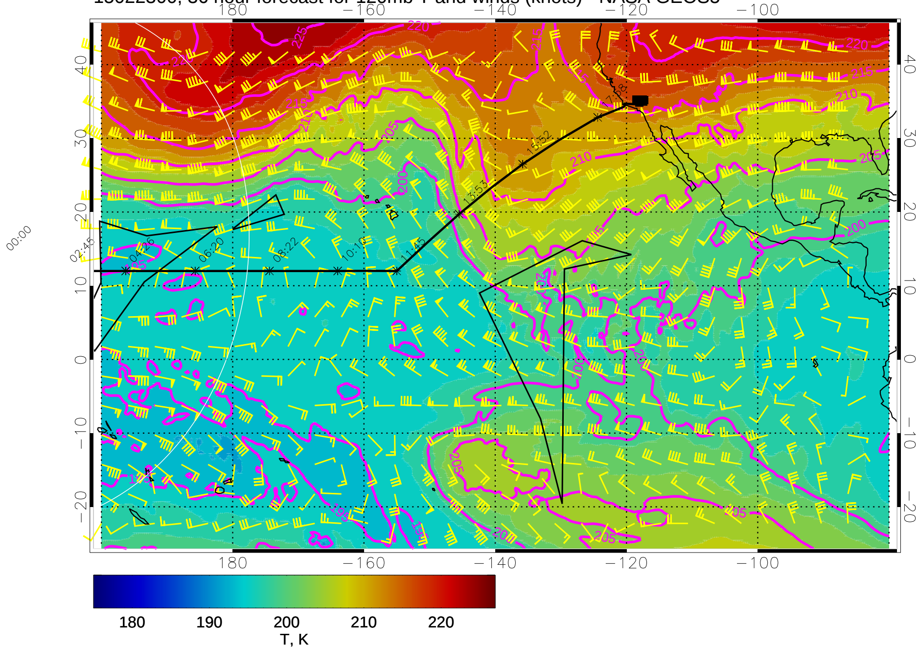
15022300, 36 hour forecast for 120mb T and winds (knots) - NASA GEOS5
