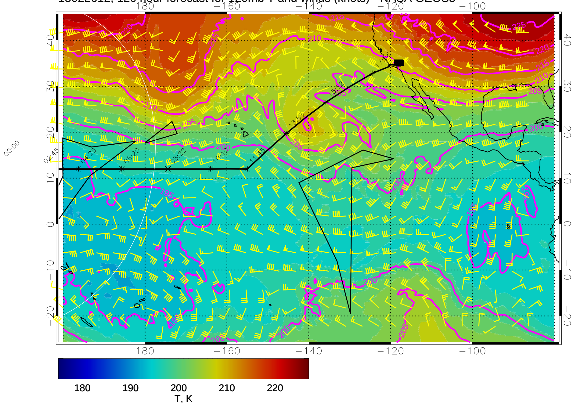
15022612, 120 hour forecast for 120mb T and winds (knots) - NASA GEOS5
