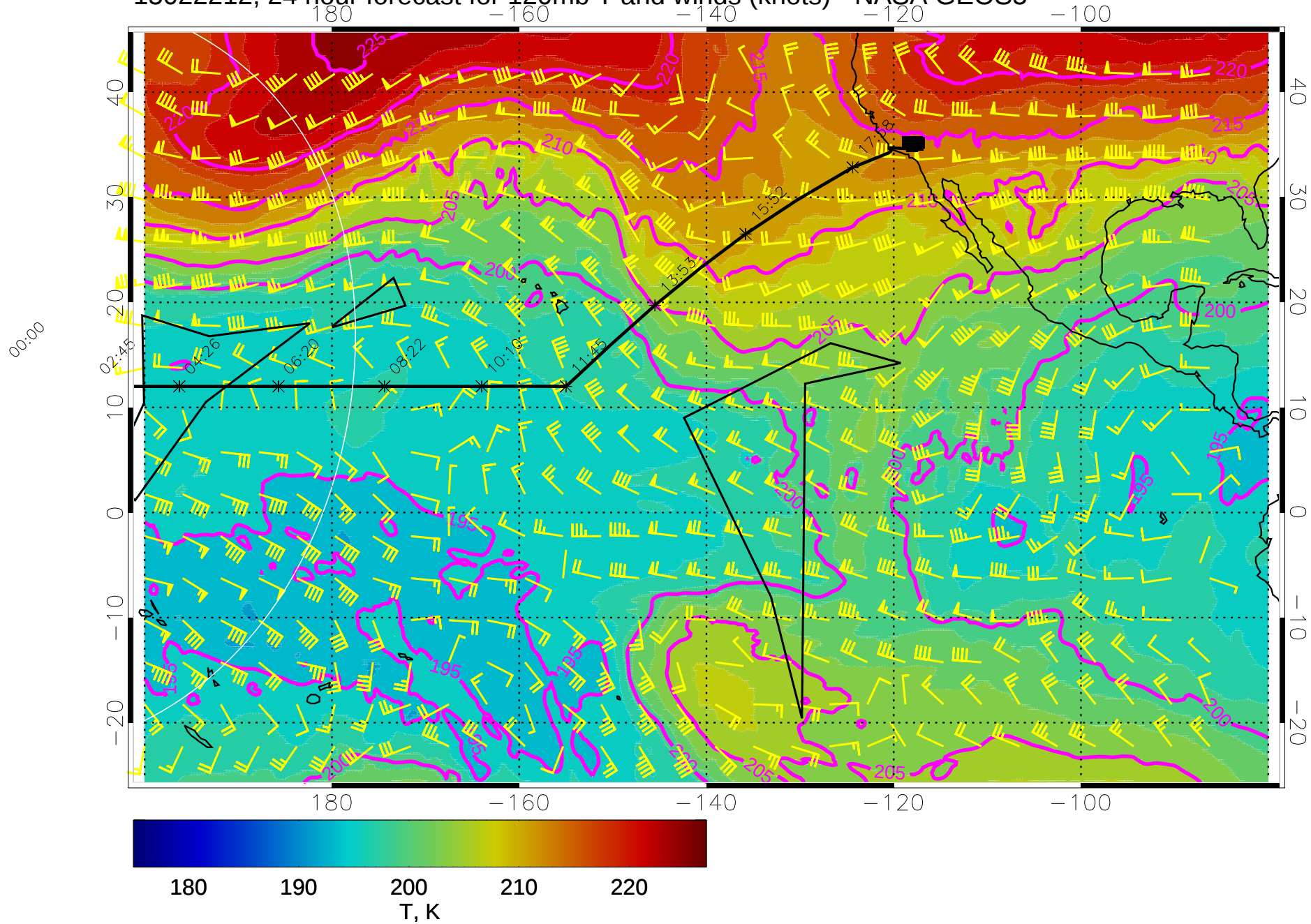
15022212, 24 hour forecast for 120mb T and winds (knots) - NASA GEOS5
