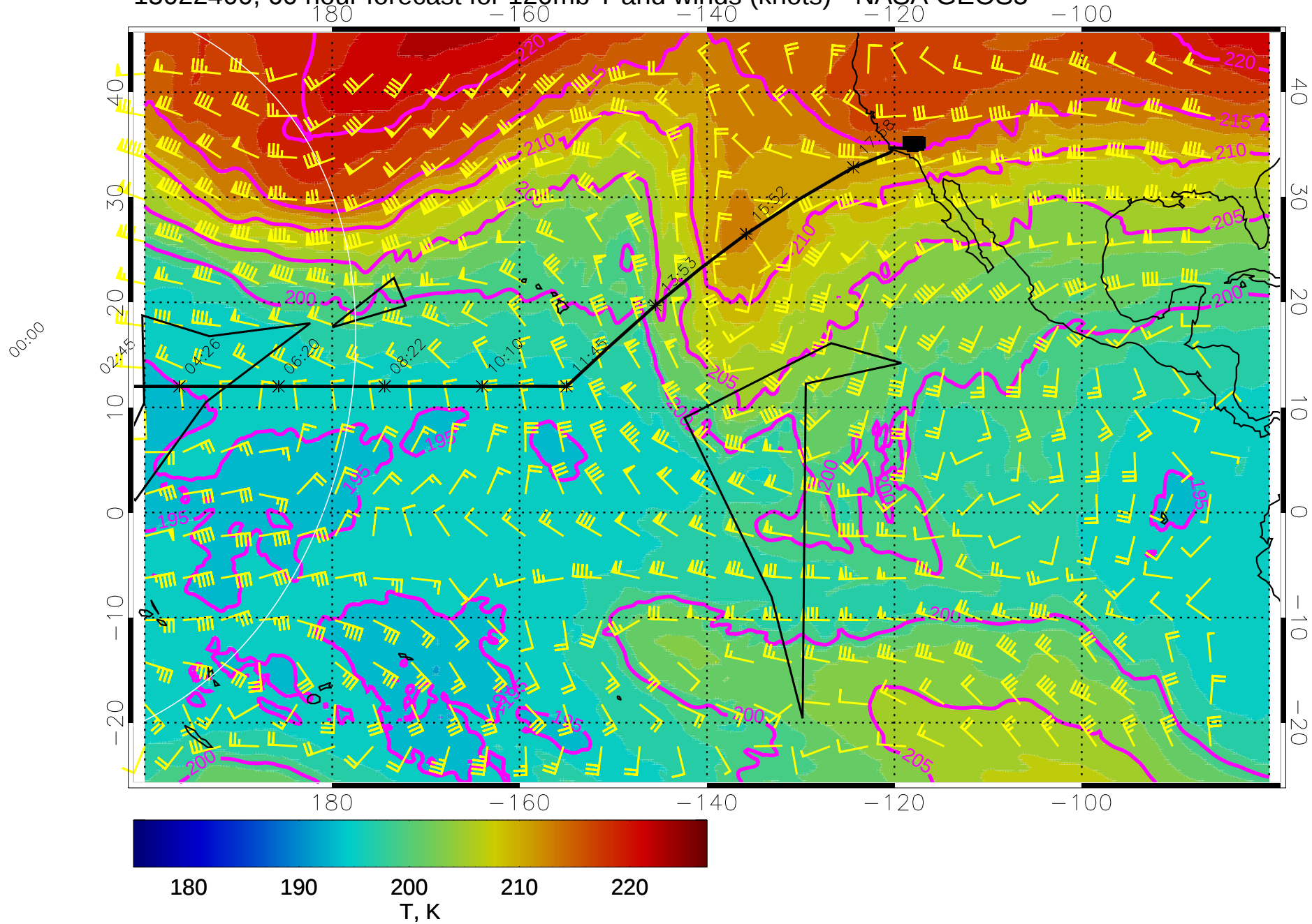
15022400, 60 hour forecast for 120mb T and winds (knots) - NASA GEOS5
