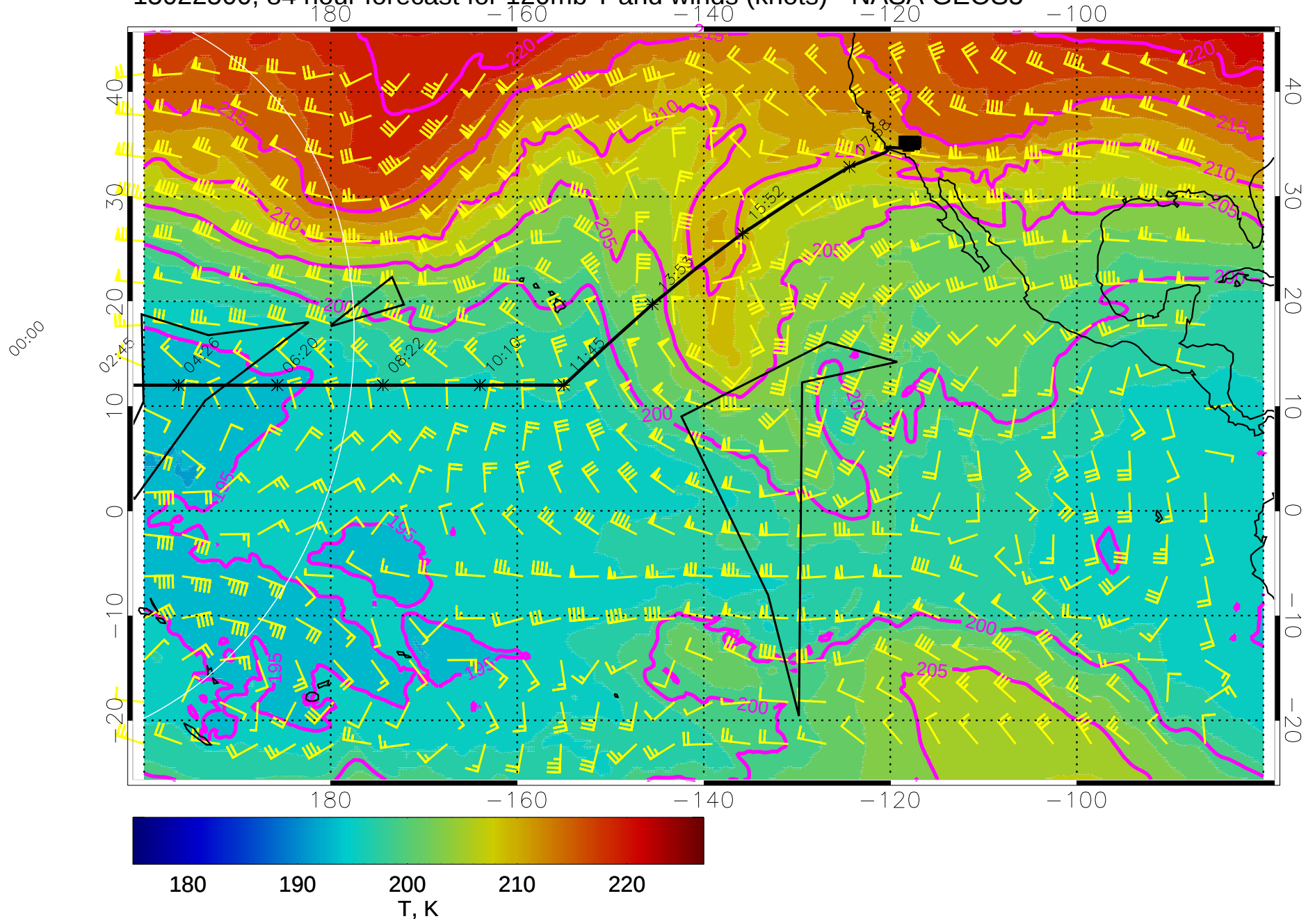
15022500, 84 hour forecast for 120mb T and winds (knots) - NASA GEOS5
