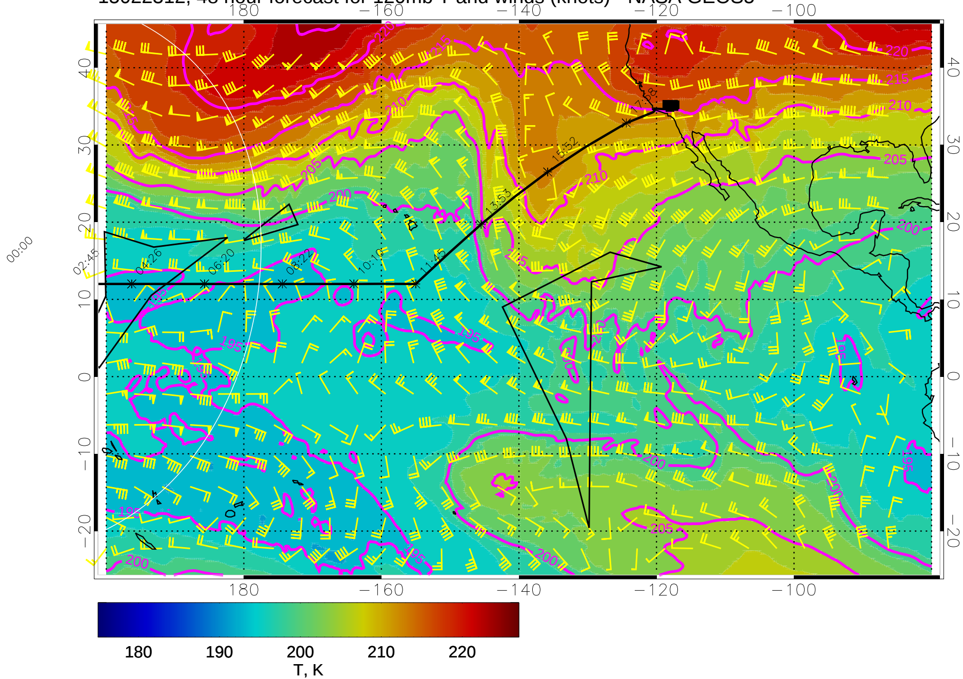
15022312, 48 hour forecast for 120mb T and winds (knots) - NASA GEOS5
