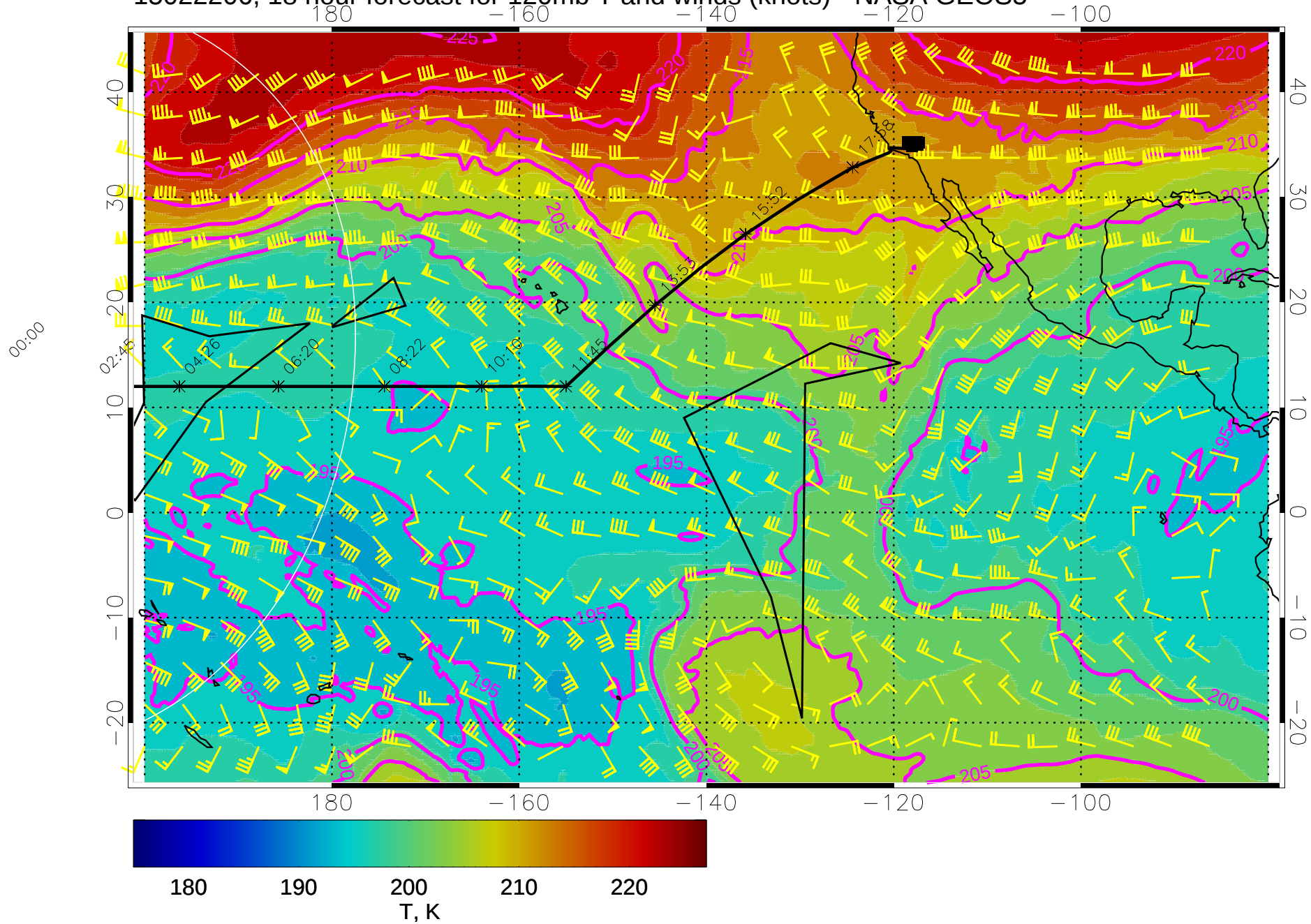
15022206, 18 hour forecast for 120mb T and winds (knots) - NASA GEOS5
