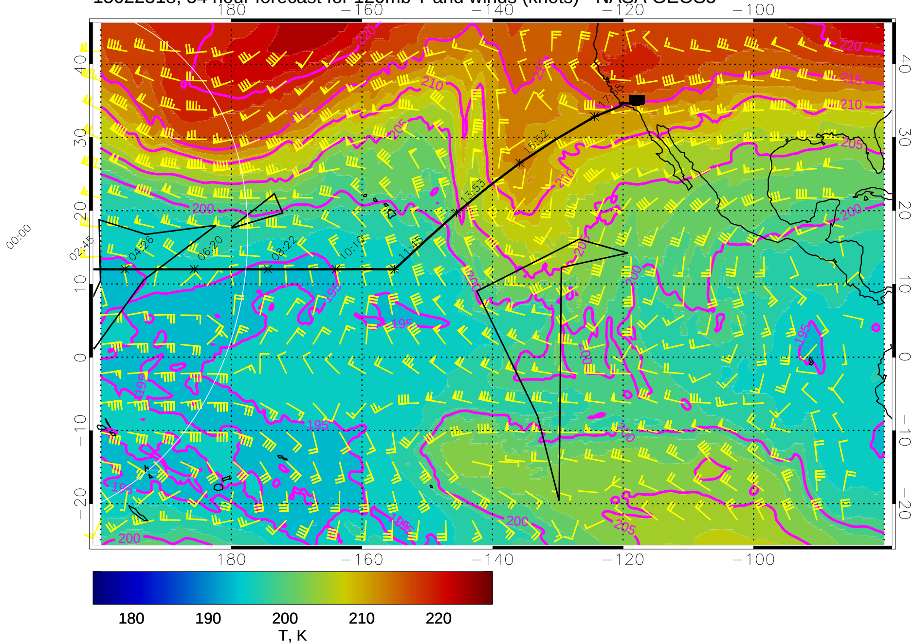
15022318, 54 hour forecast for 120mb T and winds (knots) - NASA GEOS5
