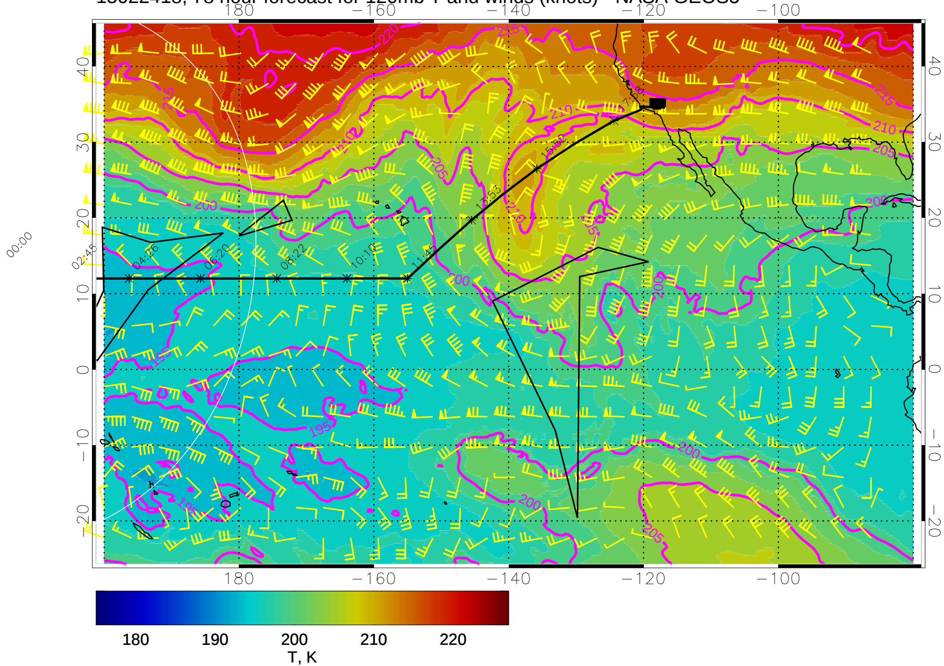
15022418, 78 hour forecast for 120mb T and winds (knots) - NASA GEOS5
