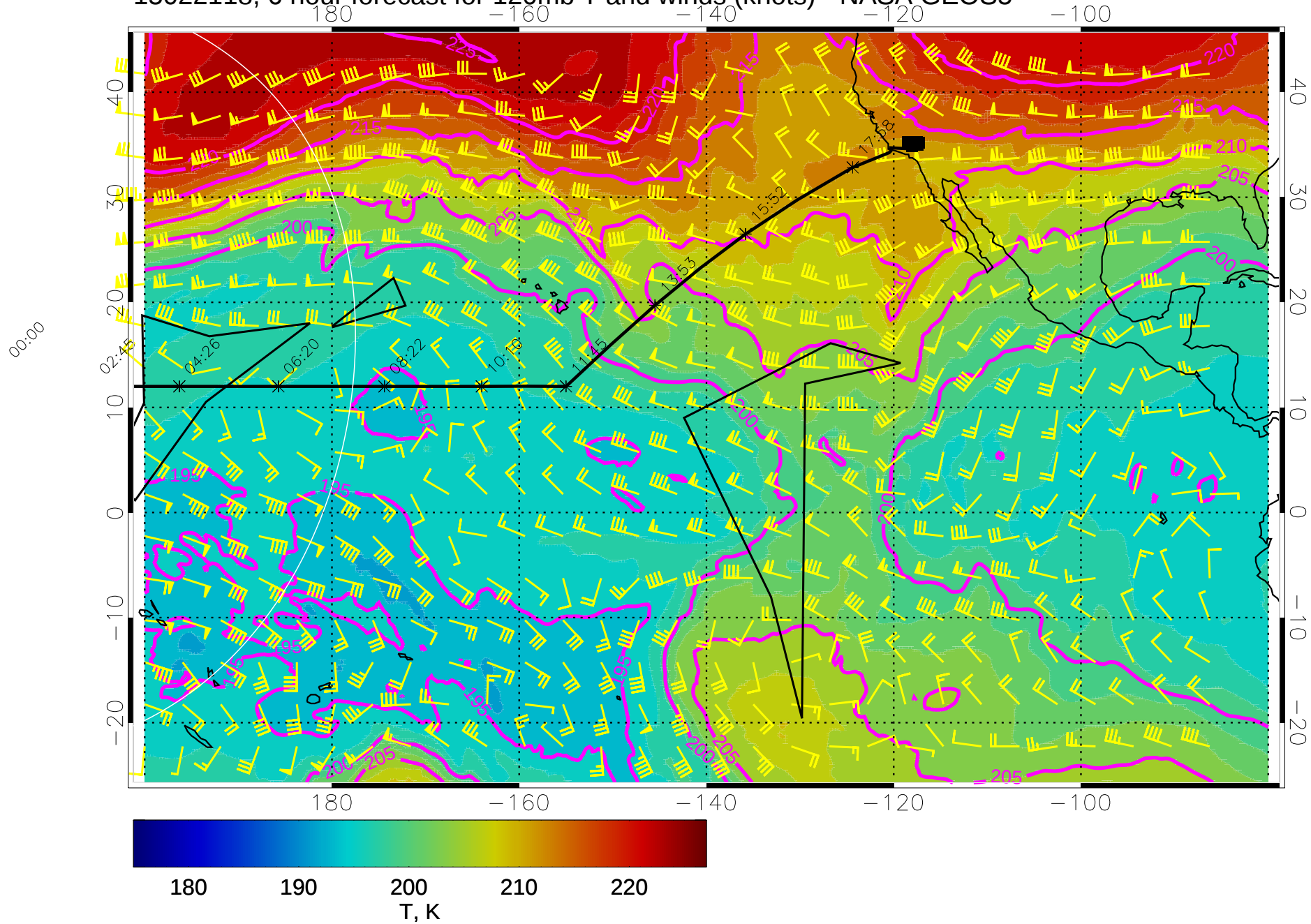
15022118, 6 hour forecast for 120mb T and winds (knots) - NASA GEOS5
