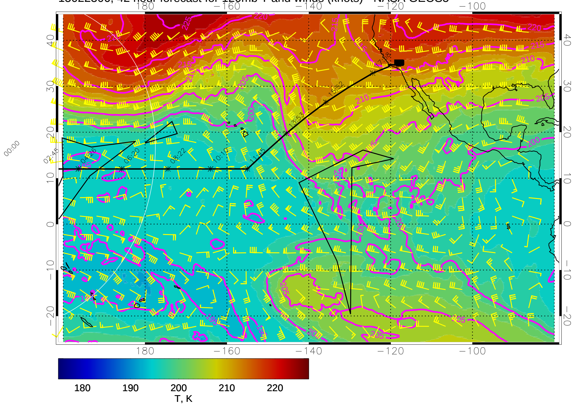
15022306, 42 hour forecast for 120mb T and winds (knots) - NASA GEOS5
