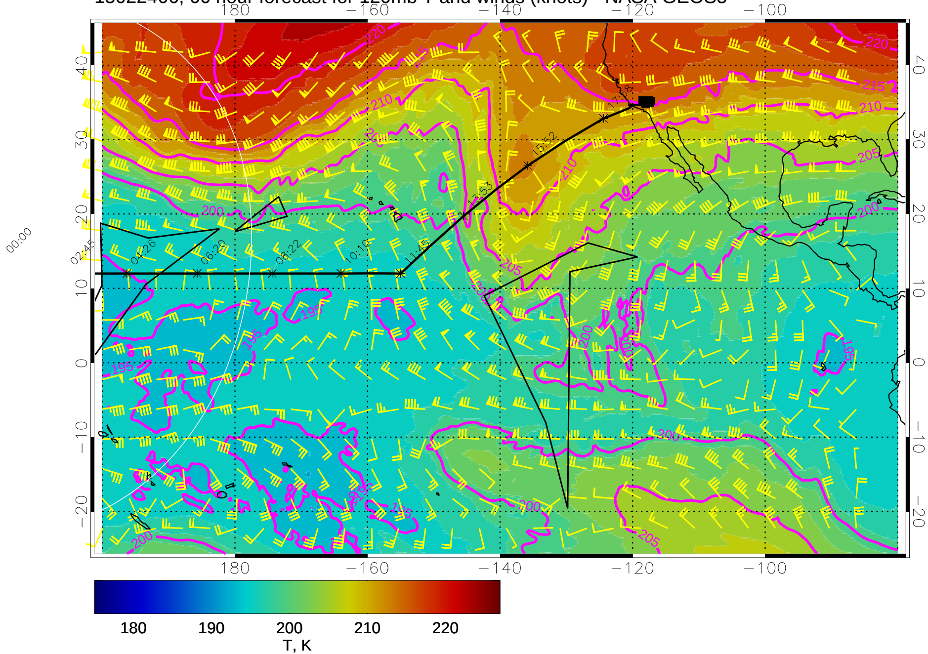
15022406, 66 hour forecast for 120mb T and winds (knots) - NASA GEOS5
