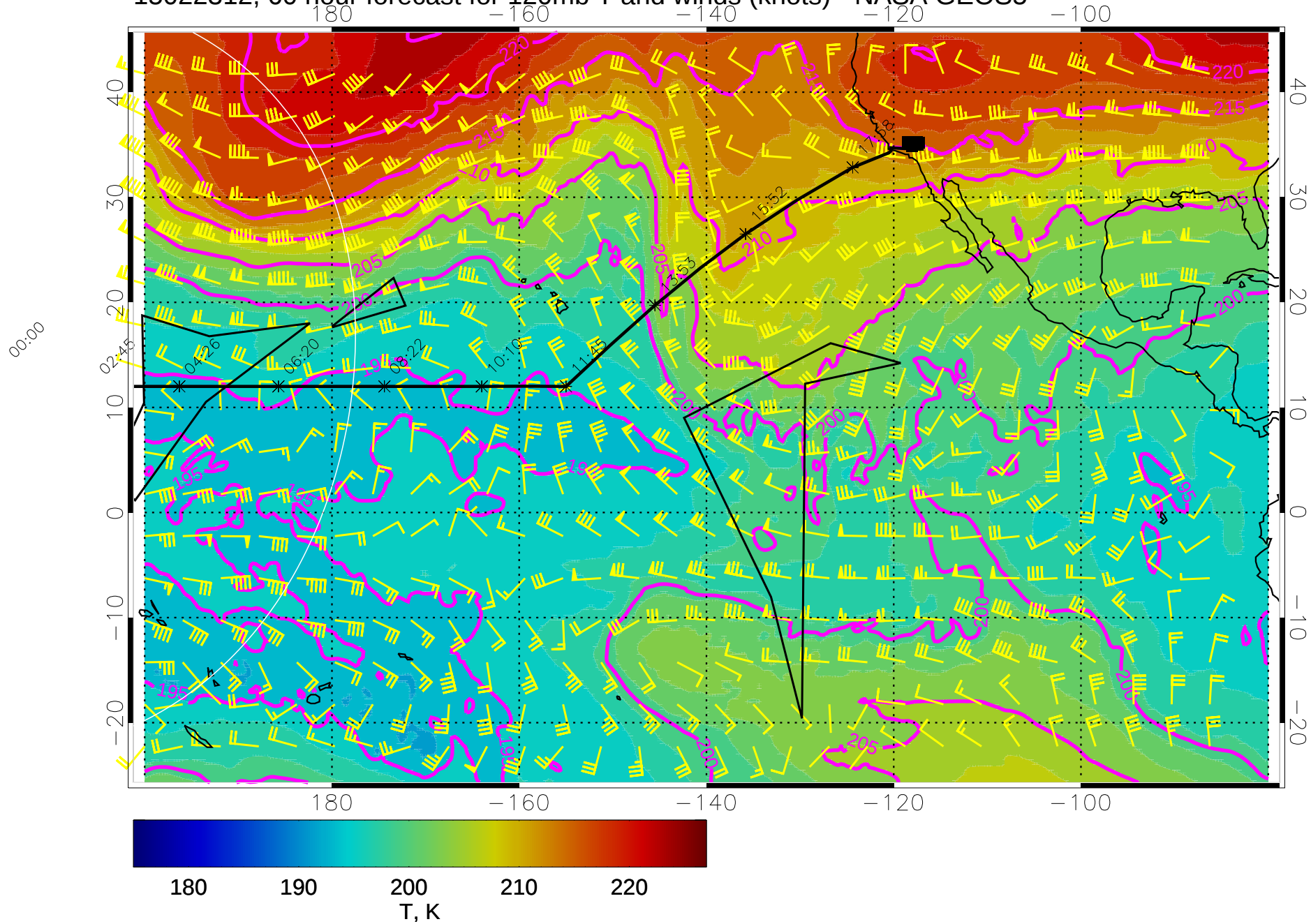
15022312, 60 hour forecast for 120mb T and winds (knots) - NASA GEOS5
