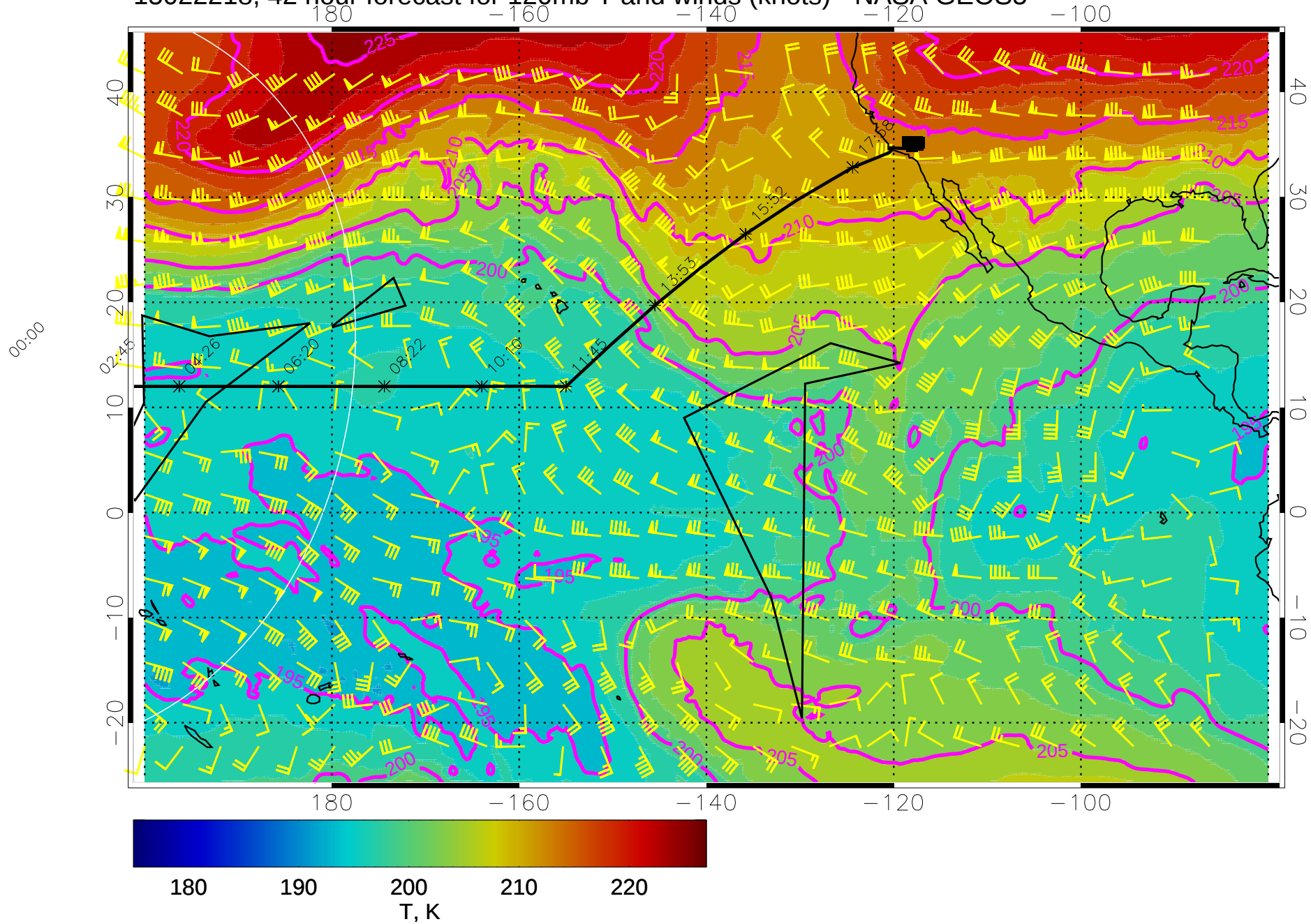
15022218, 42 hour forecast for 120mb T and winds (knots) - NASA GEOS5
