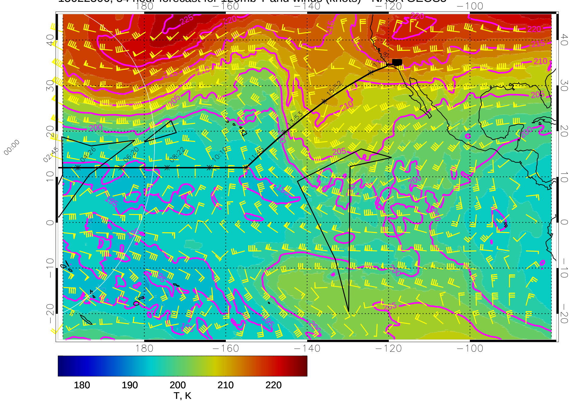
15022306, 54 hour forecast for 120mb T and winds (knots) - NASA GEOS5
