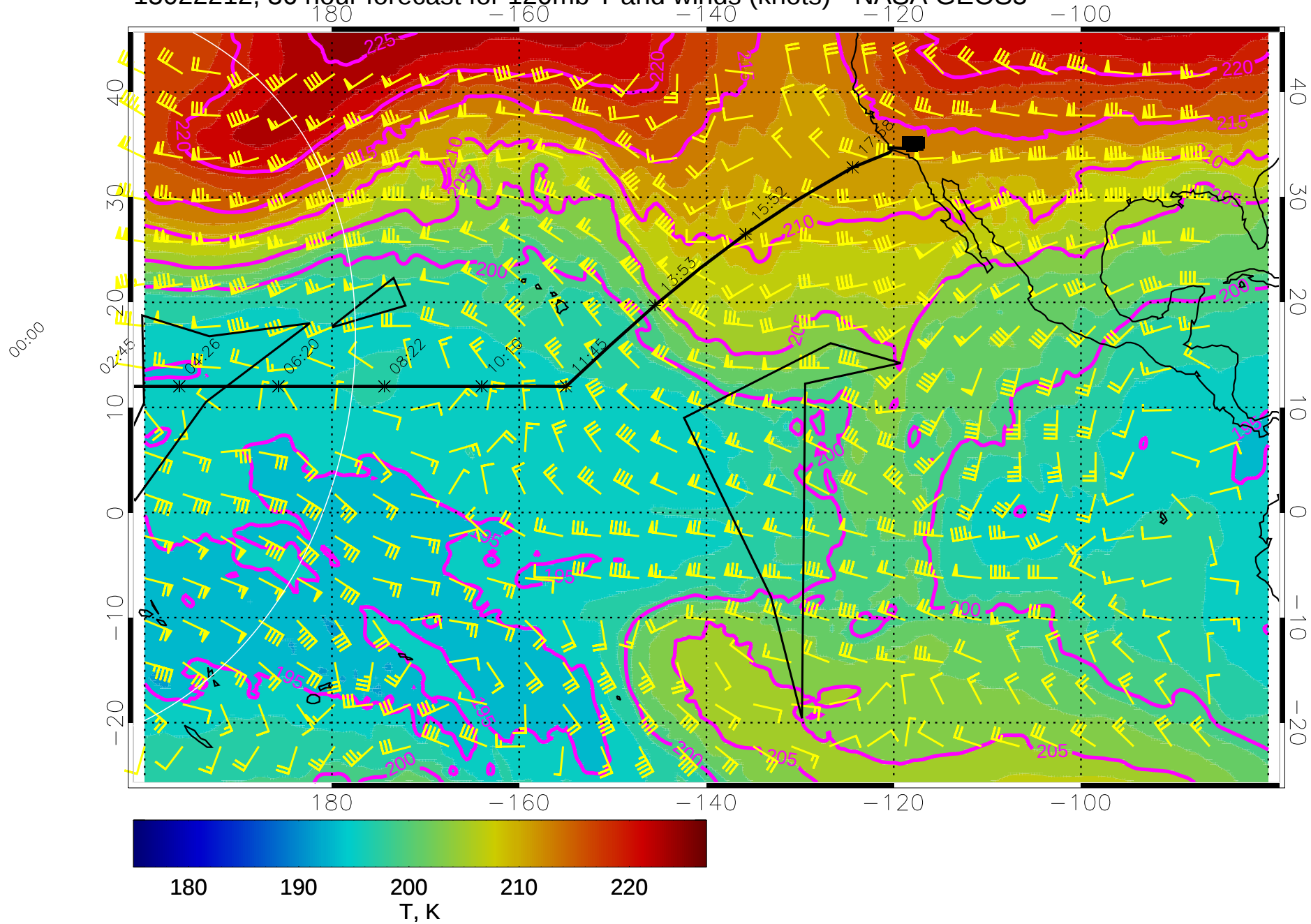
15022212, 36 hour forecast for 120mb T and winds (knots) - NASA GEOS5
