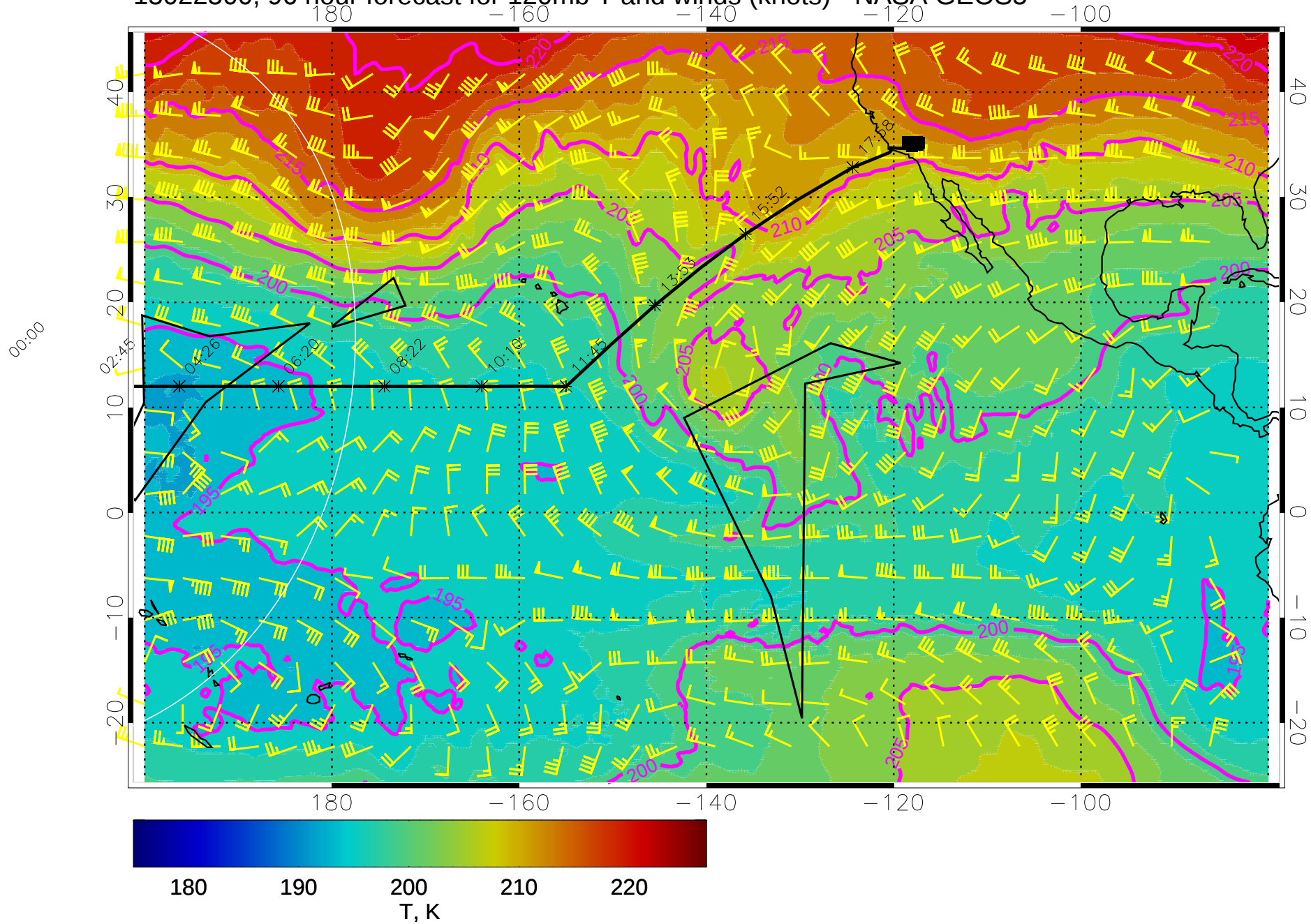
15022500, 96 hour forecast for 120mb T and winds (knots) - NASA GEOS5
