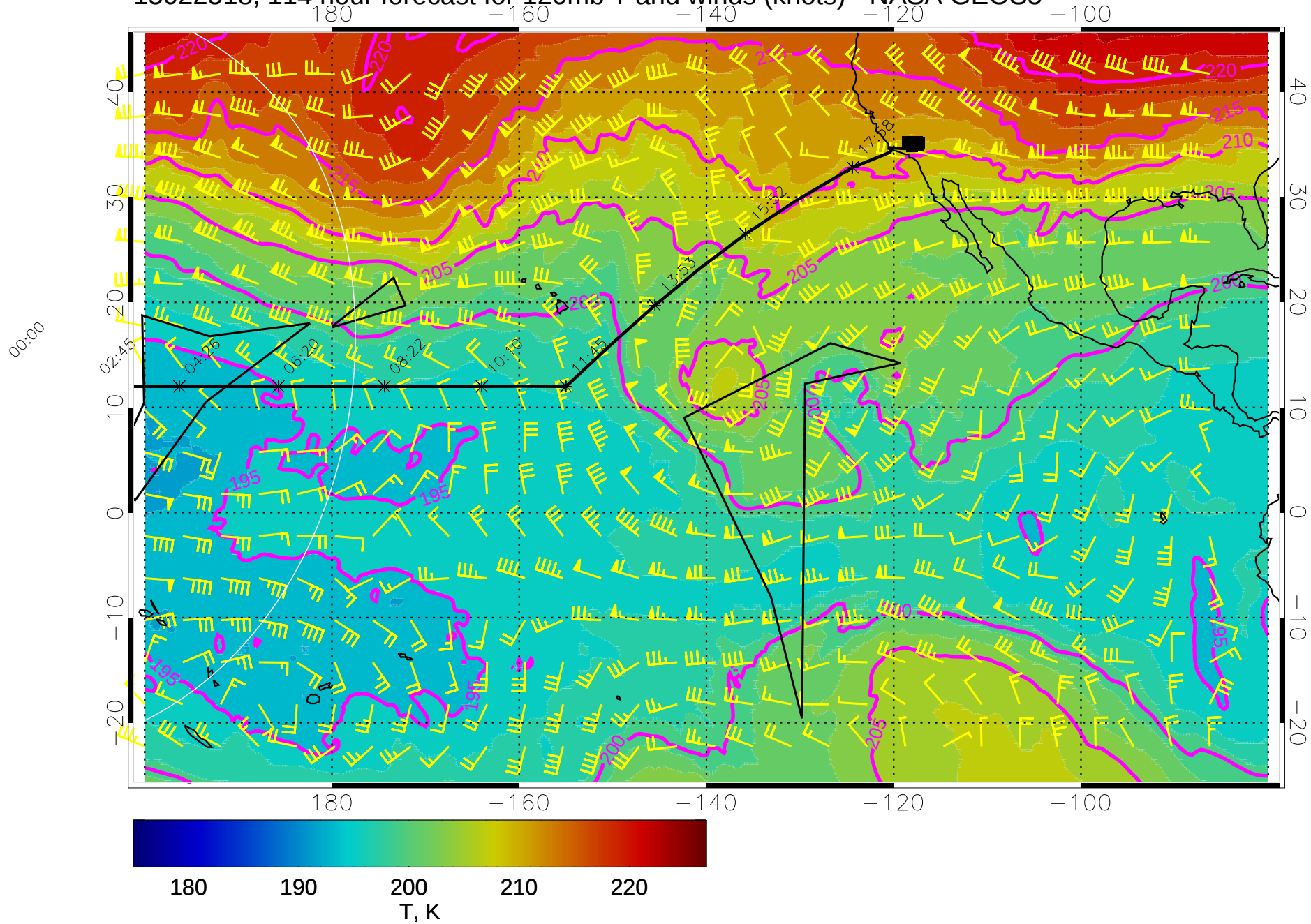
15022518, 114 hour forecast for 120mb T and winds (knots) - NASA GEOS5
