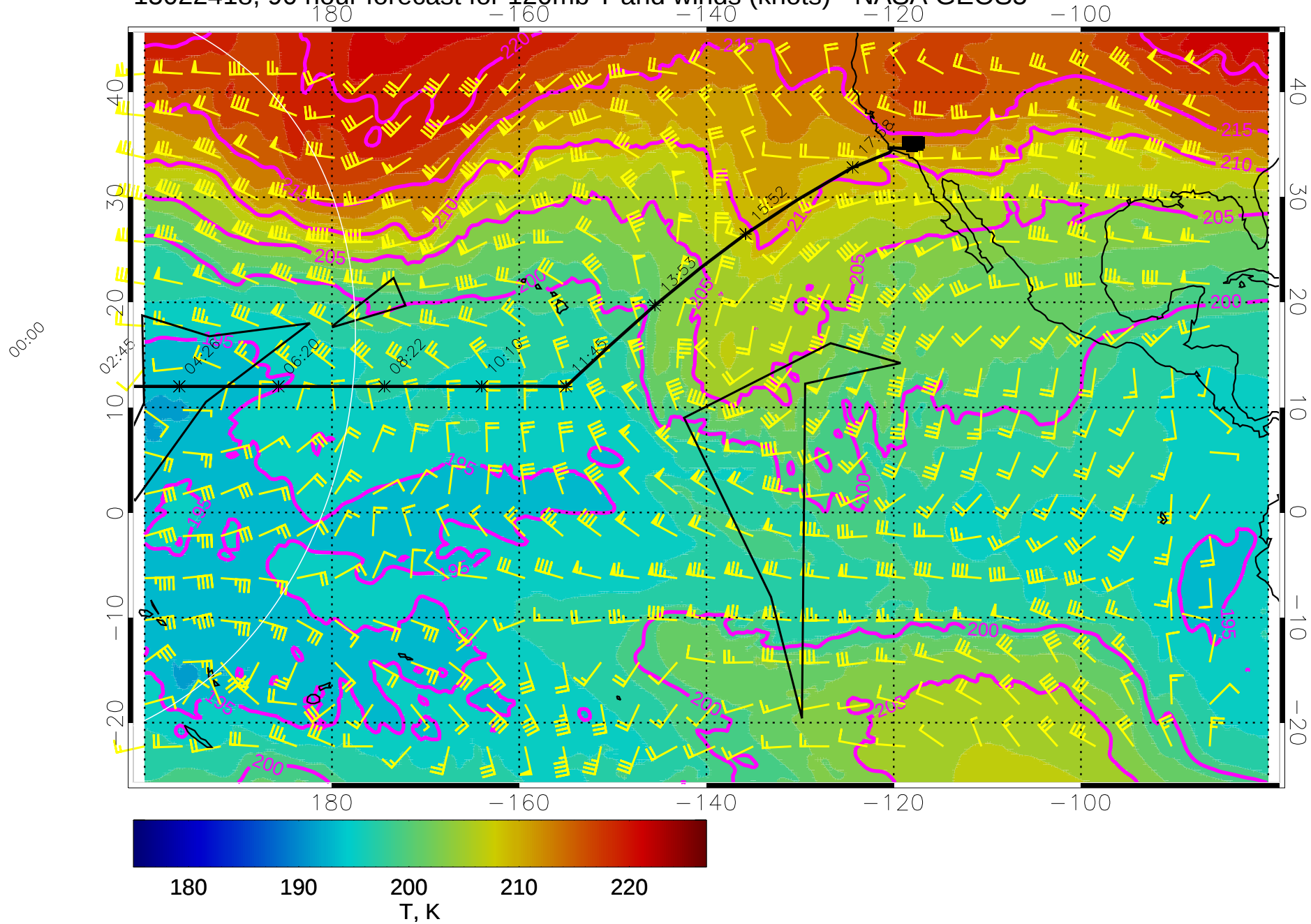
15022418, 90 hour forecast for 120mb T and winds (knots) - NASA GEOS5
