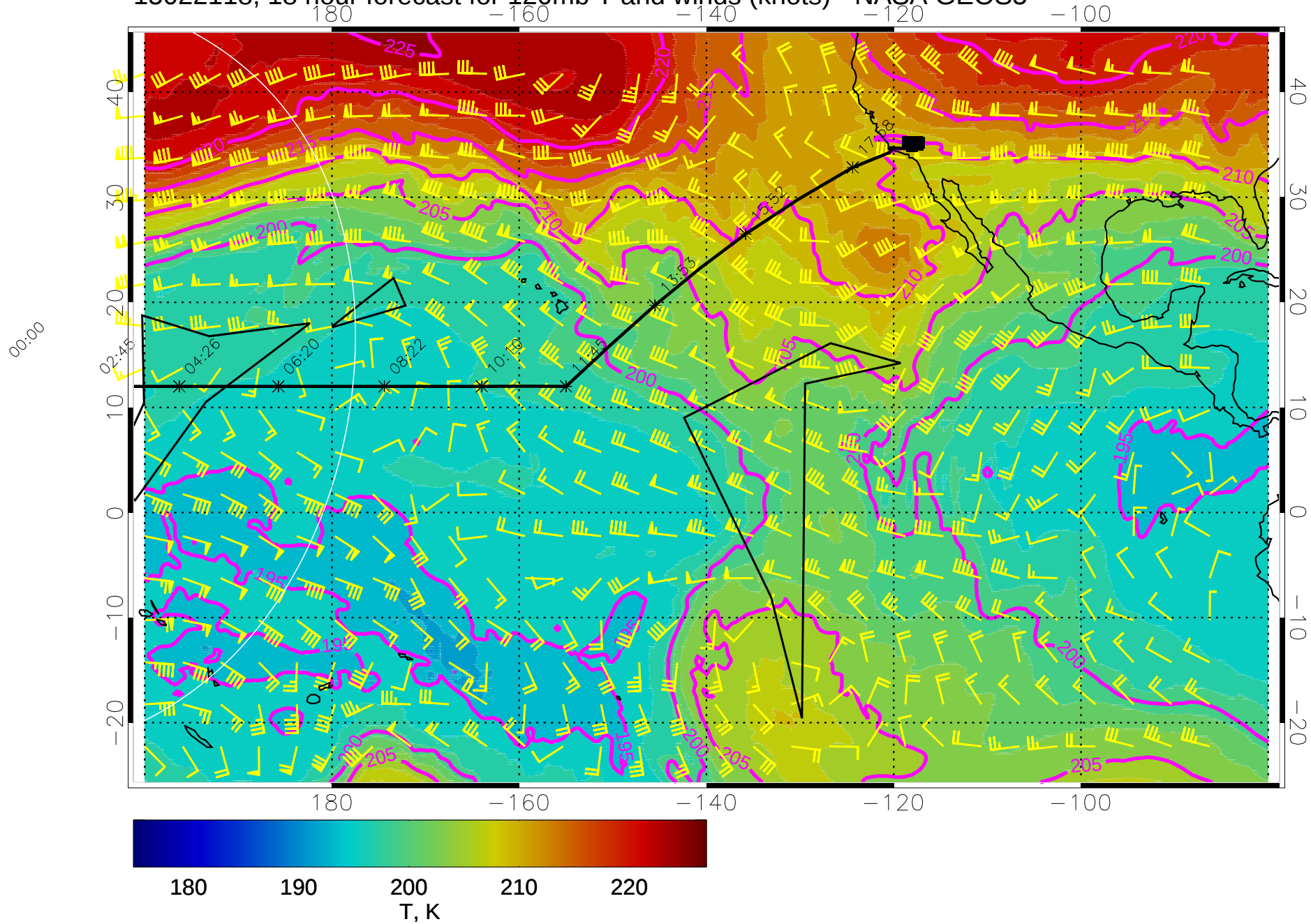
15022118, 18 hour forecast for 120mb T and winds (knots) - NASA GEOS5
