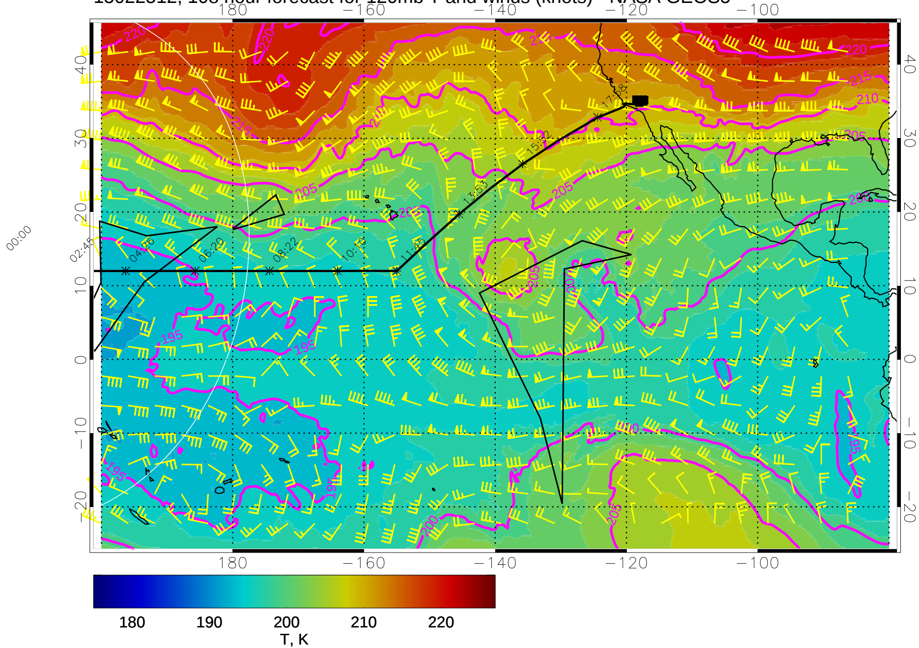
15022512, 108 hour forecast for 120mb T and winds (knots) - NASA GEOS5
