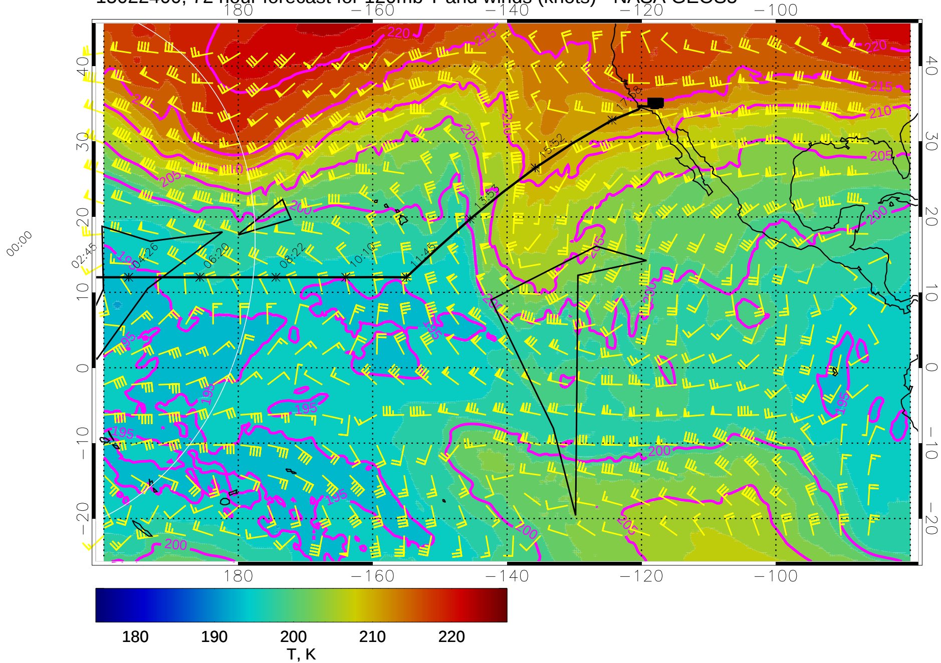
15022400, 72 hour forecast for 120mb T and winds (knots) - NASA GEOS5
