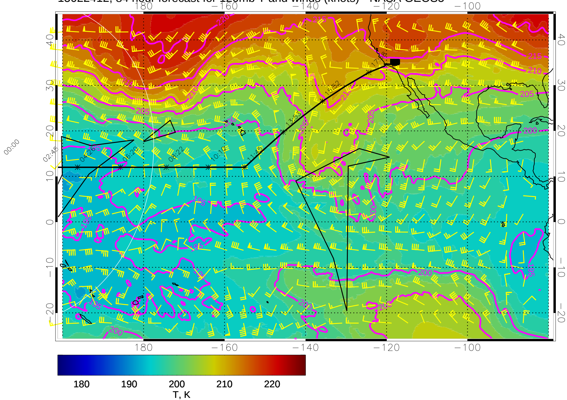
15022412, 84 hour forecast for 120mb T and winds (knots) - NASA GEOS5
