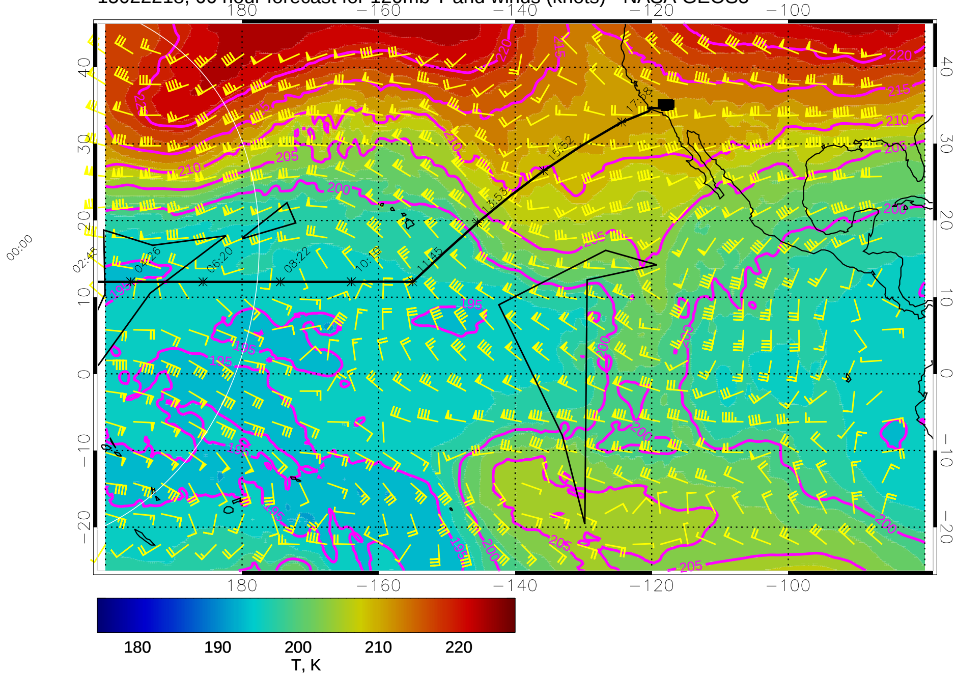
15022218, 66 hour forecast for 120mb T and winds (knots) - NASA GEOS5
