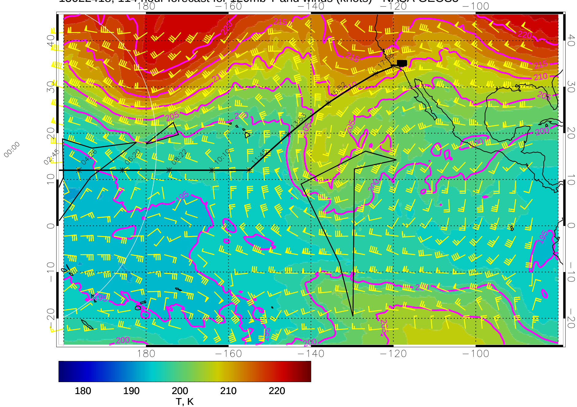
15022418, 114 hour forecast for 120mb T and winds (knots) - NASA GEOS5
