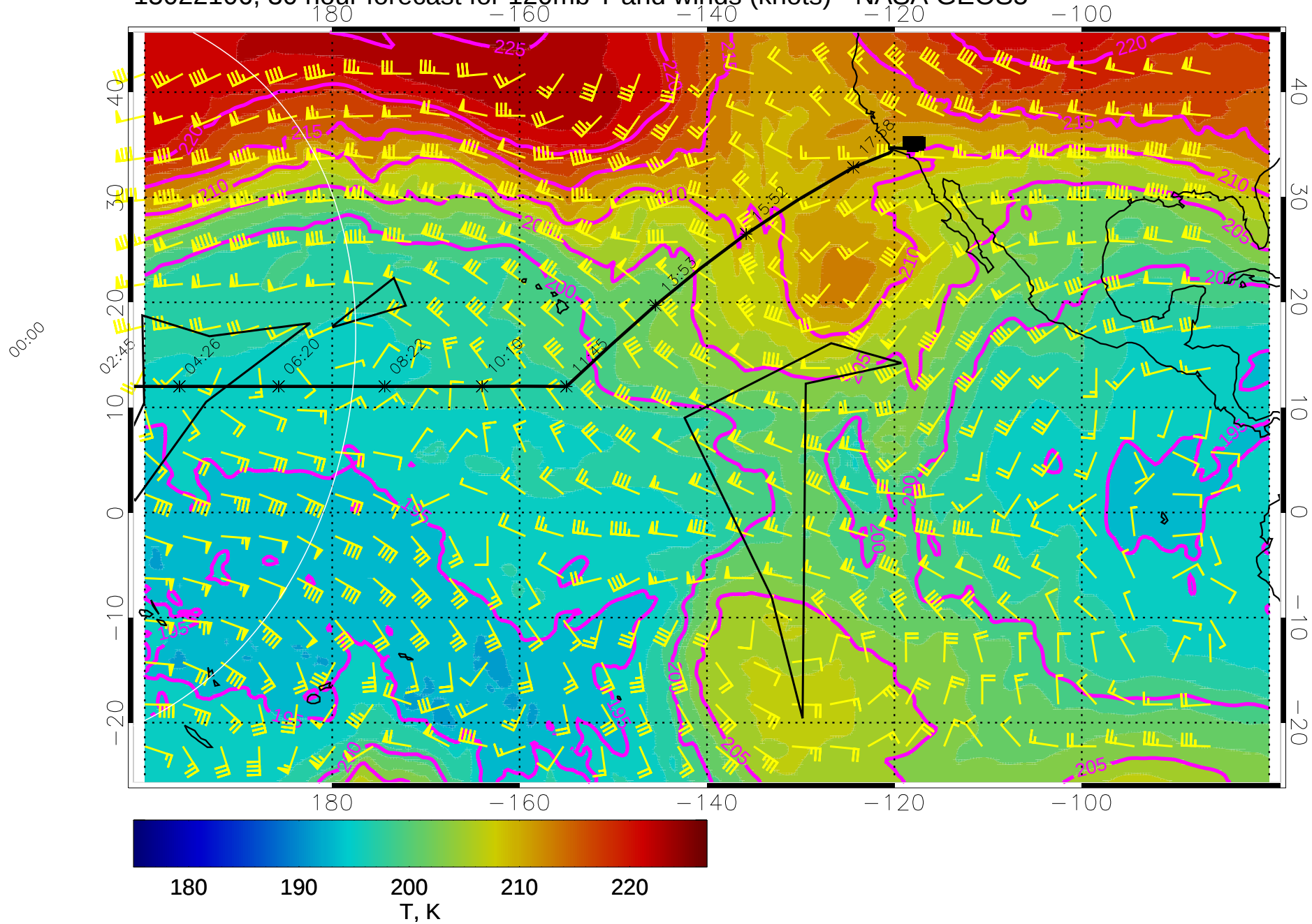
15022106, 30 hour forecast for 120mb T and winds (knots) - NASA GEOS5
