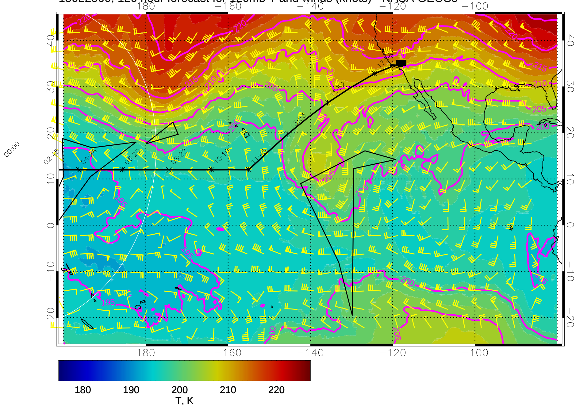
15022500, 120 hour forecast for 120mb T and winds (knots) - NASA GEOS5
