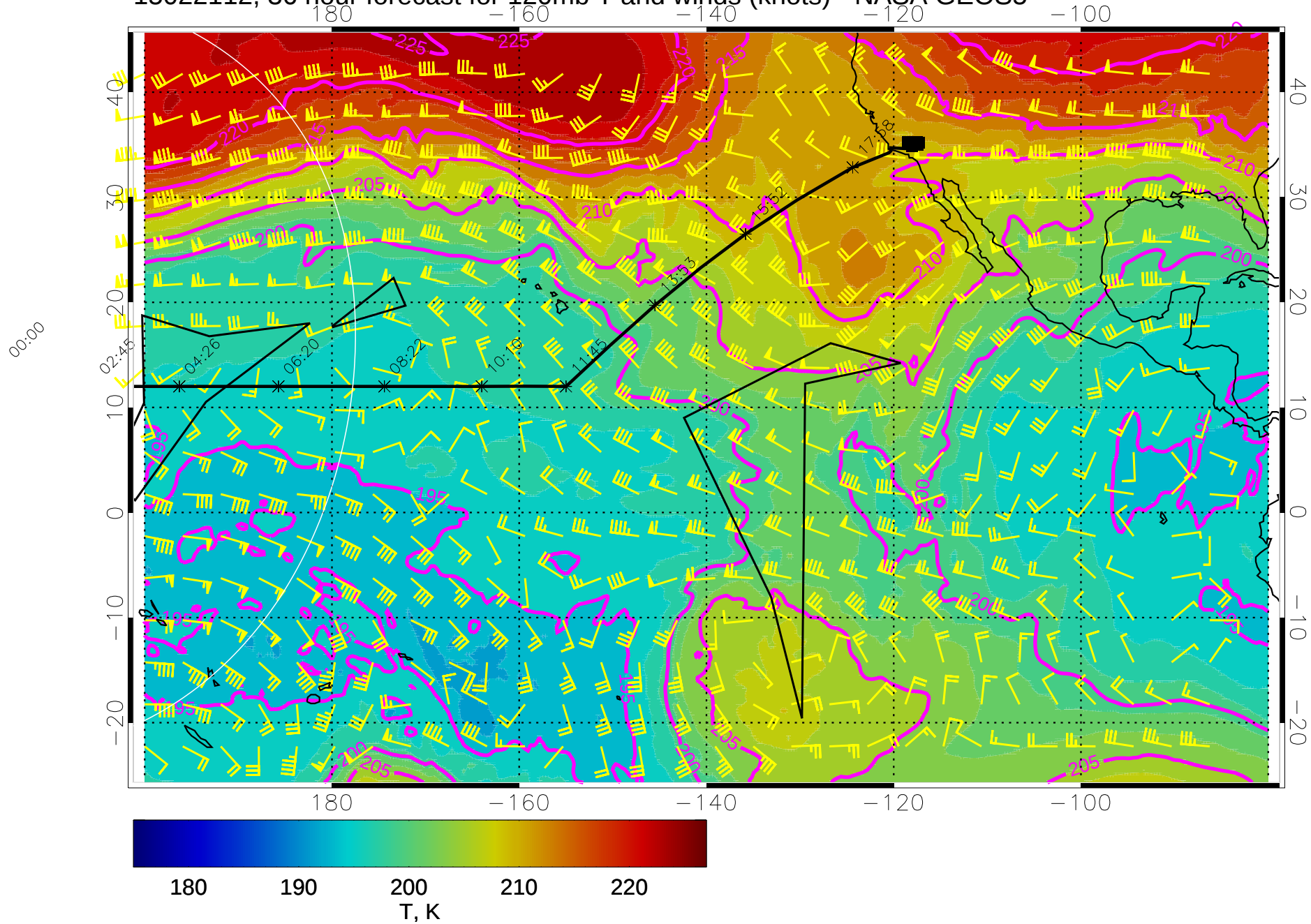
15022112, 36 hour forecast for 120mb T and winds (knots) - NASA GEOS5
