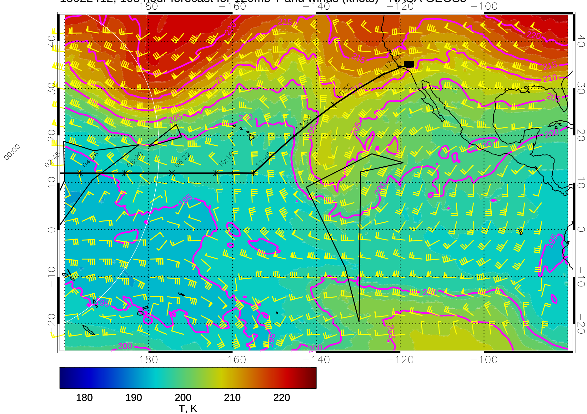
15022412, 108 hour forecast for 120mb T and winds (knots) - NASA GEOS5
