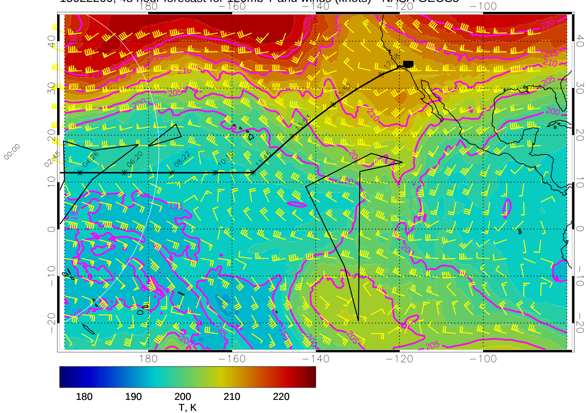
15022200, 48 hour forecast for 120mb T and winds (knots) - NASA GEOS5
