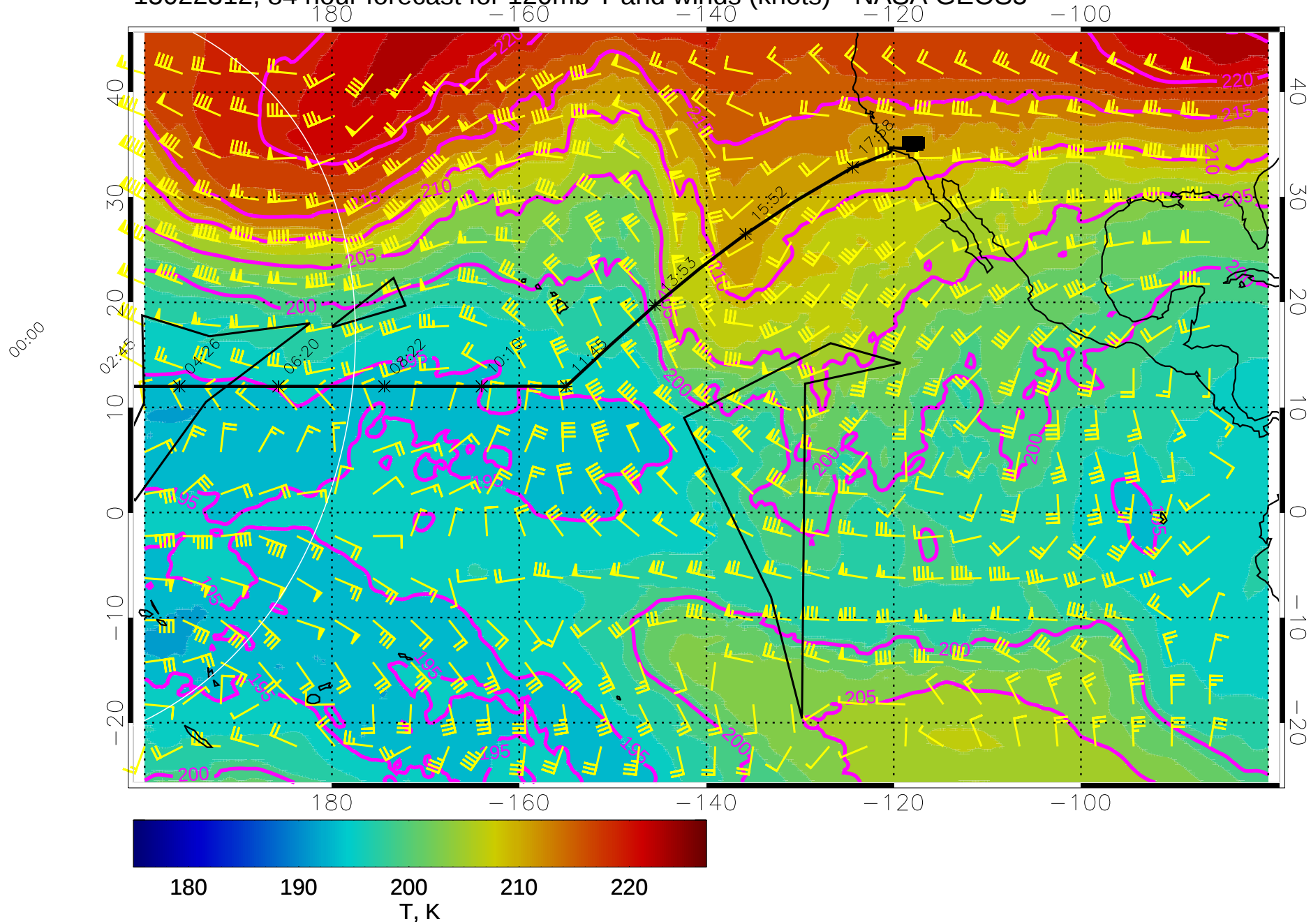
15022312, 84 hour forecast for 120mb T and winds (knots) - NASA GEOS5
