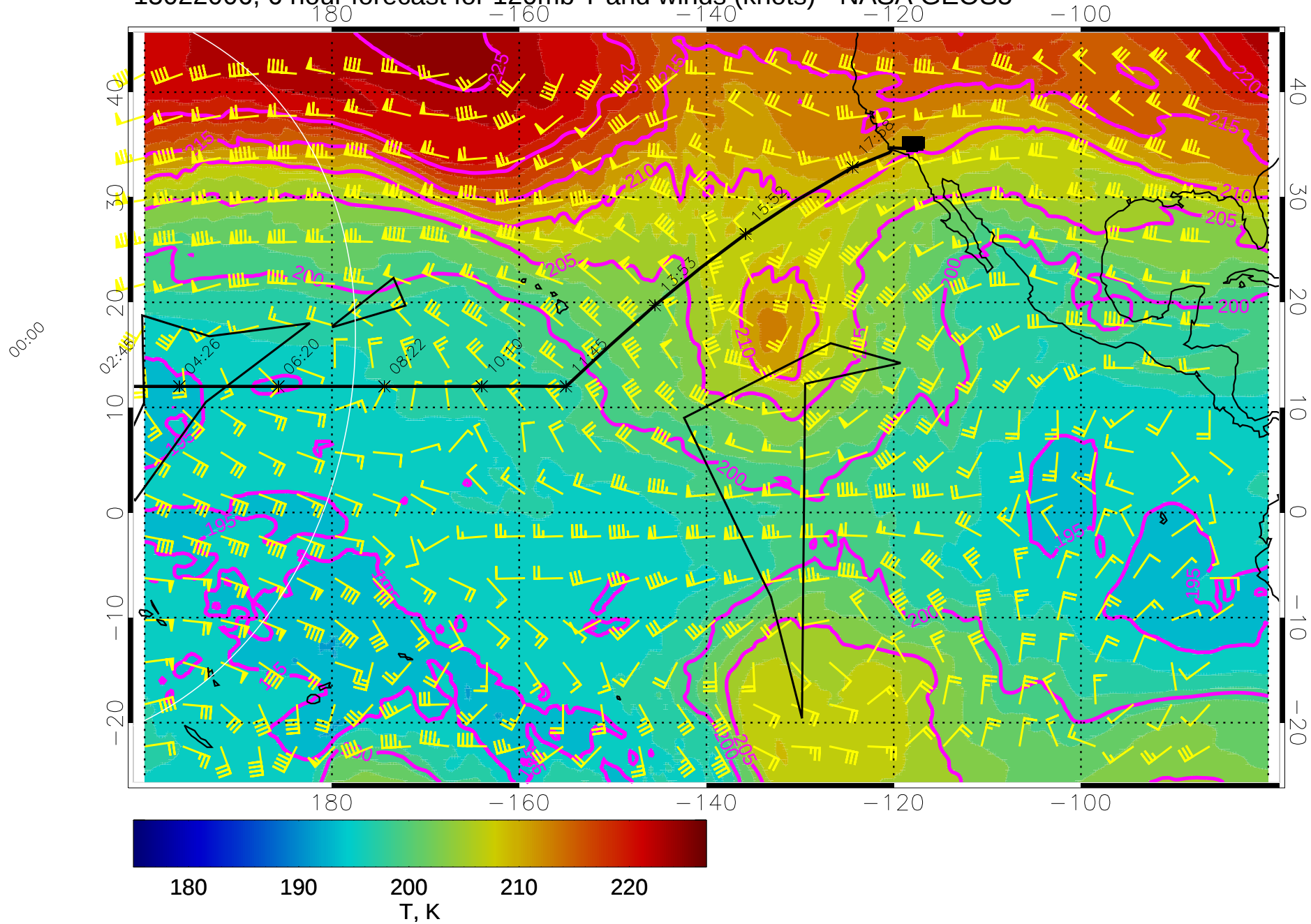
15022006, 6 hour forecast for 120mb T and winds (knots) - NASA GEOS5
