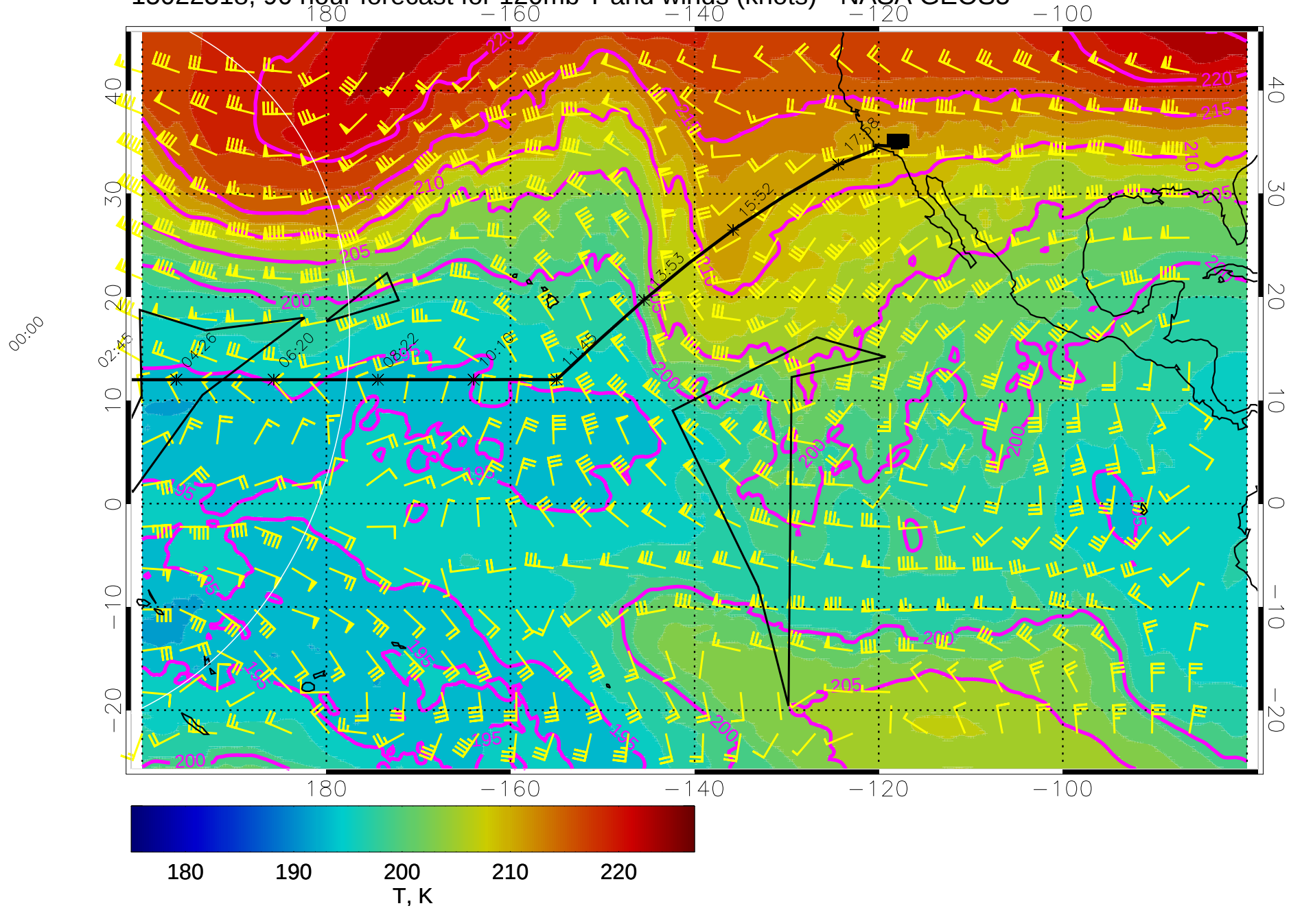
15022318, 90 hour forecast for 120mb T and winds (knots) - NASA GEOS5
