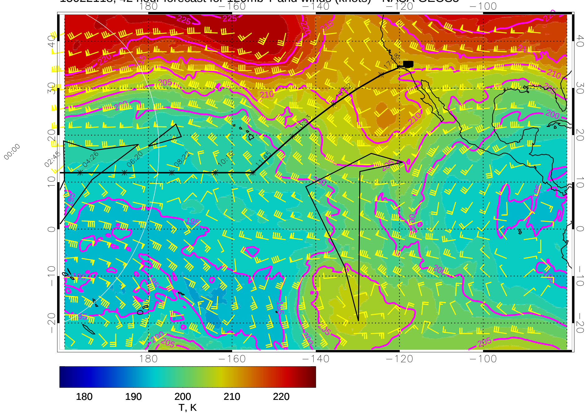
15022118, 42 hour forecast for 120mb T and winds (knots) - NASA GEOS5
