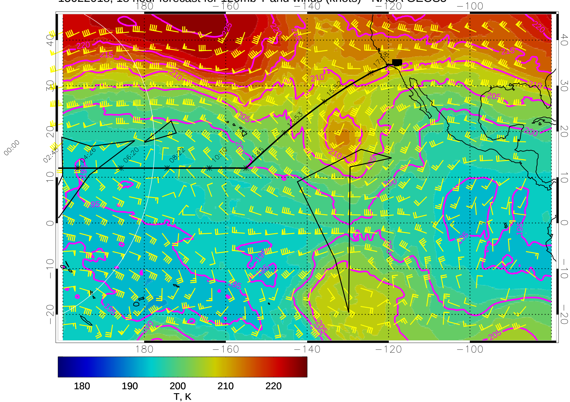
15022018, 18 hour forecast for 120mb T and winds (knots) - NASA GEOS5
