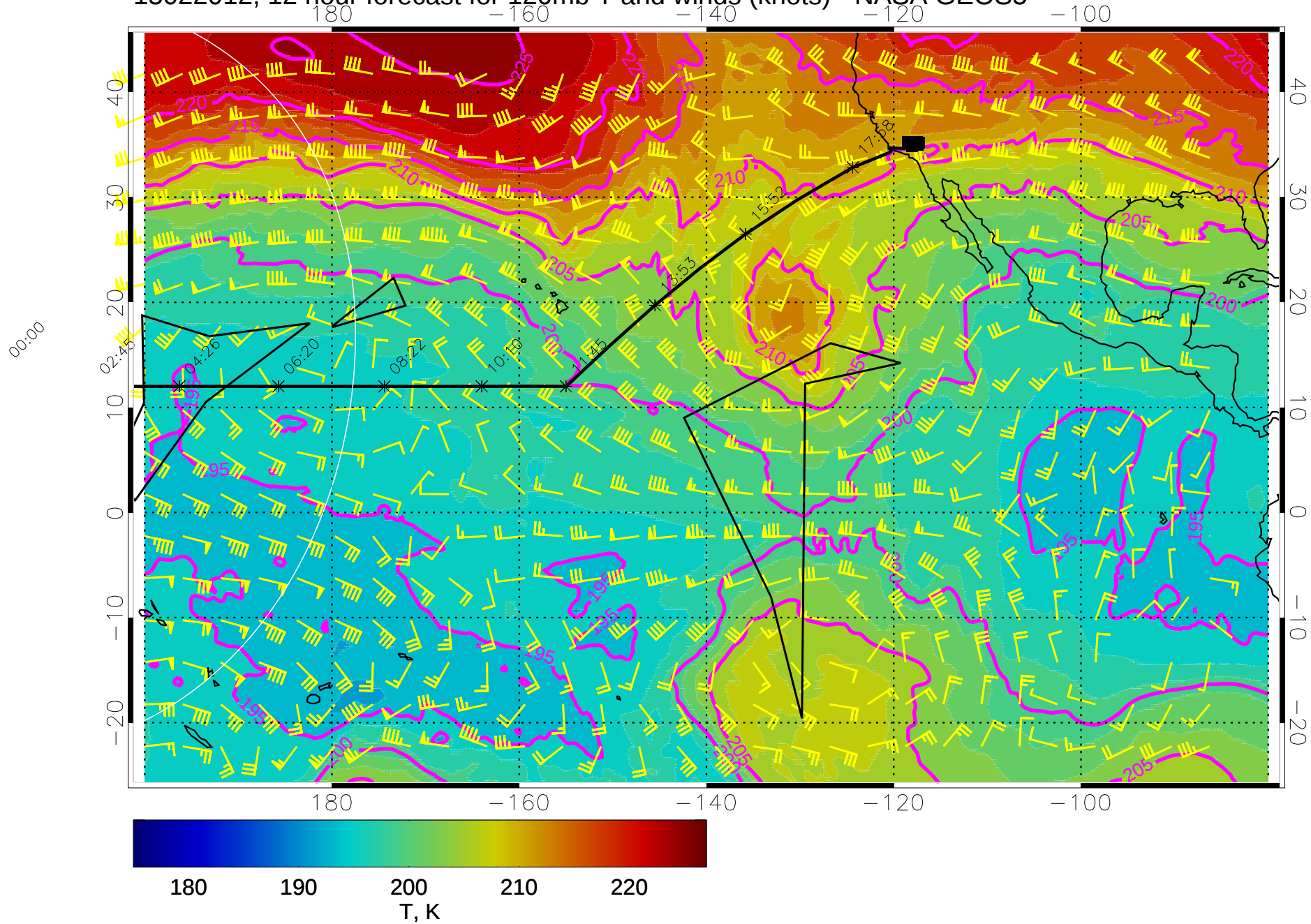
15022012, 12 hour forecast for 120mb T and winds (knots) - NASA GEOS5
