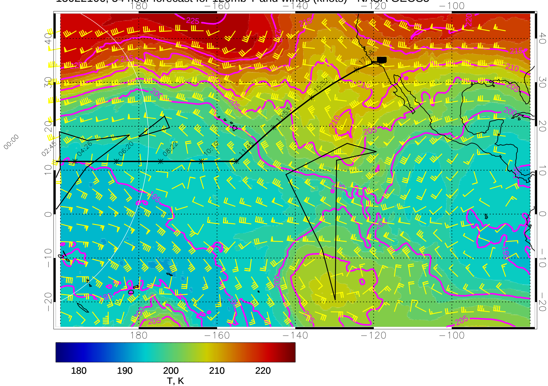
15022106, 54 hour forecast for 120mb T and winds (knots) - NASA GEOS5
