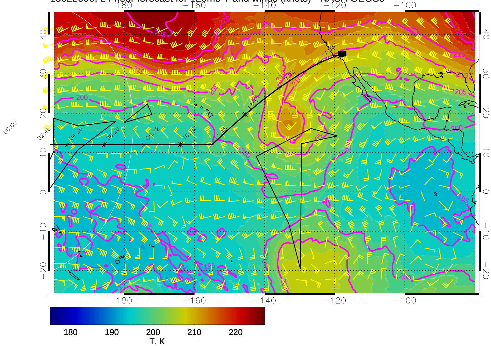
15022000, 24 hour forecast for 120mb T and winds (knots) - NASA GEOS5
