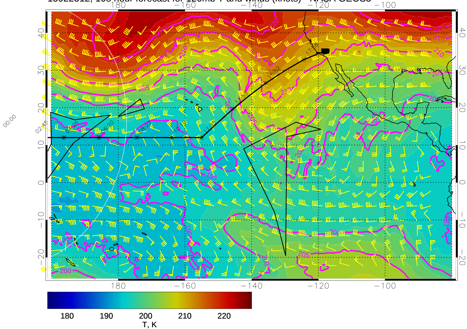
15022312, 108 hour forecast for 120mb T and winds (knots) - NASA GEOS5
