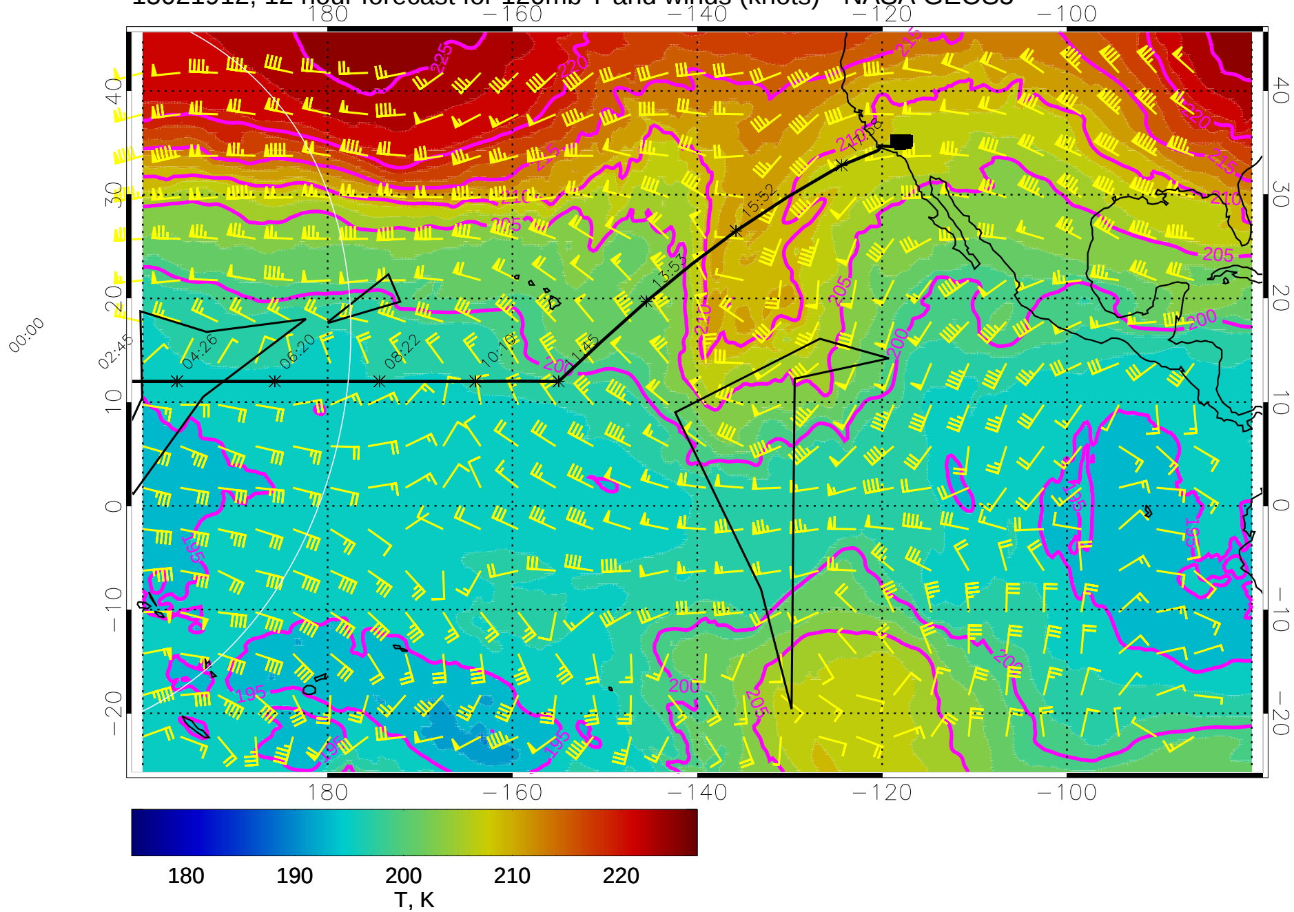
15021912, 12 hour forecast for 120mb T and winds (knots) - NASA GEOS5
