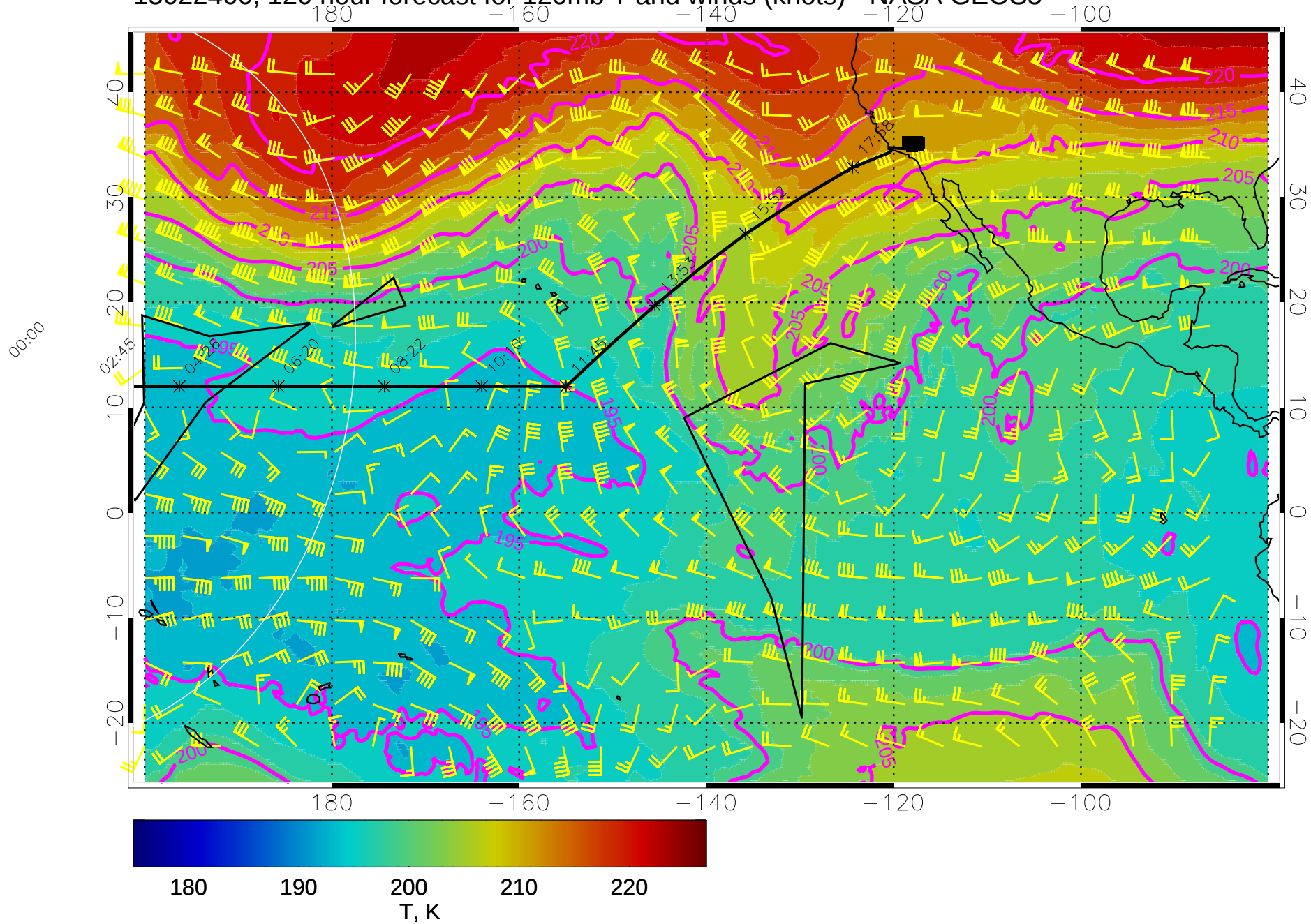
15022400, 120 hour forecast for 120mb T and winds (knots) - NASA GEOS5
