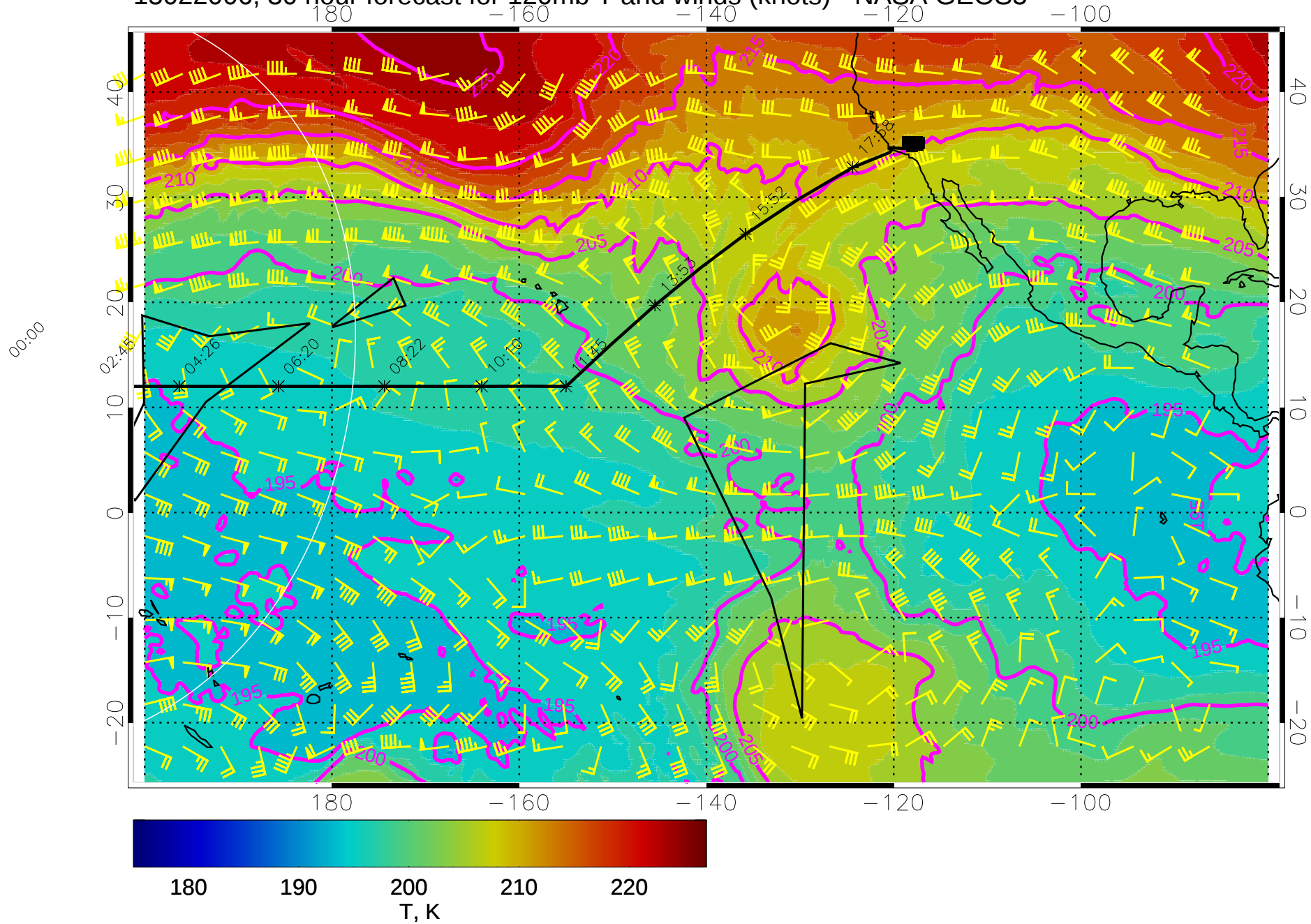
15022006, 30 hour forecast for 120mb T and winds (knots) - NASA GEOS5
