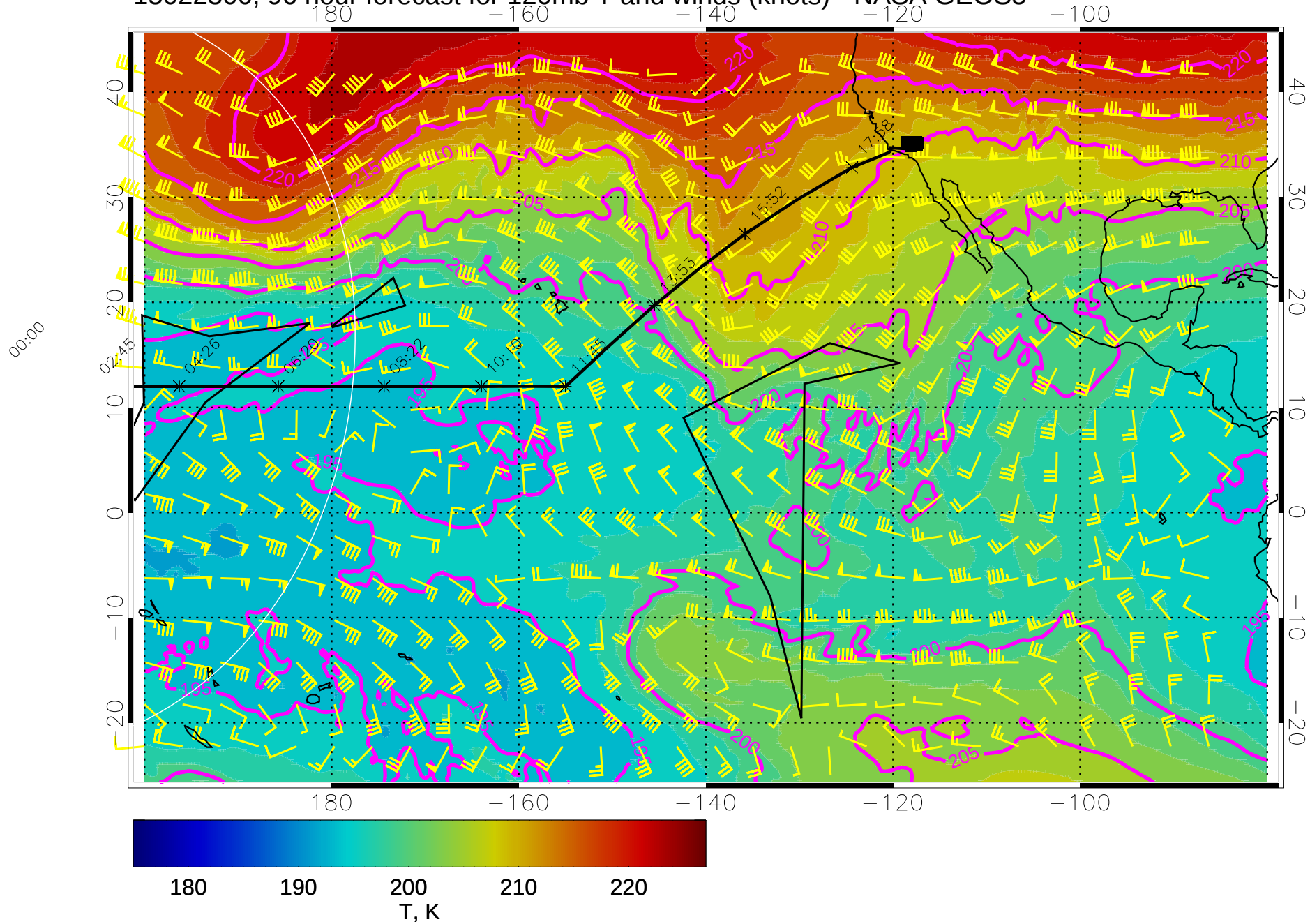
15022300, 96 hour forecast for 120mb T and winds (knots) - NASA GEOS5
