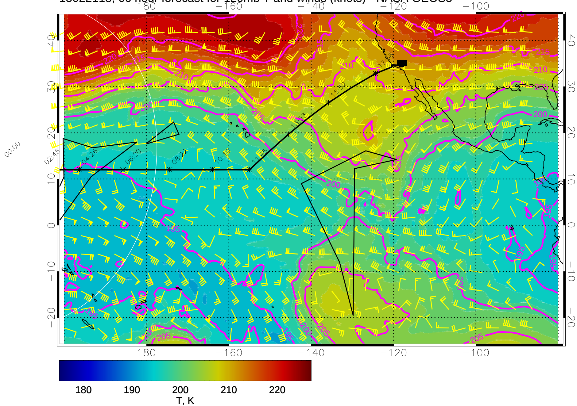
15022118, 66 hour forecast for 120mb T and winds (knots) - NASA GEOS5
