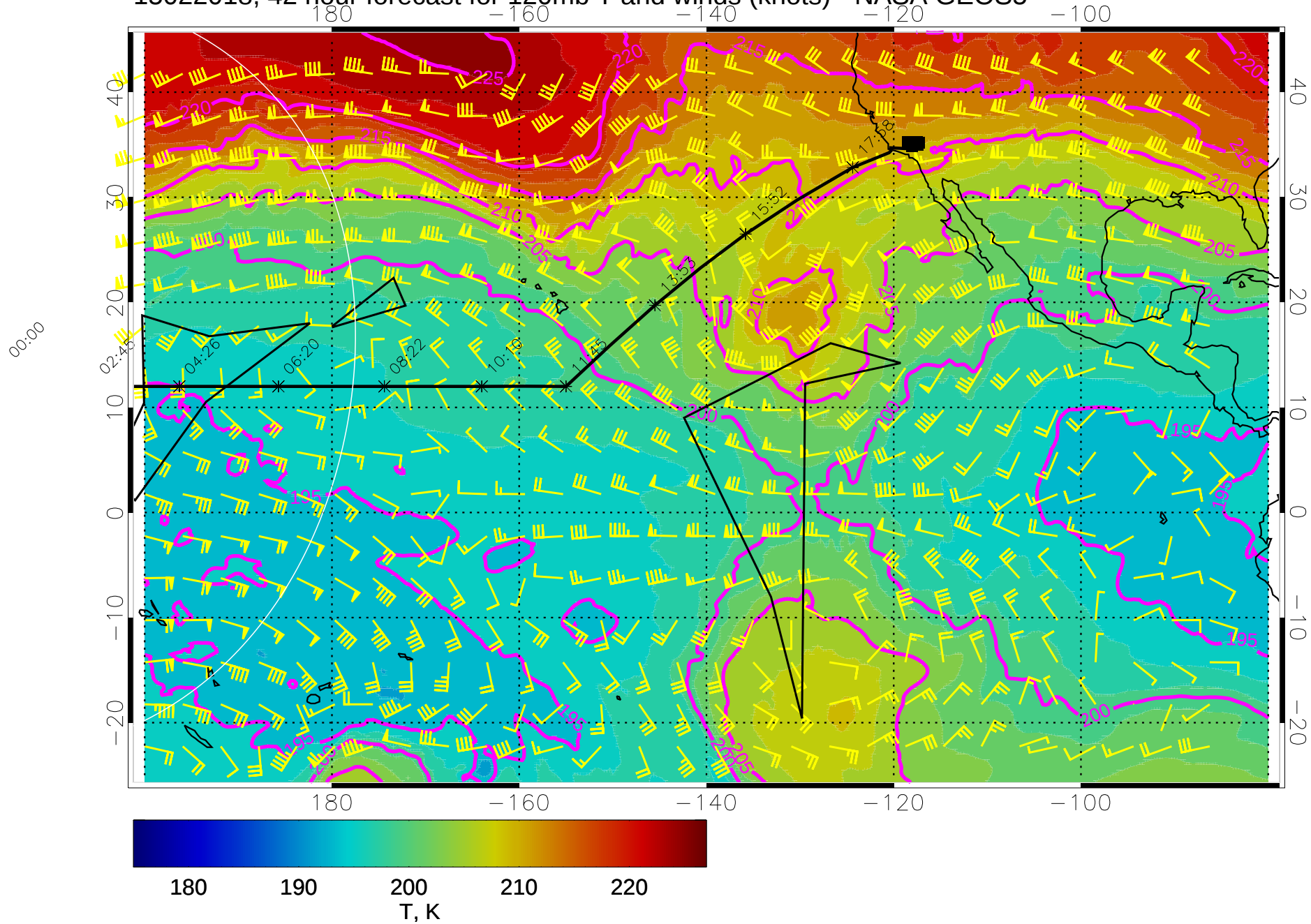
15022018, 42 hour forecast for 120mb T and winds (knots) - NASA GEOS5
