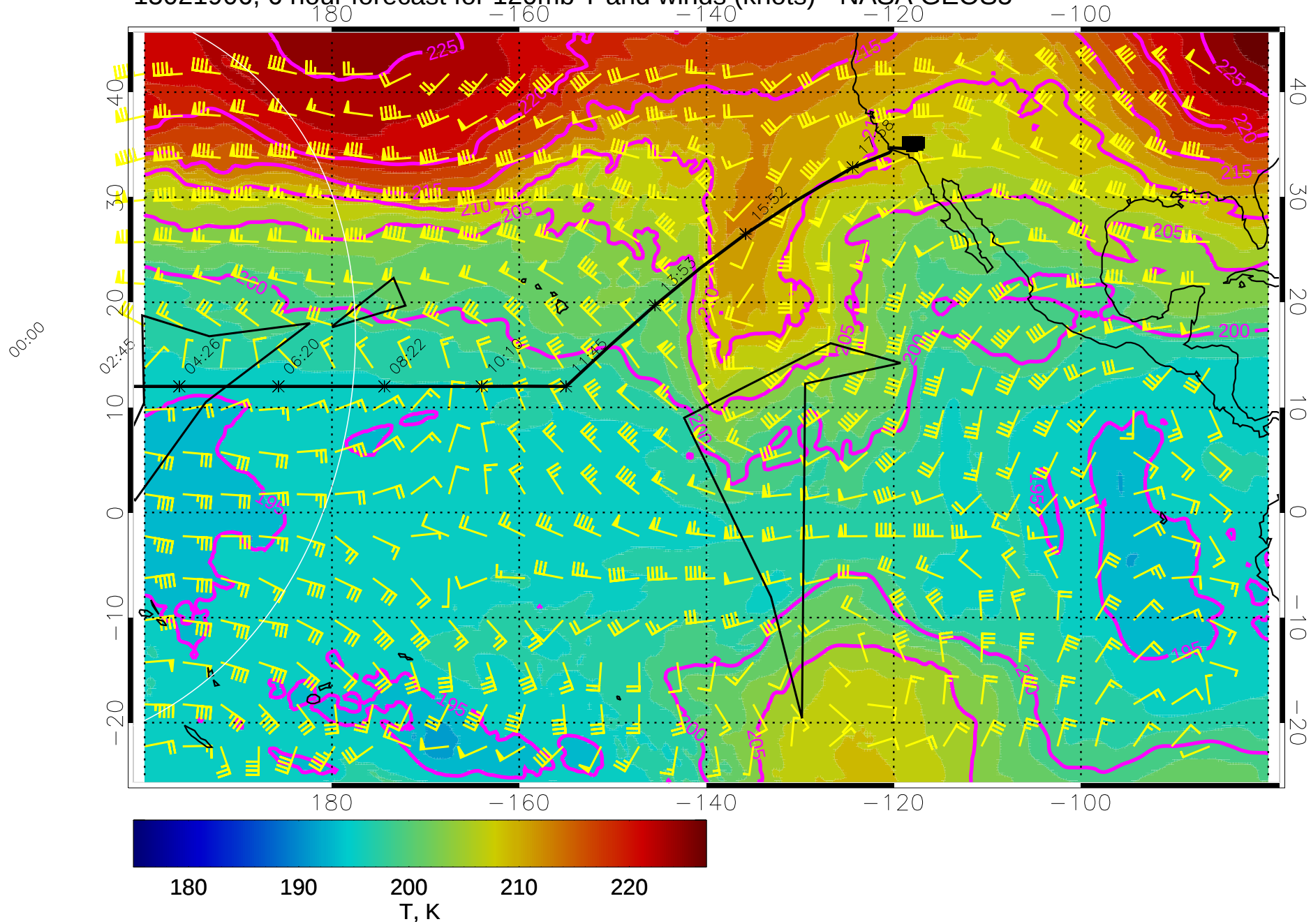
15021906, 6 hour forecast for 120mb T and winds (knots) - NASA GEOS5
