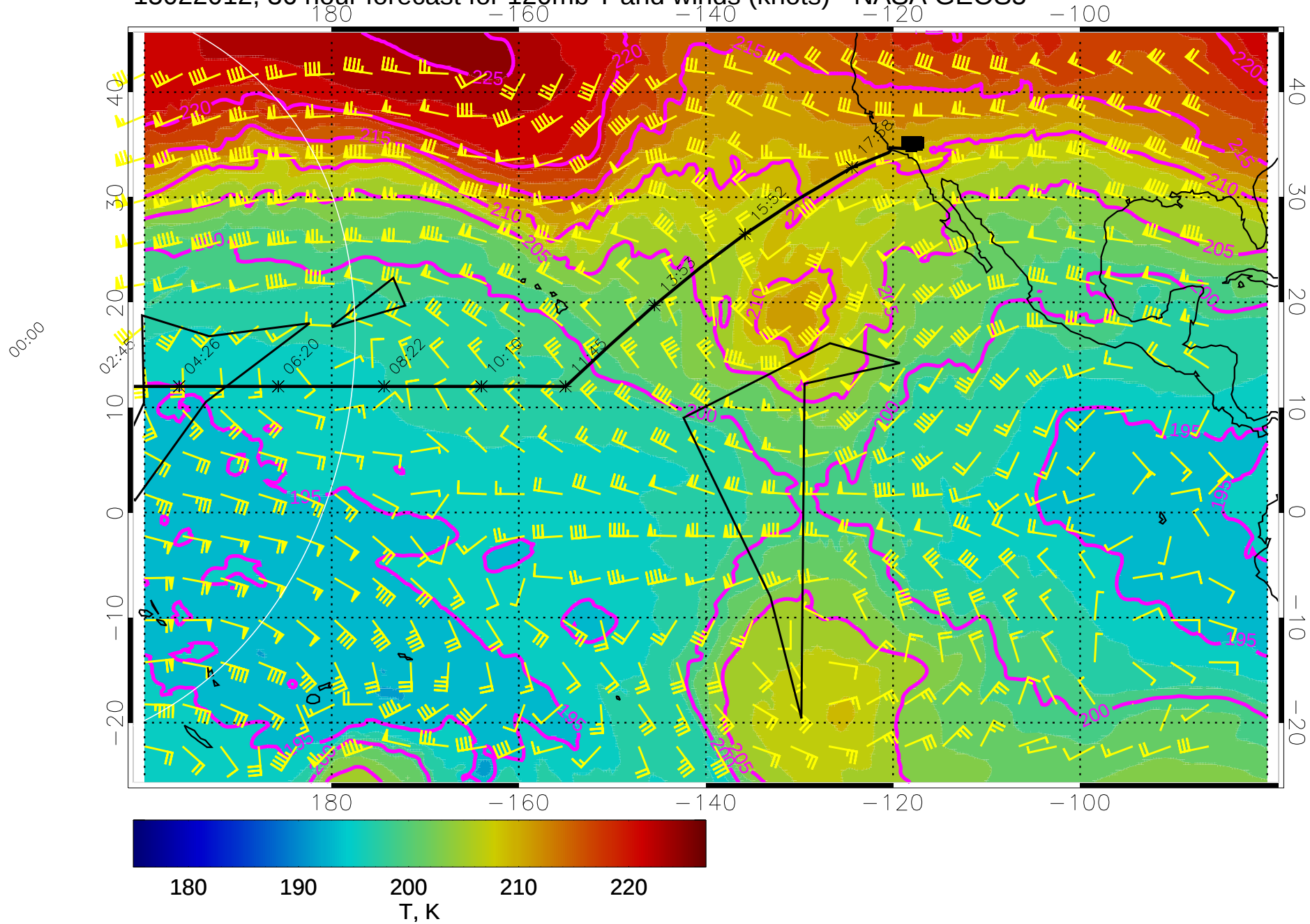
15022012, 36 hour forecast for 120mb T and winds (knots) - NASA GEOS5
