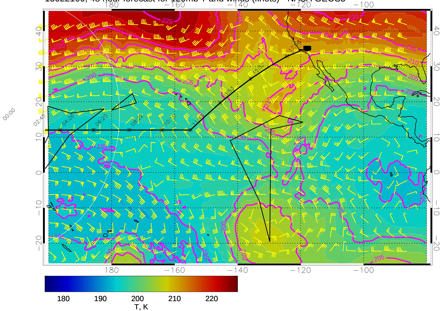
15022100, 48 hour forecast for 120mb T and winds (knots) - NASA GEOS5
