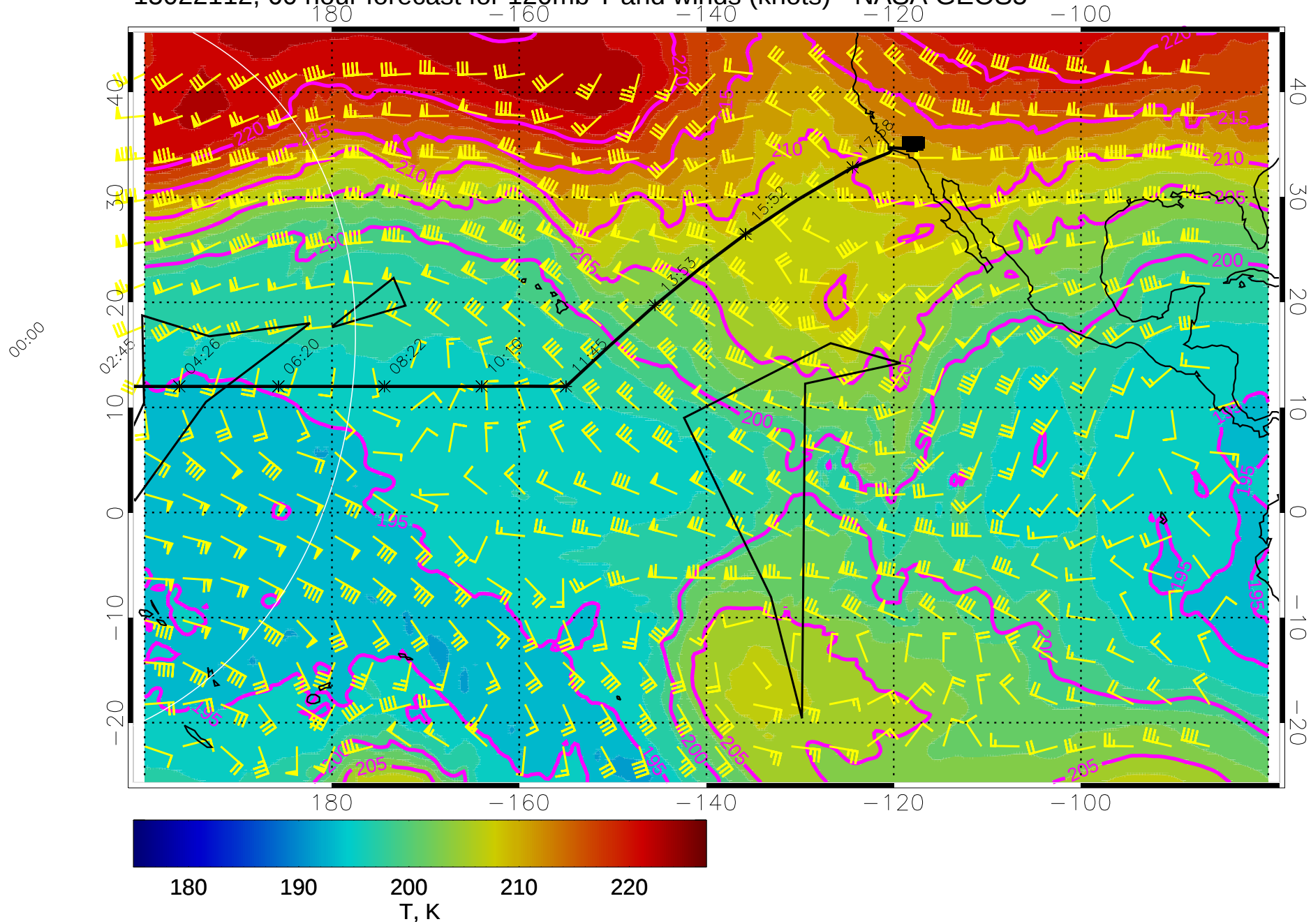
15022112, 60 hour forecast for 120mb T and winds (knots) - NASA GEOS5
