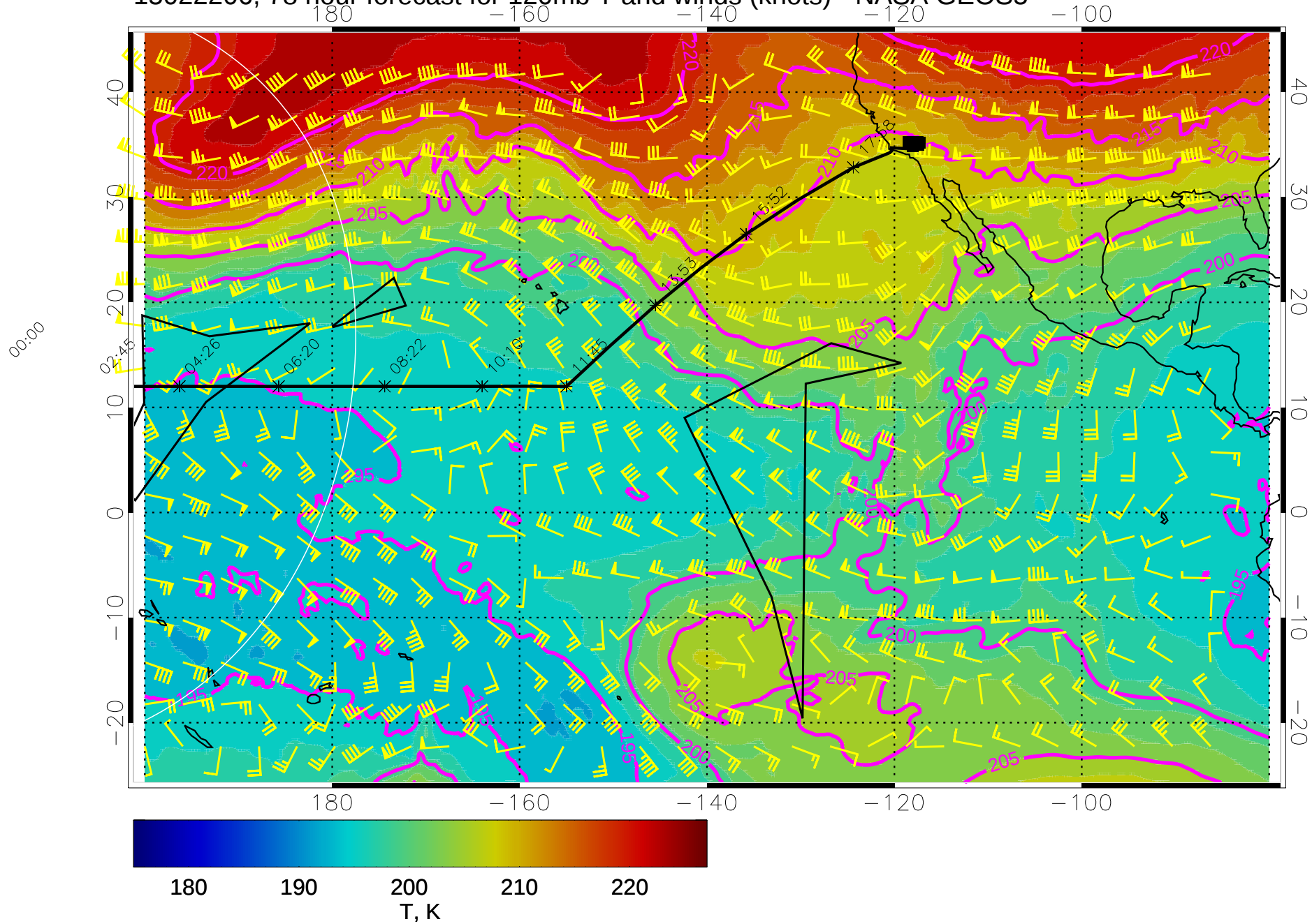
15022206, 78 hour forecast for 120mb T and winds (knots) - NASA GEOS5
