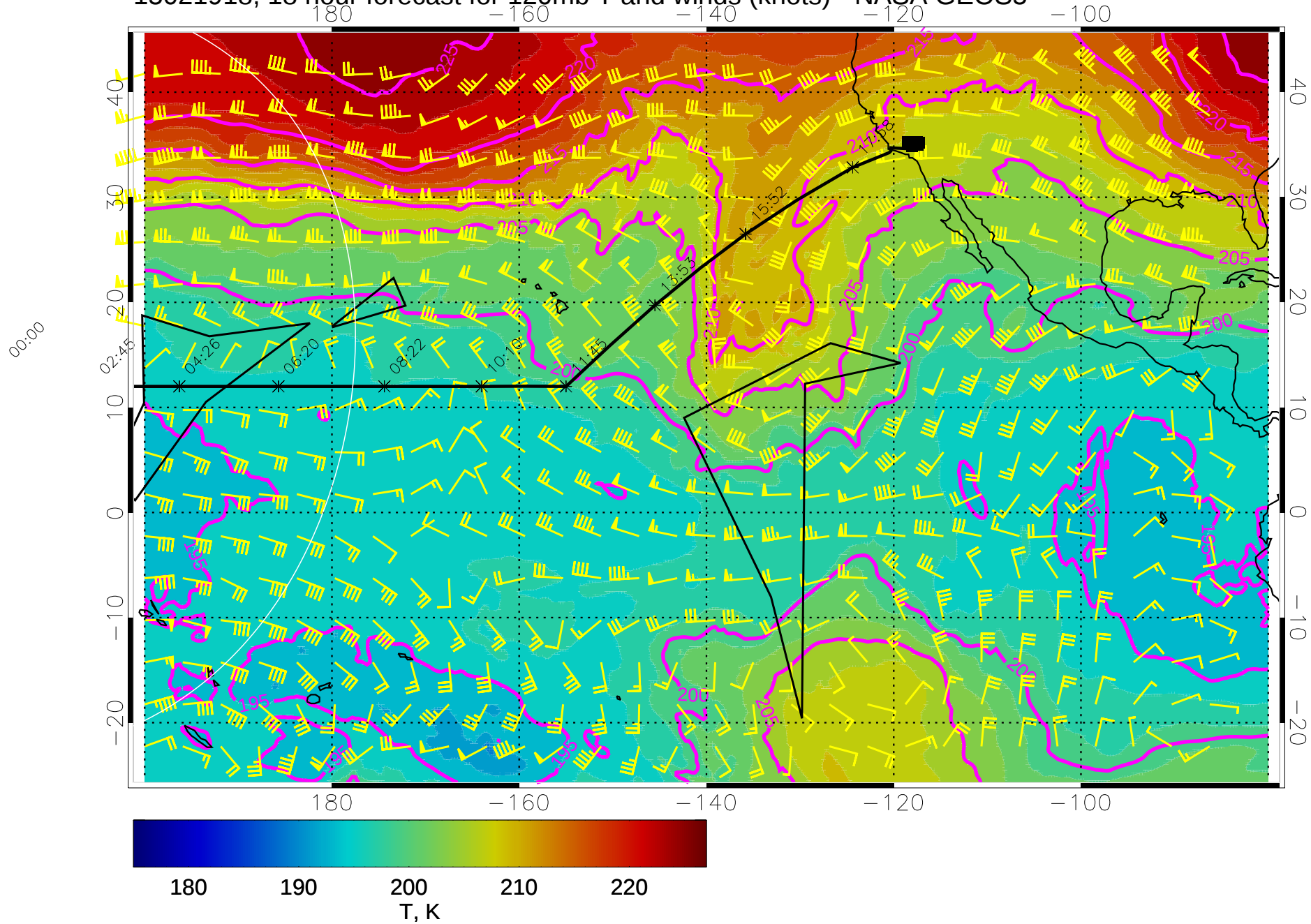
15021918, 18 hour forecast for 120mb T and winds (knots) - NASA GEOS5
