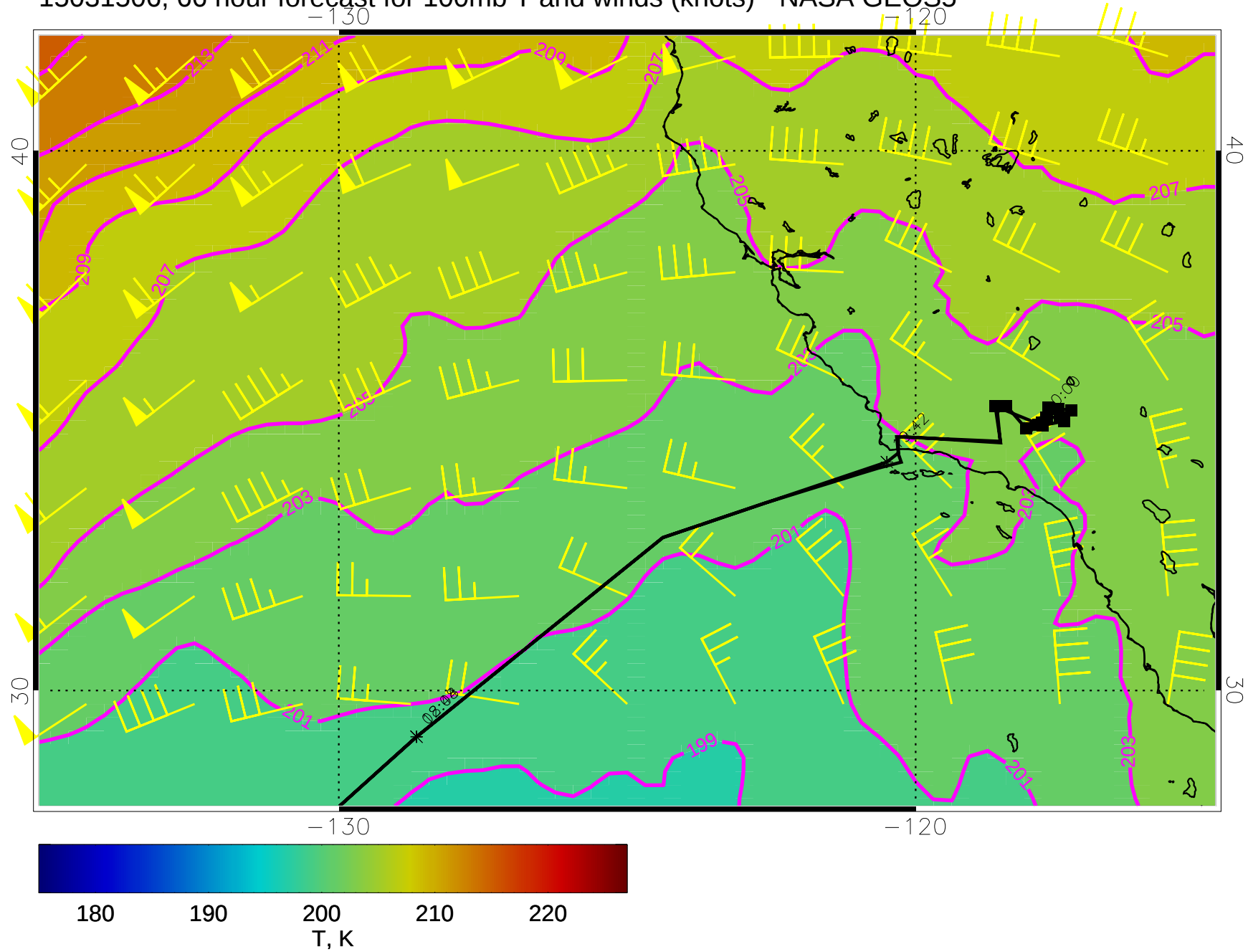
15031506, 66 hour forecast for 100mb T and winds (knots) - NASA GEOS5
