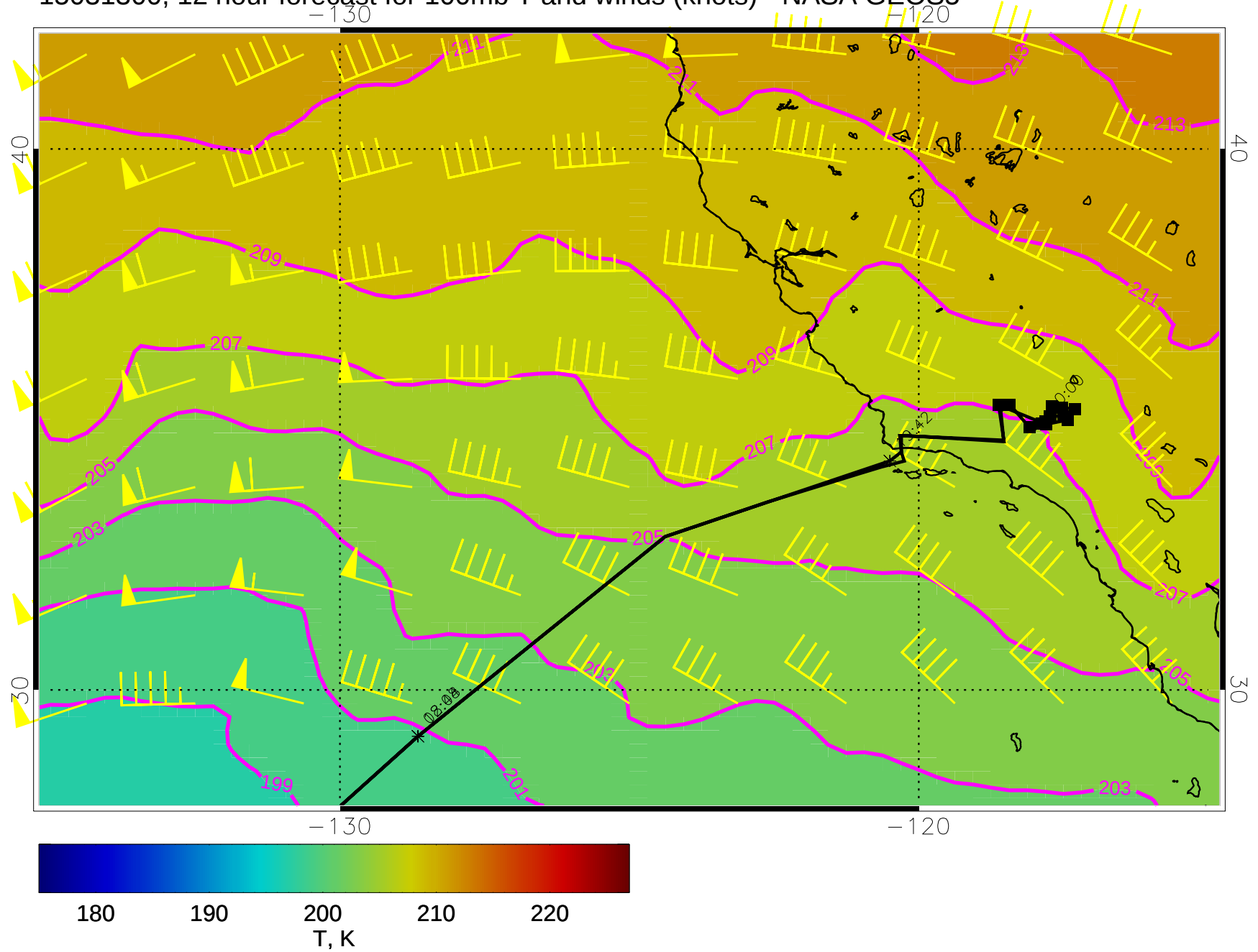
15031300, 12 hour forecast for 100mb T and winds (knots) - NASA GEOS5
