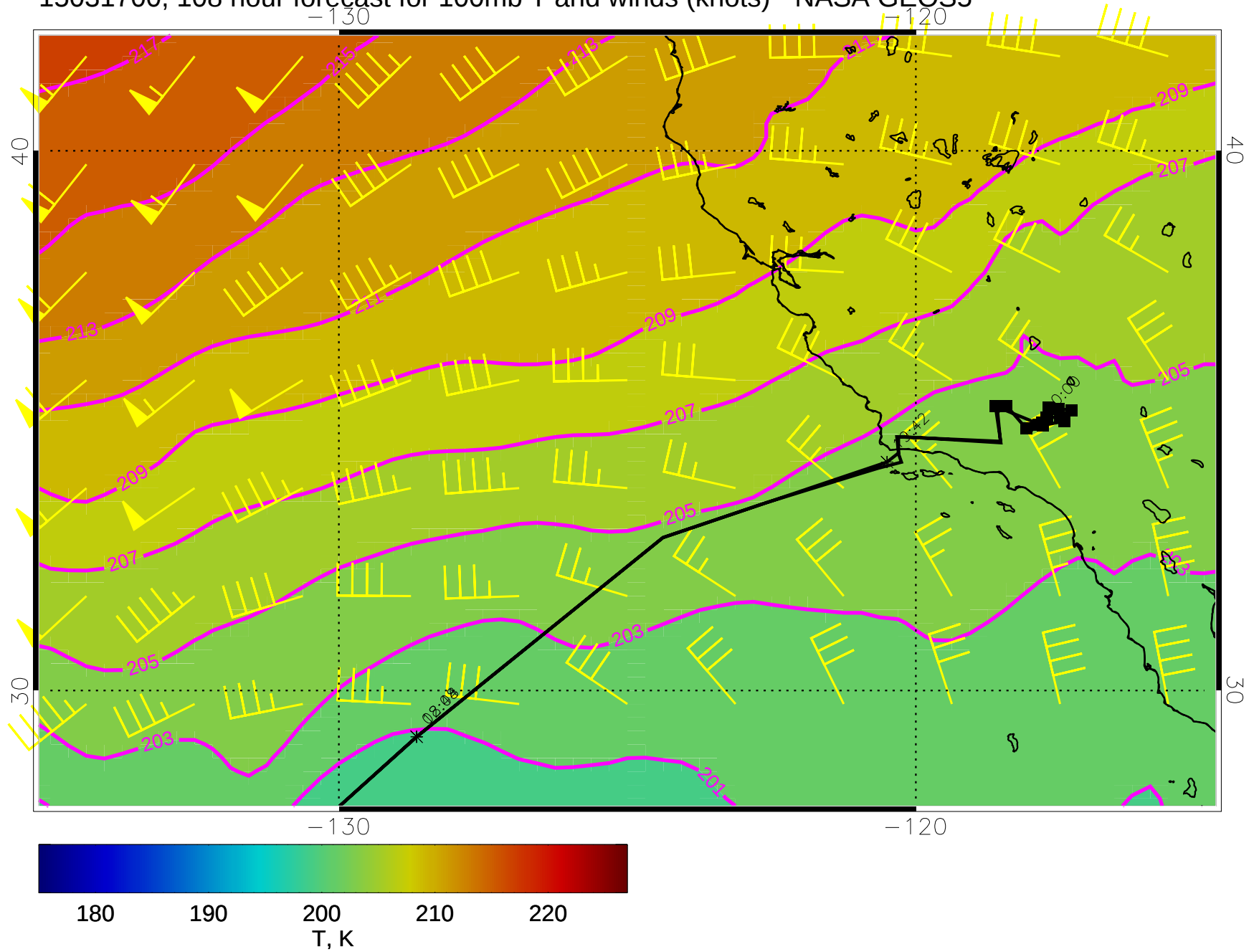
15031700, 108 hour forecast for 100mb T and winds (knots) - NASA GEOS5
