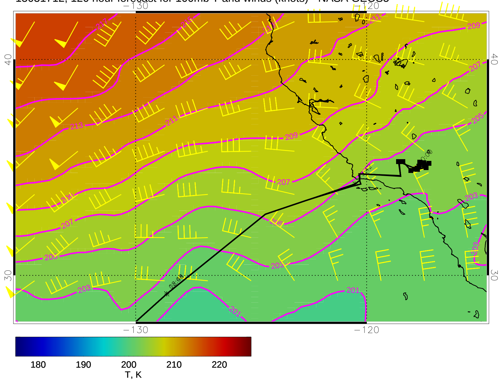
15031712, 120 hour forecast for 100mb T and winds (knots) - NASA GEOS5
