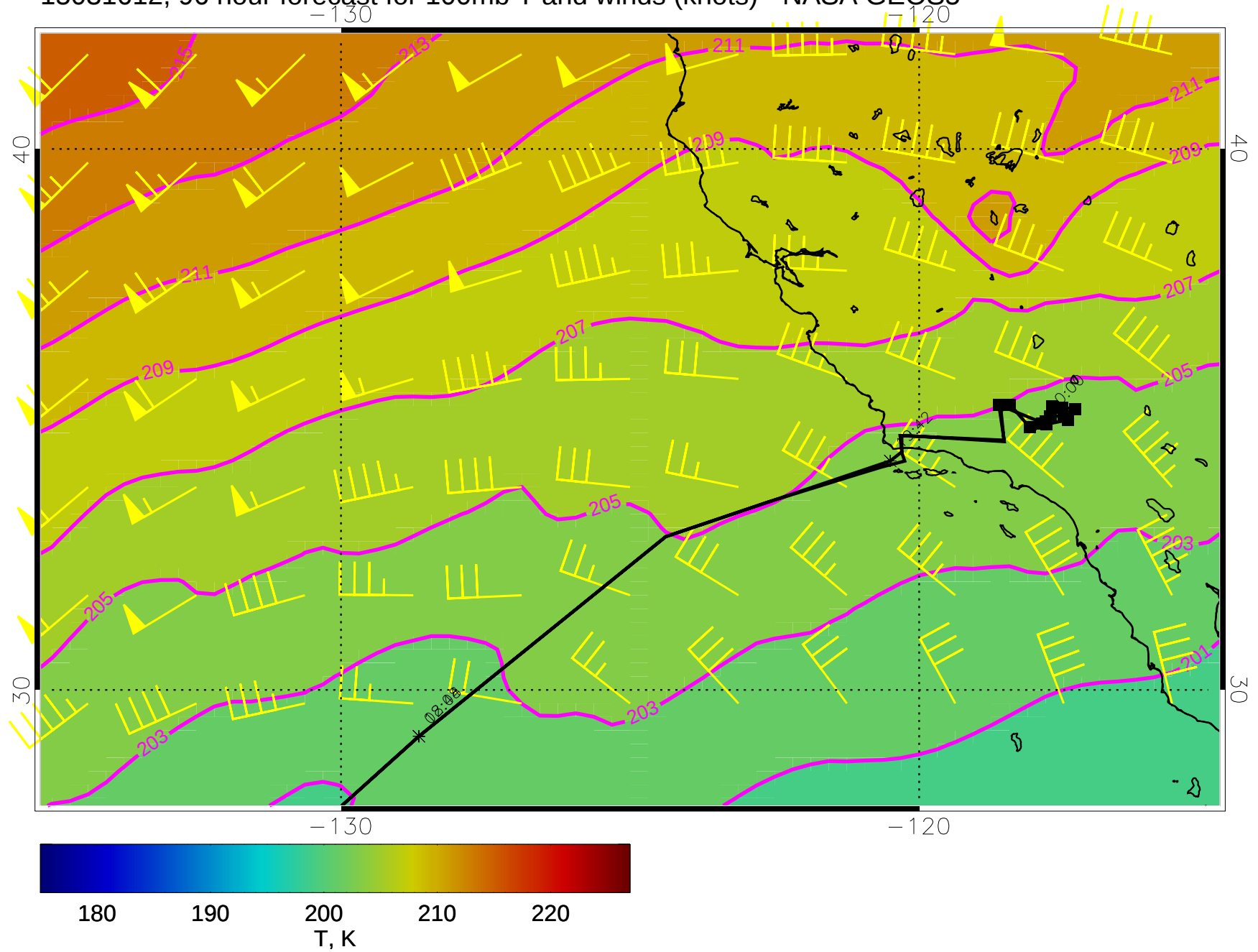
15031612, 96 hour forecast for 100mb T and winds (knots) - NASA GEOS5
