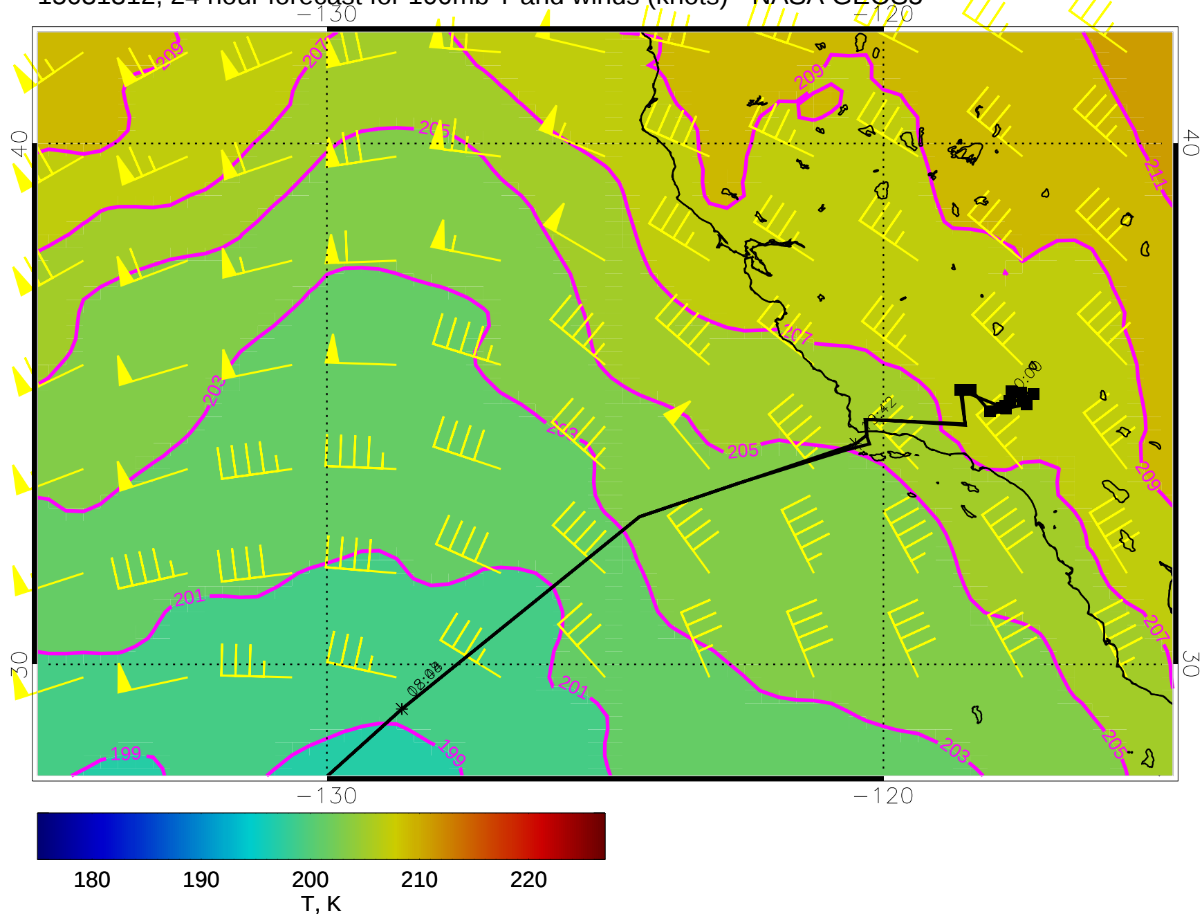
15031312, 24 hour forecast for 100mb T and winds (knots) - NASA GEOS5
