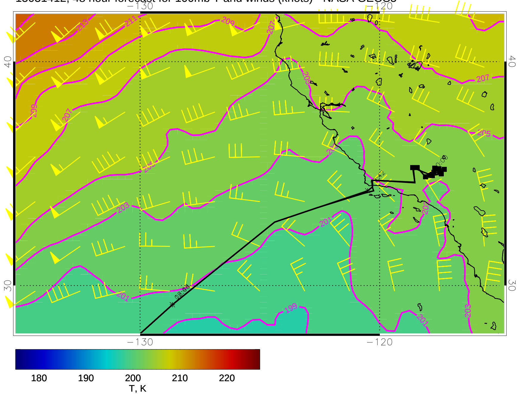
15031412, 48 hour forecast for 100mb T and winds (knots) - NASA GEOS5
