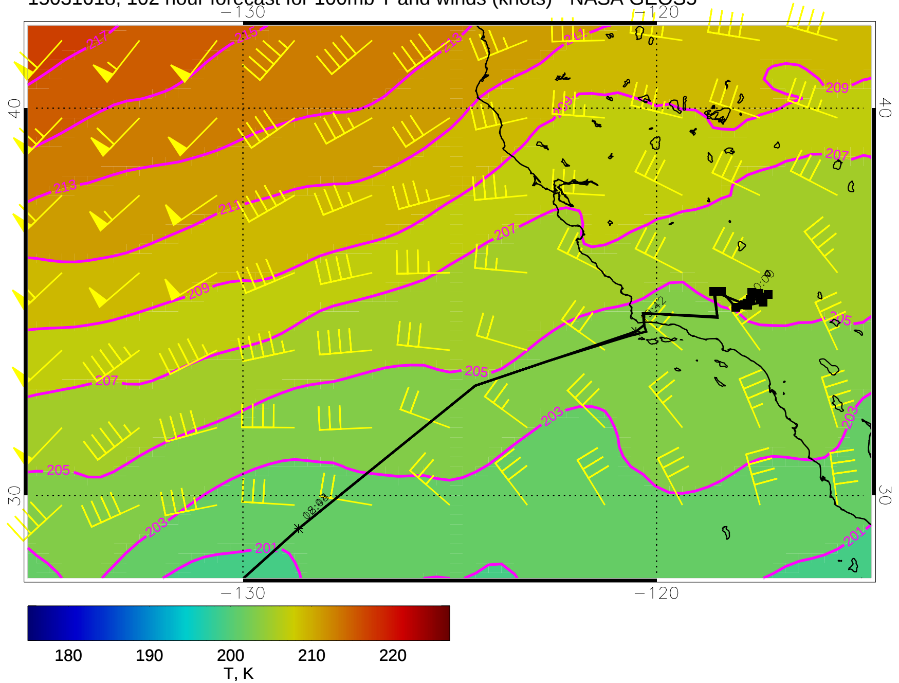
15031618, 102 hour forecast for 100mb T and winds (knots) - NASA GEOS5
