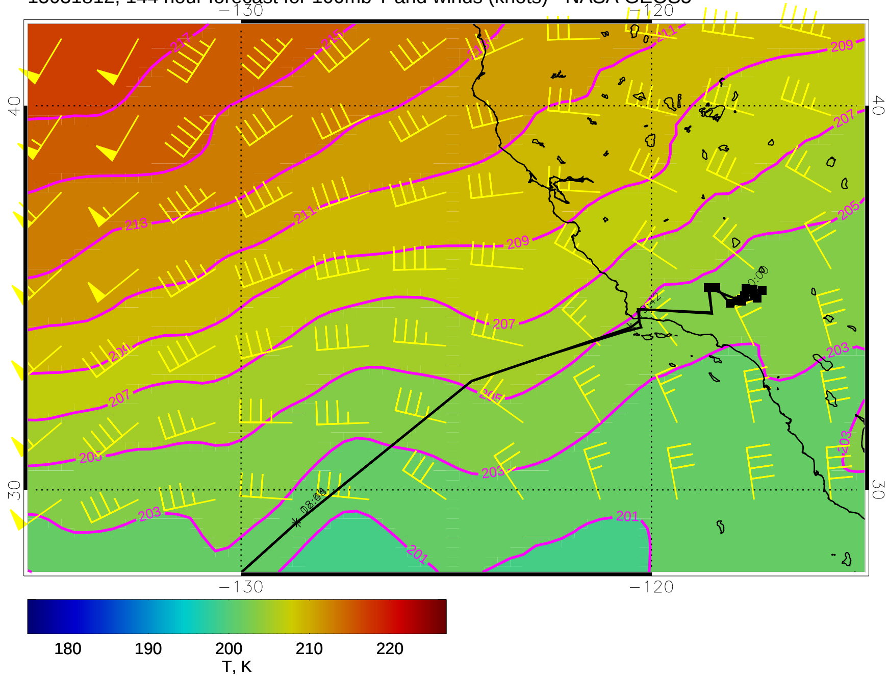
15031812, 144 hour forecast for 100mb T and winds (knots) - NASA GEOS5
