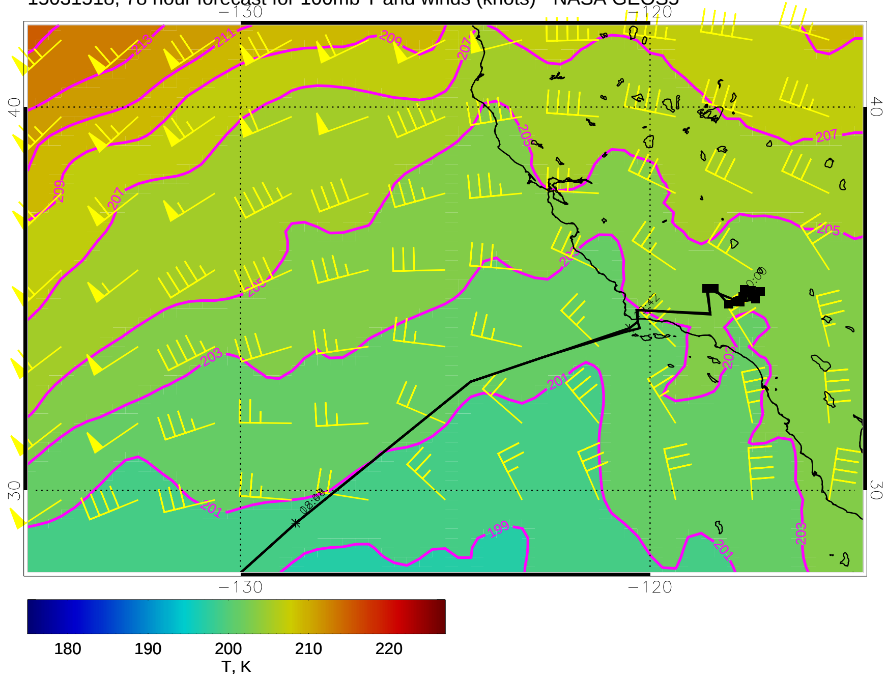
15031518, 78 hour forecast for 100mb T and winds (knots) - NASA GEOS5
