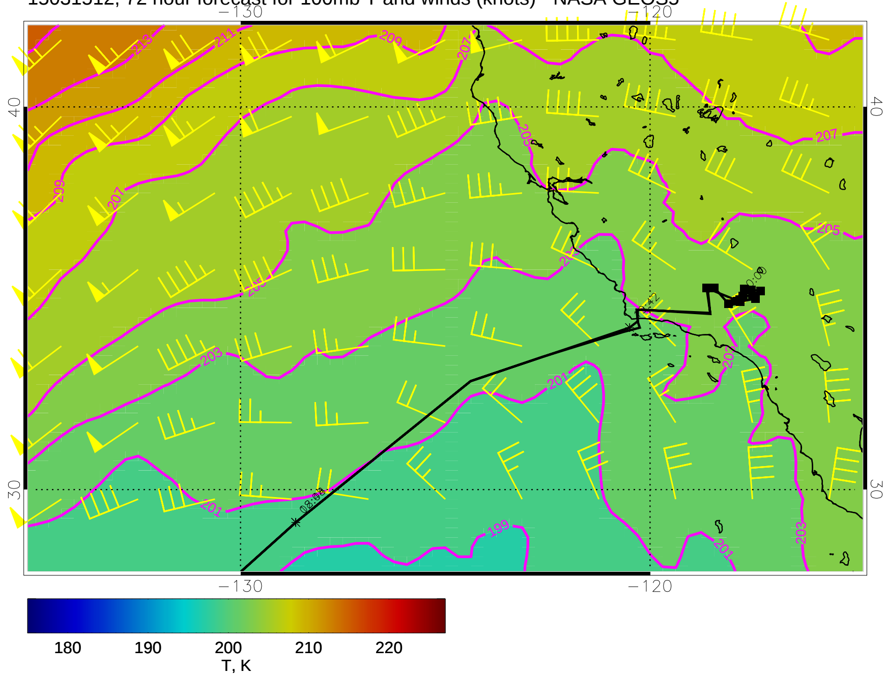
15031512, 72 hour forecast for 100mb T and winds (knots) - NASA GEOS5
