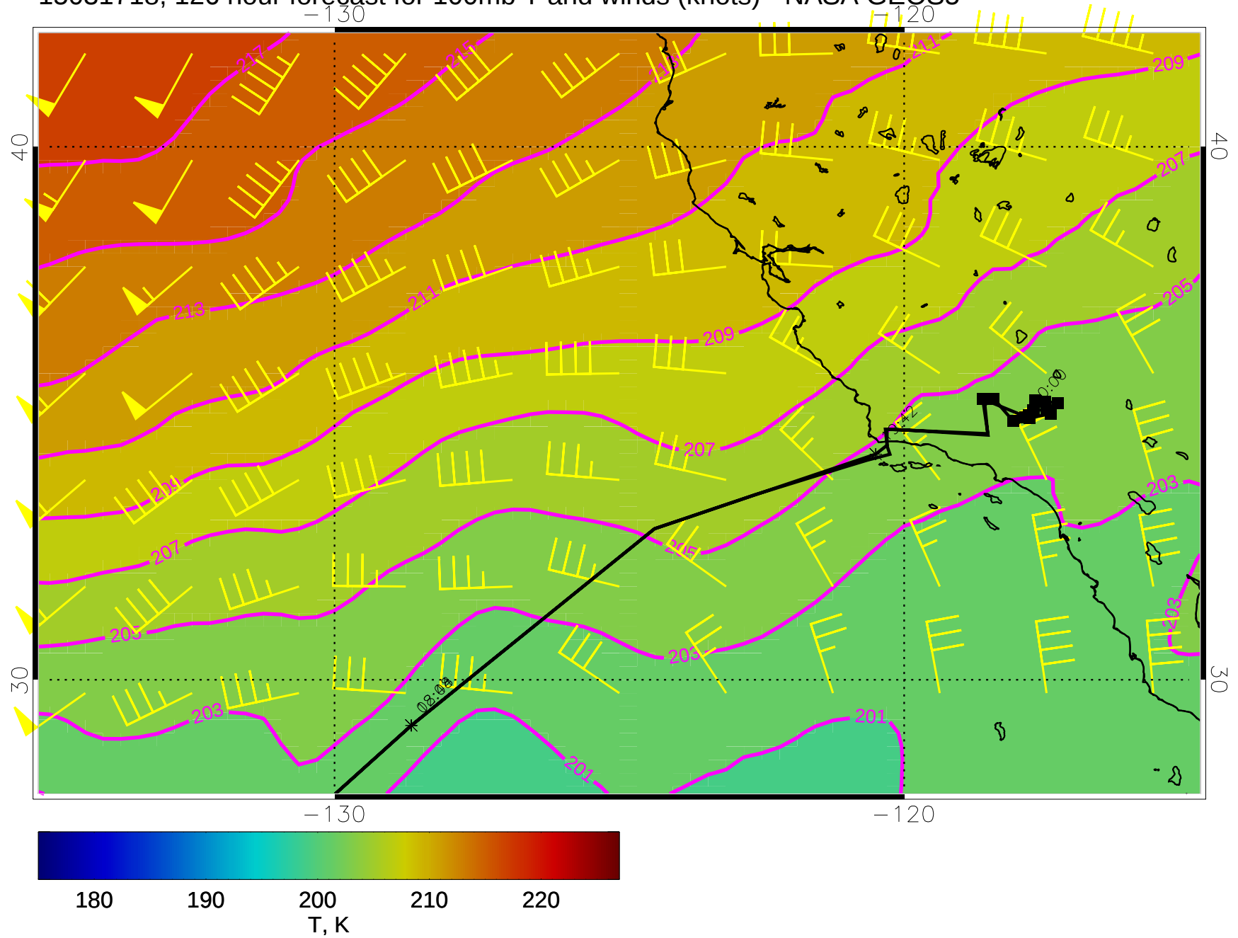
15031718, 126 hour forecast for 100mb T and winds (knots) - NASA GEOS5
