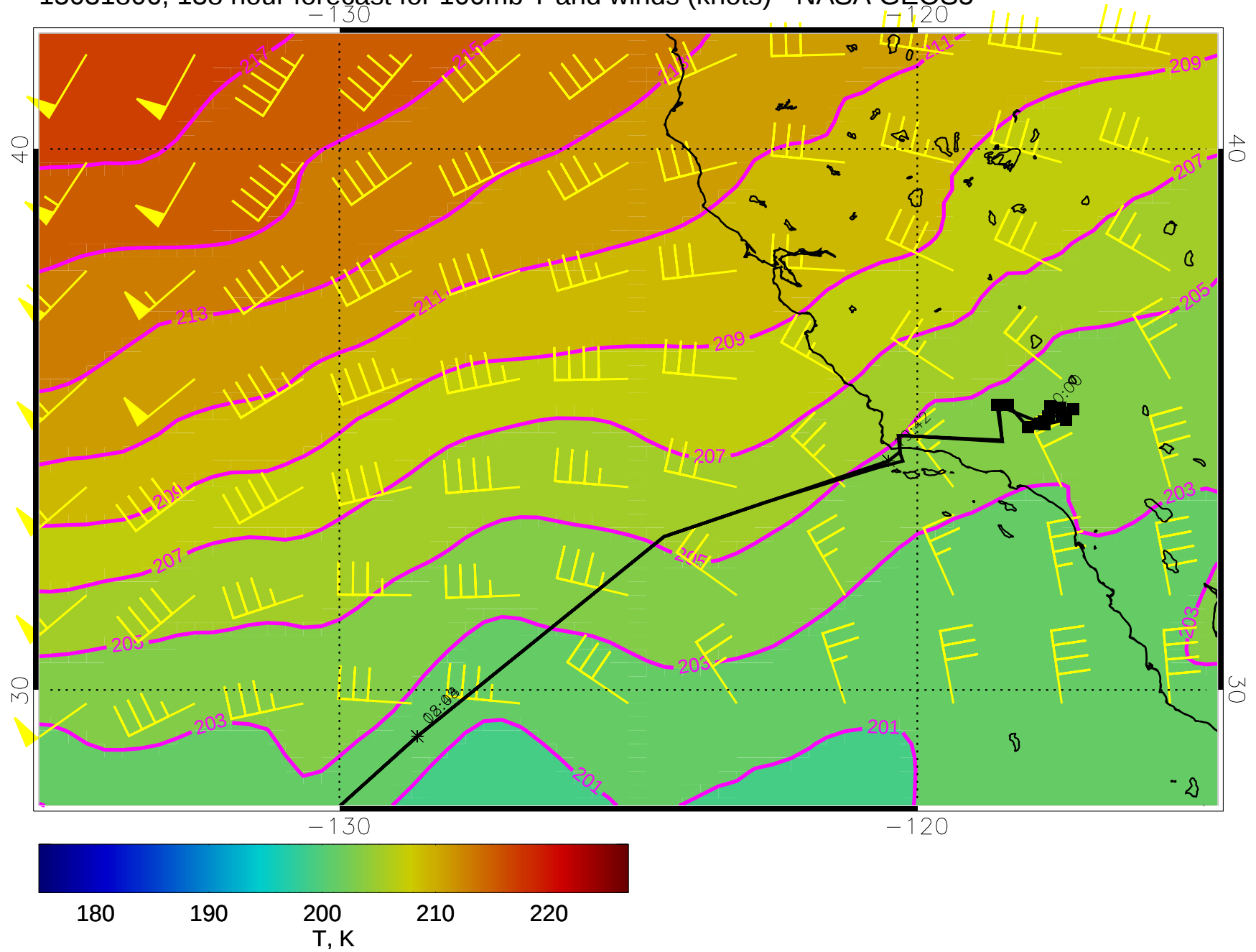
15031806, 138 hour forecast for 100mb T and winds (knots) - NASA GEOS5
