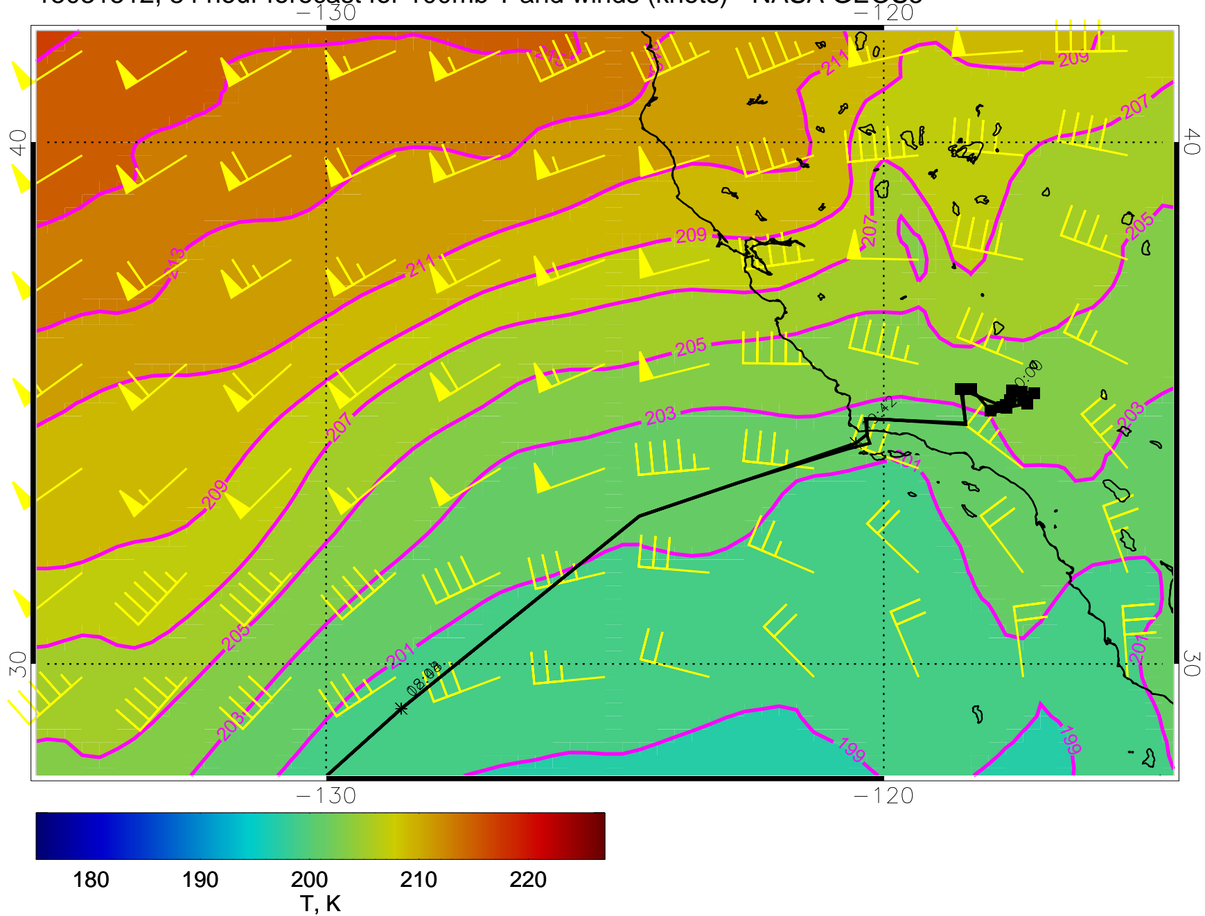
15031512, 84 hour forecast for 100mb T and winds (knots) - NASA GEOS5
