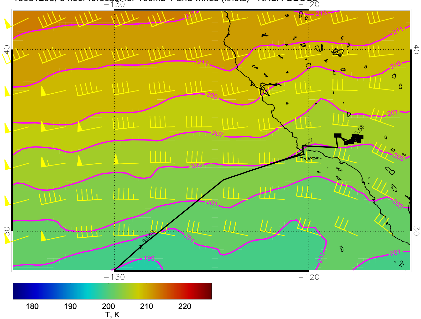
15031206, 6 hour forecast for 100mb T and winds (knots) - NASA GEOS5
