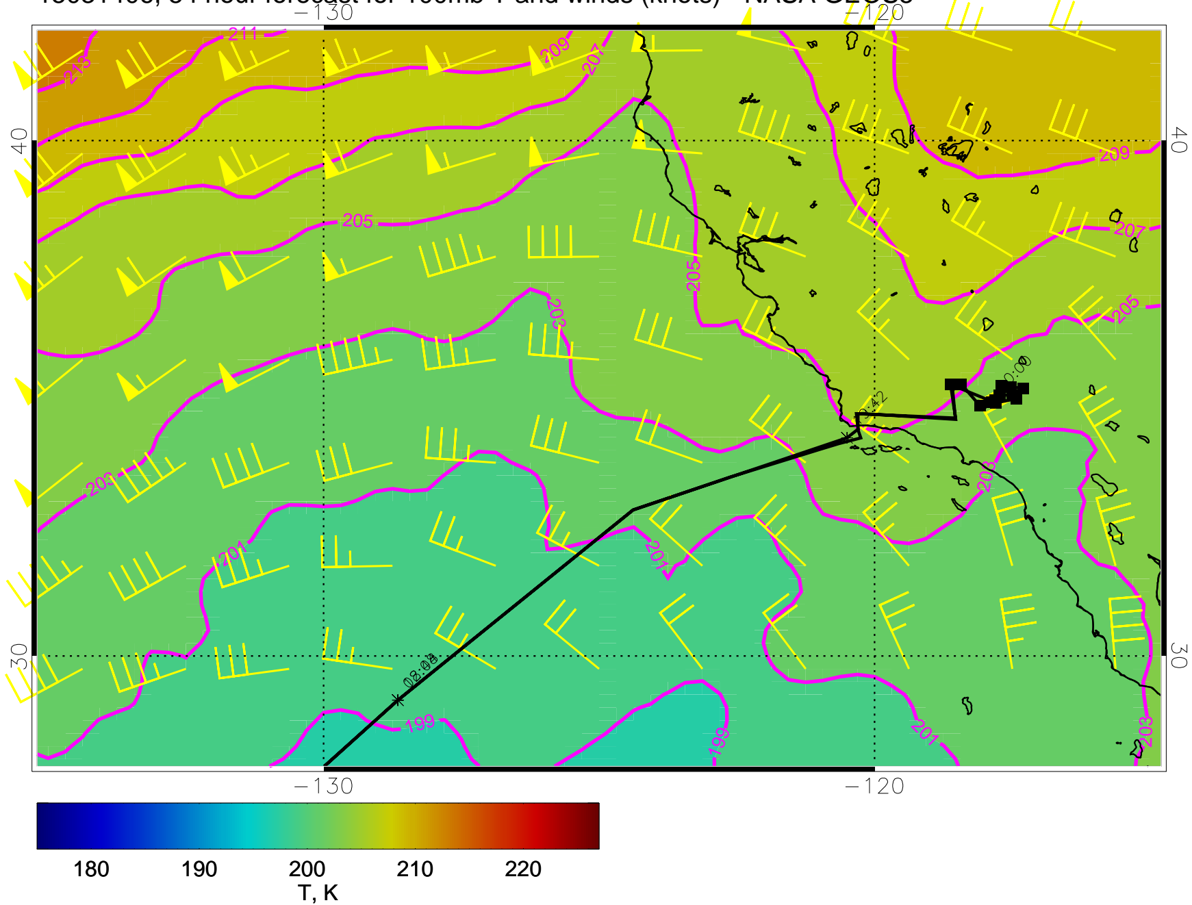
15031406, 54 hour forecast for 100mb T and winds (knots) - NASA GEOS5
