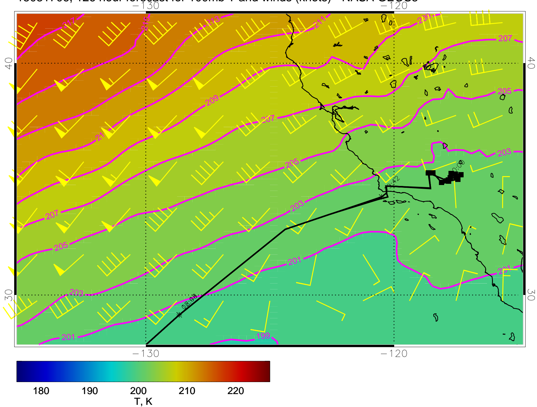
15031706, 126 hour forecast for 100mb T and winds (knots) - NASA GEOS5
