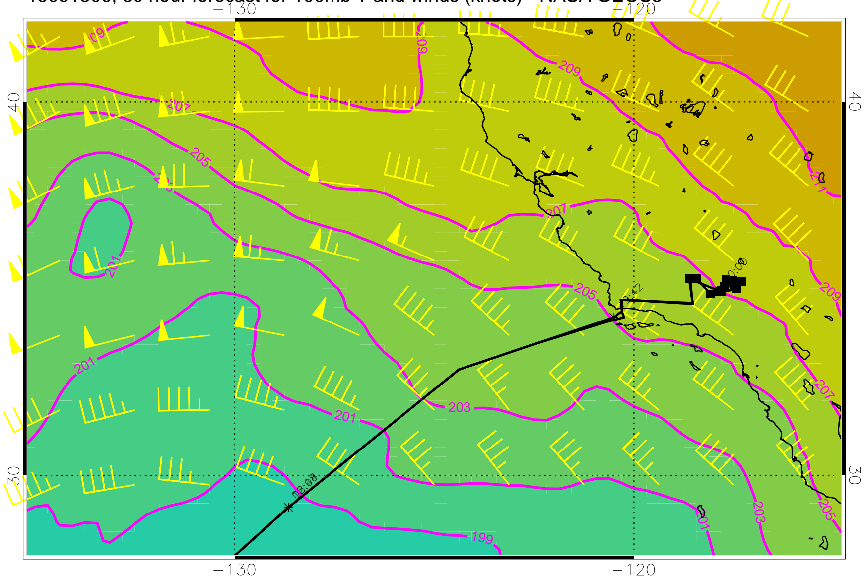
15031306, 30 hour forecast for 100mb T and winds (knots) - NASA GEOS5
