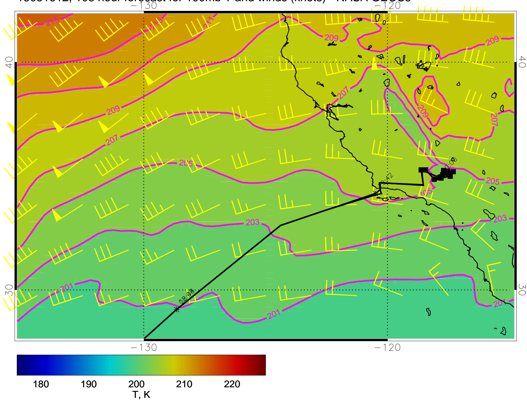
15031612, 108 hour forecast for 100mb T and winds (knots) - NASA GEOS5
