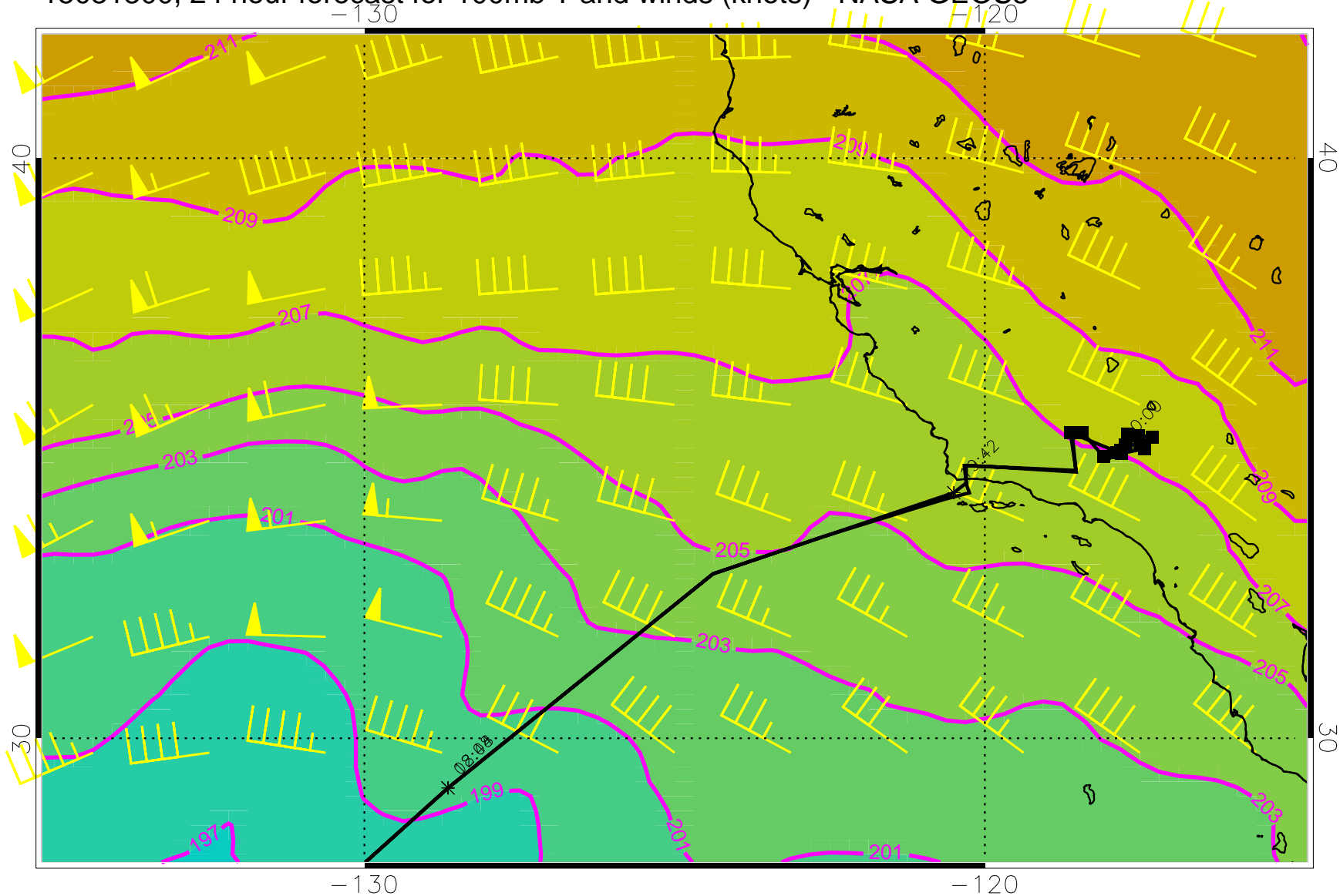
15031300, 24 hour forecast for 100mb T and winds (knots) - NASA GEOS5
