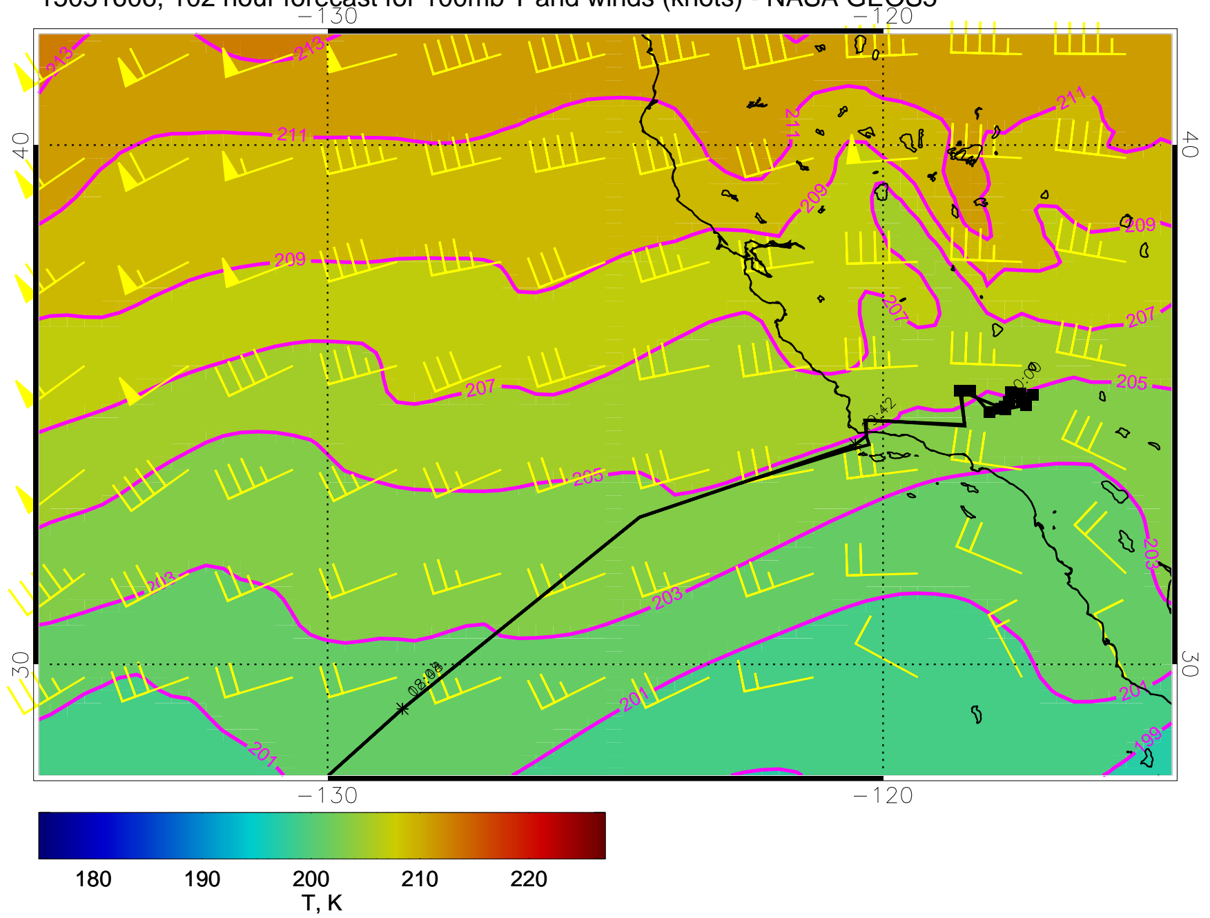
15031606, 102 hour forecast for 100mb T and winds (knots) - NASA GEOS5
