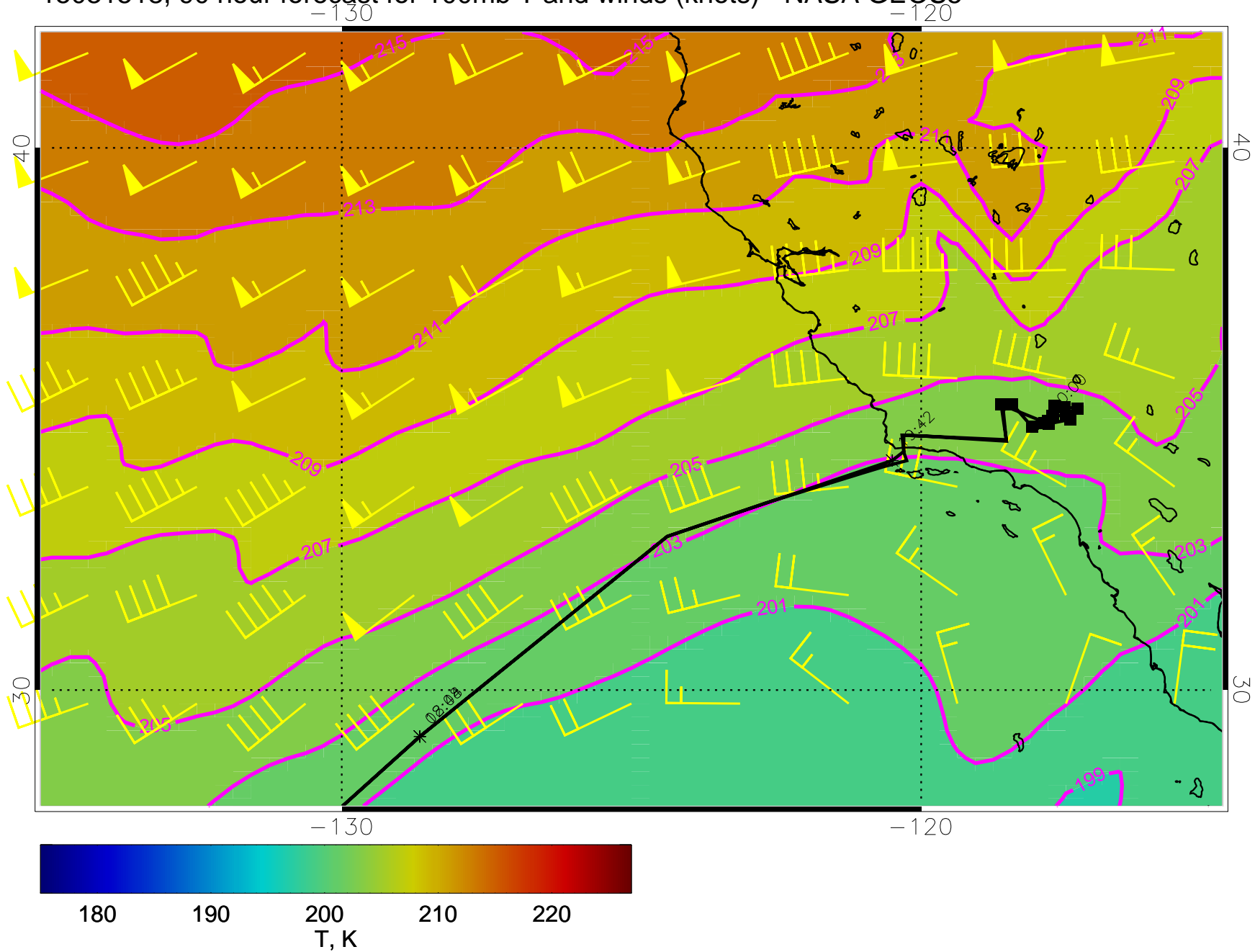
15031518, 90 hour forecast for 100mb T and winds (knots) - NASA GEOS5
