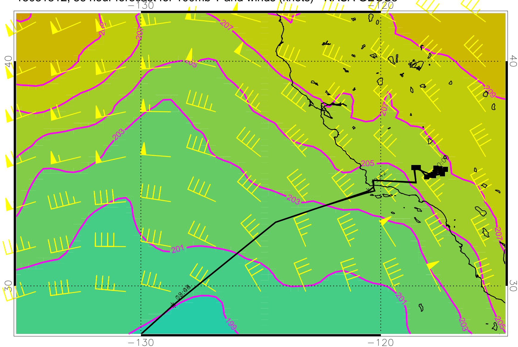
15031312, 36 hour forecast for 100mb T and winds (knots) - NASA GEOS5
