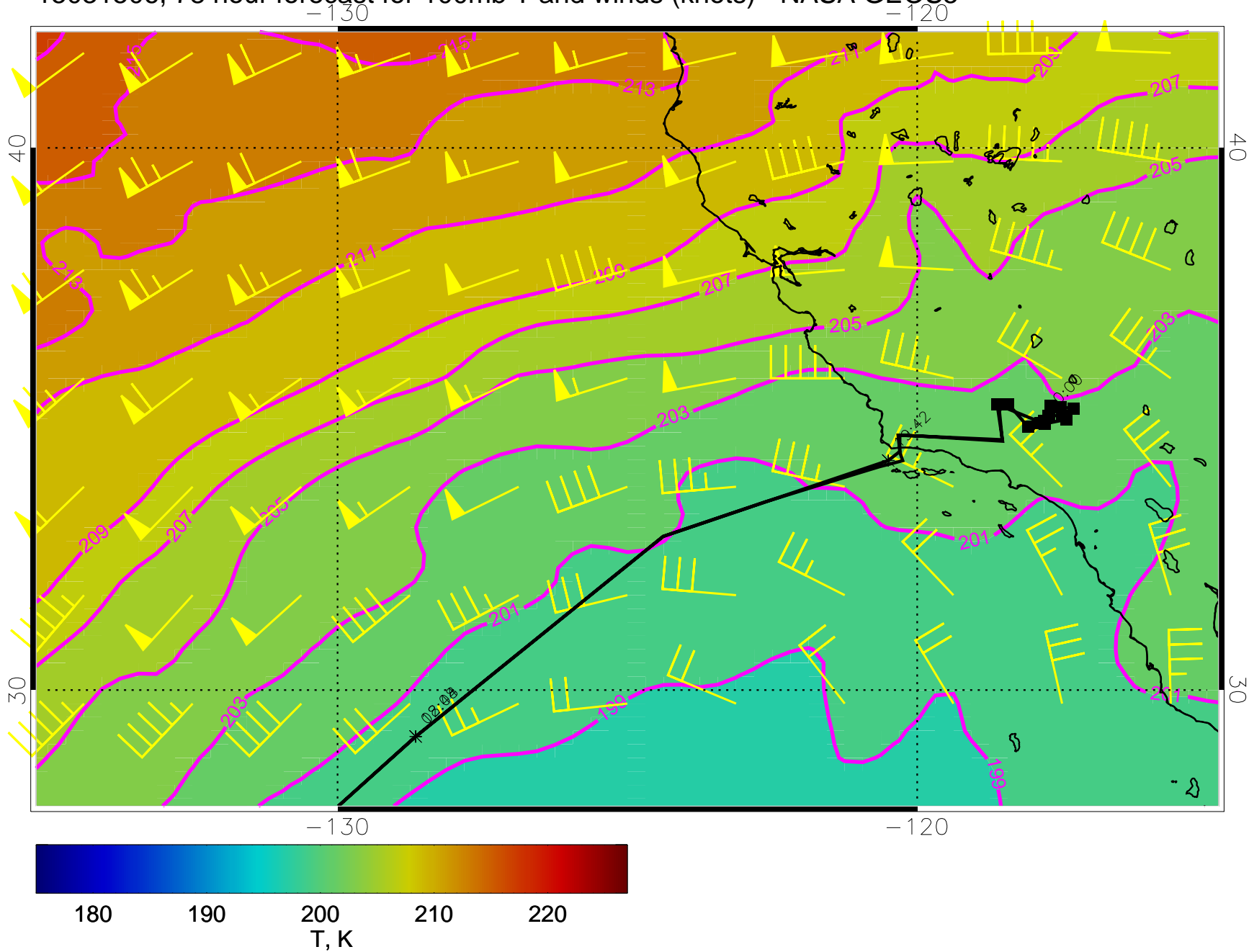
15031506, 78 hour forecast for 100mb T and winds (knots) - NASA GEOS5
