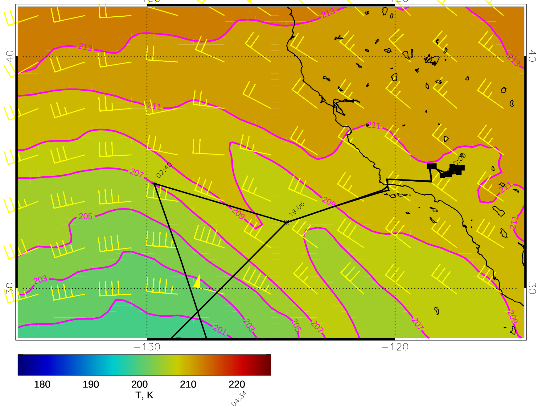
15030906, 6 hour forecast for 100mb T and winds (knots) - NASA GEOS5
