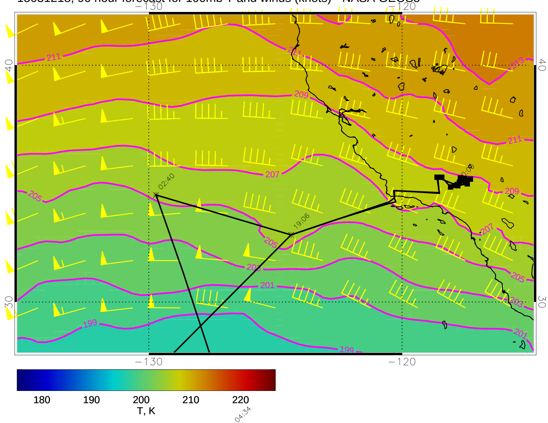
15031218, 90 hour forecast for 100mb T and winds (knots) - NASA GEOS5
