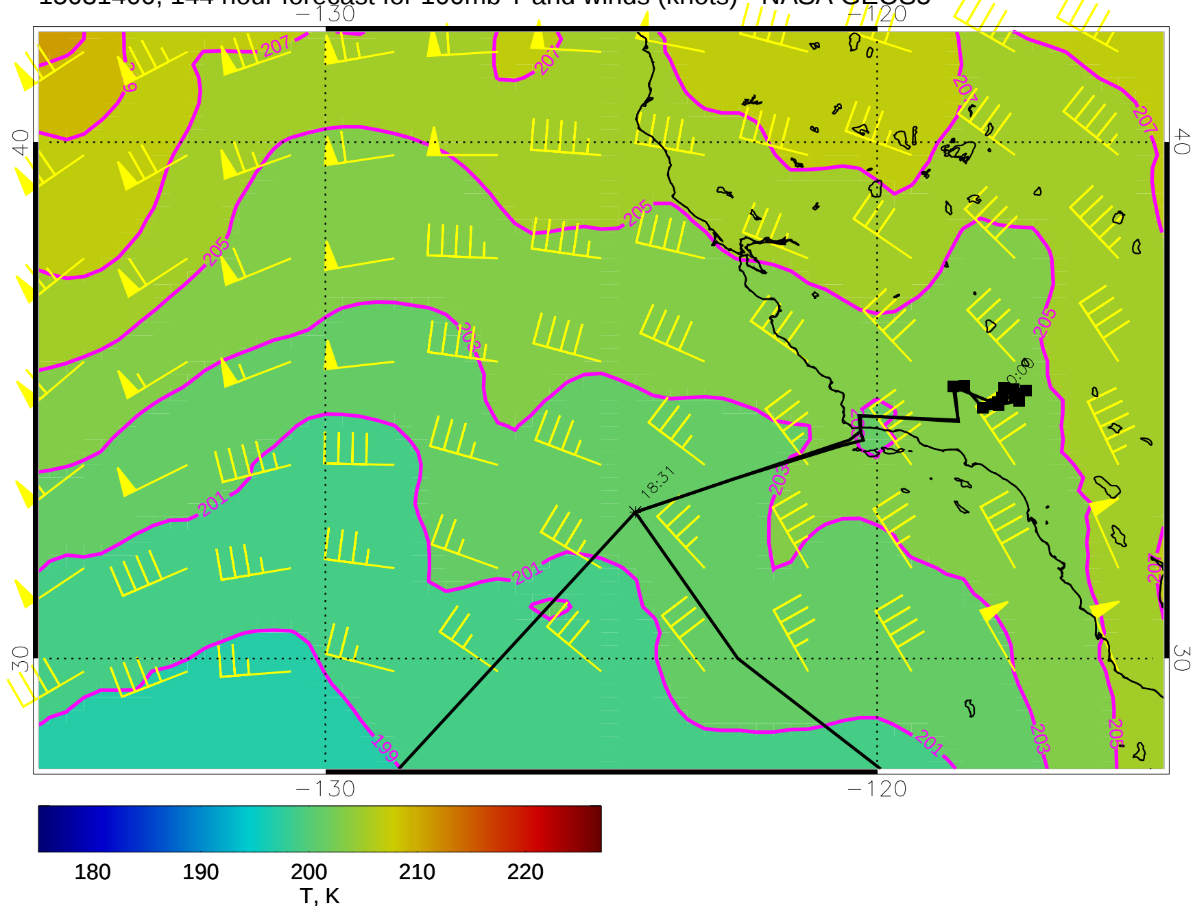
15031400, 144 hour forecast for 100mb T and winds (knots) - NASA GEOS5
