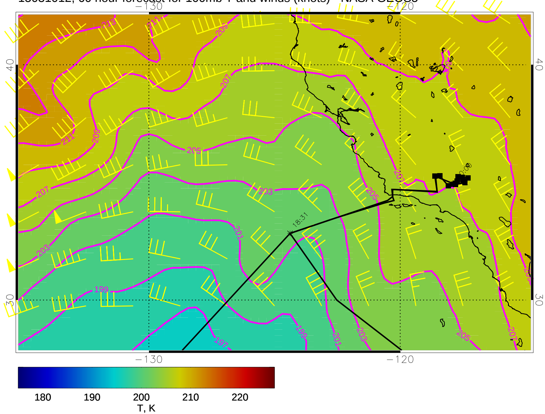
15031012, 60 hour forecast for 100mb T and winds (knots) - NASA GEOS5
