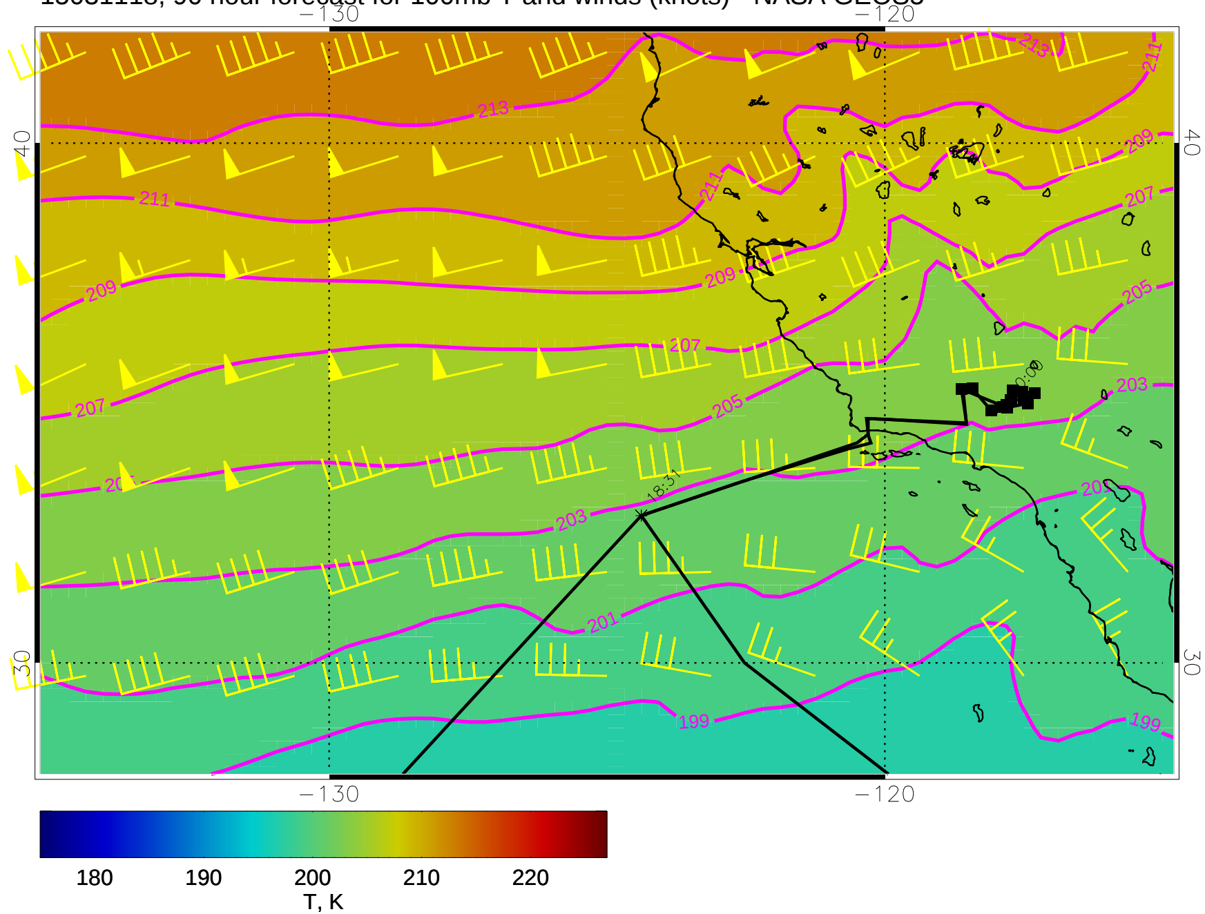
15031118, 90 hour forecast for 100mb T and winds (knots) - NASA GEOS5
