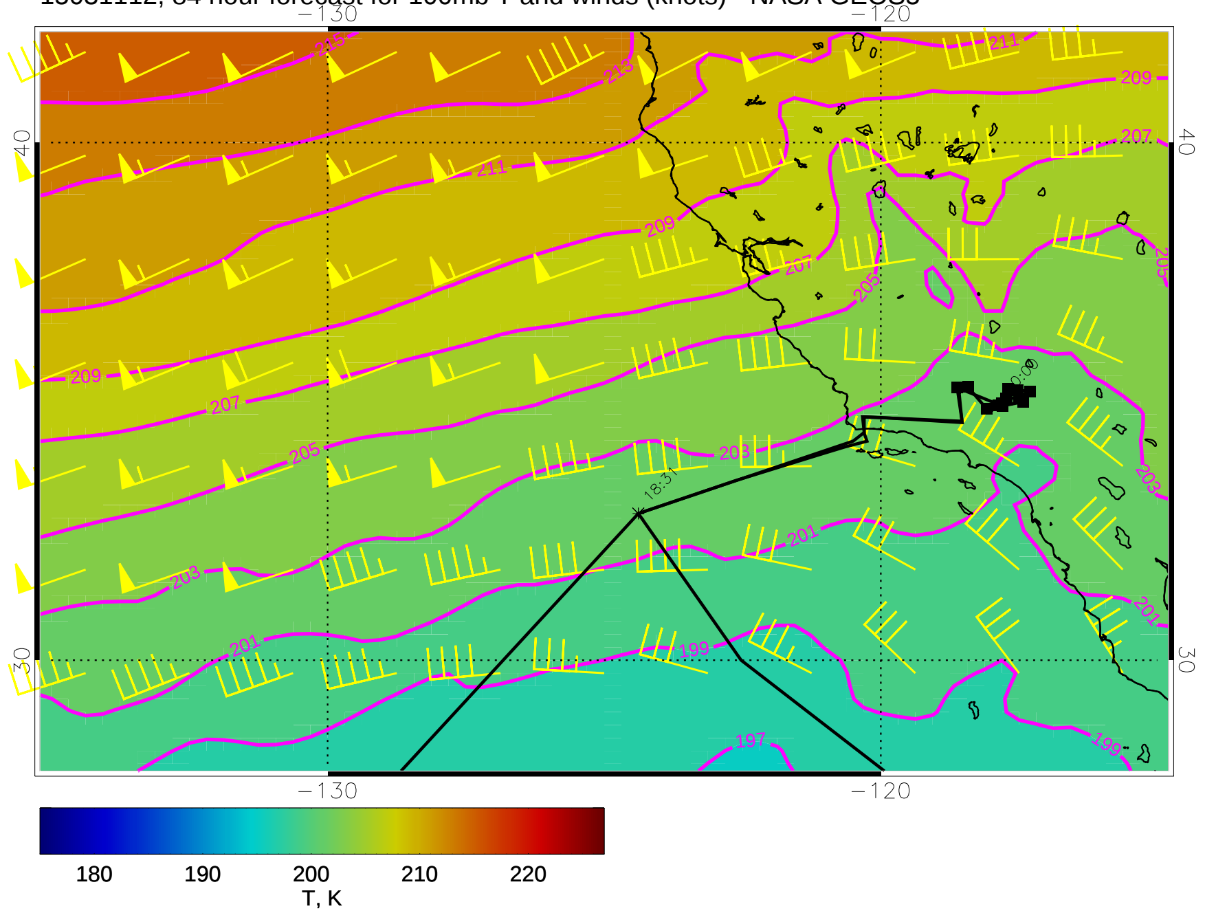
15031112, 84 hour forecast for 100mb T and winds (knots) - NASA GEOS5
