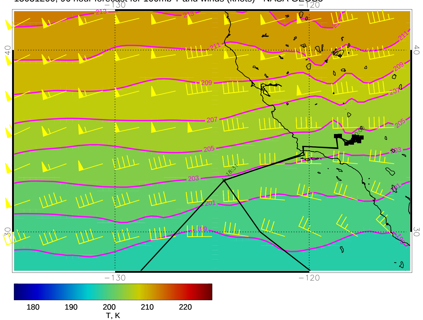
15031200, 96 hour forecast for 100mb T and winds (knots) - NASA GEOS5
