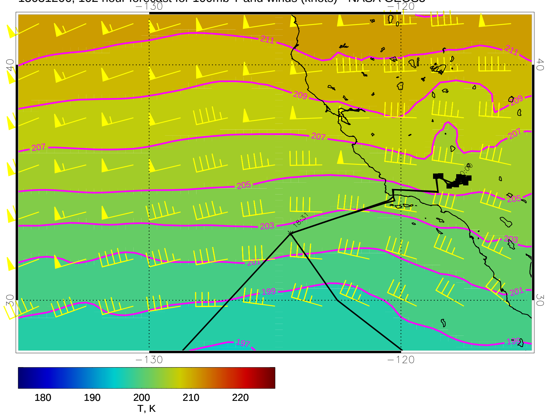
15031206, 102 hour forecast for 100mb T and winds (knots) - NASA GEOS5
