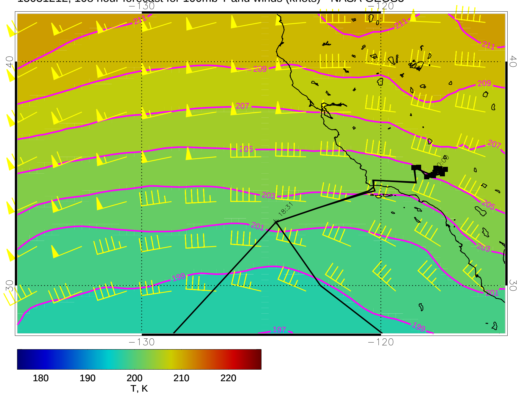
15031212, 108 hour forecast for 100mb T and winds (knots) - NASA GEOS5
