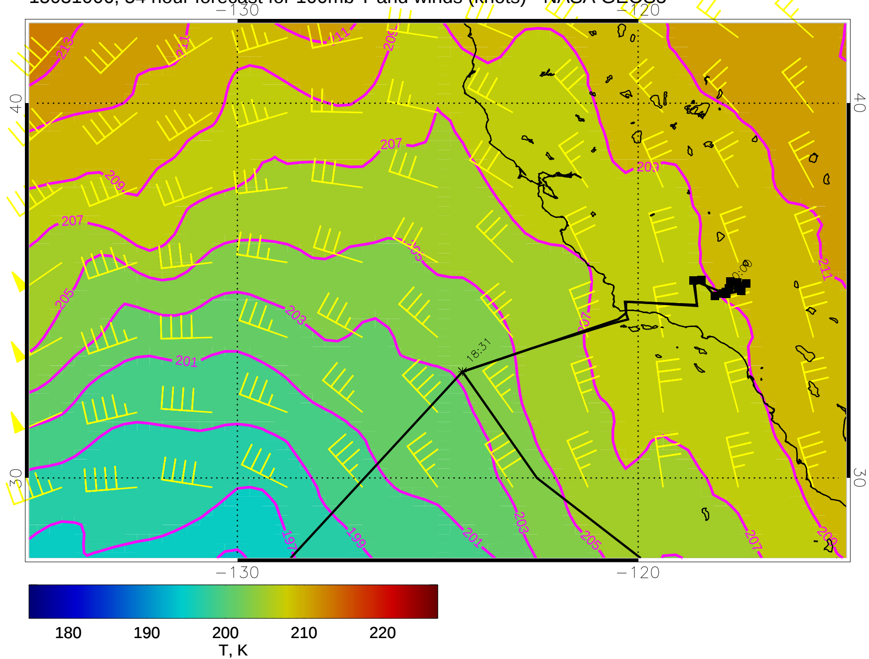
15031006, 54 hour forecast for 100mb T and winds (knots) - NASA GEOS5
