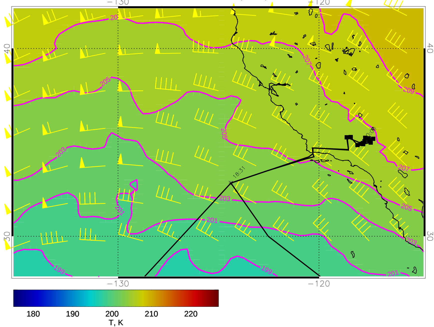
15031312, 132 hour forecast for 100mb T and winds (knots) - NASA GEOS5
