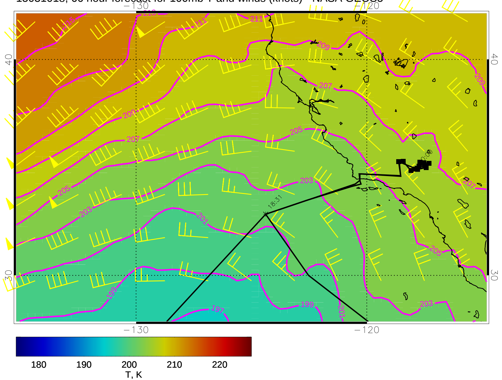
15031018, 66 hour forecast for 100mb T and winds (knots) - NASA GEOS5
