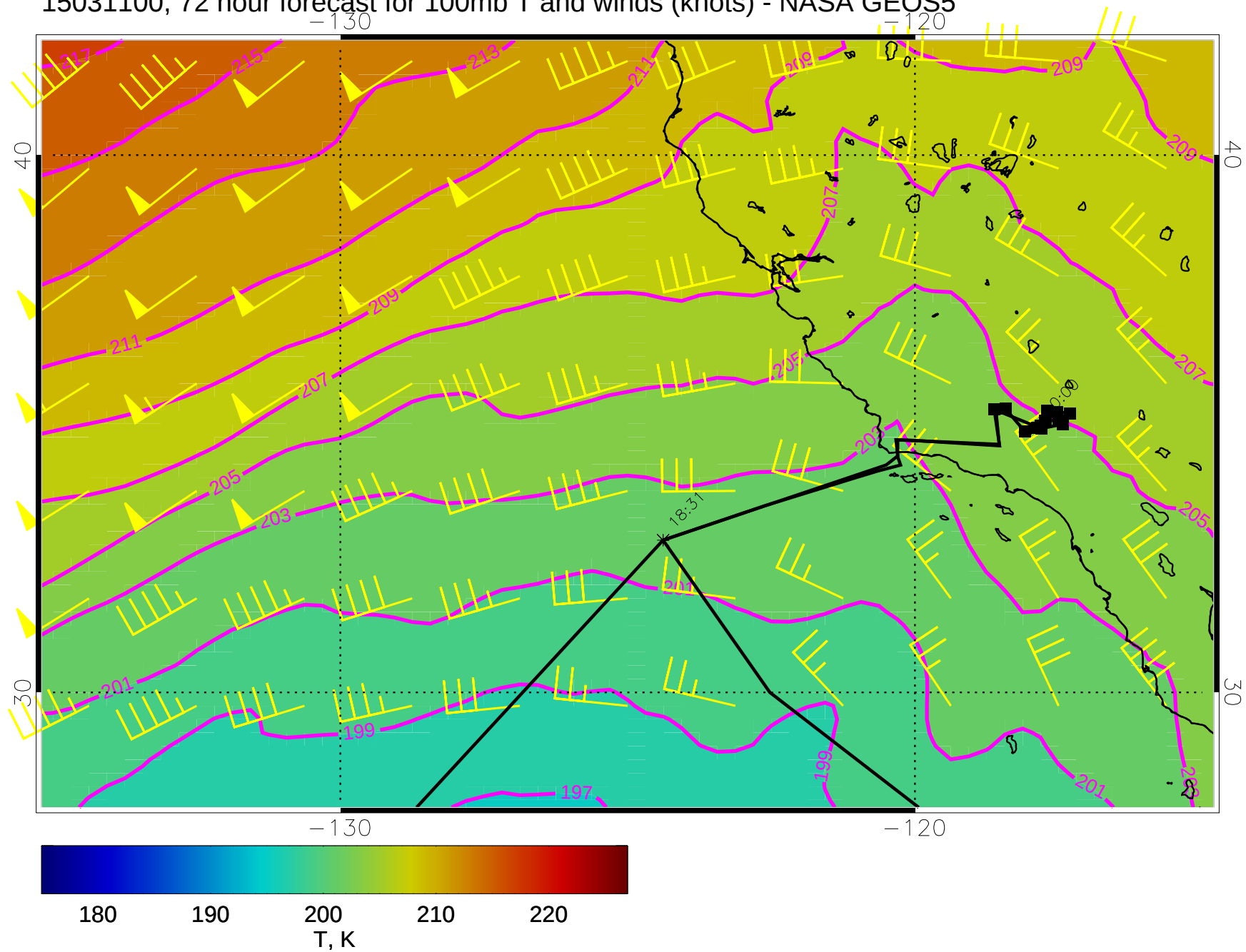
15031100, 72 hour forecast for 100mb T and winds (knots) - NASA GEOS5
