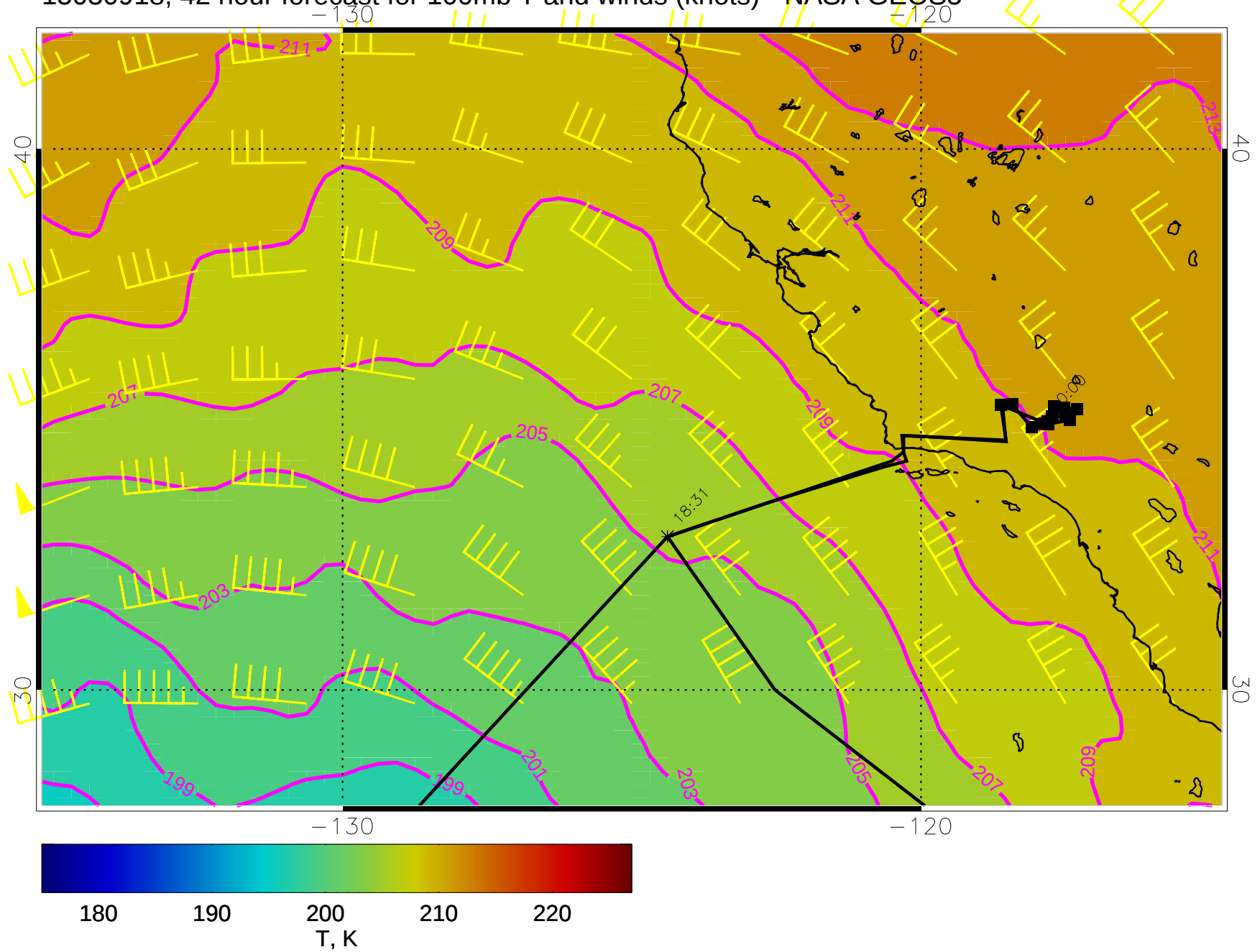
15030918, 42 hour forecast for 100mb T and winds (knots) - NASA GEOS5
