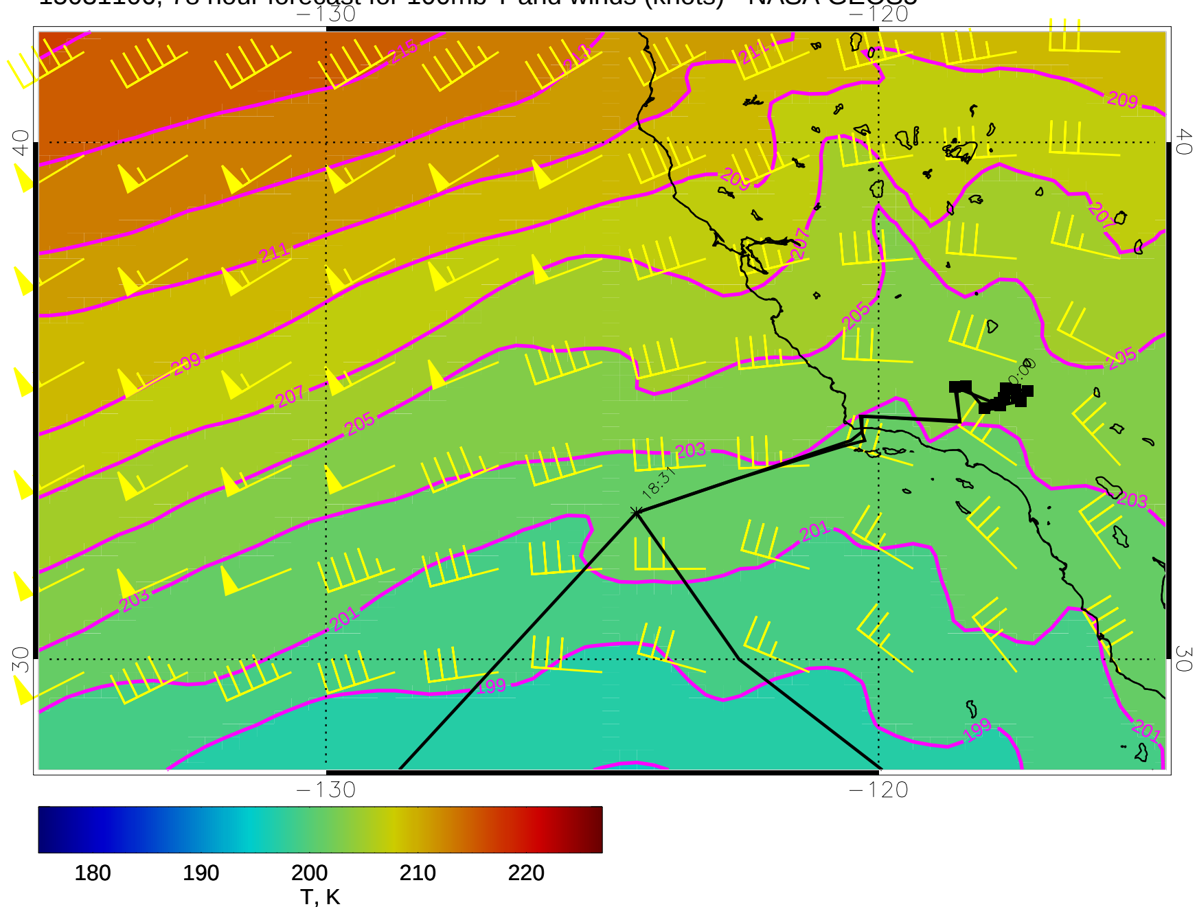
15031106, 78 hour forecast for 100mb T and winds (knots) - NASA GEOS5
