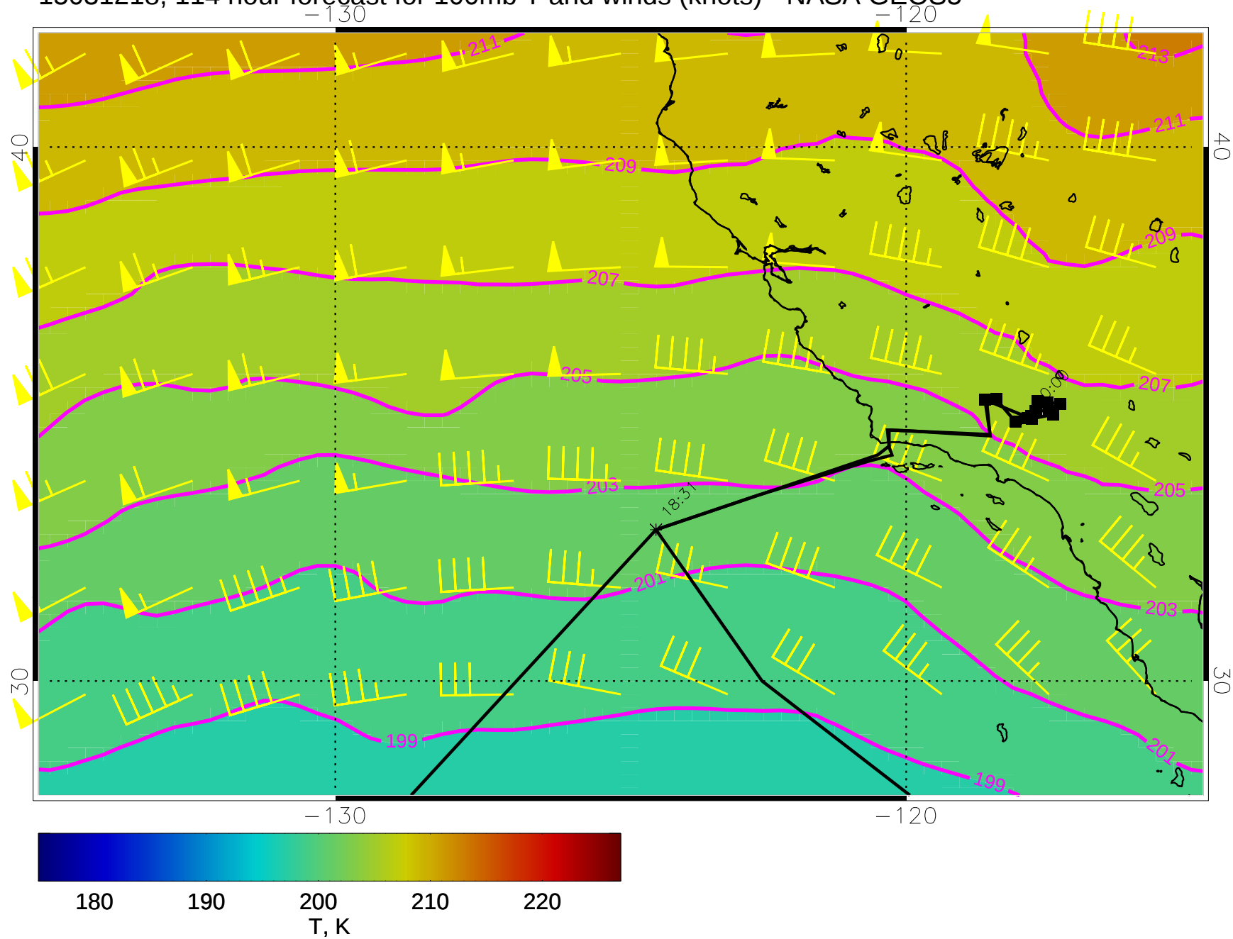
15031218, 114 hour forecast for 100mb T and winds (knots) - NASA GEOS5
