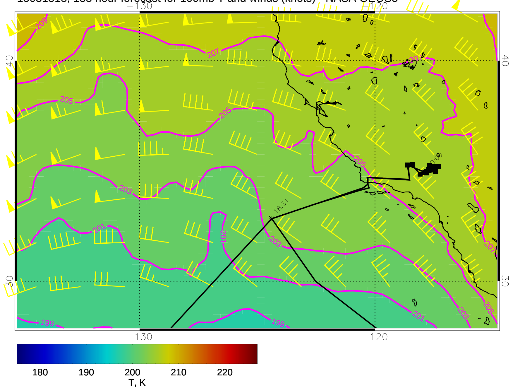
15031318, 138 hour forecast for 100mb T and winds (knots) - NASA GEOS5
