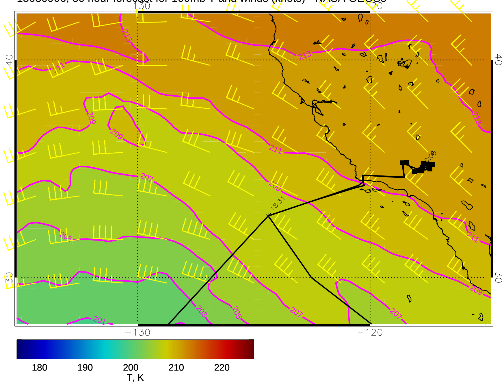
15030906, 30 hour forecast for 100mb T and winds (knots) - NASA GEOS5
