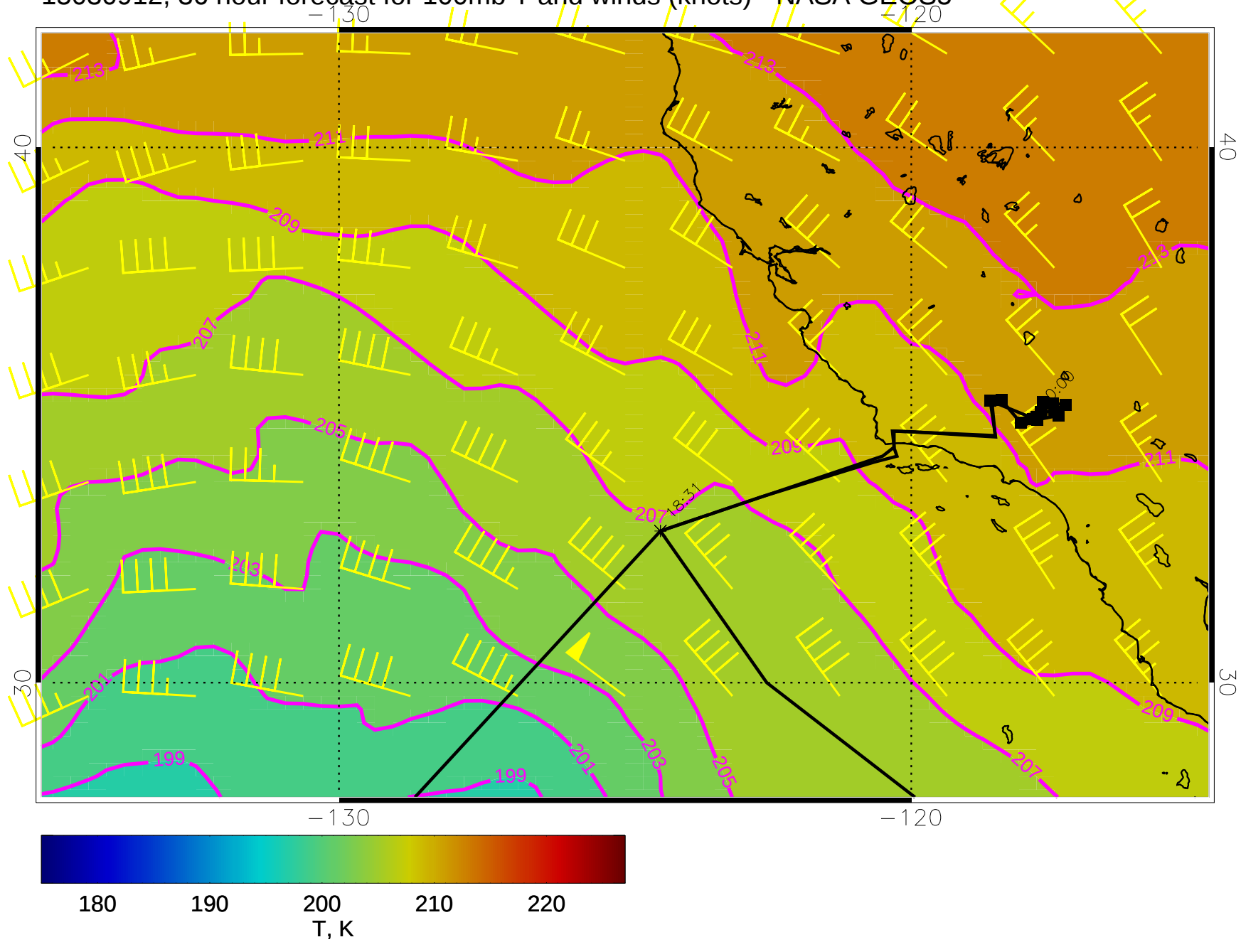
15030912, 36 hour forecast for 100mb T and winds (knots) - NASA GEOS5
