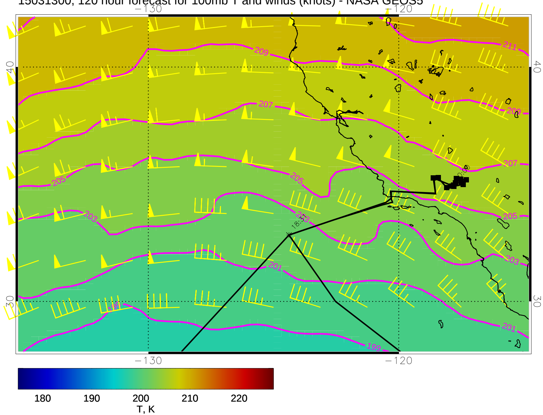
15031300, 120 hour forecast for 100mb T and winds (knots) - NASA GEOS5
