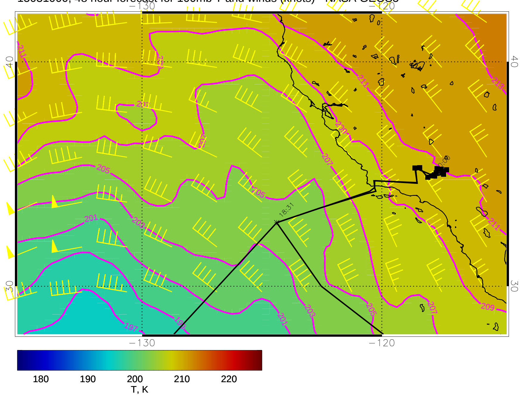
15031000, 48 hour forecast for 100mb T and winds (knots) - NASA GEOS5
