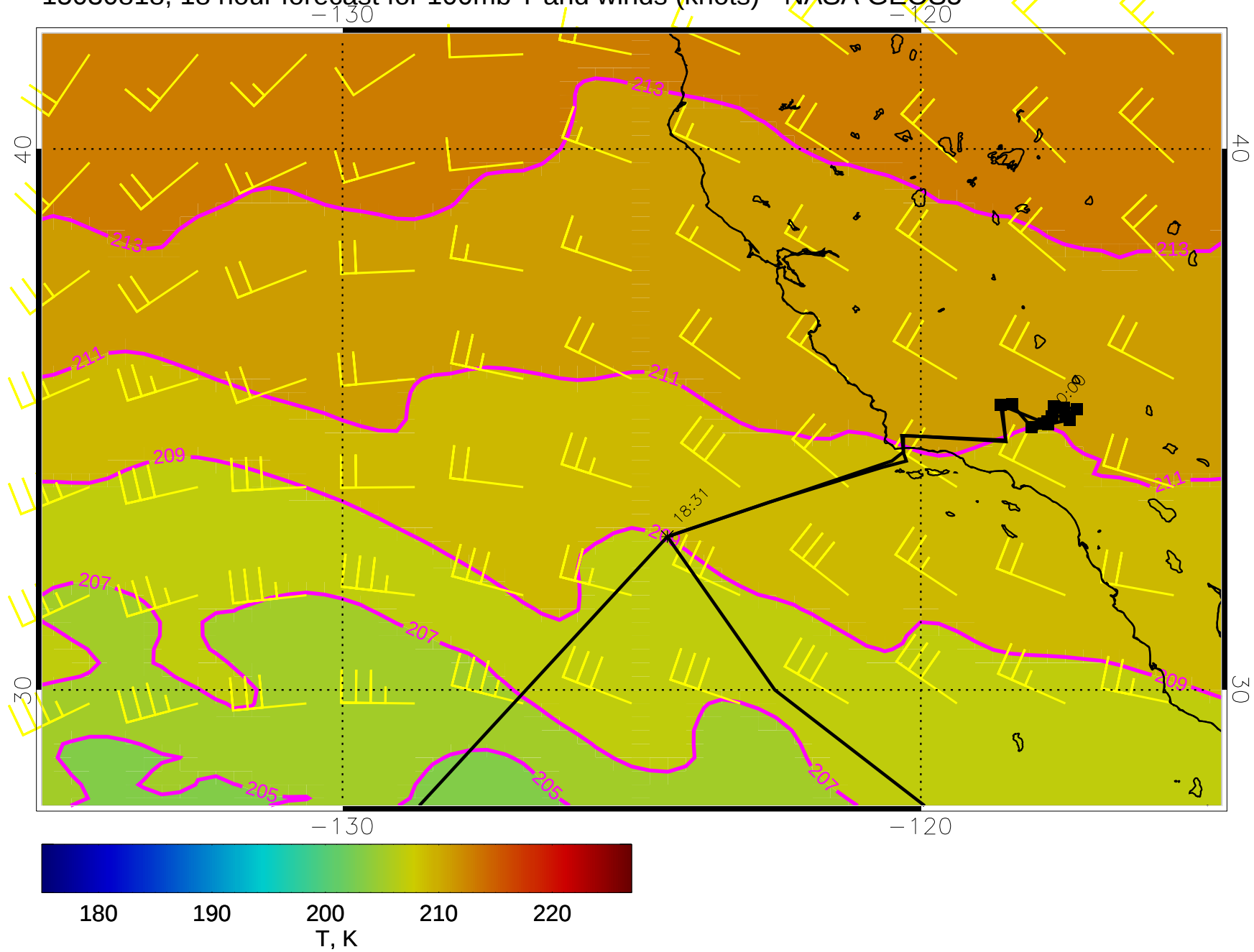
15030818, 18 hour forecast for 100mb T and winds (knots) - NASA GEOS5
