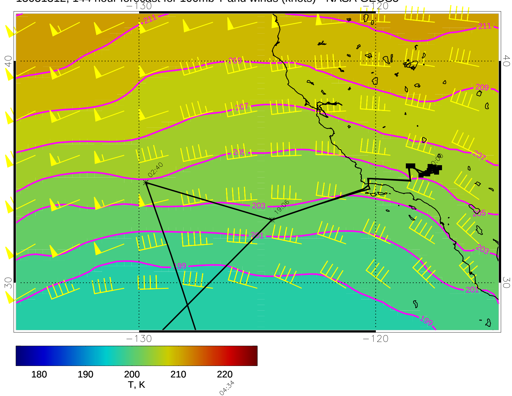
15031312, 144 hour forecast for 100mb T and winds (knots) - NASA GEOS5
