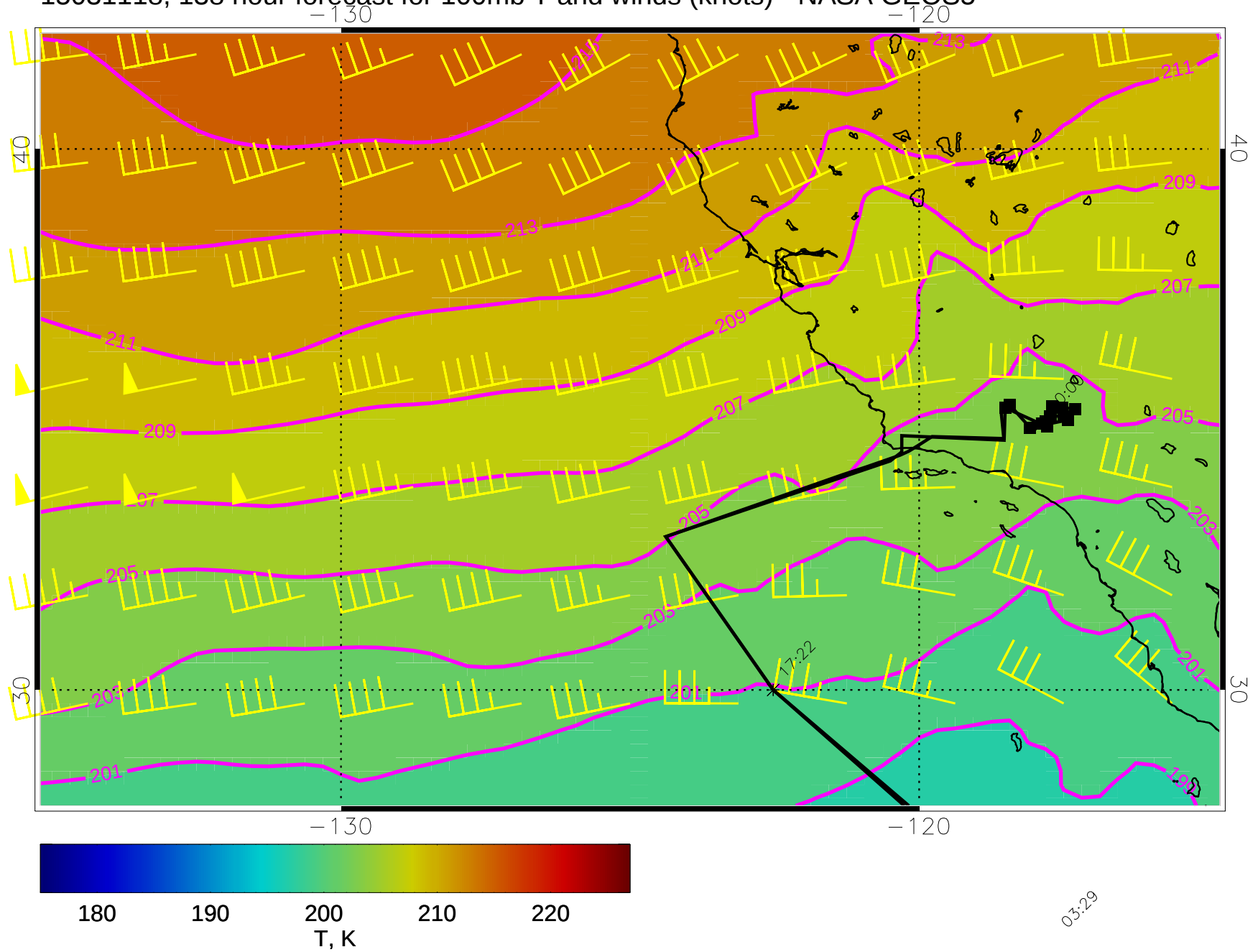
15031118, 138 hour forecast for 100mb T and winds (knots) - NASA GEOS5
