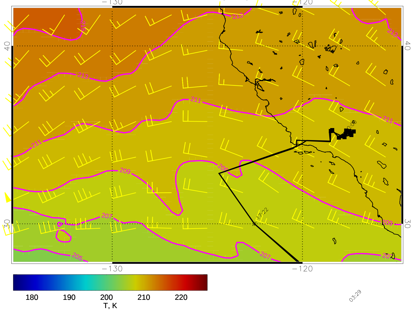
15030818, 66 hour forecast for 100mb T and winds (knots) - NASA GEOS5
