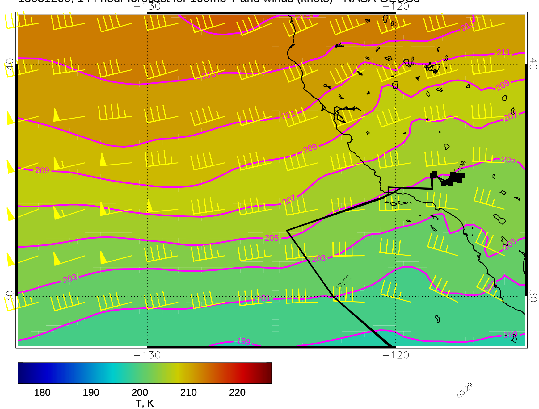
15031200, 144 hour forecast for 100mb T and winds (knots) - NASA GEOS5
