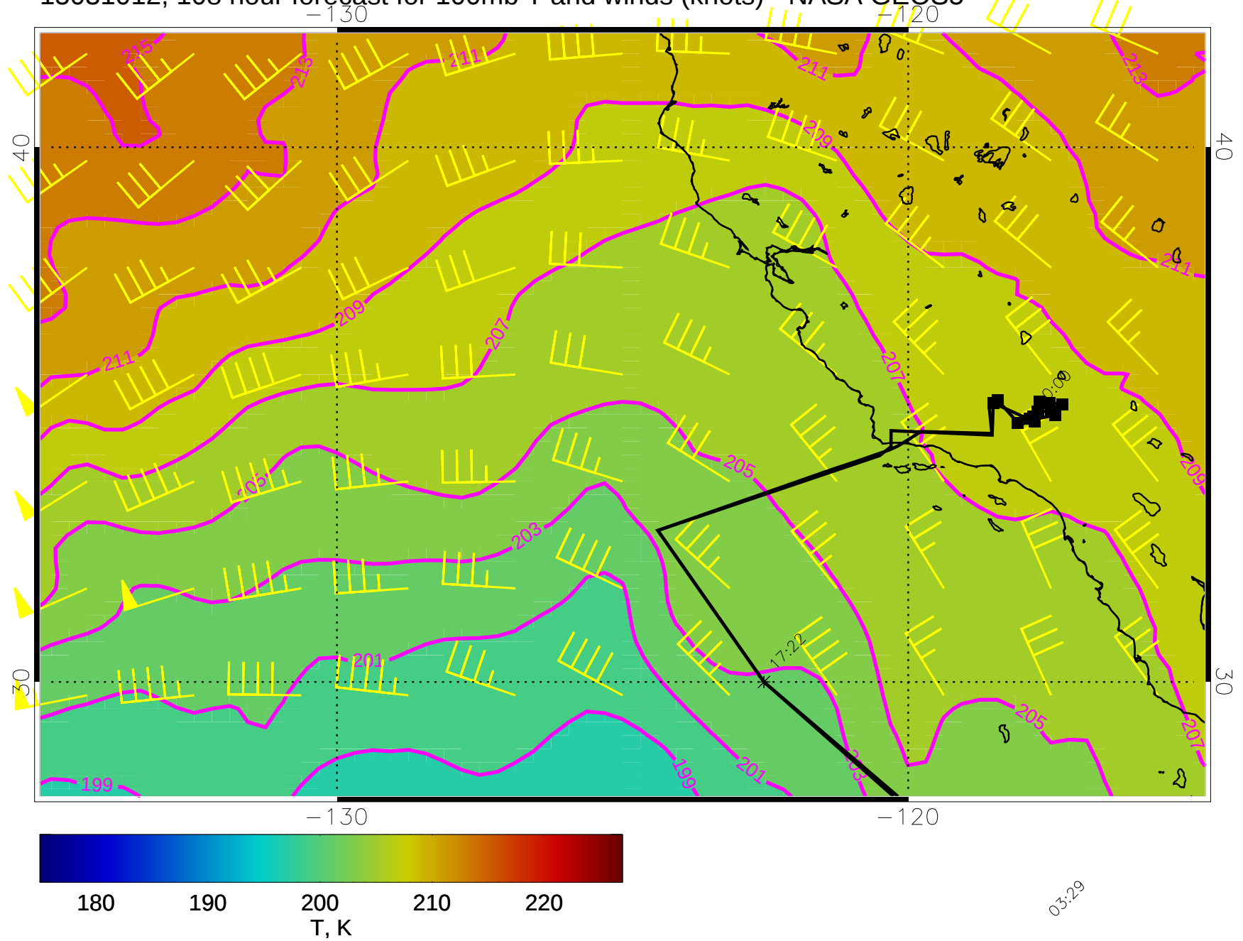
15031012, 108 hour forecast for 100mb T and winds (knots) - NASA GEOS5
