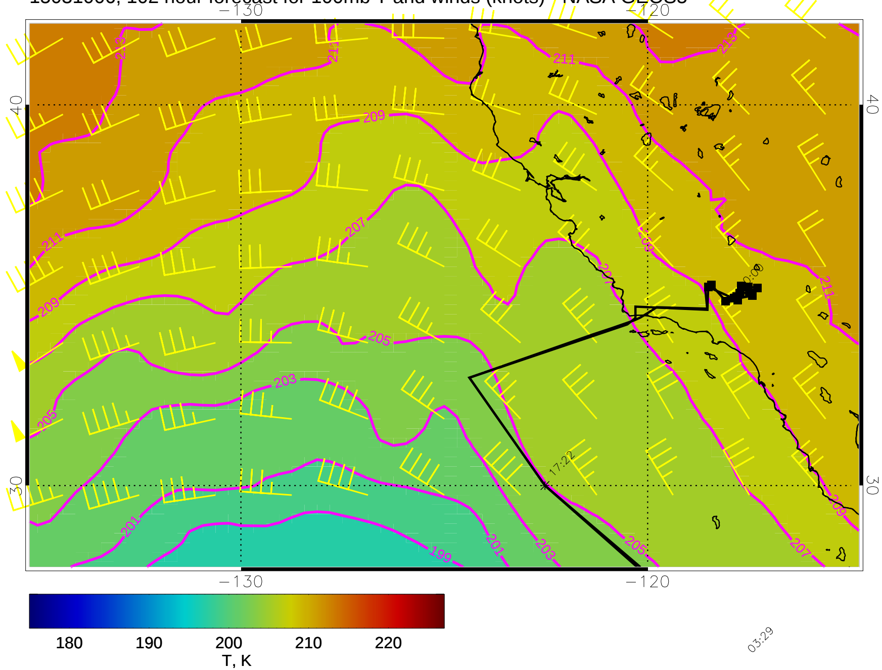
15031006, 102 hour forecast for 100mb T and winds (knots) - NASA GEOS5
