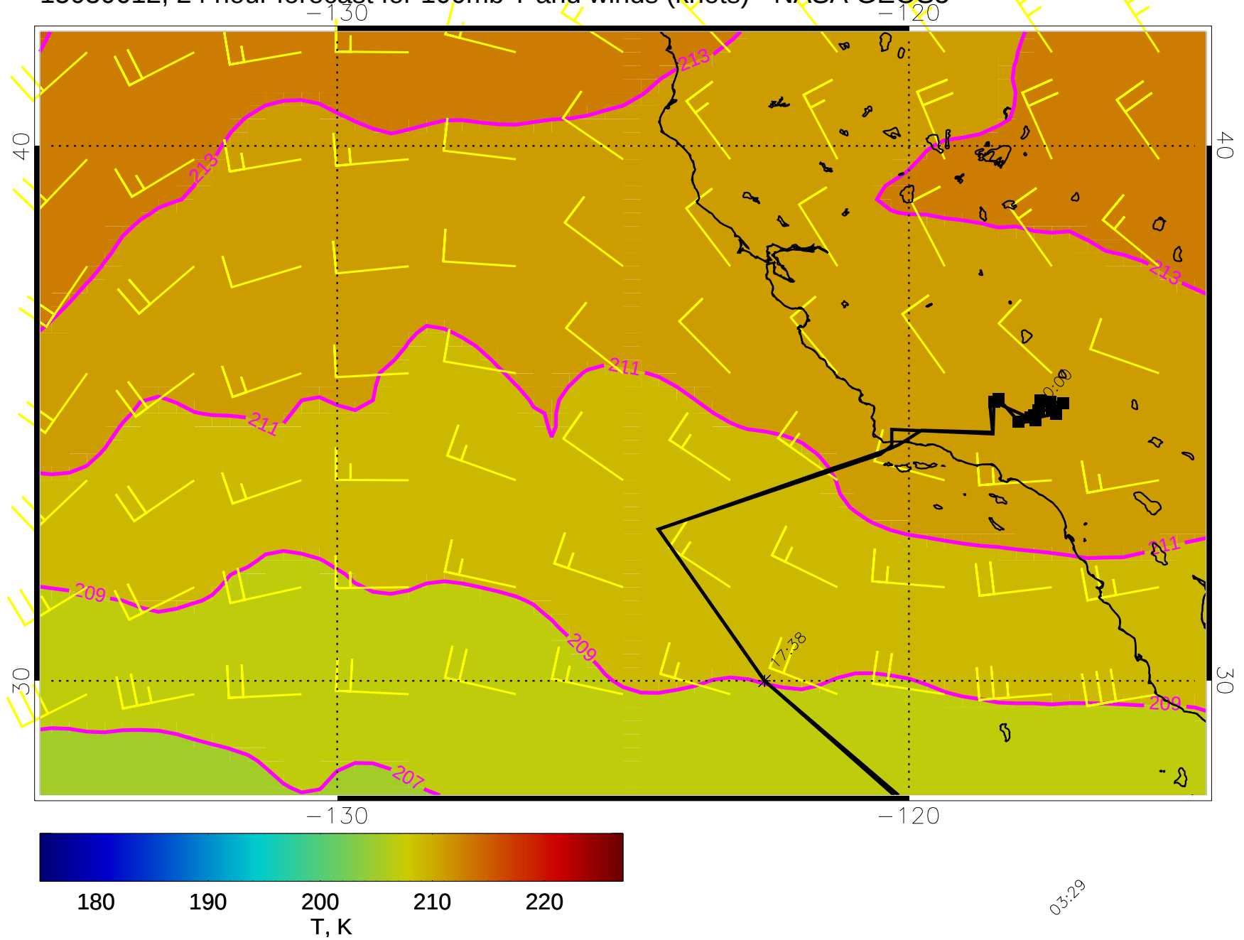
15030612, 24 hour forecast for 100mb T and winds (knots) - NASA GEOS5
