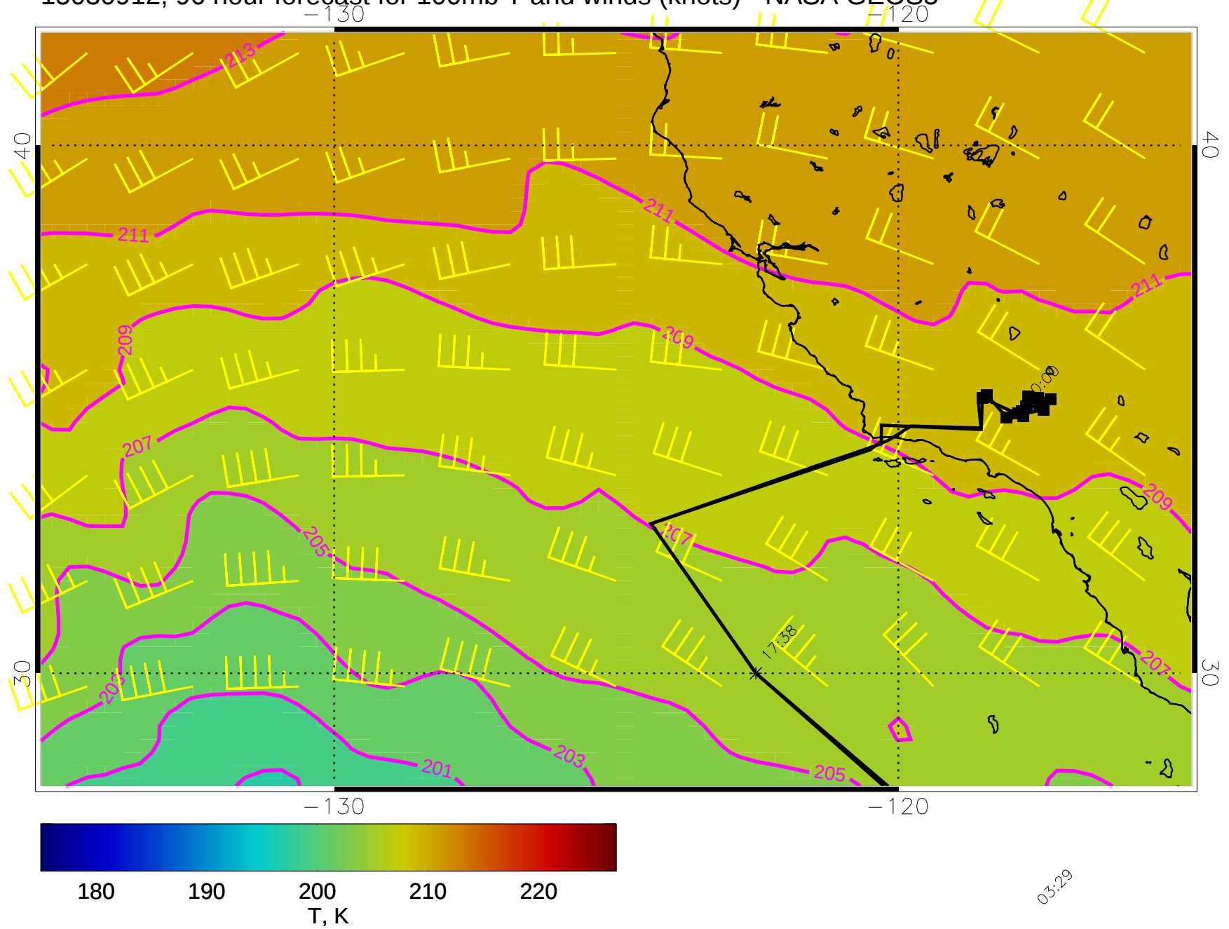
15030912, 96 hour forecast for 100mb T and winds (knots) - NASA GEOS5
