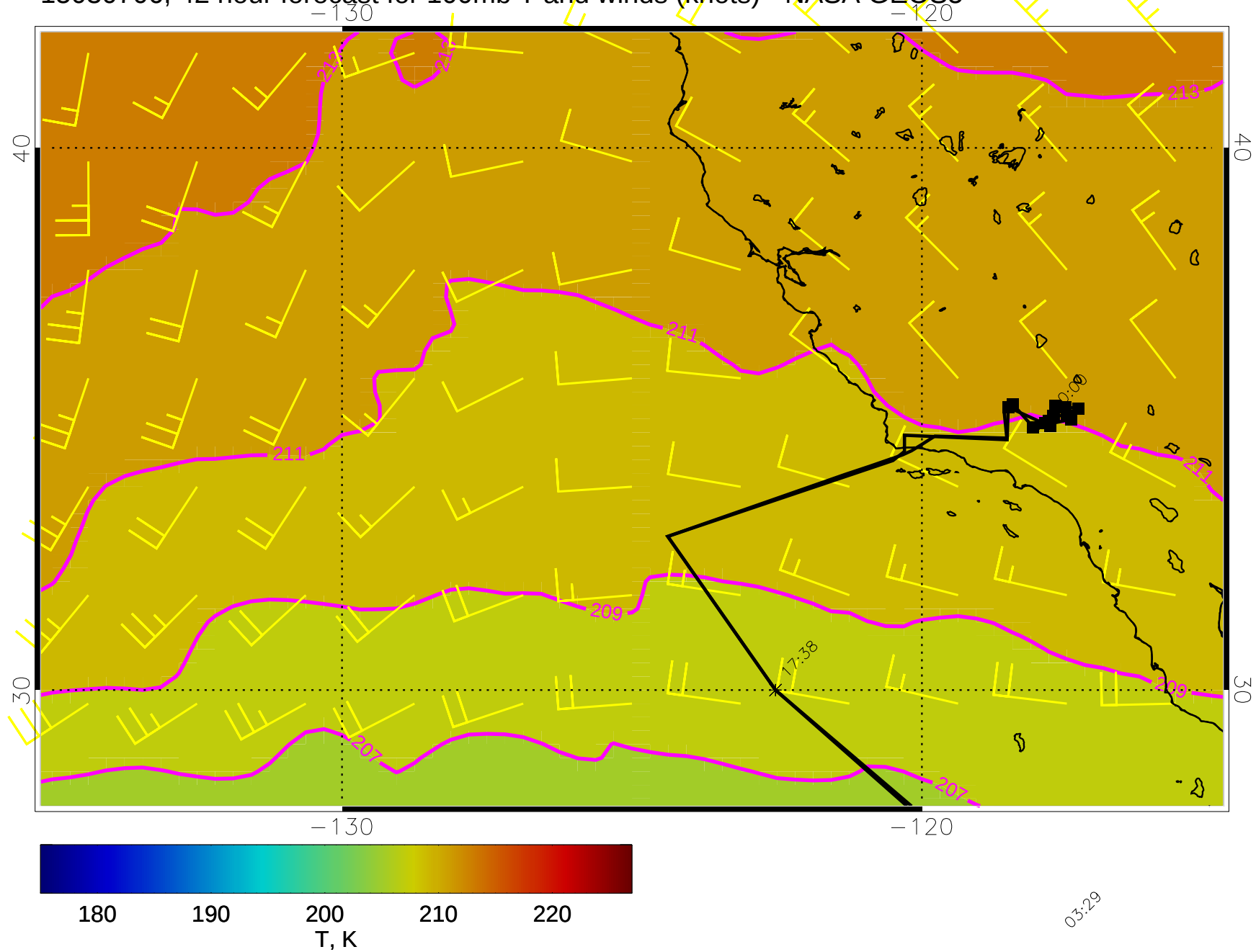
15030706, 42 hour forecast for 100mb T and winds (knots) - NASA GEOS5
