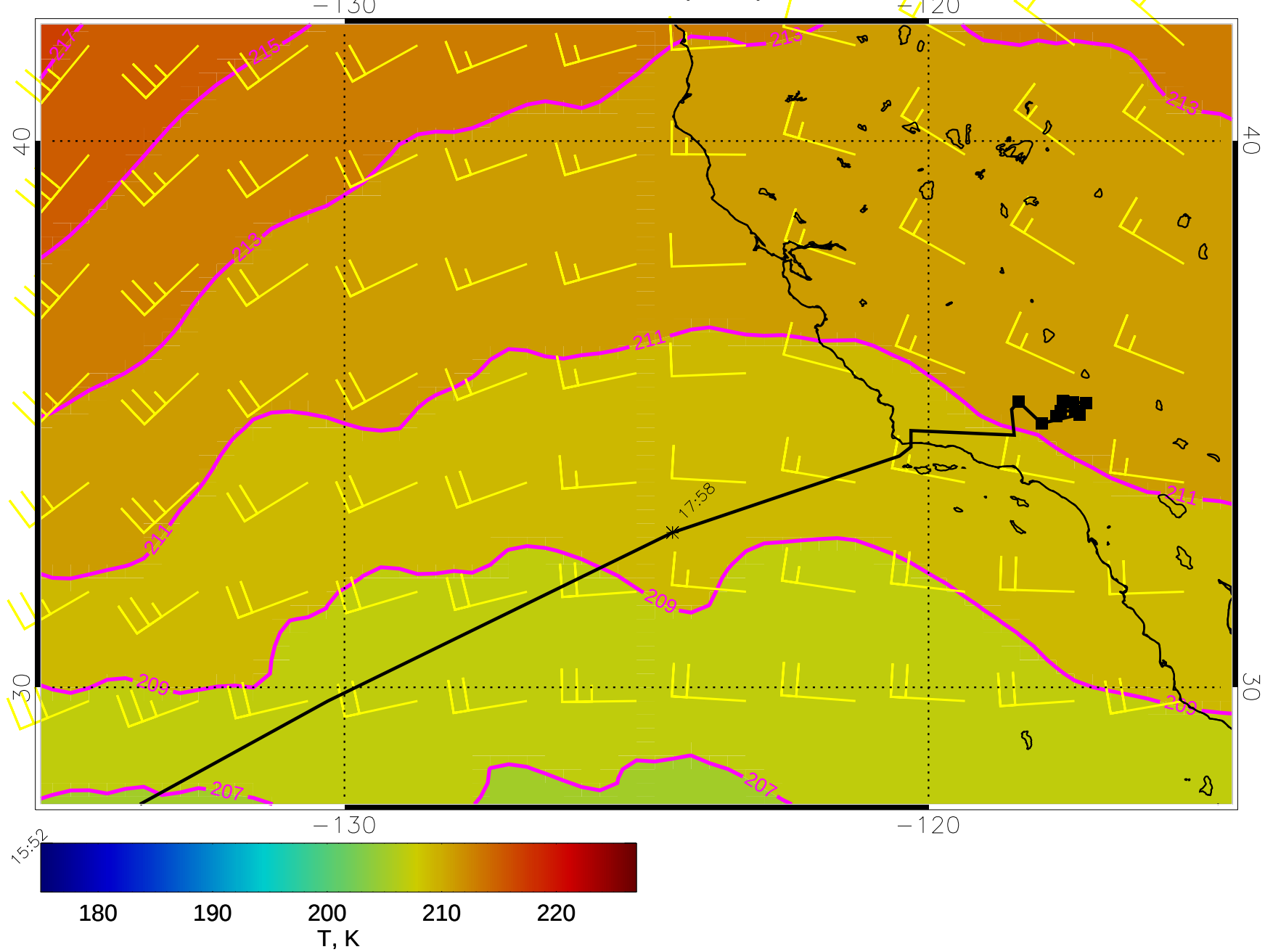
15030612, 96 hour forecast for 100mb T and winds (knots) - NASA GEOS5
