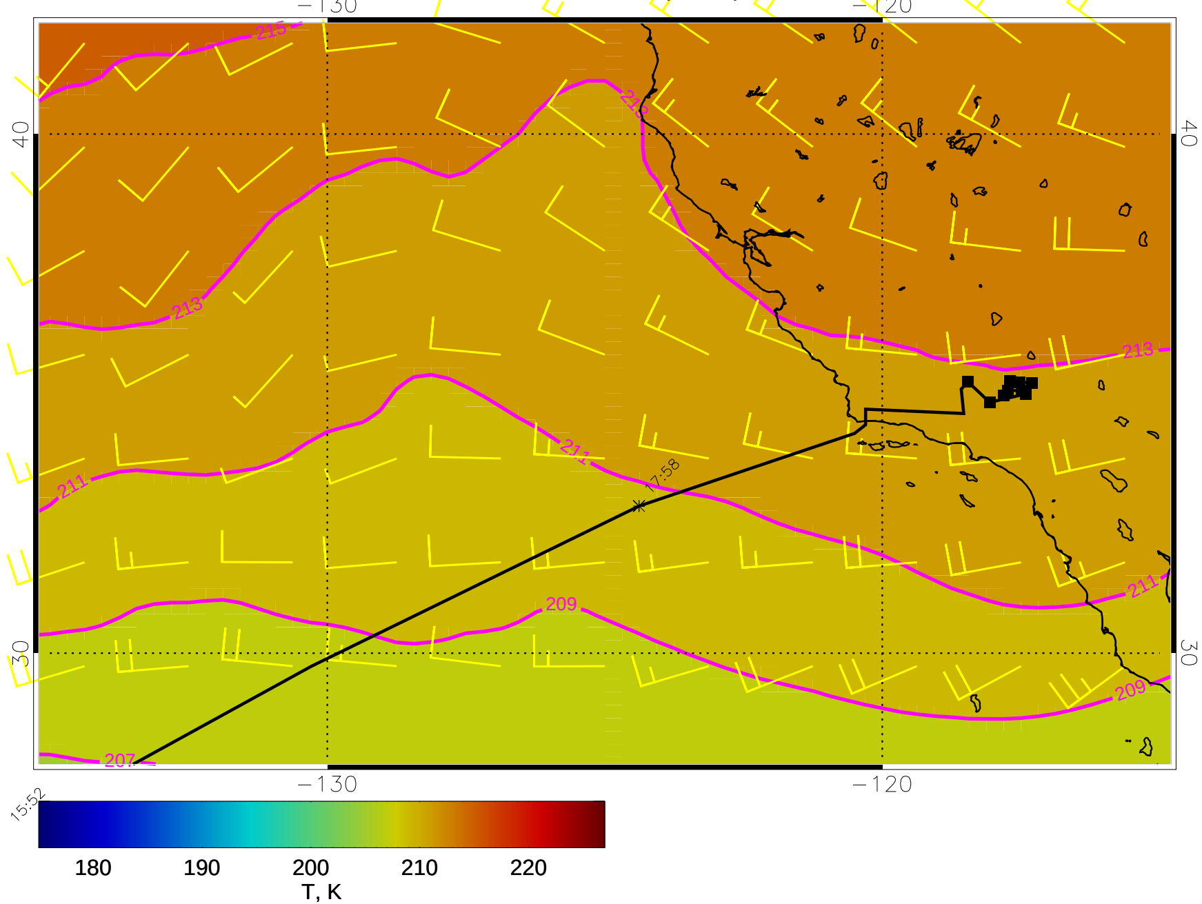
15030518, 102 hour forecast for 100mb T and winds (knots) - NASA GEOS5
