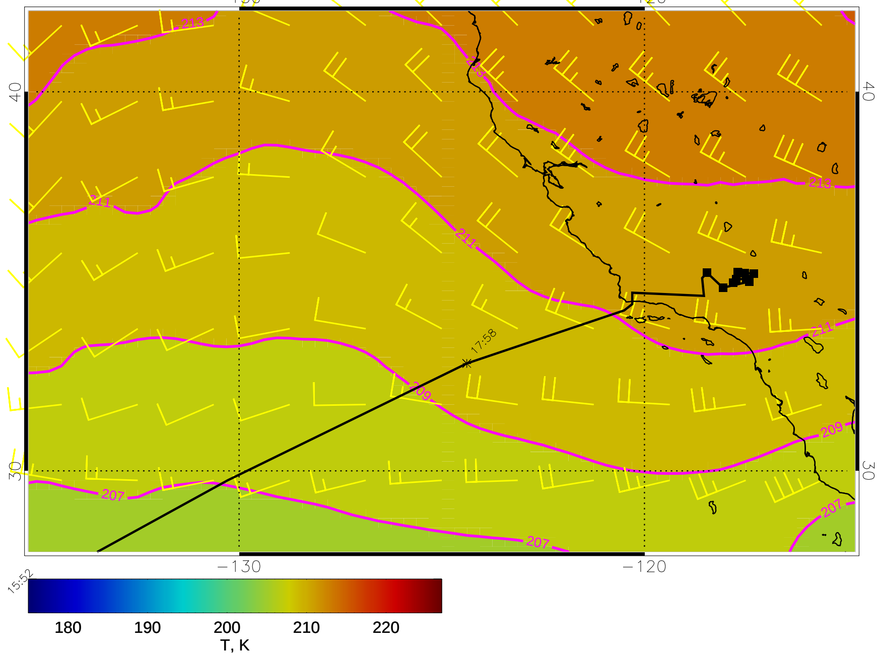
15030500, 96 hour forecast for 100mb T and winds (knots) - NASA GEOS5
