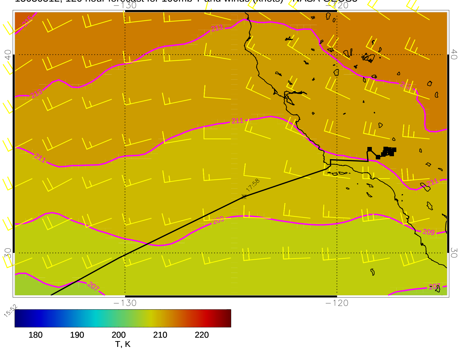
15030512, 120 hour forecast for 100mb T and winds (knots) - NASA GEOS5
