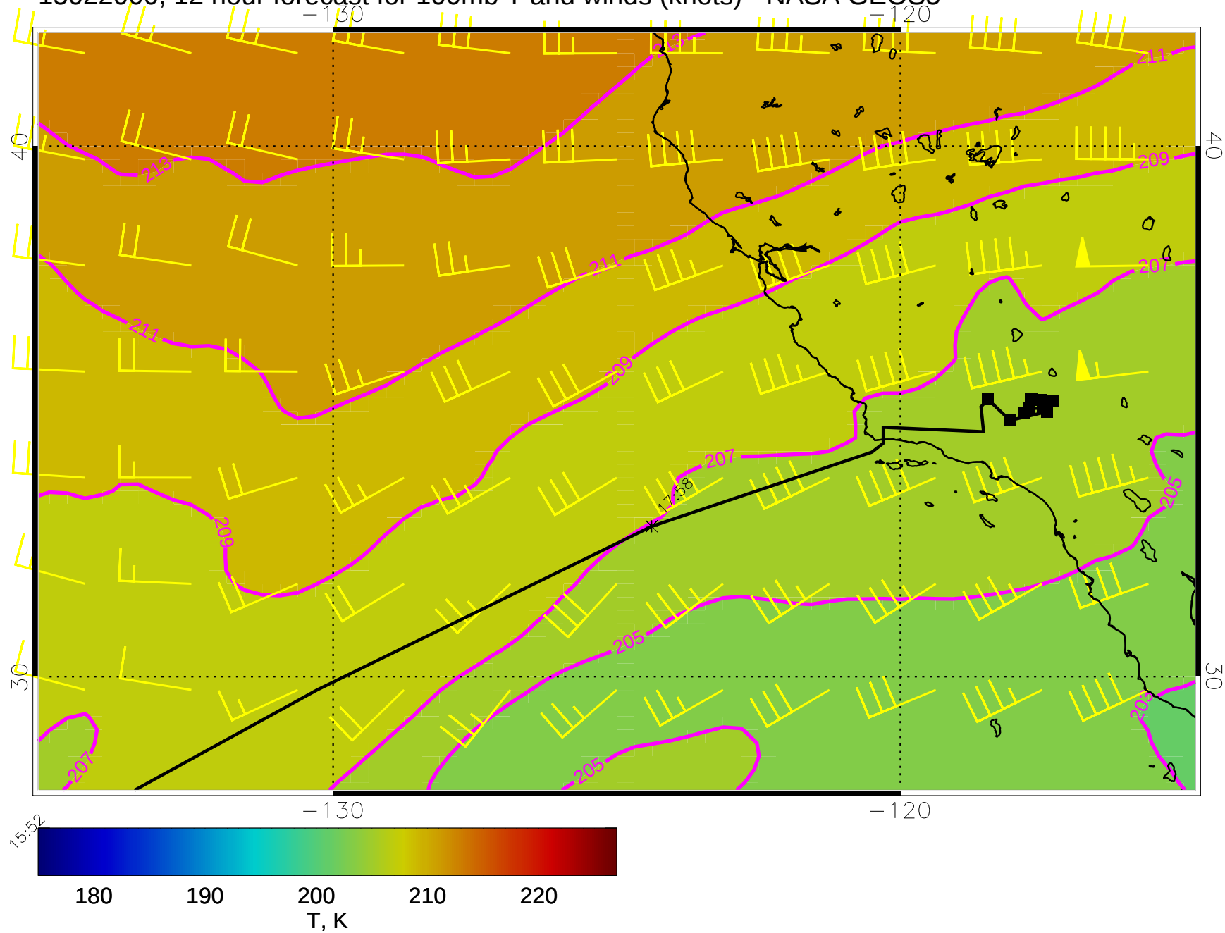
15022000, 12 hour forecast for 100mb T and winds (knots) - NASA GEOS5
