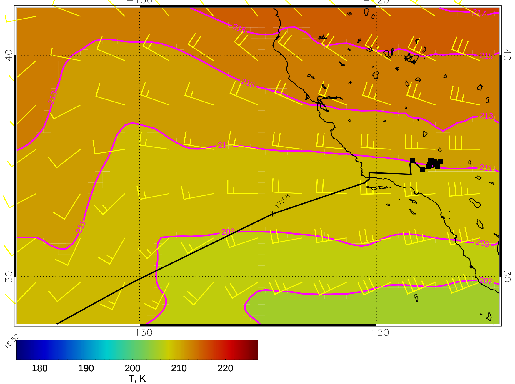
15022306, 90 hour forecast for 100mb T and winds (knots) - NASA GEOS5
