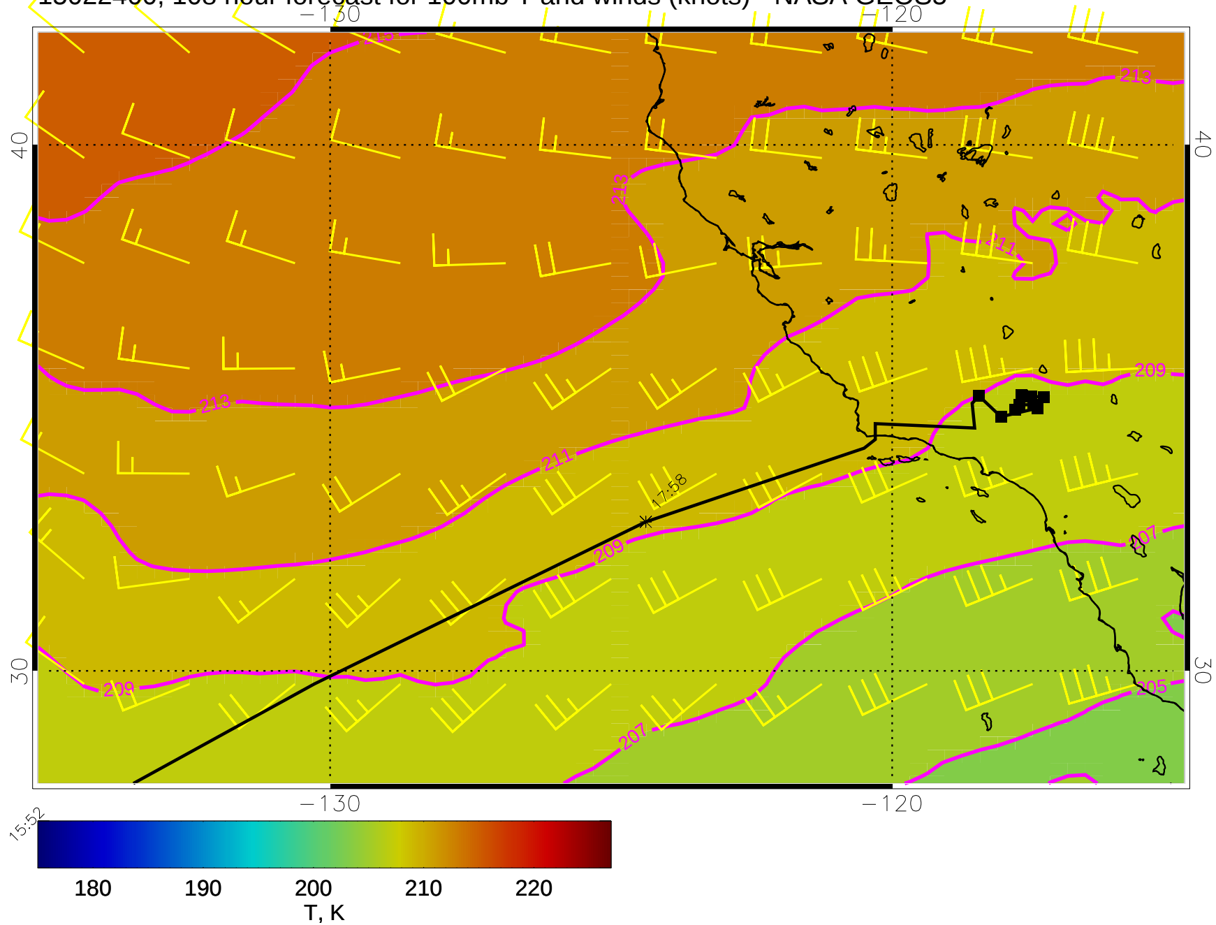
15022400, 108 hour forecast for 100mb T and winds (knots) - NASA GEOS5
