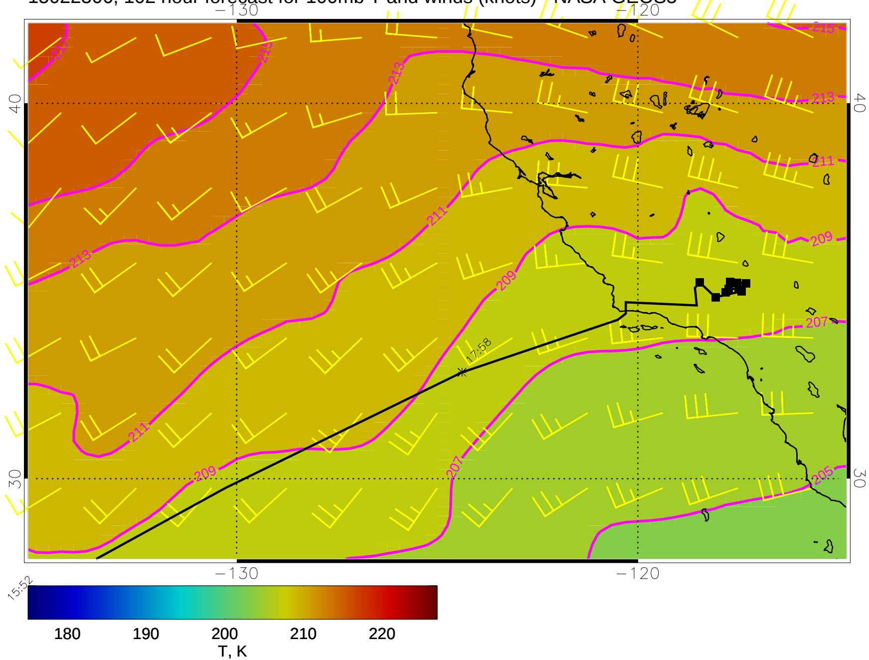
15022306, 102 hour forecast for 100mb T and winds (knots) - NASA GEOS5
