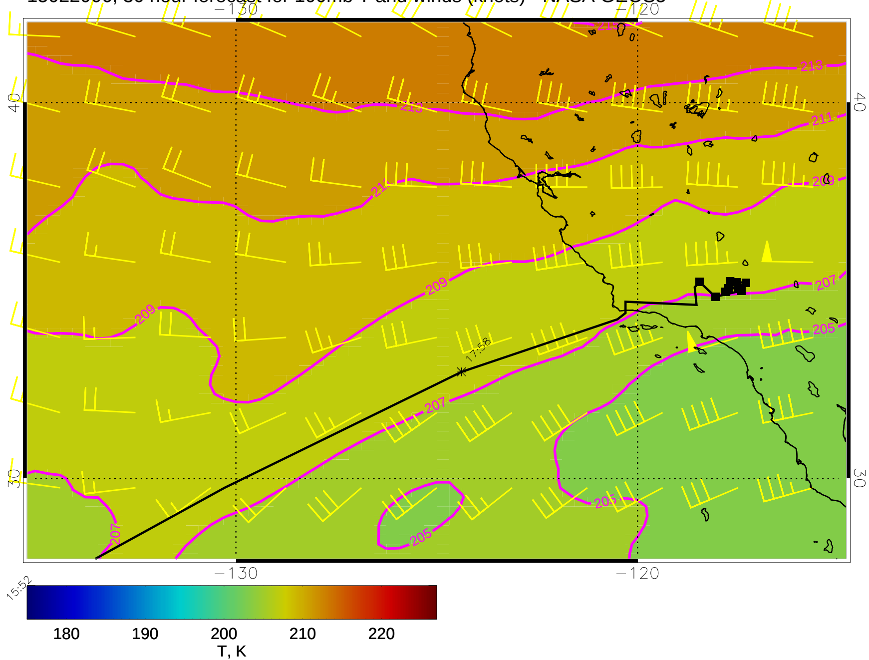
15022006, 30 hour forecast for 100mb T and winds (knots) - NASA GEOS5
