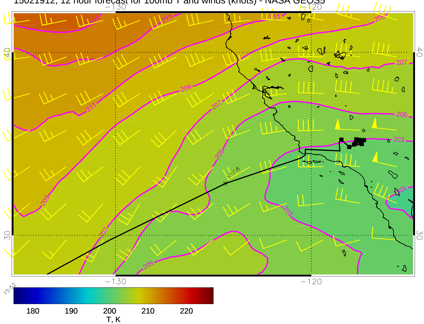
15021912, 12 hour forecast for 100mb T and winds (knots) - NASA GEOS5
