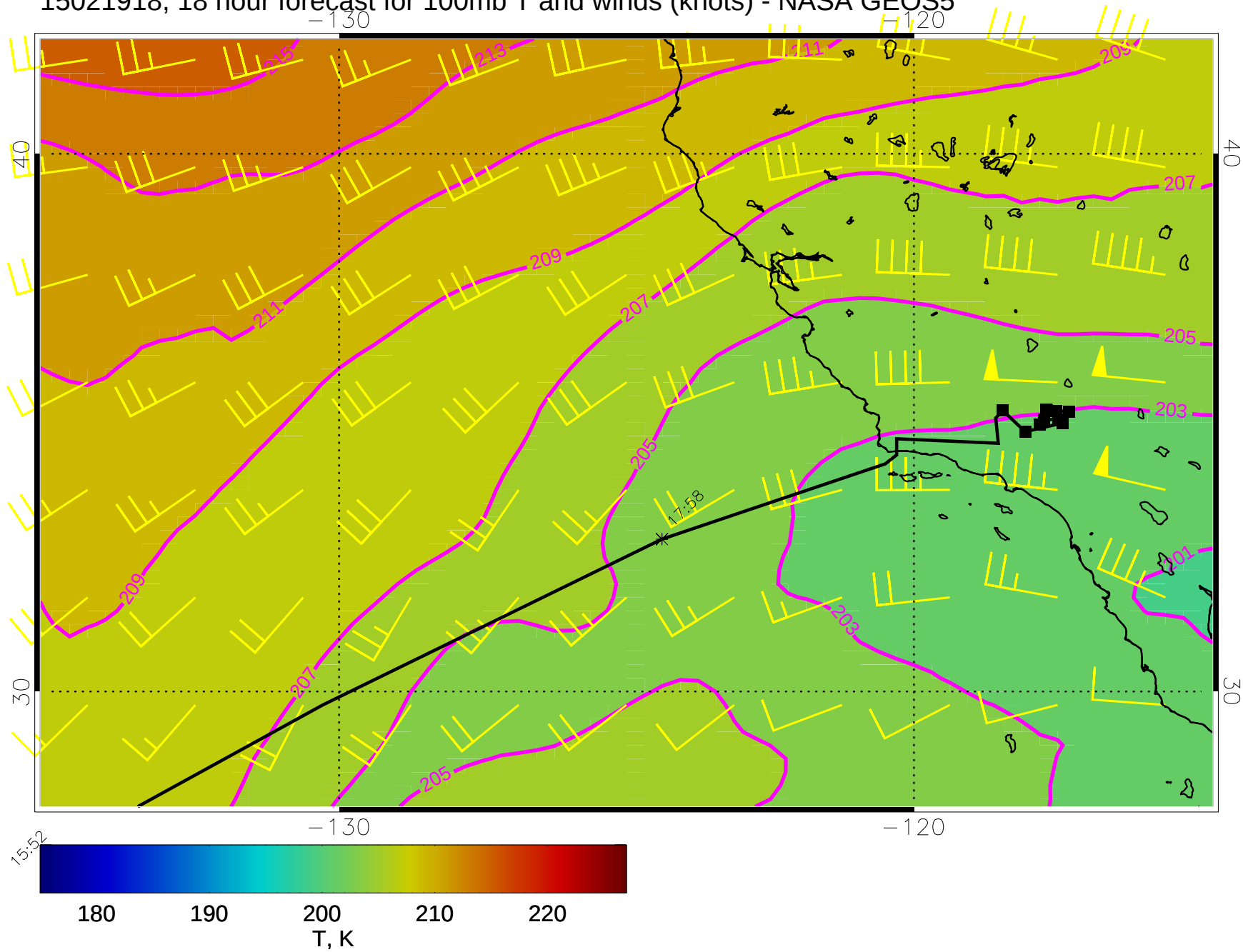
15021918, 18 hour forecast for 100mb T and winds (knots) - NASA GEOS5
