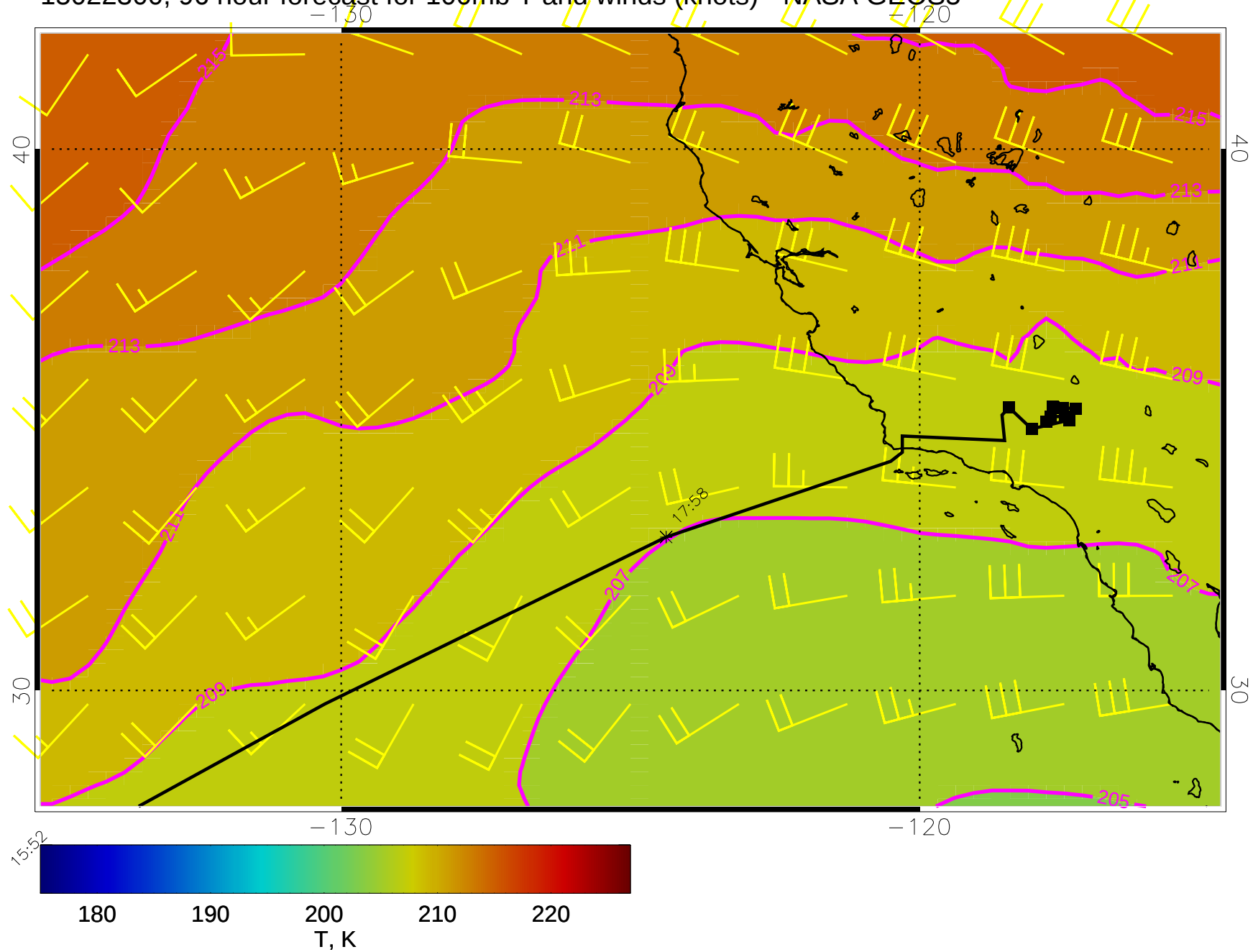
15022300, 96 hour forecast for 100mb T and winds (knots) - NASA GEOS5
