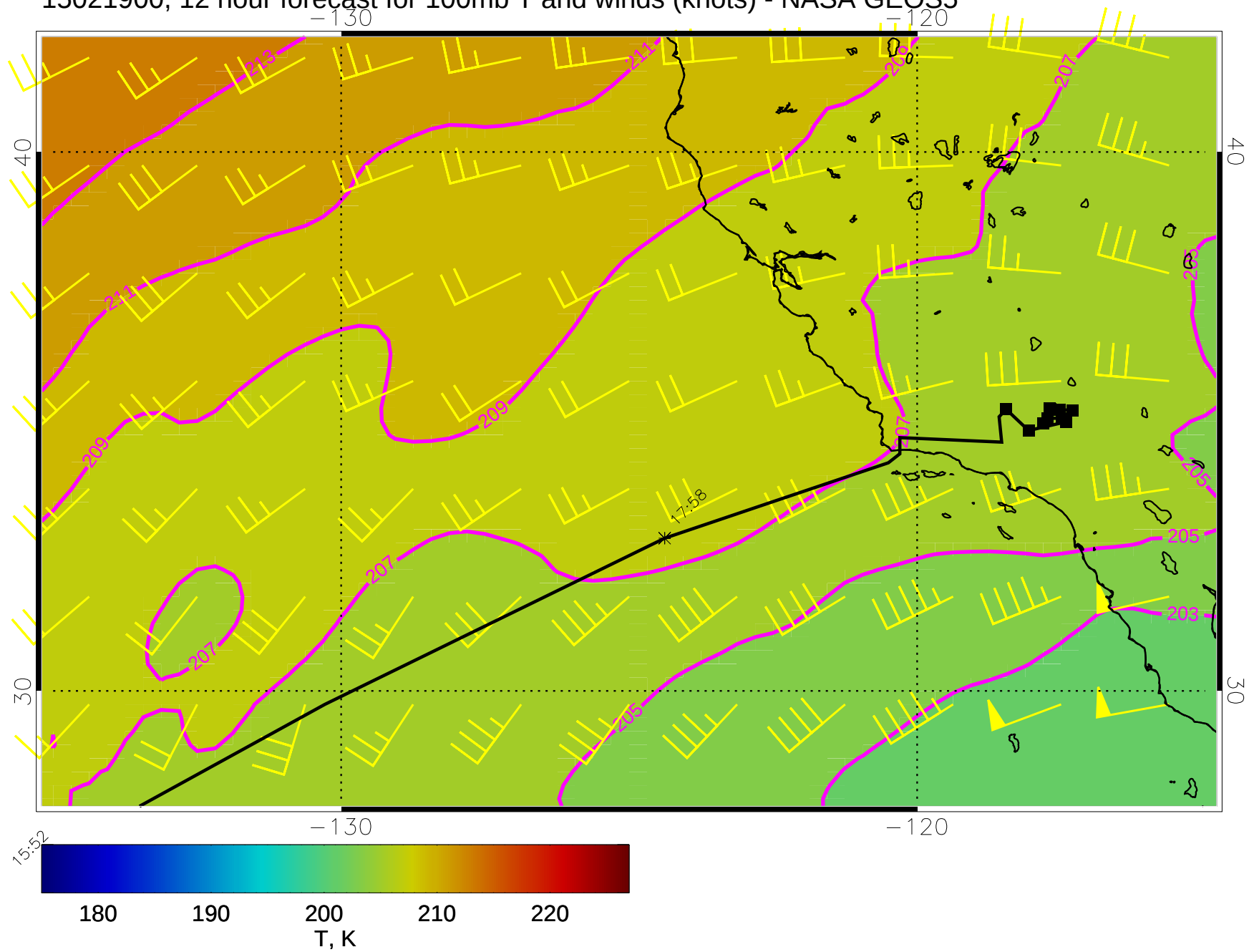
15021900, 12 hour forecast for 100mb T and winds (knots) - NASA GEOS5
