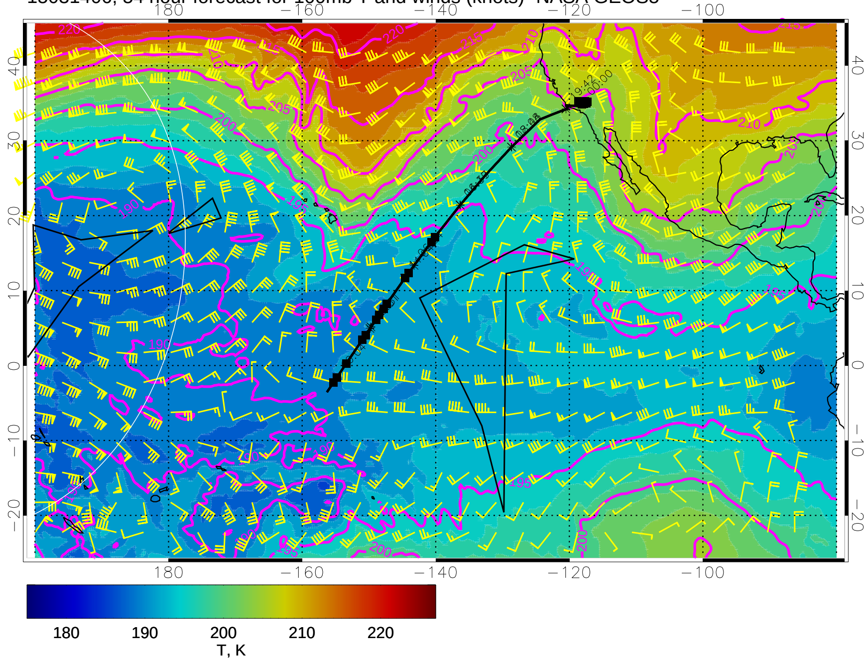
15031406, 54 hour forecast for 100mb T and winds (knots)- NASA GEOS5
