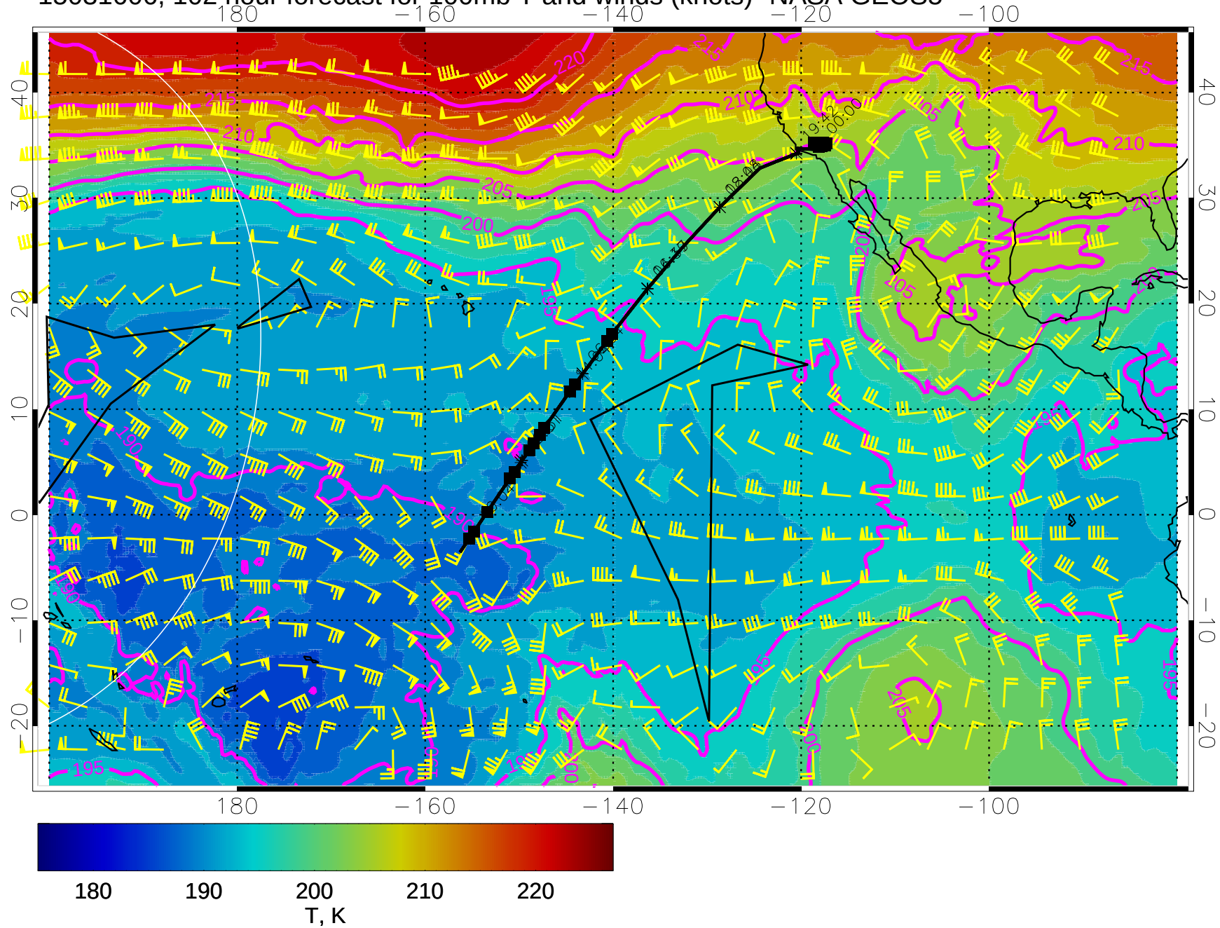
15031606, 102 hour forecast for 100mb T and winds (knots)- NASA GEOS5
