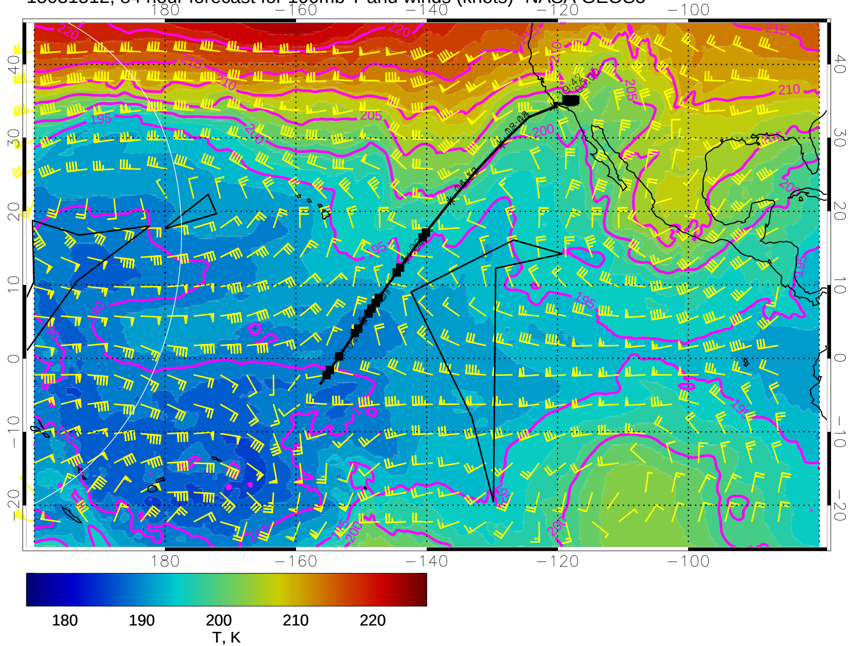
15031512, 84 hour forecast for 100mb T and winds (knots)- NASA GEOS5
