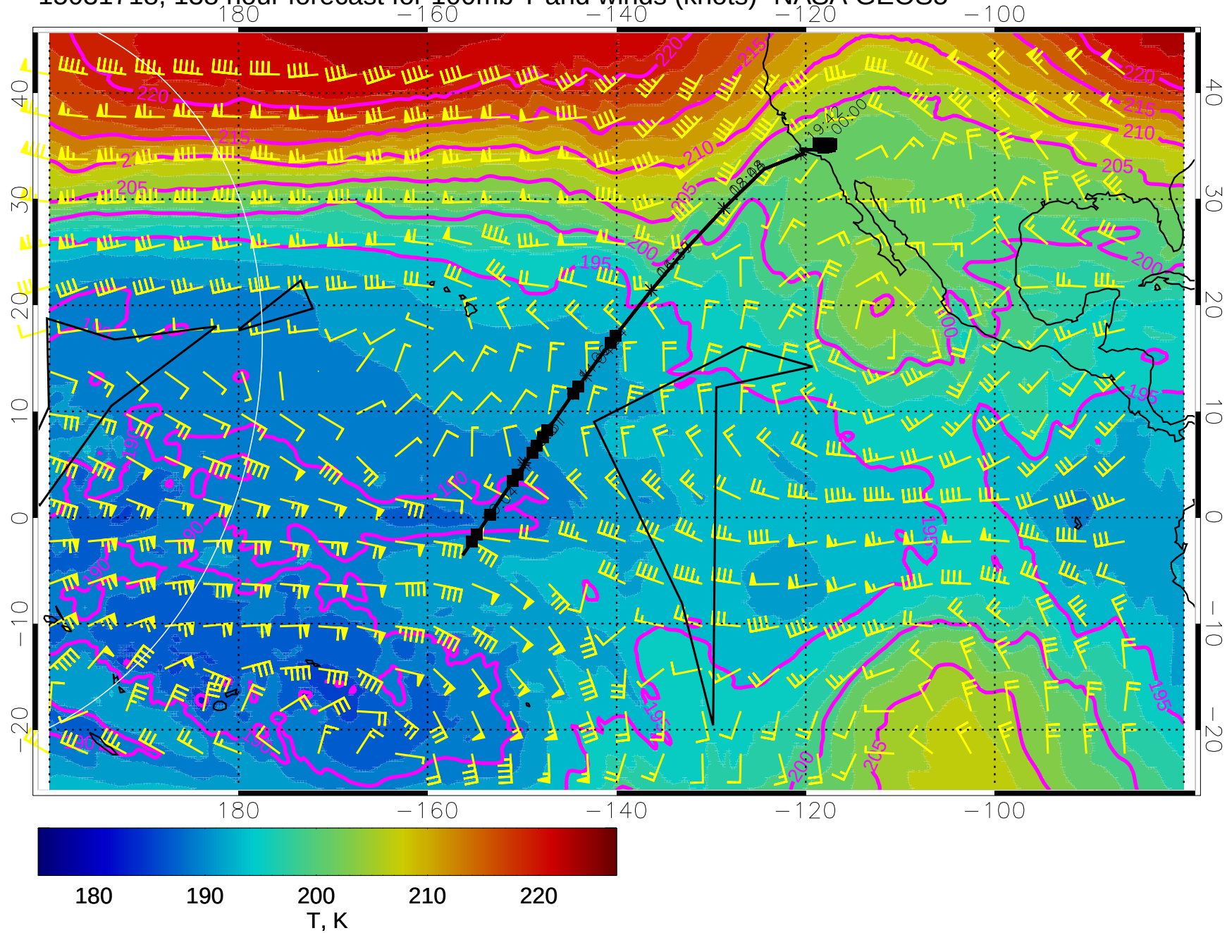
15031718, 138 hour forecast for 100mb T and winds (knots)- NASA GEOS5
