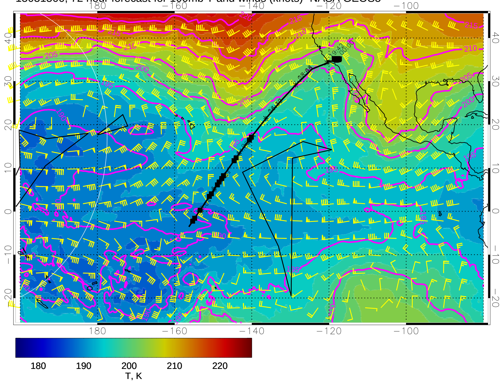
15031500, 72 hour forecast for 100mb T and winds (knots)- NASA GEOS5
