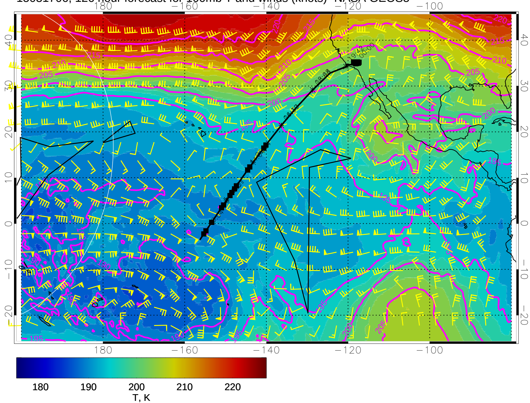
15031706, 126 hour forecast for 100mb T and winds (knots)- NASA GEOS5
