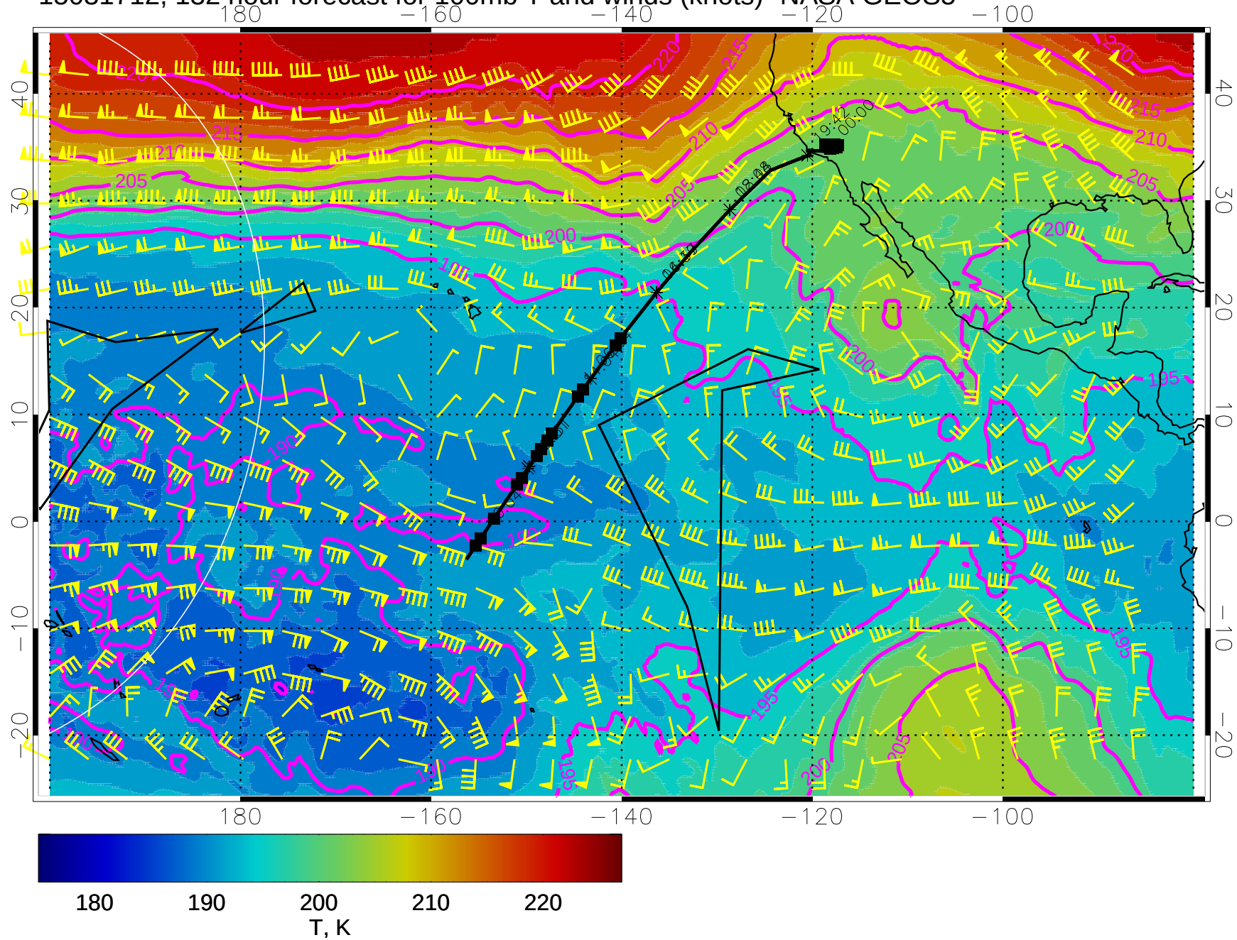
15031712, 132 hour forecast for 100mb T and winds (knots)- NASA GEOS5
