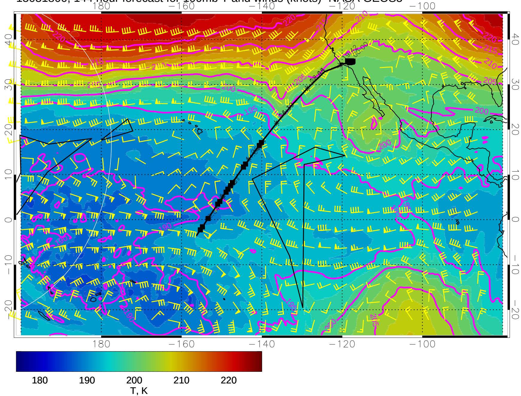
15031800, 144 hour forecast for 100mb T and winds (knots)- NASA GEOS5
