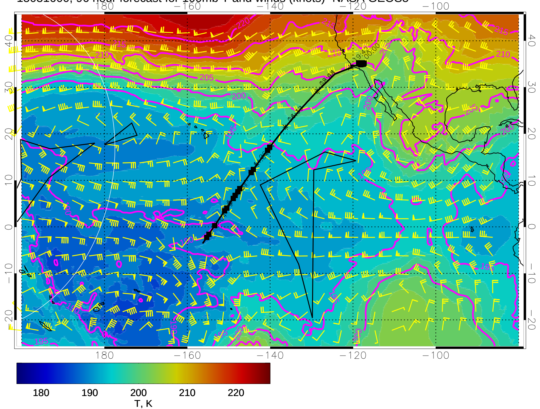
15031600, 96 hour forecast for 100mb T and winds (knots)- NASA GEOS5
