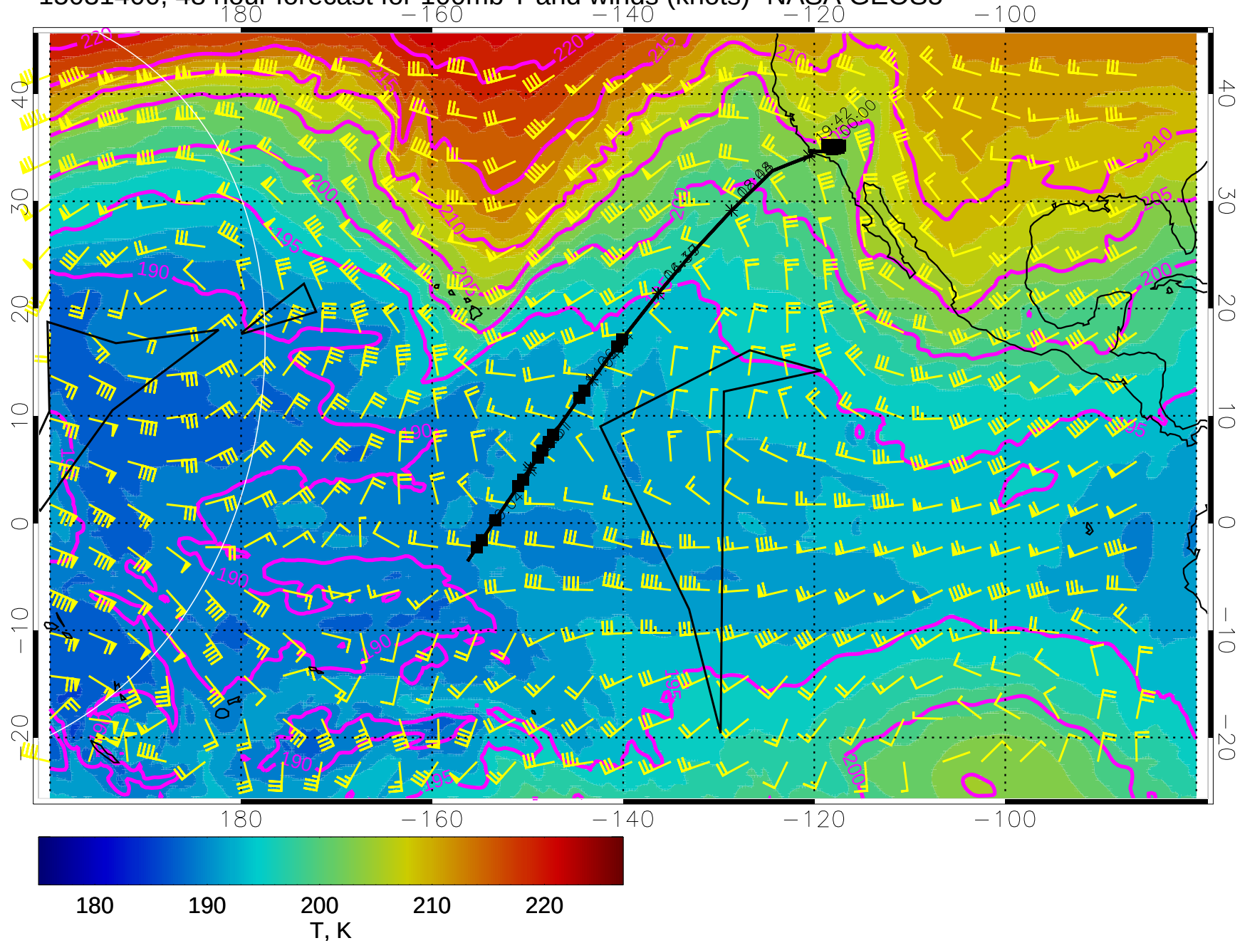
15031400, 48 hour forecast for 100mb T and winds (knots)- NASA GEOS5
