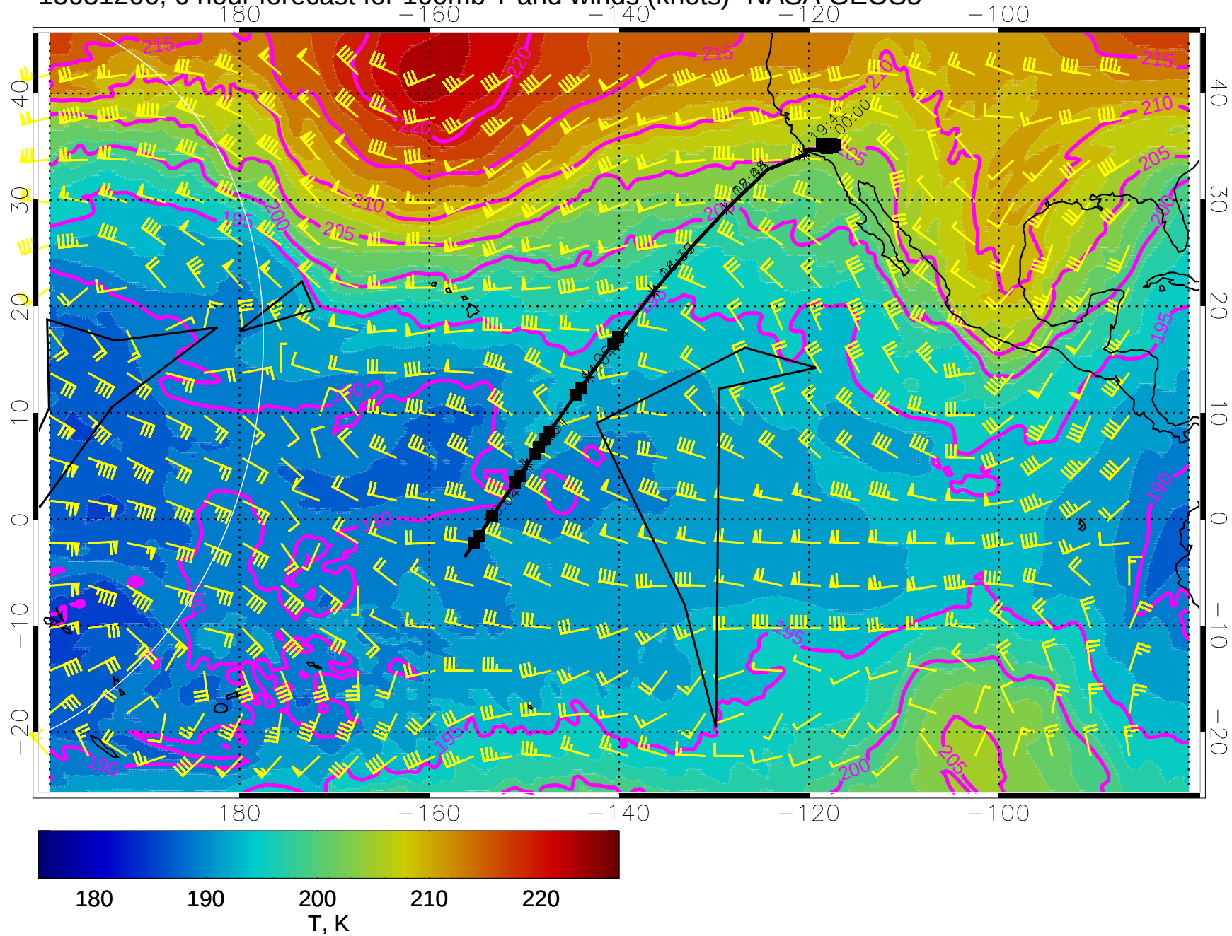
15031206, 6 hour forecast for 100mb T and winds (knots)- NASA GEOS5
