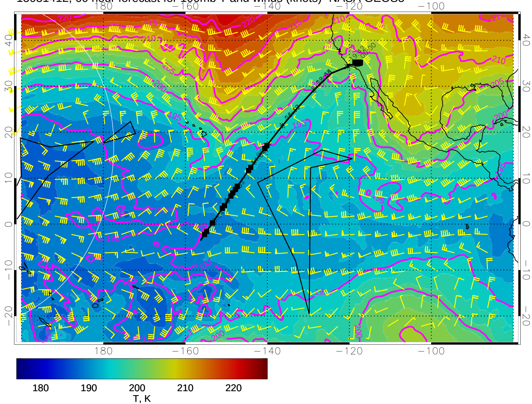
15031412, 60 hour forecast for 100mb T and winds (knots)- NASA GEOS5
