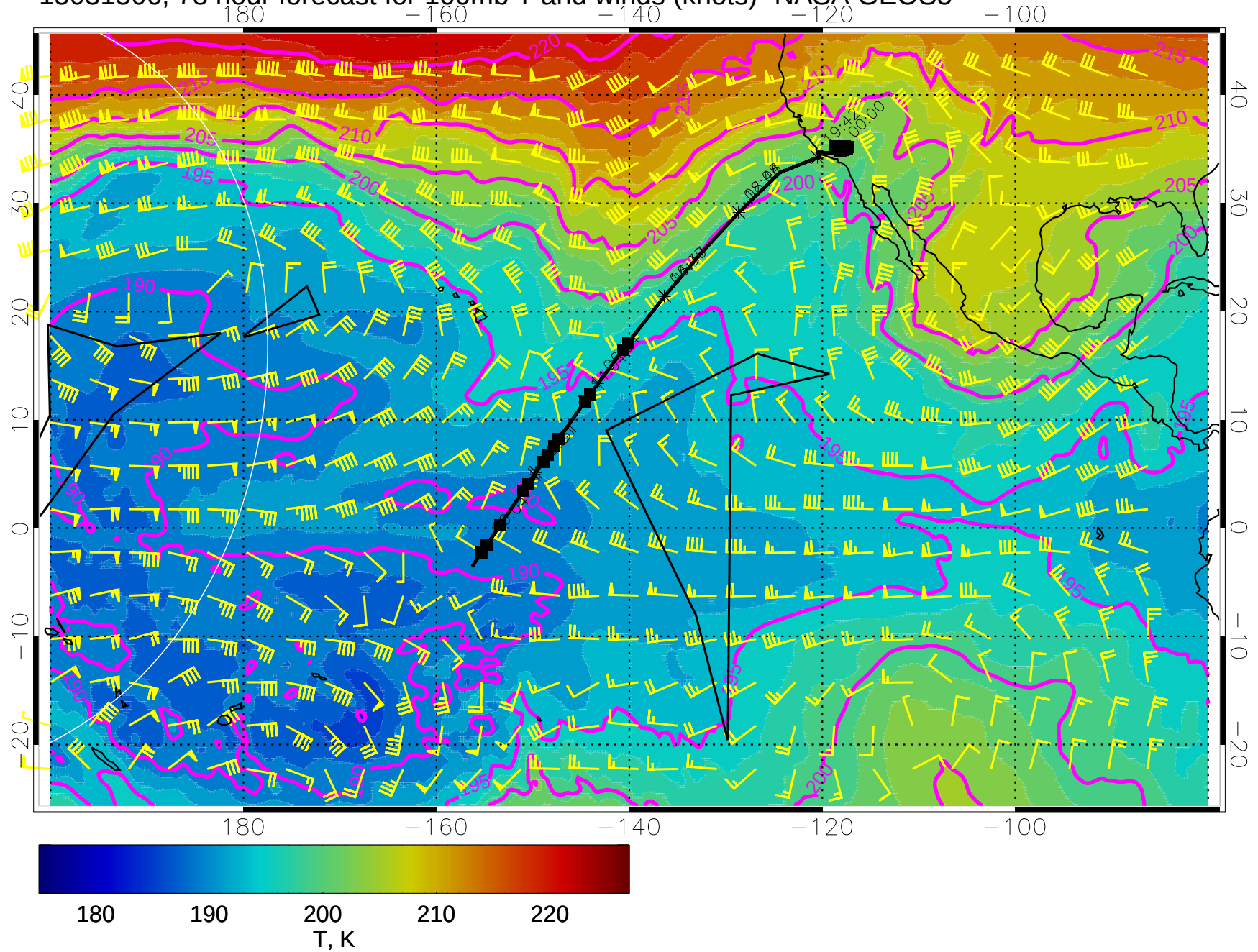
15031506, 78 hour forecast for 100mb T and winds (knots)- NASA GEOS5
