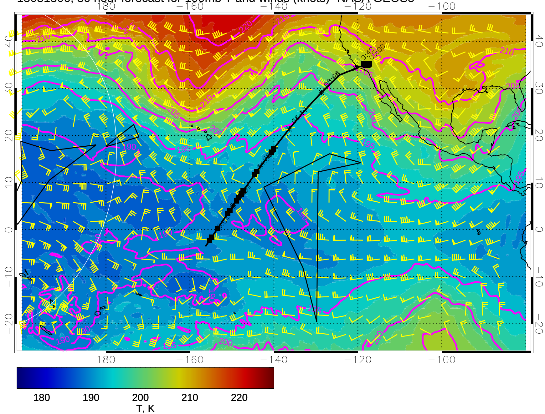
15031306, 30 hour forecast for 100mb T and winds (knots)- NASA GEOS5
