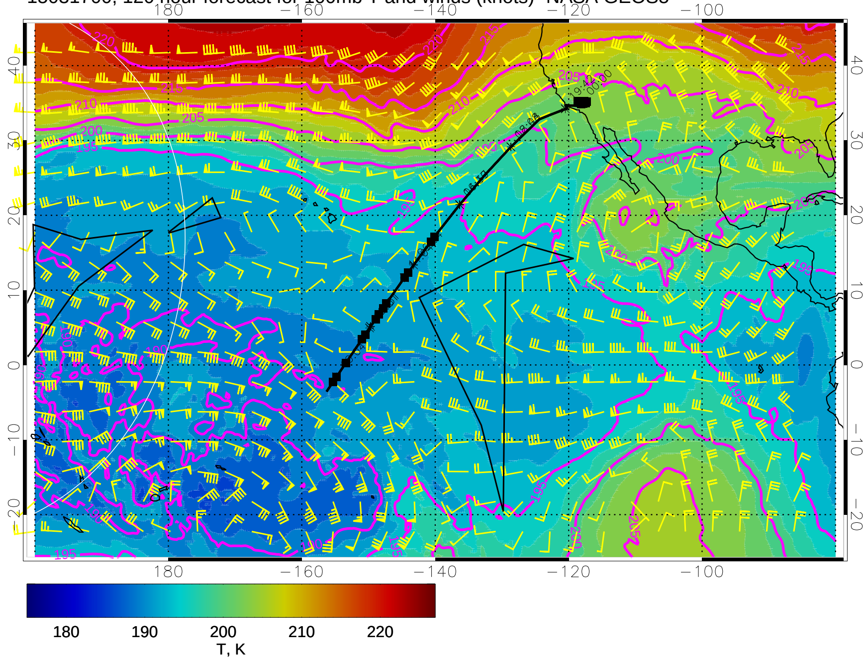
15031700, 120 hour forecast for 100mb T and winds (knots)- NASA GEOS5
