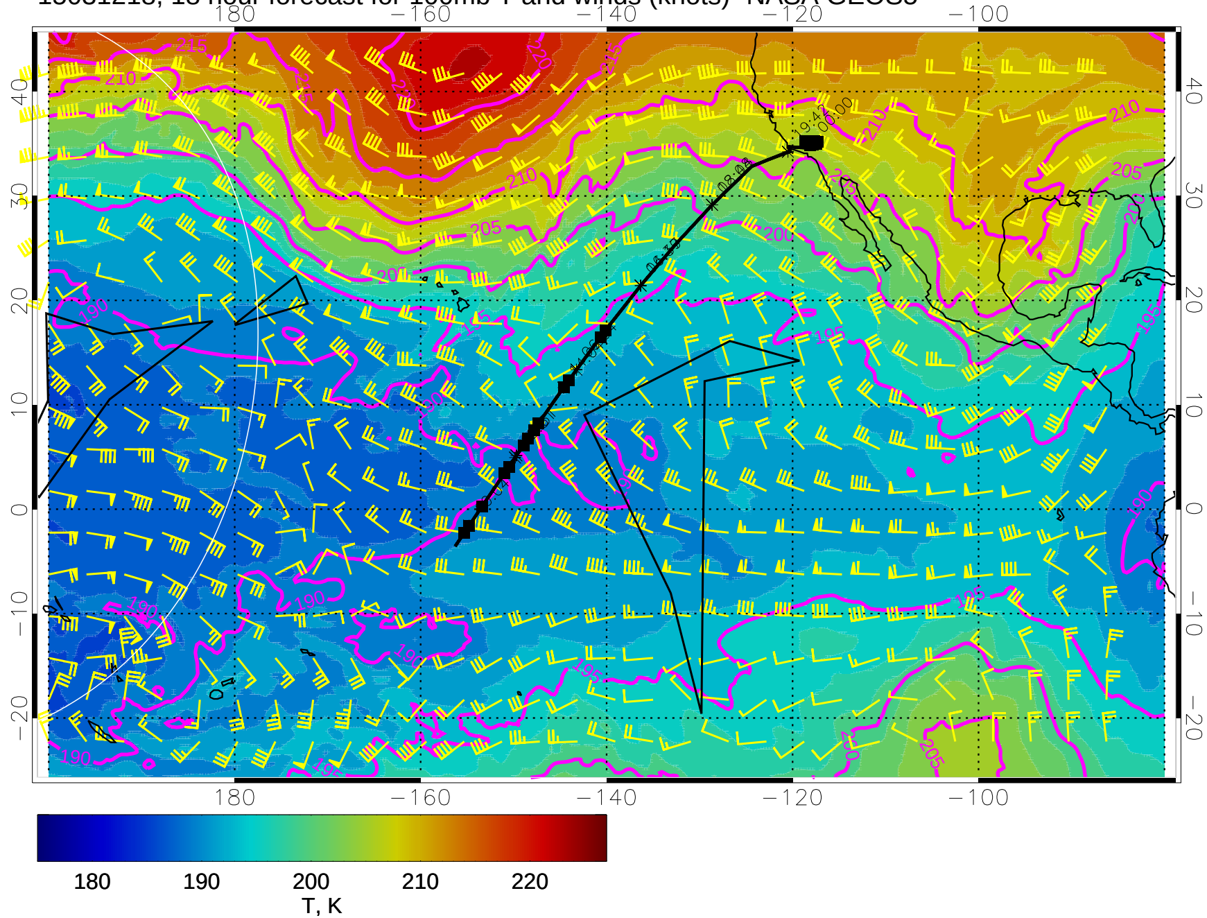
15031218, 18 hour forecast for 100mb T and winds (knots)- NASA GEOS5
