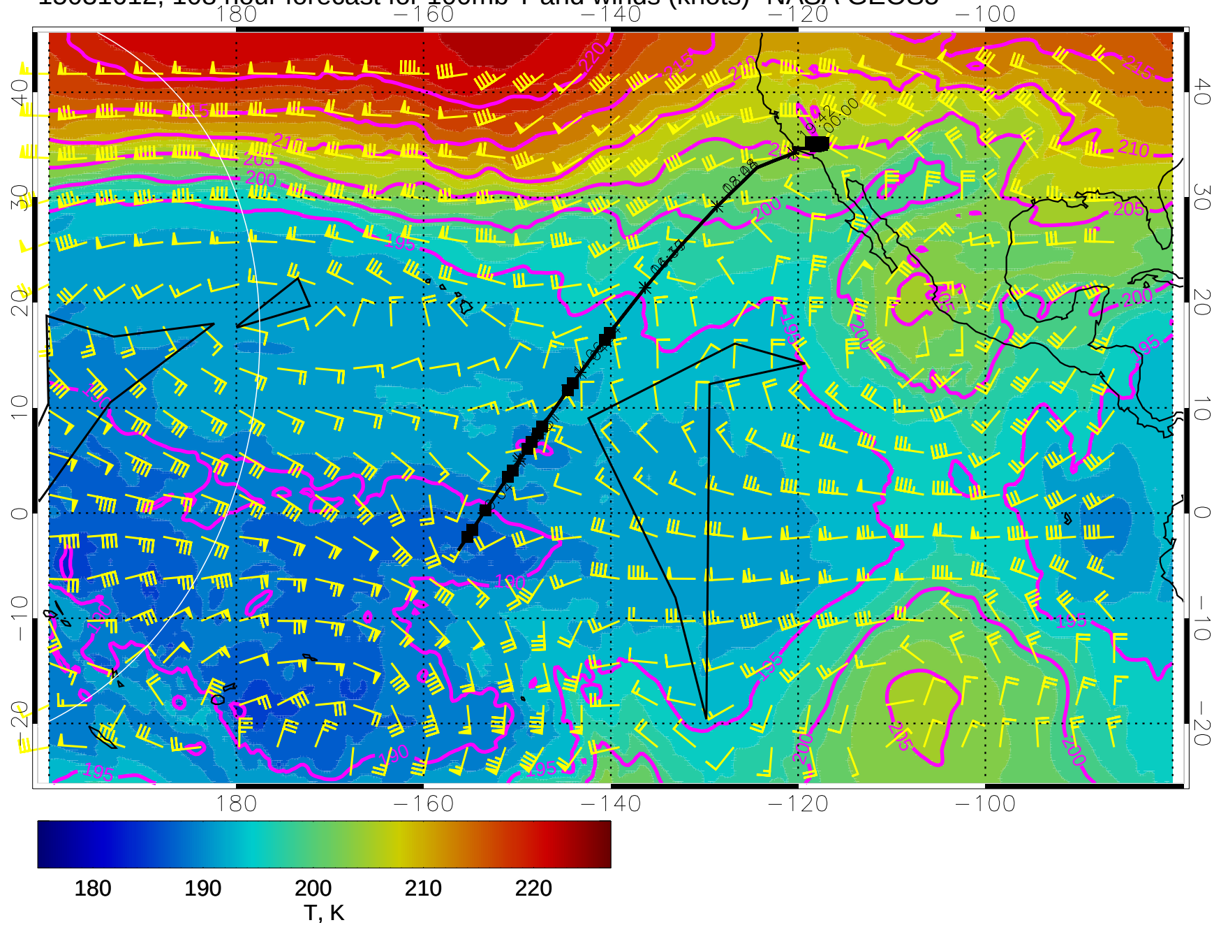
15031612, 108 hour forecast for 100mb T and winds (knots)- NASA GEOS5
