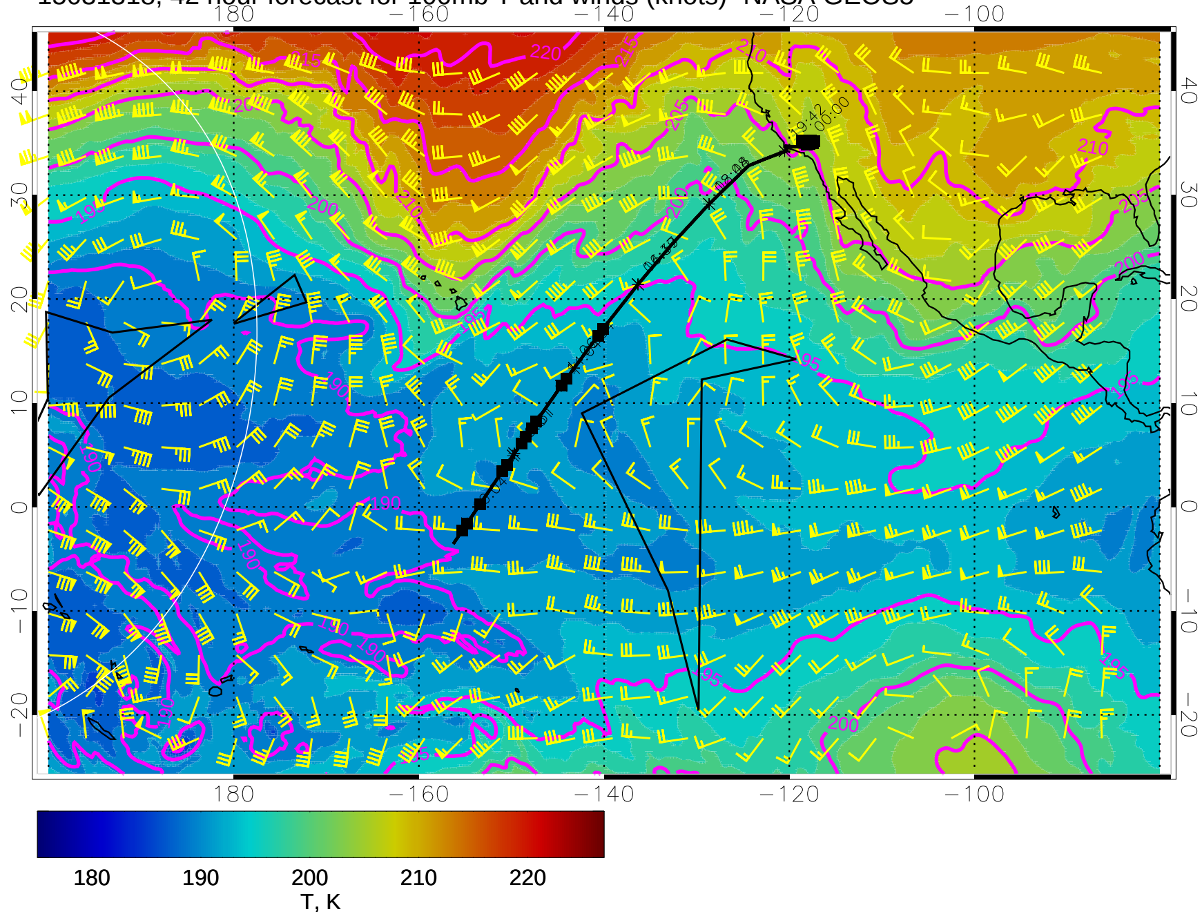
15031318, 42 hour forecast for 100mb T and winds (knots)- NASA GEOS5
