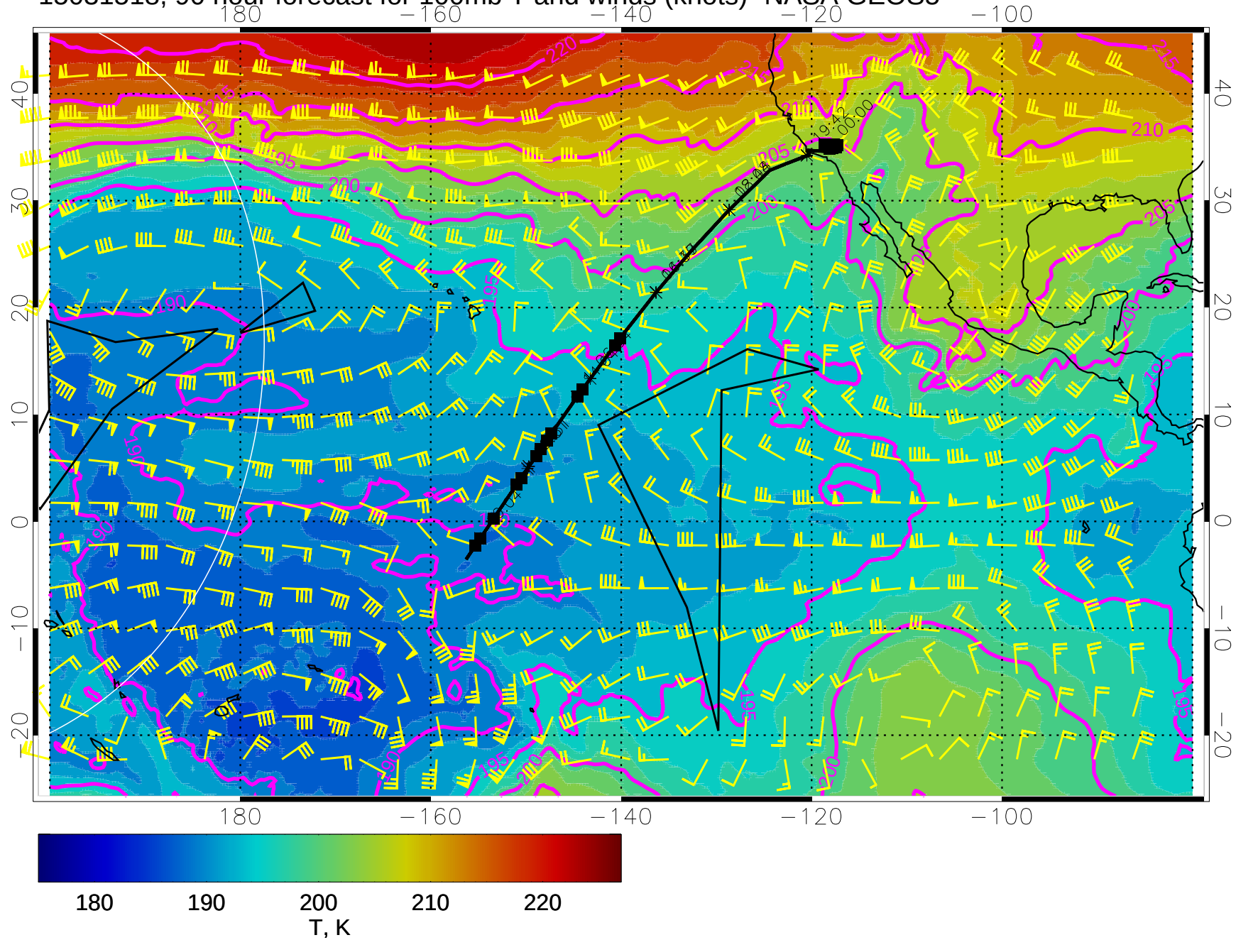
15031518, 90 hour forecast for 100mb T and winds (knots)- NASA GEOS5
