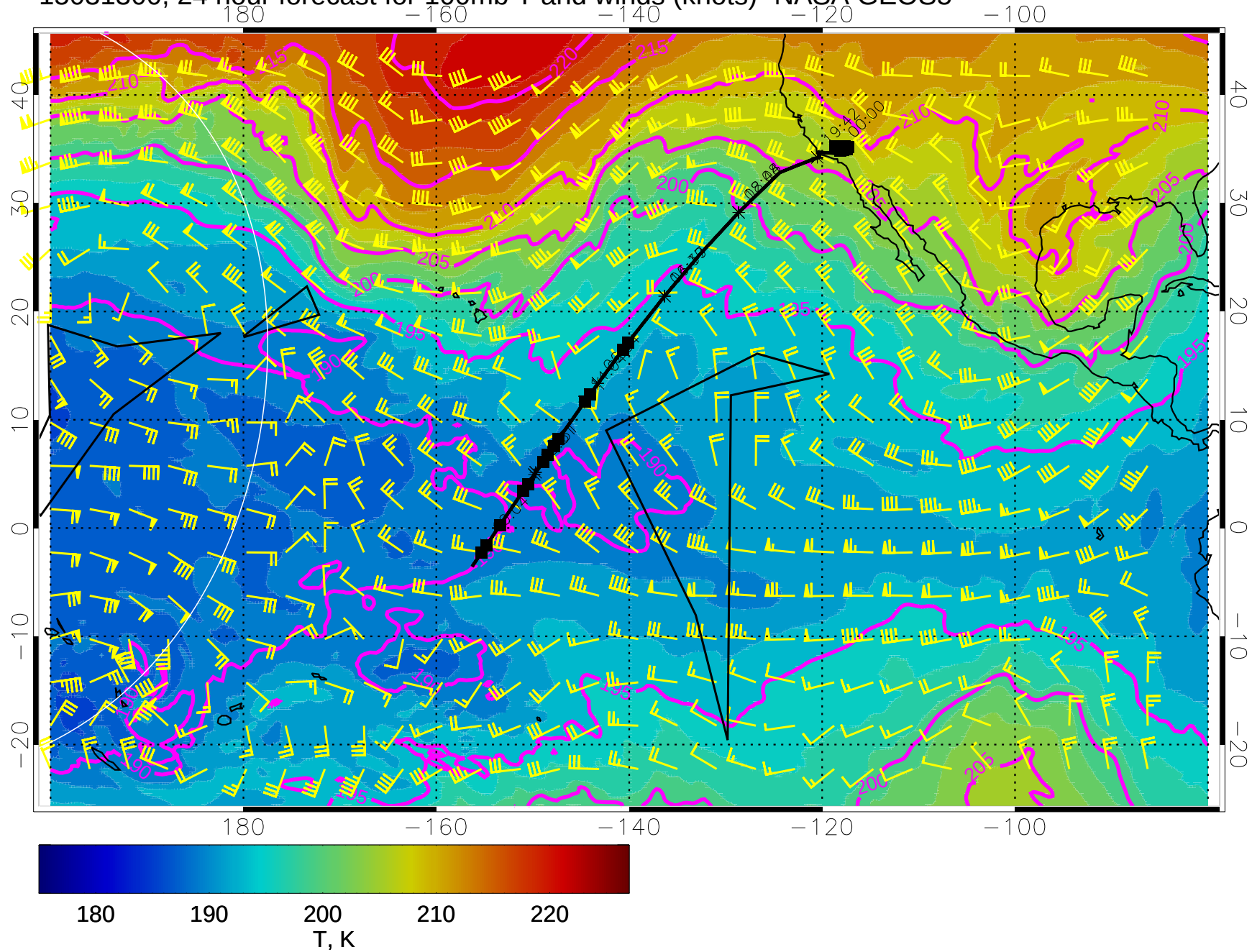
15031300, 24 hour forecast for 100mb T and winds (knots)- NASA GEOS5
