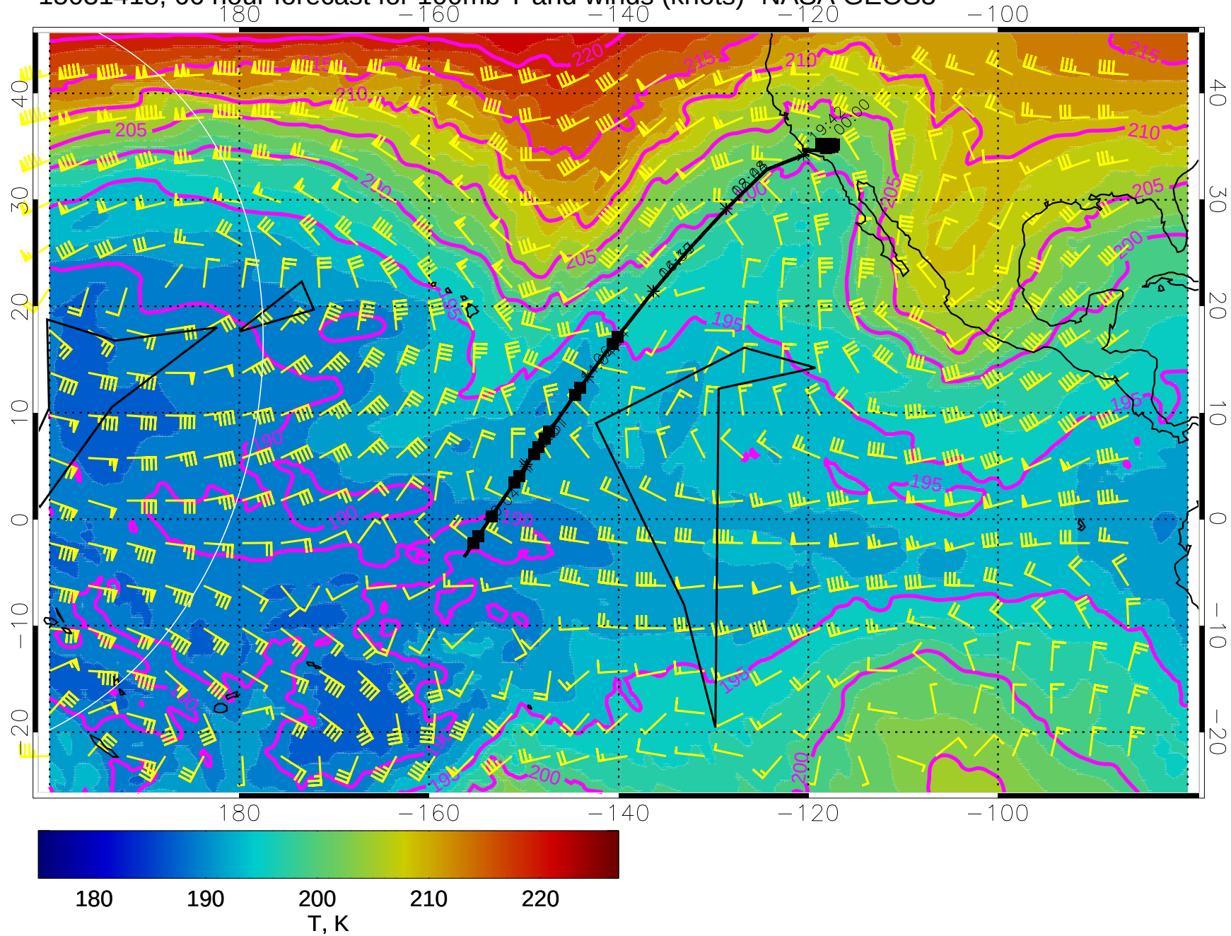
15031418, 66 hour forecast for 100mb T and winds (knots)- NASA GEOS5
