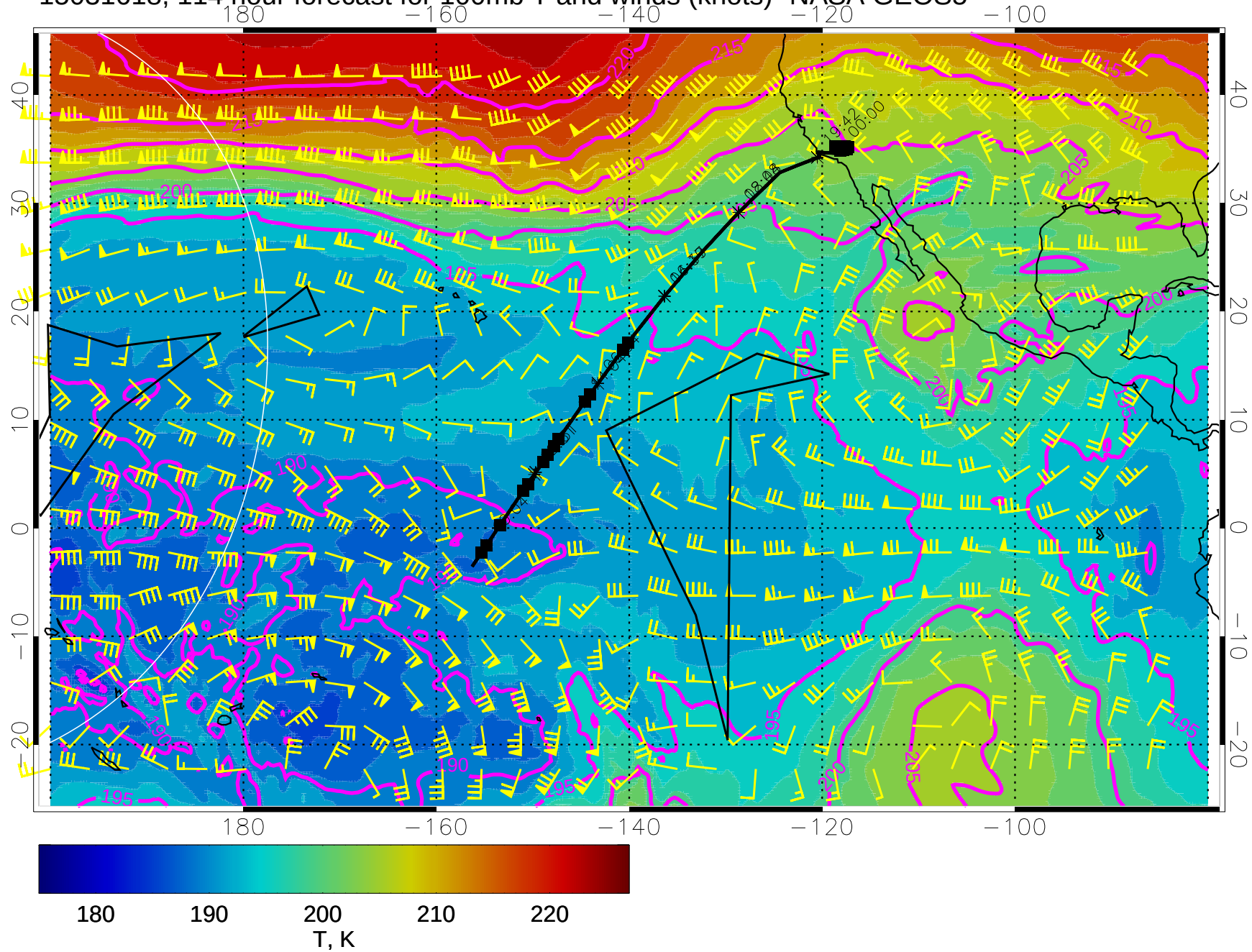
15031618, 114 hour forecast for 100mb T and winds (knots)- NASA GEOS5
