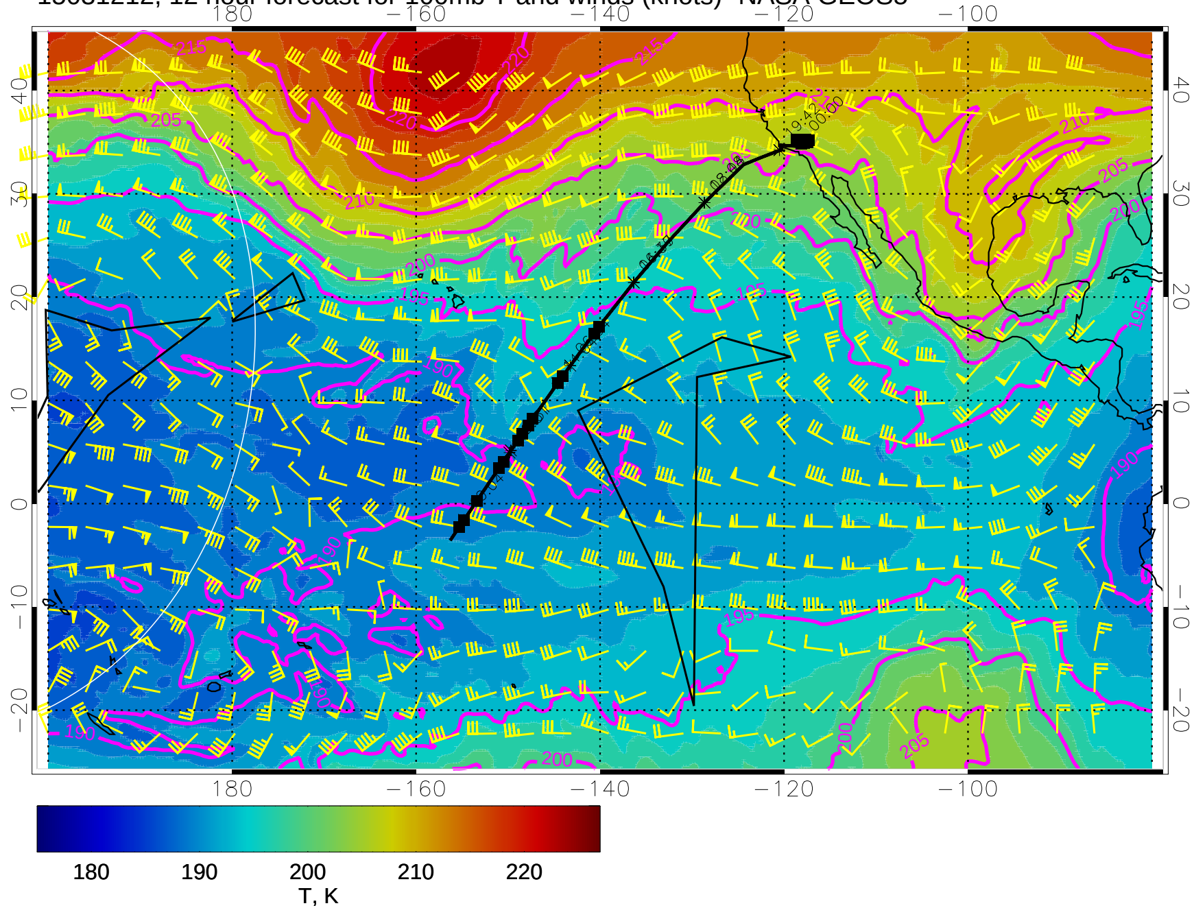
15031212, 12 hour forecast for 100mb T and winds (knots)- NASA GEOS5
