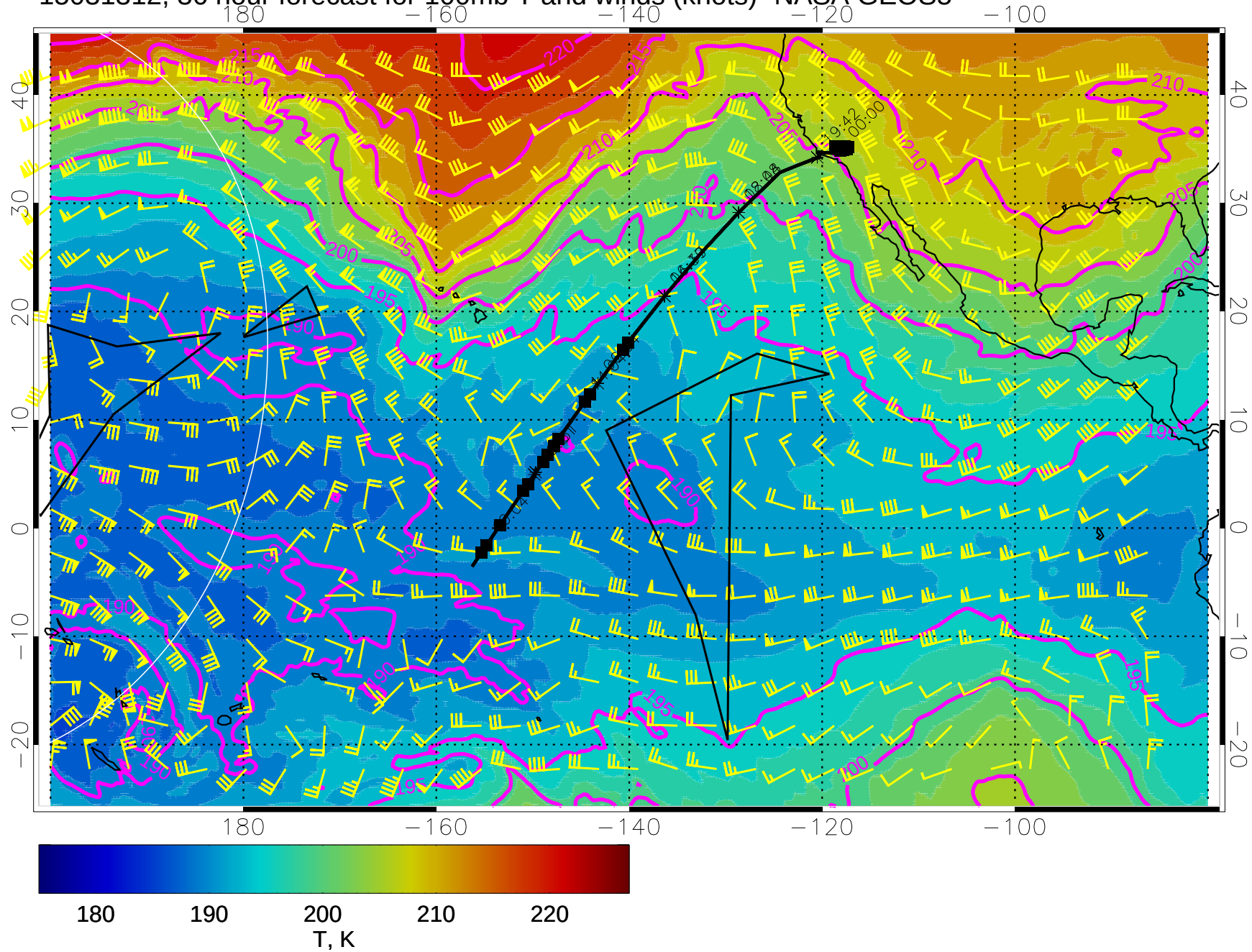
15031312, 36 hour forecast for 100mb T and winds (knots)- NASA GEOS5
