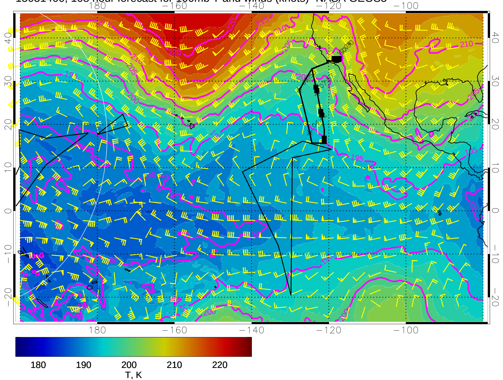
15031400, 108 hour forecast for 100mb T and winds (knots)- NASA GEOS5
