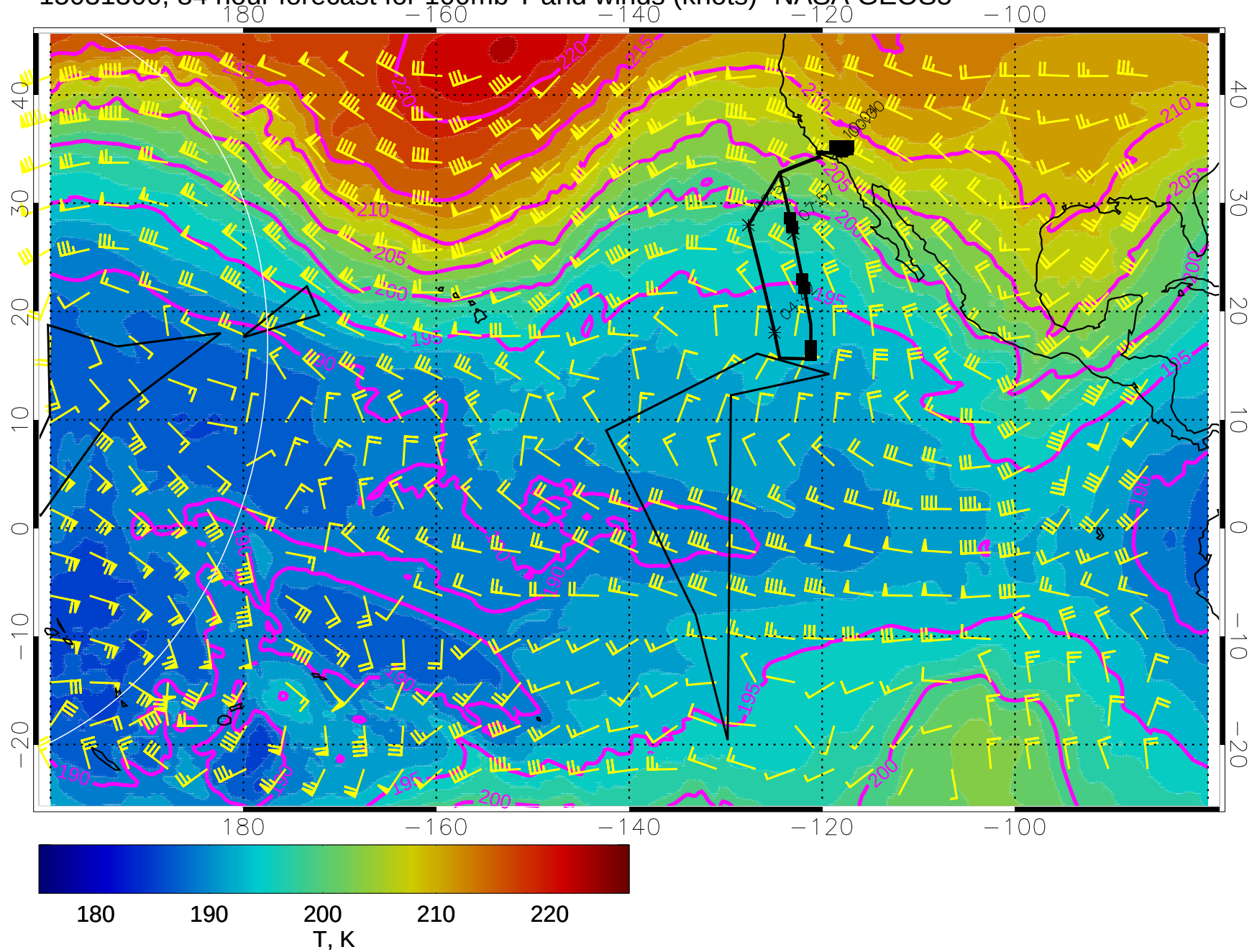
15031300, 84 hour forecast for 100mb T and winds (knots)- NASA GEOS5
