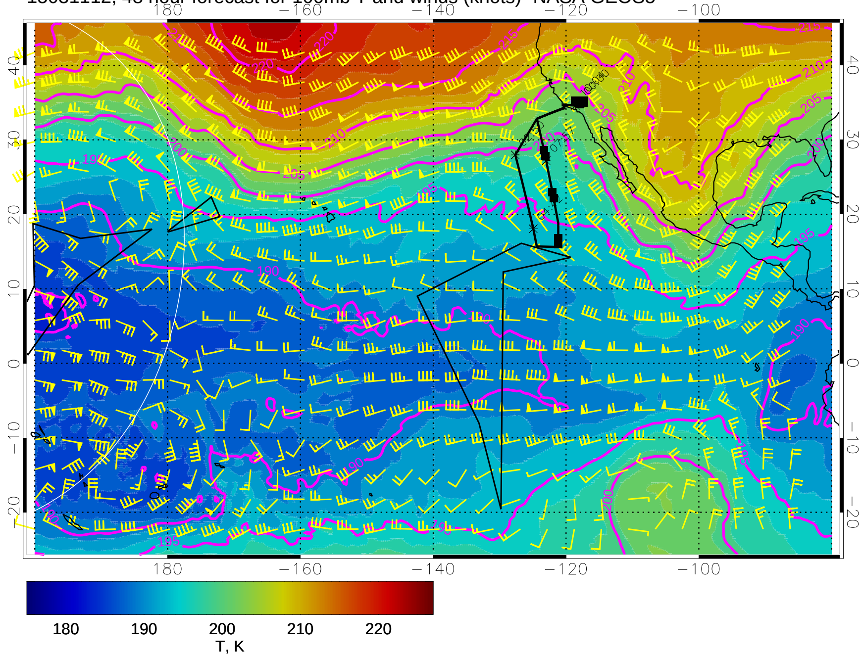
15031112, 48 hour forecast for 100mb T and winds (knots)- NASA GEOS5
