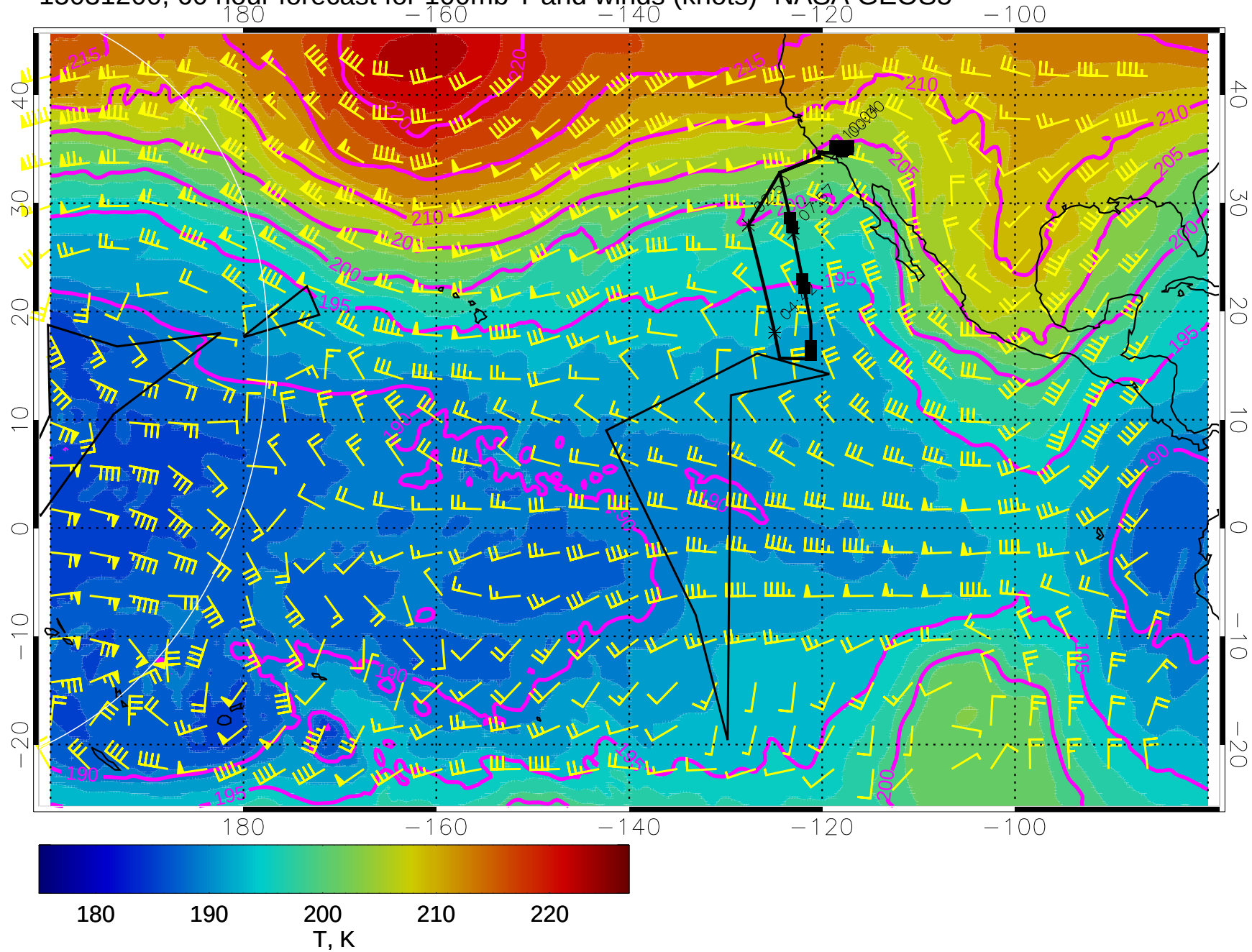
15031200, 60 hour forecast for 100mb T and winds (knots)- NASA GEOS5
