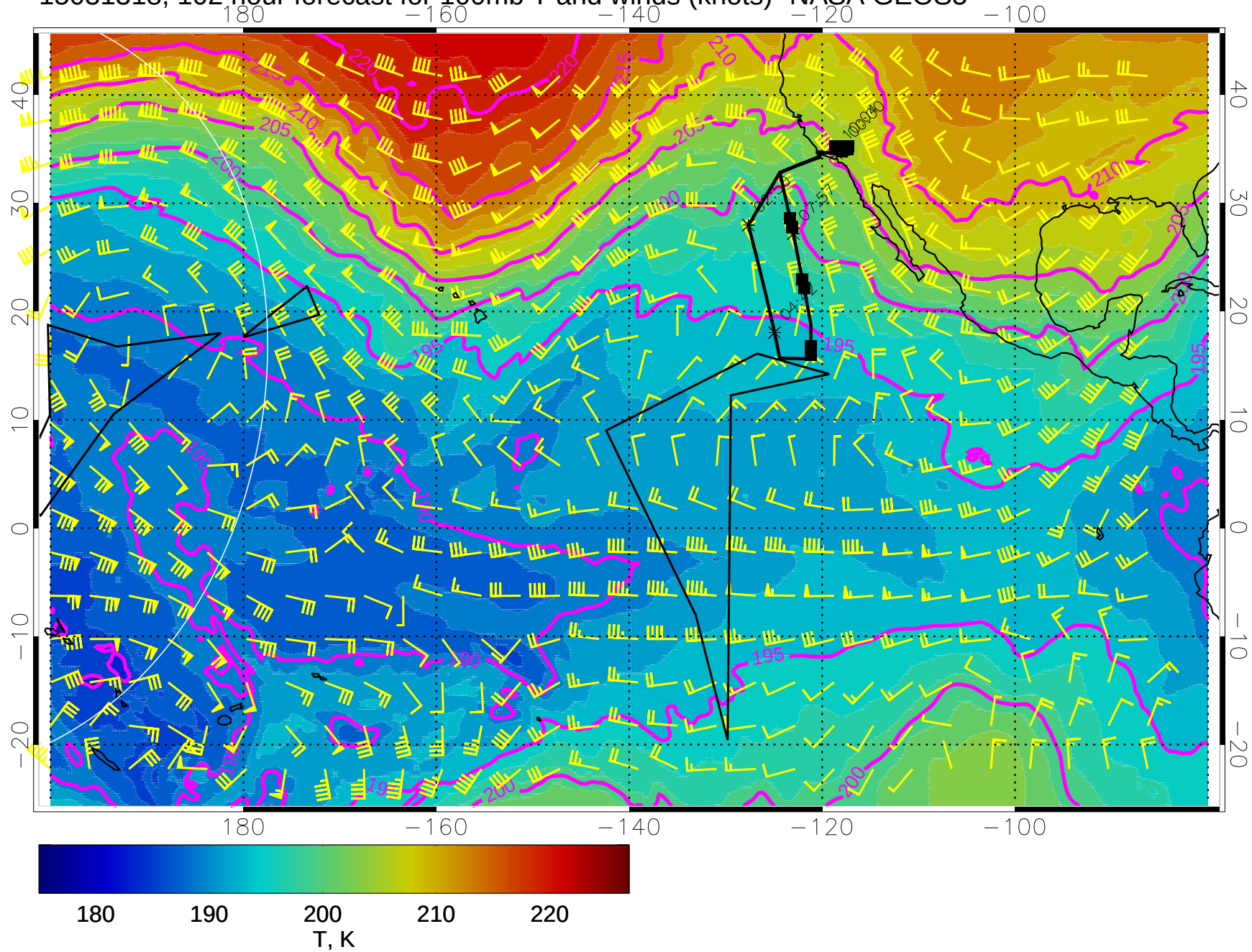
15031318, 102 hour forecast for 100mb T and winds (knots)- NASA GEOS5
