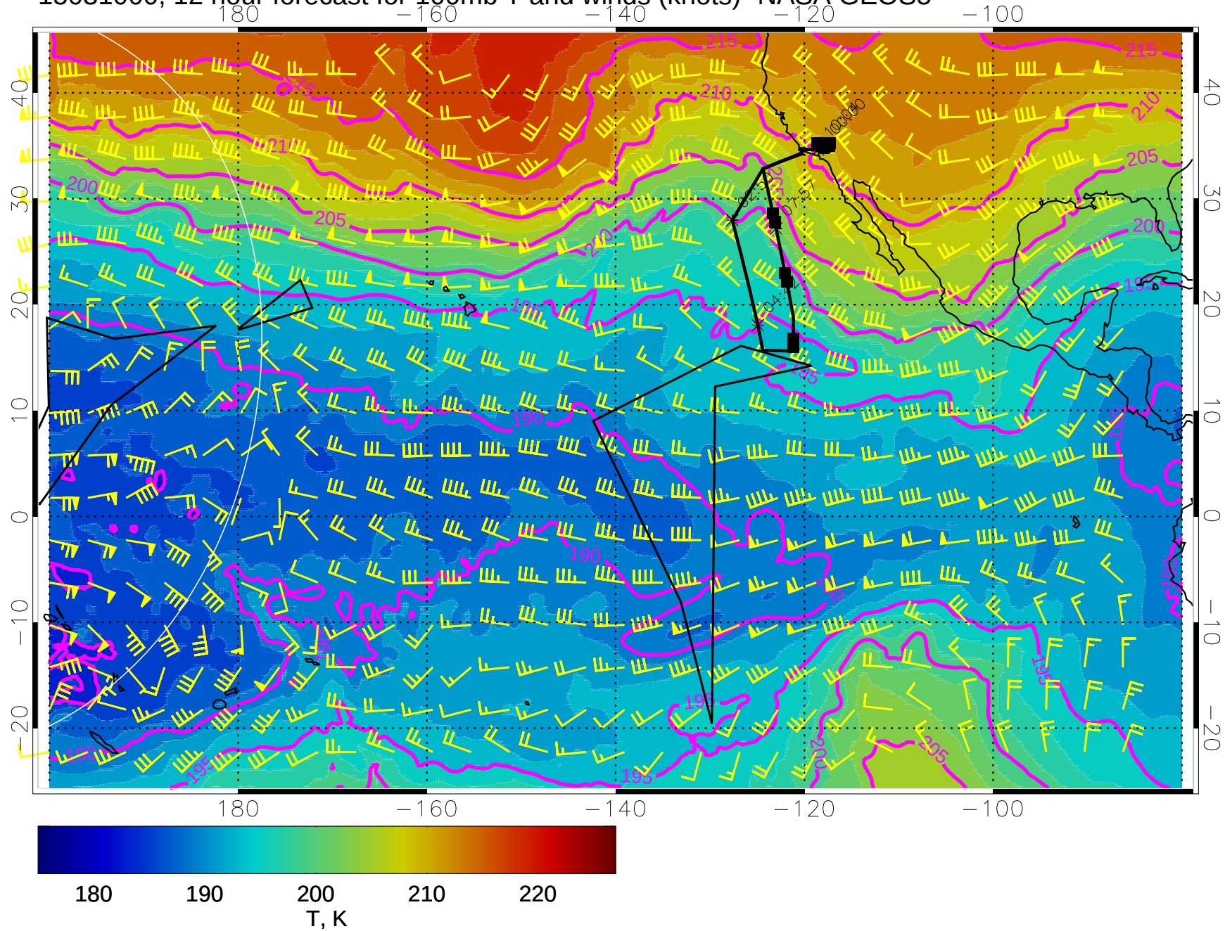
15031000, 12 hour forecast for 100mb T and winds (knots)- NASA GEOS5
