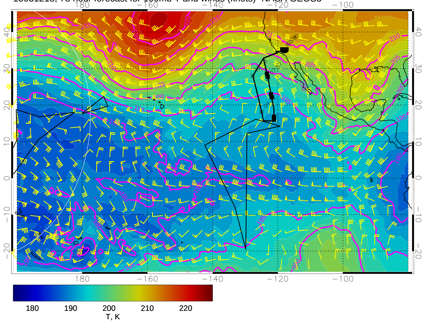
15031218, 78 hour forecast for 100mb T and winds (knots)- NASA GEOS5
