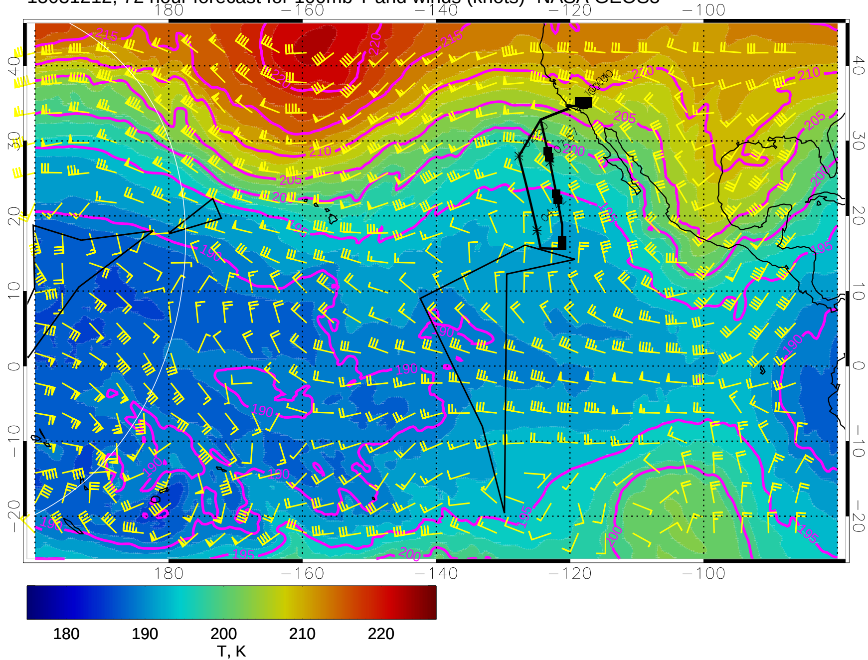
15031212, 72 hour forecast for 100mb T and winds (knots)- NASA GEOS5
