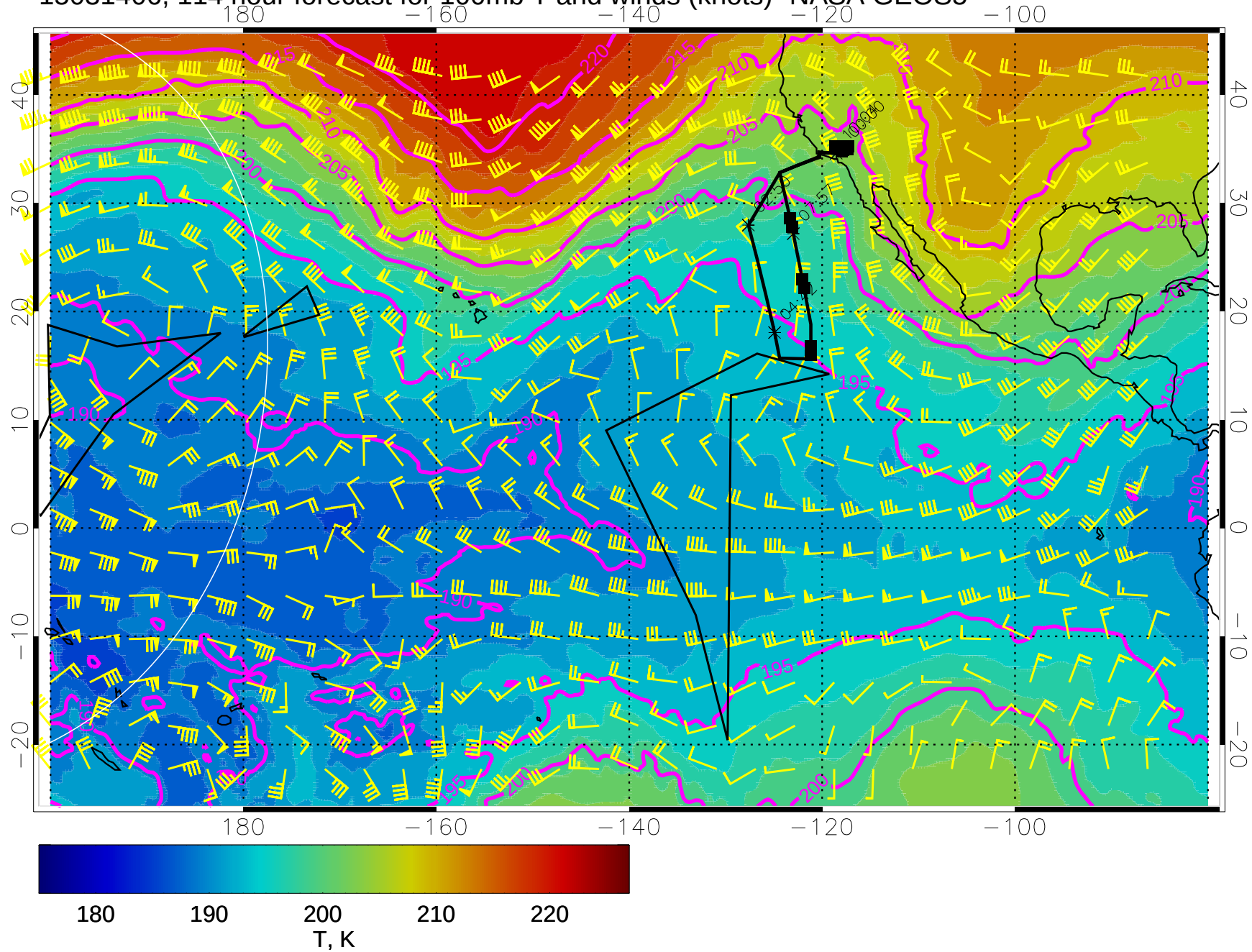
15031406, 114 hour forecast for 100mb T and winds (knots)- NASA GEOS5
