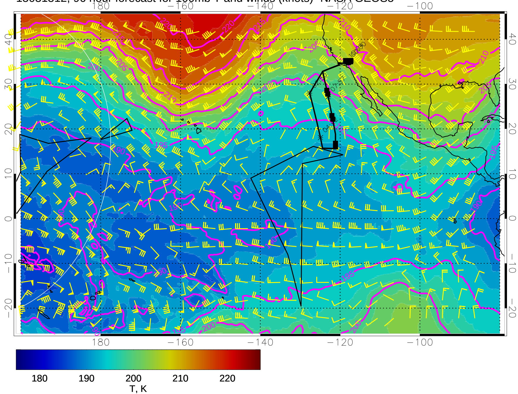
15031312, 96 hour forecast for 100mb T and winds (knots)- NASA GEOS5
