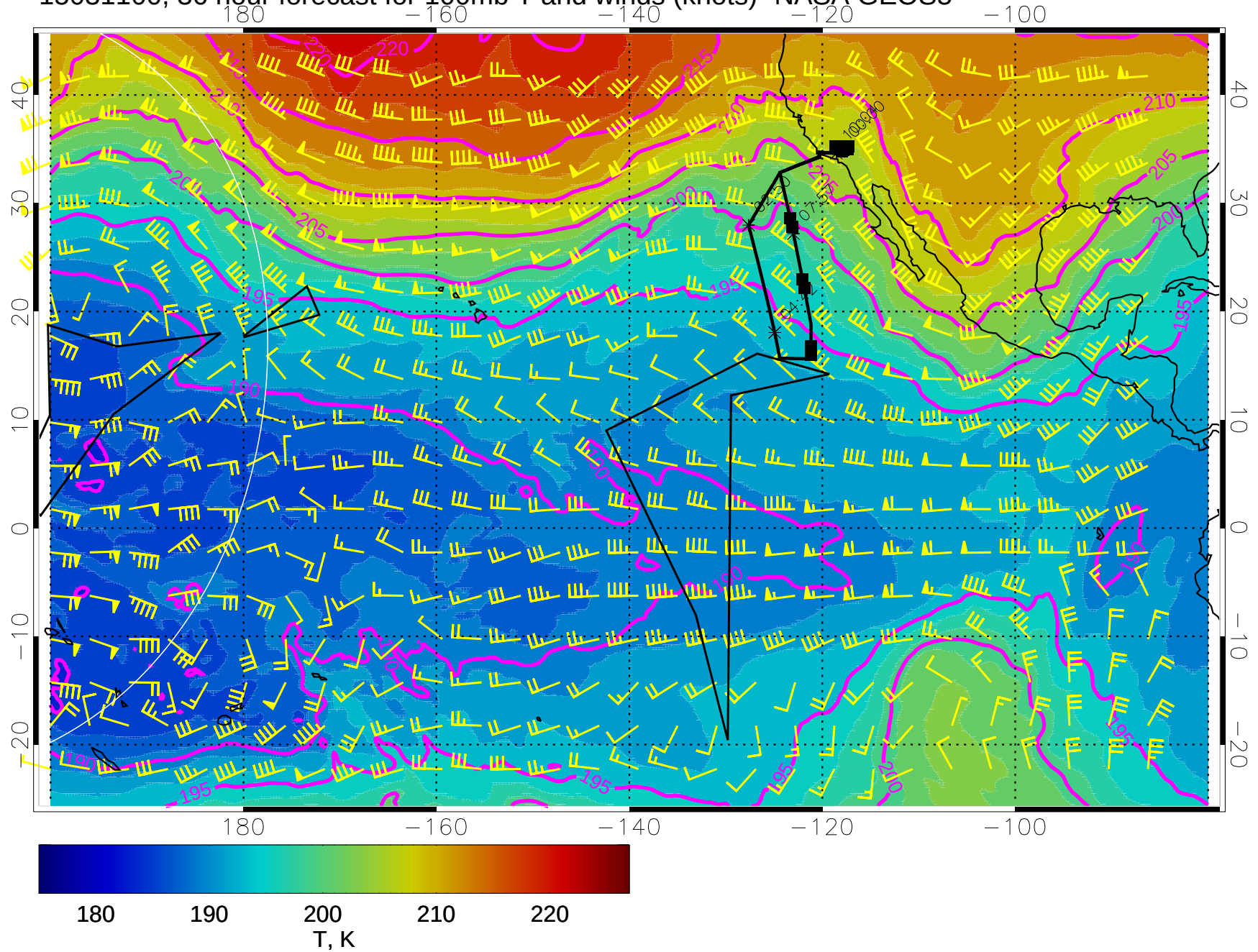
15031100, 36 hour forecast for 100mb T and winds (knots)- NASA GEOS5
