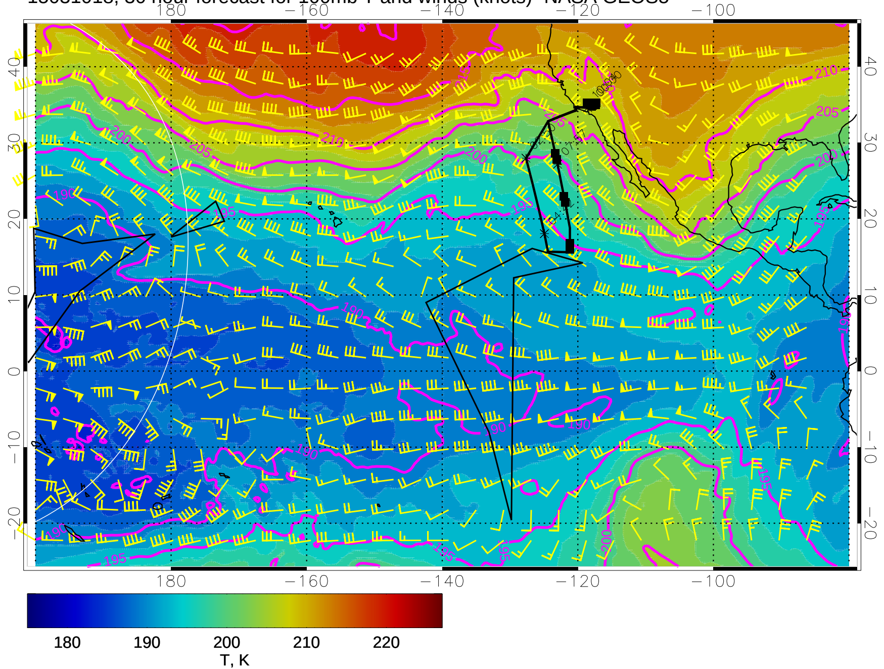
15031018, 30 hour forecast for 100mb T and winds (knots)- NASA GEOS5
