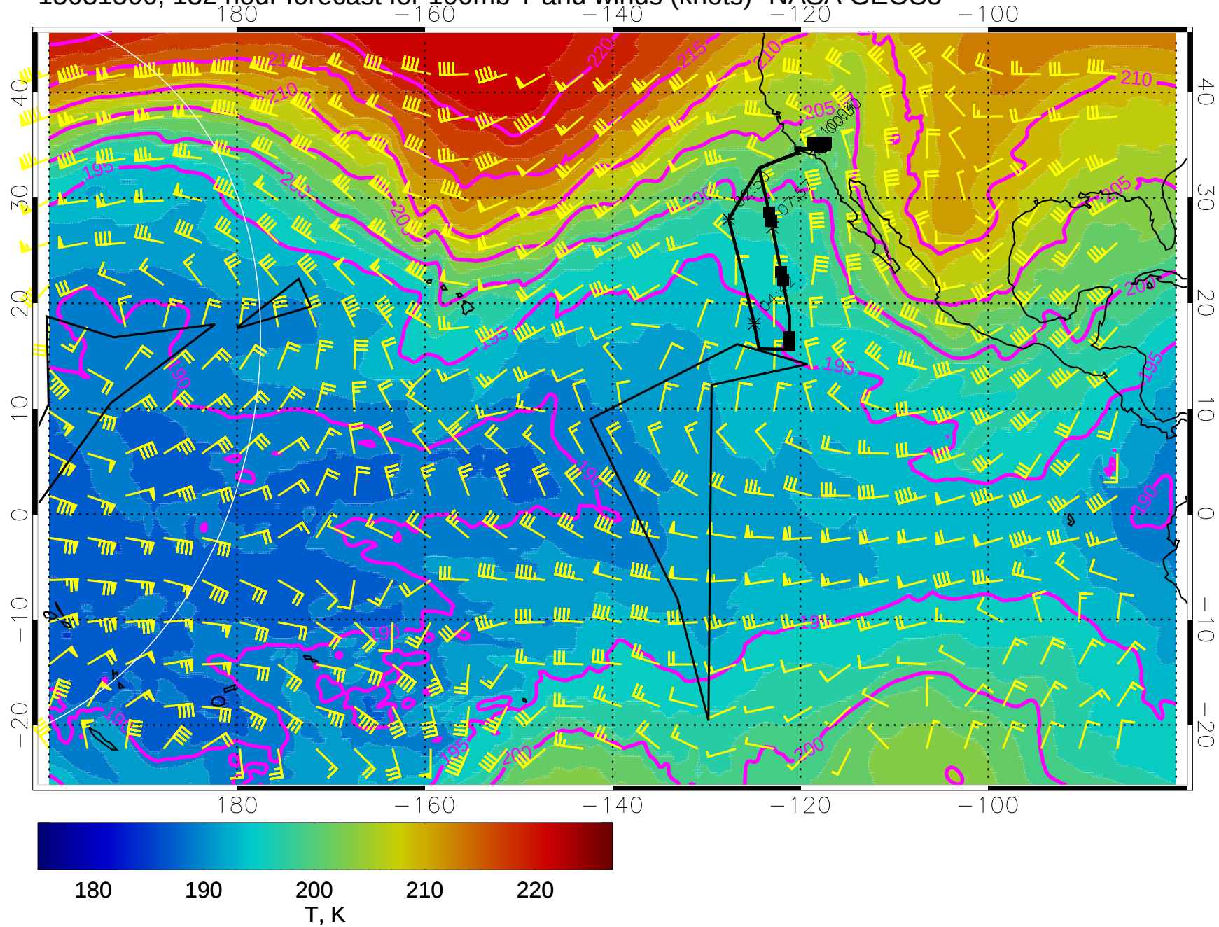
15031500, 132 hour forecast for 100mb T and winds (knots)- NASA GEOS5
