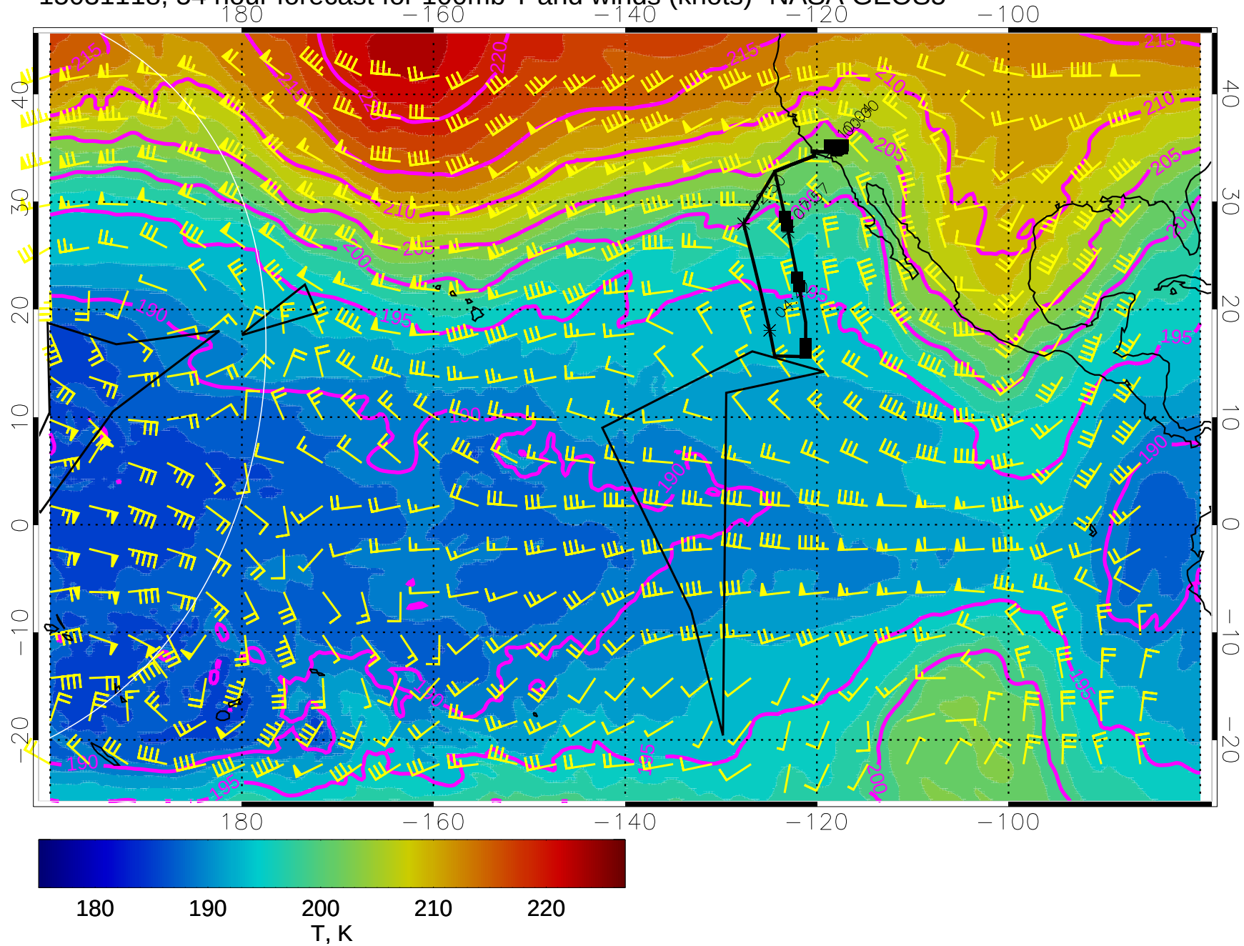
15031118, 54 hour forecast for 100mb T and winds (knots)- NASA GEOS5
