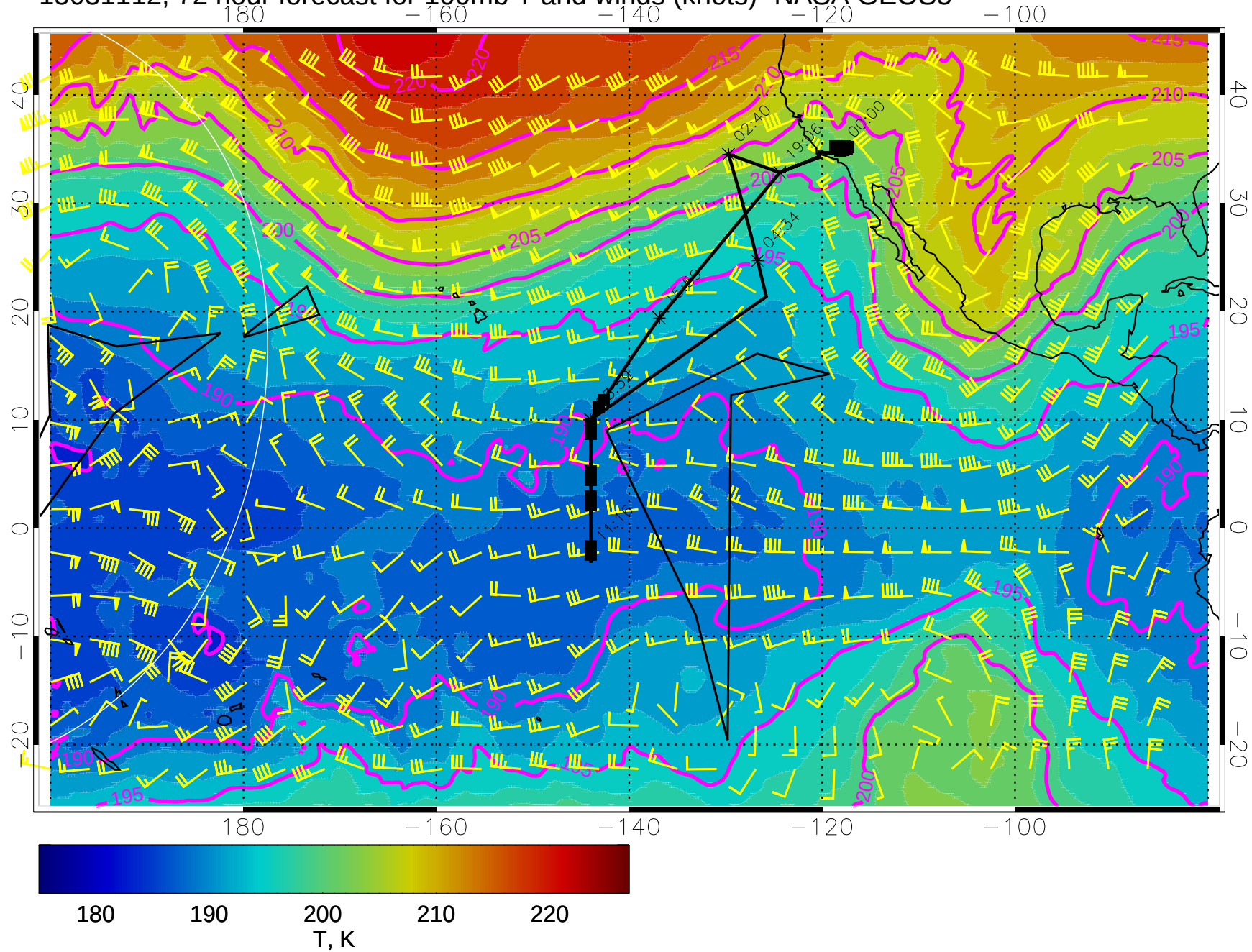
15031112, 72 hour forecast for 100mb T and winds (knots)- NASA GEOS5
