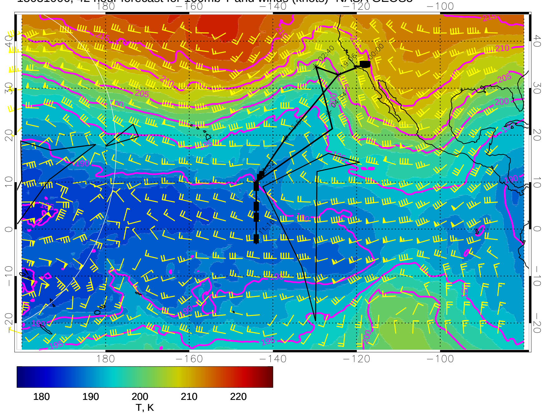
15031006, 42 hour forecast for 100mb T and winds (knots)- NASA GEOS5
