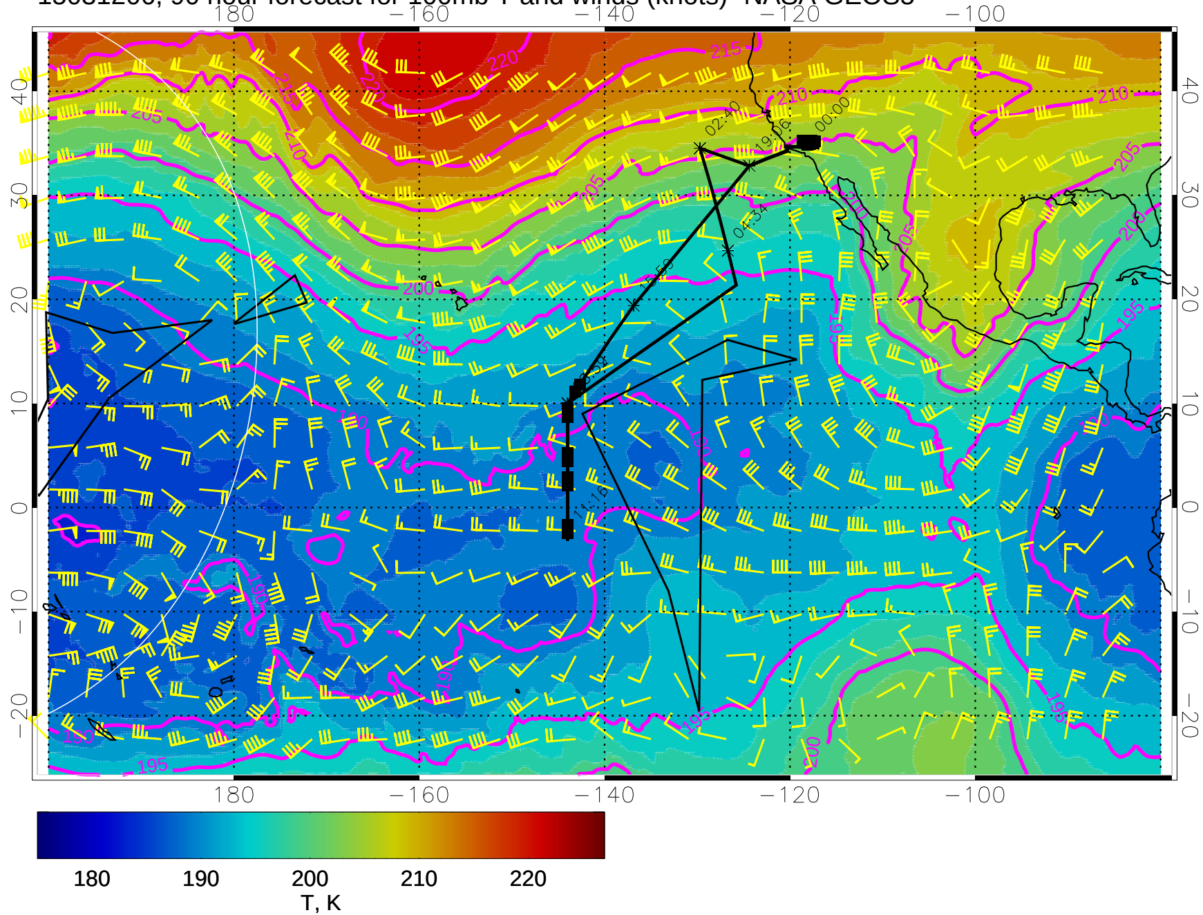
15031206, 90 hour forecast for 100mb T and winds (knots)- NASA GEOS5
