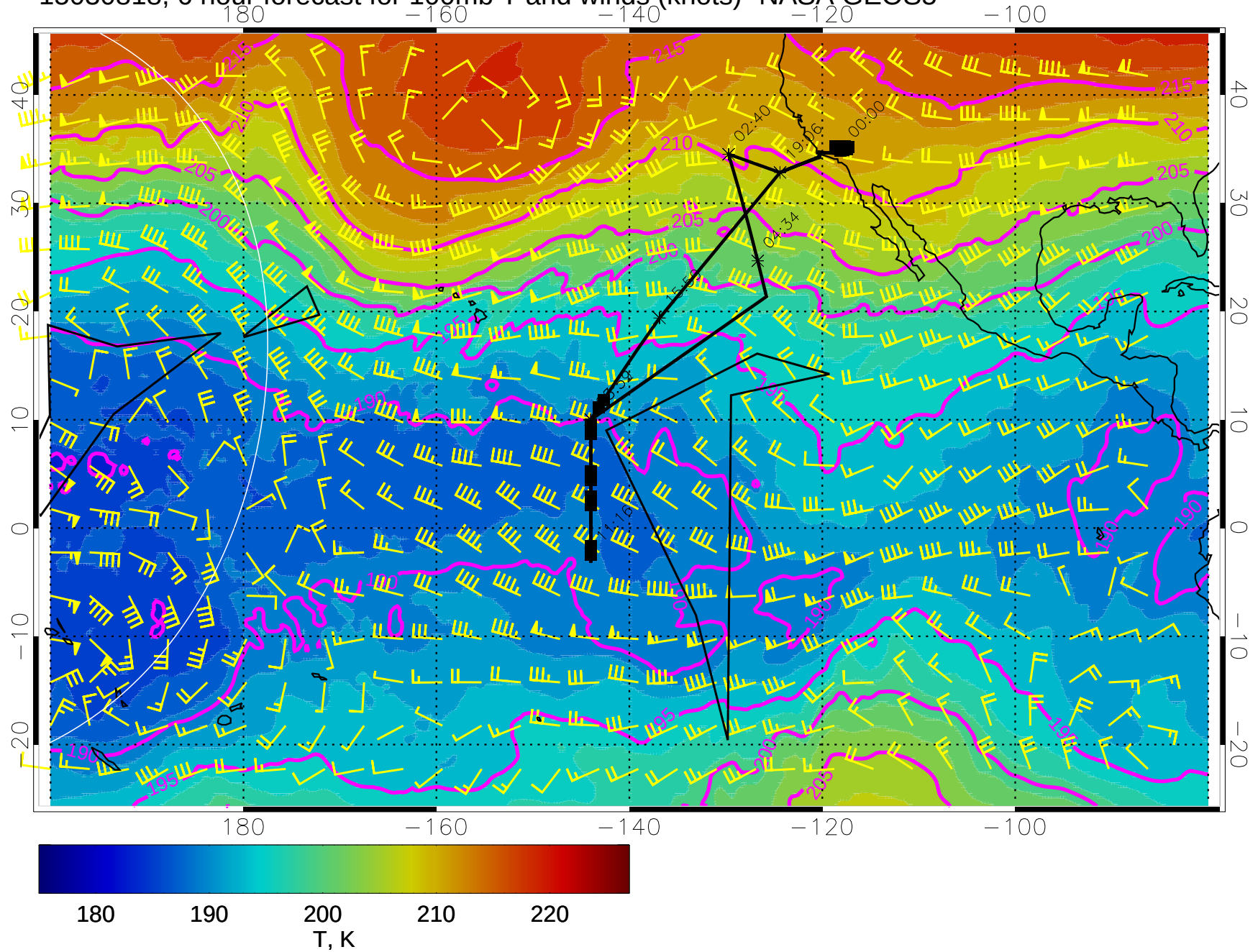
15030818, 6 hour forecast for 100mb T and winds (knots)- NASA GEOS5
