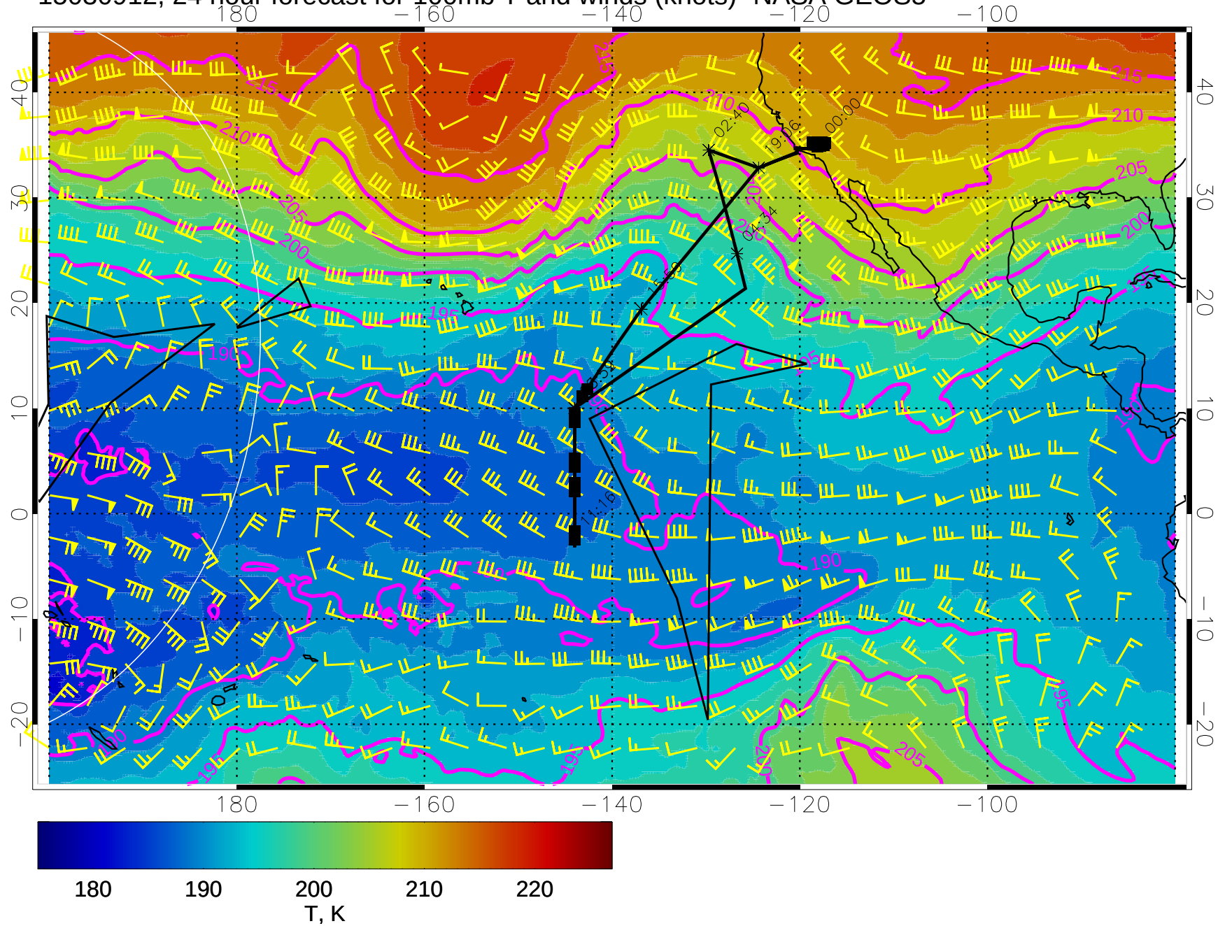
15030912, 24 hour forecast for 100mb T and winds (knots)- NASA GEOS5
