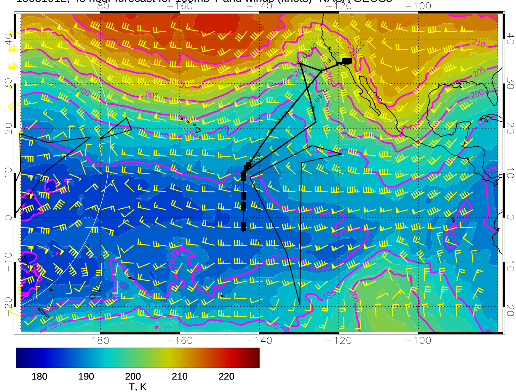
15031012, 48 hour forecast for 100mb T and winds (knots)- NASA GEOS5
