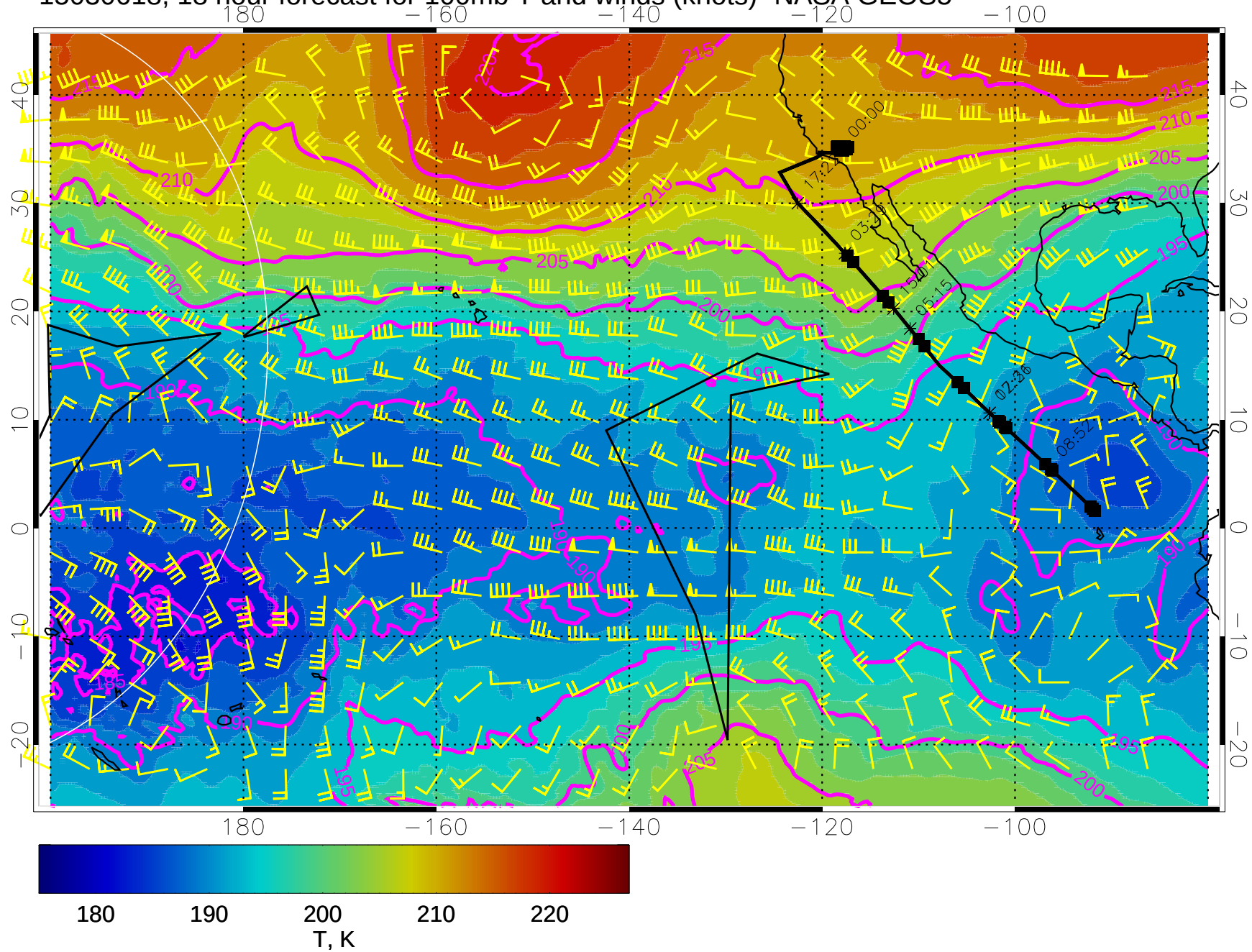
15030618, 18 hour forecast for 100mb T and winds (knots)- NASA GEOS5
