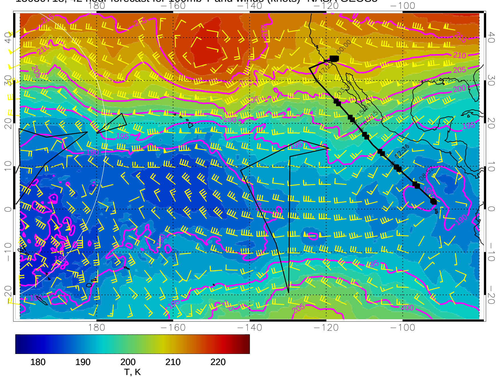
15030718, 42 hour forecast for 100mb T and winds (knots)- NASA GEOS5
