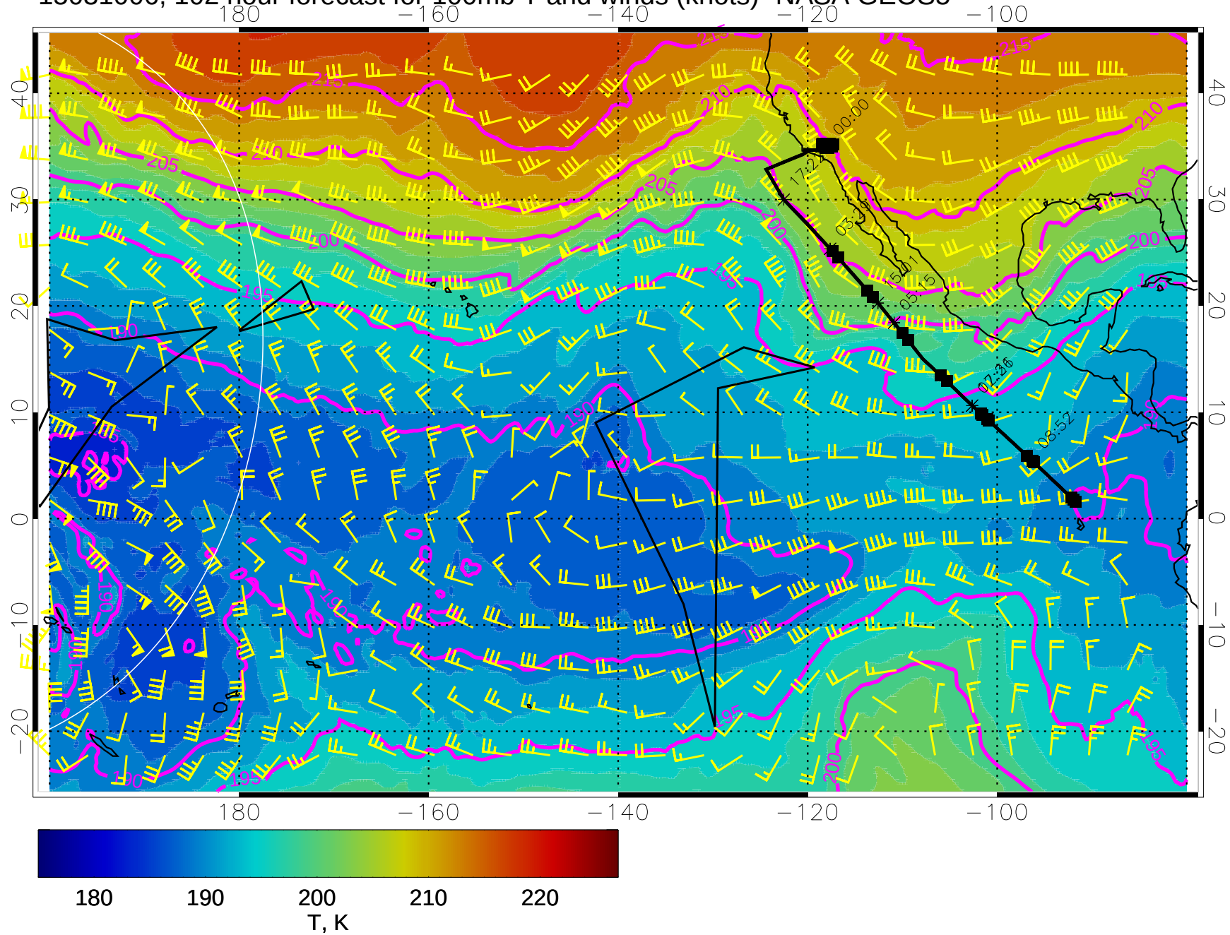
15031006, 102 hour forecast for 100mb T and winds (knots)- NASA GEOS5
