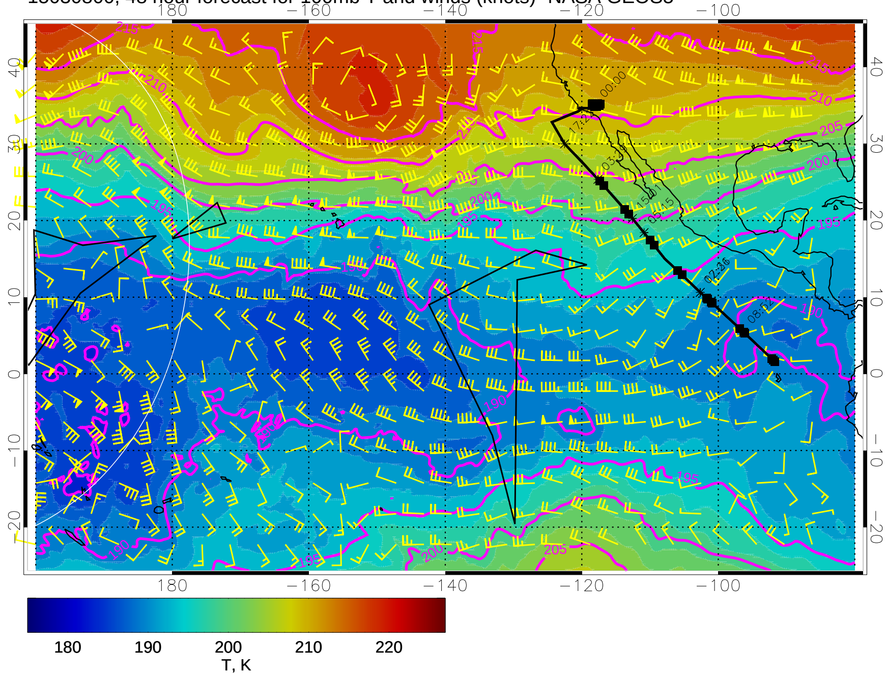
15030800, 48 hour forecast for 100mb T and winds (knots)- NASA GEOS5
