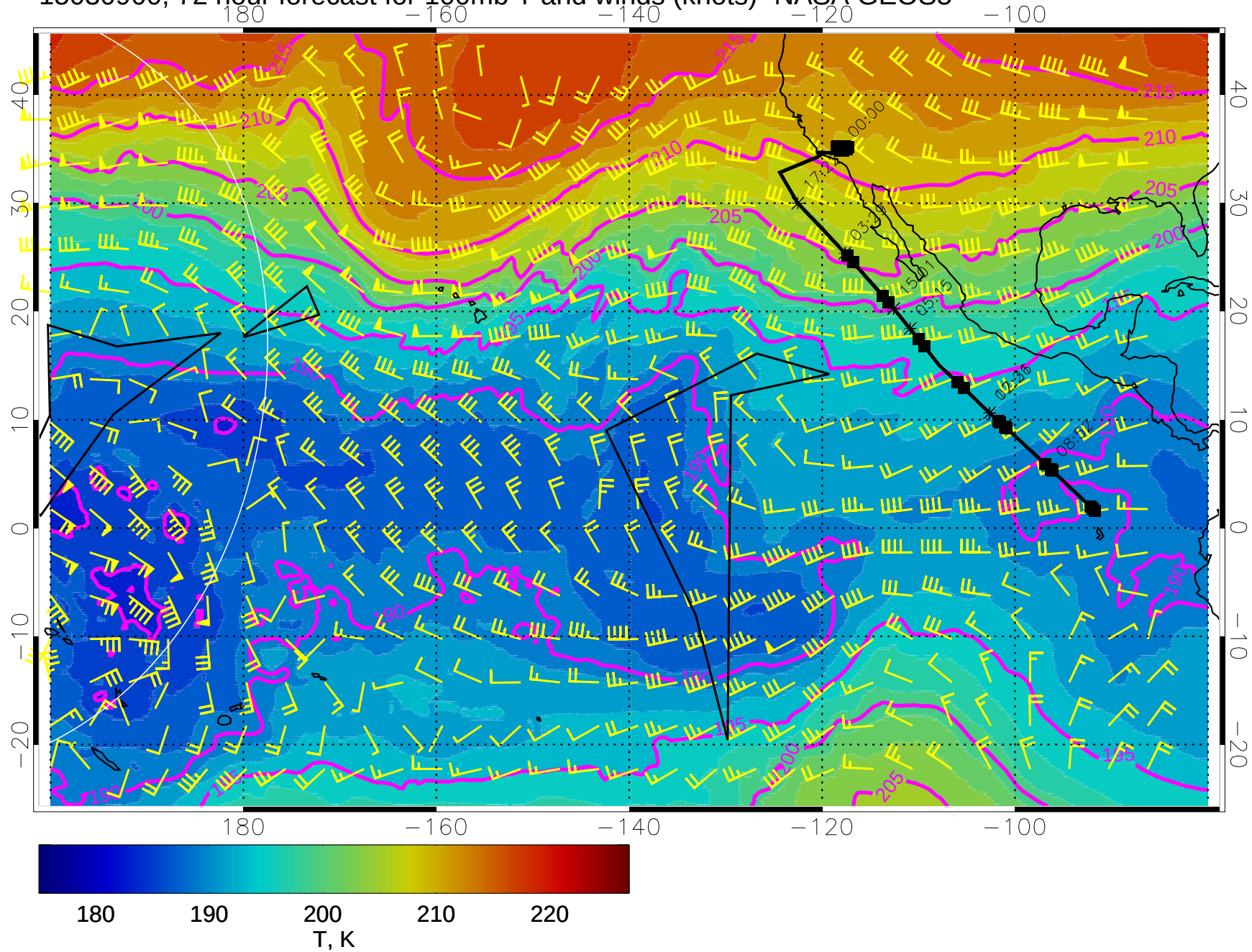
15030900, 72 hour forecast for 100mb T and winds (knots)- NASA GEOS5
