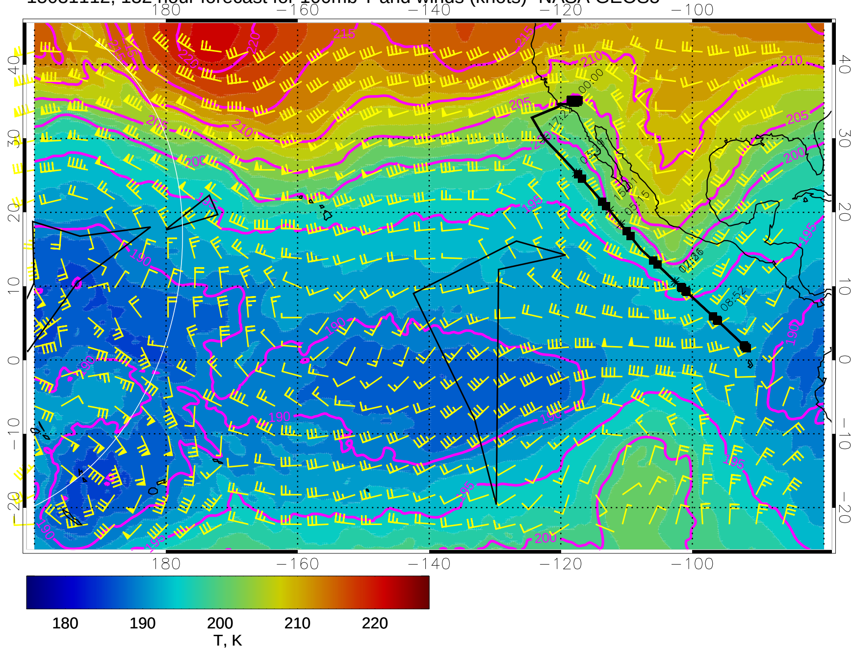
15031112, 132 hour forecast for 100mb T and winds (knots)- NASA GEOS5
