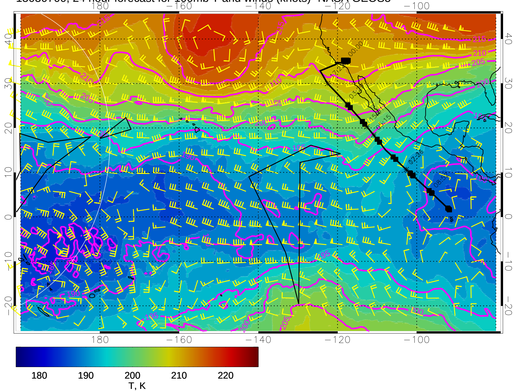
15030700, 24 hour forecast for 100mb T and winds (knots)- NASA GEOS5
