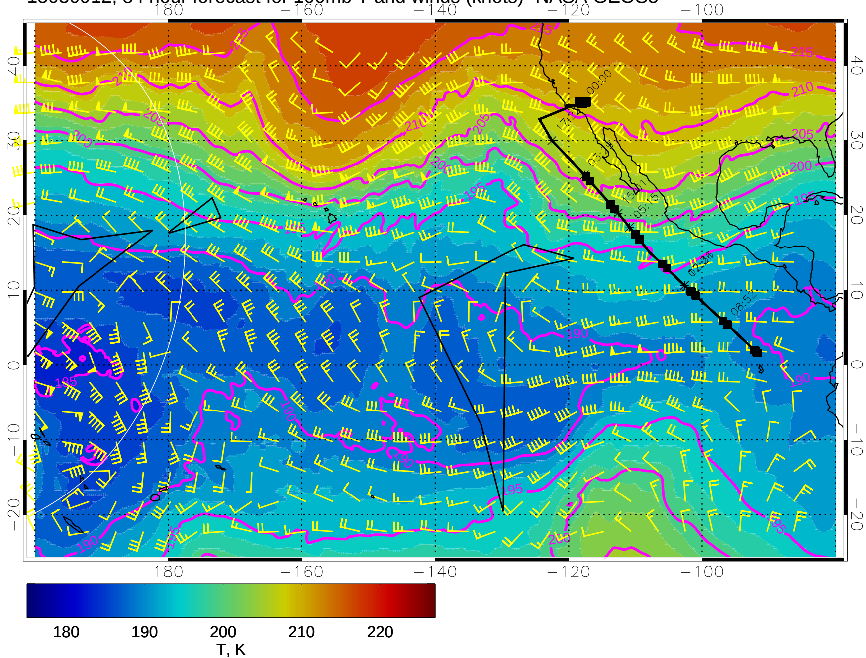
15030912, 84 hour forecast for 100mb T and winds (knots)- NASA GEOS5
