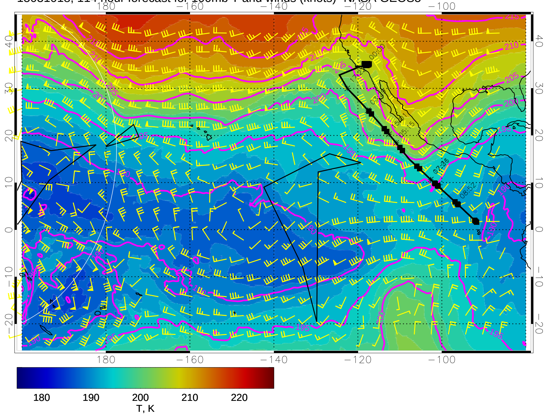
15031018, 114 hour forecast for 100mb T and winds (knots)- NASA GEOS5
