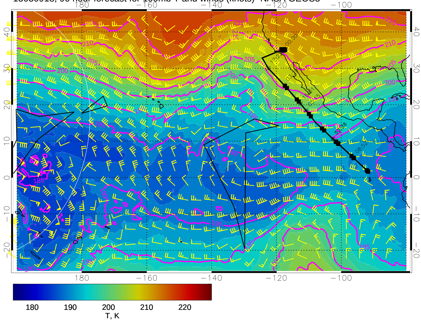
15030918, 90 hour forecast for 100mb T and winds (knots)- NASA GEOS5
