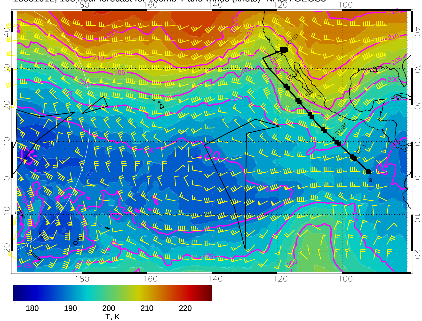
15031012, 108 hour forecast for 100mb T and winds (knots)- NASA GEOS5
