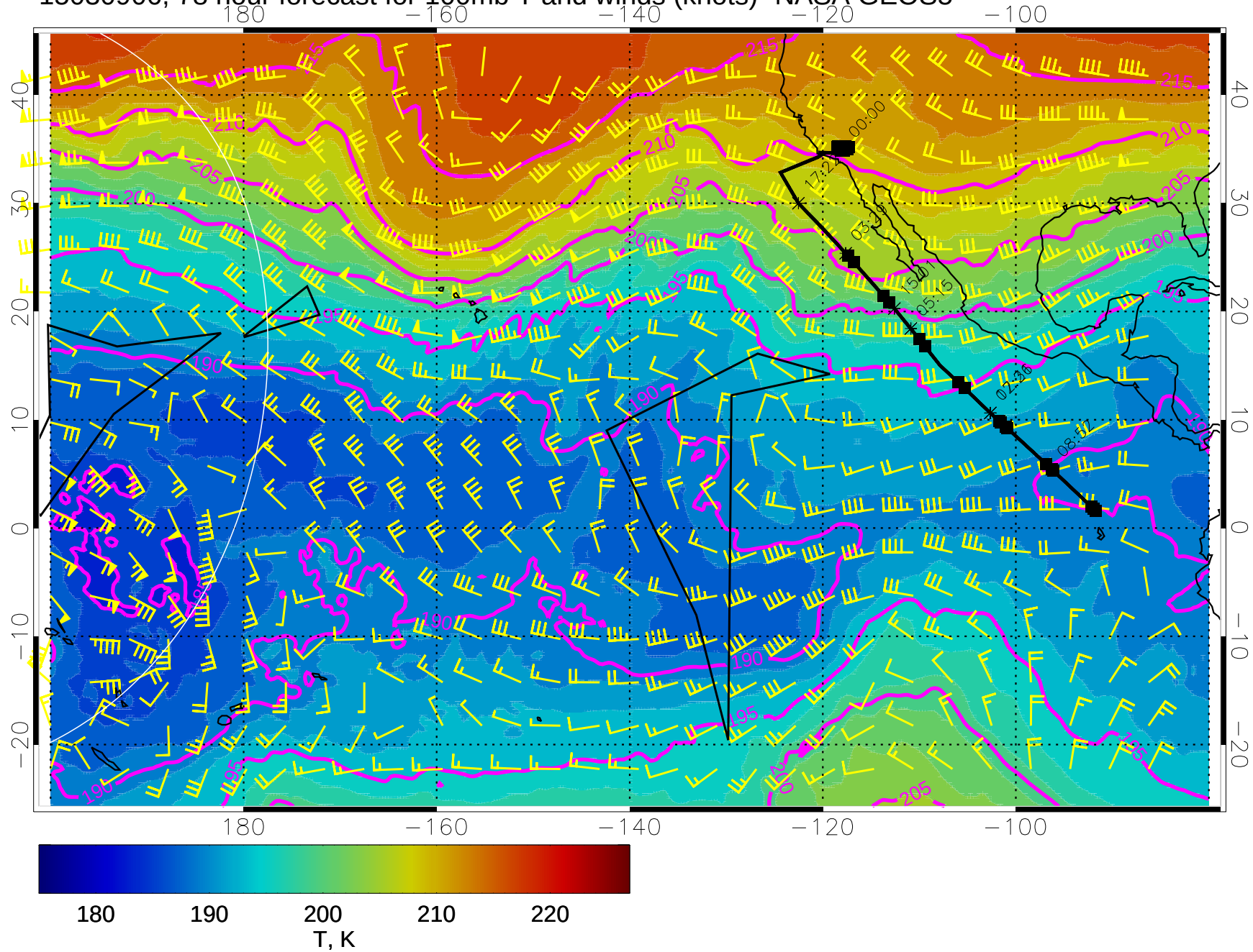
15030906, 78 hour forecast for 100mb T and winds (knots)- NASA GEOS5
