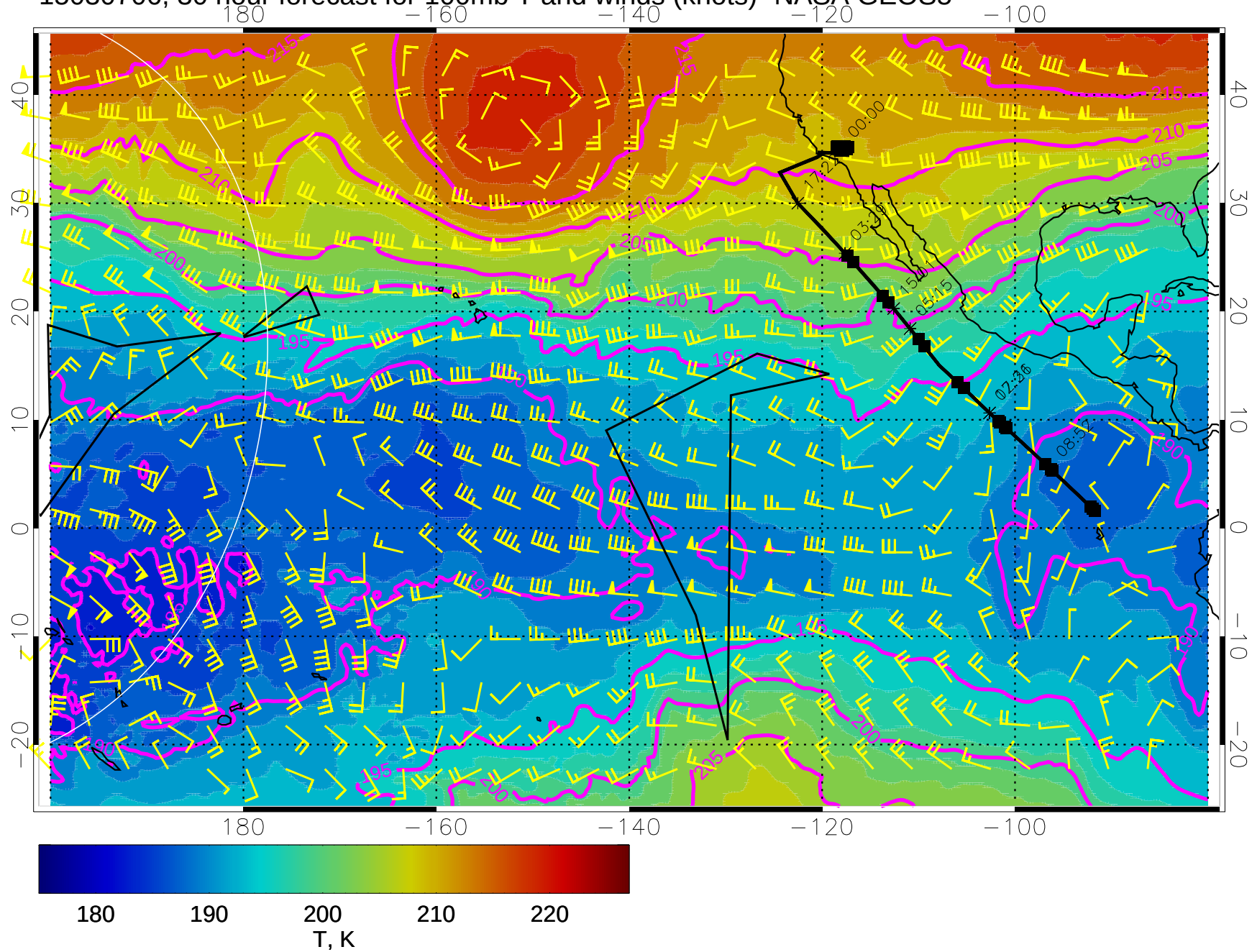
15030706, 30 hour forecast for 100mb T and winds (knots)- NASA GEOS5
