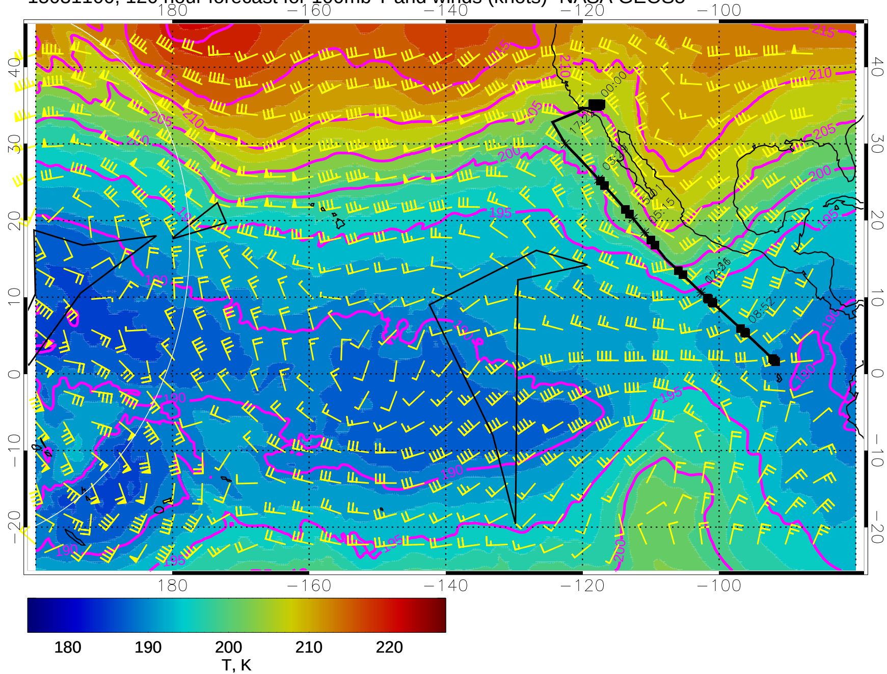
15031100, 120 hour forecast for 100mb T and winds (knots)- NASA GEOS5
