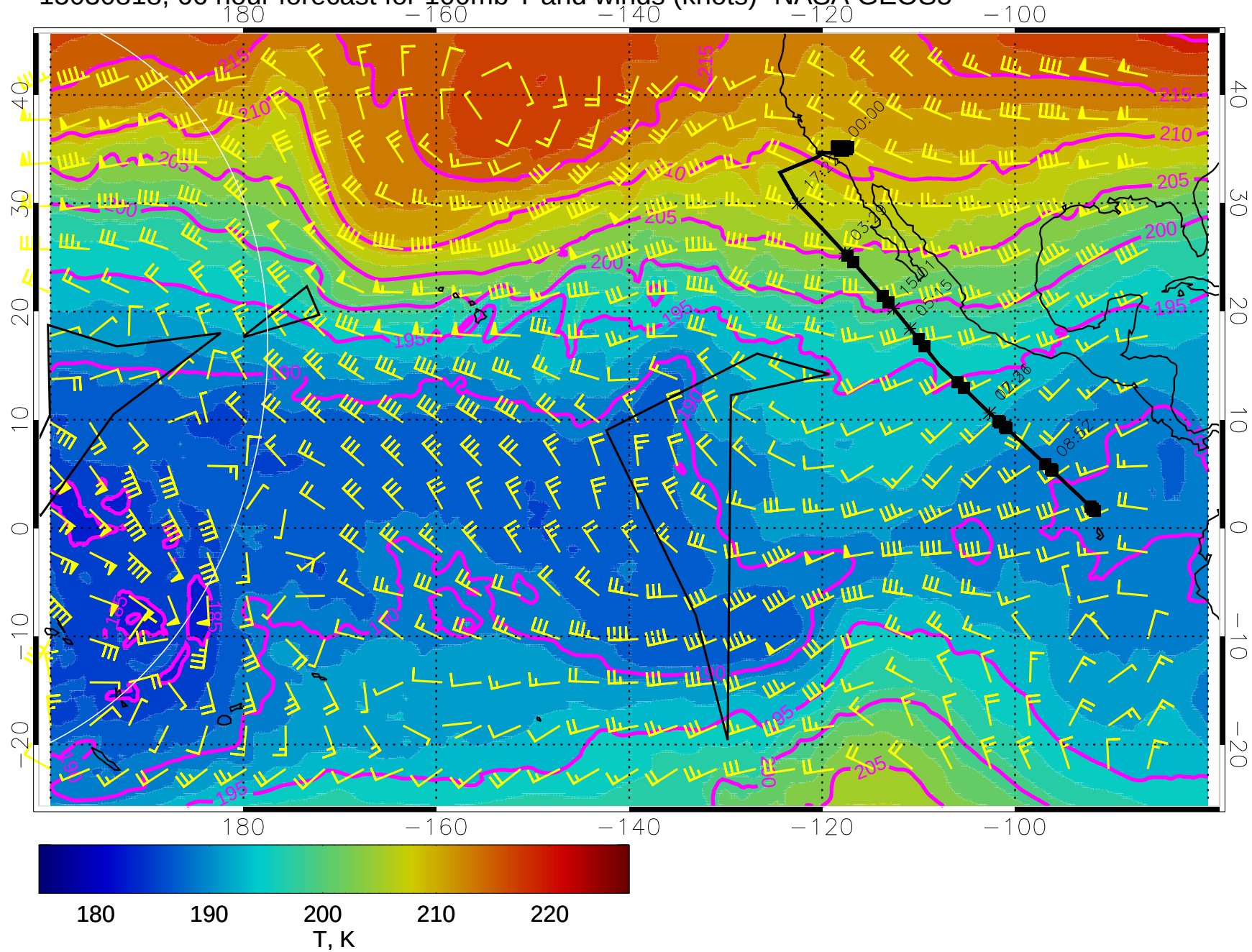
15030818, 66 hour forecast for 100mb T and winds (knots)- NASA GEOS5
