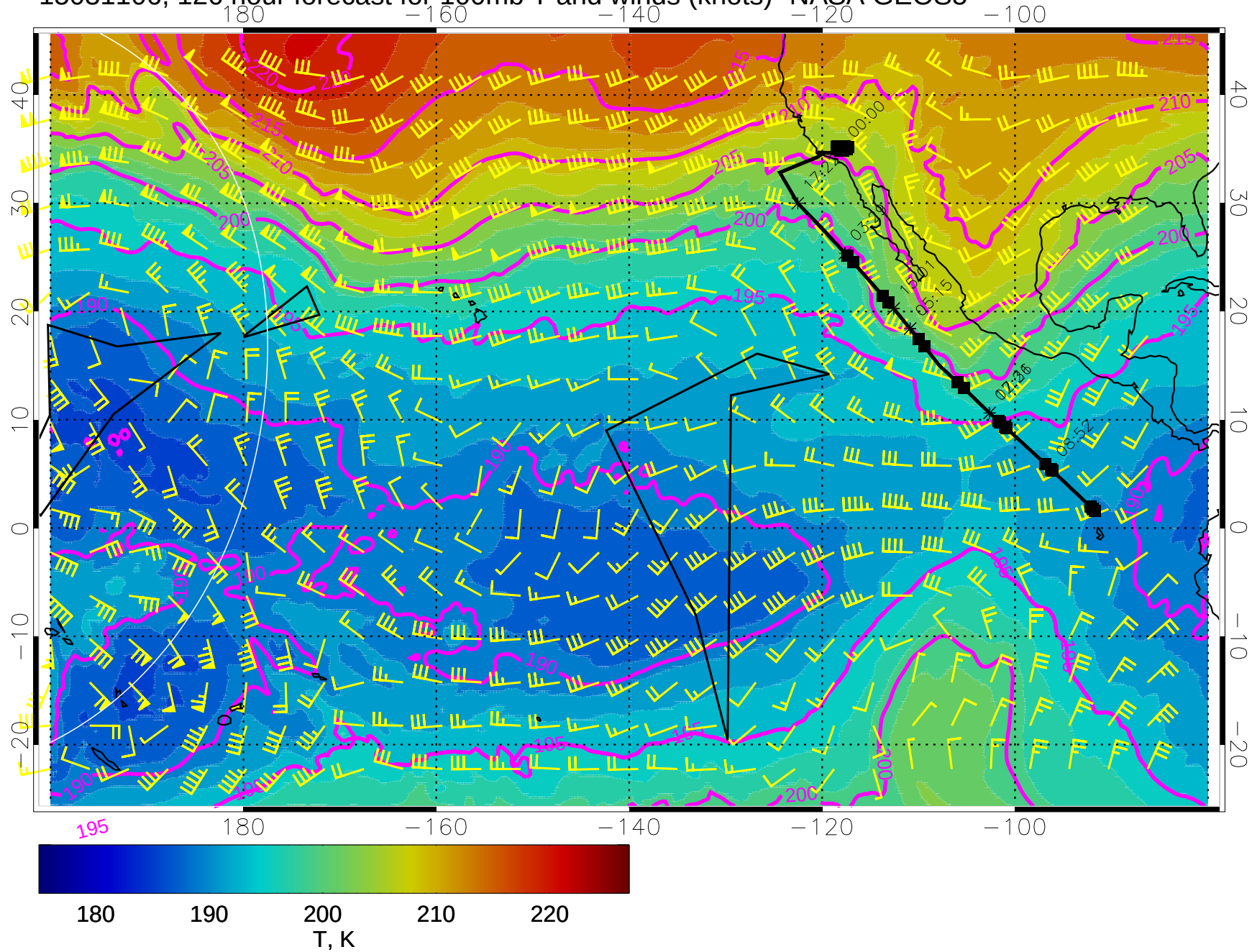
15031106, 126 hour forecast for 100mb T and winds (knots)- NASA GEOS5
