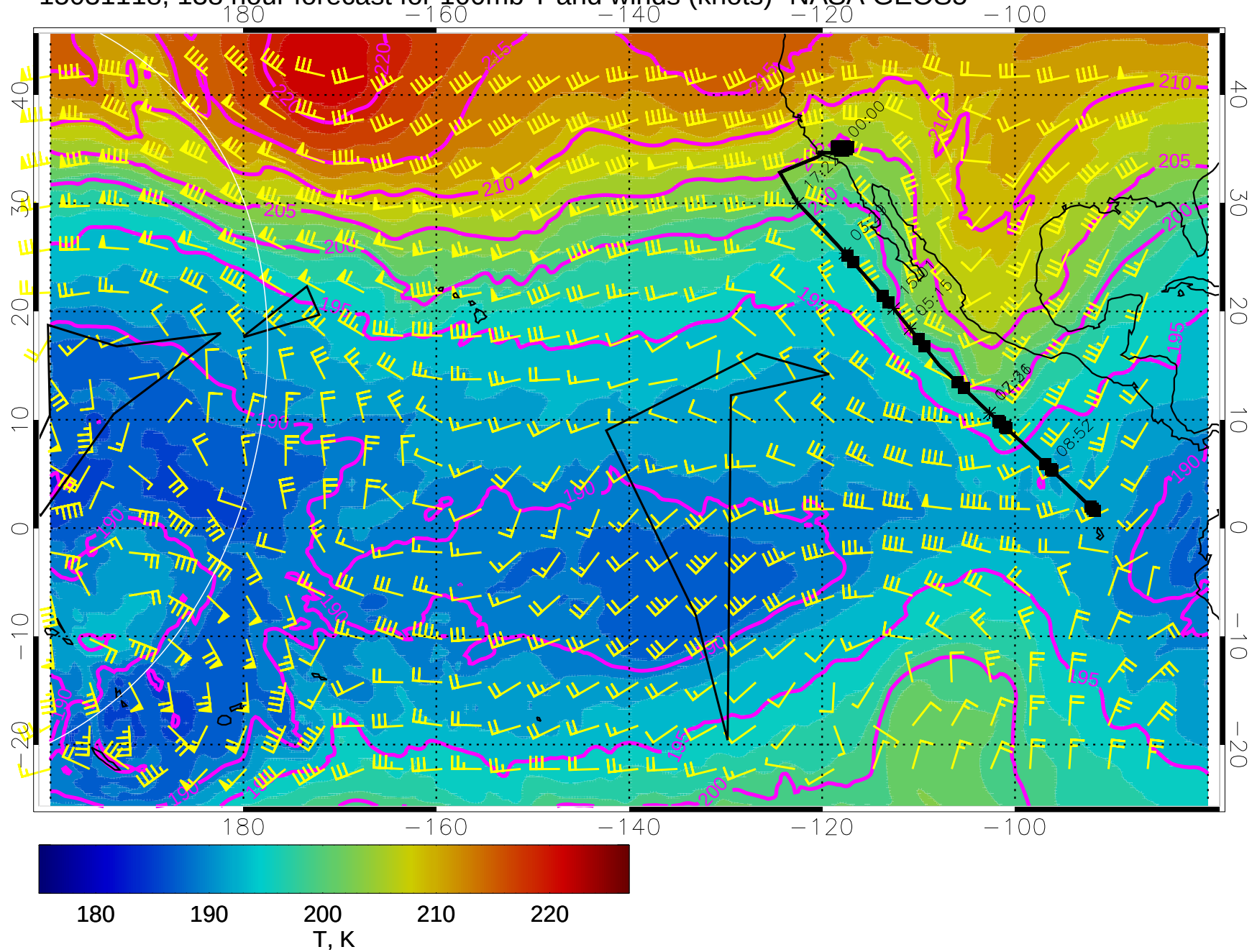
15031118, 138 hour forecast for 100mb T and winds (knots)- NASA GEOS5
