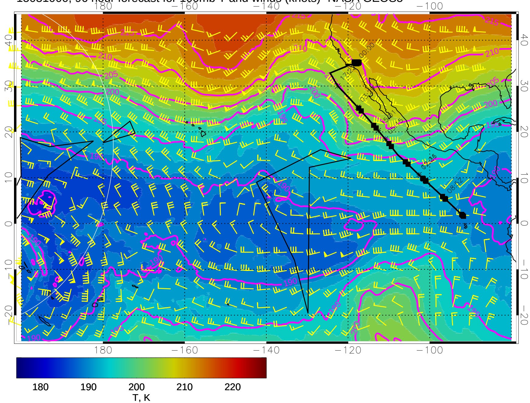
15031000, 96 hour forecast for 100mb T and winds (knots)- NASA GEOS5
