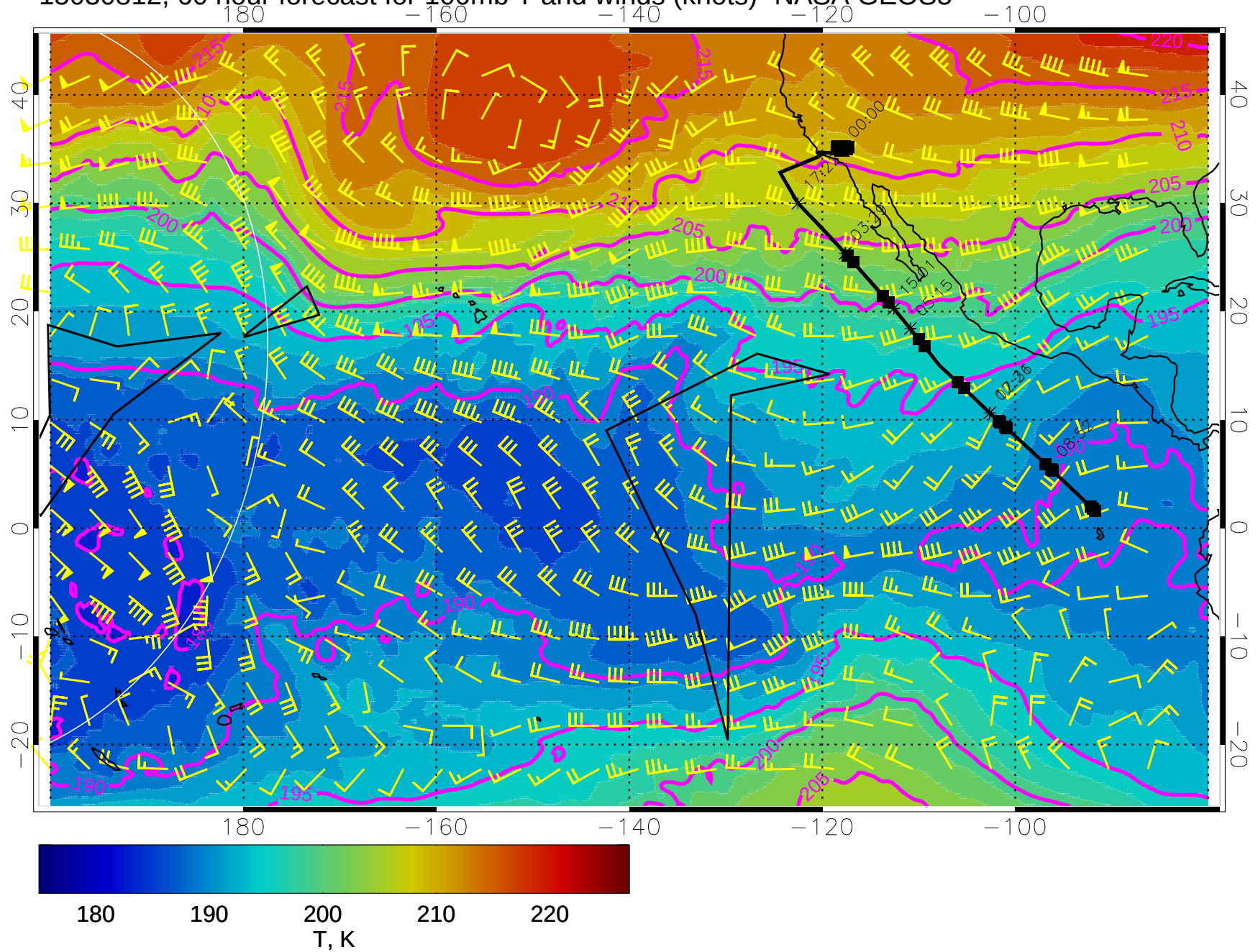
15030812, 60 hour forecast for 100mb T and winds (knots)- NASA GEOS5
