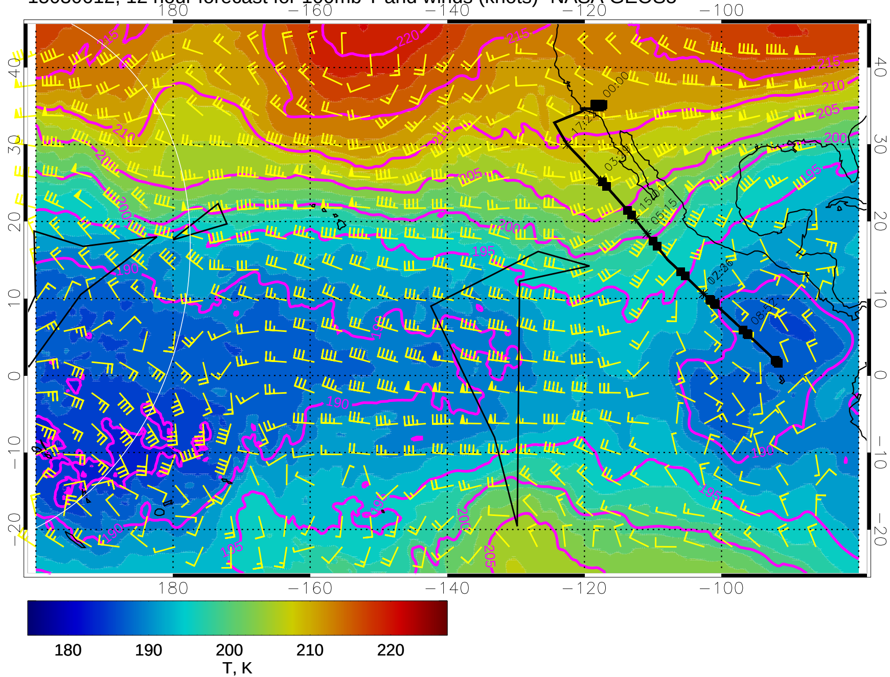
15030612, 12 hour forecast for 100mb T and winds (knots)- NASA GEOS5
