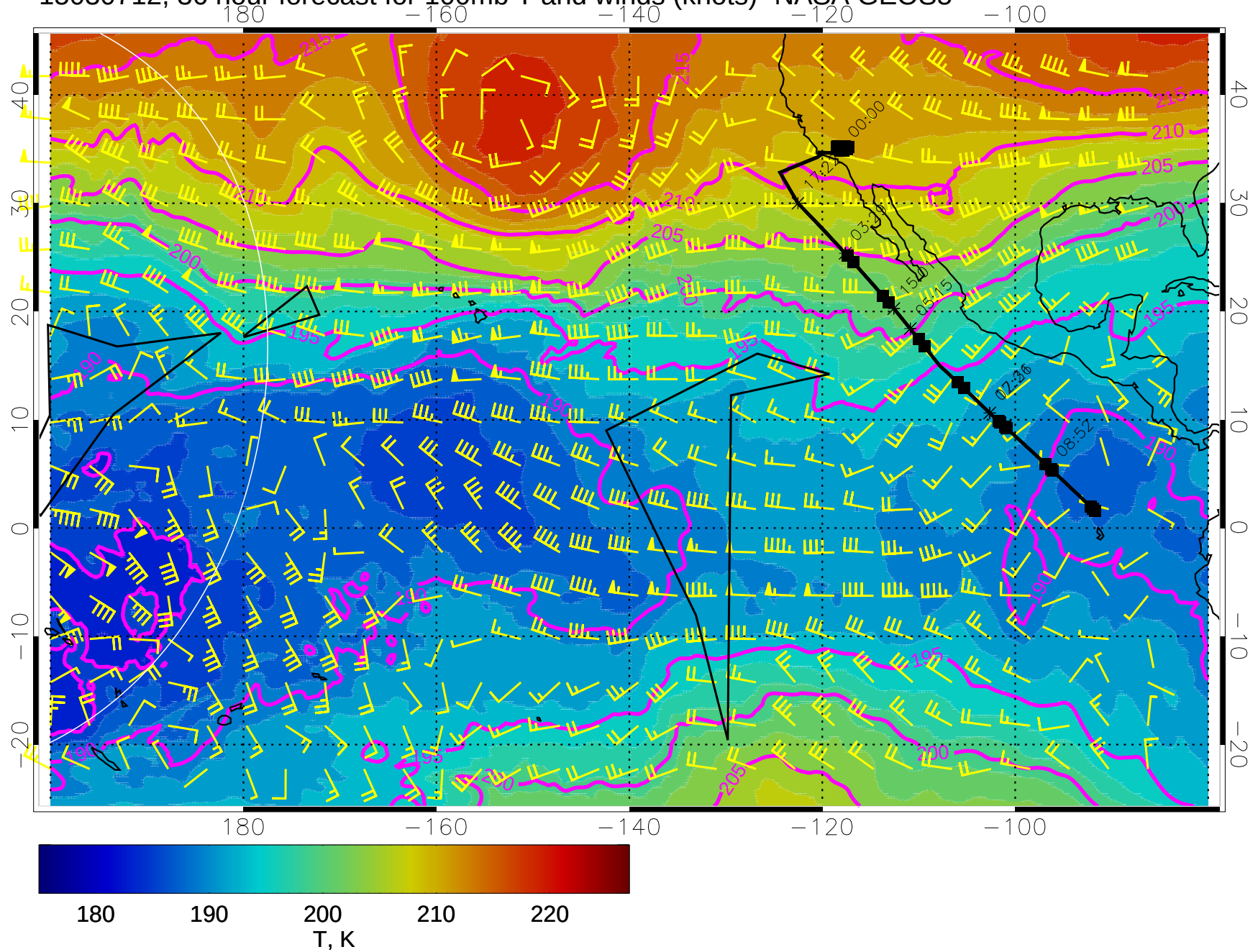
15030712, 36 hour forecast for 100mb T and winds (knots)- NASA GEOS5
