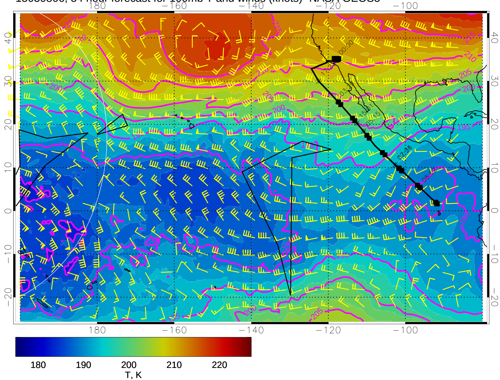
15030806, 54 hour forecast for 100mb T and winds (knots)- NASA GEOS5
