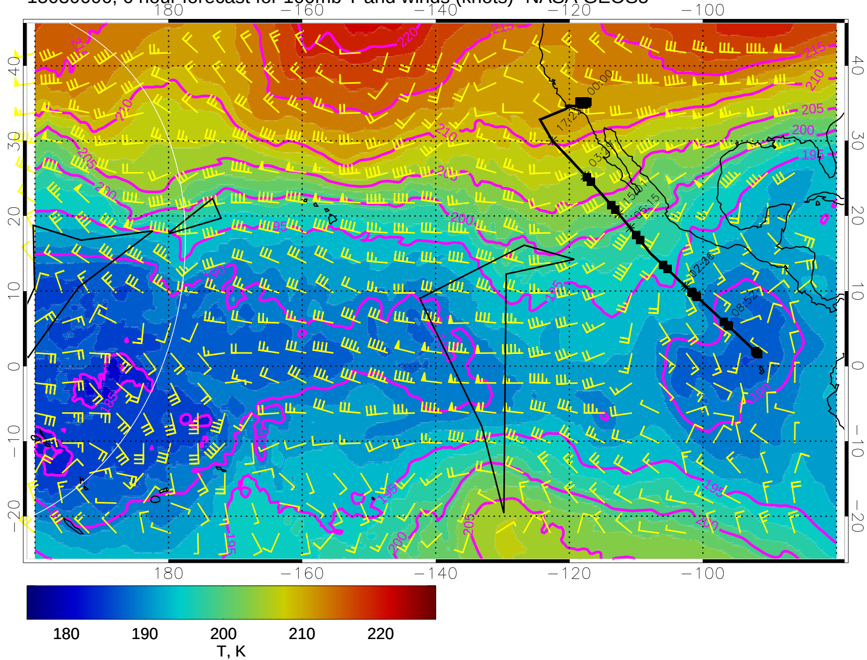
15030606, 6 hour forecast for 100mb T and winds (knots)- NASA GEOS5
